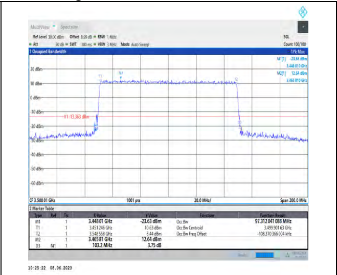
1-N78-3450-3550-PC3-30-100-M-8-CP-64QAM-Outer_Full-273@0-Ant1-97.312-103.200-≤100-PASS
