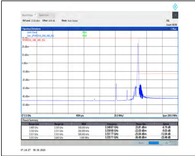
1-N78-3450-3550-PC3-30-30-H-2-DFT-PI2BPSK-Edge_1RB_Right-1@77-Ant1-1--PASS-see graph
