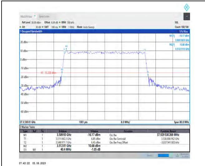
1-N78-3450-3550-PC3-30-40-H-9-CP-256QAM-Outer_Full-106@0-Ant1-37.93-40.400-<math>\leq 40</math>-PASS
