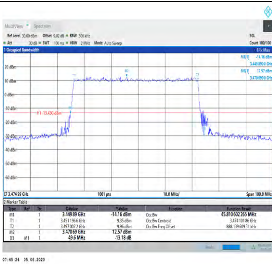
1-N78-3450-3550-PC3-30-50-L-4-DFT-64QAM-Outer_Full-128@0-Ant1-45.811-49.600-≤50-PASS
