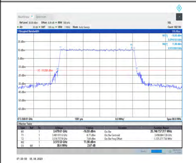
1-N78-3450-3550-PC3-30-40-M-5-DFT-256QAM-Outer_Full-100@0-Ant1-35.746-38.400-≤40-PASS
