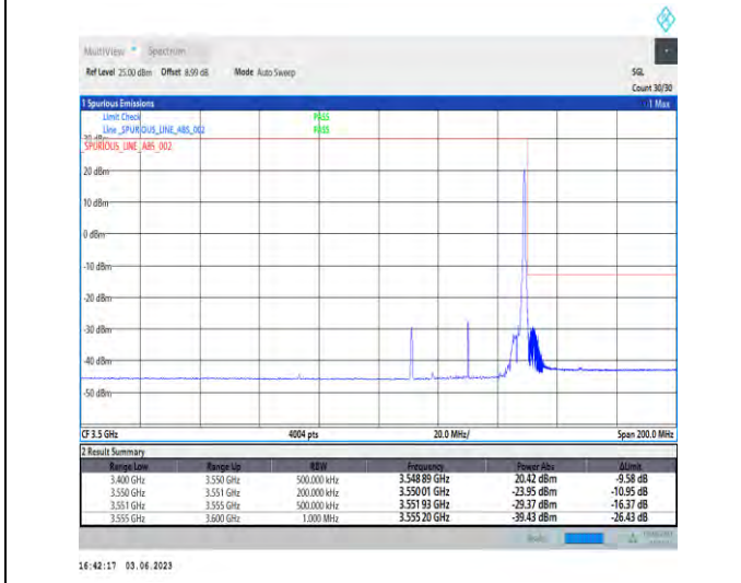
1-N78-3450-3550-PC3-30-40-H-5-CP-QPSK-Edge_1RB_Right-1@105-Ant1-1--PASS-see graph
