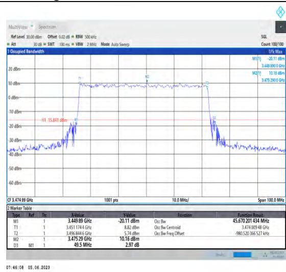
1-N78-3450-3550-PC3-30-50-L-5-DFT-256QAM-Outer_Full-128@0-Ant1-45.67-49.500-≤50-PASS
