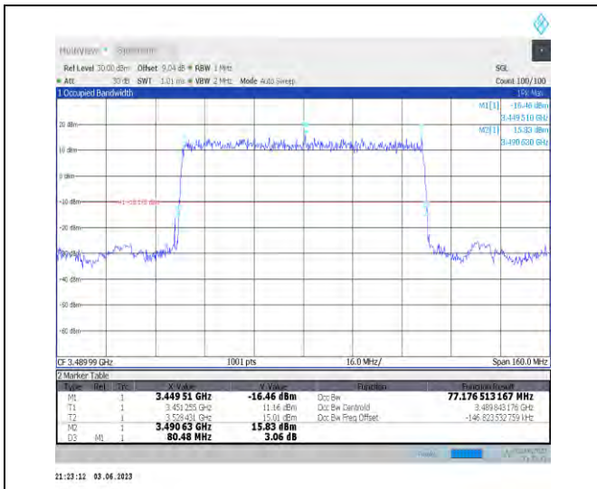
1-N78-3450-3550-PC3-30-80-L-2-DFT-PI2BPSK-Out_er_Full-216@0-Ant1-77.177-80.480-<80-PASS
