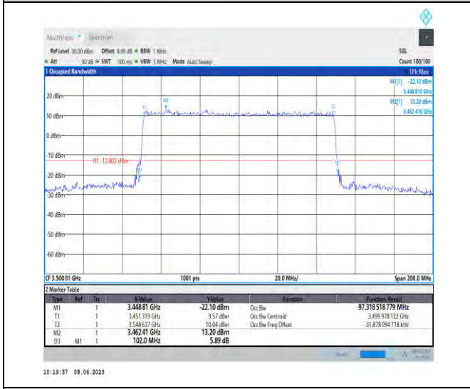
1-N78-3450-3550-PC3-30-100-L-6-CP-QPSK-Outer Full-273@0-Ant1-97.319-102.000-≤100-PASS
