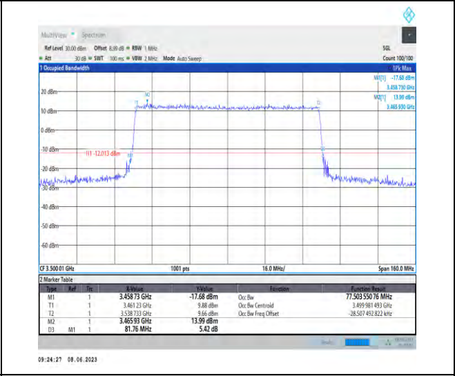
1-N78-3450-3550-PC3-30-80-M-8-CP-64QAM-Outer _Full-217@0-Ant1-77.504-81.760-≤80-PASS
