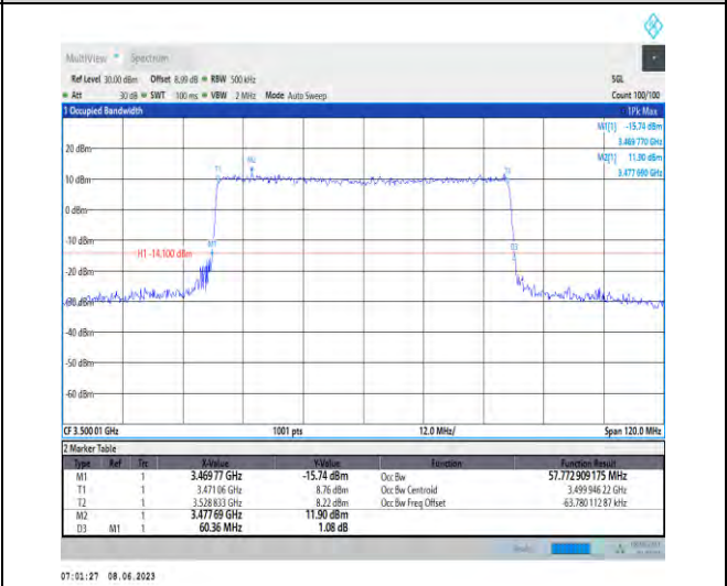
1-N78-3450-3550-PC3-30-60-M-7-CP-16QAM-Outer_Full-162@0-Ant1-57.773-60.360-≤60-PASS
