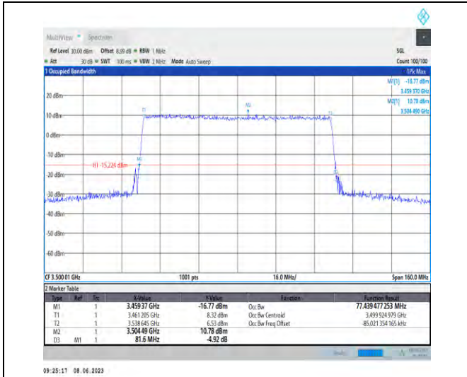
1-N78-3450-3550-PC3-30-80-M-9-CP-256QAM-Outer_Full-217@0-Ant1-77.439-81.600-≤80-PASS
