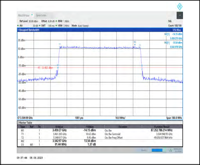
1-N78-3450-3550-PC3-30-90-H-8-CP-64QAM-Outer_Full-245@0-Ant1-87.353-91.440-≤90-PASS
