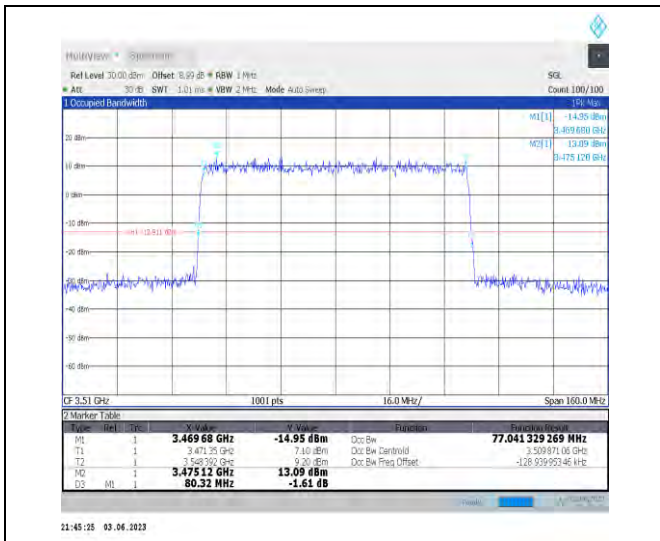
1-N78-3450-3550-PC3-30-80-H-4-DFT-64QAM-Outer_Full-216@0-Ant1-77.041-80.320-≤80-PASS
