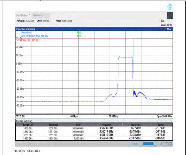
1-N78-3450-3550-PC3-30-20-H-3-DFT-PI2BPSK-Outer_Full-50@0-Ant1-1--PASS-see graph
