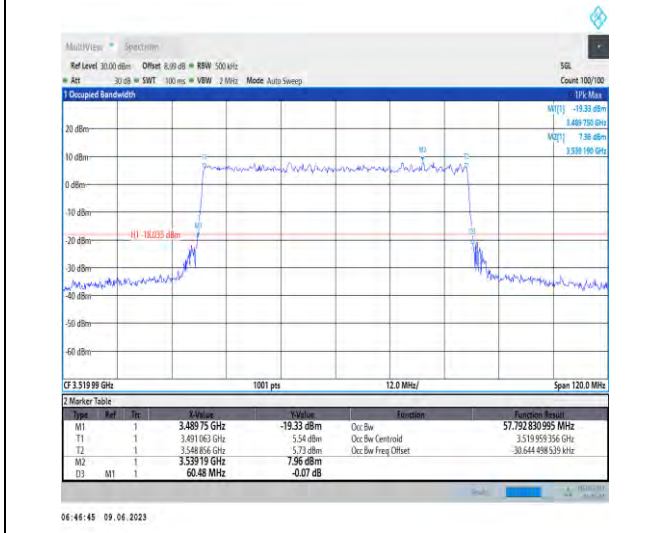
1-N78-3450-3550-PC3-30-60-H-9-CP-256QAM-Outer_Full-162@0-Ant1-57.793-60.480-≤60-PASS
