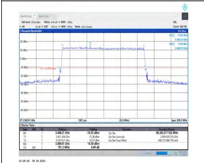
1-N78-3450-3550-PC3-30-100-H-4-DFT-64QAM-Out_Full-270@0-Ant1-96.363-101.200-≤100-PASS
