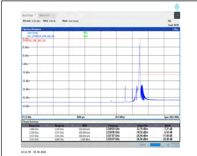
1-N78-3450-3550-PC3-30-20-H-2-DFT-PI2BPSK-Edge_1RB_Right-1@50-Ant1-1--PASS-see graph
