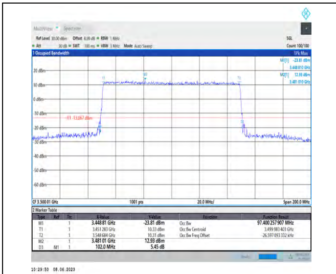
1-N78-3450-3550-PC3-30-100-H-6-CP-QPSK-Outer_Full-273@0-Ant1-97.4-102.000-≤100-PASS
