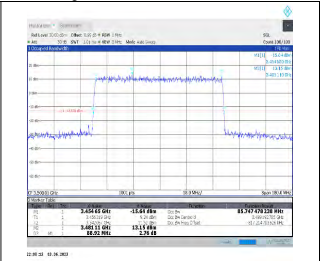
1-N78-3450-3550-PC3-30-90-M-3-DFT-16QAM-Out_er_Full-240@0-Ant1-85.747-88.920-≤90-PASS
