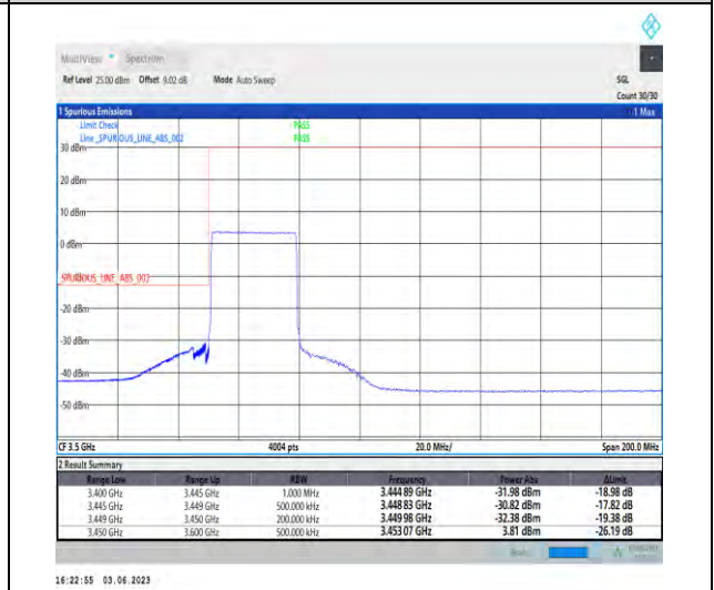
1-N78-3450-3550-PC3-30-30-L-6-CP-QPSK-Outer_Full-78@0-Ant1-1--PASS-see graph
