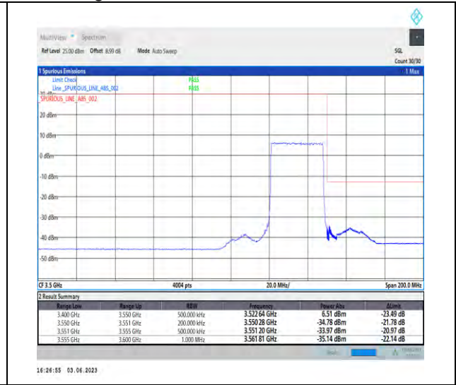
1-N78-3450-3550-PC3-30-30-H-3-DFT-PI2BPSK-Outer_Full-75@0-Ant1-1--PASS-see graph
