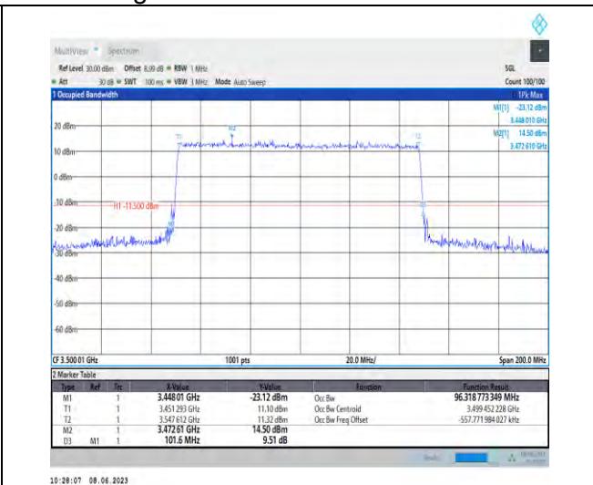
1-N78-3450-3550-PC3-30-100-H-3-DFT-16QAM-Out_Full-270@0-Ant1-96.319-101.600-≤100-PASS
