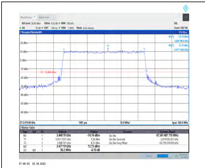
1-N78-3450-3550-PC3-30-50-L-8-CP-64QAM-Outer_Full-133@0-Ant1-47.541-50.200-≤50-PASS
