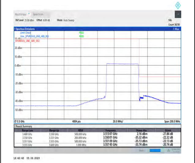
1-N78-3450-3550-PC3-30-40-H-6-CP-QPSK-Outer_Full-106@0-Ant1-1--PASS-see graph
