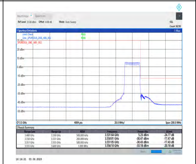
1-N78-3450-3550-PC3-30-20-H-6-CP-QPSK-Outer_Full-51@0-Ant1-1--PASS-see graph
