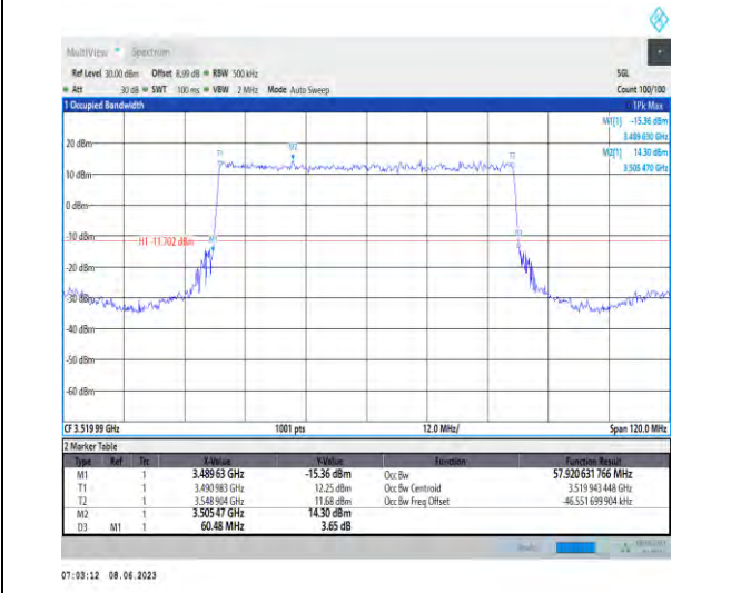
1-N78-3450-3550-PC3-30-60-H-2-DFT-PI2BPSK-Outer_Full-162@0-Ant1-57.921-60.480-≤60-PASS
