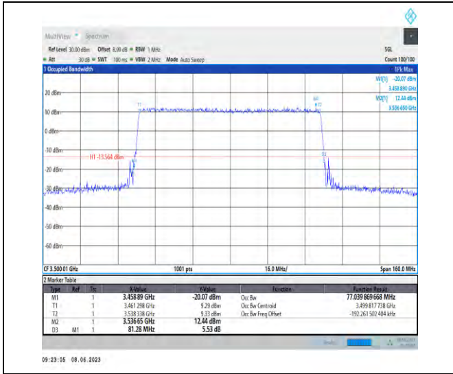
1-N78-3450-3550-PC3-30-80-M-5-DFT-256QAM-Out _Full-216@0-Ant1-77.04-81.280-≤80-PASS
