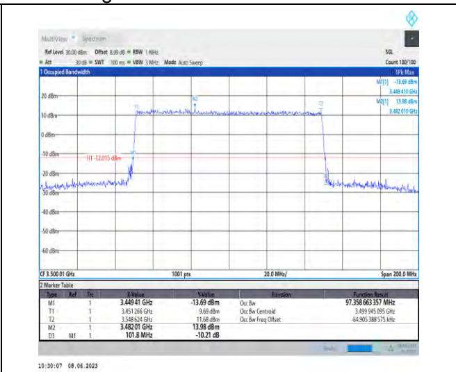
1-N78-3450-3550-PC3-30-100-H-7-CP-16QAM-Outer_Full-273@0-Ant1-97.359-101.800-≤100-PASS
