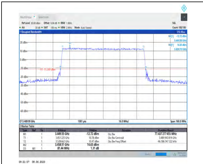
1-N78-3450-3550-PC3-30-80-L-6-CP-QPSK-Outer_Full-217@0-Ant1-77.437-81.440-≤80-PASS
