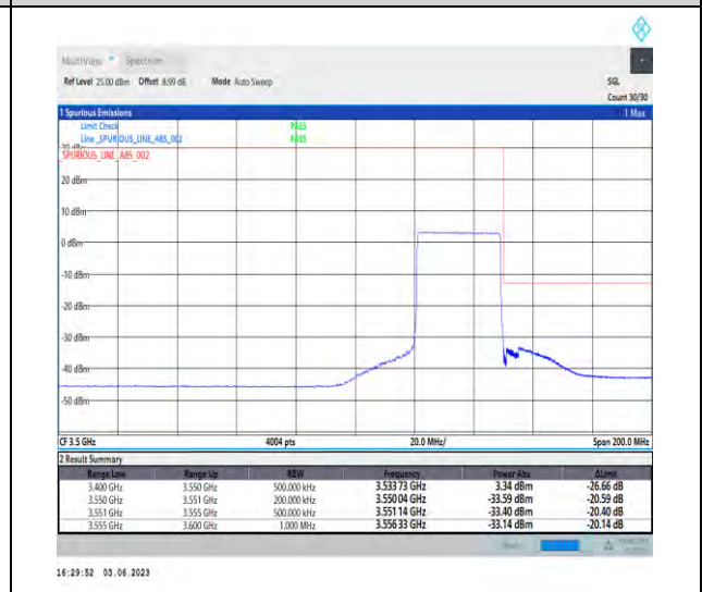
1-N78-3450-3550-PC3-30-30-H-6-CP-QPSK-Outer_Full-78@0-Ant1-1--PASS-see graph
