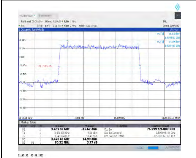
1-N78-3450-3550-PC3-30-80-H-2-DFT-PI2BPSK-Outer_Full-216@0-Ant1-76.999-80.320-≤80-PASS
