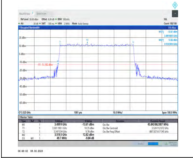
1-N78-3450-3550-PC3-30-50-H-4-DFT-64QAM-Outer_Full-128@0-Ant1-45.844-49.700-≤50-PASS
