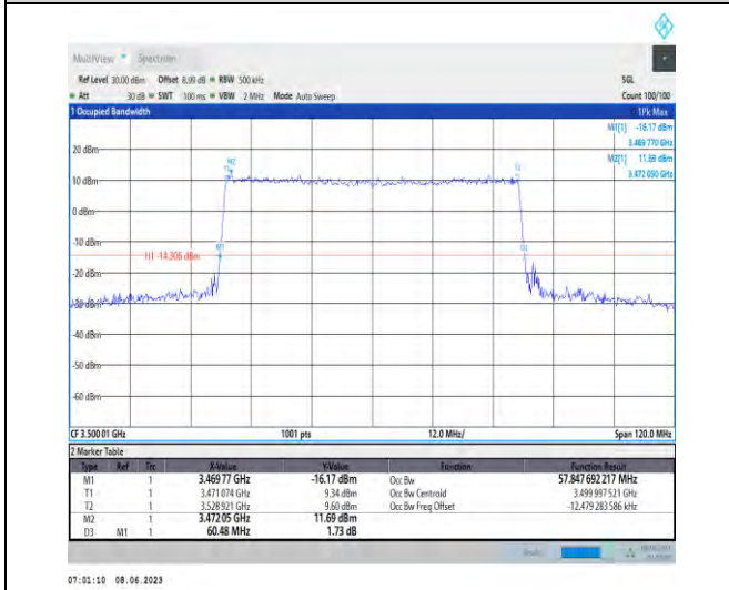
1-N78-3450-3550-PC3-30-60-M-6-CP-QPSK-Outer_Full-162@0-Ant1-57.848-60.480-≤60-PASS
