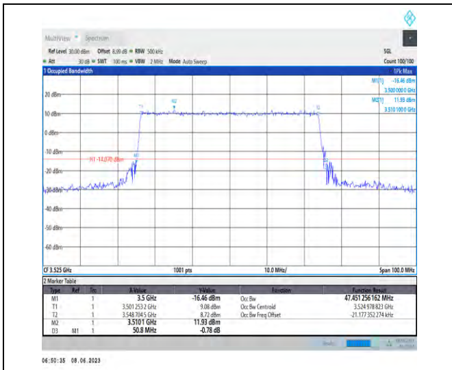
1-N78-3450-3550-PC3-30-50-H-6-CP-QPSK-Outer_Full-133@0-Ant1-47.451-50.800-≤50-PASS
