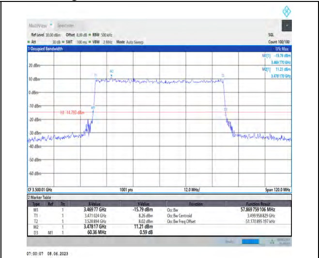
1-N78-3450-3550-PC3-30-60-M-5-DFT-256QAM-Outer_Full-162@0-Ant1-57.87-60.360-≤60-PASS
