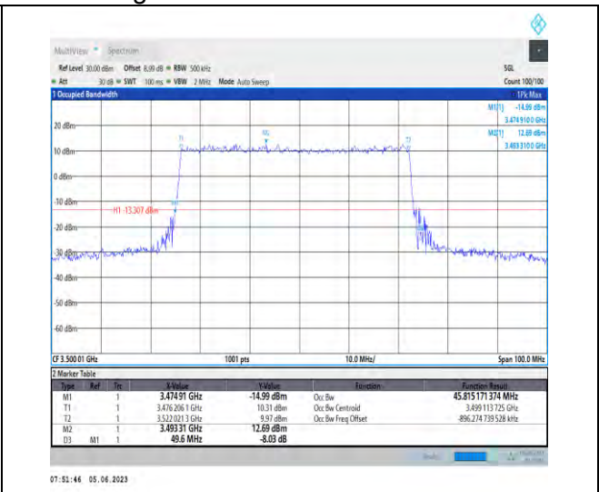
1-N78-3450-3550-PC3-30-50-M-4-DFT-64QAM-Outer_Full-128@0-Ant1-45.815-49.600-≤50-PASS
