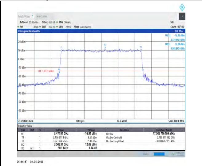
1-N78-3450-3550-PC3-30-50-M-8-CP-64QAM-Outer_Full-133@0-Ant1-47.507-50.100-≤50-PASS
