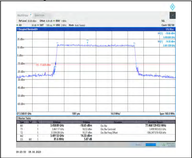
1-N78-3450-3550-PC3-30-80-M-6-CP-QPSK-Outer_ Full-217@0-Ant1-77.468-81.600-≤80-PASS
