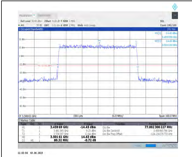
1-N78-3450-3550-PC3-30-80-M-1-DFT-QPSK-Outer_Full-216@0-Ant1-77.002-80.320-≤80-PASS
