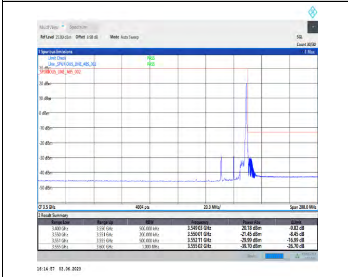
1-N78-3450-3550-PC3-30-20-H-5-CP-QPSK-Edge_1RB_Right-1@50-Ant1-1--PASS-see graph
