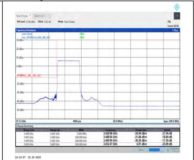
1-N78-3450-3550-PC3-30-30-L-3-DFT-PI2BPSK-Outer_Full-75@0-Ant1-1--PASS-see graph
