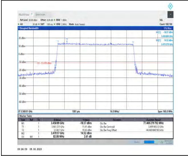
1-N78-3450-3550-PC3-30-80-M-7-CP-16QAM-Outer _Full-217@0-Ant1-77.469-82.080-≤80-PASS
