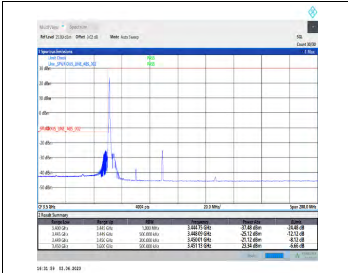
1-N78-3450-3550-PC3-30-40-L-1-DFT-PI2BPSK-Edge_1RB_Left-1@0-Ant1-1--PASS-see graph
