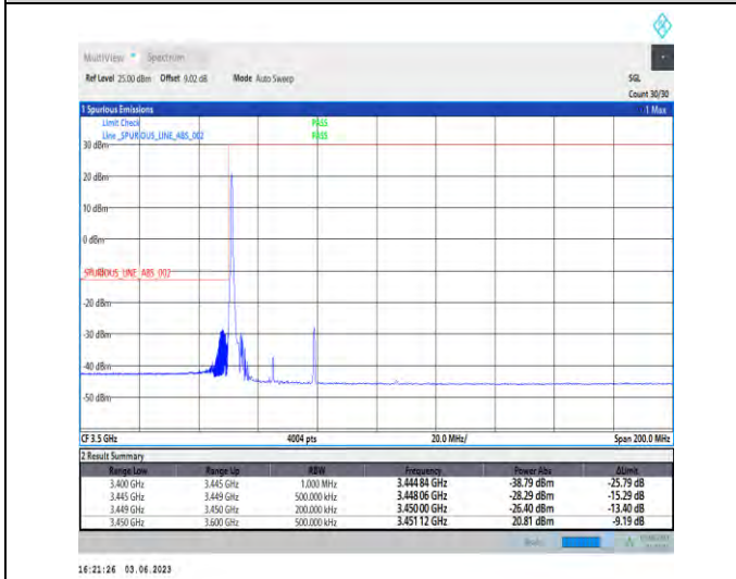
1-N78-3450-3550-PC3-30-30-L-4-CP-QPSK-Edge_1RB_Left-1@0-Ant1-1--PASS-see graph
