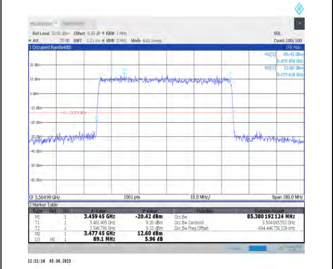
1-N78-3450-3550-PC3-30-90-H-4-DFT-64QAM-Outer_Full-240@0-Ant1-85.38-89.100-≤90-PASS
