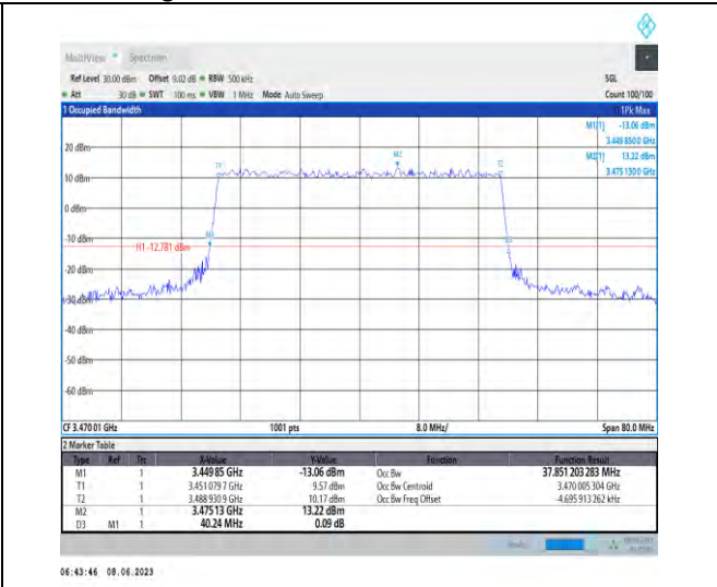
1-N78-3450-3550-PC3-30-40-L-8-CP-64QAM-Outer_Full-106@0-Ant1-37.851-40.240-≤40-PASS
