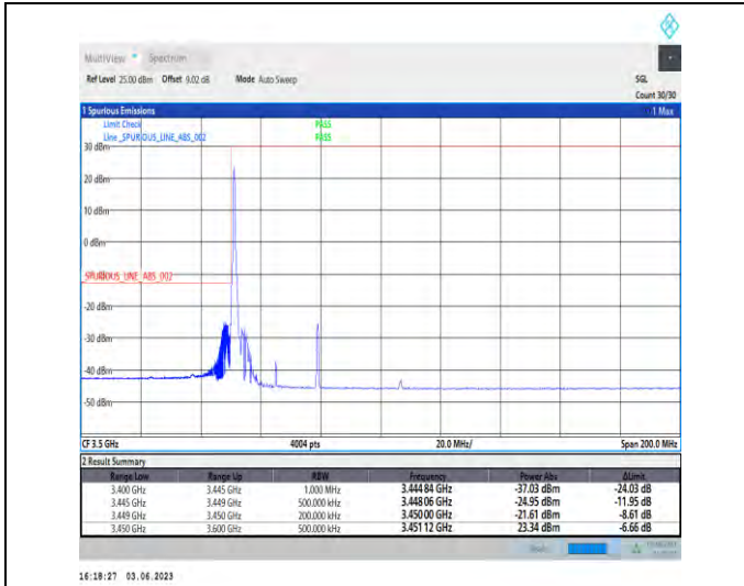
1-N78-3450-3550-PC3-30-30-L-1-DFT-PI2BPSK-Edge_1RB_Left-1@0-Ant1-1--PASS-see graph
