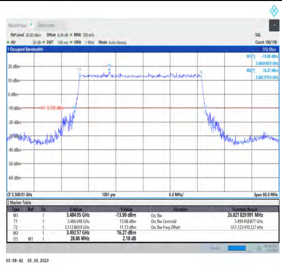
1-N78-3450-3550-PC3-30-30-M-2-DFT-PI2BPSK-Outer_Full-75@0-Ant1-26.822-28.860-≤30-PASS
