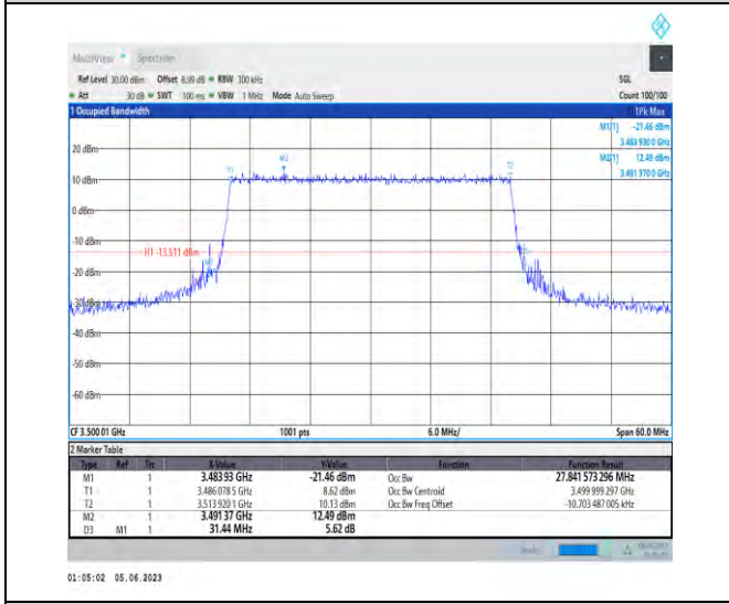
1-N78-3450-3550-PC3-30-30-M-7-CP-16QAM-Outer_Full-78@0-Ant1-27.842-31.440-≤30-PASS
