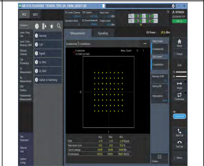
1-N78-3450-3550-PC3-30-100-M-8-CP-64QAM-Outer_Full-273@0-Ant1-see graph-PASS
