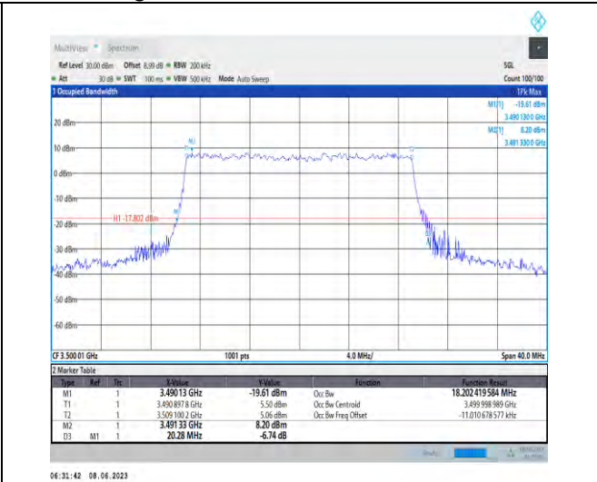
1-N78-3450-3550-PC3-30-20-M-9-CP-256QAM-Outer_Full-51@0-Ant1-18.202-20.280-≤20-PASS
