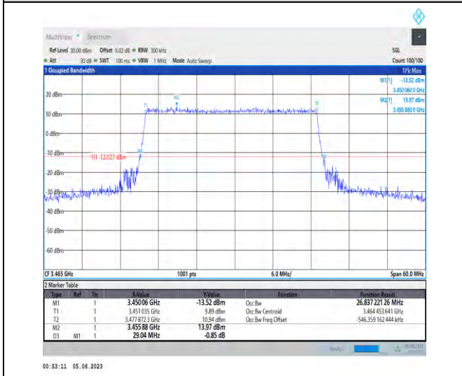
1-N78-3450-3550-PC3-30-30-L-4-DFT-64QAM-Out _Full-75@0-Ant1-26.837-29.040-≤30-PASS
