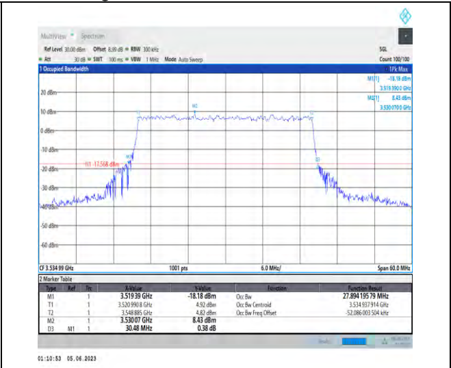
1-N78-3450-3550-PC3-30-30-H-9-CP-256QAM-Outer_Full-78@0-Ant1-27.894-30.480-≤30-PASS
