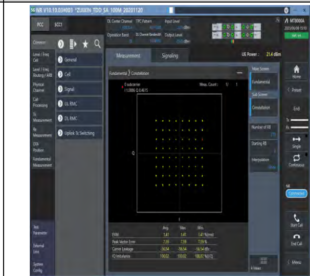
1-N78-3450-3550-PC3-30-100-M-4-DFT-64QAM-Out er_Full-270@0-Ant1-see graph-PASS
