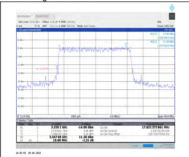
1-N78-3450-3550-PC3-30-20-H-4-DFT-64QAM-Outer_Full-50@0-Ant1-17.832-19.080-≤20-PASS
