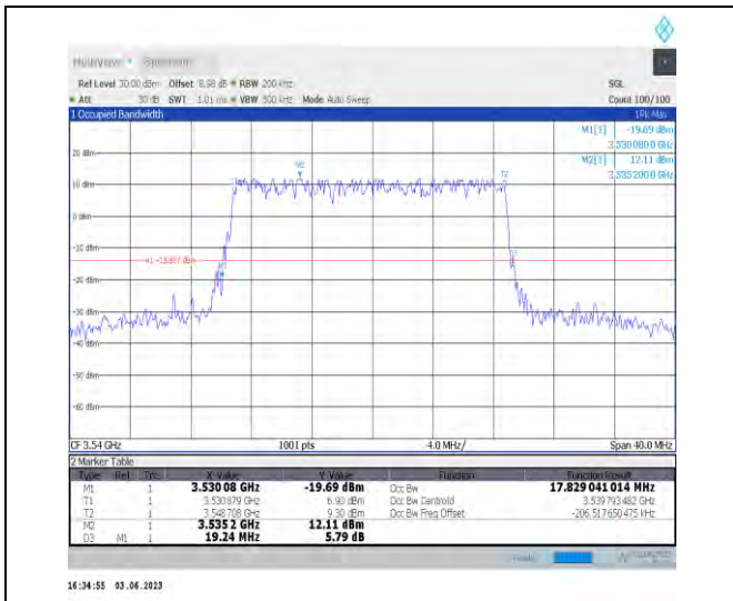
1-N78-3450-3550-PC3-30-20-H-3-DFT-16QAM-Outer_Full-50@0-Ant1-17.829-19.240-≤20-PASS
