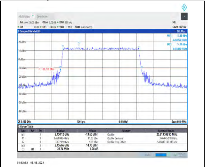
1-N78-3450-3550-PC3-30-30-L-3-DFT-16QAM-Out r_Full-75@0-Ant1-26.814-28.740-≤30-PASS
