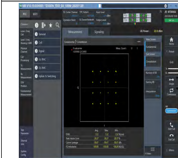
1-N78-3450-3550-PC3-30-100-M-3-DFT-16QAM-Out er_Full-270@0-Ant1-see graph-PASS
