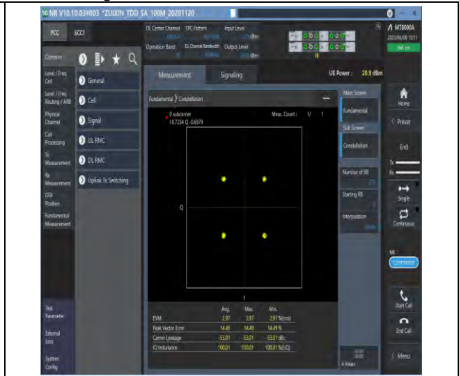
1-N78-3450-3550-PC3-30-100-M-6-CP-QPSK-Outer_Full-273@0-Ant1-see graph-PASS
