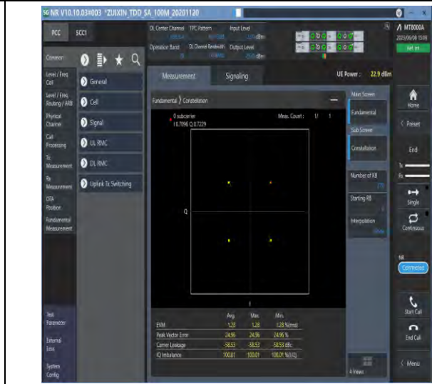
1-N78-3450-3550-PC3-30-100-M-2-DFT-QPSK-Out er_Full-270@0-Ant1-see graph-PASS
