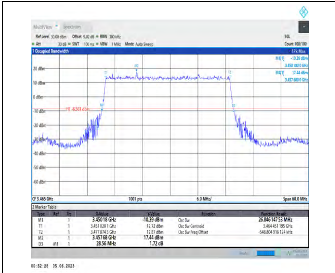
1-N78-3450-3550-PC3-30-30-L-2-DFT-PI2BPSK-Out er_Full-75@0-Ant1-26.846-28.560-≤30-PASS
