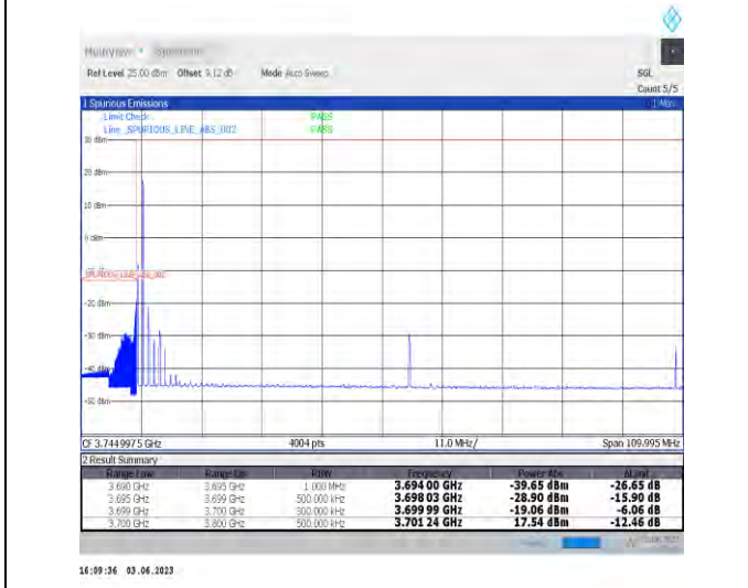
1-N77-3700-3980-PC3-30-100-L-4-CP-QPSK-Edge_1RB_Left-1@0-Ant1-1--PASS-see graph
