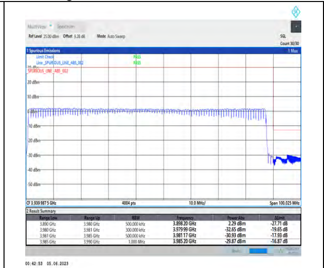
1-N77-3700-3980-PC3-30-90-H-3-DFT-PI2BPSK-Outer_Full-240@0-Ant1-1--PASS-see graph
