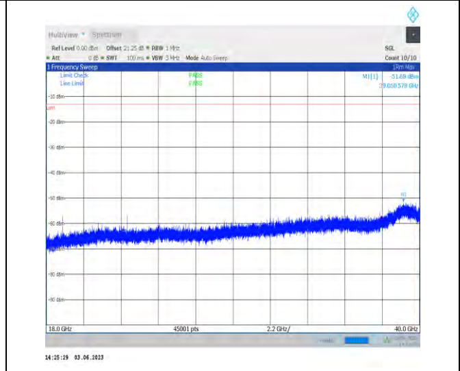
1-N77-3700-3980-PC3-30-100-M-1-N/A-DFT-PI2BPS K-Inner_1RB_Left-1@1-18000-40000-Ant1-39050.58-51.68-13-PASS
