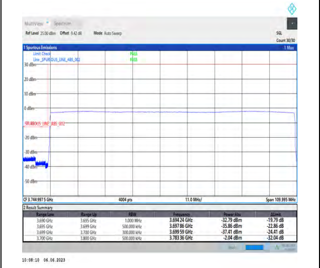
1-N77-3700-3980-PC3-30-100-L-6-CP-QPSK-Outer_Full-273@0-Ant1-1--PASS-see graph
