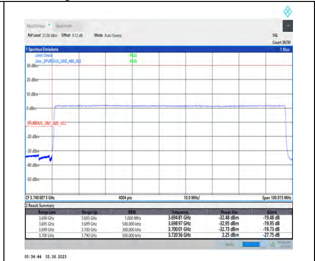
1-N77-3700-3980-PC3-30-90-L-3-DFT-PI2BPSK-Outer_Full-240@0-Ant1-1--PASS-see graph
