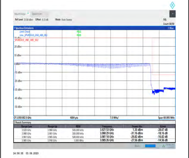
1-N77-3700-3980-PC3-30-60-H-6-CP-QPSK-Outer_Full-162@0-Ant1-1--PASS-see graph
