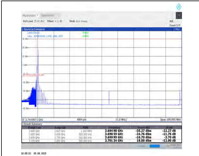
1-N77-3700-3980-PC3-30-100-L-1-DFT-PI2BPSK-Edge_1RB_Left-1@0-Ant1-1--PASS-see graph
