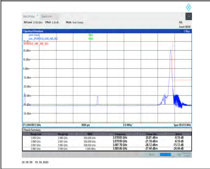
1-N77-3700-3980-PC3-30-80-H-5-CP-QPSK-Edge_1RB_Right-1@216-Ant1-1--PASS-see graph
