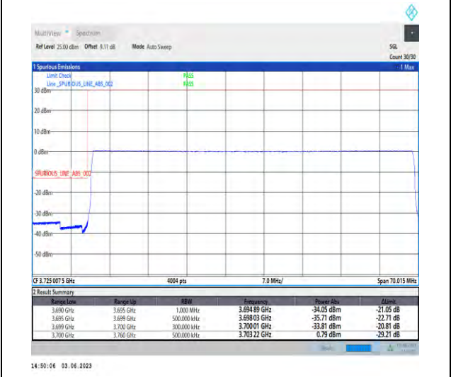
1-N77-3700-3980-PC3-30-60-L-6-CP-QPSK-Outer_Full-162@0-Ant1-1--PASS-see graph
