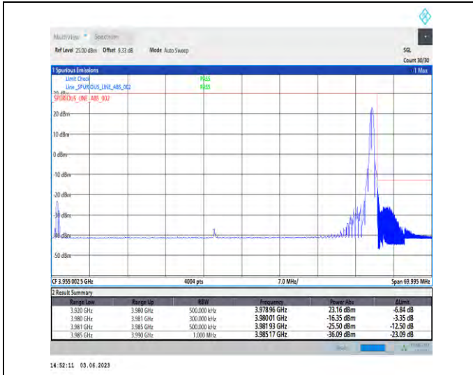
1-N77-3700-3980-PC3-30-60-H-2-DFT-PI2BPSK-Edge_1RB_Right-1@161-Ant1-1--PASS-see graph
