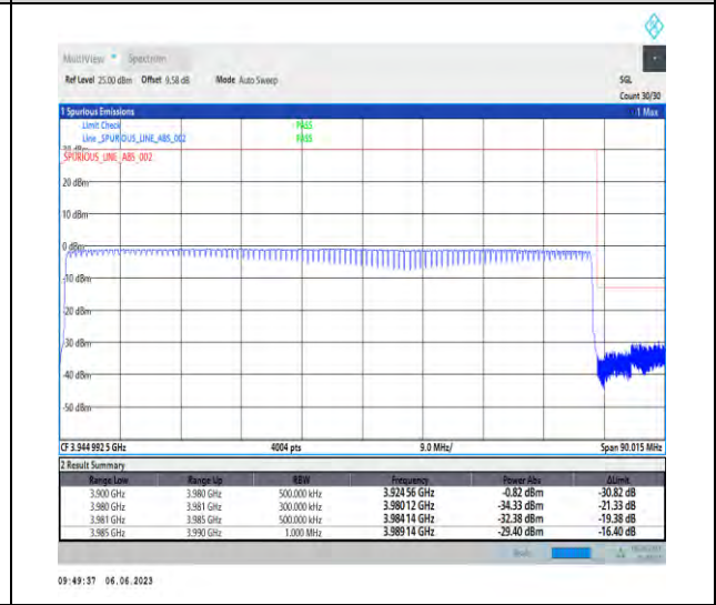
1-N77-3700-3980-PC3-30-80-H-6-CP-QPSK-Outer_Full-217@0-Ant1-1--PASS-see graph
