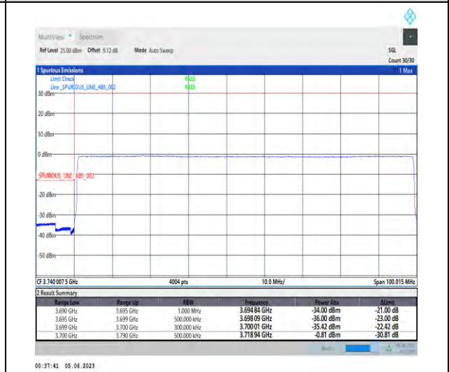
1-N77-3700-3980-PC3-30-90-L-6-CP-QPSK-Outer_Full-245@0-Ant1-1--PASS-see graph
