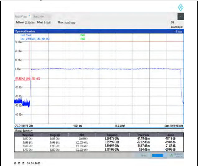
1-N77-3700-3980-PC3-30-100-L-3-DFT-PI2BPSK-Outer_Full-270@0-Ant1-1--PASS-see graph
