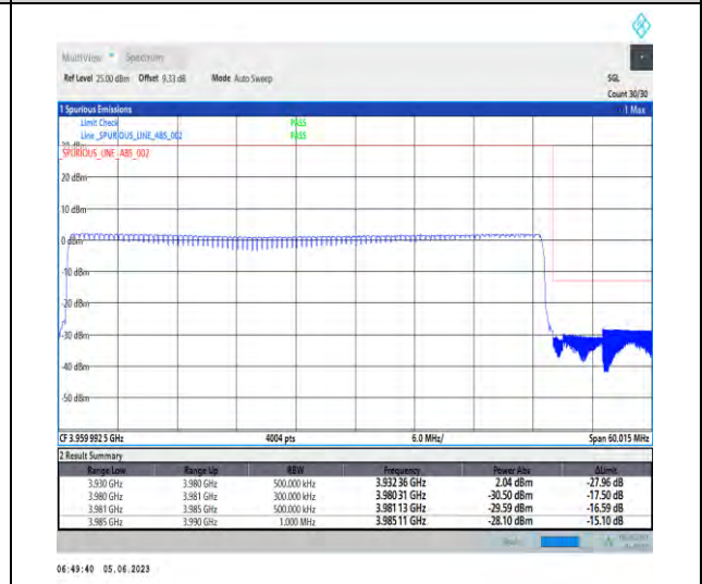
1-N77-3700-3980-PC3-30-50-H-6-CP-QPSK-Outer_Full-133@0-Ant1-1--PASS-see graph
