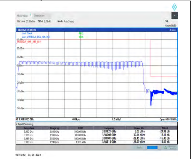
1-N77-3700-3980-PC3-30-50-H-3-DFT-PI2BPSK-Outer_Full-128@0-Ant1-1--PASS-see graph
