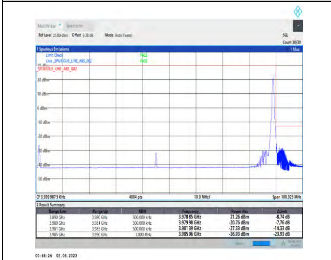
1-N77-3700-3980-PC3-30-90-H-5-CP-QPSK-Edge_1RB_Right-1@244-Ant1-1--PASS-see graph
