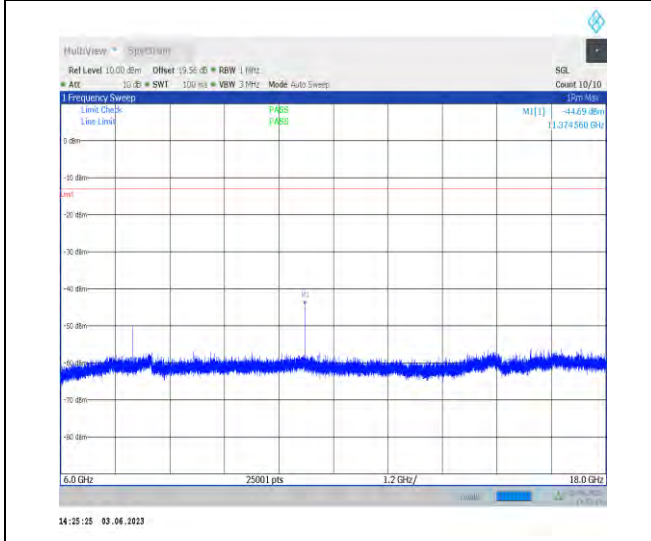
1-N77-3700-3980-PC3-30-100-M-1-N/A-DFT-PI2BP SK-Inner_1RB_Left-1@1-6000-18000-Ant1-11374.56-44.69-13-PASS
