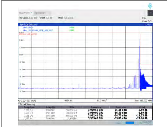
1-N77-3700-3980-PC3-30-100-H-2-DFT-PI2BPSK-Edge_1RB_Right-1@272-Ant1-1--PASS-see graph
