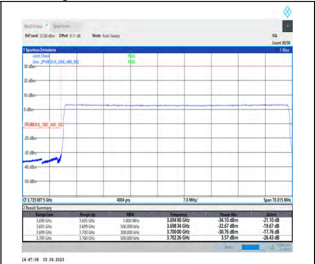
1-N77-3700-3980-PC3-30-60-L-3-DFT-PI2BPSK-Outer_Full-162@0-Ant1-1--PASS-see graph
