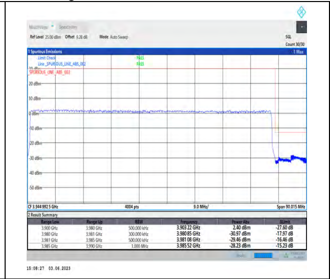
1-N77-3700-3980-PC3-30-80-H-3-DFT-PI2BPSK-Outer_Full-216@0-Ant1-1--PASS-see graph
