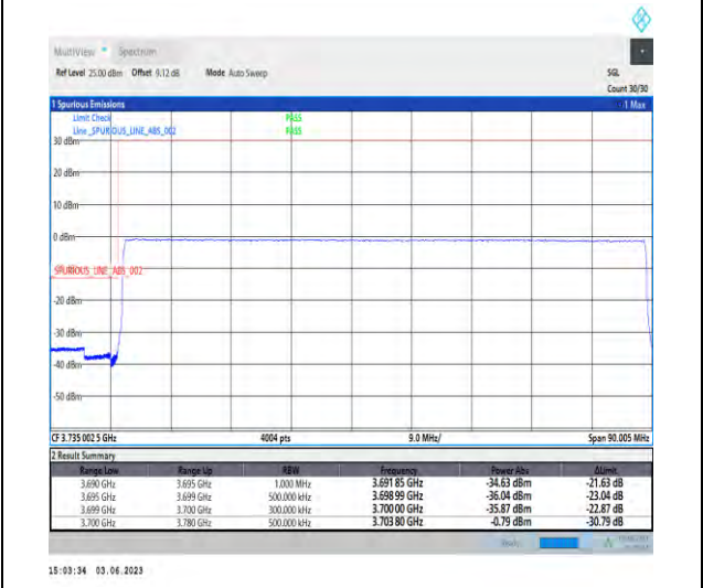
1-N77-3700-3980-PC3-30-80-L-6-CP-QPSK-Outer_Full-217@0-Ant1-1--PASS-see graph
