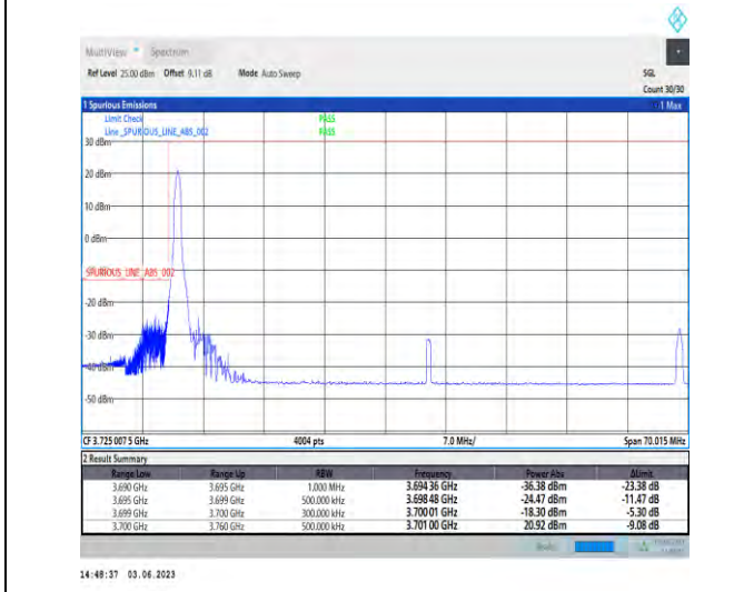
1-N77-3700-3980-PC3-30-60-L-4-CP-QPSK-Edge_1RB_Left-1@0-Ant1-1--PASS-see graph
