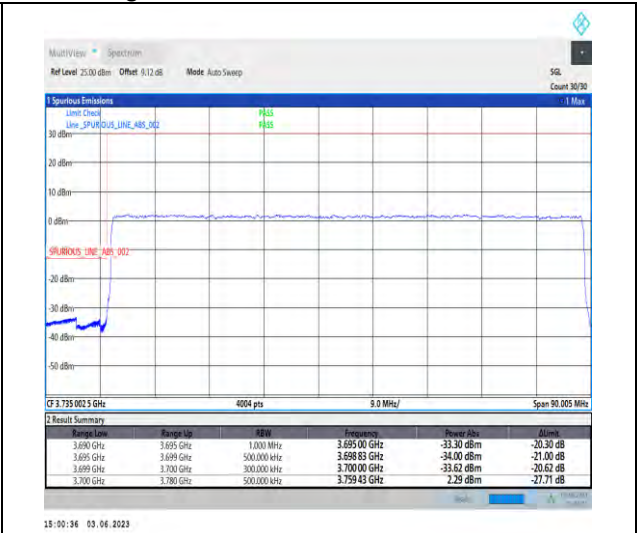
1-N77-3700-3980-PC3-30-80-L-3-DFT-PI2BPSK-Outer_Full-216@0-Ant1-1--PASS-see graph
