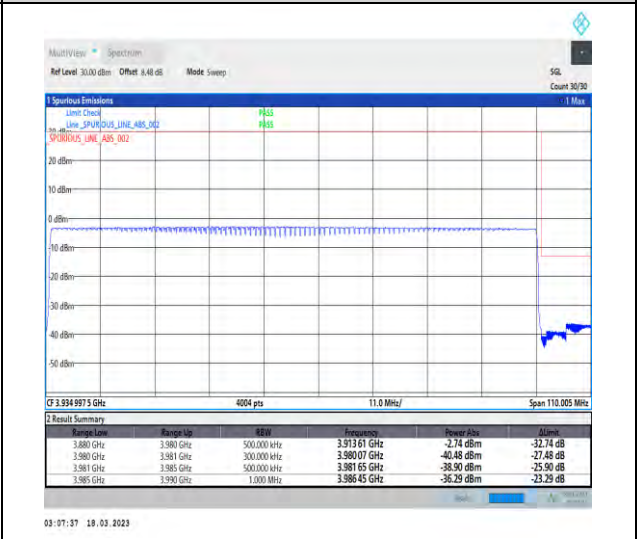
1-N77-3700-3980-PC3-30-100-H-6-CP-QPSK-Outer_Full-273@0-Ant1-1--PASS-see graph
