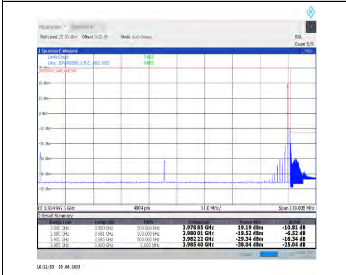
1-N77-3700-3980-PC3-30-100-H-5-CP-QPSK-Edge_1RB_Right-1@272-Ant1-1--PASS-see graph
