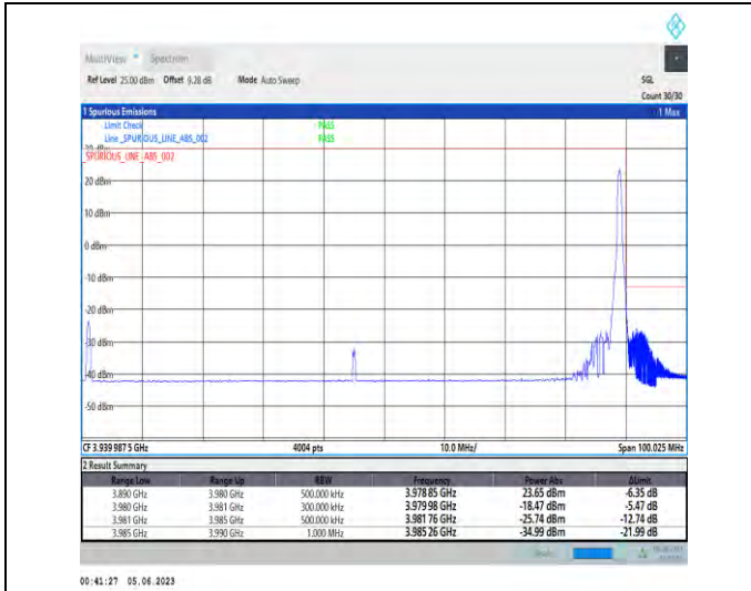
1-N77-3700-3980-PC3-30-90-H-2-DFT-PI2BPSK-Edge_1RB_Right-1@244-Ant1-1--PASS-see graph
