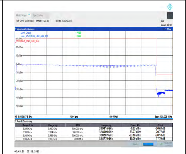
1-N77-3700-3980-PC3-30-90-H-6-CP-QPSK-Outer_Full-245@0-Ant1-1--PASS-see graph
