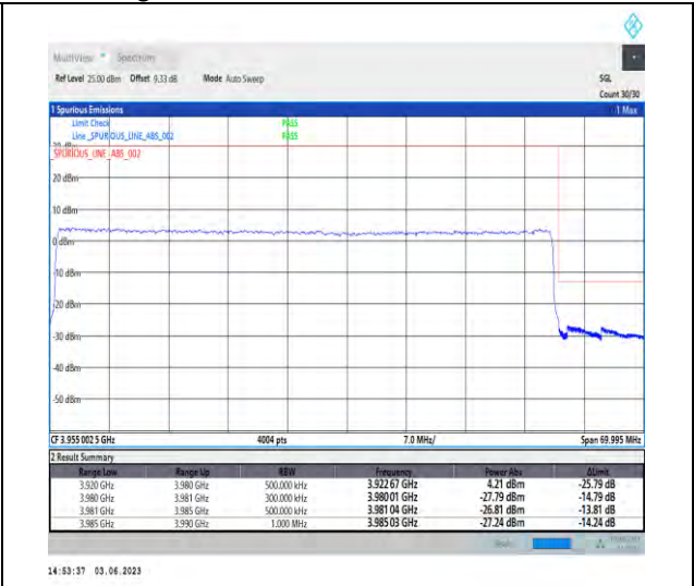
1-N77-3700-3980-PC3-30-60-H-3-DFT-PI2BPSK-Outer_Full-162@0-Ant1-1--PASS-see graph
