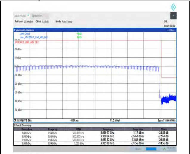
1-N77-3700-3980-PC3-30-100-H-3-DFT-PI2BPSK-Outer_Full-270@0-Ant1-1--PASS-see graph
