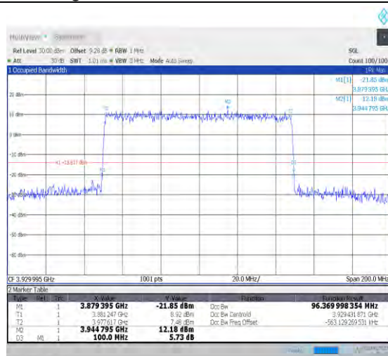
1-N77-3700-3980-PC3-30-100-H-3-DFT-16QAM-Outer_Full-270@0-Ant1-96.37-100.000-≤100-PASS
