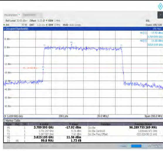
1-N77-3700-3980-PC3-30-100-M-4-DFT-64QAM-Ou ter_Full-270@0-Ant1-96.29-99.800-≤100-PASS
