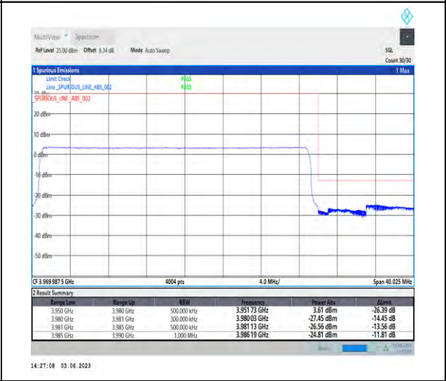
1-N77-3700-3980-PC3-30-30-H-6-CP-QPSK-Outer_Full-78@0-Ant1-1--PASS-see graph
