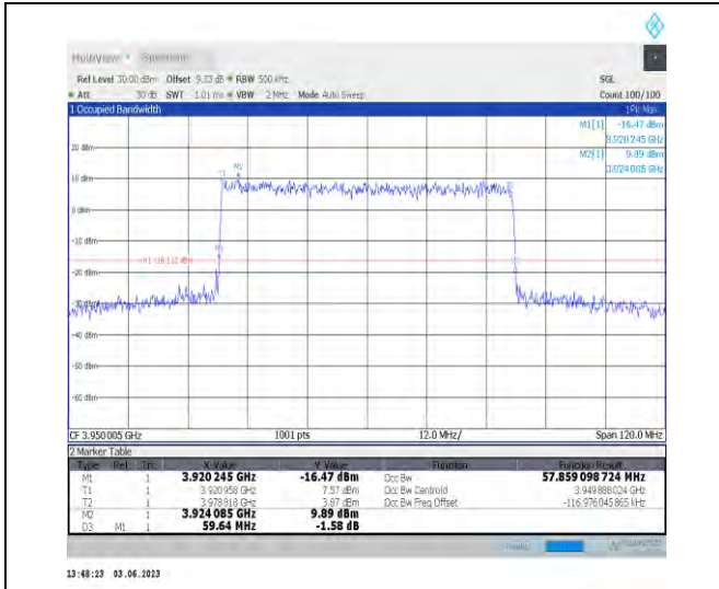
1-N77-3700-3980-PC3-30-60-H-7-CP-16QAM-Outer _Full-162@0-Ant1-57.859-59.640-≤60-PASS
