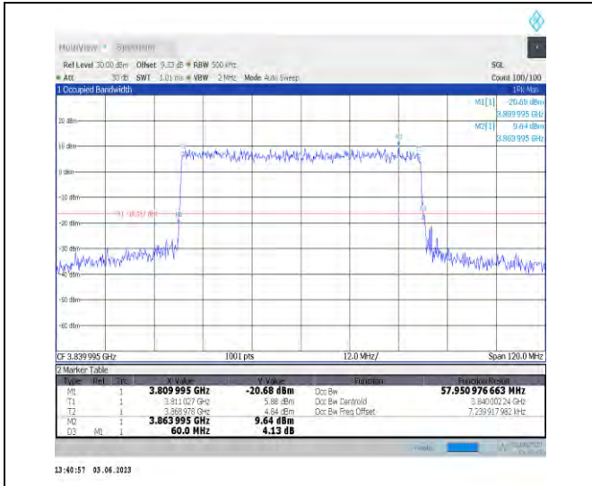
1-N77-3700-3980-PC3-30-60-M-8-CP-64QAM-Outer_Full-162@0-Ant1-57.951-60.000-≤60-PASS
