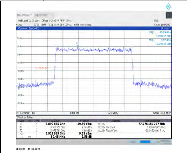
1-N77-3700-3980-PC3-30-80-H-9-CP-256QAM-Outer_Full-217@0-Ant1-77.276-80.480-≤80-PASS
