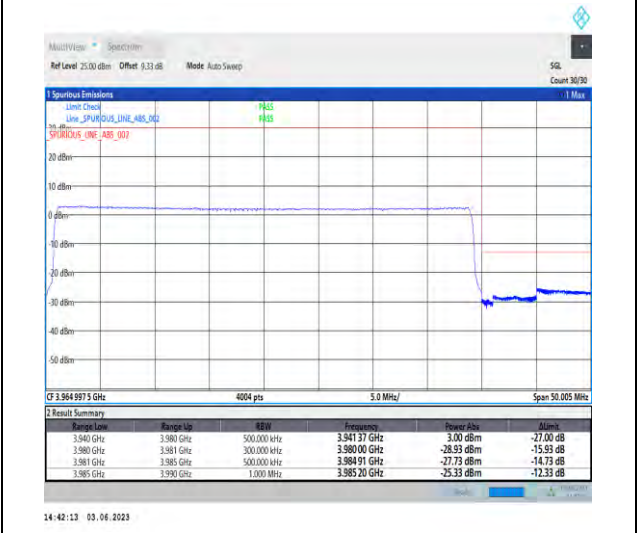
1-N77-3700-3980-PC3-30-40-H-6-CP-QPSK-Outer_Full-106@0-Ant1-1--PASS-see graph
