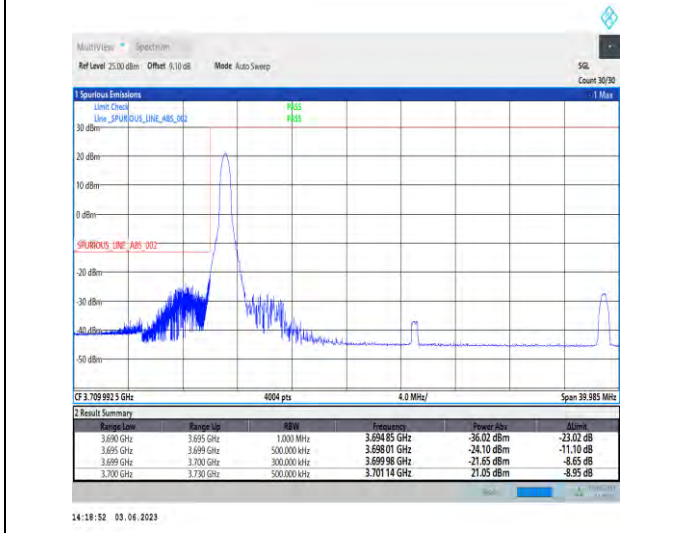
1-N77-3700-3980-PC3-30-30-L-4-CP-QPSK-Edge_1RB_Left-1@0-Ant1-1--PASS-see graph
