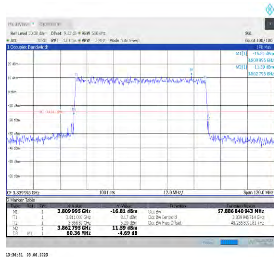
1-N77-3700-3980-PC3-30-60-M-3-DFT-16QAM-Outer_Full-162@0-Ant1-57.887-60.360-≤60-PASS
