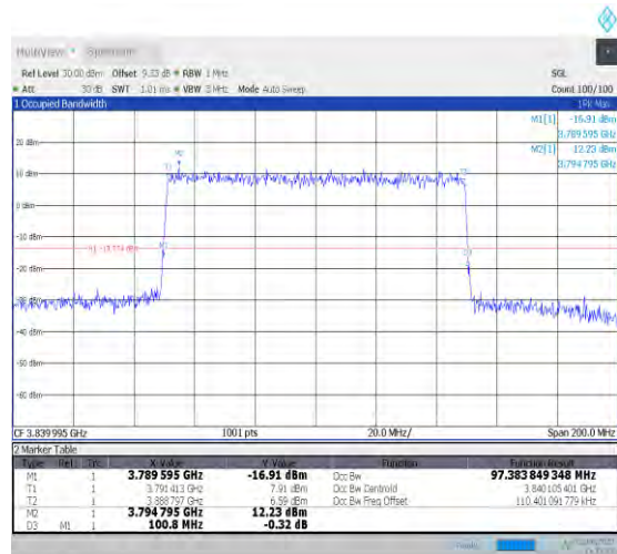
1-N77-3700-3980-PC3-30-100-M-4-DFT-64QAM-Ou ter_Full-270@0-Ant1-96.29-99.800-≤100-PASS
