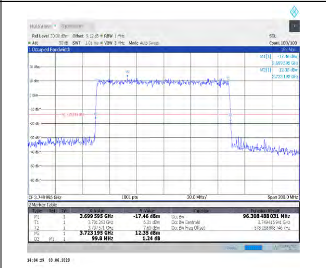
1-N77-3700-3980-PC3-30-100-L-3-DFT-16QAM-Outer_Full-270@0-Ant1-96.308-99.800-≤100-PASS
