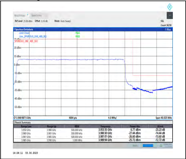
1-N77-3700-3980-PC3-30-30-H-3-DFT-PI2BPSK-Outer_Full-75@0-Ant1-1--PASS-see graph
