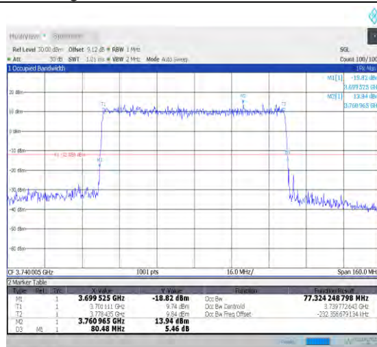
1-N77-3700-3980-PC3-30-80-L-3-DFT-16QAM-Out er_Full-216@0-Ant1-77.324-80.480-≤80-PASS
