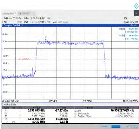
1-N77-3700-3980-PC3-30-80-M-5-DFT-256QAM-Out er_Full-216@0-Ant1-76.95-80.320-≤80-PASS
