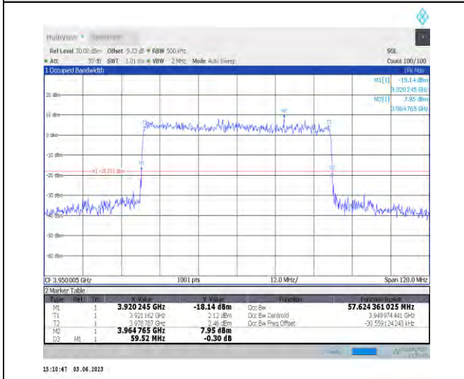
1-N77-3700-3980-PC3-30-60-H-9-CP-256QAM-Outer _Full-162@0-Ant1-57.624-59.520-≤60-PASS
