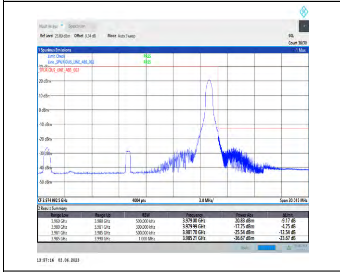
1-N77-3700-3980-PC3-30-20-H-5-CP-QPSK-Edge_1RB_Right-1@50-Ant1-1--PASS-see graph
