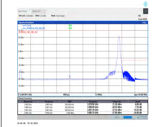
1-N77-3700-3980-PC3-30-40-H-5-CP-QPSK-Edge_1RB_Right-1@105-Ant1-1--PASS-see graph
