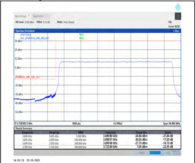
1-N77-3700-3980-PC3-30-30-L-3-DFT-PI2BPSK-Outer_Full-75@0-Ant1-1--PASS-see graph
