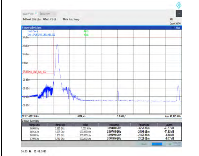
1-N77-3700-3980-PC3-30-40-L-4-CP-QPSK-Edge_1RB_Left-1@0-Ant1-1--PASS-see graph
