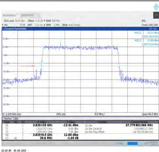
1-N77-3700-3980-PC3-30-40-M-6-CP-QPSK-Outer_Full-106@0-Ant1-37.78-39.600-≤40-PASS
