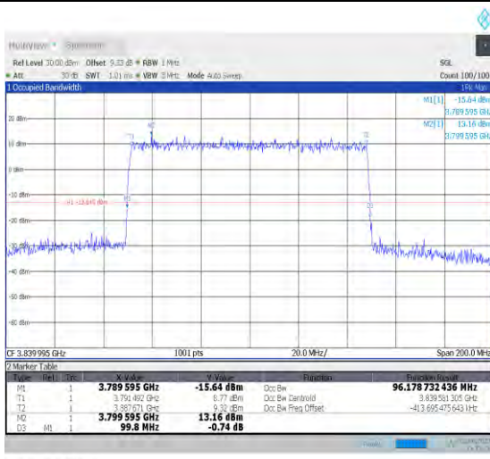
1-N77-3700-3980-PC3-30-100-M-3-DFT-16QAM-Out er_Full-270@0-Ant1-96.179-99.800-≤100-PASS
