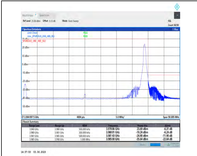
1-N77-3700-3980-PC3-30-40-H-2-DFT-PI2BPSK-Edge_1RB_Right-1@105-Ant1-1--PASS-see graph
