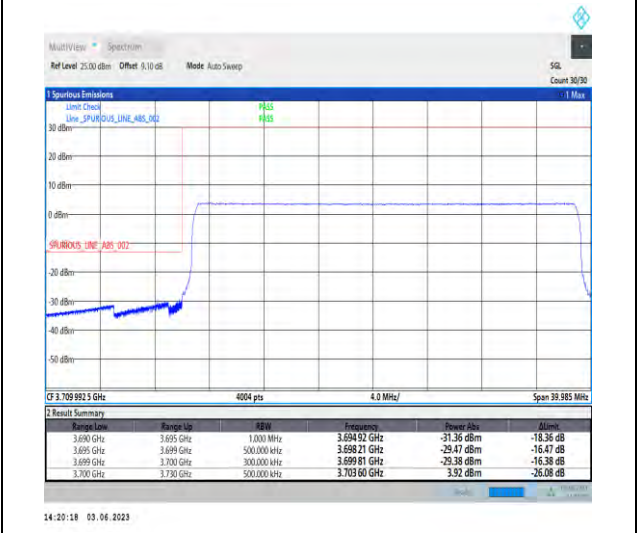
1-N77-3700-3980-PC3-30-30-L-6-CP-QPSK-Outer_Full-78@0-Ant1-1--PASS-see graph
