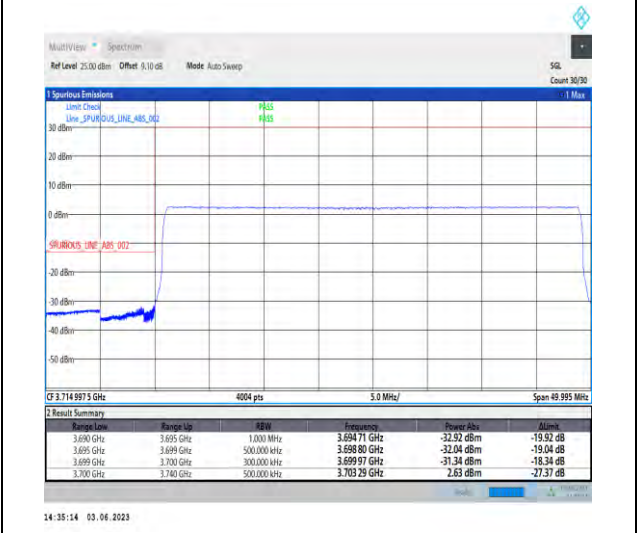
1-N77-3700-3980-PC3-30-40-L-6-CP-QPSK-Outer_Full-106@0-Ant1-1--PASS-see graph
