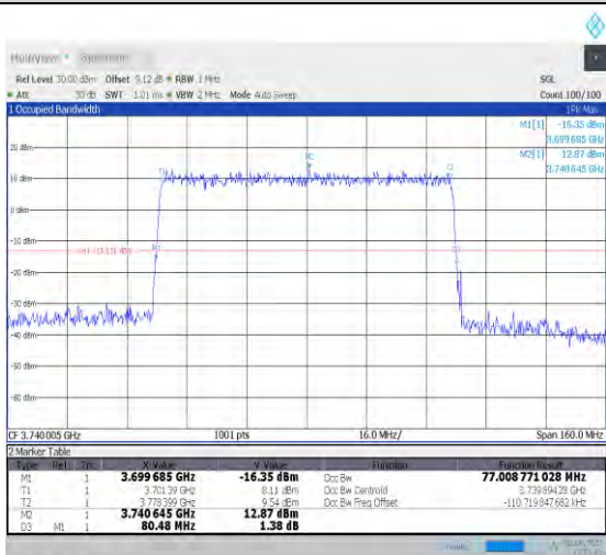
1-N77-3700-3980-PC3-30-80-L-2-DFT-PI2BPSK-Out er_Full-216@0-Ant1-77.233-80.320-≤80-PASS
