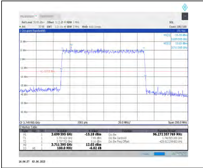
1-N77-3700-3980-PC3-30-100-L-4-DFT-64QAM-Out_er_Full-270@0-Ant1-96.272-100.000-≤100-PASS
