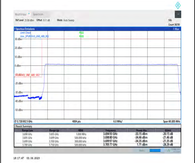
1-N77-3700-3980-PC3-30-50-L-6-CP-QPSK-Outer_Full-133@0-Ant1-1--PASS-see graph
