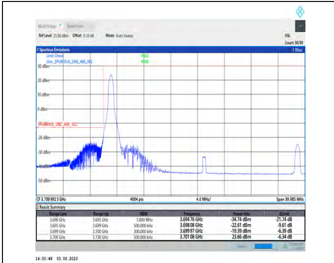
1-N77-3700-3980-PC3-30-30-L-1-DFT-PI2BPSK-Edge_1RB_Left-1@0-Ant1-1--PASS-see graph
