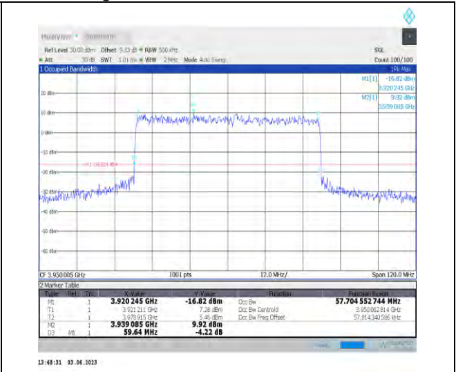
1-N77-3700-3980-PC3-30-60-H-8-CP-64QAM-Outer _Full-162@0-Ant1-57.705-59.640-≤60-PASS
