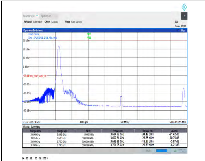
1-N77-3700-3980-PC3-30-40-L-1-DFT-PI2BPSK-Edge_1RB_Left-1@0-Ant1-1--PASS-see graph
