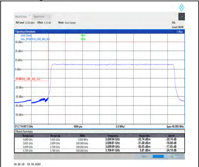
1-N77-3700-3980-PC3-30-40-L-3-DFT-PI2BPSK-Outer_Full-100@0-Ant1-1--PASS-see graph
