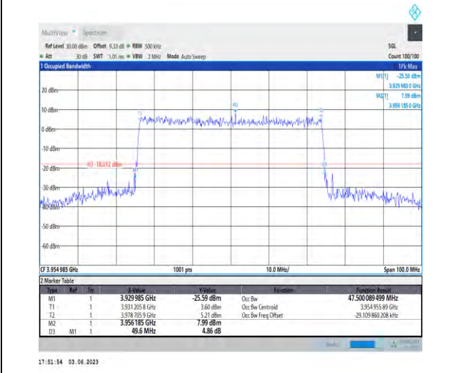
1-N77-3700-3980-PC3-30-50-H-9-CP-256QAM-Outer_Full-133@0-Ant1-47.5-49.600-≤50-PASS
