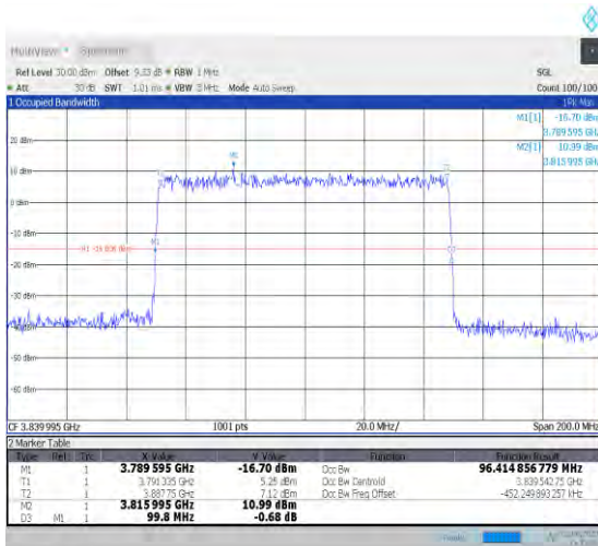
1-N77-3700-3980-PC3-30-100-M-3-DFT-16QAM-Out er_Full-270@0-Ant1-96.179-99.800-≤100-PASS
