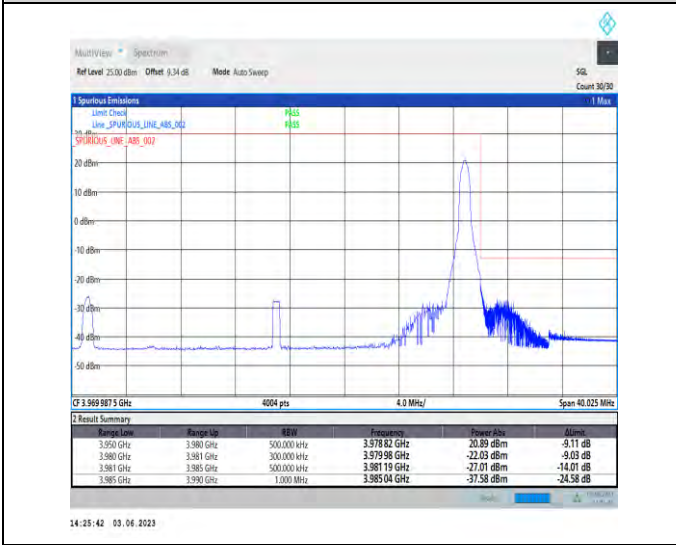
1-N77-3700-3980-PC3-30-30-H-5-CP-QPSK-Edge_1RB_Right-1@77-Ant1-1--PASS-see graph
