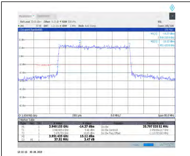
1-N77-3700-3980-PC3-30-40-H-1-DFT-QPSK-Outer_Full-100@0-Ant1-35.798-37.520-≤40-PASS
