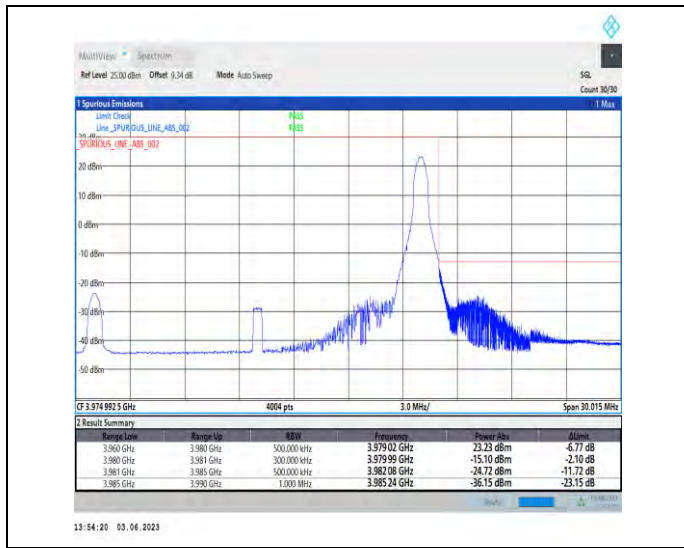
1-N77-3700-3980-PC3-30-20-H-2-DFT-PI2BPSK-Edge_1RB_Right-1@50-Ant1-1--PASS-see graph
