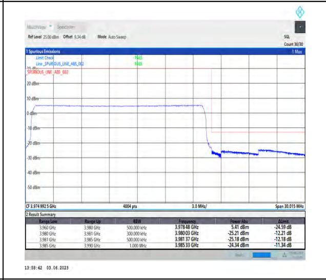
1-N77-3700-3980-PC3-30-20-H-6-CP-QPSK-Outer_Full-51@0-Ant1-1--PASS-see graph
