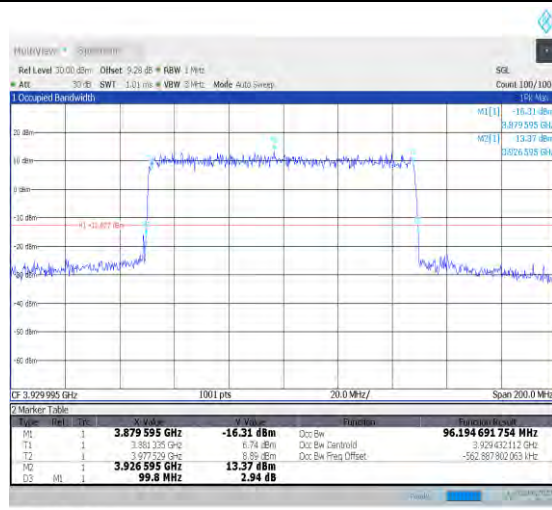
1-N77-3700-3980-PC3-30-100-M-8-CP-64QAM-Outer_Full-273@0-Ant1-97.168-101.000-≤100-PASS
