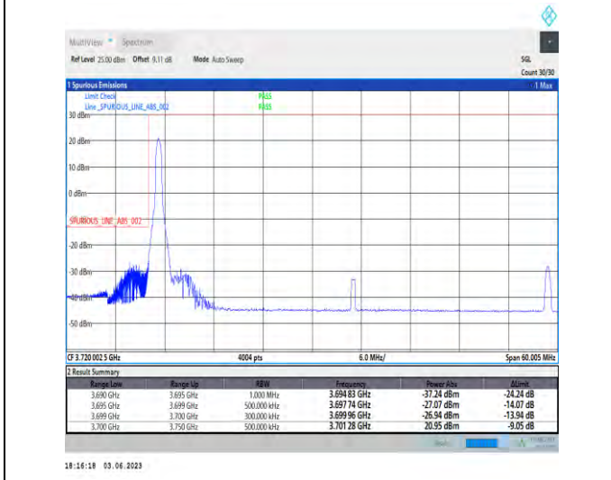
1-N77-3700-3980-PC3-30-50-L-4-CP-QPSK-Edge_1RB_Left-1@0-Ant1-1--PASS-see graph
