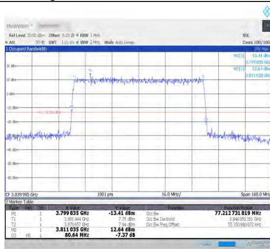
1-N77-3700-3980-PC3-30-80-M-6-CP-QPSK-Outer_ Full-217@0-Ant1-77.213-80.640-≤80-PASS
