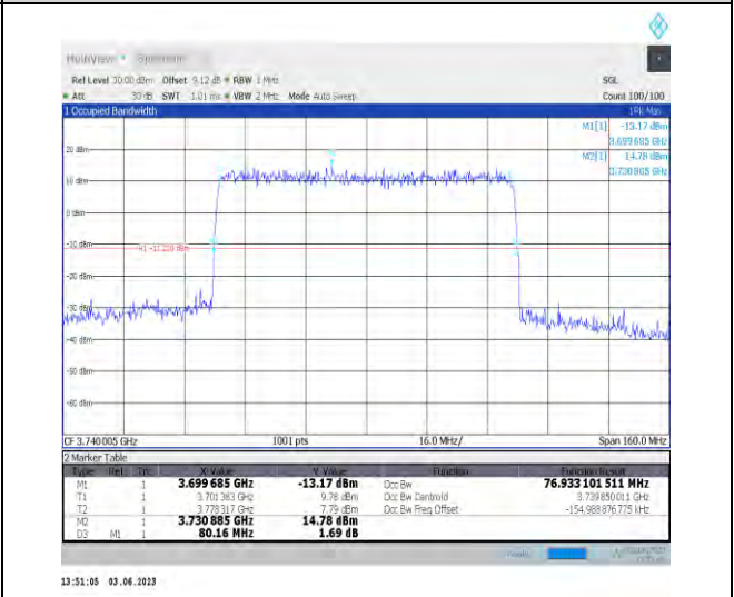
1-N77-3700-3980-PC3-30-80-L-1-DFT-QPSK-Outer _Full-216@0-Ant1-76.933-80.160-≤80-PASS
