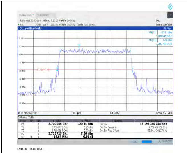
1-N77-3700-3980-PC3-30-20-L-9-CP-256QAM-Outer_Full-51@0-Ant1-18.198-19.640-≤20-PASS
