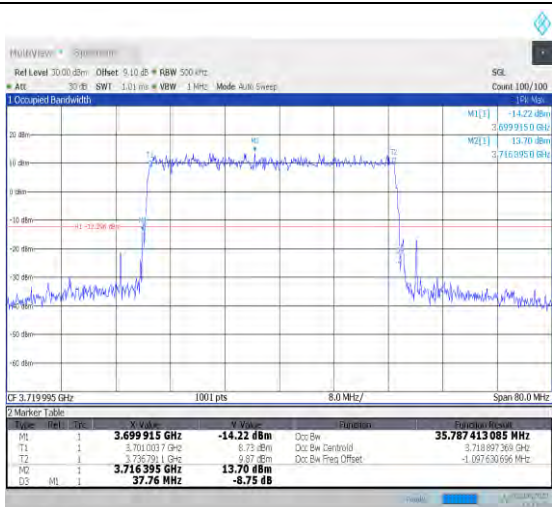
1-N77-3700-3980-PC3-30-40-L-3-DFT-16QAM-Outer_Full-100@0-Ant1-35.787-37.760-≤40-PASS
