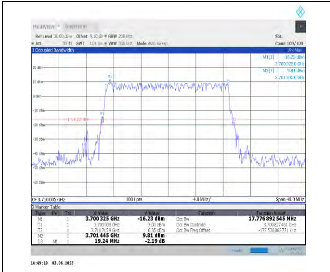
1-N77-3700-3980-PC3-30-20-L-5-DFT-256QAM-Outer_Full-50@0-Ant1-17.777-19.240-≤20-PASS
