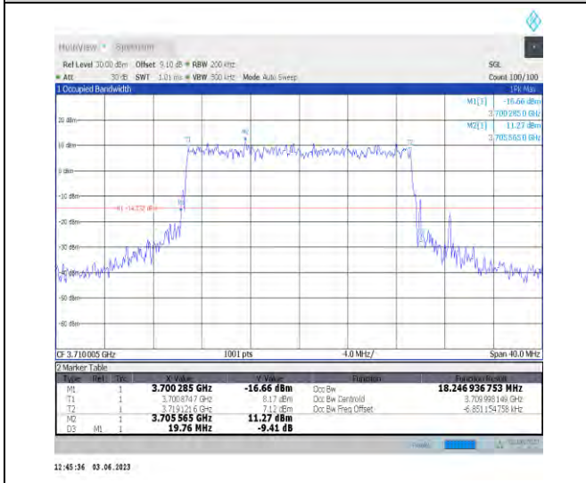
1-N77-3700-3980-PC3-30-20-L-7-CP-16QAM-Outer_Full-51@0-Ant1-18.247-19.760-≤20-PASS
