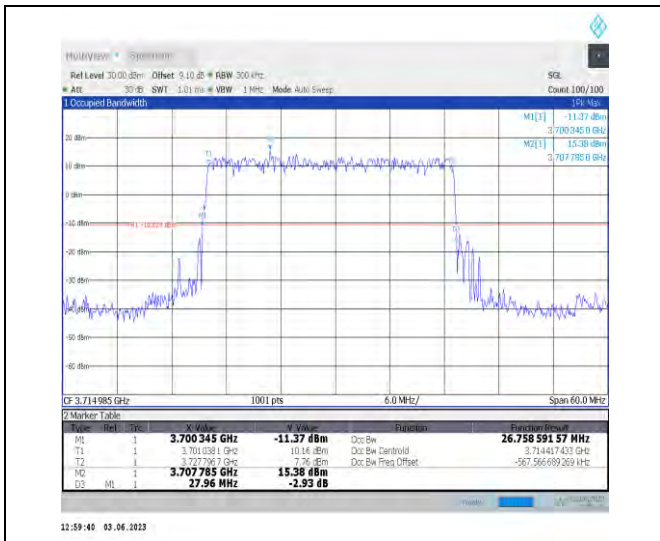
1-N77-3700-3980-PC3-30-30-L-2-DFT-PI2BPSK-Out er_Full-75@0-Ant1-26.759-27.960-≤30-PASS
