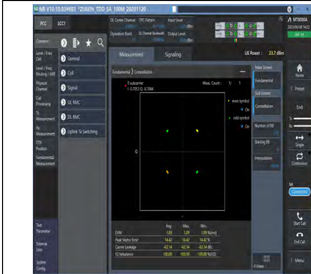
1-N77-3700-3980-PC3-30-100-M-1-DFT-PI2BPSK-Outer_Full-270@0-Ant1-see graph-PASS
