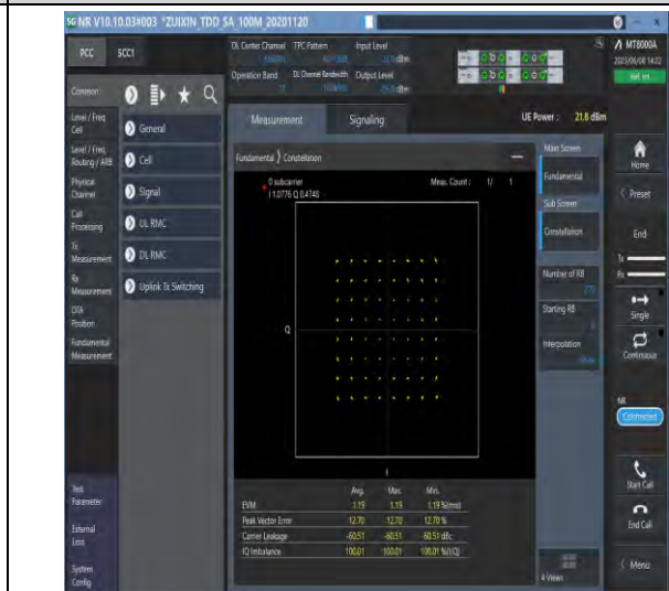
1-N77-3700-3980-PC3-30-100-M-4-DFT-64QAM-Out er_Full-270@0-Ant1-see graph-PASS
