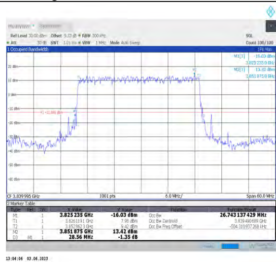
1-N77-3700-3980-PC3-30-30-M-2-DFT-PI2BPSK-Outer_Full-75@0-Ant1-26.743-28.560-≤30-PASS
