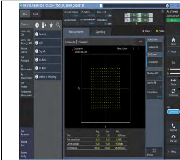
1-N77-3700-3980-PC3-30-100-M-5-DFT-256QAM-Outer_Full-270@0-Ant1-see graph-PASS
