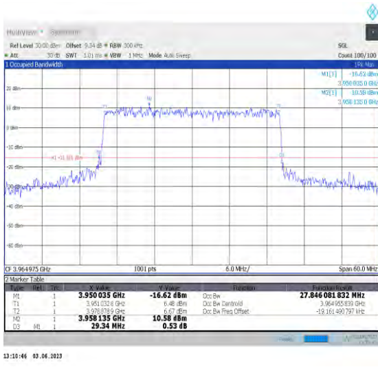
1-N77-3700-3980-PC3-30-30-H-6-CP-QPSK-Outer_Full-78@0-Ant1-27.846-29.340-≤30-PASS
