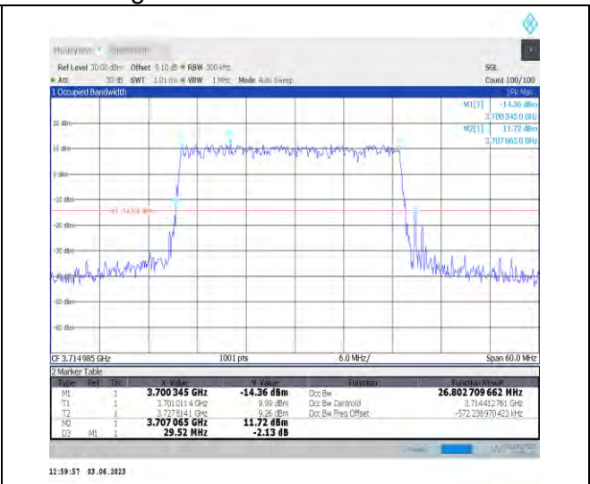
1-N77-3700-3980-PC3-30-30-L-3-DFT-16QAM-Out er_Full-75@0-Ant1-26.803-29.520-≤30-PASS
