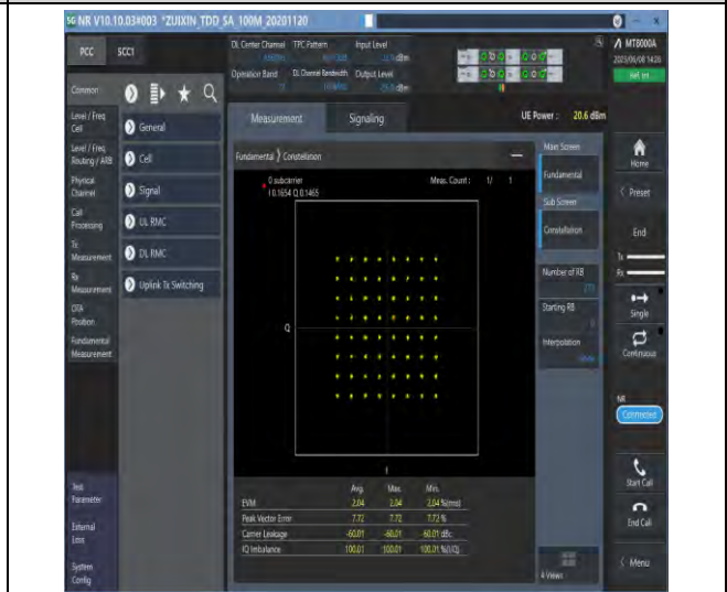
1-N77-3700-3980-PC3-30-100-M-8-CP-64QAM-Outer_Full-273@0-Ant1-see graph-PASS
