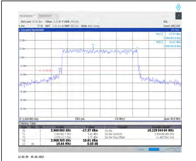
1-N77-3700-3980-PC3-30-20-H-7-CP-16QAM-Outer_Full-51@0-Ant1-18.23-19.640-≤20-PASS
