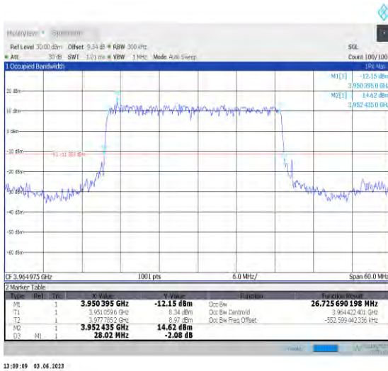
1-N77-3700-3980-PC3-30-30-H-2-DFT-PI2BPSK-Outer_Full-75@0-Ant1-26.726-28.020-≤30-PASS
