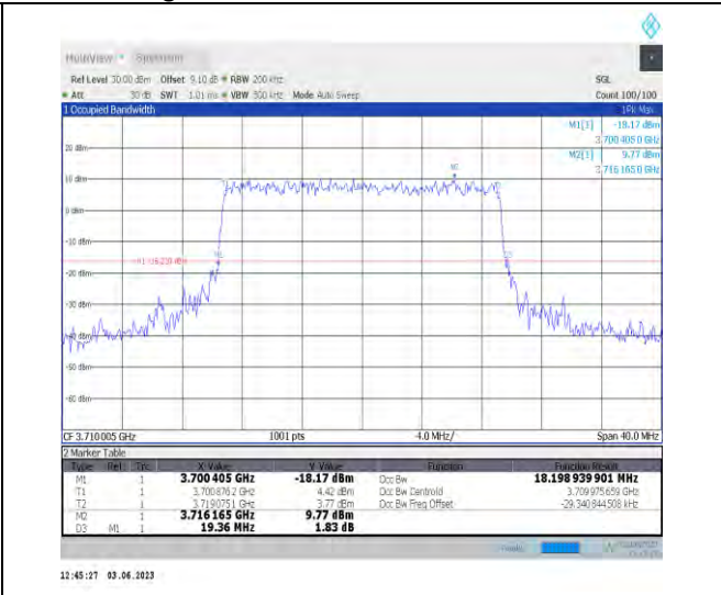
1-N77-3700-3980-PC3-30-20-L-6-CP-QPSK-Outer_Full-51@0-Ant1-18.199-19.360-≤20-PASS
