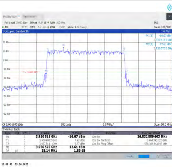
1-N77-3700-3980-PC3-30-30-H-4-DFT-64QAM-Outer_Full-75@0-Ant1-26.833-28.140-≤30-PASS
