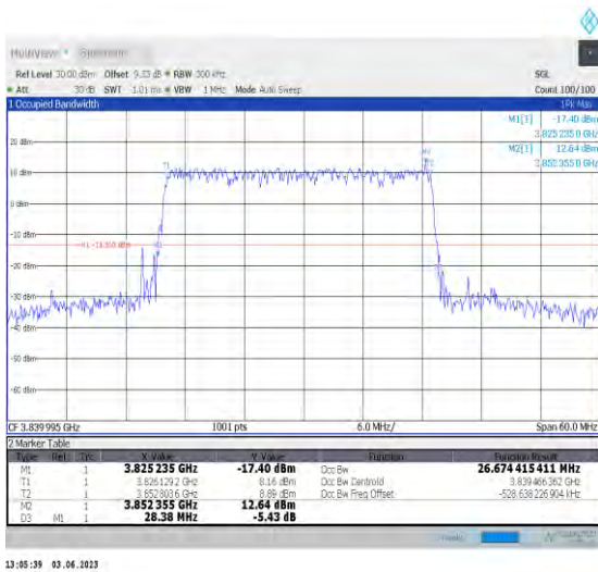
1-N77-3700-3980-PC3-30-30-M-3-DFT-16QAM-Outer_Full-75@0-Ant1-26.674-28.380-≤30-PASS
