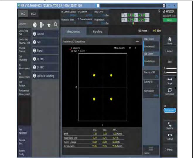
1-N77-3700-3980-PC3-30-100-M-6-CP-QPSK-Outer_Full-273@0-Ant1-see graph-PASS
