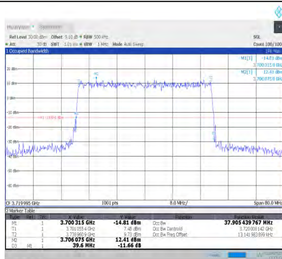
1-N77-3700-3980-PC3-30-40-L-4-DFT-64QAM-Outer_Full-100@0-Ant1-35.753-37.840-≤40-PASS
