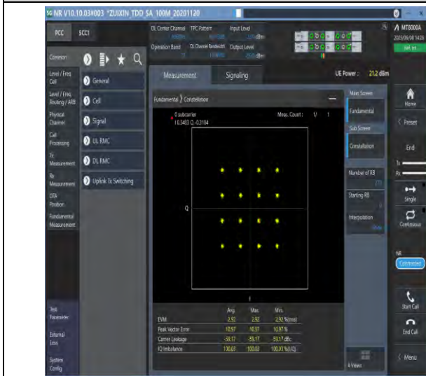
1-N77-3700-3980-PC3-30-100-M-7-CP-16QAM-Outer_Full-273@0-Ant1-see graph-PASS
