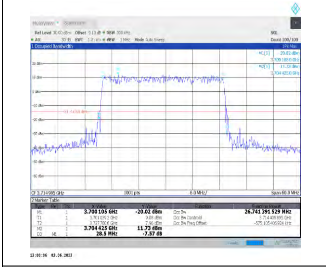
1-N77-3700-3980-PC3-30-30-L-4-DFT-64QAM-Out er_Full-75@0-Ant1-26.741-28.500-≤30-PASS
