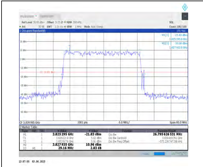
1-N77-3700-3980-PC3-30-30-M-5-DFT-256QAM-Out _Full-75@0-Ant1-26.796-29.160-≤30-PASS
