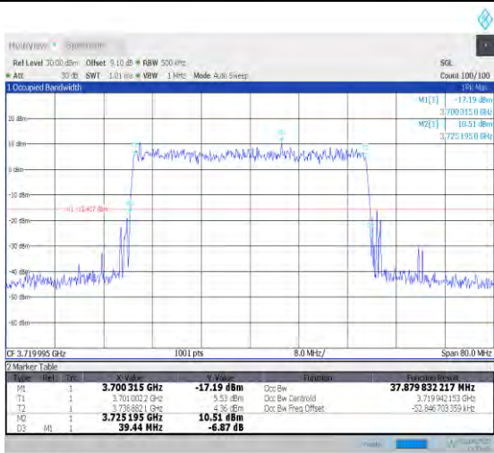
1-N77-3700-3980-PC3-30-40-L-7-CP-16QAM-Outer _Full-106@0-Ant1-37.806-39.760-≤40-PASS
