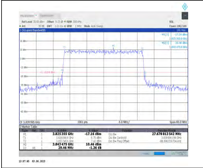
1-N77-3700-3980-PC3-30-30-M-7-CP-16QAM-Outer _Full-78@0-Ant1-27.679-29.460-≤30-PASS
