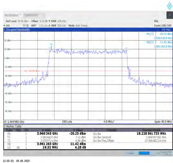
1-N77-3700-3980-PC3-30-20-H-6-CP-QPSK-Outer_Full-51@0-Ant1-18.229-19.520-≤20-PASS
