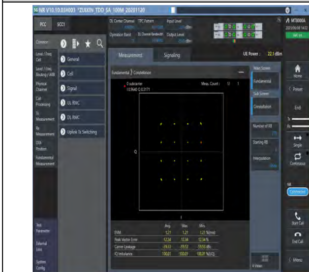
1-N77-3700-3980-PC3-30-100-M-3-DFT-16QAM-Out er_Full-270@0-Ant1-see graph-PASS
