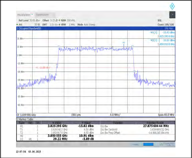
1-N77-3700-3980-PC3-30-30-M-8-CP-64QAM-Outer _Full-78@0-Ant1-27.876-29.220-≤30-PASS
