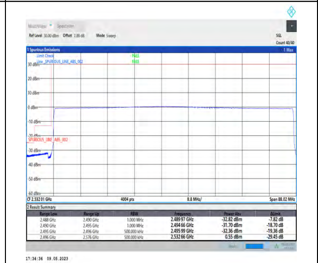
1-N41-PC3-30-80-L-6-CP-QPSK-Outer_Full-217@0-Ant1-1--PASS-see graph
