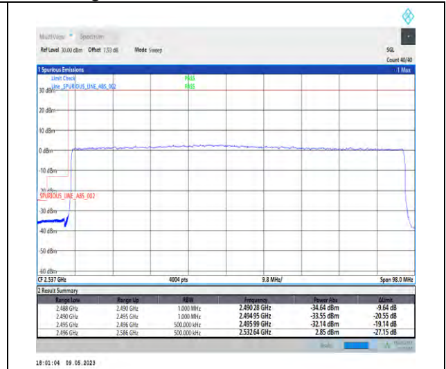
1-N41-PC3-30-90-L-3-DFT-PI2BPSK-Outer_Full-240@0-Ant1-1--PASS-see graph
