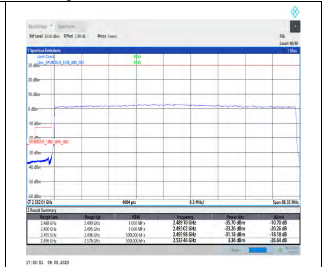
1-N41-PC3-30-80-L-3-DFT-PI2BPSK-Outer_Full-216@0-Ant1-1--PASS-see graph
