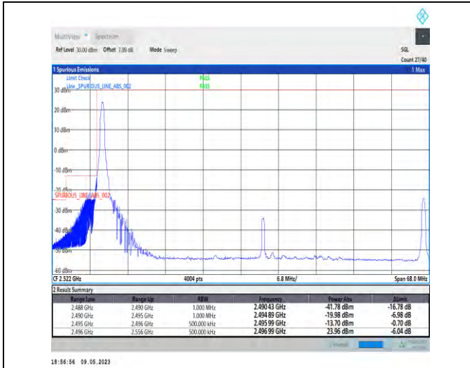
1-N41-PC3-30-60-L-1-DFT-PI2BPSK-Edge_1RB_Left-1@0-Ant1-1--PASS-see graph
