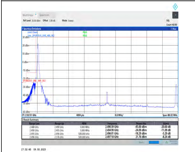
1-N41-PC3-30-80-L-4-CP-QPSK-Edge_1RB_Left-1@0-Ant1-1--PASS-see graph
