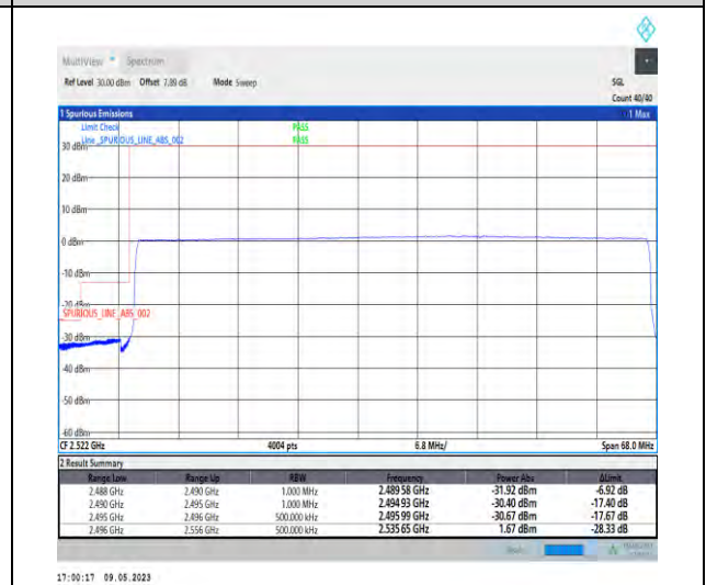
1-N41-PC3-30-60-L-6-CP-QPSK-Outer_Full-162@0-Ant1-1--PASS-see graph
