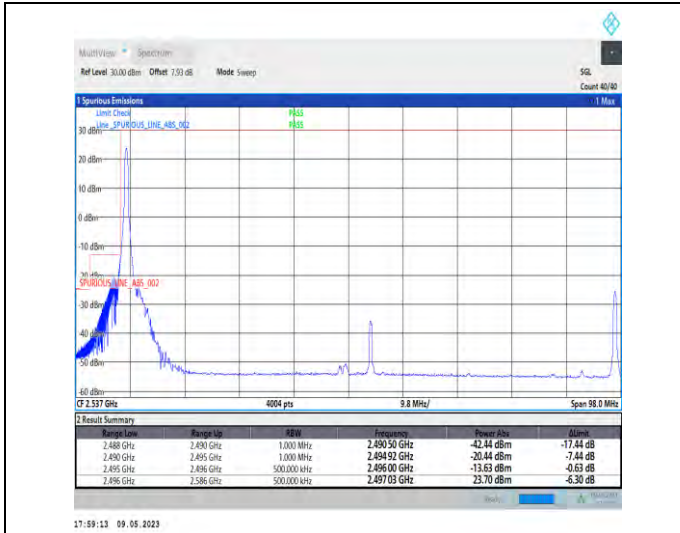
1-N41-PC3-30-90-L-1-DFT-PI2BPSK-Edge_1RB_Left-1@0-Ant1-1--PASS-see graph
