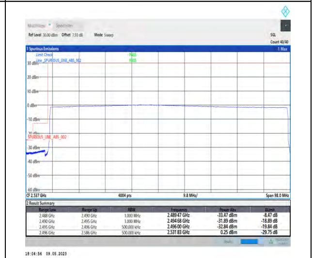
1-N41-PC3-30-90-L-6-CP-QPSK-Outer_Full-245@0-Ant1-1--PASS-see graph
