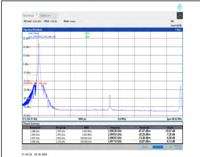
1-N41-PC3-30-80-L-1-DFT-PI2BPSK-Edge_1RB_Left-1@0-Ant1-1--PASS-see graph
