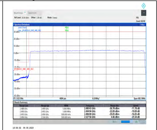
1-N41-PC3-30-60-L-3-DFT-PI2BPSK-Outer_Full-162@0-Ant1-1--PASS-see graph
