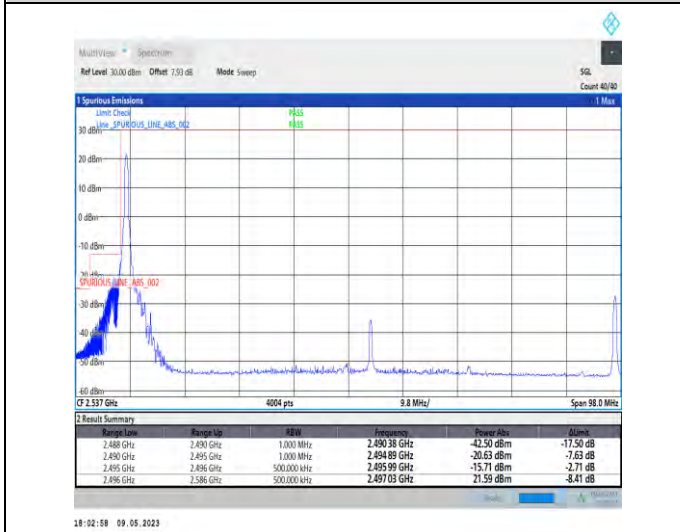
1-N41-PC3-30-90-L-4-CP-QPSK-Edge_1RB_Left-1@0-Ant1-1--PASS-see graph
