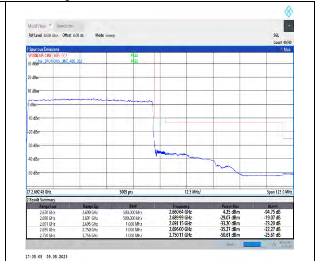
1-N41-PC3-30-60-H-3-DFT-PI2BPSK-Outer_Full-1 62@0-Ant1-1--PASS-see graph
