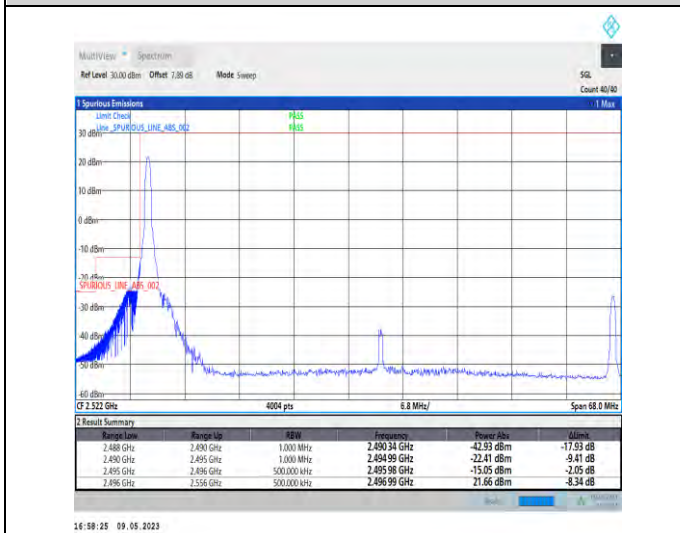
1-N41-PC3-30-60-L-4-CP-QPSK-Edge_1RB_Left-1@0-Ant1-1--PASS-see graph
