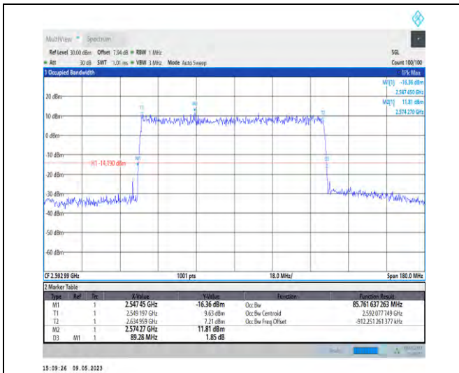
1-N41-PC3-30-90-M-5-DFT-256QAM-Outer_Full-240 @0-Ant1-85.762-89.280-≤90-PASS
