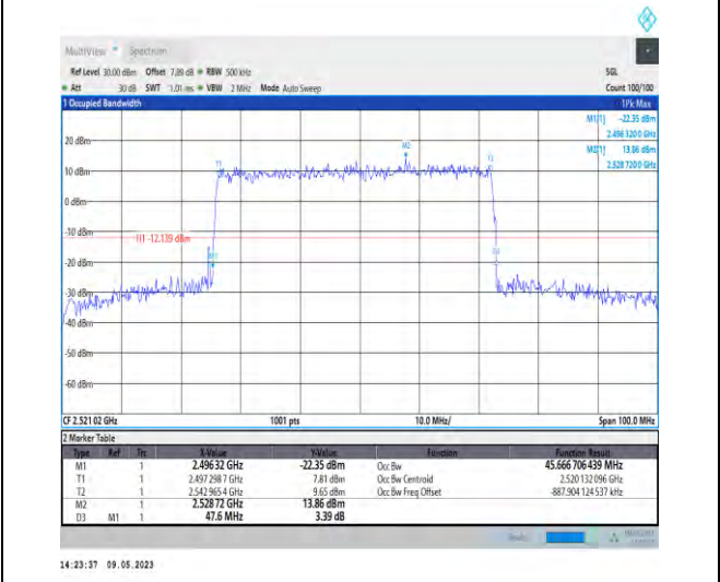
1-N41-PC3-30-50-L-3-DFT-16QAM-Outer_Full-128 @0-Ant1-45.667-47.600-≤50-PASS
