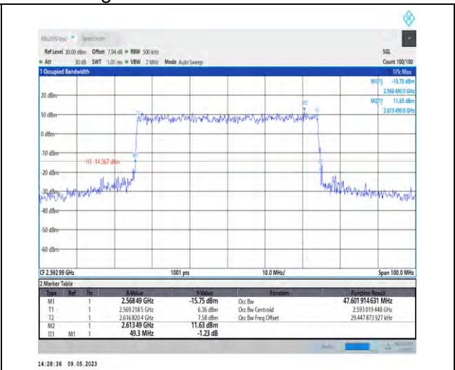
1-N41-PC3-30-50-M-8-CP-64QAM-Outer_Full-133@ 0-Ant1-47.602-49.300-≤50-PASS
