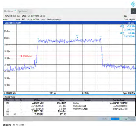
1-N41-PC3-30-40-M-9-CP-256QAM-Outer_Full-106@0 @Ant1-37.695-39.920-≤40-PASS
