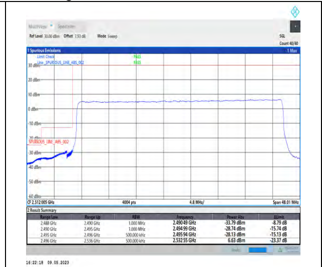
1-N41-PC3-30-40-L-3-DFT-PI2BPSK-Outer_Full-100@0-Ant1-1--PASS-see graph
