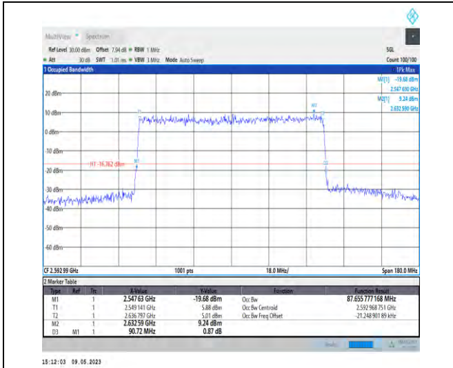
1-N41-PC3-30-90-M-9-CP-256QAM-Outer_Full-245 @0-Ant1-87.656-90.720-≤90-PASS
