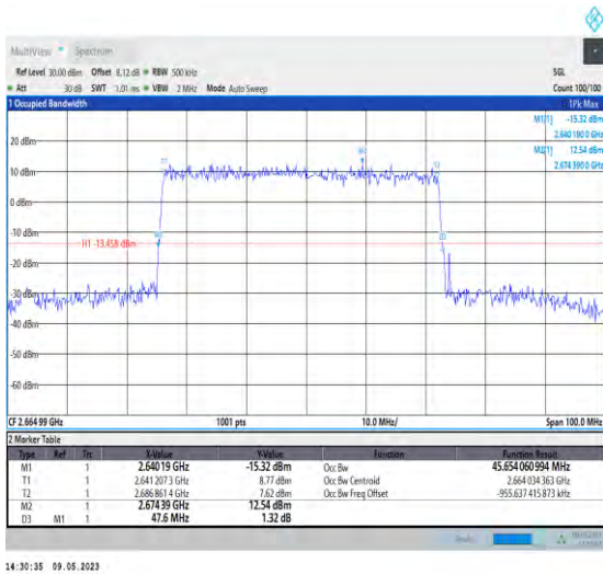
1-N41-PC3-30-50-H-4-DFT-64QAM-Outer_Full-128 @0-Ant1-45.654-47.600-≤50-PASS
