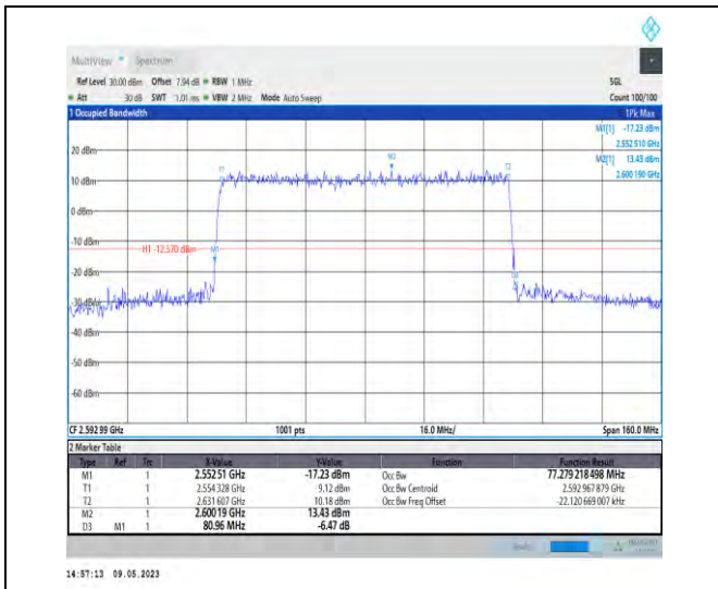
1-N41-PC3-30-80-M-4-DFT-64QAM-Outer_Full-216 @0-Ant1-77.279-80.960-≤80-PASS
