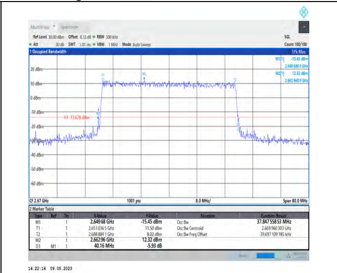
1-N41-PC3-30-40-H-6-CP-QPSK-Outer_Full-106@0-Ant1-37.848-40.160-<math>\leq 40</math>-PASS
