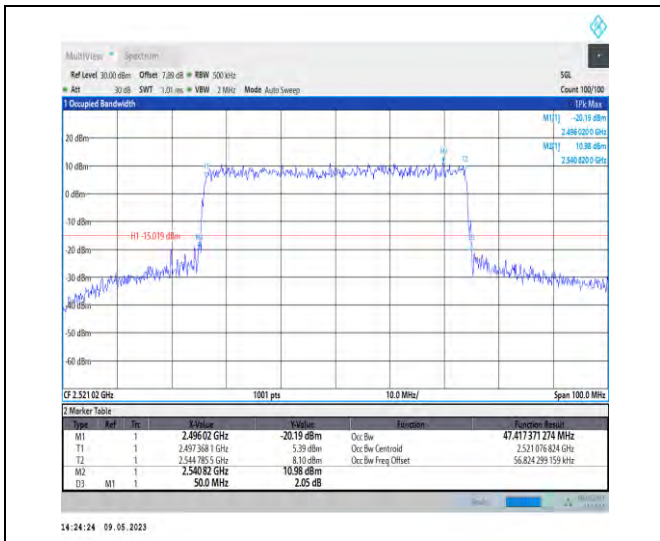
1-N41-PC3-30-50-L-8-CP-64QAM-Outer_Full-133@0-Ant1-47.417-50.000-≤50-PASS
