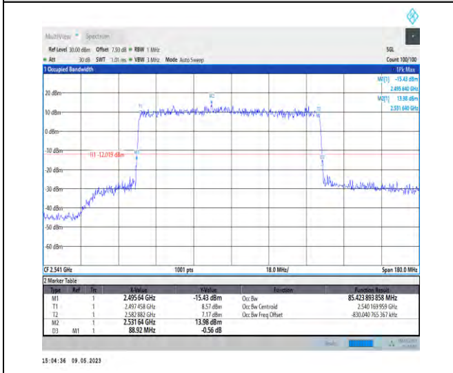
1-N41-PC3-30-90-L-4-DFT-64QAM-Outer_Full-240 @0-Ant1-85.424-88.920-≤90-PASS
