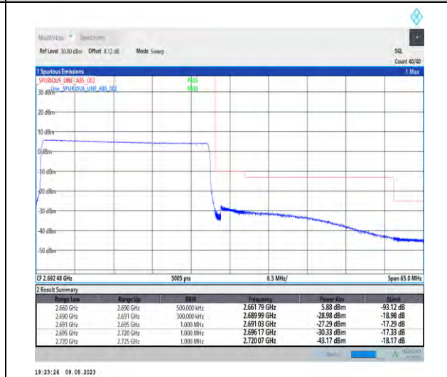
1-N41-PC3-30-30-H-6-CP-QPSK-Outer_Full-78@0-Ant1-1--PASS-see graph
