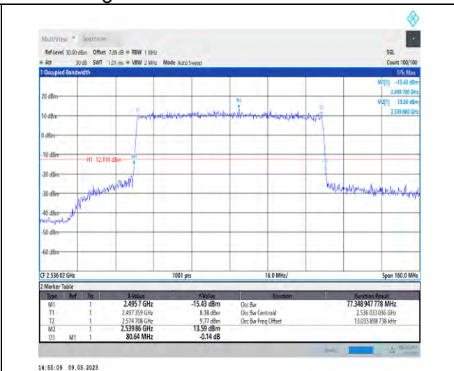
1-N41-PC3-30-80-L-6-CP-QPSK-Outer_Full-217@0-Ant1-77.349-80.640-≤80-PASS
