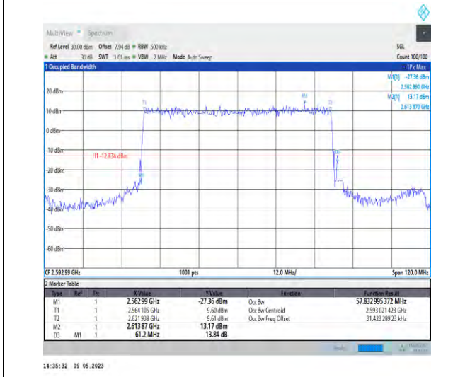
1-N41-PC3-30-60-M-2-DFT-PI2BPSK-Outer_Full-162 @0-Ant1-57.833-61.200-≤60-PASS
