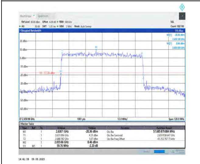
1-N41-PC3-30-60-H-9-CP-256QAM-Outer_Full-162 @0-Ant1-57.686-59.760-≤60-PASS
