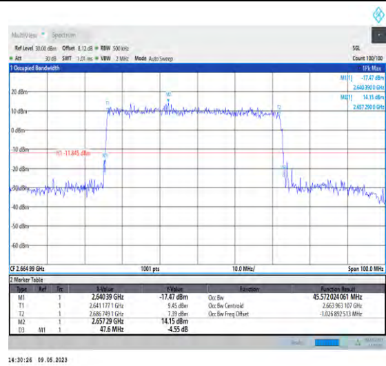
1-N41-PC3-30-50-H-3-DFT-16QAM-Outer_Full-128 @0-Ant1-45.572-47.600-≤50-PASS
