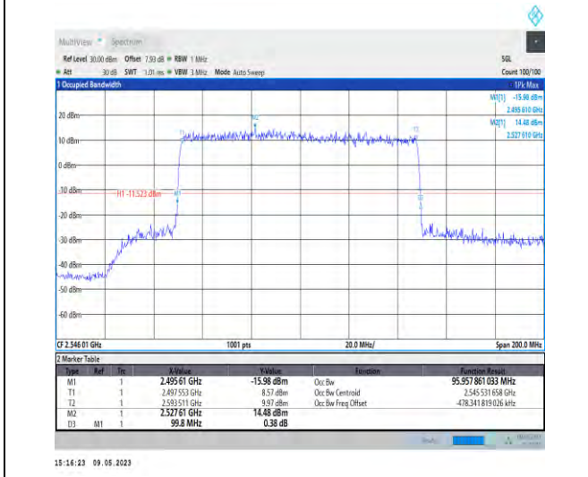
1-N41-PC3-30-100-L-1-DFT-QPSK-Outer_Full-270@ 0-Ant1-95.958-99.800-<=100-PASS
