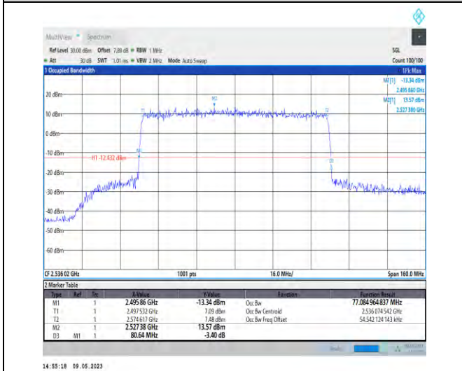
1-N41-PC3-30-80-L-7-CP-16QAM-Outer_Full-217@0-Ant1-77.085-80.640-≤80-PASS
