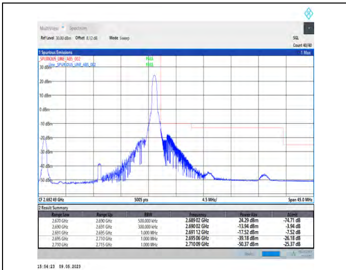
1-N41-PC3-30-20-H-2-DFT-PI2BPSK-Edge_1RB_Right-t-1@50-Ant1-1--PASS-see graph
