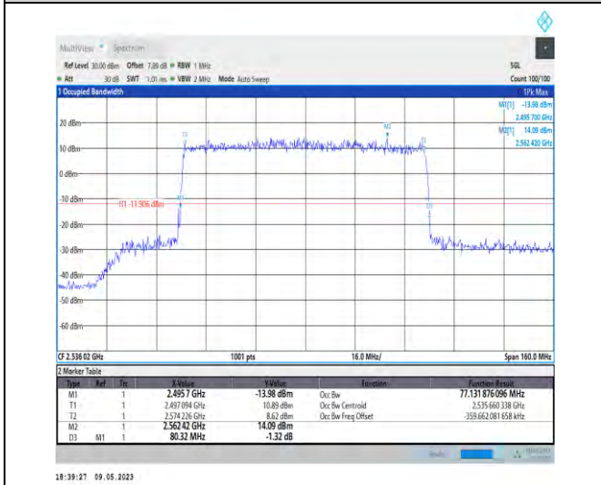
1-N41-PC3-30-80-L-3-DFT-16QAM-Outer_Full-216 @0-Ant1-77.132-80.320-≤80-PASS
