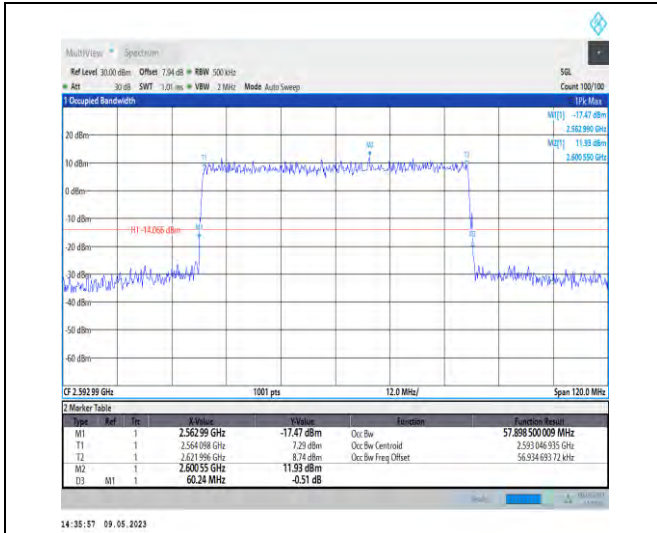
1-N41-PC3-30-60-M-4-DFT-64QAM-Outer_Full-162 @0-Ant1-57.899-60.240-≤60-PASS
