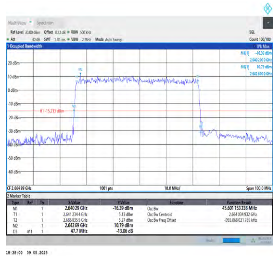
1-N41-PC3-30-50-H-5-DFT-256QAM-Outer_Full-128 @0-Ant1-45.601-47.700-≤50-PASS
