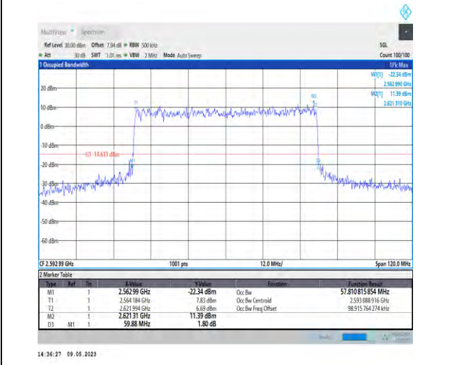
1-N41-PC3-30-60-M-7-CP-16QAM-Outer_Full-162@0 -Ant1-57.811-59.880-≤60-PASS
