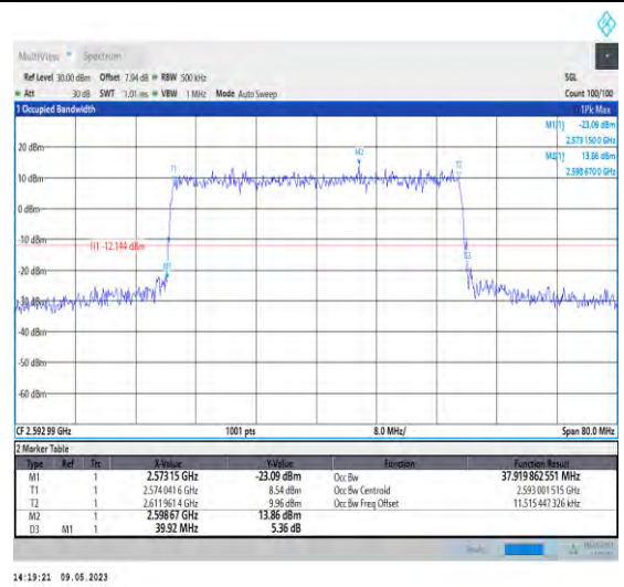
1-N41-PC3-30-40-M-7-CP-16QAM-Outer_Full-106@0 0-Ant1-37.92-39.920-≤40-PASS
