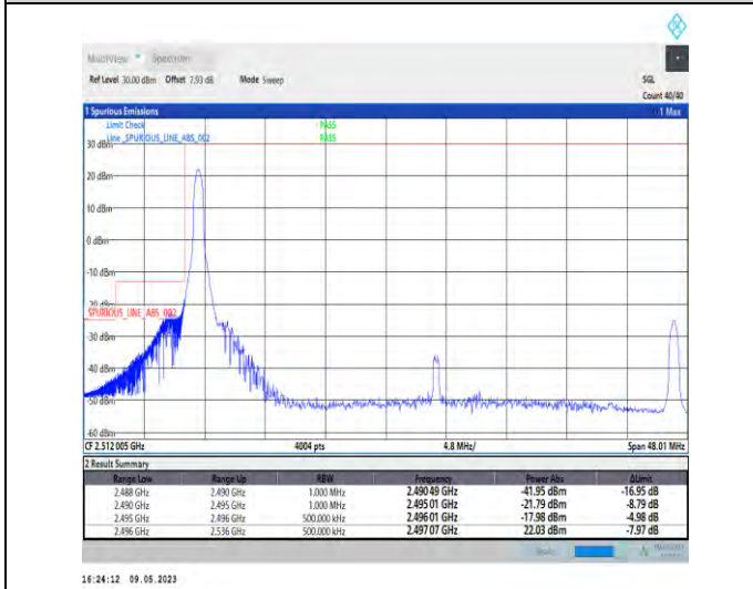
1-N41-PC3-30-40-L-4-CP-QPSK-Edge_1RB_Left-1@0-Ant1-1--PASS-see graph
