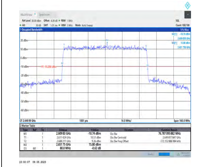
1-N41-PC3-30-80-H-1-DFT-QPSK-Outer_Full-216@0-Ant1-76.787-80.000-<=80-PASS
