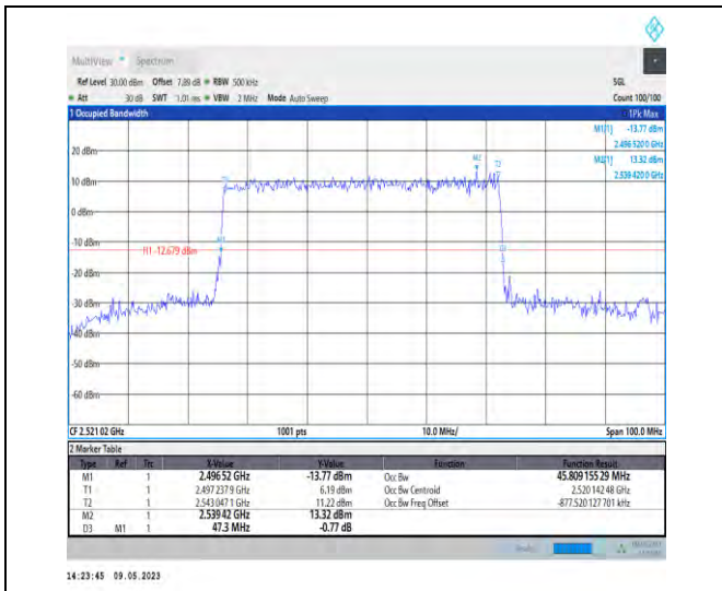
1-N41-PC3-30-50-L-4-DFT-64QAM-Outer_Full-128 @0-Ant1-45.809-47.300-≤50-PASS
