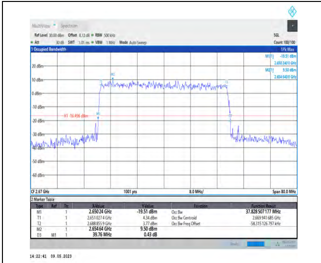
1-N41-PC3-30-40-H-9-CP-256QAM-Outer_Full-106 @0-Ant1-37.829-39.760-≤40-PASS
