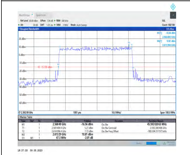
1-N41-PC3-30-50-M-5-DFT-256QAM-Outer_Full-128 @0-Ant1-45.592-47.300-≤50-PASS
