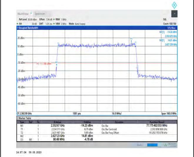
1-N41-PC3-30-80-M-3-DFT-16QAM-Outer_Full-216 @0-Ant1-77.175-80.480-≤80-PASS
