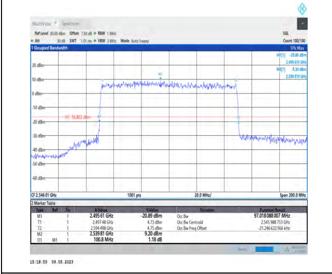
1-N41-PC3-30-100-L-9-CP-256QAM-Outer_Full-273 @0-Ant1-97.018-100.800-≤100-PASS
