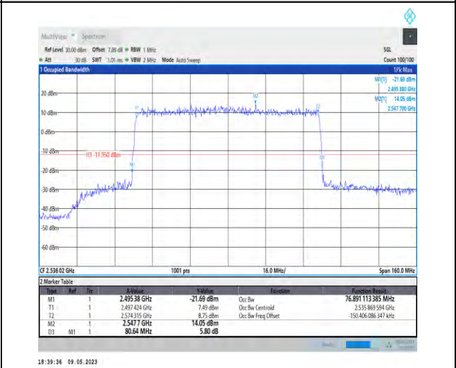
1-N41-PC3-30-80-L-4-DFT-64QAM-Outer_Full-216 @0-Ant1-76.891-80.640-≤80-PASS
