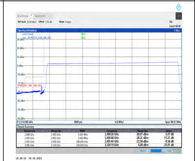
1-N41-PC3-30-40-L-6-CP-QPSK-Outer_Full-106@0-Ant1-1--PASS-see graph
