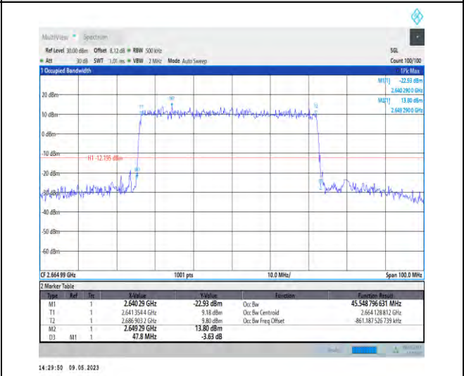
1-N41-PC3-30-50-H-1-DFT-QPSK-Outer_Full-128@ 0-Ant1-45.549-47.800-≤50-PASS
