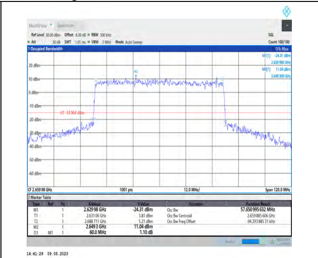
1-N41-PC3-30-60-H-8-CP-64QAM-Outer_Full-162@ 0-Ant1-57.651-60.000-≤60-PASS
