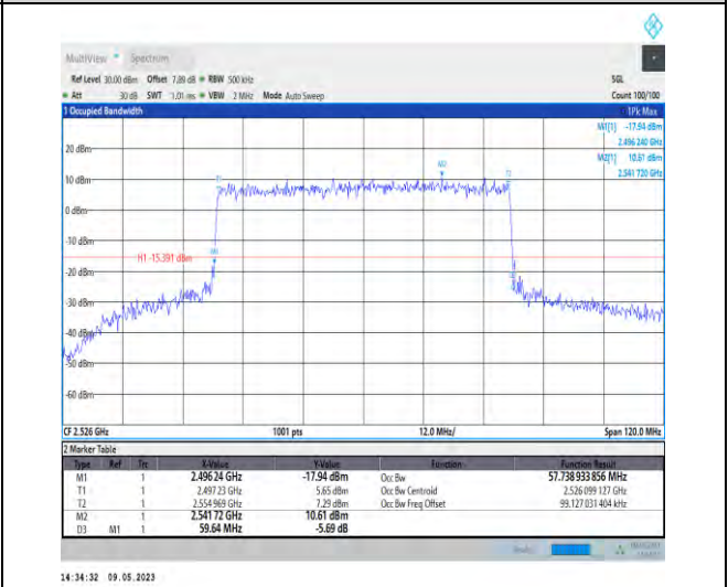
1-N41-PC3-30-60-L-8-CP-64QAM-Outer_Full-162@0-Ant1-57.739-59.640-≤60-PASS
