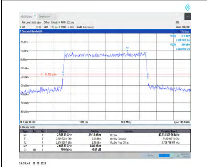
1-N41-PC3-30-50-M-9-CP-256QAM-Outer_Full-133 @0-Ant1-47.331-49.600-≤50-PASS
