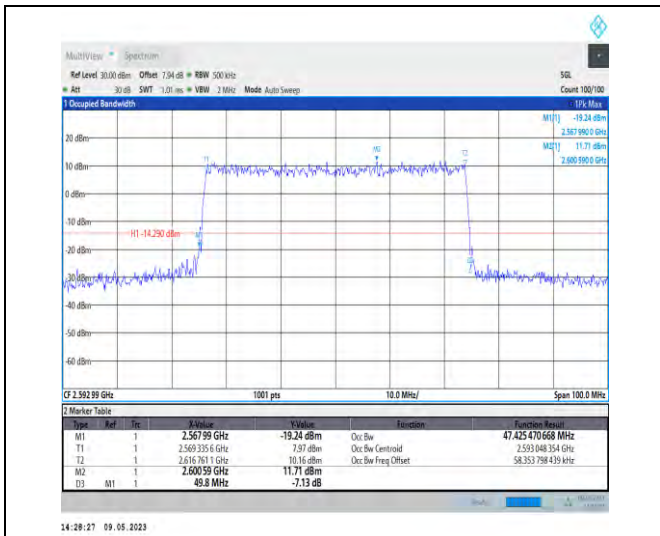
1-N41-PC3-30-50-M-7-CP-16QAM-Outer_Full-133@ 0-Ant1-47.425-49.800-≤50-PASS
