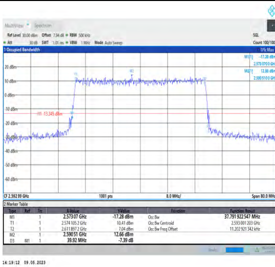
1-N41-PC3-30-40-M-6-CP-QPSK-Outer_Full-106@0 -Ant1-37.792-39.920-≤40-PASS
