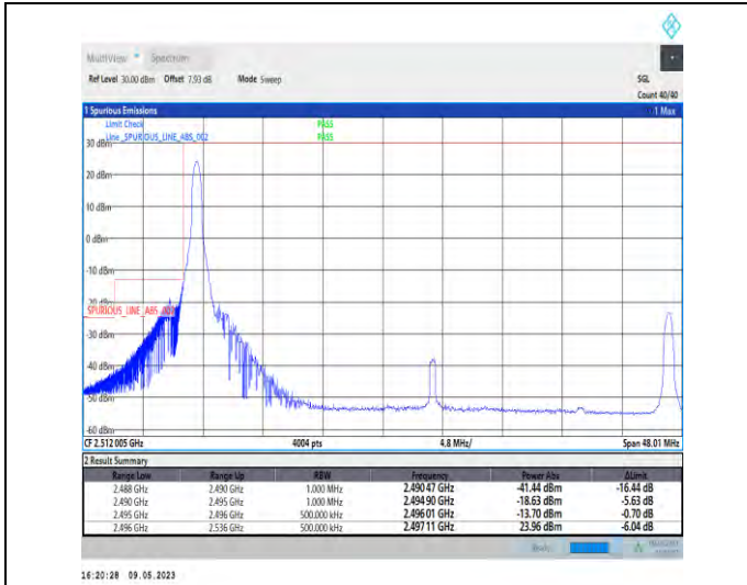
1-N41-PC3-30-40-L-1-DFT-PI2BPSK-Edge_1RB_Left-1@0-Ant1-1--PASS-see graph
