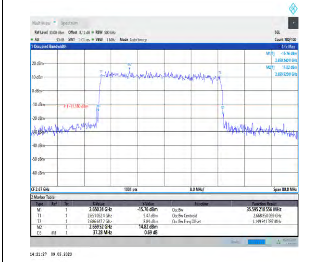
1-N41-PC3-30-40-H-3-DFT-16QAM-Outer_Full-100@0-Ant1-35.595-37.280-≤40-PASS
