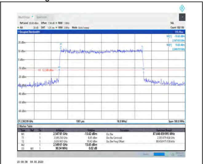
1-N41-PC3-30-90-M-6-CP-QPSK-Outer_Full-245@0-Ant1-87.646-90.540-≤90-PASS
