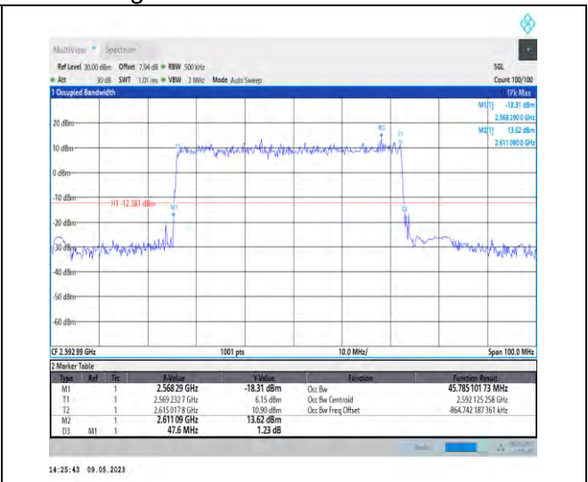
1-N41-PC3-30-50-M-4-DFT-64QAM-Outer_Full-128 @0-Ant1-45.785-47.600-≤50-PASS
