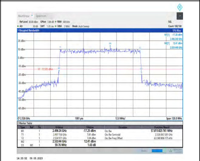
1-N41-PC3-30-60-L-4-DFT-64QAM-Outer_Full-162@0-Ant1-57.816-59.760-≤60-PASS
