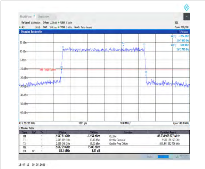
1-N41-PC3-30-90-M-1-DFT-QPSK-Outer_Full-240@0-Ant1-85.739-89.100-≤90-PASS
