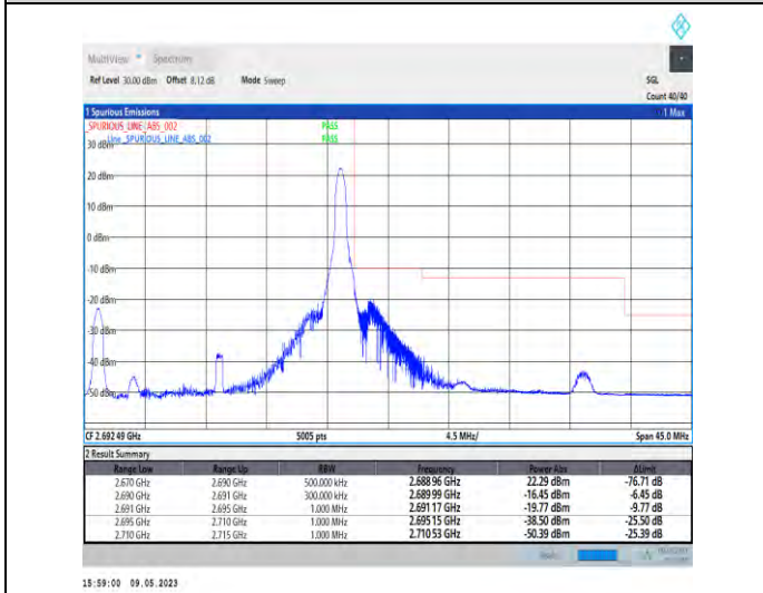
1-N41-PC3-30-20-H-5-CP-QPSK-Edge_1RB_Right-1@50-Ant1-1--PASS-see graph
