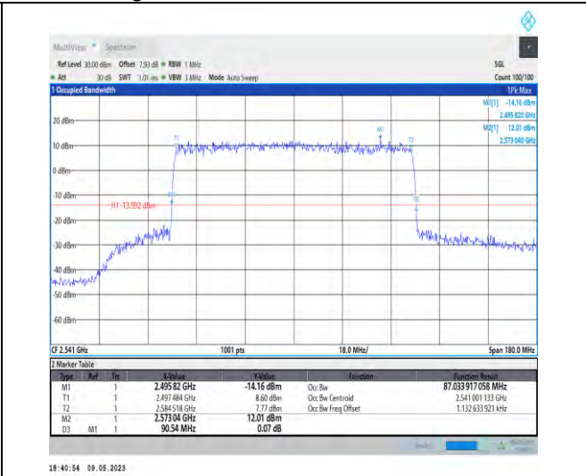
1-N41-PC3-30-90-L-7-CP-16QAM-Outer_Full-245@0-Ant1-87.034-90.540-≤90-PASS
