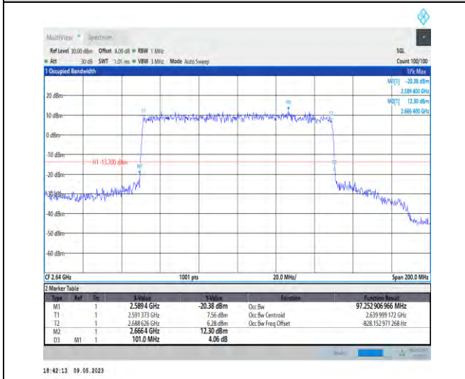
1-N41-PC3-30-100-H-7-CP-16QAM-Outer_Full-273 @0-Ant1-97.253-101.000-≤100-PASS
