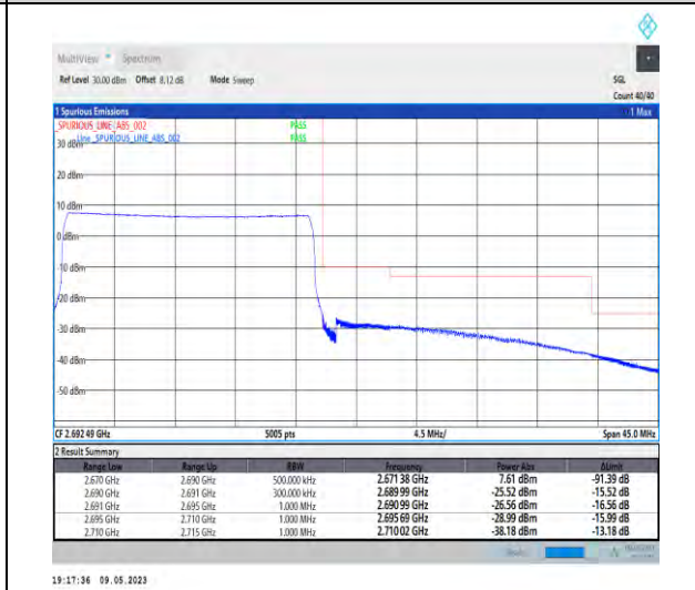
1-N41-PC3-30-20-H-6-CP-QPSK-Outer_Full-51@0-Ant1-1--PASS-see graph
