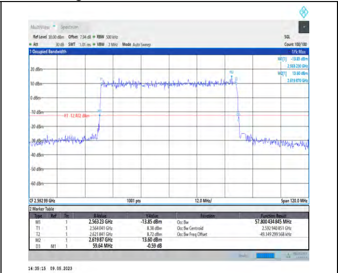
1-N41-PC3-30-60-M-1-DFT-QPSK-Outer_Full-162 @0-Ant1-57.8-59.640-≤60-PASS
