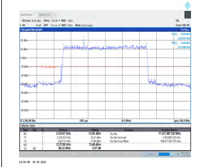
1-N41-PC3-30-80-M-2-DFT-PI2BPSK-Outer_Full-216 @0-Ant1-77.257-80.320-≤80-PASS
