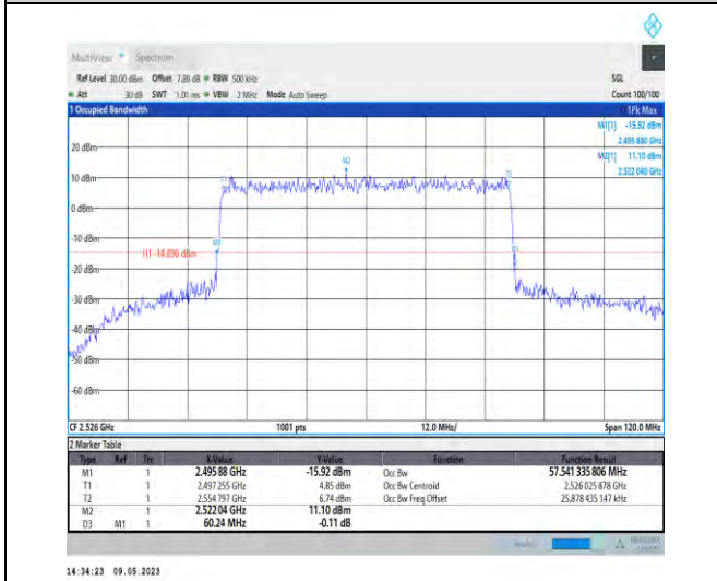
1-N41-PC3-30-60-L-7-CP-16QAM-Outer_Full-162@0-Ant1-57.541-60.240-≤60-PASS
