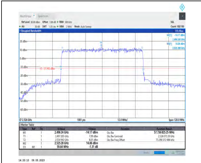
1-N41-PC3-30-60-L-1-DFT-QPSK-Outer_Full-162@0-Ant1-57.737-59.640-≤60-PASS
