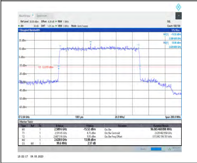
1-N41-PC3-30-100-H-3-DFT-16QAM-Outer_Full-270 @0-Ant1-96.065-99.600-≤100-PASS
