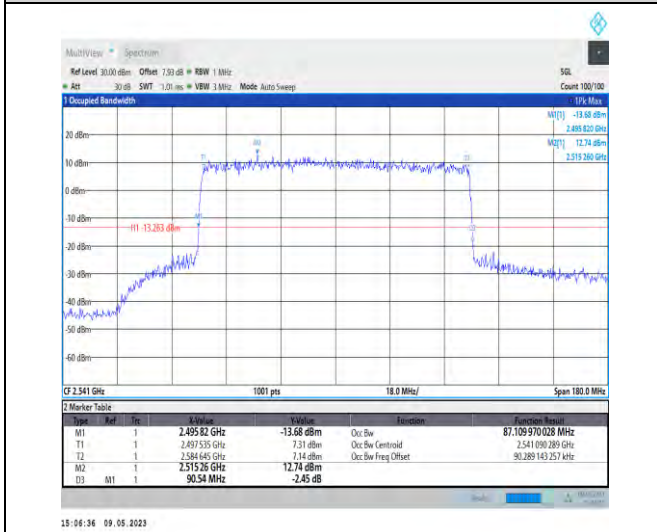
1-N41-PC3-30-90-L-8-CP-64QAM-Outer_Full-245@0-Ant1-87.11-90.540-≤90-PASS
