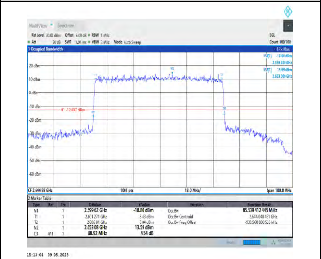
1-N41-PC3-30-90-H-3-DFT-16QAM-Outer_Full-240 @0-Ant1-85.539-88.920-≤90-PASS
