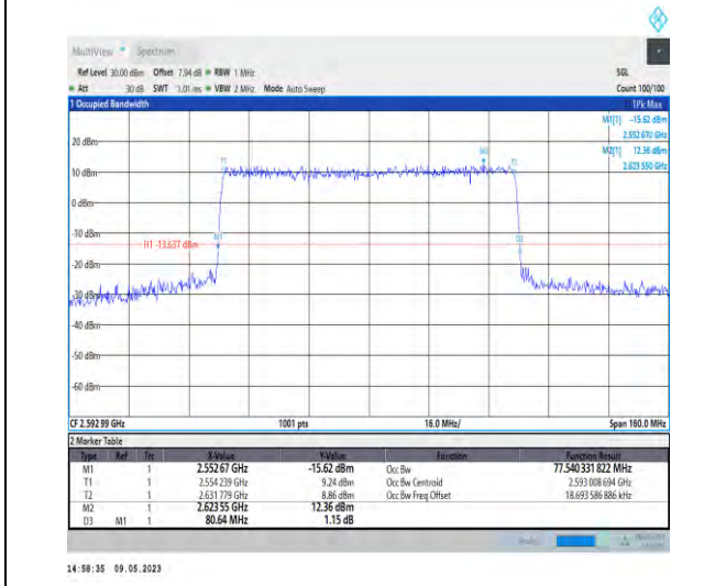
1-N41-PC3-30-80-M-6-CP-QPSK-Outer_Full-217@0 -Ant1-77.54-80.640-≤80-PASS
