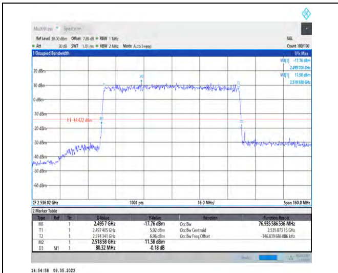
1-N41-PC3-30-80-L-5-DFT-256QAM-Outer_Full-216 @0-Ant1-76.936-80.320-≤80-PASS
