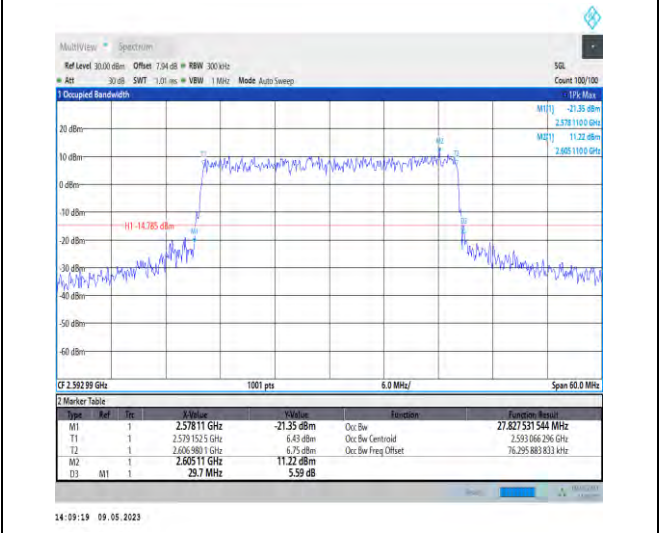
1-N41-PC3-30-30-M-8-CP-64QAM-Outer_Full-78@0-Ant1-27.828-29.700-≤30-PASS
