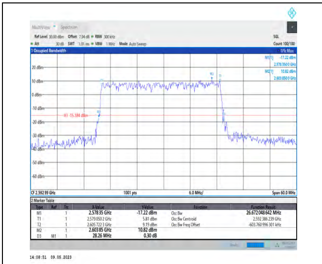
1-N41-PC3-30-30-M-5-DFT-256QAM-Outer_Full-75@0-Ant1-26.672-28.260-≤30-PASS
