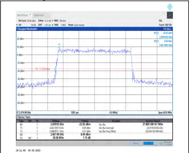
1-N41-PC3-30-30-H-9-CP-256QAM-Outer_Full-78@0-Ant1-27.809-29.580-≤30-PASS
