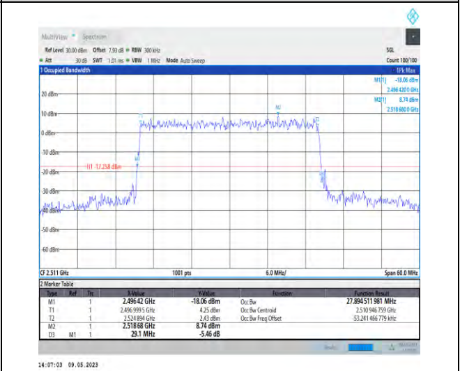
1-N41-PC3-30-30-L-9-CP-256QAM-Outer_Full-78@0-A Ant1-27.895-29.100-≤30-PASS
