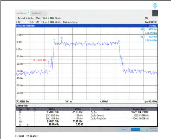
1-N41-PC3-30-20-M-6-CP-QPSK-Outer_Full-51@0-Ant1-18.291-19.880-<=20-PASS
