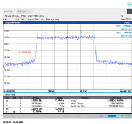
1-N41-PC3-30-40-L-4-DFT-64QAM-Outer_Full-100 @0-Ant1-35.668-37.680-≤40-PASS
