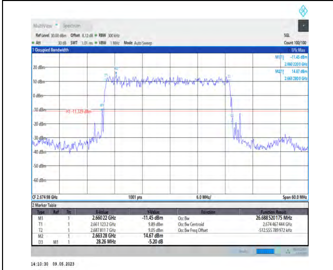
1-N41-PC3-30-30-H-2-DFT-PI2BPSK-Outer_Full-75 @0-Ant1-26.689-28.260-≤30-PASS
