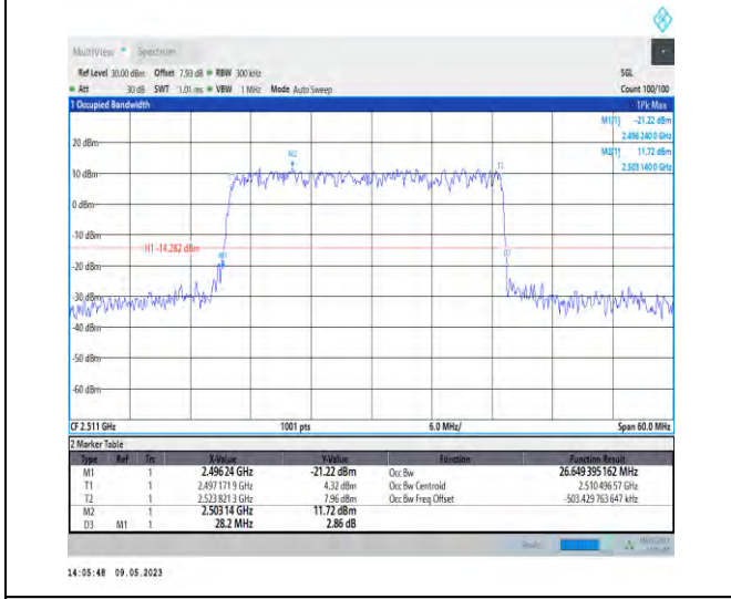
1-N41-PC3-30-30-L-4-DFT-64QAM-Outer_Full-75 @0-Ant1-26.649-28.200-≤30-PASS
