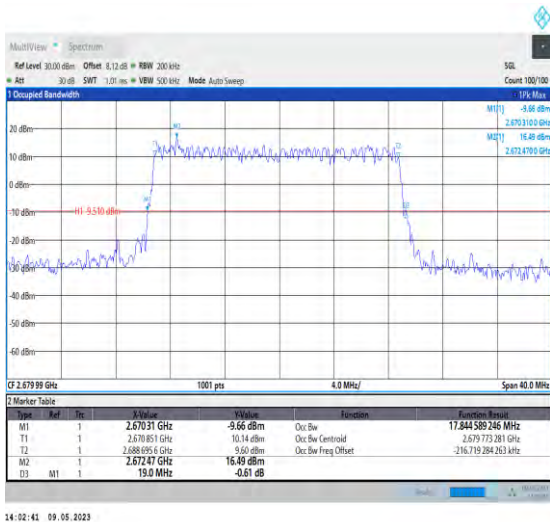
1-N41-PC3-30-20-H-1-DFT-QPSK-Outer_Full-50@0- Ant1-17.845-19.000-≤20-PASS
