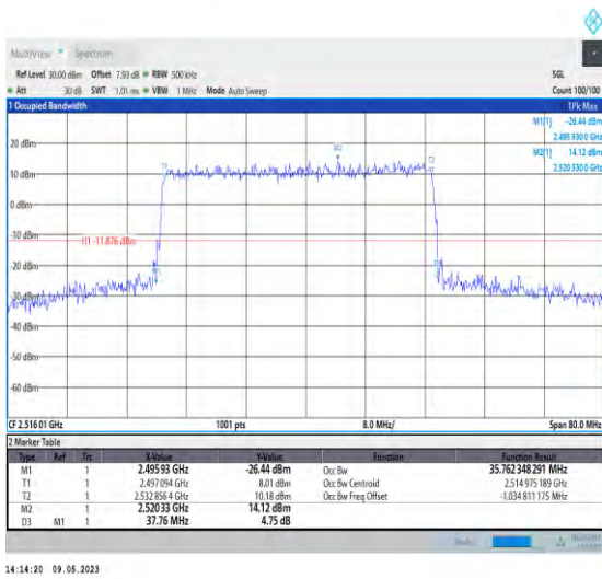
1-N41-PC3-30-40-L-3-DFT-16QAM-Outer_Full-100 @0-Ant1-35.762-37.760-≤40-PASS
