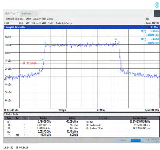
1-N41-PC3-30-40-L-6-CP-QPSK-Outer_Full-106@0-Ant1-37.815-40.240-≤40-PASS
