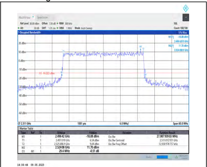
1-N41-PC3-30-30-L-7-CP-16QAM-Outer_Full-78@0-A Ant1-27.988-29.400-≤30-PASS
