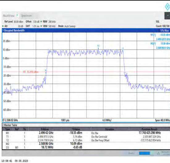
1-N41-PC3-30-20-L-5-DFT-256QAM-Outer_Full-50 @0-Ant1-17.743-18.720-≤20-PASS
