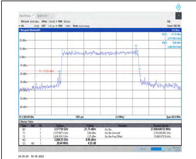
1-N41-PC3-30-30-M-9-CP-256QAM-Outer_Full-78@ 0-Ant1-27.837-29.640-≤30-PASS
