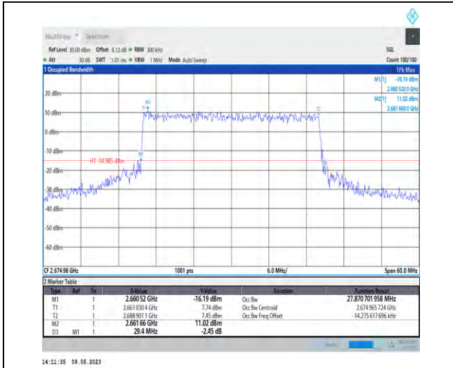
1-N41-PC3-30-30-H-8-CP-64QAM-Outer_Full-78@0 -Ant1-27.871-29.400-≤30-PASS
