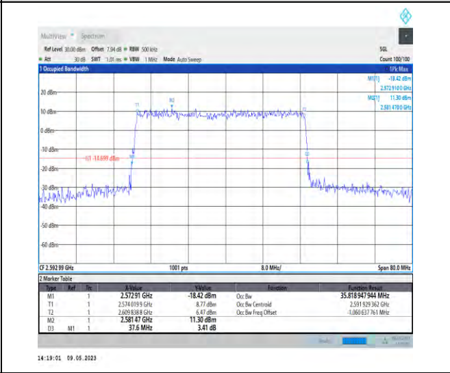
1-N41-PC3-30-40-M-5-DFT-256QAM-Outer_Full-100@0-Ant1-35.819-37.600-≤40-PASS
