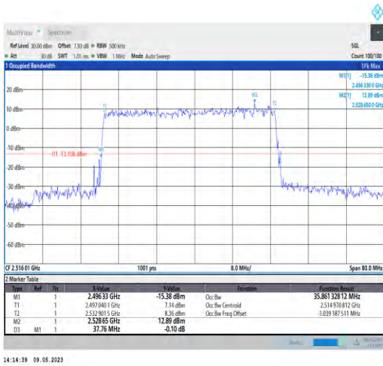
1-N41-PC3-30-40-L-5-DFT-256QAM-Outer_Full-100 @0-Ant1-35.861-37.760-≤40-PASS
