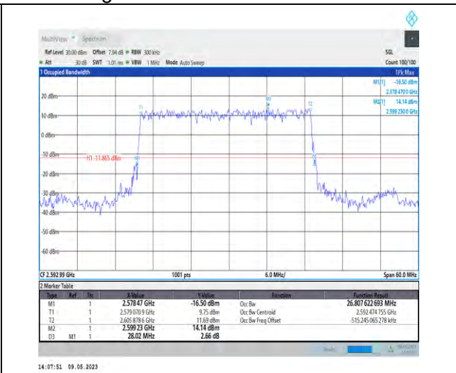
1-N41-PC3-30-30-M-2-DFT-PI2BPSK-Outer_Full-75@0 @0-Ant1-26.808-28.020-≤30-PASS
