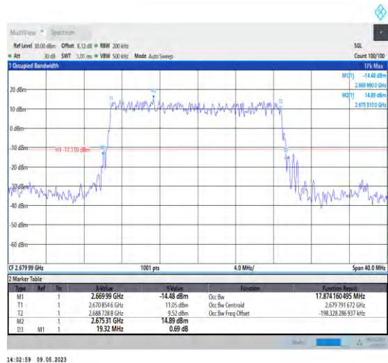
1-N41-PC3-30-20-H-2-DFT-PI2BPSK-Outer_Full-50@0- Ant1-17.874-19.320-≤20-PASS
