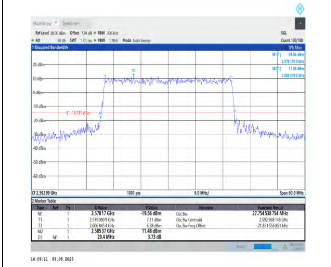
1-N41-PC3-30-30-M-7-CP-16QAM-Outer_Full-78@0-Ant1-27.755-29.400-≤30-PASS
