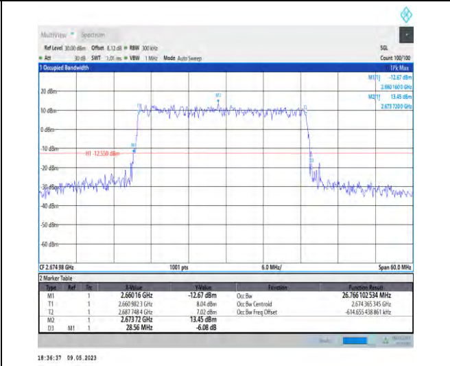
1-N41-PC3-30-30-H-3-DFT-16QAM-Outer_Full-75@ 0-Ant1-26.766-28.560-≤30-PASS
