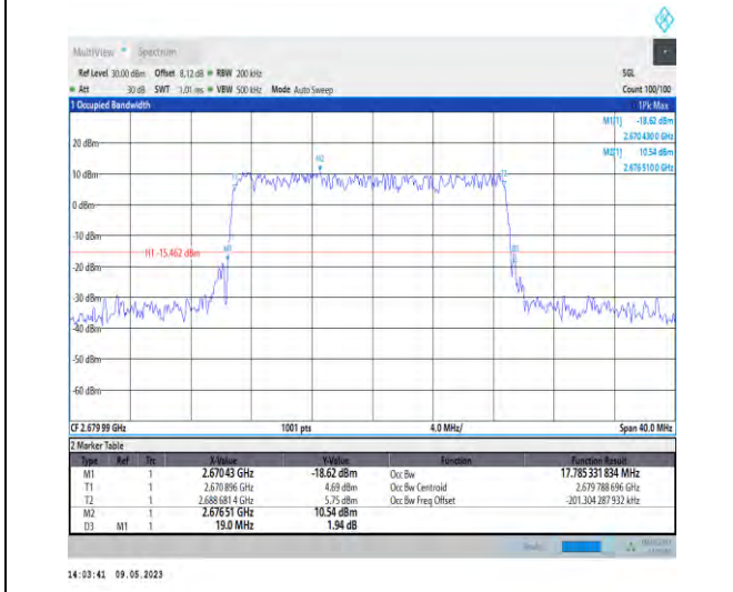
1-N41-PC3-30-20-H-5-DFT-256QAM-Outer_Full-50@0-Ant1-17.785-19.000-≤20-PASS
