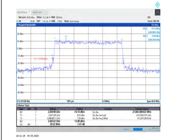
1-N41-PC3-30-30-H-6-CP-QPSK-Outer_Full-78@0-Ant1-27.843-29.520-≤30-PASS
