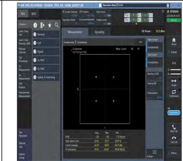
1-N41-PC3-30-100-M-2-DFT-QPSK-Outer_Full-270 @0-Ant1-see graph-PASS
