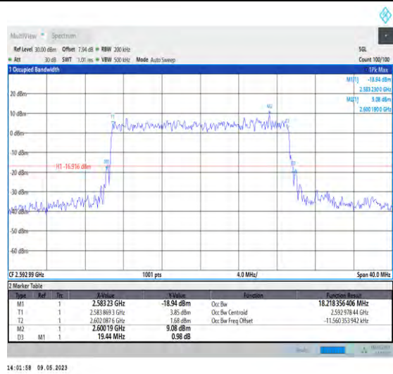
1-N41-PC3-30-20-M-9-CP-256QAM-Outer_Full-51@0 -Ant1-18.218-19.440-≤20-PASS
