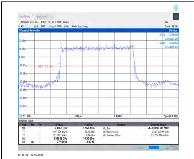
1-N41-PC3-30-30-L-2-DFT-PI2BPSK-Outer_Full-75 @0-Ant1-26.781-27.900-≤30-PASS
