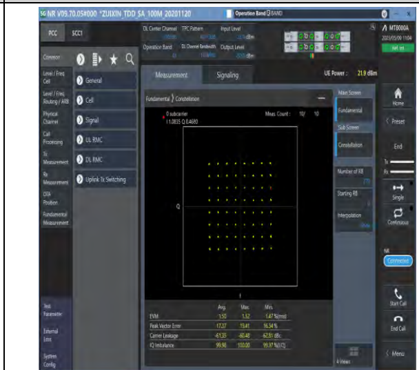
1-N41-PC3-30-100-M-4-DFT-64QAM-Outer_Full-27 @0-Ant1-see graph-PASS
