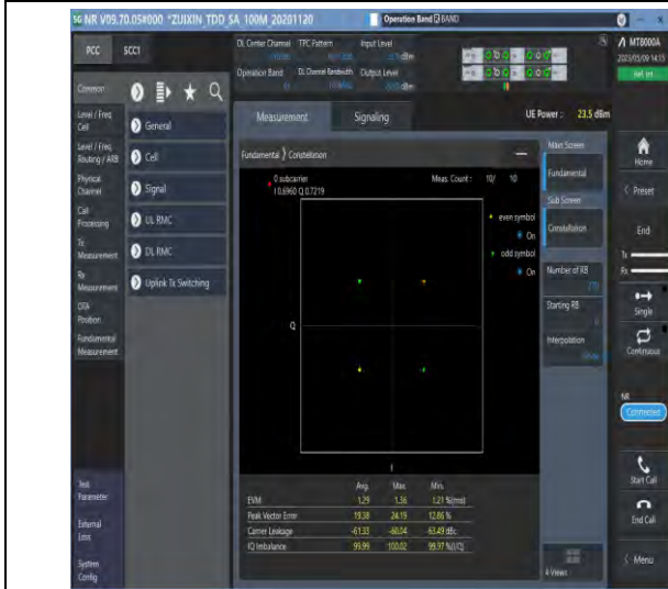
1-N41-PC3-30-100-M-1-DFT-PI2BPSK-Outer_Full-27 @0-Ant1-see graph-PASS
