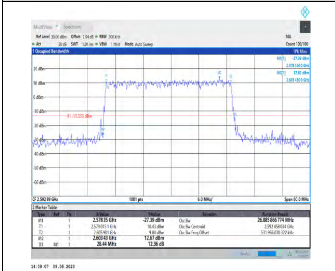
1-N41-PC3-30-30-M-3-DFT-16QAM-Outer_Full-75@0 0-Ant1-26.886-28.440-≤30-PASS
