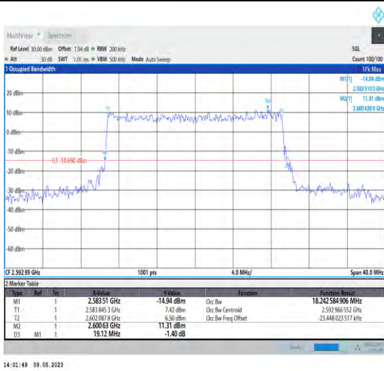
1-N41-PC3-30-20-M-8-CP-64QAM-Outer_Full-51@0 -Ant1-18.243-19.120-≤20-PASS
