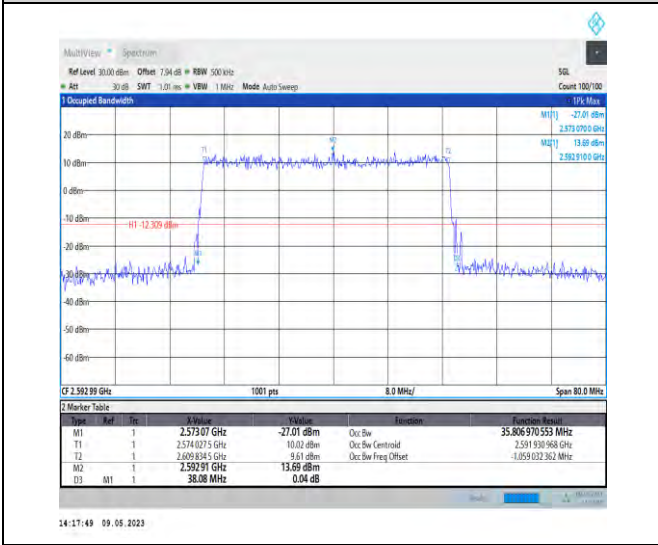
1-N41-PC3-30-40-M-4-DFT-64QAM-Outer_Full-100@0-Ant1-35.807-38.080-≤40-PASS
