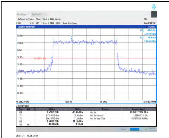
1-N41-PC3-30-30-M-1-DFT-QPSK-Outer_Full-75@0 -Ant1-26.858-28.080-≤30-PASS
