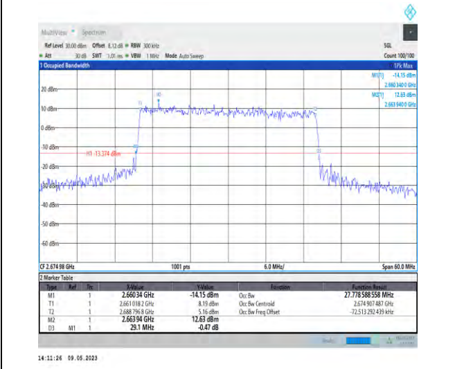
1-N41-PC3-30-30-H-7-CP-16QAM-Outer_Full-78@0-Ant1-27.779-29.100-≤30-PASS
