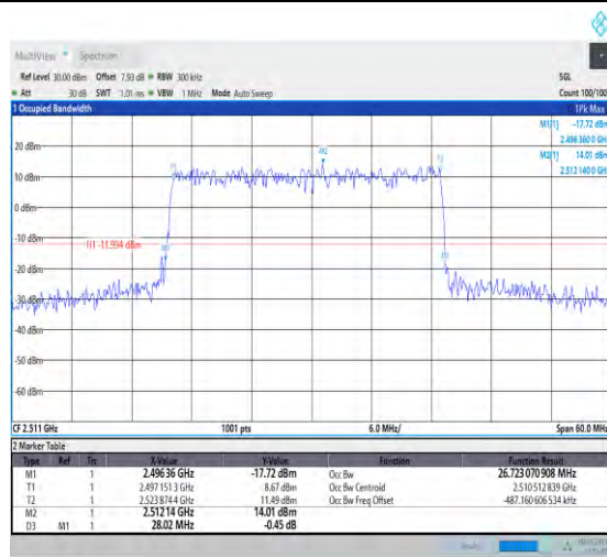
1-N41-PC3-30-20-H-8-CP-64QAM-Outer_Full-51@0 -Ant1-18.213-19.280-≤20-PASS
