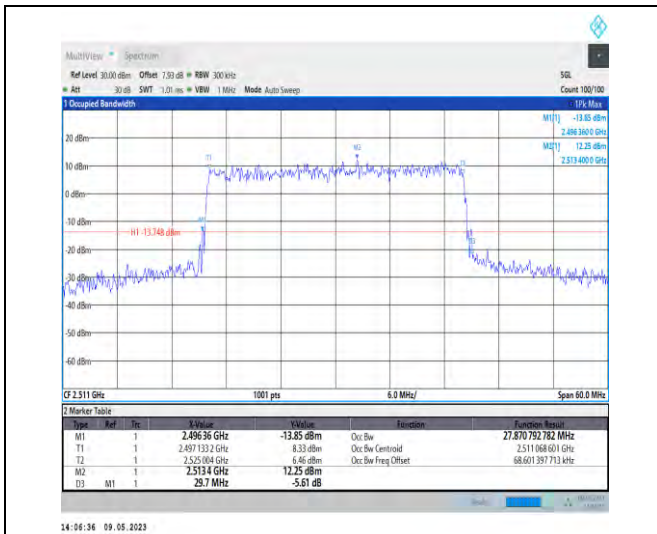
1-N41-PC3-30-30-L-6-CP-QPSK-Outer_Full-78@0-A Ant1-27.871-29.700-≤30-PASS
