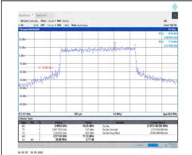
1-N41-PC3-30-30-L-8-CP-64QAM-Outer_Full-78@0-A Ant1-27.815-28.980-≤30-PASS
