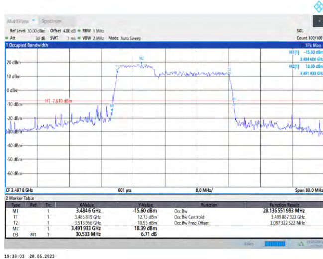
42-42-10MHz-20MHz-QPSK-QPSK-42496-42640-50RB#0-100RB#0
