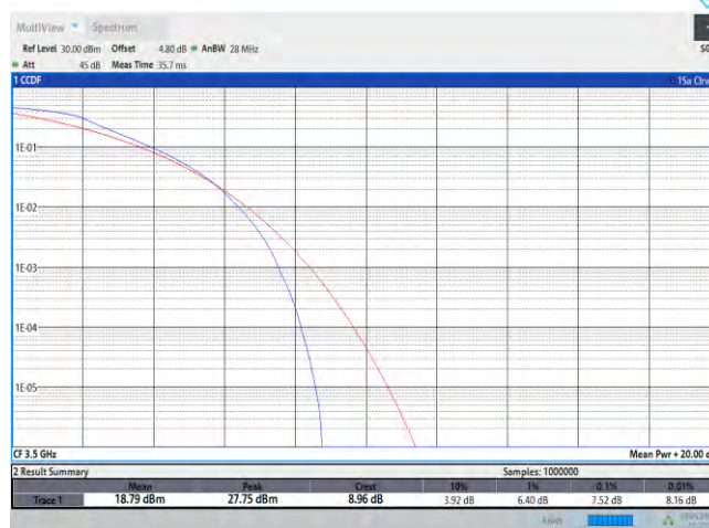
Band42-20MHz-QPSK-42590-100RB#0
