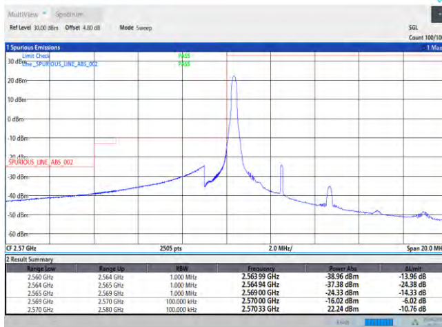
Band38-5MHz-QPSK-37775-25RB#0
