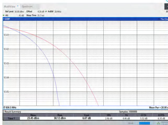
Band26-15MHz-QPSK-26915-75RB#0
