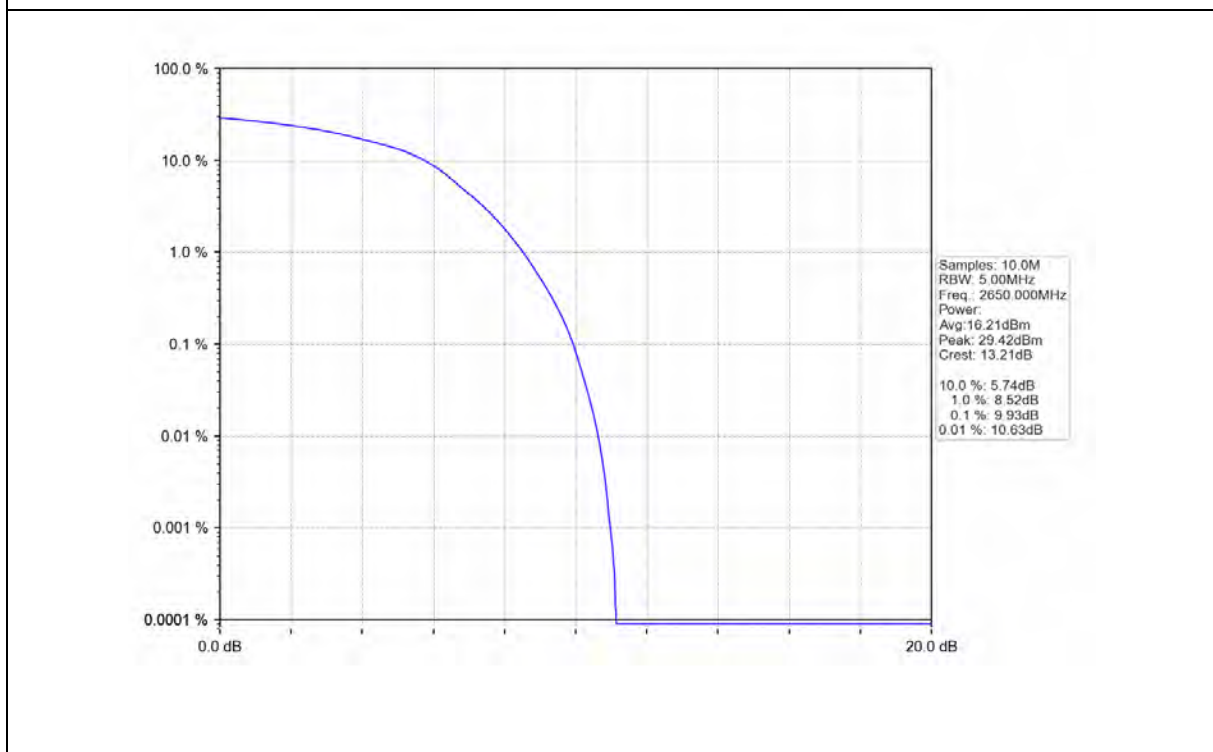
Band41_10MHz_16QAM_HCH_2650MHz_RB_50_0_NTNV
