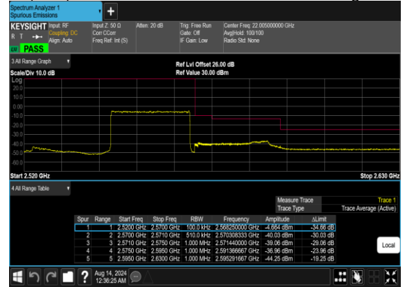
N7(25M)_DFT-s-OFDM_QPSK_Outer_Full_High_CH
