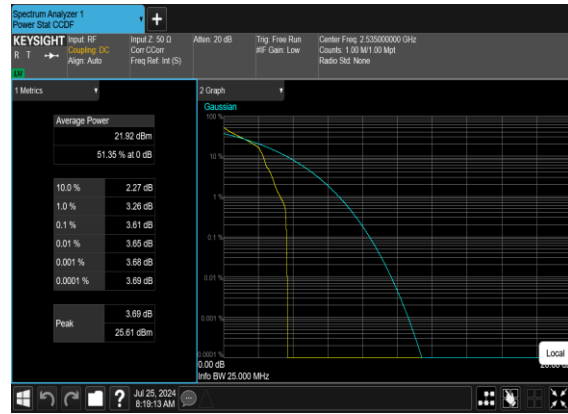
N7(20M)_DFT-s-OFDM_PI_2-BPSK_Edge_1RB_Left_Mid_CH
