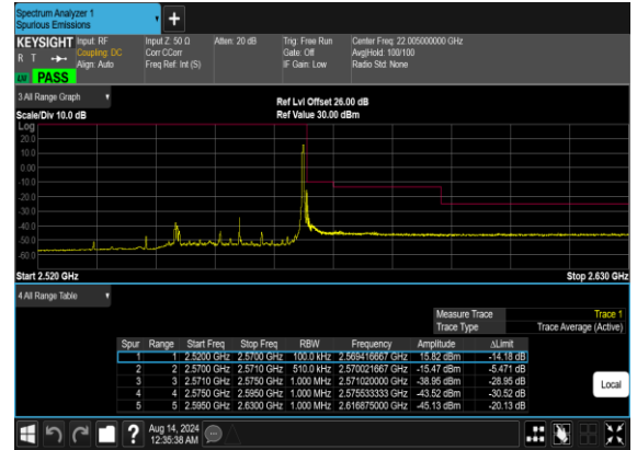
N7(25M)_DFT-s-OFDM_QPSK_Edge_1RB_Right_High_CH
