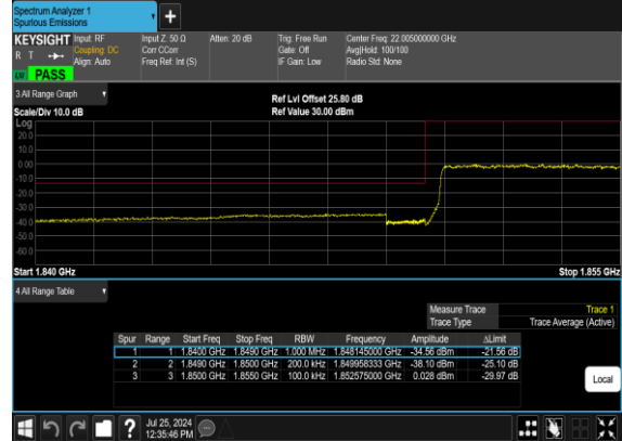
N2(20M)_DFT-s-OFDM_QPSK_Outer_Full_Low_CH
