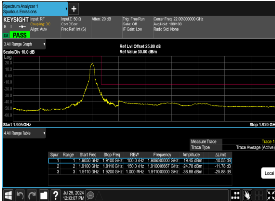
N2(15M)_DFT-s-OFDM_BPSK_Edge_1RB_Right_High_CH
