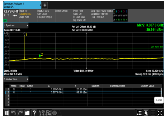
N2(5M)_DFT-s-OFDM_QPSK_Edge_1RB_Left_High_CH
