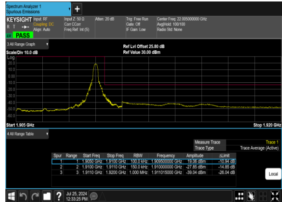
N2(15M)_DFT-s-OFDM_QPSK_Edge_1RB_Right_High_CH
