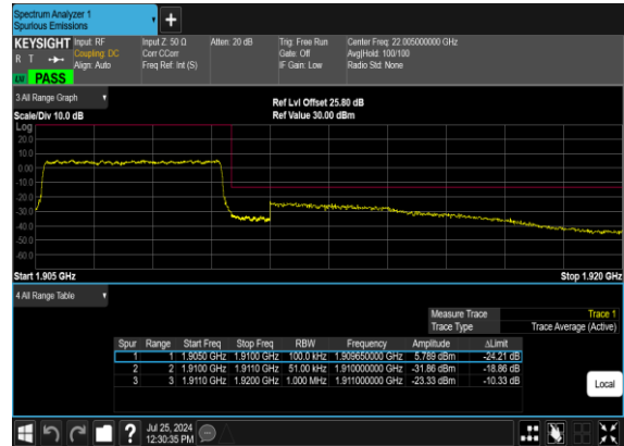
N2(5M)_DFT-s-OFDM_QPSK_Outer_Full_High_CH
