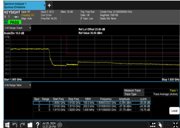
N2(20M)_DFT-s-OFDM_QPSK_Outer_Full_High_CH
