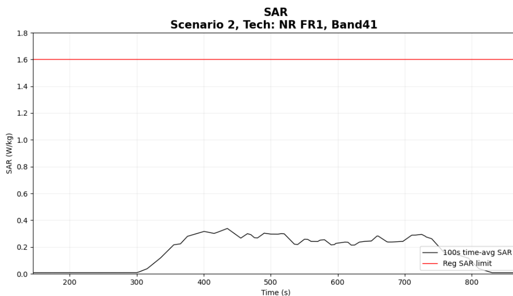
Figure 5- 32 Time-averaged SAR
