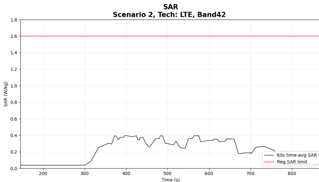
Figure 5- 28 Time-averaged SAR
