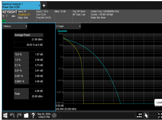
N48(20M)_DFT-s-OFDM_PI_2- BPSK_Outer_Full_Mid_CH
