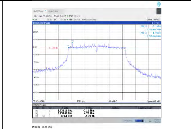
11ac20MIMO-Ant12-5745
