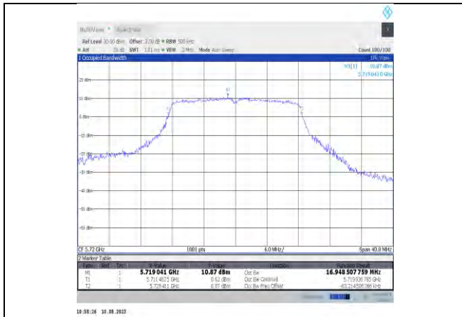
11a-CDD-Ant11-5720
