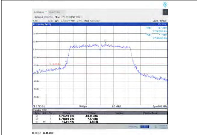
11ac40MIMO-Ant11-5755
