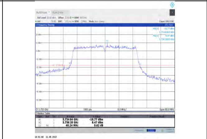
11ac40MIMO-Ant12-5755
