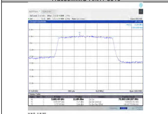
11ac80MIMO-Ant11-5690
