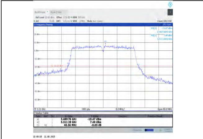
11ac40MIMO-Ant11-5510
