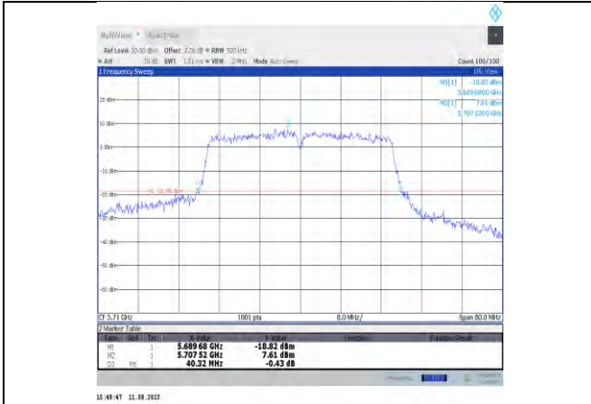
11ac40MIMO-Ant11-5710
