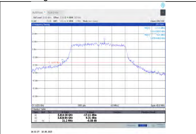
11a-CDD-Ant12-5825
