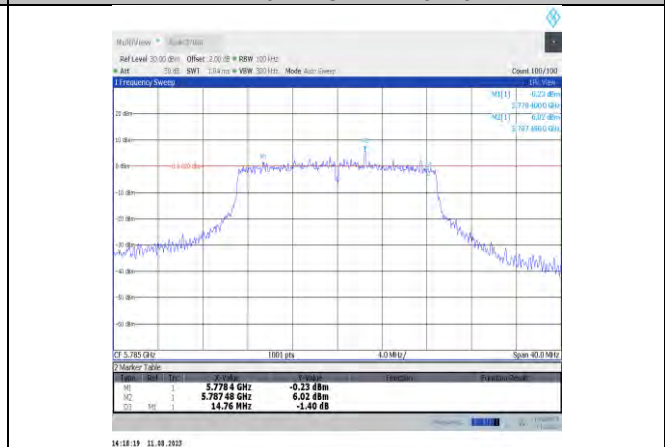
11ac20MIMO-Ant12-5785
