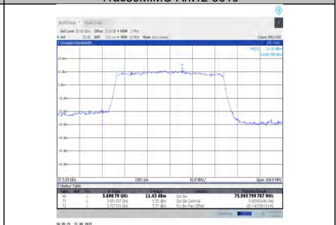
11ac80MIMO-Ant12-5690
