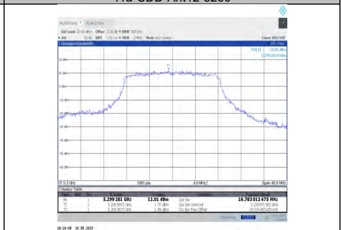
11a-CDD-Ant12-5300
