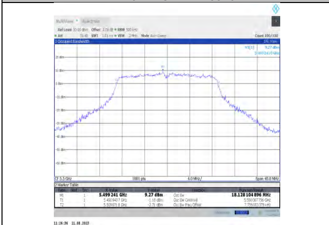
11ac20MIMO-Ant11-5500
