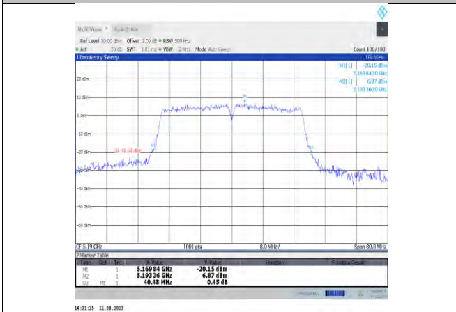
11ac40MIMO-Ant11-5190
