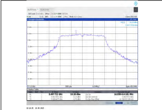
11a-CDD-Ant11-5500
