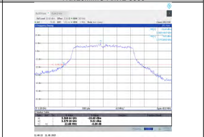
11ac20MIMO-Ant12-5580
