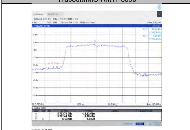
11ac80MIMO-Ant11-5775
