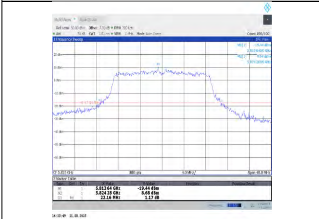
11ac20MIMO-Ant11-5825
