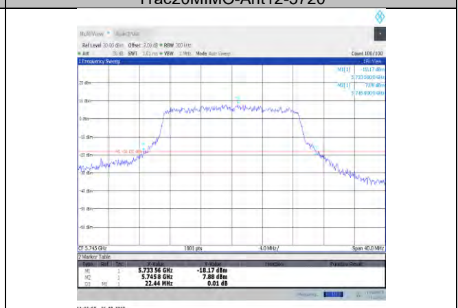
11ac20MIMO-Ant12-5745
