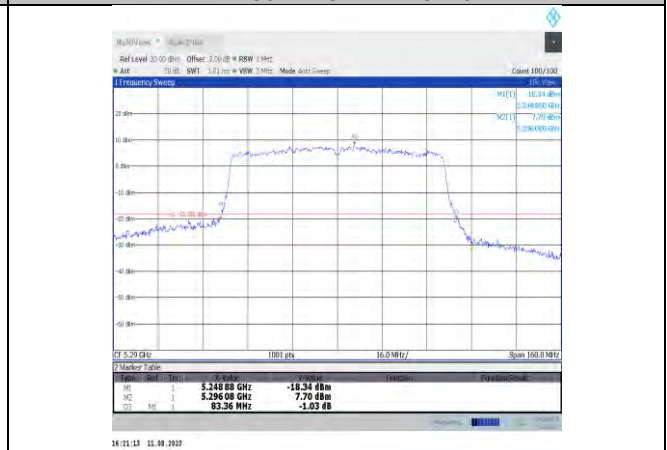
11ac80MIMO-Ant12-5290
