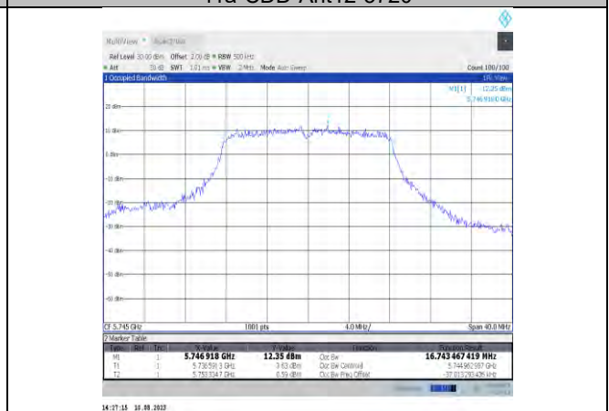
11a-CDD-Ant12-5745
