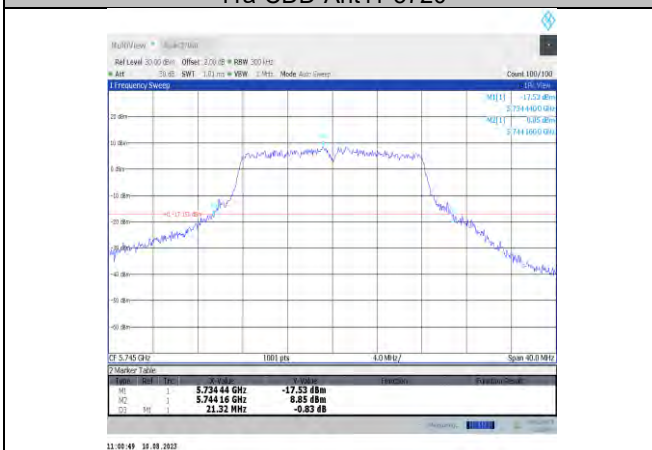
11a-CDD-Ant11-5745
