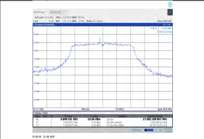
11ac20MIMO-Ant12-5700
