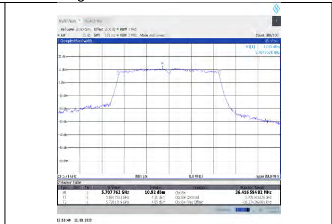
11ac40MIMO-Ant12-5710
