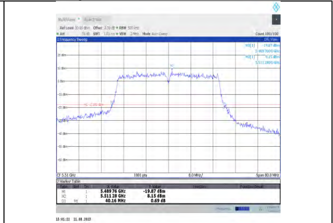
11ac40MIMO-Ant12-5510
