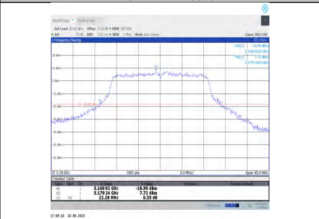
11ac20MIMO-Ant12-5180
