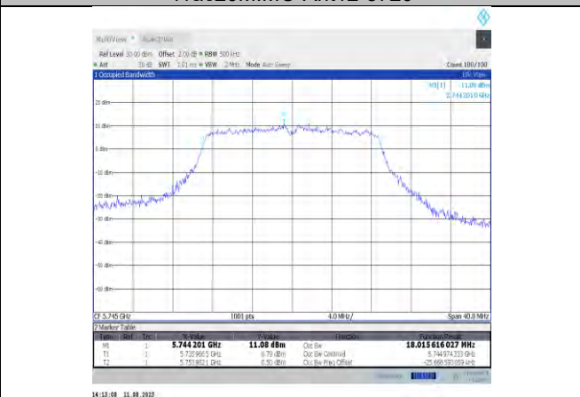
11ac20MIMO-Ant12-5745
