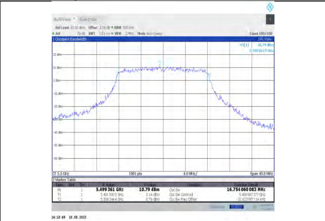
11a-CDD-Ant12-5500
