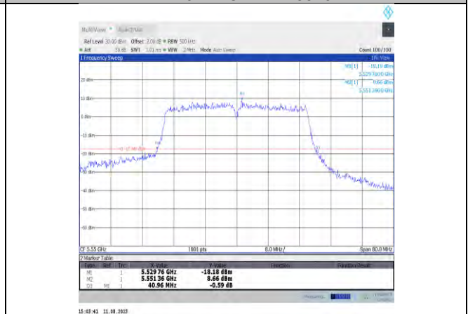
11ac40MIMO-Ant12-5550
