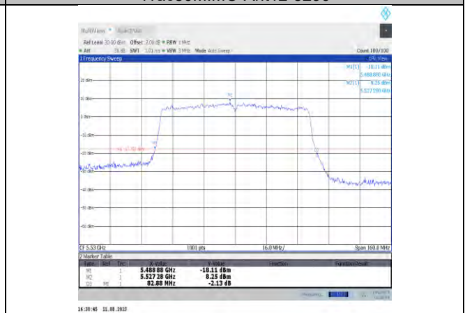
11ac80MIMO-Ant12-5530
