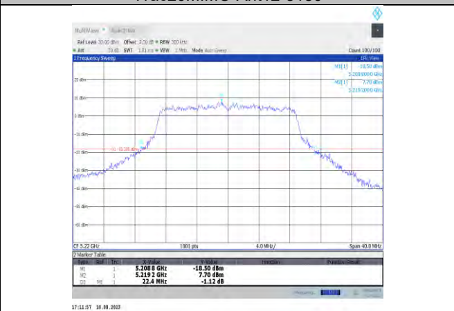
11ac20MIMO-Ant12-5220
