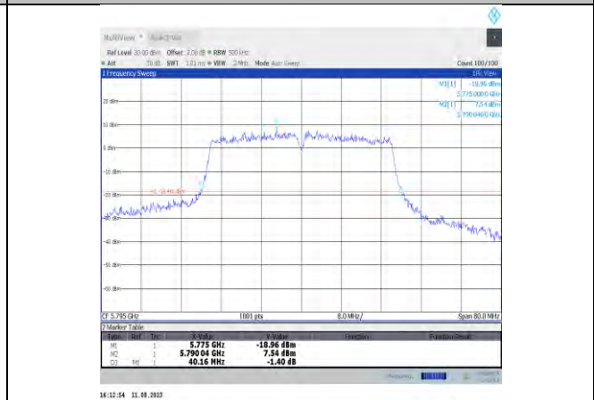
11ac40MIMO-Ant12-5795
