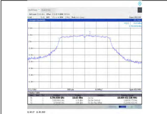
11ac20MIMO-Ant11-5700
