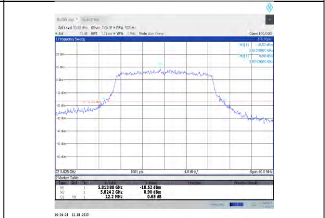
11ac20MIMO-Ant12-5825
