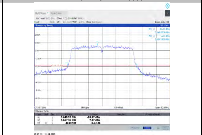
11ac40MIMO-Ant12-5670
