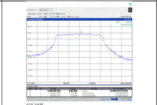
11ac20MIMO-Ant12-5500
