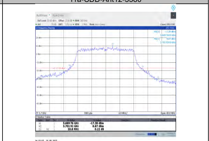
11a-CDD-Ant12-5700
