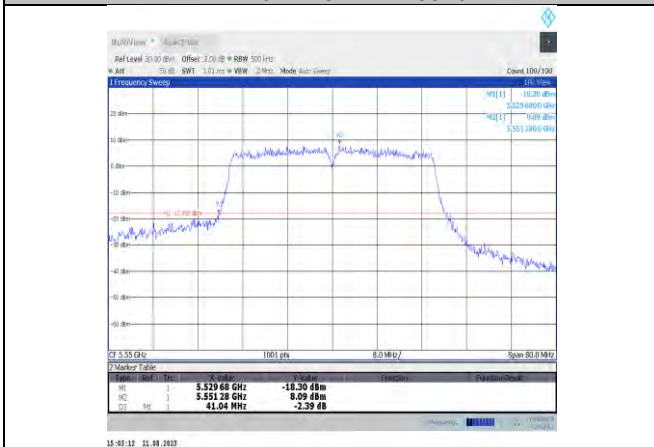
11ac40MIMO-Ant11-5550
