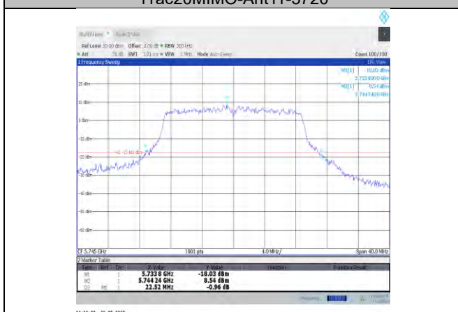
11ac20MIMO-Ant11-5745
