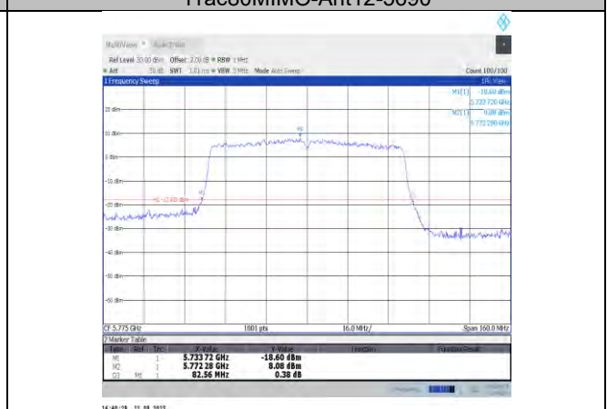
11ac80MIMO-Ant12-5775
