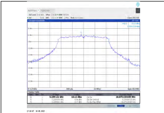
11ac20MIMO-Ant11-5240
