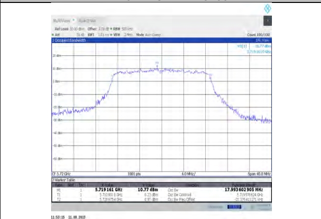
11ac20MIMO-Ant12-5720
