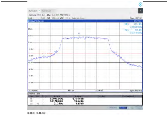
11a-CDD-Ant11-5720
