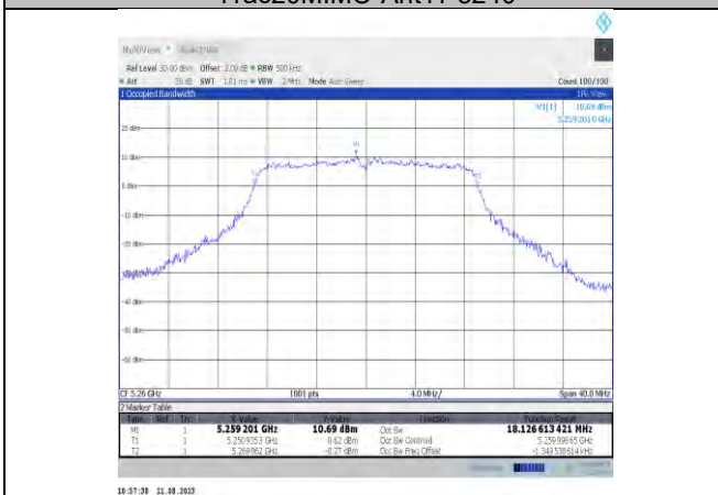
11ac20MIMO-Ant11-5260
