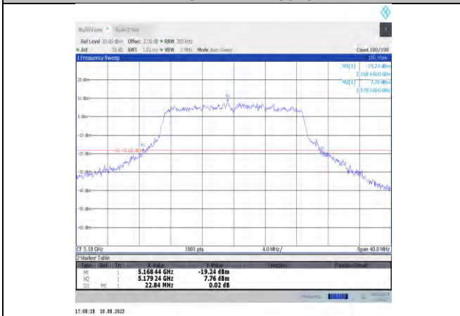
11ac20MIMO-Ant11-5180
