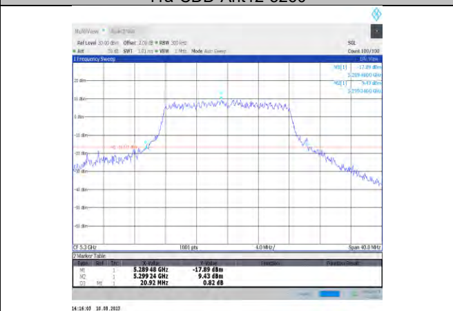
11a-CDD-Ant12-5300
