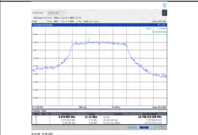
11a-CDD-Ant12-5580
