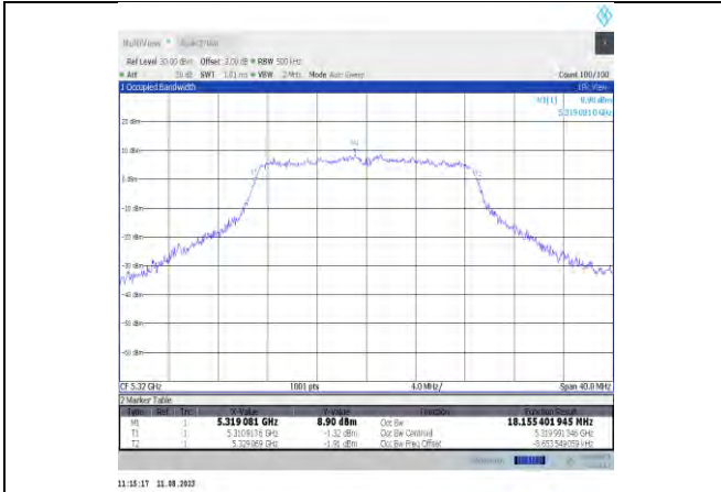
11ac20MIMO-Ant11-5320
