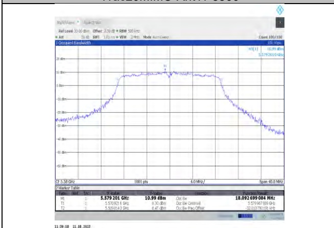
11ac20MIMO-Ant11-5580
