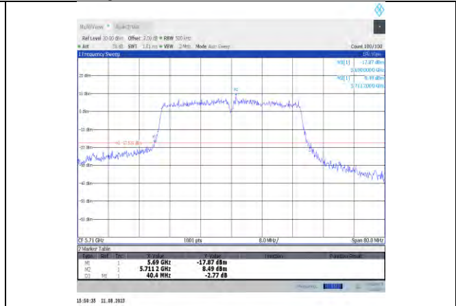
11ac40MIMO-Ant12-5710
