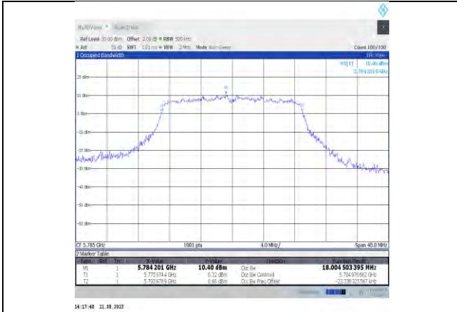
11ac20MIMO-Ant11-5785
