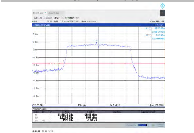
11ac80MIMO-Ant11-5530
