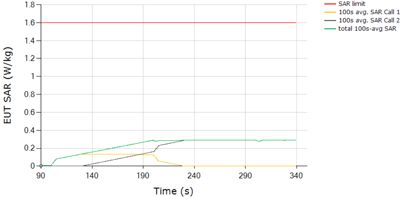
SAR Call Drop Tech: LTE, Band 41
