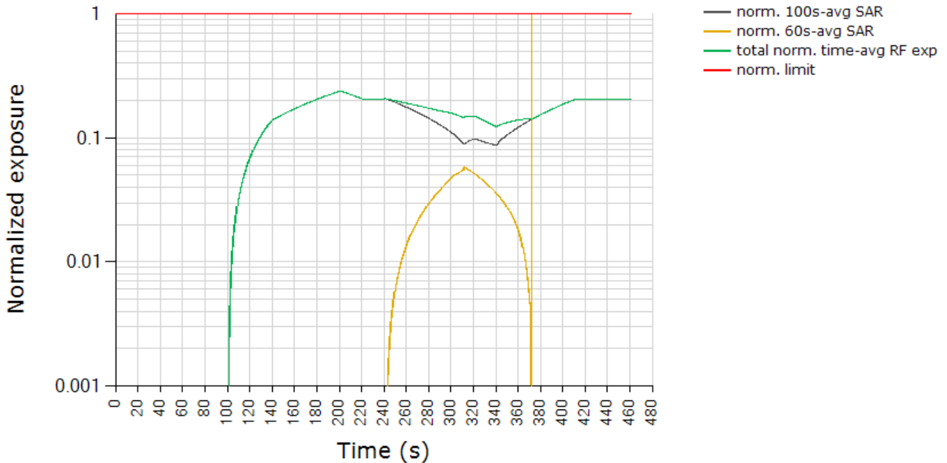
Total Normalized Time-averaged RF Exposure Tech: NR5G SUB6, Band n5 / Tech: NR5G SUB6, Band n77
