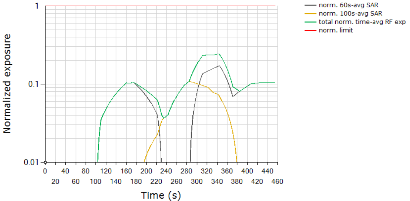
Total Normalized Time-averaged RF Exposure Tech: NR5G SUB6, Band n77 / Tech: NR5G SUB6, Band n5
