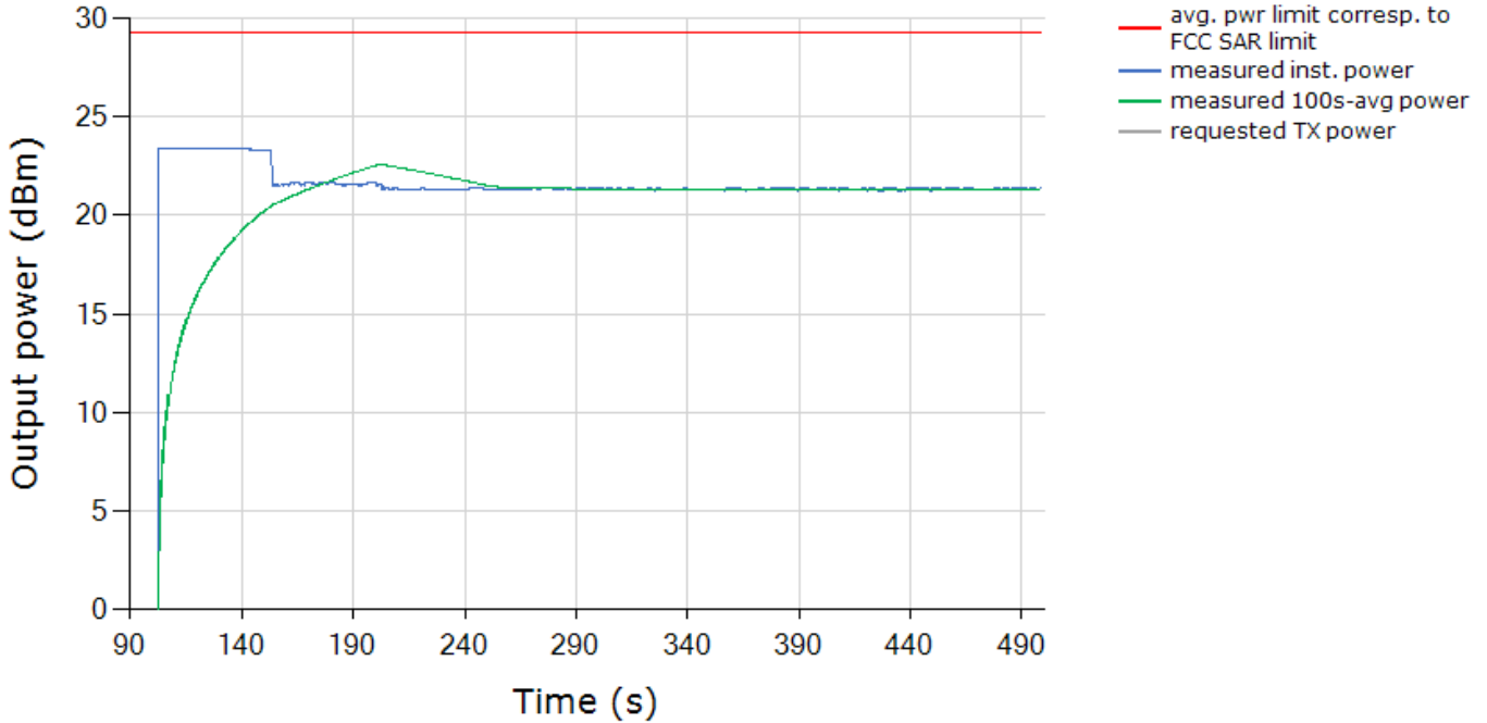
Conducted Power Tech: NR5G SUB6, Band n5
