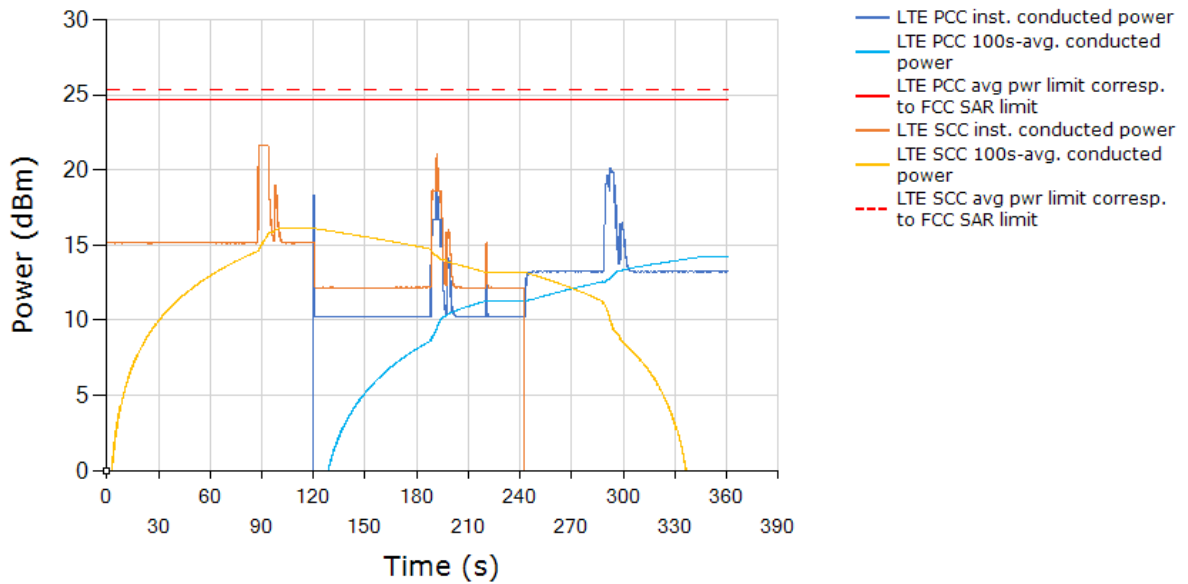
LTE PCC/SCC Instantaneous and Time-averaged TX Power Tech: LTE, Band 4 / Tech: LTE, Band 2
