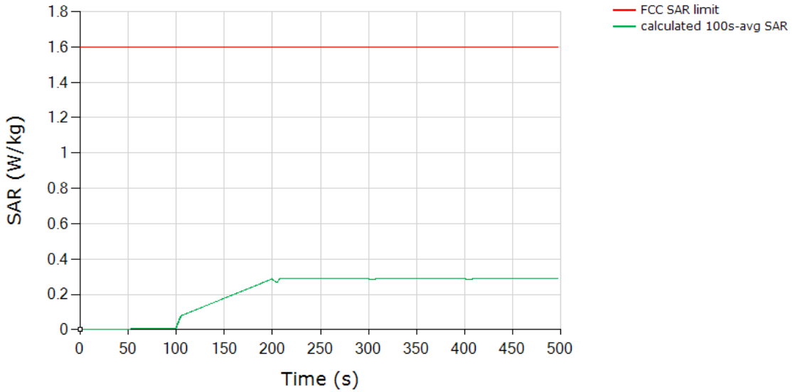
SAR Tech: LTE, Band 41
