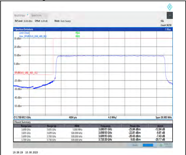
1-N78-3700-3800-PC2-30-30-L-3-DFT-PI2BPSK-Outer_Full-75@0-Ant1-1--PASS-see graph
