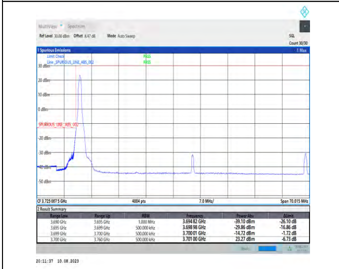
1-N78-3700-3800-PC2-30-60-L-4-CP-QPSK-Edge_1RB_Left-1@0-Ant1-1--PASS-see graph
