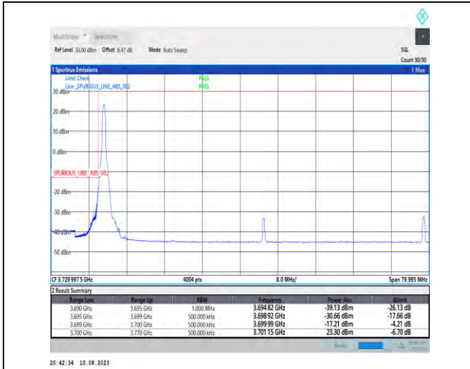
1-N78-3700-3800-PC2-30-70-L-1-DFT-PI2BPSK-Edge_1RB_Left-1@0-Ant1-1--PASS-see graph
