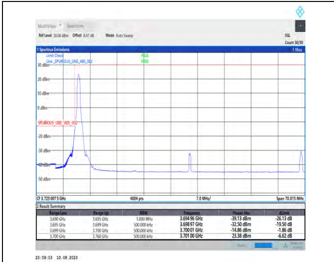
1-N78-3700-3800-PC2-30-60-L-1-DFT-PI2BPSK-Edge_1RB_Left-1@0-Ant1-1--PASS-see graph
