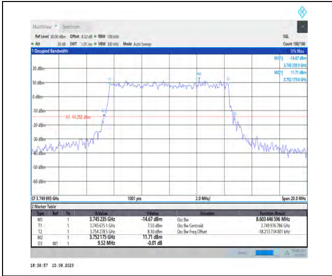
1-N78-3700-3800-PC2-30-10-M-5-DFT-256QAM-Out _Full-24@0-Ant1-8.603-9.520-≤10-PASS
