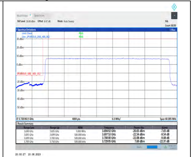
1-N78-3700-3800-PC2-30-50-L-3-DFT-PI2BPSK-Outer_Full-128@0-Ant1-1--PASS-see graph
