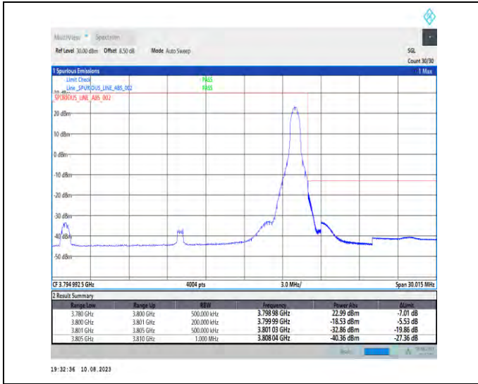
1-N78-3700-3800-PC2-30-20-H-2-DFT-PI2BPSK-Edge_1RB_Right-1@50-Ant1-1--PASS-see graph
