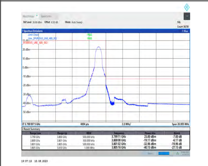
1-N78-3700-3800-PC2-30-10-H-5-CP-QPSK-Edge_1RB_Right-1@23-Ant1-1--PASS-see graph
