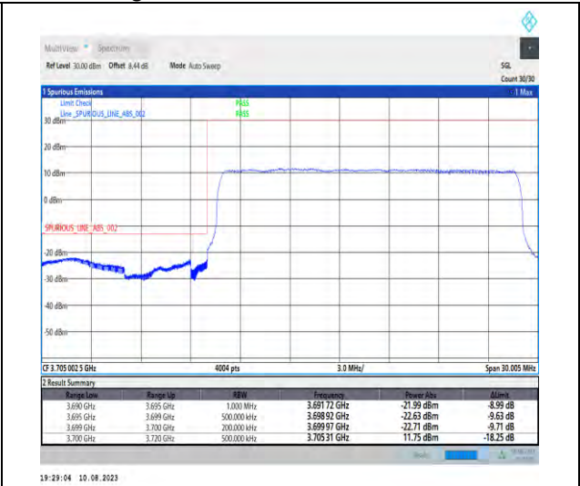
1-N78-3700-3800-PC2-30-20-L-3-DFT-PI2BPSK-Outer_Full-50@0-Ant1-1--PASS-see graph
