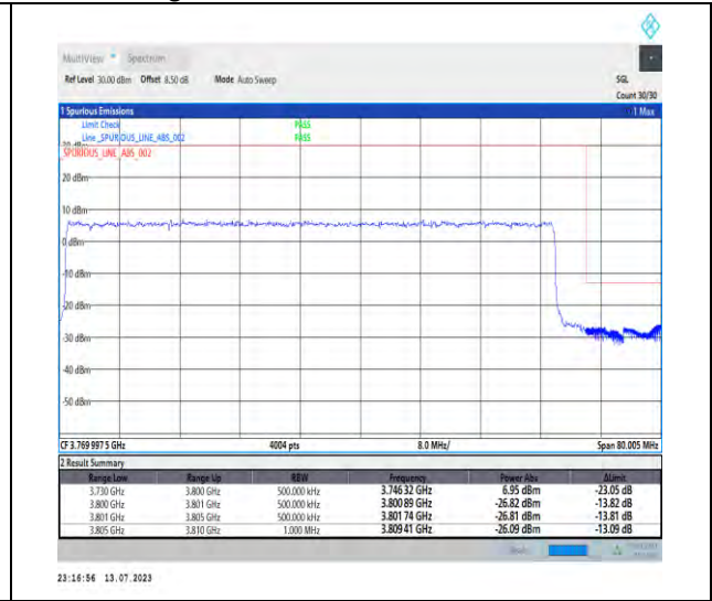
1-N78-3700-3800-PC2-30-70-H-3-DFT-PI2BPSK-Outer_Full-180@0-Ant1-1--PASS-see graph
