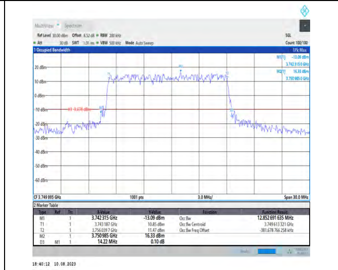
1-N78-3700-3800-PC2-30-15-M-3-DFT-16QAM-Outer _Full-36@0-Ant1-12.853-14.220-≤15-PASS
