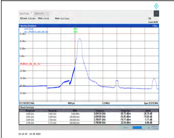
1-N78-3700-3800-PC2-30-15-L-4-CP-QPSK-Edge_1RB_Left-1@0-Ant1-1--PASS-see graph
