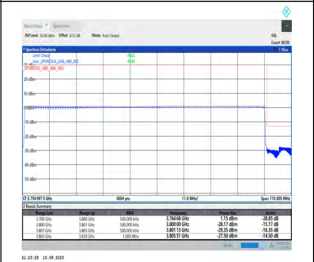
1-N78-3700-3800-PC2-30-100-H-6-CP-QPSK-Outer_Full-273@0-Ant1-1--PASS-see graph
