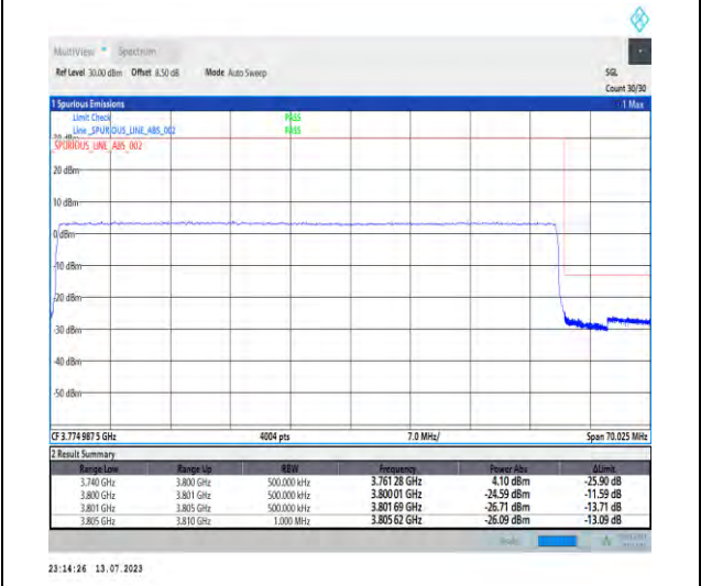
1-N78-3700-3800-PC2-30-60-H-6-CP-QPSK-Outer_Full-162@0-Ant1-1--PASS-see graph
