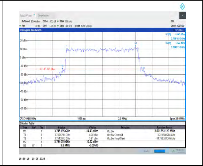
1-N78-3700-3800-PC2-30-10-M-8-CP-64QAM-Outer _Full-24@0-Ant1-8.602-9.800-≤10-PASS
