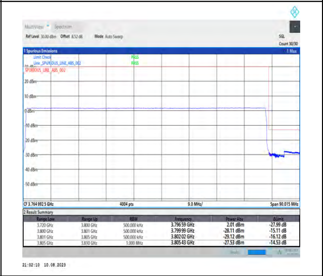
1-N78-3700-3800-PC2-30-80-H-6-CP-QPSK-Outer_Full-217@0-Ant1-1--PASS-see graph
