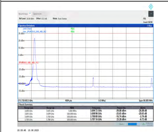
1-N78-3700-3800-PC2-30-80-L-4-CP-QPSK-Edge_1RB_Left-1@0-Ant1-1--PASS-see graph
