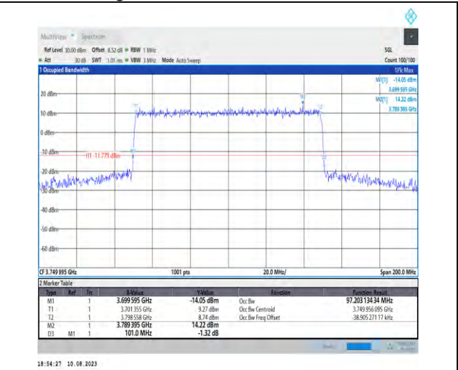
1-N78-3700-3800-PC2-30-100-M-8-CP-64QAM-Outer_Full-273@0-Ant1-97.203-101.000-≤100-PASS
