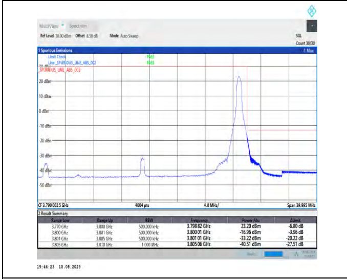
1-N78-3700-3800-PC2-30-30-H-5-CP-QPSK-Edge_1RB_Right-1@77-Ant1-1--PASS-see graph
