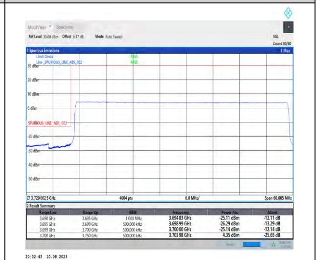
1-N78-3700-3800-PC2-30-50-L-6-CP-QPSK-Outer_Full-133@0-Ant1-1--PASS-see graph
