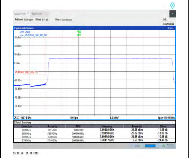
1-N78-3700-3800-PC2-30-40-L-6-CP-QPSK-Outer_Full-106@0-Ant1-1--PASS-see graph
