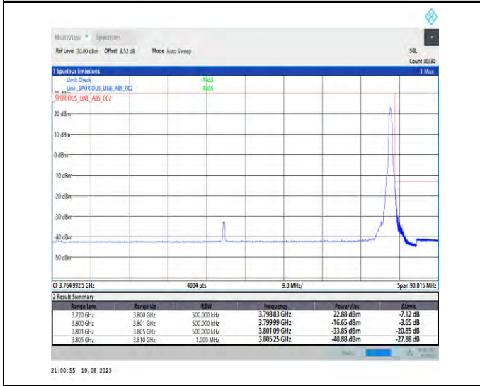
1-N78-3700-3800-PC2-30-80-H-5-CP-QPSK-Edge_1RB_Right-1@216-Ant1-1--PASS-see graph
