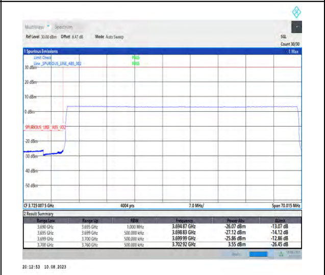
1-N78-3700-3800-PC2-30-60-L-6-CP-QPSK-Outer_Full-162@0-Ant1-1--PASS-see graph
