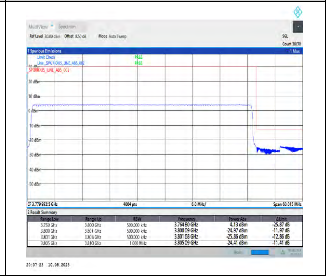
1-N78-3700-3800-PC2-30-50-H-6-CP-QPSK-Outer_Full-133@0-Ant1-1--PASS-see graph
