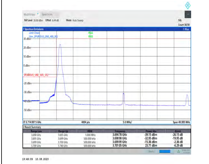
1-N78-3700-3800-PC2-30-40-L-4-CP-QPSK-Edge_1RB_Left-1@0-Ant1-1--PASS-see graph
