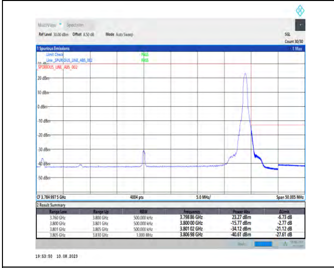
1-N78-3700-3800-PC2-30-40-H-5-CP-QPSK-Edge_1RB_Right-1@105-Ant1-1--PASS-see graph
