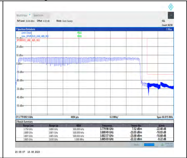
1-N78-3700-3800-PC2-30-50-H-3-DFT-PI2BPSK-Outer_Full-128@0-Ant1-1--PASS-see graph
