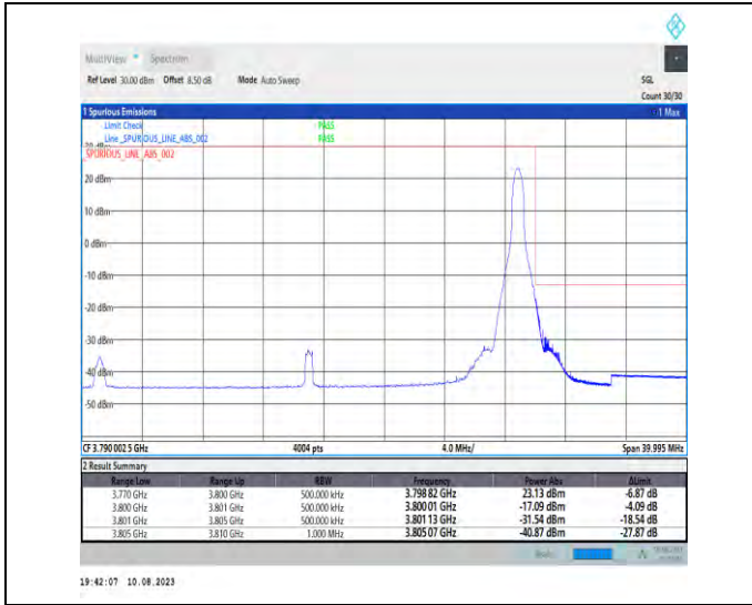
1-N78-3700-3800-PC2-30-30-H-2-DFT-PI2BPSK-Edge_1RB_Right-1@77-Ant1-1--PASS-see graph
