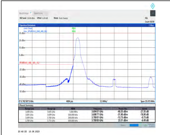
1-N78-3700-3800-PC2-30-15-L-1-DFT-PI2BPSK-Edge_1RB_Left-1@0-Ant1-1--PASS-see graph
