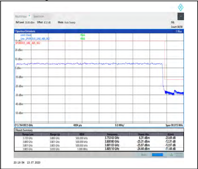
1-N78-3700-3800-PC2-30-80-H-3-DFT-PI2BPSK-Outer_Full-216@0-Ant1-1--PASS-see graph
