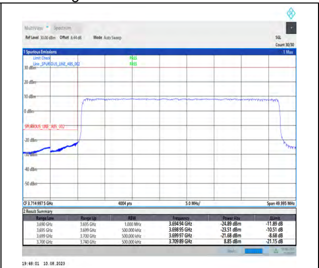
1-N78-3700-3800-PC2-30-40-L-3-DFT-PI2BPSK-Outer_Full-100@0-Ant1-1--PASS-see graph
