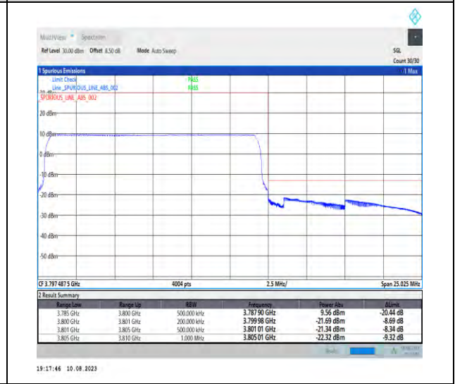
1-N78-3700-3800-PC2-30-15-H-6-CP-QPSK-Outer_Full-38@0-Ant1-1--PASS-see graph
