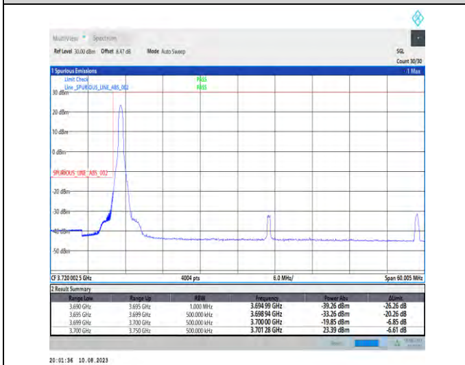
1-N78-3700-3800-PC2-30-50-L-4-CP-QPSK-Edge_1RB_Left-1@0-Ant1-1--PASS-see graph
