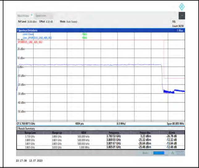
1-N78-3700-3800-PC2-30-70-H-6-CP-QPSK-Outer_Full-189@0-Ant1-1--PASS-see graph
