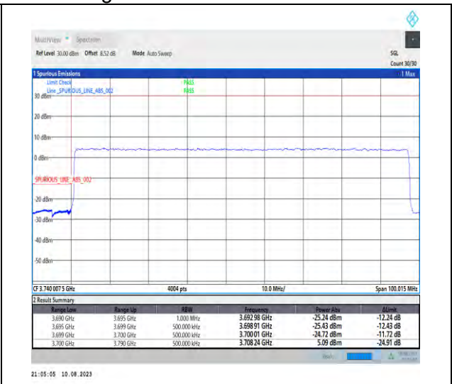
1-N78-3700-3800-PC2-30-90-L-3-DFT-PI2BPSK-Outer_Full-240@0-Ant1-1--PASS-see graph
