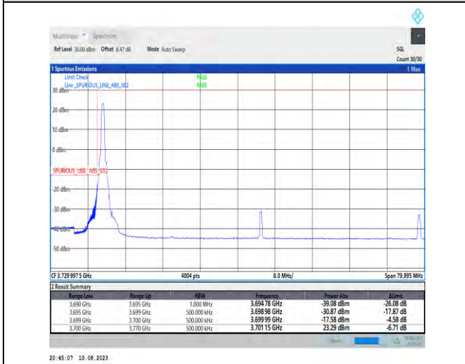
1-N78-3700-3800-PC2-30-70-L-4-CP-QPSK-Edge_1RB_Left-1@0-Ant1-1--PASS-see graph
