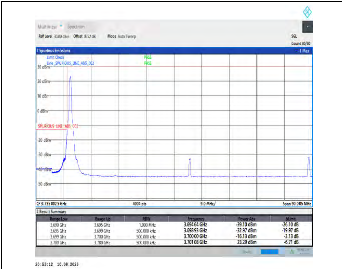
1-N78-3700-3800-PC2-30-80-L-1-DFT-PI2BPSK-Edge_1RB_Left-1@0-Ant1-1--PASS-see graph
