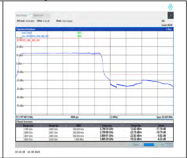
1-N78-3700-3800-PC2-30-15-H-3-DFT-PI2BPSK-Outer_Full-36@0-Ant1-1--PASS-see graph
