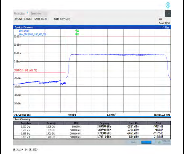
1-N78-3700-3800-PC2-30-20-L-6-CP-QPSK-Outer_Full-51@0-Ant1-1--PASS-see graph
