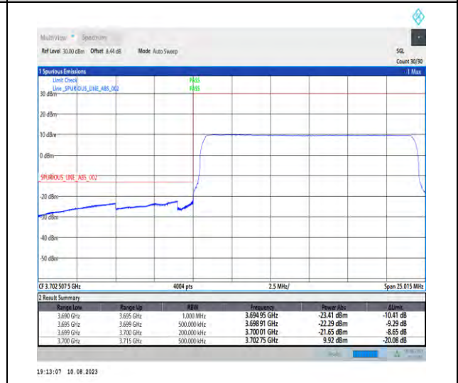
1-N78-3700-3800-PC2-30-15-L-6-CP-QPSK-Outer_Full-38@0-Ant1-1--PASS-see graph
