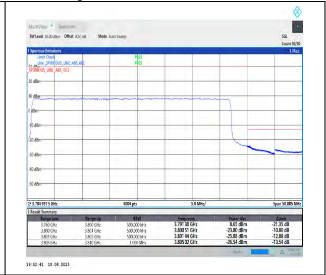
1-N78-3700-3800-PC2-30-40-H-3-DFT-PI2BPSK-Outer_Full-100@0-Ant1-1--PASS-see graph
