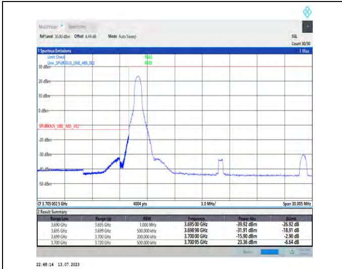
1-N78-3700-3800-PC2-30-20-L-1-DFT-PI2BPSK-Edge_1RB_Left-1@0-Ant1-1--PASS-see graph
