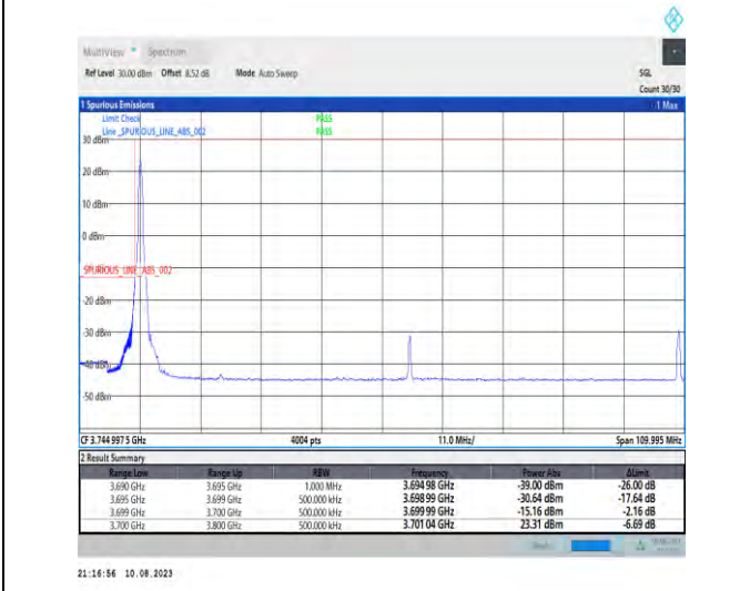
1-N78-3700-3800-PC2-30-100-L-4-CP-QPSK-Edge_1RB_Left-1@0-Ant1-1--PASS-see graph
