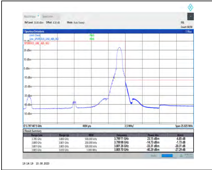
1-N78-3700-3800-PC2-30-15-H-2-DFT-PI2BPSK-Edge_1RB_Right-1@37-Ant1-1--PASS-see graph
