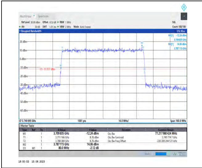
1-N78-3700-3800-PC2-30-80-M-5-DFT-256QAM-Out_er_Full-216@0-Ant1-77.218-80.000-≤80-PASS
