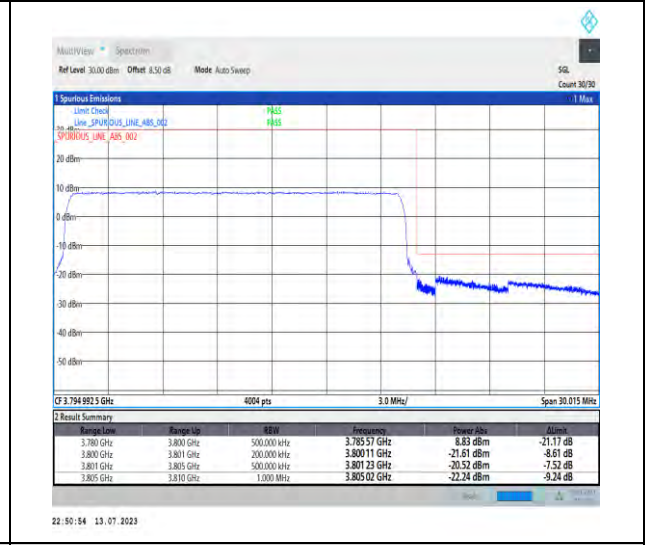
1-N78-3700-3800-PC2-30-30-H-6-CP-QPSK-Outer_Full-78@0-Ant1-1--PASS-see graph
