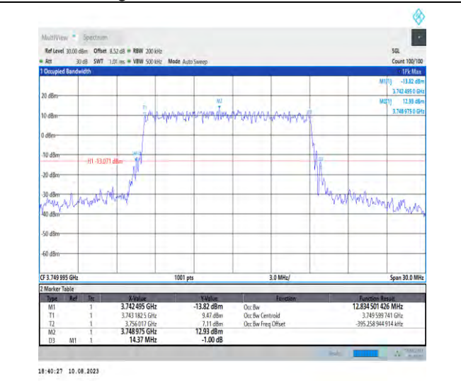
1-N78-3700-3800-PC2-30-15-M-5-DFT-256QAM-Outer_Full-36@0-Ant1-12.835-14.370-≤15-PASS
