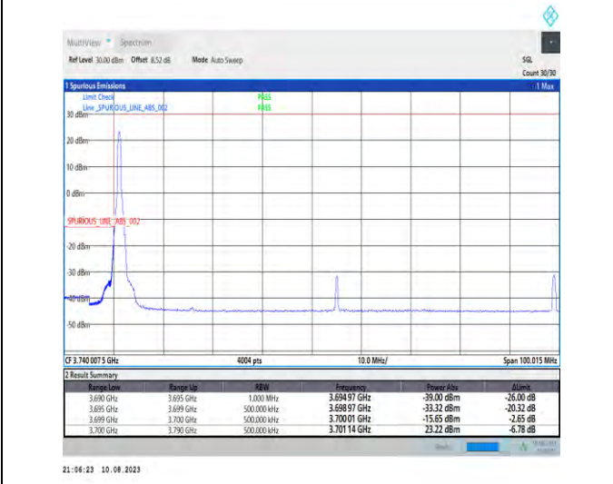
1-N78-3700-3800-PC2-30-90-L-4-CP-QPSK-Edge_1RB_Left-1@0-Ant1-1--PASS-see graph
