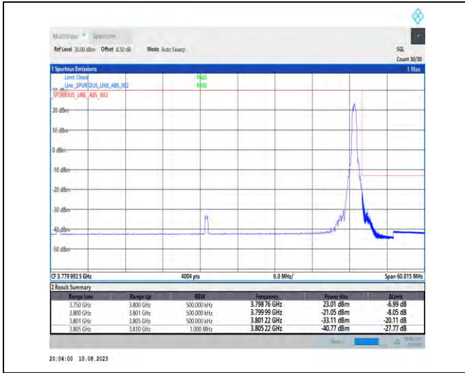
1-N78-3700-3800-PC2-30-50-H-2-DFT-PI2BPSK-Edge_1RB_Right-1@132-Ant1-1--PASS-see graph
