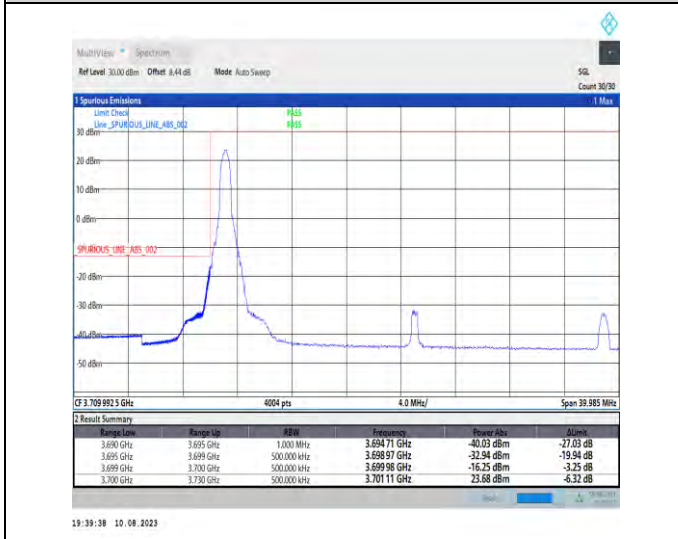
1-N78-3700-3800-PC2-30-30-L-4-CP-QPSK-Edge_1RB_Left-1@0-Ant1-1--PASS-see graph
