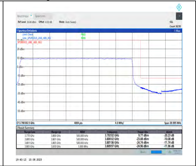
1-N78-3700-3800-PC2-30-30-H-3-DFT-PI2BPSK-Outer_Full-75@0-Ant1-1--PASS-see graph
