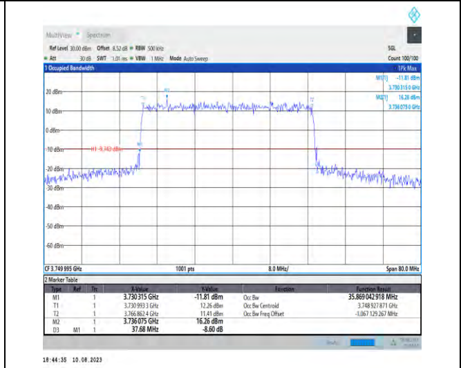
1-N78-3700-3800-PC2-30-40-M-4-DFT-64QAM-Outer_Full-100@0-Ant1-35.869-37.680-≤40-PASS
