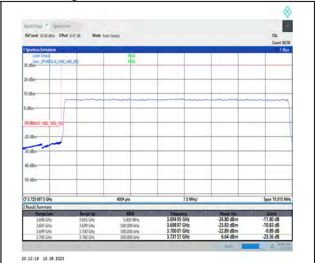
1-N78-3700-3800-PC2-30-60-L-3-DFT-PI2BPSK-Outer_Full-162@0-Ant1-1--PASS-see graph
