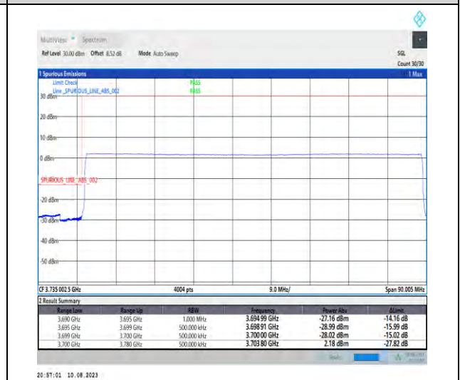
1-N78-3700-3800-PC2-30-80-L-6-CP-QPSK-Outer_Full-217@0-Ant1-1--PASS-see graph
