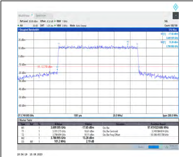
1-N78-3700-3800-PC2-30-100-M-7-CP-16QAM-Out er_Full-273@0-Ant1-97.419-101.200-≤100-PASS
