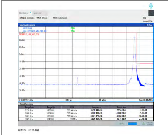
1-N78-3700-3800-PC2-30-70-H-2-DFT-PI2BPSK-Edge_1RB_Right-1@188-Ant1-1--PASS-see graph
