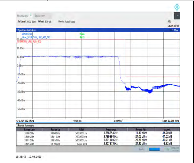
1-N78-3700-3800-PC2-30-20-H-3-DFT-PI2BPSK-Outer_Full-50@0-Ant1-1--PASS-see graph
