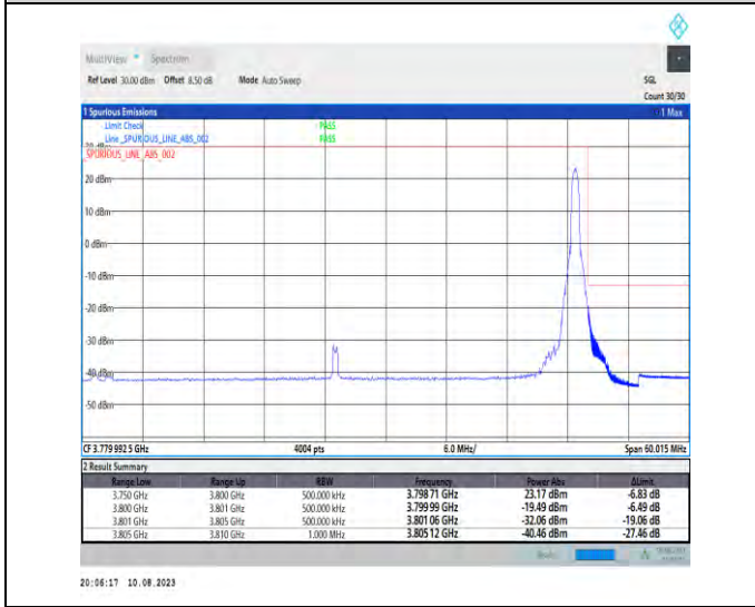
1-N78-3700-3800-PC2-30-50-H-5-CP-QPSK-Edge_1RB_Right-1@132-Ant1-1--PASS-see graph
