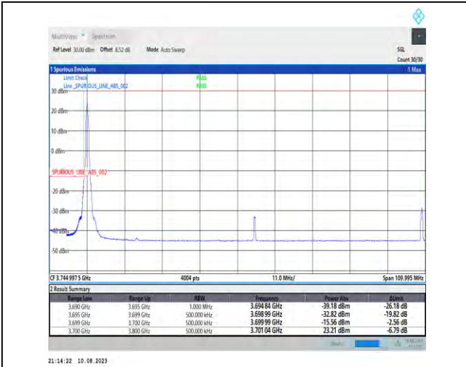
1-N78-3700-3800-PC2-30-100-L-1-DFT-PI2BPSK-Edge_e_1RB_Left-1@0-Ant1-1--PASS-see graph
