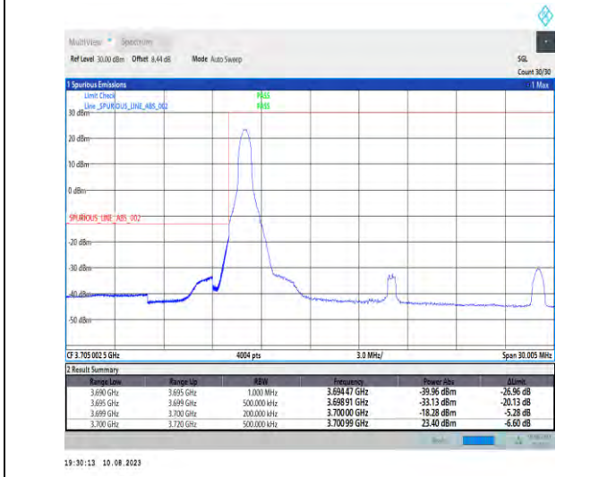
1-N78-3700-3800-PC2-30-20-L-4-CP-QPSK-Edge_1RB_Left-1@0-Ant1-1--PASS-see graph
