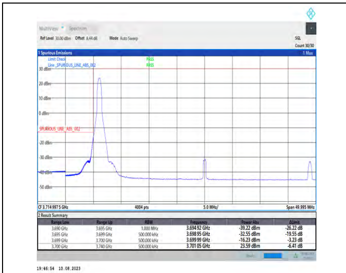
1-N78-3700-3800-PC2-30-40-L-1-DFT-PI2BPSK-Edge_1RB_Left-1@0-Ant1-1--PASS-see graph
