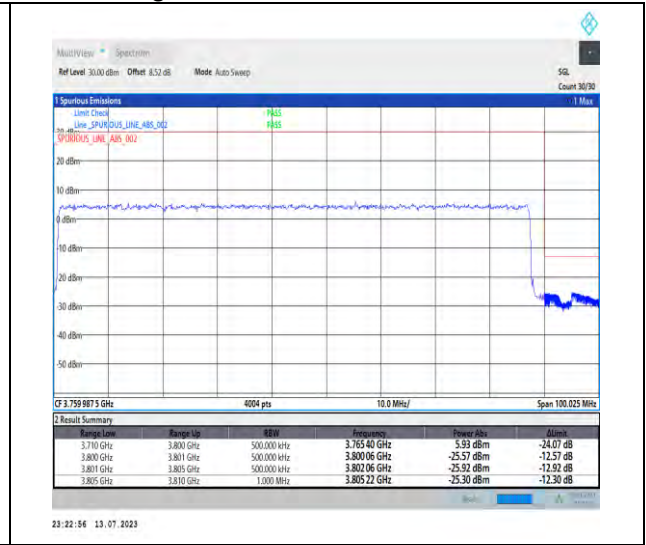
1-N78-3700-3800-PC2-30-90-H-3-DFT-PI2BPSK-Outer_Full-240@0-Ant1-1--PASS-see graph
