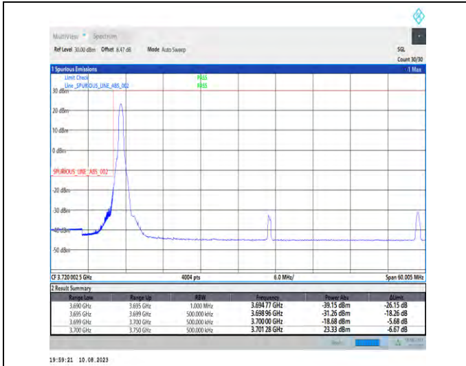
1-N78-3700-3800-PC2-30-50-L-1-DFT-PI2BPSK-Edge_1RB_Left-1@0-Ant1-1--PASS-see graph
