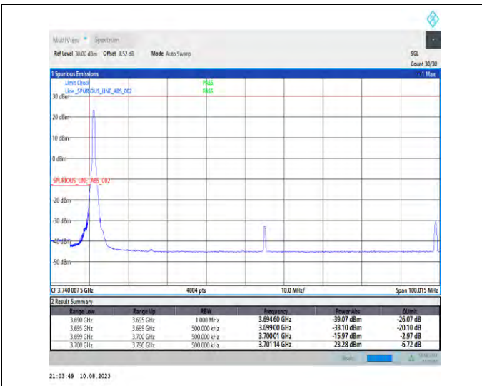
1-N78-3700-3800-PC2-30-90-L-1-DFT-PI2BPSK-Edge_1RB_Left-1@0-Ant1-1--PASS-see graph
