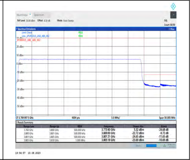
1-N78-3700-3800-PC2-30-40-H-6-CP-QPSK-Outer_Full-106@0-Ant1-1--PASS-see graph
