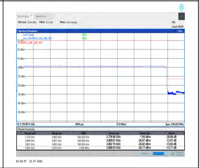
1-N78-3700-3800-PC2-30-90-H-6-CP-QPSK-Outer_Full-245@0-Ant1-1--PASS-see graph
