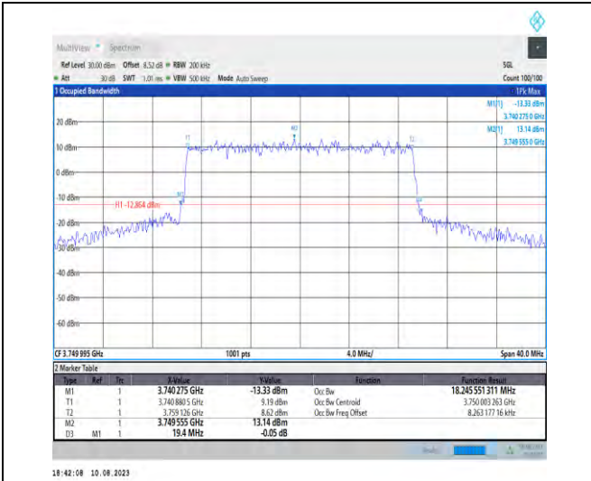
1-N78-3700-3800-PC2-30-20-M-7-CP-16QAM-Outer_Full-51@0-Ant1-18.246-19.400-≤20-PASS
