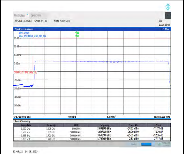
1-N78-3700-3800-PC2-30-70-L-6-CP-QPSK-Outer_Full-189@0-Ant1-1--PASS-see graph
