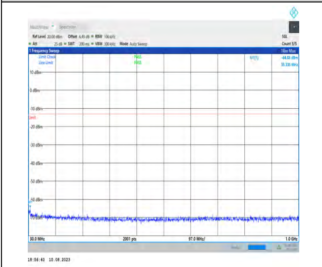
1-N78-3700-3800-PC2-30-100-H-1-N/A-DFT-PI2BP SK-Inner_1RB_Left-1@1-30-1000-Ant1-35.34--64.8 8--13-PASS
