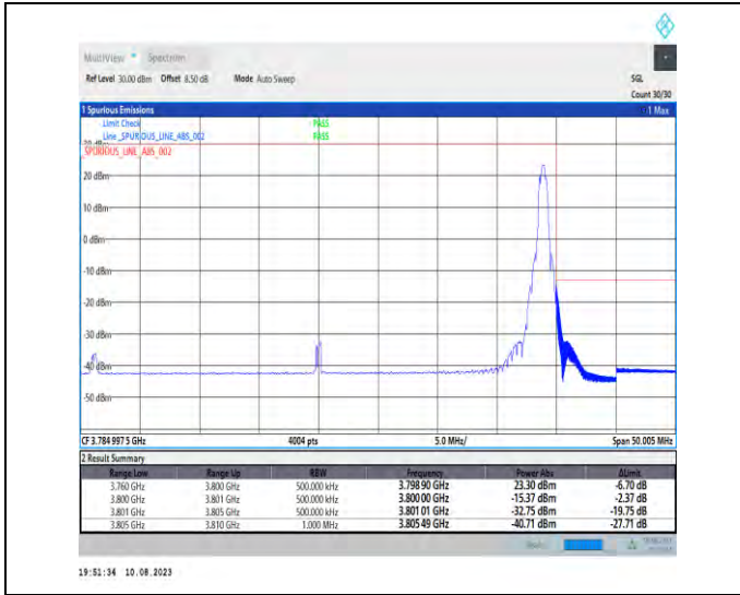
1-N78-3700-3800-PC2-30-40-H-2-DFT-PI2BPSK-Edge_1RB_Right-1@105-Ant1-1--PASS-see graph
