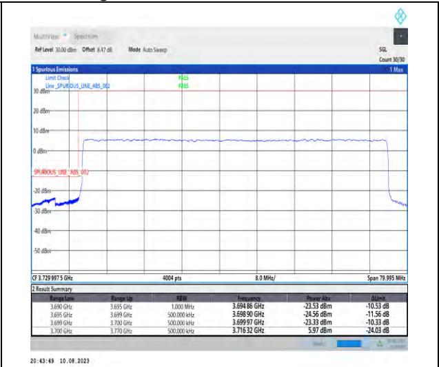
1-N78-3700-3800-PC2-30-70-L-3-DFT-PI2BPSK-Outer_Full-180@0-Ant1-1--PASS-see graph
