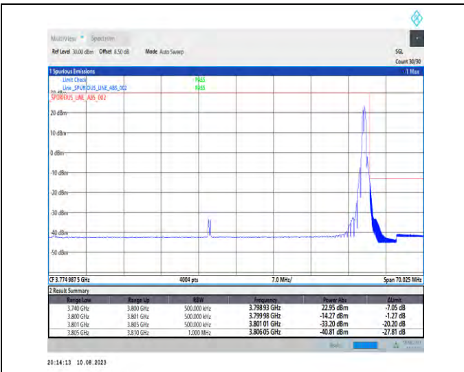
1-N78-3700-3800-PC2-30-60-H-2-DFT-PI2BPSK-Edge_1RB_Right-1@161-Ant1-1--PASS-see graph
