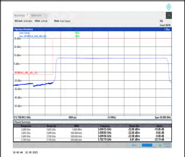
1-N78-3700-3800-PC2-30-30-L-6-CP-QPSK-Outer_Full-78@0-Ant1-1--PASS-see graph
