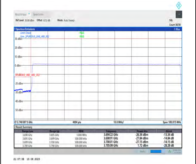
1-N78-3700-3800-PC2-30-90-L-6-CP-QPSK-Outer_Full-245@0-Ant1-1--PASS-see graph
