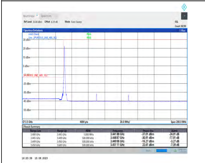
1-N78-3450-3550-PC2-30-80-L-4-CP-QPSK-Edge_1RB_Left-1@0-Ant1-1--PASS-see graph
