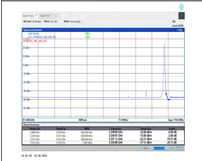
1-N78-3450-3550-PC2-30-40-H-5-CP-QPSK-Edge_1RB_Right-1@105-Ant1-1--PASS-see graph
