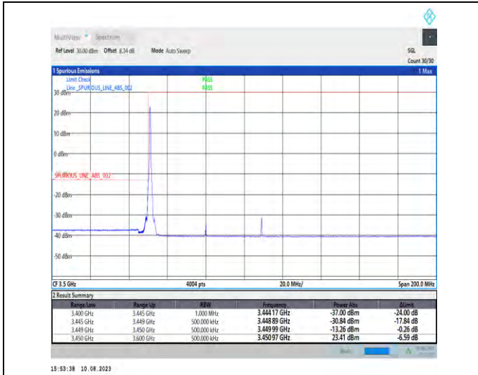
1-N78-3450-3550-PC2-30-60-L-1-DFT-PI2BPSK-Edge_1RB_Left-1@0-Ant1-1--PASS-see graph
