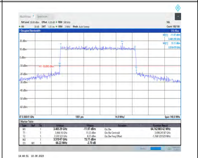
1-N78-3450-3550-PC2-30-70-M-1-DFT-QPSK-Outer_Full-180@0-Ant1-64.163-66.220-≤70-PASS
