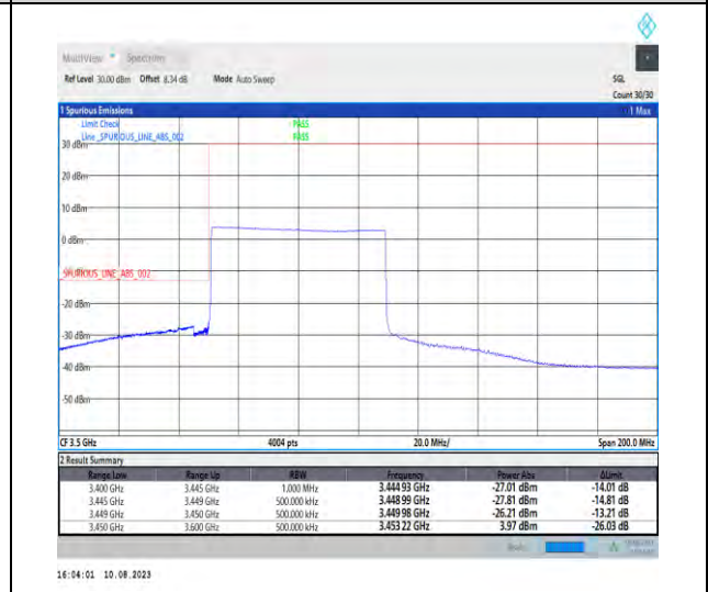
1-N78-3450-3550-PC2-30-60-L-6-CP-QPSK-Outer_Full-162@0-Ant1-1--PASS-see graph
