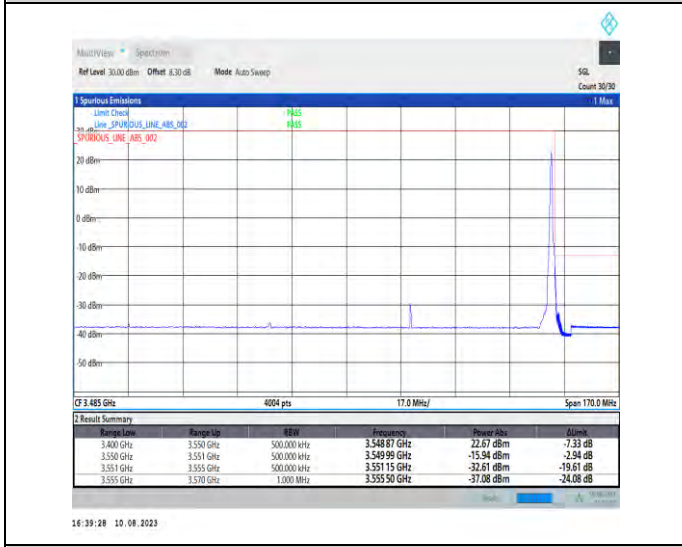
1-N78-3450-3550-PC2-30-90-H-5-CP-QPSK-Edge_1RB_Right-1@244-Ant1-1--PASS-see graph
