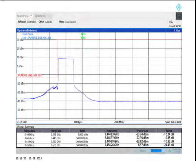
1-N78-3450-3550-PC2-30-20-L-6-CP-QPSK-Outer_Full-51@0-Ant1-1--PASS-see graph
