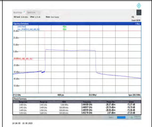
1-N78-3450-3550-PC2-30-80-L-6-CP-QPSK-Outer_Full-217@0-Ant1-1--PASS-see graph
