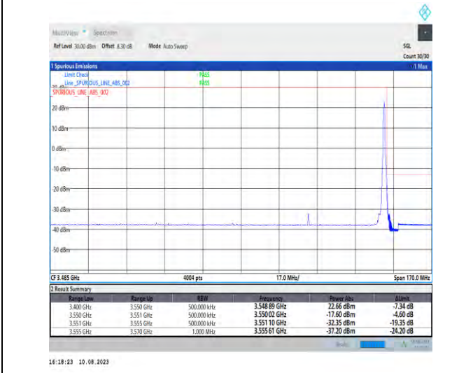
1-N78-3450-3550-PC2-30-70-H-5-CP-QPSK-Edge_1RB_Right-1@188-Ant1-1--PASS-see graph
