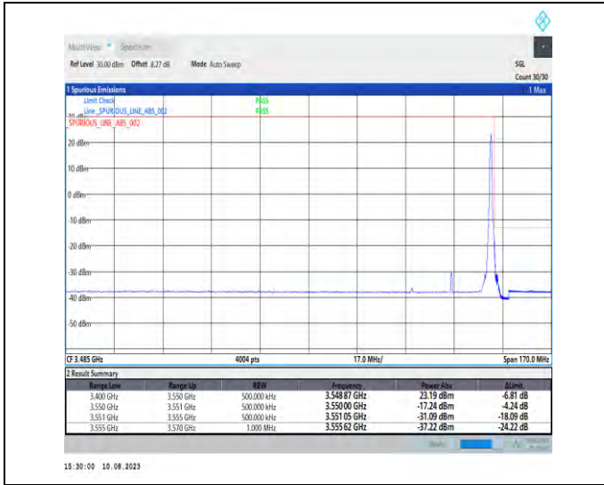
1-N78-3450-3550-PC2-30-30-H-2-DFT-PI2BPSK-Edge_1RB_Right-1@77-Ant1-1--PASS-see graph
