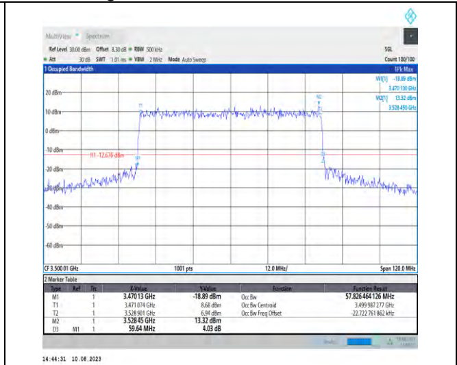
1-N78-3450-3550-PC2-30-60-M-8-CP-64QAM-Outer_Full-162@0-Ant1-57.826-59.640-≤60-PASS
