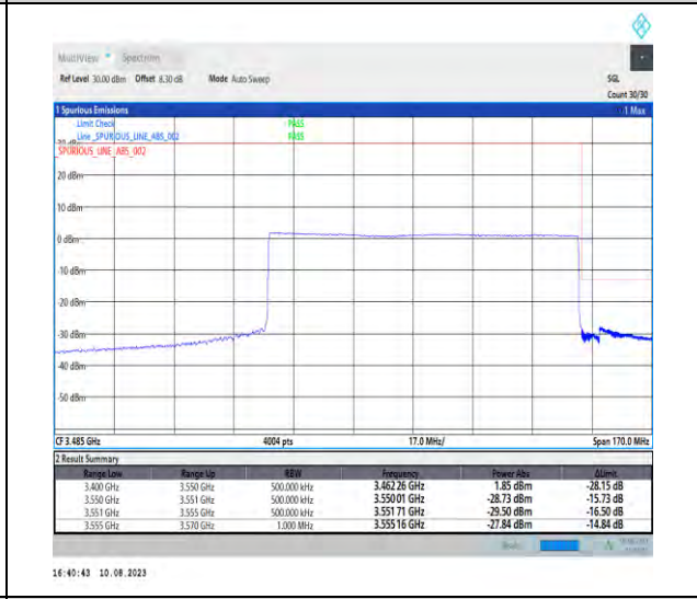
1-N78-3450-3550-PC2-30-90-H-6-CP-QPSK-Outer_Full-245@0-Ant1-1--PASS-see graph
