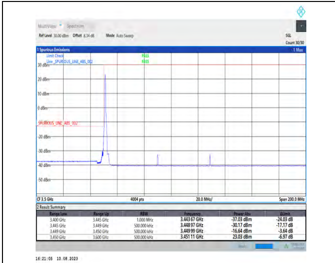
1-N78-3450-3550-PC2-30-80-L-1-DFT-PI2BPSK-Edge_1RB_Left-1@0-Ant1-1--PASS-see graph
