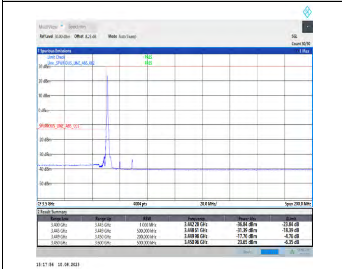
1-N78-3450-3550-PC2-30-20-L-4-CP-QPSK-Edge_1RB_Left-1@0-Ant1-1--PASS-see graph
