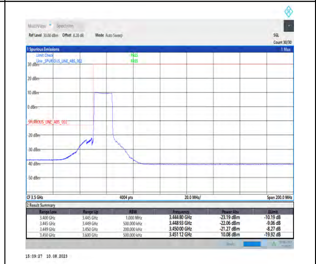
1-N78-3450-3550-PC2-30-15-L-6-CP-QPSK-Outer_Full-38@0-Ant1-1--PASS-see graph
