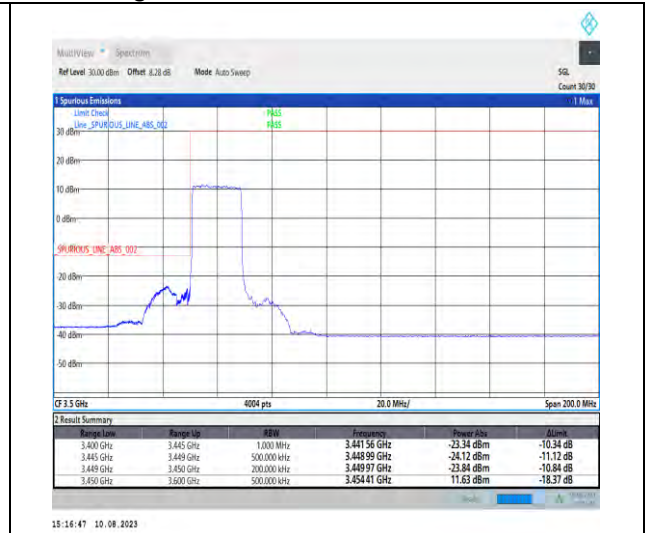
1-N78-3450-3550-PC2-30-20-L-3-DFT-PI2BPSK-Outer_Full-50@0-Ant1-1--PASS-see graph
