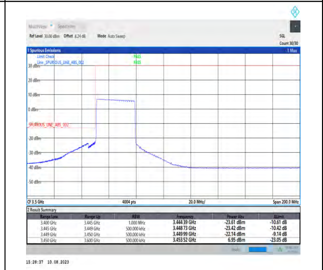
1-N78-3450-3550-PC2-30-30-L-6-CP-QPSK-Outer_Full-78@0-Ant1-1--PASS-see graph
