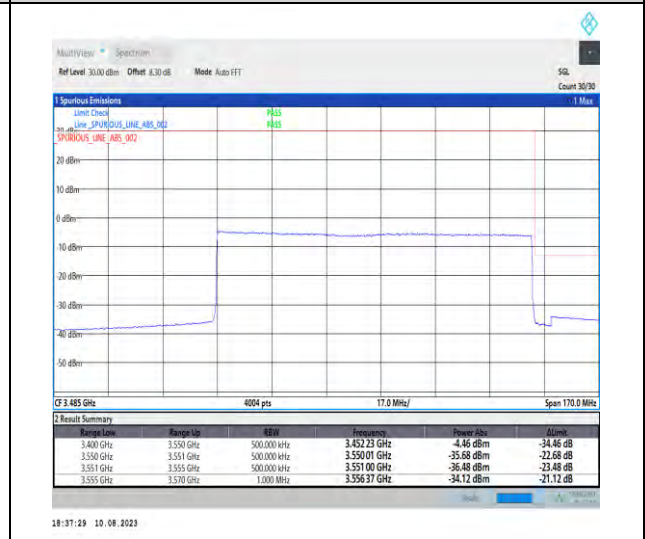
1-N78-3450-3550-PC2-30-100-H-6-CP-QPSK-Outer_Full-273@0-Ant1-1--PASS-see graph
