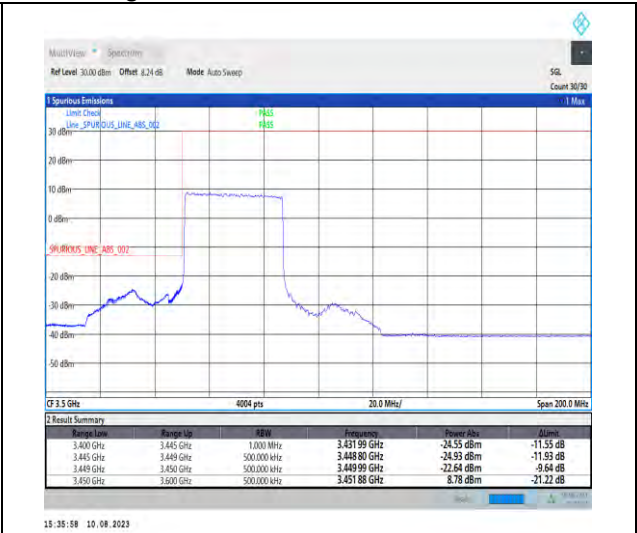
1-N78-3450-3550-PC2-30-40-L-3-DFT-PI2BPSK-Outer_Full-100@0-Ant1-1--PASS-see graph
