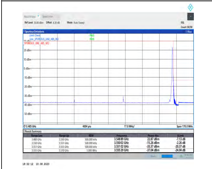
1-N78-3450-3550-PC2-30-100-H-5-CP-QPSK-Edge_1RB_Right-1@272-Ant1-1--PASS-see graph
