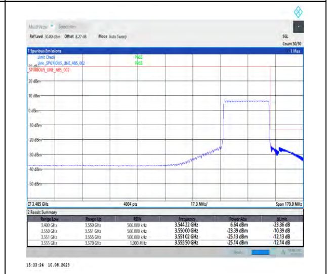
1-N78-3450-3550-PC2-30-30-H-6-CP-QPSK-Outer_Full-78@0-Ant1-1--PASS-see graph
