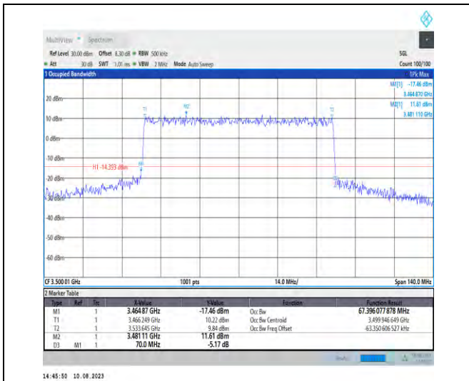
1-N78-3450-3550-PC2-30-70-M-6-CP-QPSK-Outer_Full-189@0-Ant1-67.396-70.000-≤70-PASS
