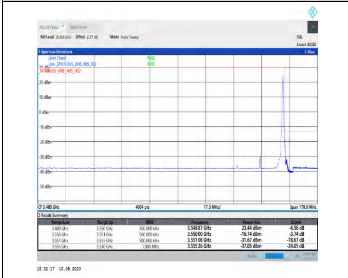
1-N78-3450-3550-PC2-30-30-H-5-CP-QPSK-Edge_1RB_Right-1@77-Ant1-1--PASS-see graph
