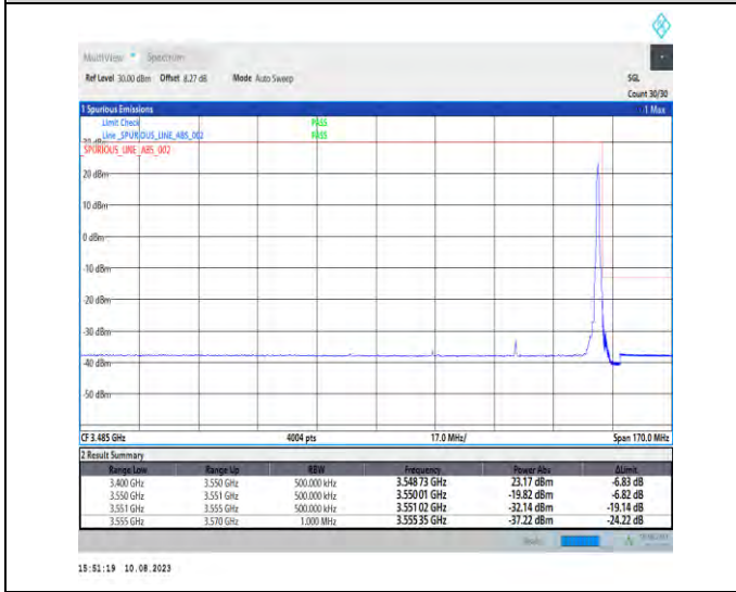
1-N78-3450-3550-PC2-30-50-H-5-CP-QPSK-Edge_1RB_Right-1@132-Ant1-1--PASS-see graph
