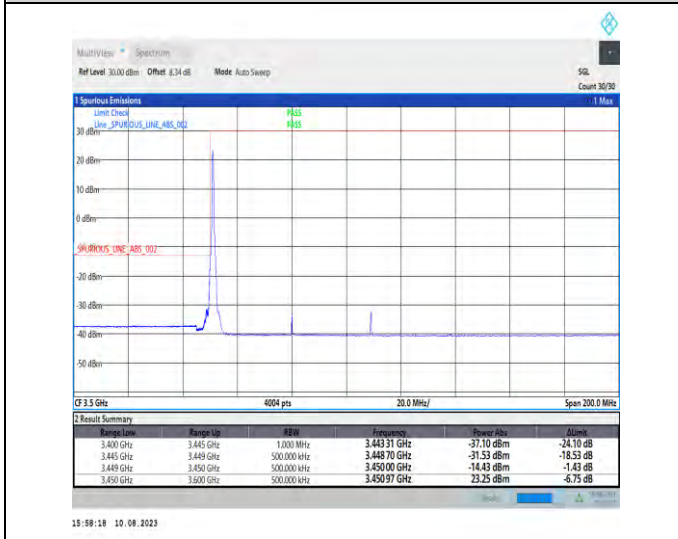
1-N78-3450-3550-PC2-30-60-L-4-CP-QPSK-Edge_1RB_Left-1@0-Ant1-1--PASS-see graph
