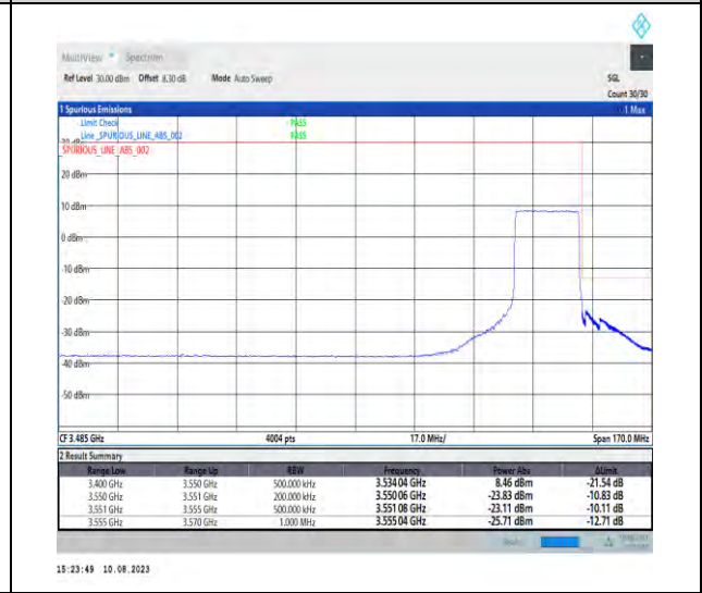
1-N78-3450-3550-PC2-30-20-H-6-CP-QPSK-Outer_Full-51@0-Ant1-1--PASS-see graph
