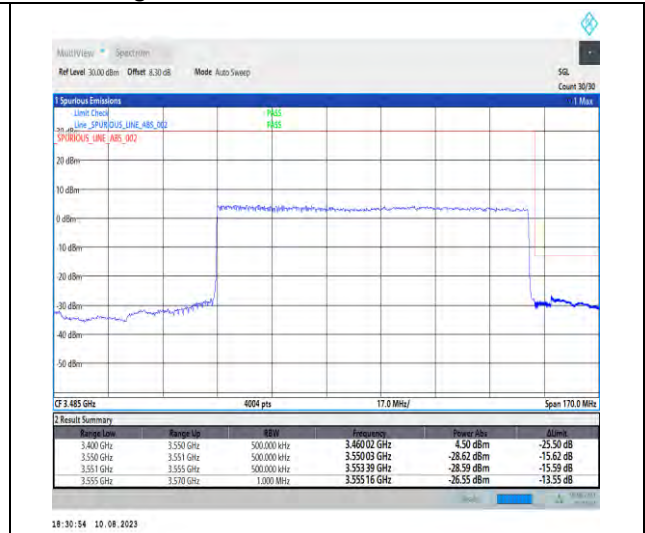
1-N78-3450-3550-PC2-30-100-H-3-DFT-PI2BPSK-Outer_Full-270@0-Ant1-1--PASS-see graph
