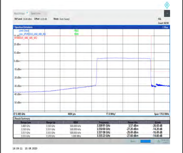
1-N78-3450-3550-PC2-30-60-H-6-CP-QPSK-Outer_Full-162@0-Ant1-1--PASS-see graph
