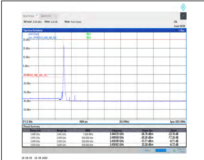
1-N78-3450-3550-PC2-30-15-L-1-DFT-PI2BPSK-Edge_1RB_Left-1@0-Ant1-1--PASS-see graph
