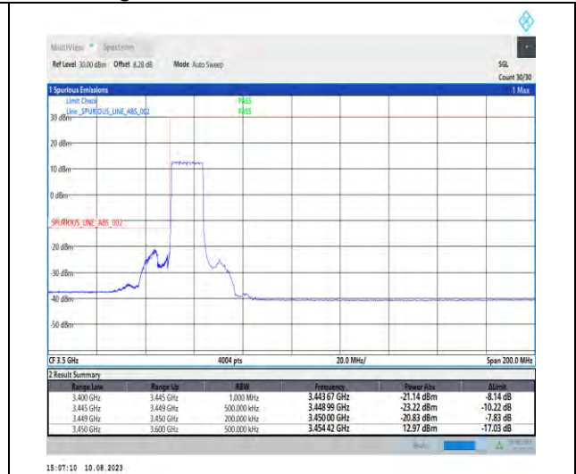
1-N78-3450-3550-PC2-30-15-L-3-DFT-PI2BPSK-Outer_Full-36@0-Ant1-1--PASS-see graph
