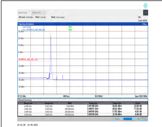
1-N78-3450-3550-PC2-30-20-L-1-DFT-PI2BPSK-Edge_1RB_Left-1@0-Ant1-1--PASS-see graph
