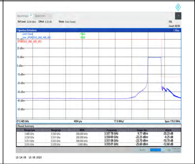
1-N78-3450-3550-PC2-30-15-H-6-CP-QPSK-Outer_Full-38@0-Ant1-1--PASS-see graph
