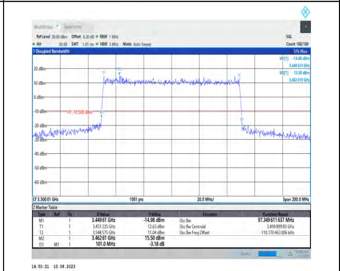
1-N78-3450-3550-PC2-30-100-M-6-CP-QPSK-Outer_Full-273@0-Ant1-97.35-101.000-≤100-PASS
