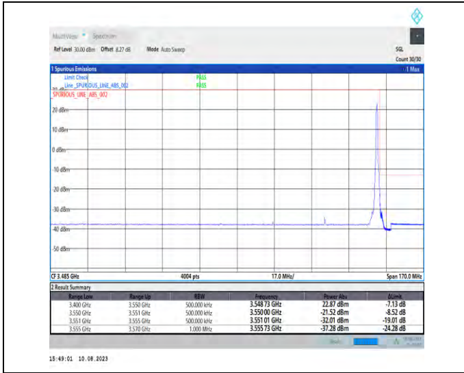
1-N78-3450-3550-PC2-30-50-H-2-DFT-PI2BPSK-Edge_1RB_Right-1@132-Ant1-1--PASS-see graph
