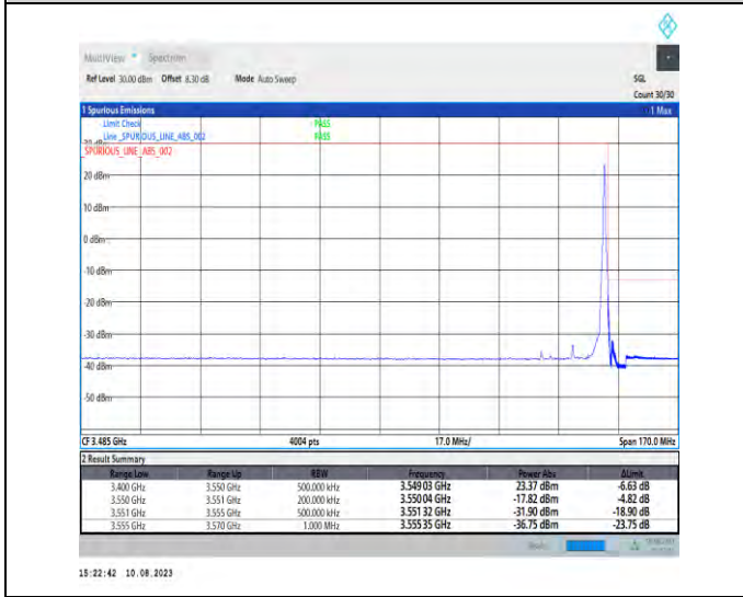
1-N78-3450-3550-PC2-30-20-H-5-CP-QPSK-Edge_1RB_Right-1@50-Ant1-1--PASS-see graph
