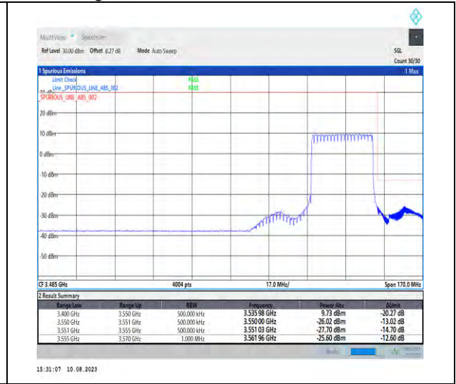
1-N78-3450-3550-PC2-30-30-H-3-DFT-PI2BPSK-Outer_Full-75@0-Ant1-1--PASS-see graph
