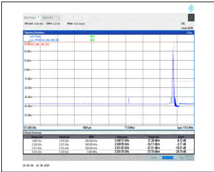
1-N78-3450-3550-PC2-30-90-H-2-DFT-PI2BPSK-Edge_1RB_Right-1@244-Ant1-1--PASS-see graph
