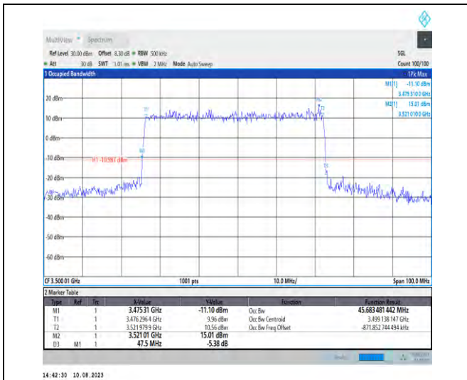
1-N78-3450-3550-PC2-30-50-M-4-DFT-64QAM-Outer_Full-128@0-Ant1-45.683-47.500-≤50-PASS
