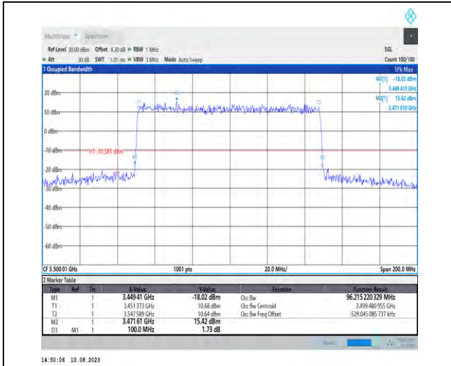
1-N78-3450-3550-PC2-30-100-M-3-DFT-16QAM-Out_er_Full-270@0-Ant1-96.215-100.000-≤100-PASS
