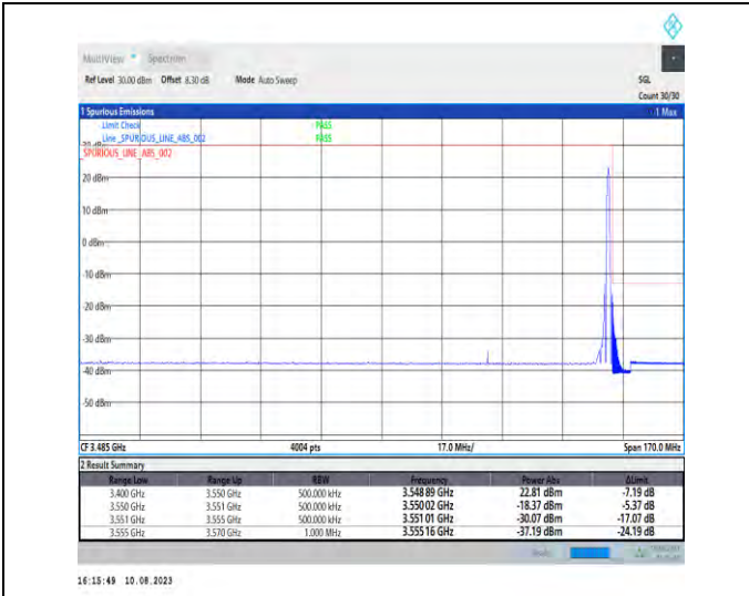
1-N78-3450-3550-PC2-30-70-H-2-DFT-PI2BPSK-Edge_1RB_Right-1@188-Ant1-1--PASS-see graph
