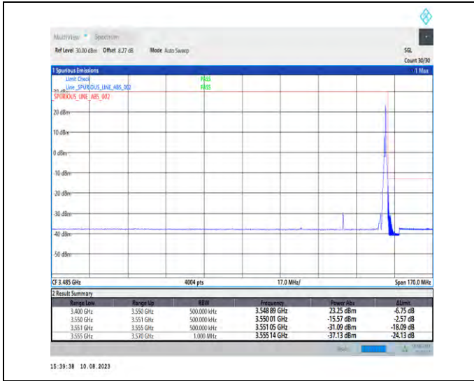
1-N78-3450-3550-PC2-30-40-H-2-DFT-PI2BPSK-Edge_1RB_Right-1@105-Ant1-1--PASS-see graph
