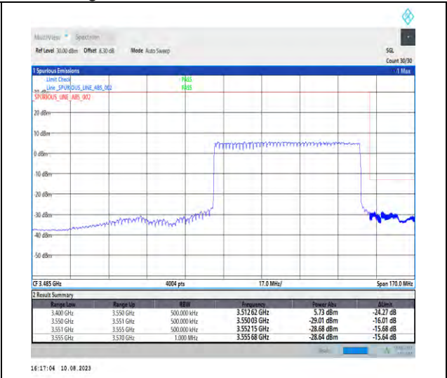
1-N78-3450-3550-PC2-30-70-H-3-DFT-PI2BPSK-Outer_Full-180@0-Ant1-1--PASS-see graph
