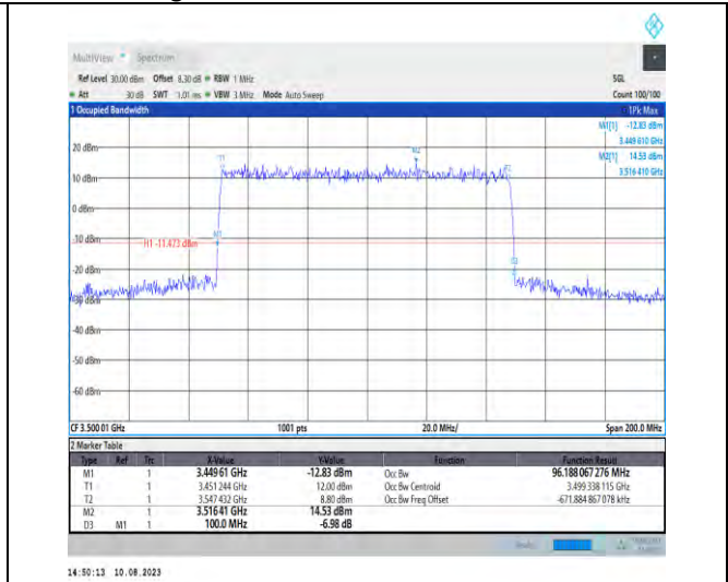
1-N78-3450-3550-PC2-30-100-M-4-DFT-64QAM-Out_er_Full-270@0-Ant1-96.188-100.000-≤100-PASS
