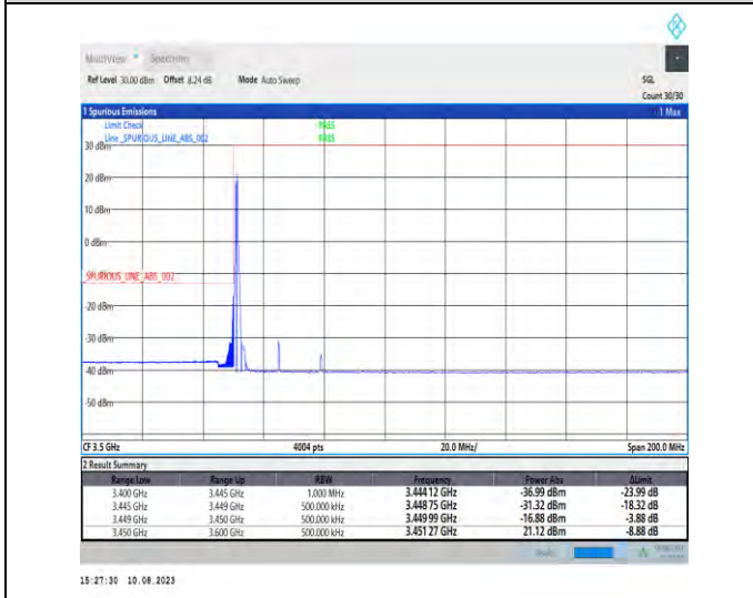
1-N78-3450-3550-PC2-30-30-L-4-CP-QPSK-Edge_1RB_Left-1@0-Ant1-1--PASS-see graph
