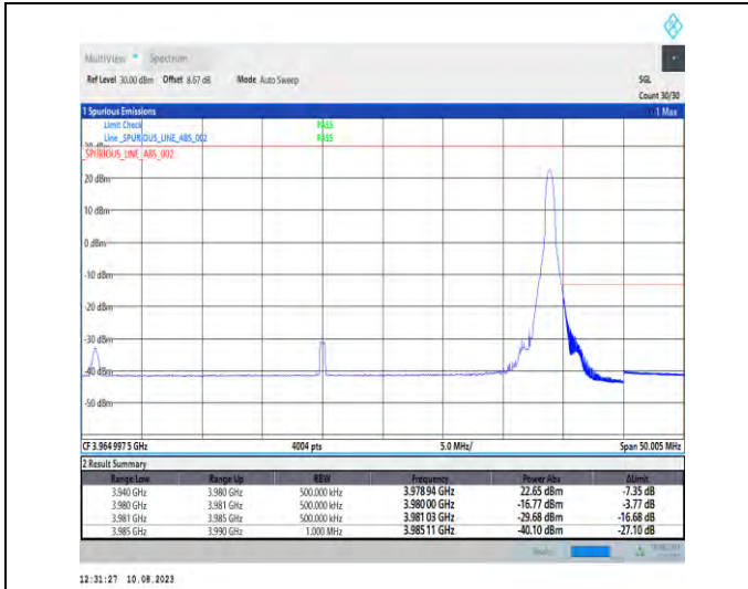
1-N77-3700-3980-PC2-30-40-H-2-DFT-PI2BPSK-Edge_1RB_Right-1@105-Ant1-1--PASS-see graph
