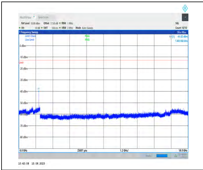
1-N77-3700-3980-PC2-30-100-L-1-N/A-DFT-PI2BPS K-Inner_1RB_Left-1@1-6000-18000-Ant1-11113.92- -41.02--13-PASS
