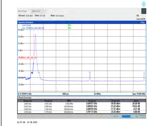
1-N77-3700-3980-PC2-30-70-L-4-CP-QPSK-Edge_1RB_Left-1@0-Ant1-1--PASS-see graph
