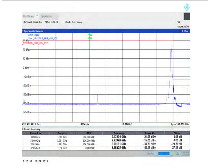
1-N77-3700-3980-PC2-30-90-H-5-CP-QPSK-Edge_1RB_Right-1@244-Ant1-1--PASS-see graph
