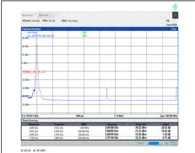
1-N77-3700-3980-PC2-30-100-L-1-DFT-PI2BPSK-Edge_e_1RB_Left-1@0-Ant1-1--PASS-see graph
