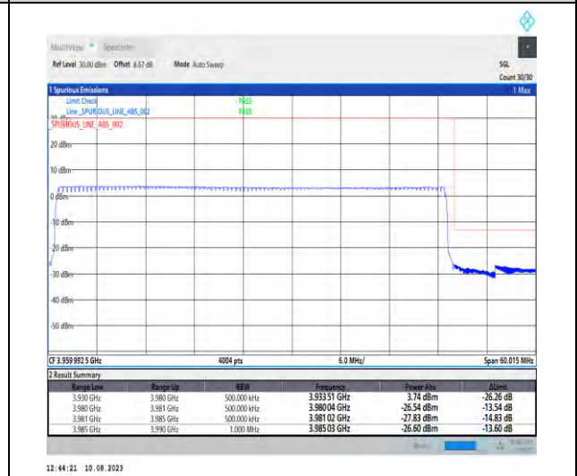
1-N77-3700-3980-PC2-30-50-H-6-CP-QPSK-Outer_Full-133@0-Ant1-1--PASS-see graph
