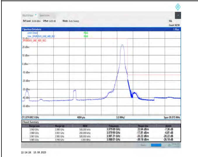
1-N77-3700-3980-PC2-30-20-H-5-CP-QPSK-Edge_1RB_Right-1@50-Ant1-1--PASS-see graph
