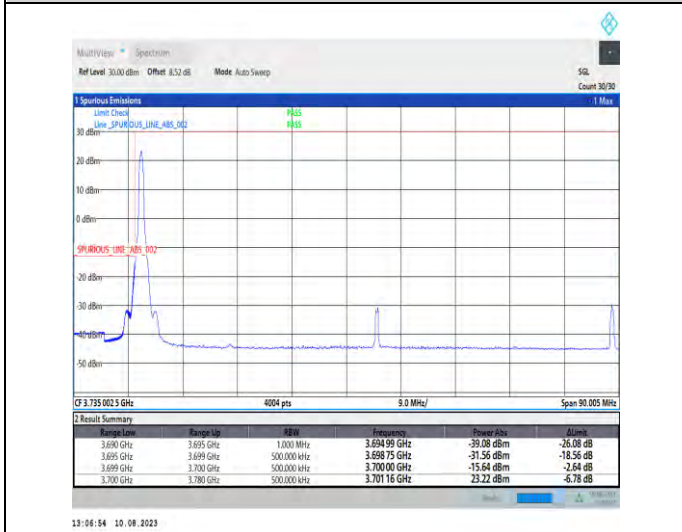
1-N77-3700-3980-PC2-30-80-L-4-CP-QPSK-Edge_1RB_Left-1@0-Ant1-1--PASS-see graph
