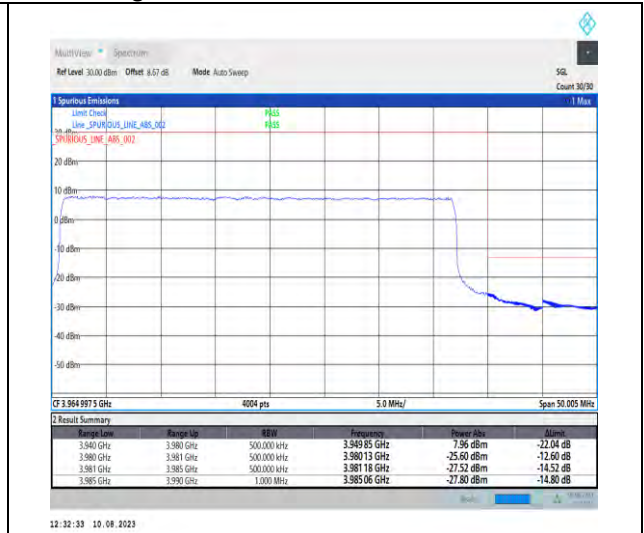
1-N77-3700-3980-PC2-30-40-H-3-DFT-PI2BPSK-Outer_Full-100@0-Ant1-1--PASS-see graph
