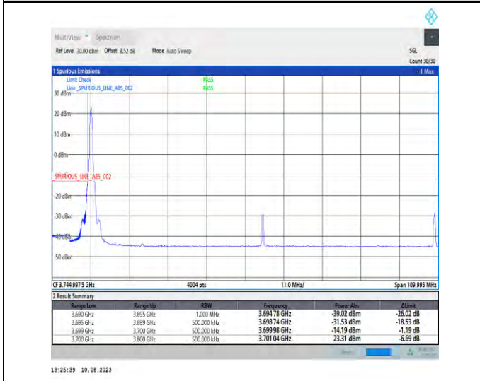
1-N77-3700-3980-PC2-30-100-L-4-CP-QPSK-Edge_1RB_Left-1@0-Ant1-1--PASS-see graph
