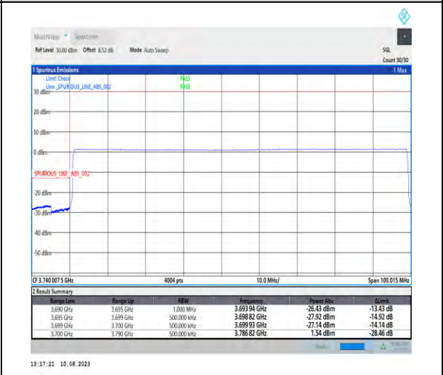
1-N77-3700-3980-PC2-30-90-L-6-CP-QPSK-Outer_Full-245@0-Ant1-1--PASS-see graph
