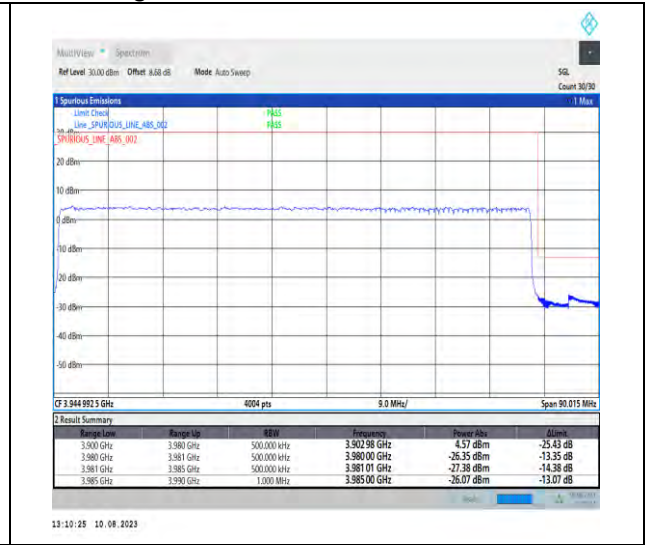
1-N77-3700-3980-PC2-30-80-H-3-DFT-PI2BPSK-Outer_Full-216@0-Ant1-1--PASS-see graph
