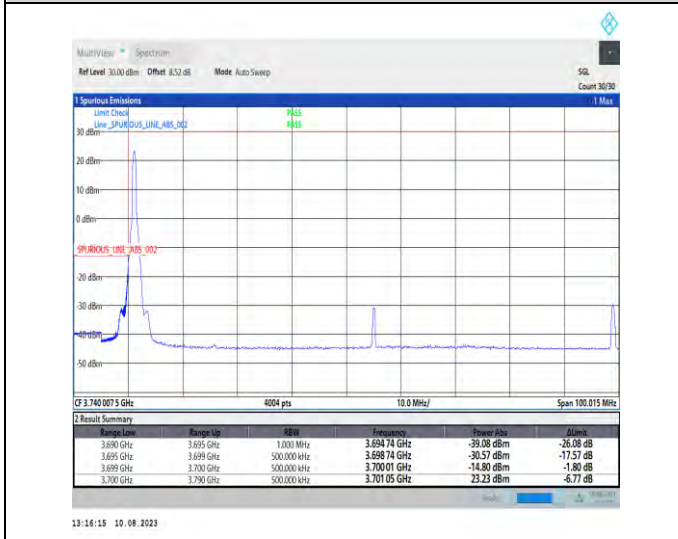
1-N77-3700-3980-PC2-30-90-L-4-CP-QPSK-Edge_1RB_Left-1@0-Ant1-1--PASS-see graph
