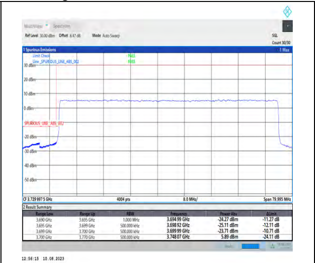
1-N77-3700-3980-PC2-30-70-L-3-DFT-PI2BPSK-Outer_Full-180@0-Ant1-1--PASS-see graph
