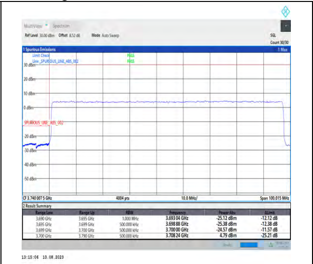
1-N77-3700-3980-PC2-30-90-L-3-DFT-PI2BPSK-Outer_Full-240@0-Ant1-1--PASS-see graph
