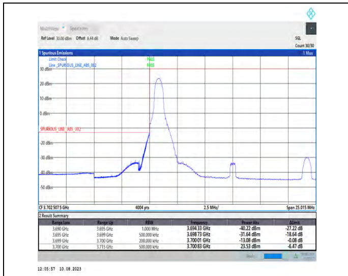
1-N77-3700-3980-PC2-30-15-L-1-DFT-PI2BPSK-Edge_1RB_Left-1@0-Ant1-1--PASS-see graph
