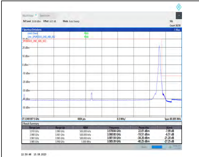
1-N77-3700-3980-PC2-30-70-H-2-DFT-PI2BPSK-Edge_1RB_Right-1@188-Ant1-1--PASS-see graph
