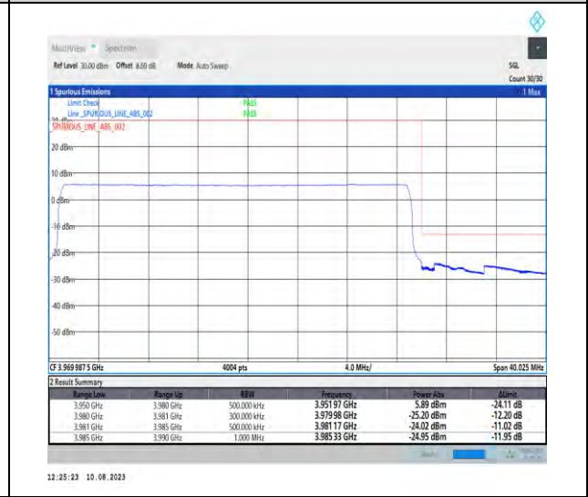
1-N77-3700-3980-PC2-30-30-H-6-CP-QPSK-Outer_Full-78@0-Ant1-1--PASS-see graph
