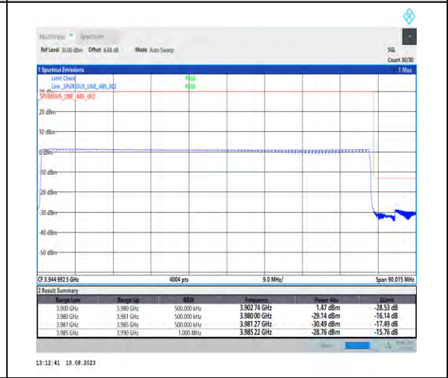
1-N77-3700-3980-PC2-30-80-H-6-CP-QPSK-Outer_Full-217@0-Ant1-1--PASS-see graph
