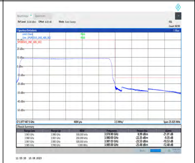
1-N77-3700-3980-PC2-30-15-H-6-CP-QPSK-Outer_Full-38@0-Ant1-1--PASS-see graph
