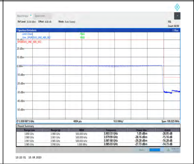
1-N77-3700-3980-PC2-30-90-H-6-CP-QPSK-Outer_Full-245@0-Ant1-1--PASS-see graph
