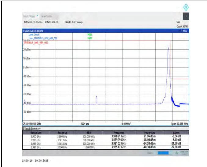
1-N77-3700-3980-PC2-30-80-H-2-DFT-PI2BPSK-Edge_1RB_Right-1@216-Ant1-1--PASS-see graph
