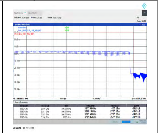
1-N77-3700-3980-PC2-30-90-H-3-DFT-PI2BPSK-Outer_Full-240@0-Ant1-1--PASS-see graph
