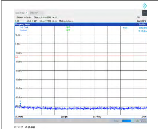
1-N77-3700-3980-PC2-30-100-M-1-N/A-DFT-PI2BP SK-Inner_1RB_Left-1@1-30-1000-Ant1-44.07--67.8 0--13-PASS
