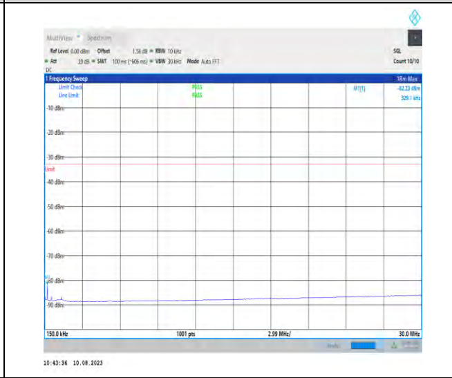
1-N77-3700-3980-PC2-30-100-M-1-N/A-DFT-PI2BPS K-Inner_1RB_Left-1@1-0.15-30-Ant1-0.33--82.23--3 3-PASS
