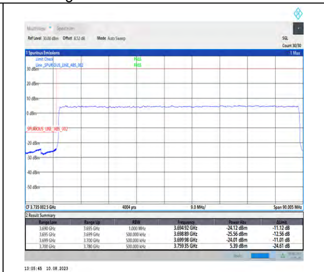
1-N77-3700-3980-PC2-30-80-L-3-DFT-PI2BPSK-Outer_Full-216@0-Ant1-1--PASS-see graph
