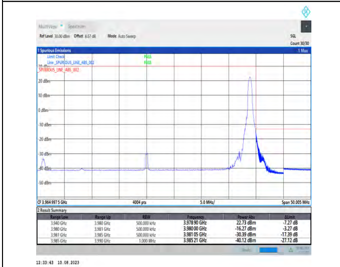
1-N77-3700-3980-PC2-30-40-H-5-CP-QPSK-Edge_1RB_Right-1@105-Ant1-1--PASS-see graph
