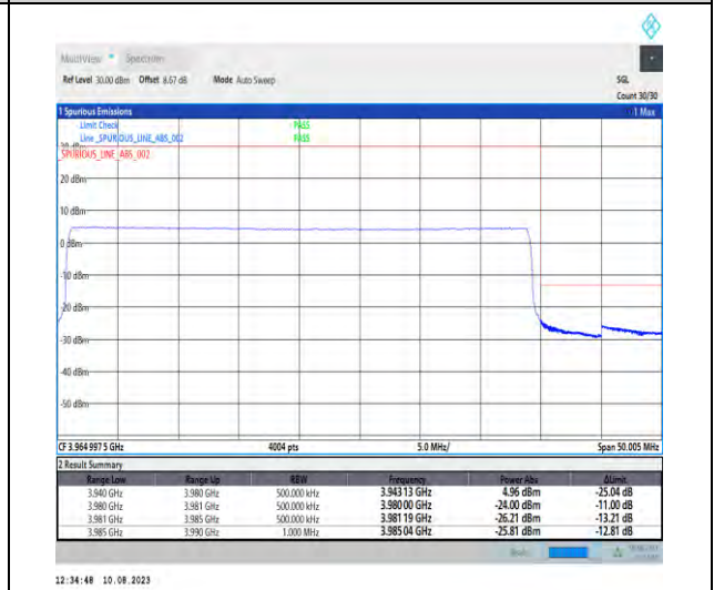
1-N77-3700-3980-PC2-30-40-H-6-CP-QPSK-Outer_Full-106@0-Ant1-1--PASS-see graph
