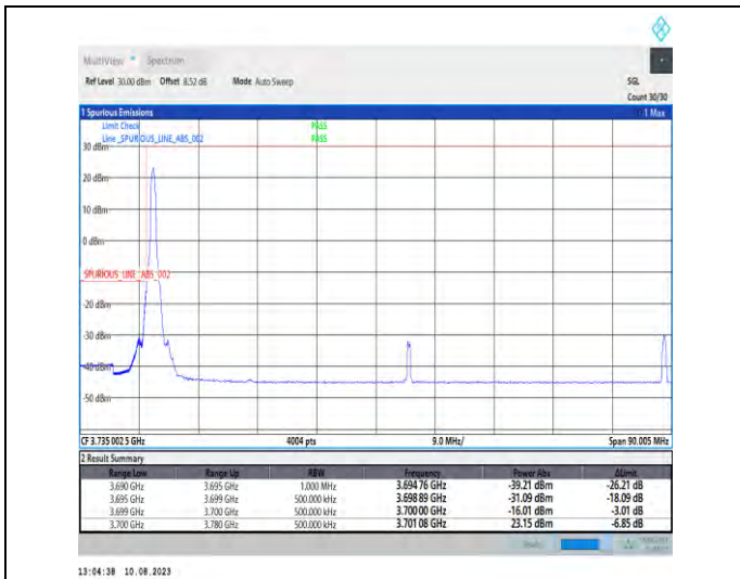
1-N77-3700-3980-PC2-30-80-L-1-DFT-PI2BPSK-Edge_1RB_Left-1@0-Ant1-1--PASS-see graph
