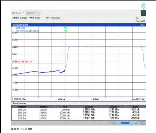
1-N77-3700-3980-PC2-30-15-L-6-CP-QPSK-Outer_Full-38@0-Ant1-1--PASS-see graph
