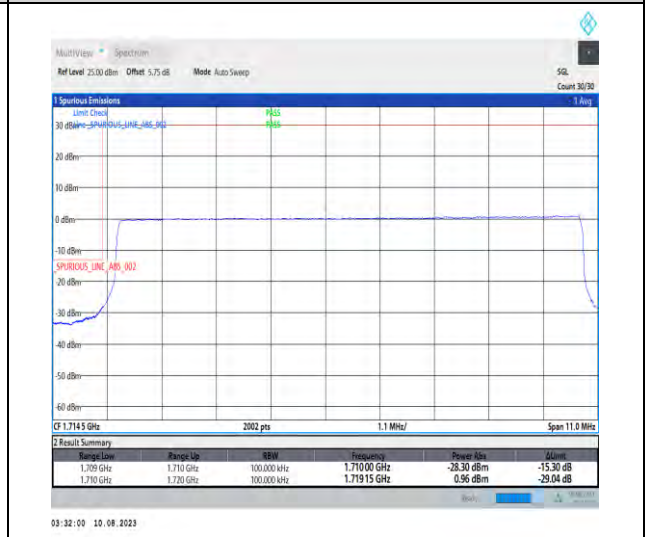
1-N66-PC3-15-10-L-6-CP-QPSK-Outer_Full-52@0-Ant1-1-seegraph-PASS-see graph
