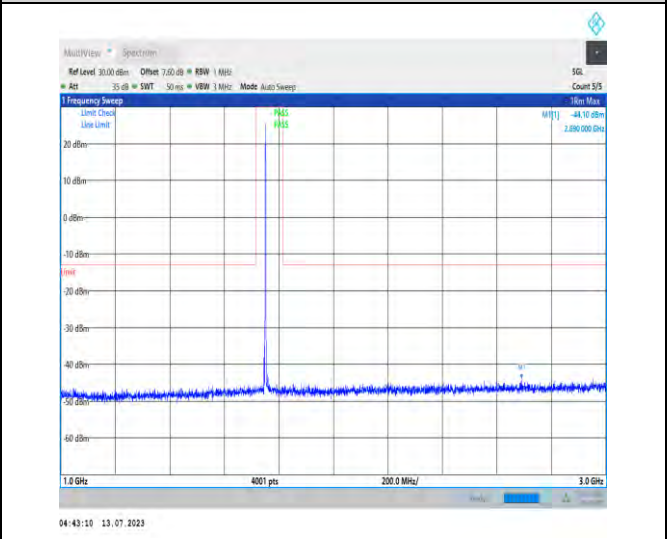
1-N66-PC3-15-30-H-1-N/A-DFT-PI2BPSK-Inner_1RB _Left-1@1-1000-3000-Ant1-2690.00--44.10--13-PASS
