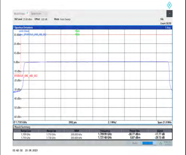
1-N66-PC3-15-20-L-6-CP-QPSK-Outer_Full-106@0-Ant1-1-seegraph-PASS-see graph
