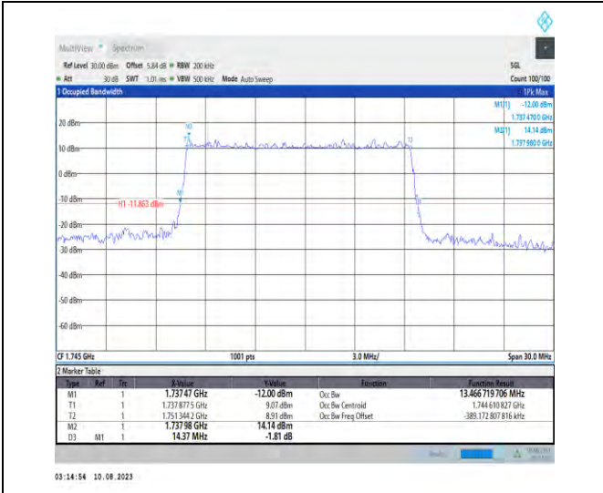
1-N66-PC3-15-15-M-3-DFT-16QAM-Outer_Full-75@ 0-Ant1-13.467-14.370≤15-PASS
