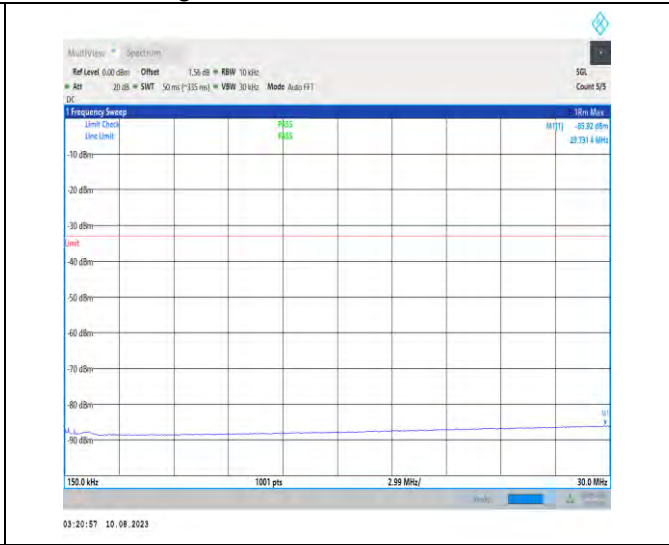
1-N66-PC3-15-40-M-1-N/A-DFT-PI2BPSK-Inner_1RB _Left-1@1-0.15-30-Ant1-0.15--85.92--33-PASS
