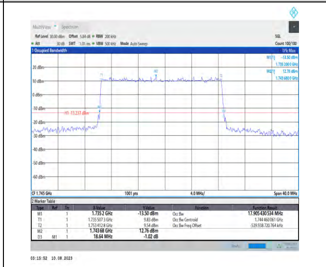
1-N66-PC3-15-20-M-1-DFT-QPSK-Outer_Full-100@0 -Ant1-17.905-18.640-<=20-PASS
