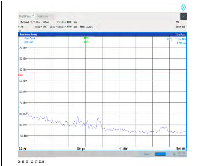
1-N66-PC3-15-30-H-1-N/A-DFT-PI2BPSK-Inner_1R B_Left-1@1-0.009-0.15-Ant1-0.01--77.73--43-PASS
