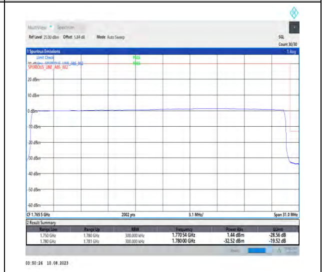
1-N66-PC3-15-30-H-6-CP-QPSK-Outer_Full-160@0-Ant1-1-seegraph-PASS-see graph
