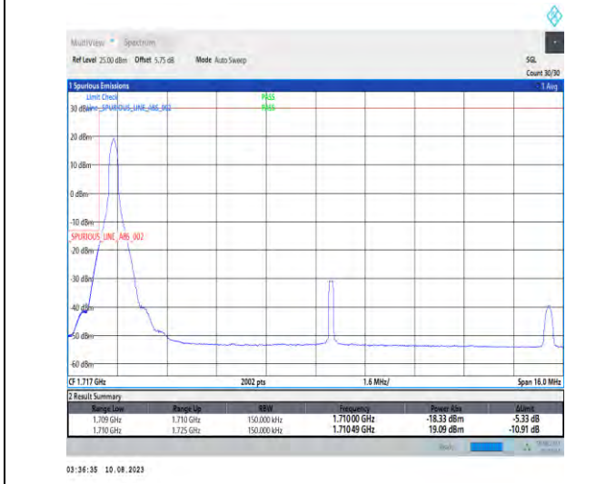
1-N66-PC3-15-15-L-4-CP-QPSK-Edge_1RB_Left-1@0-Ant1-1-seegraph-PASS-see graph
