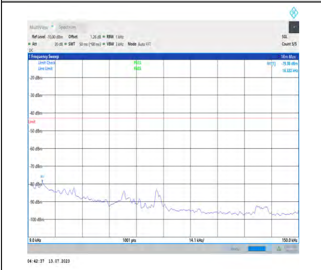
1-N66-PC3-15-30-M-1-N/A-DFT-PI2BPSK-Inner_1R B_Left-1@1-0.009-0.15-Ant1-0.02--79.38--43-PASS
