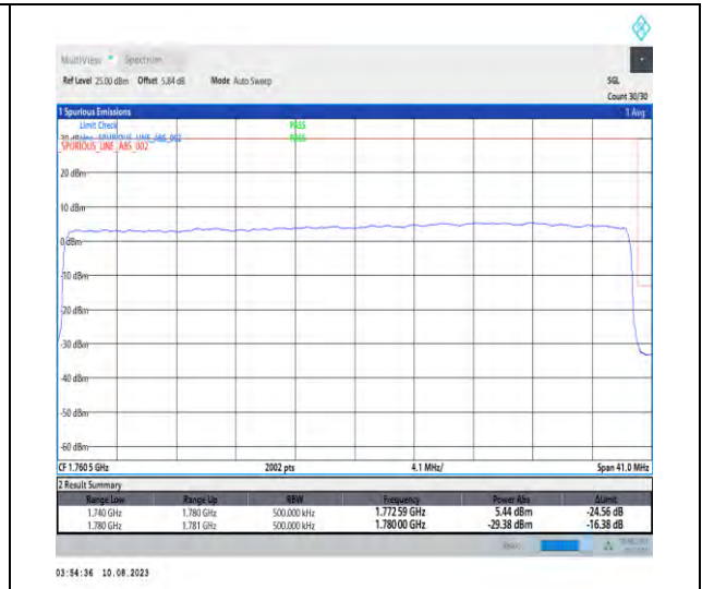
1-N66-PC3-15-40-H-3-DFT-PI2BPSK-Outer_Full-216@0-Ant1-1-seegraph-PASS-see graph
