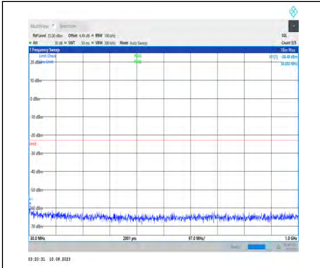
1-N66-PC3-15-40-L-1-N/A-DFT-PI2BPSK-Inner_1R B_Left-1@1-30-1000-Ant1-31.94--58.48--23-PASS
