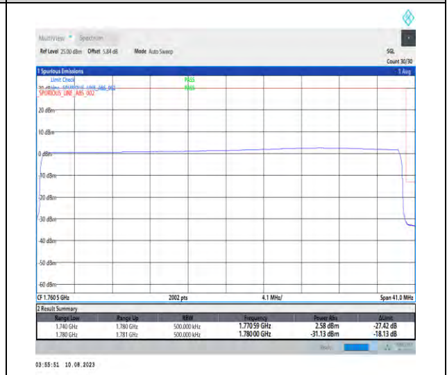
1-N66-PC3-15-40-H-6-CP-QPSK-Outer_Full-216@0-Ant1-1-seegraph-PASS-see graph
