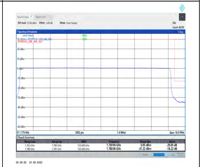
1-N66-PC3-15-15-H-6-CP-QPSK-Outer_Full-79@0-Ant1-1-seegraph-PASS-see graph
