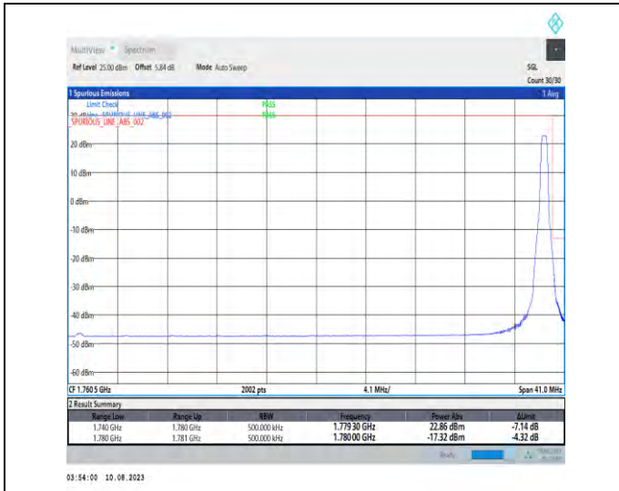
1-N66-PC3-15-40-H-2-DFT-PI2BPSK-Edge_1RB_Right-t-1@215-Ant1-1-seegraph-PASS-see graph
