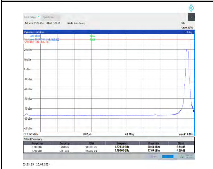
1-N66-PC3-15-40-H-5-CP-QPSK-Edge_1RB_Right-1@215-Ant1-1-seegraph-PASS-see graph
