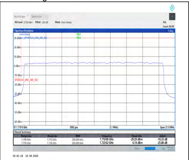
1-N66-PC3-15-20-L-3-DFT-PI2BPSK-Outer_Full-100@0-Ant1-1-seegraph-PASS-see graph
