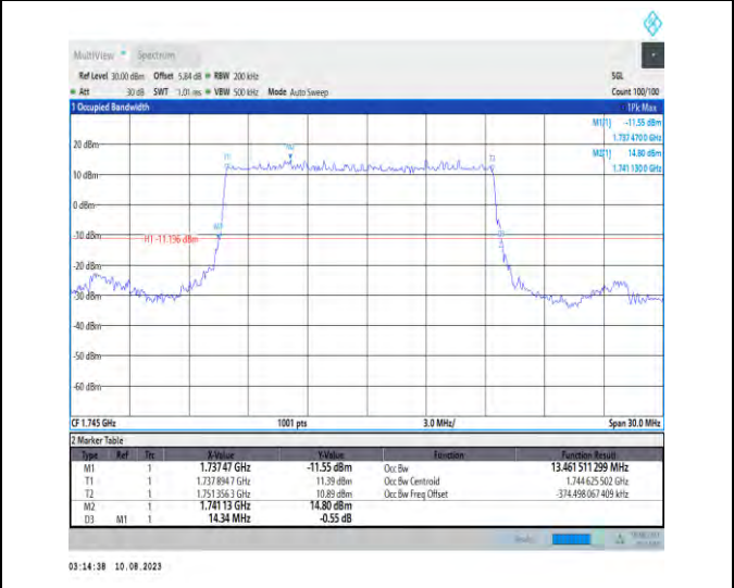
1-N66-PC3-15-15-M-2-DFT-PI2BPSK-Outer_Full-75 @0-Ant1-13.462-14.340-≤15-PASS
