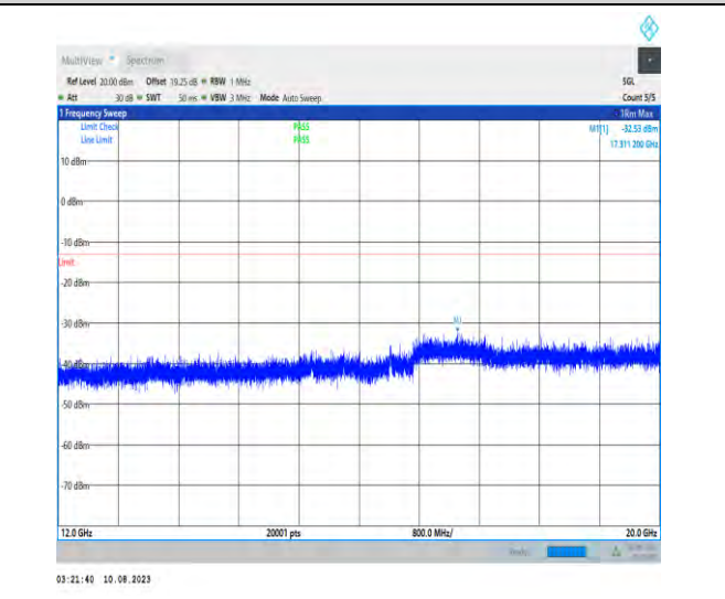
1-N66-PC3-15-40-H-1-N/A-DFT-PI2BPSK-Inner_1RB_Left-1@1-12000-20000-Ant1-17303.20--32.53--13-PASS
