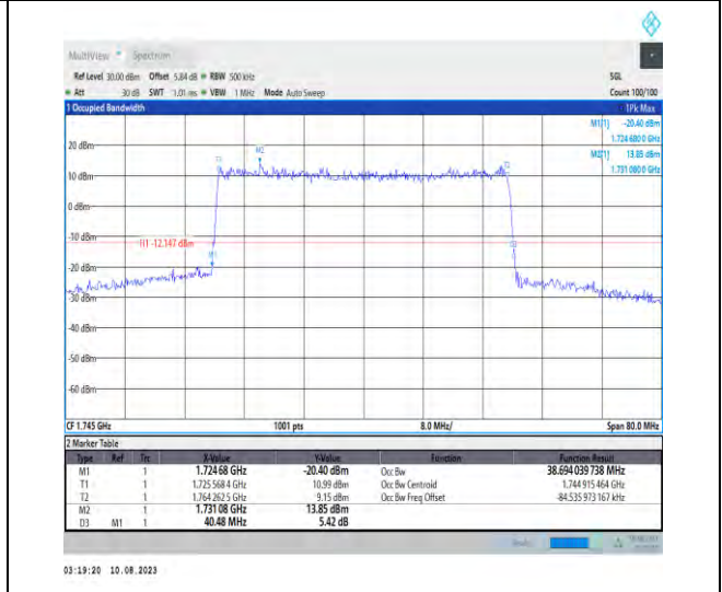
1-N66-PC3-15-40-M-3-DFT-16QAM-Outer_Full-216 @0-Ant1-38.694-40.480-<40-PASS
