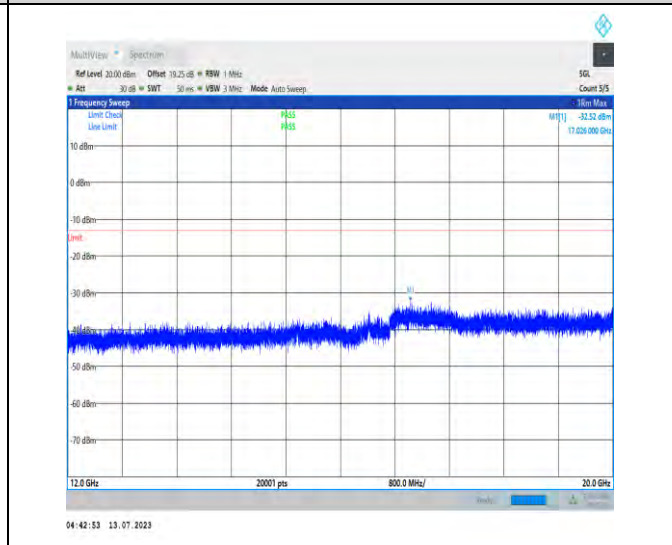
1-N66-PC3-15-30-M-1-N/A-DFT-PI2BPSK-Inner_1RB _Left-1@1-12000-20000-Ant1-17026.00--32.52--13-PASS
