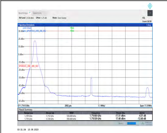
1-N66-PC3-15-10-L-4-CP-QPSK-Edge_1RB_Left-1@0-Ant1-1-seegraph-PASS-see graph
