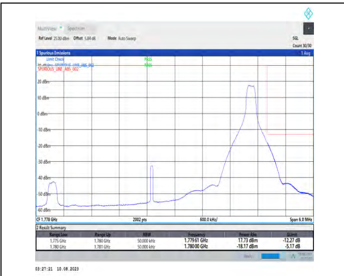
1-N66-PC3-15-5-H-2-DFT-PI2BPSK-Edge_1RB_Right-1@24-Ant1-1-seegraph-PASS-see graph
