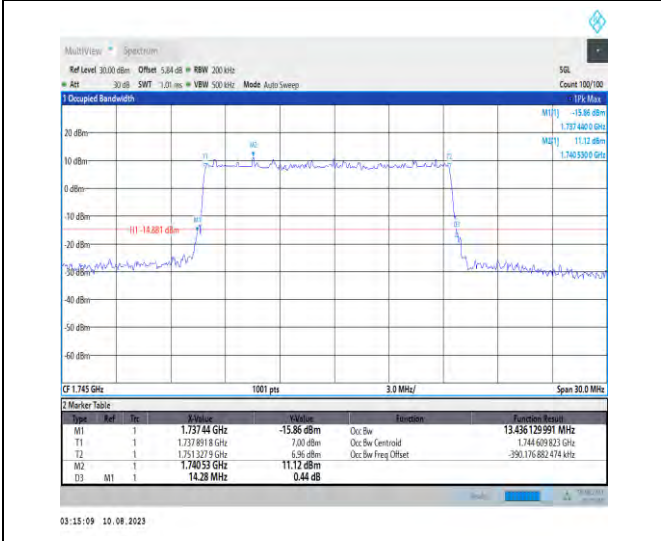
1-N66-PC3-15-15-M-5-DFT-256QAM-Outer_Full-75 @0-Ant1-13.436-14.280≤15-PASS
