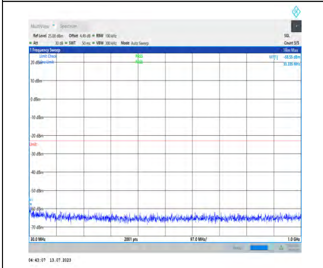
1-N66-PC3-15-30-H-1-N/A-DFT-PI2BPSK-Inner_1R B_Left-1@1-30-1000-Ant1-35.34--58.55--23-PASS
