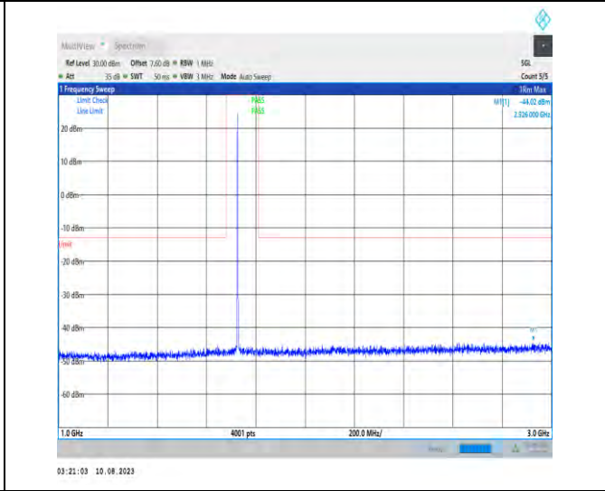
1-N66-PC3-15-40-M-1-N/A-DFT-PI2BPSK-Inner_1RB _Left-1@1-1000-3000-Ant1-2994.00--44.02--13-PASS
