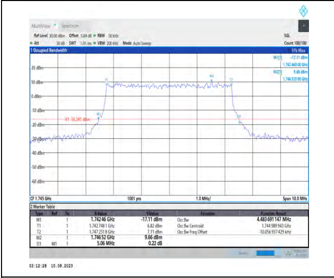
1-N66-PC3-15-5-M-7-CP-16QAM-Outer_Full-25@0-Ant1-4.484-5.060-≤5-PASS
