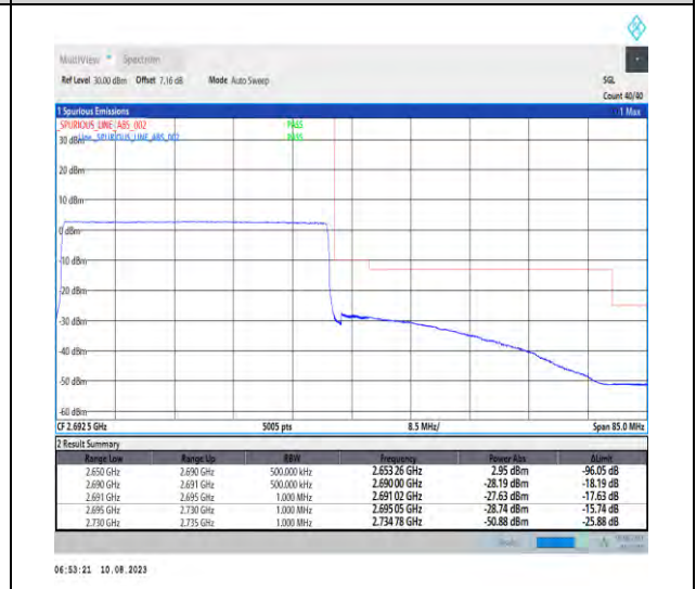
1-N41-PC3-30-40-H-6-CP-QPSK-Outer_Full-106@0-Ant1-1--PASS-see graph
