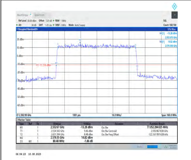
1-N41-PC3-30-80-M-1-DFT-QPSK-Outer_Full-216 @0-Ant1-77.052-80.480-<=80-PASS
