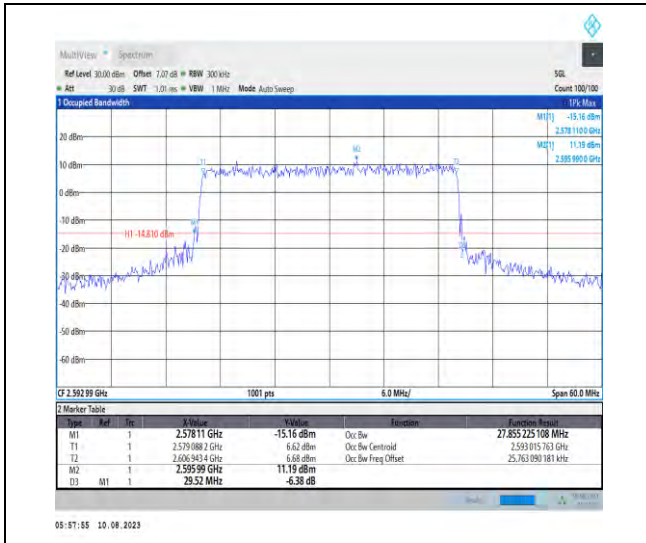
1-N41-PC3-30-30-M-8-CP-64QAM-Outer_Full-78@ @0-Ant1-27.855-29.520-≤30-PASS
