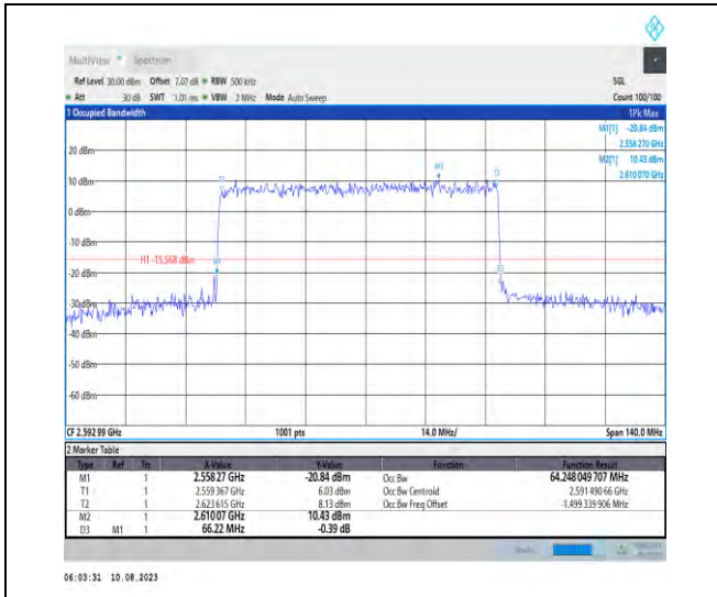
1-N41-PC3-30-70-M-4-DFT-64QAM-Outer_Full-180 @0-Ant1-64.248-66.220-<=70-PASS
