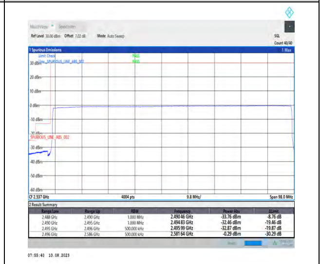
1-N41-PC3-30-90-L-6-CP-QPSK-Outer_Full-245@0-Ant1-1--PASS-see graph
