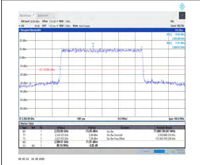
1-N41-PC3-30-80-M-5-DFT-256QAM-Outer_Full-216 @0-Ant1-77.09-80.160-<80-PASS
