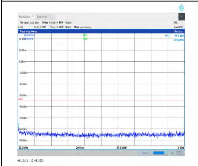
1-N41-PC3-30-100-H-1-N/A-DFT-PI2BPSK-Inner_1 RB_Left-1@1-30-1000-Ant1-30.49--59.15--35-PASS
