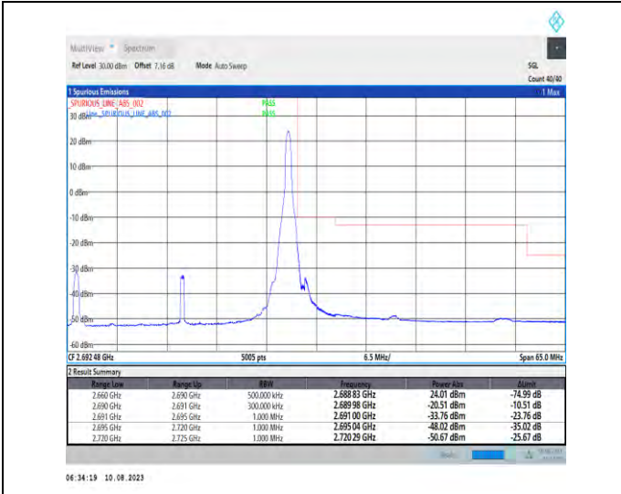
1-N41-PC3-30-30-H-2-DFT-PI2BPSK-Edge_1RB_Right-t1@77-Ant1-1--PASS-see graph
