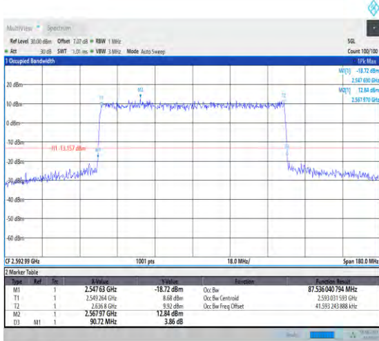
1-N41-PC3-30-90-M-6-CP-QPSK-Outer_Full-245@ 0-Ant1-87.536-90.720-≤90-PASS
