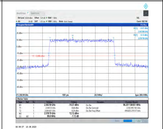
1-N41-PC3-30-100-M-4-DFT-64QAM-Outer_Full-270 @0-Ant1-96.331-99.800-≤100-PASS
