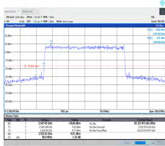
1-N41-PC3-30-90-M-9-CP-256QAM-Outer_Full-245 @0-Ant1-87.252-90.900-≤90-PASS
