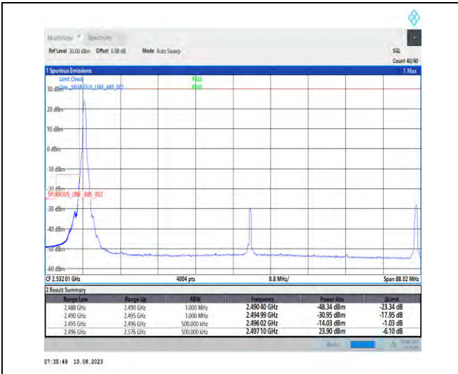
1-N41-PC3-30-80-L-1-DFT-PI2BPSK-Edge_1RB_Left-1@0-Ant1-1--PASS-see graph
