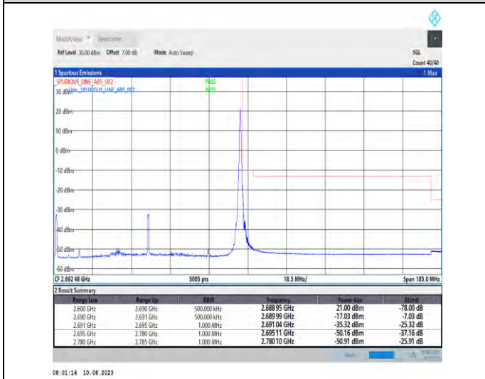
1-N41-PC3-30-90-H-5-CP-QPSK-Edge_1RB_Right-1@244-Ant1-1--PASS-see graph
