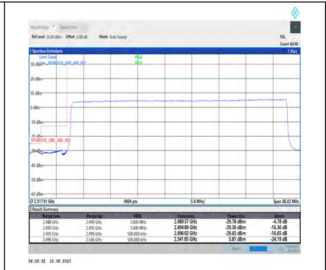
1-N41-PC3-30-50-L-3-DFT-PI2BPSK-Outer_Full-128@0-Ant1-1--PASS-see graph
