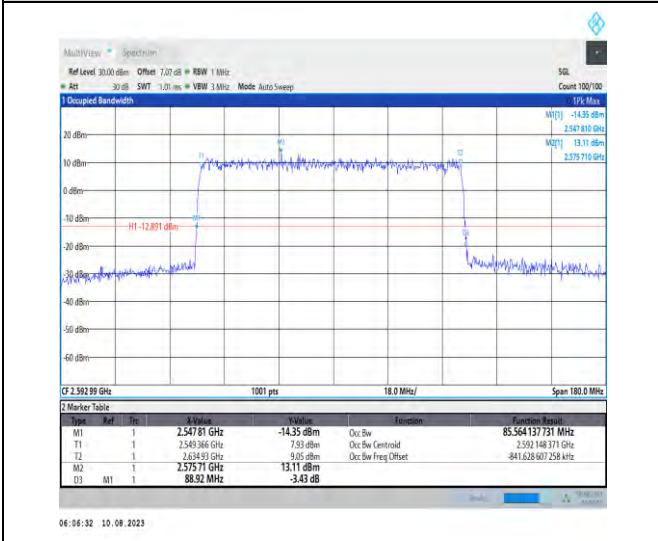
1-N41-PC3-30-90-M-4-DFT-64QAM-Outer_Full-240 @0-Ant1-85.564-88.920-<90-PASS
