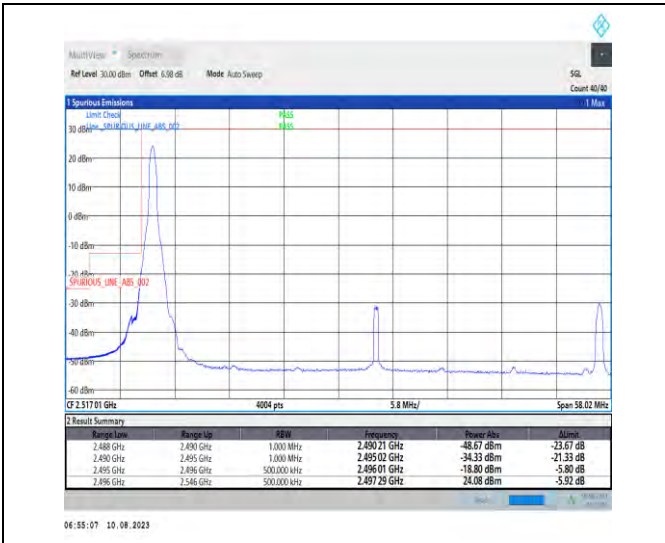
1-N41-PC3-30-50-L-1-DFT-PI2BPSK-Edge_1RB_Left-1@0-Ant1-1--PASS-see graph
