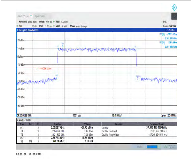
1-N41-PC3-30-60-M-3-DFT-16QAM-Outer_Full-162 @0-Ant1-57.878-60.240-≤60-PASS
