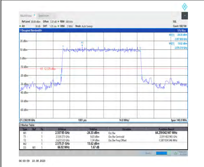
1-N41-PC3-30-70-M-2-DFT-PI2BPSK-Outer_Full-180 @0-Ant1-64.259-66.920-≤70-PASS
