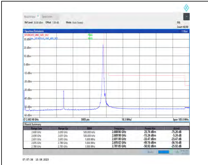
1-N41-PC3-30-90-H-2-DFT-PI2BPSK-Edge_1RB_Right-t-1@244-Ant1-1--PASS-see graph
