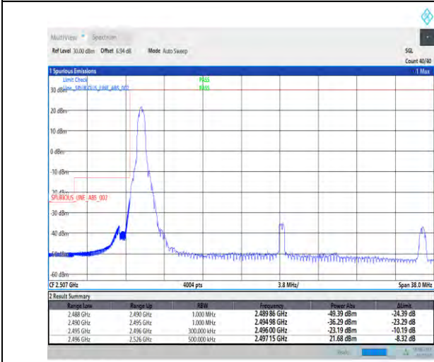
1-N41-PC3-30-30-L-1-DFT-PI2BPSK-Edge_1RB_Left-1@0-Ant1-1--PASS-see graph
