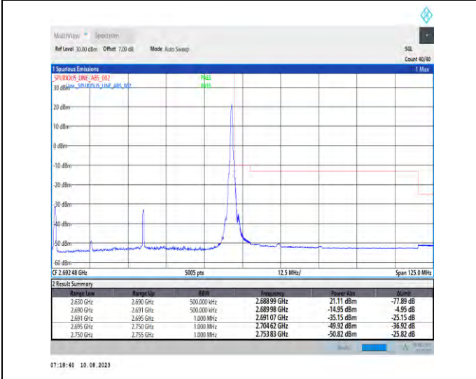
1-N41-PC3-30-60-H-5-CP-QPSK-Edge_1RB_Right-1@161-Ant1-1--PASS-see graph
