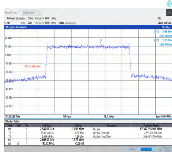
1-N41-PC3-30-90-M-7-CP-16QAM-Outer_Full-245@ 0-Ant1-87.347-90.720-≤90-PASS
