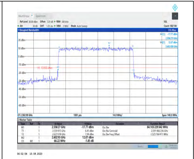
1-N41-PC3-30-70-M-1-DFT-QPSK-Outer_Full-180@ 0-Ant1-64.103-66.220-≤70-PASS
