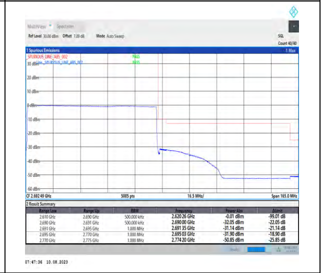
1-N41-PC3-30-80-H-6-CP-QPSK-Outer_Full-217@0-Ant1-1--PASS-see graph
