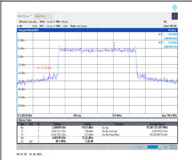
1-N41-PC3-30-50-M-8-CP-64QAM-Outer_Full-133 @0-Ant1-47.561-49.100-<=50-PASS
