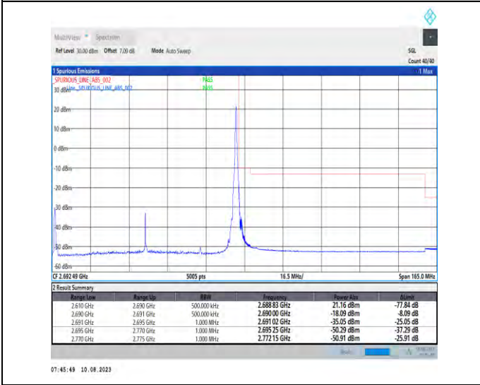
1-N41-PC3-30-80-H-5-CP-QPSK-Edge_1RB_Right-1@216-Ant1-1--PASS-see graph
