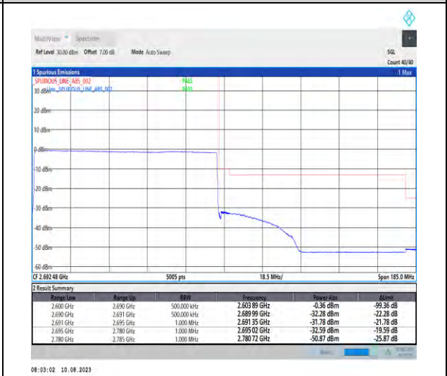
1-N41-PC3-30-90-H-6-CP-QPSK-Outer_Full-245@0-Ant1-1--PASS-see graph
