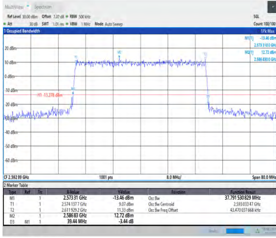
1-N41-PC3-30-40-M-7-CP-16QAM-Outer_Full-106@ @0-Ant1-37.792-39.440-<40-PASS
