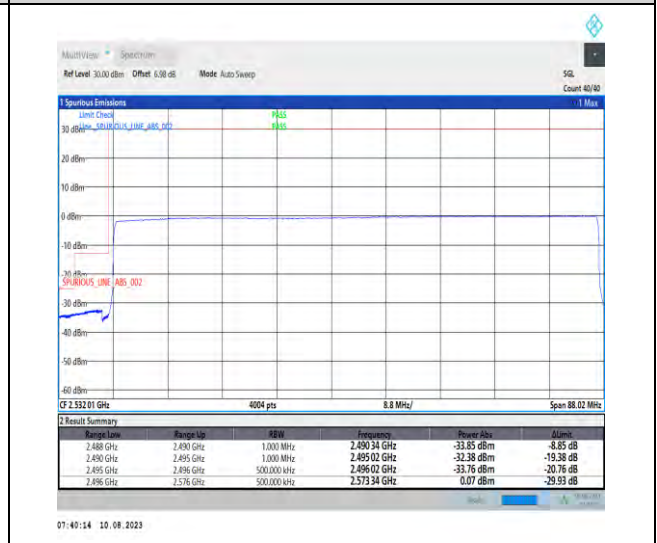
1-N41-PC3-30-80-L-6-CP-QPSK-Outer_Full-217@0-Ant1-1--PASS-see graph
