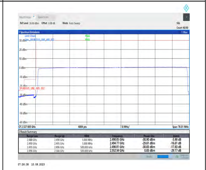
1-N41-PC3-30-70-L-6-CP-QPSK-Outer_Full-189@0-Ant1-1--PASS-see graph
