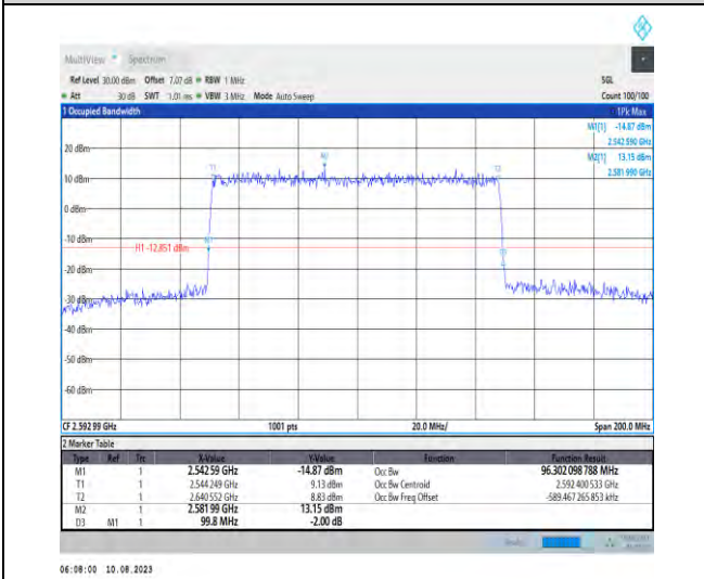
1-N41-PC3-30-100-M-3-DFT-16QAM-Outer_Full-270 @0-Ant1-96.302-99.800-≤100-PASS
