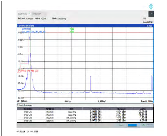
1-N41-PC3-30-90-L-1-DFT-PI2BPSK-Edge_1RB_Left-1@0-Ant1-1--PASS-see graph
