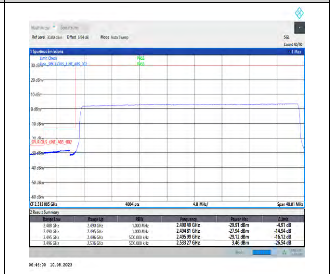
1-N41-PC3-30-40-L-6-CP-QPSK-Outer_Full-106@0-Ant1-1--PASS-see graph
