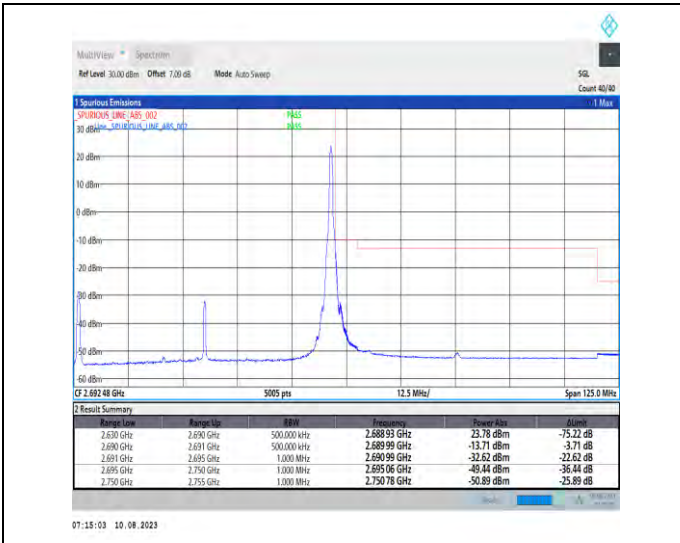
1-N41-PC3-30-60-H-2-DFT-PI2BPSK-Edge_1RB_Right-t-1@161-Ant1-1--PASS-see graph
