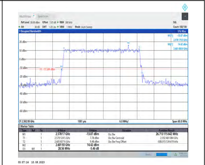
1-N41-PC3-30-30-M-3-DFT-16QAM-Outer_Full-75 @0-Ant1-26.713-28.560-<30-PASS
