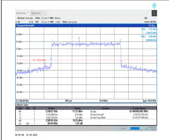
1-N41-PC3-30-70-M-6-CP-QPSK-Outer_Full-189@0 -Ant1-67.47-69.440-<=70-PASS
