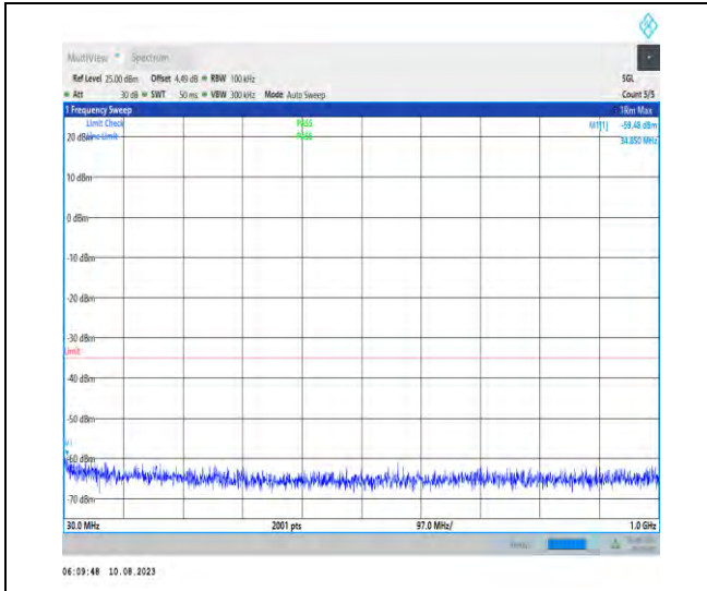
1-N41-PC3-30-100-M-1-N/A-DFT-PI2BPSK-Inner_1 RB_Left-1@1-30-1000-Ant1-32.91--59.48--35-PASS
