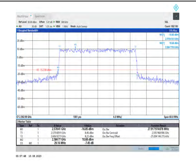
1-N41-PC3-30-30-M-7-CP-16QAM-Outer_Full-78@0 -Ant1-27.918-29.160-≤30-PASS
