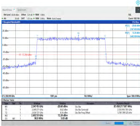
1-N41-PC3-30-90-M-8-CP-64QAM-Outer_Full-245 @0-Ant1-87.45-90.900-≤90-PASS
