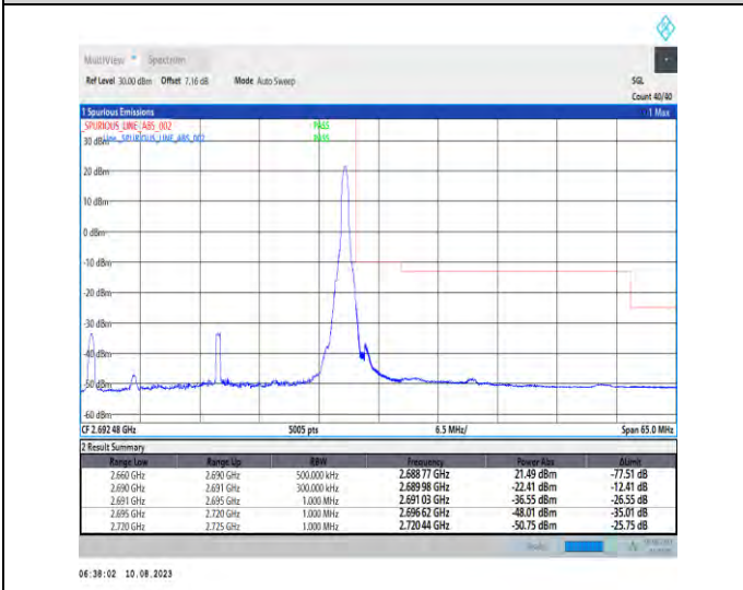
1-N41-PC3-30-30-H-5-CP-QPSK-Edge_1RB_Right-1@77-Ant1-1--PASS-see graph
