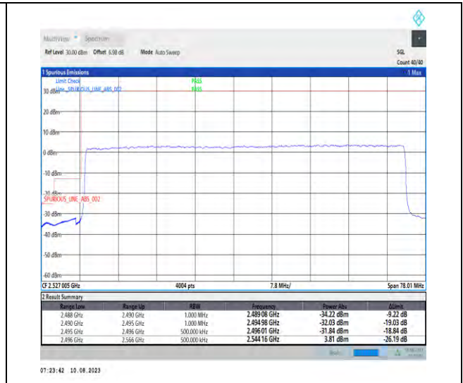
1-N41-PC3-30-70-L-3-DFT-PI2BPSK-Outer_Full-180@0-Ant1-1--PASS-see graph
