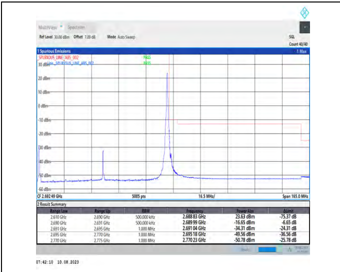
1-N41-PC3-30-80-H-2-DFT-PI2BPSK-Edge_1RB_Right-t-1@216-Ant1-1--PASS-see graph
