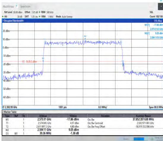
1-N41-PC3-30-40-M-9-CP-256QAM-Outer_Full-106@ @0-Ant1-37.852-39.360-<40-PASS
