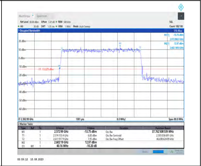
1-N41-PC3-30-40-M-6-CP-QPSK-Outer_Full-106@ -Ant1-37.763-40.160-<40-PASS
