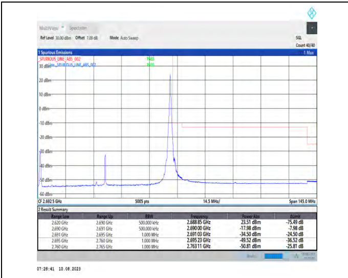
1-N41-PC3-30-70-H-2-DFT-PI2BPSK-Edge_1RB_Right-t-1@188-Ant1-1--PASS-see graph
