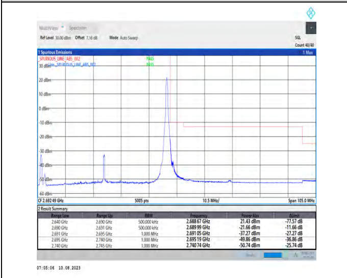
1-N41-PC3-30-50-H-5-CP-QPSK-Edge_1RB_Right-1@132-Ant1-1--PASS-see graph
