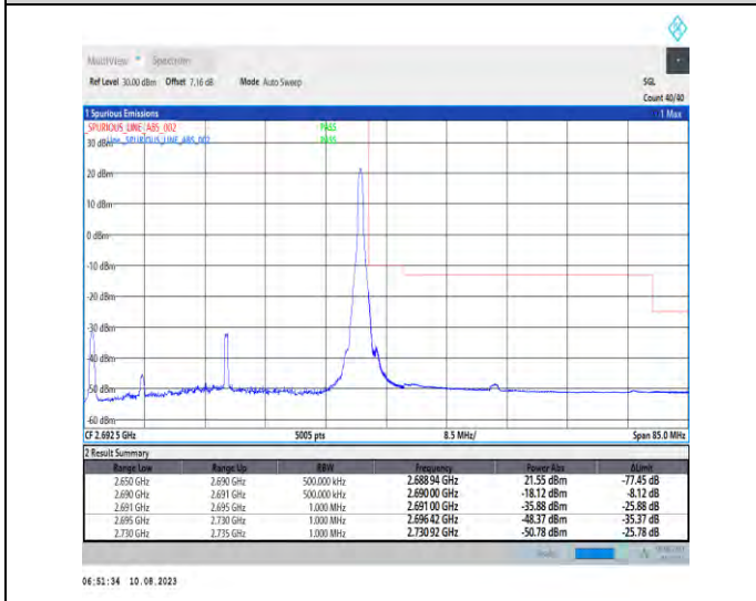
1-N41-PC3-30-40-H-5-CP-QPSK-Edge_1RB_Right-1@105-Ant1-1--PASS-see graph
