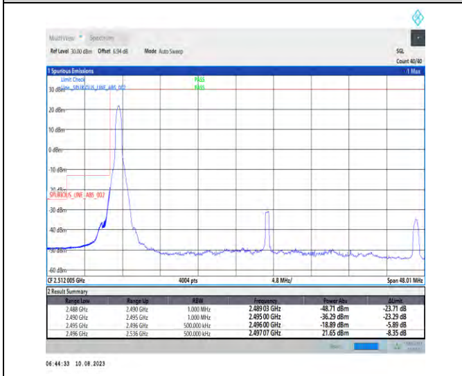
1-N41-PC3-30-40-L-4-CP-QPSK-Edge_1RB_Left-1@0-Ant1-1--PASS-see graph
