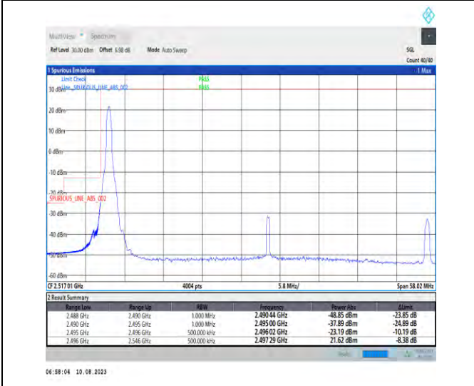
1-N41-PC3-30-50-L-4-CP-QPSK-Edge_1RB_Left-1@0-Ant1-1--PASS-see graph
