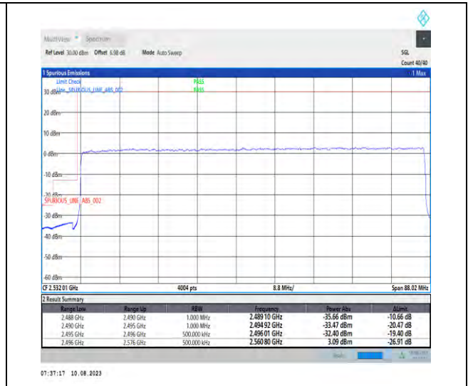
1-N41-PC3-30-80-L-3-DFT-PI2BPSK-Outer_Full-216@0-Ant1-1--PASS-see graph
