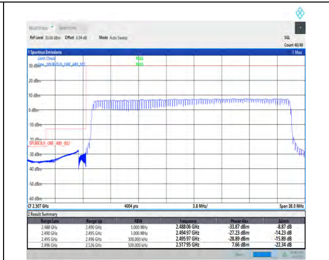
1-N41-PC3-30-30-L-3-DFT-PI2BPSK-Outer_Full-75@0-Ant1-1--PASS-see graph
