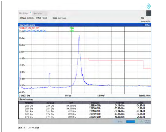
1-N41-PC3-30-40-H-2-DFT-PI2BPSK-Edge_1RB_Right-t-1@105-Ant1-1--PASS-see graph
