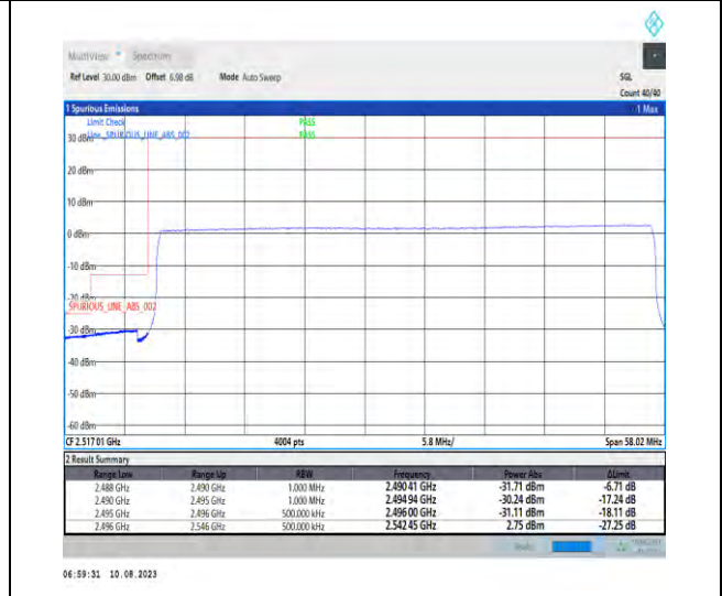
1-N41-PC3-30-50-L-6-CP-QPSK-Outer_Full-133@0-Ant1-1--PASS-see graph
