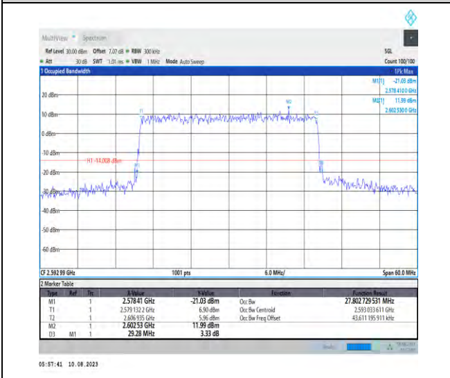
1-N41-PC3-30-30-M-6-CP-QPSK-Outer_Full-78@0- Ant1-27.803-29.280-≤30-PASS
