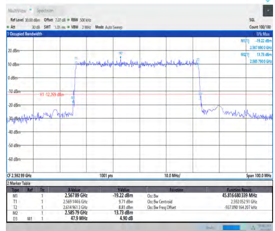
1-N41-PC3-30-50-M-1-DFT-QPSK-Outer_Full-128@ @0-Ant1-45.817-47.900-<50-PASS
