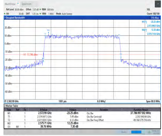
1-N41-PC3-30-40-M-8-CP-64QAM-Outer_Full-106@ @0-Ant1-37.787-39.760-<40-PASS
