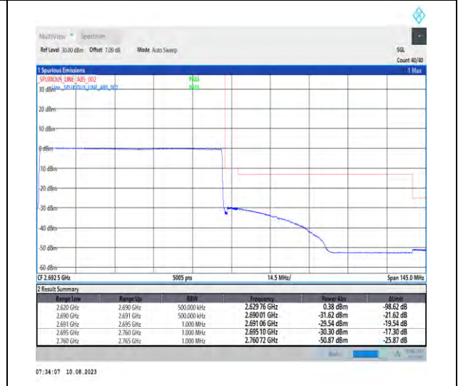
1-N41-PC3-30-70-H-6-CP-QPSK-Outer_Full-189@0-Ant1-1--PASS-see graph
