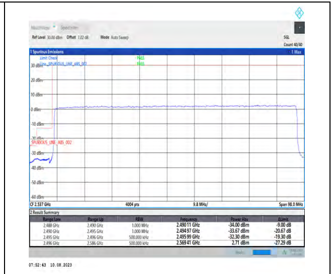
1-N41-PC3-30-90-L-3-DFT-PI2BPSK-Outer_Full-240@0-Ant1-1--PASS-see graph
