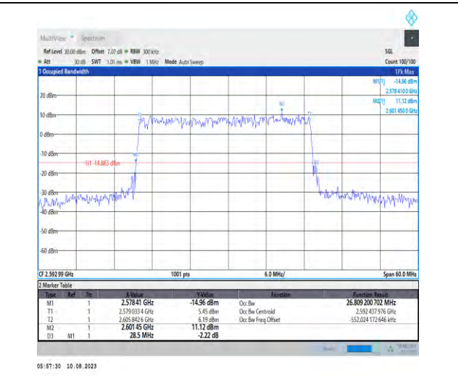
1-N41-PC3-30-30-M-5-DFT-256QAM-Outer_Full-75 @0-Ant1-26.809-28.500-≤30-PASS
