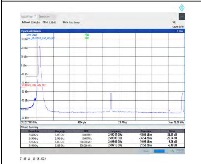
1-N41-PC3-30-70-L-4-CP-QPSK-Edge_1RB_Left-1@0-Ant1-1--PASS-see graph
