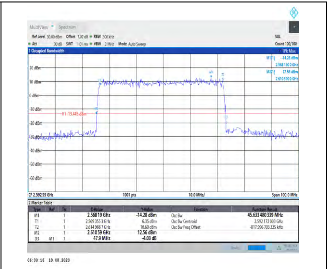
1-N41-PC3-30-50-M-3-DFT-16QAM-Outer_Full-128 @0-Ant1-45.633-47.900-≤50-PASS
