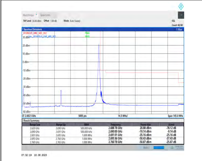
1-N41-PC3-30-70-H-5-CP-QPSK-Edge_1RB_Right-1@188-Ant1-1--PASS-see graph
