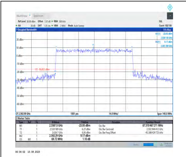
1-N41-PC3-30-70-M-8-CP-64QAM-Outer_Full-189 @0-Ant1-67.51-69.720-<=70-PASS
