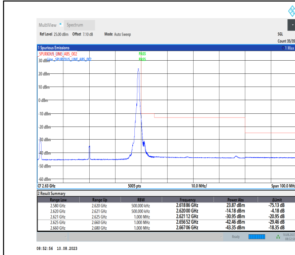
1-N38-PC3-30-40-H-2-DFT-PI2BPSK-Edge_1RB_Right t1@105-Ant1-1--PASS-see graph
