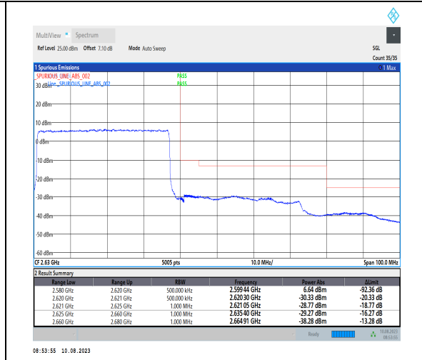
1-N38-PC3-30-40-H-3-DFT-PI2BPSK-Outer_Full-1 00@0-Ant1-1--PASS-see graph
