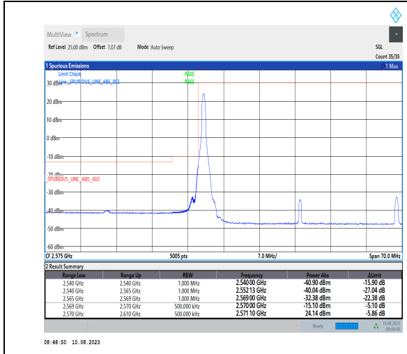
1-N38-PC3-30-40-L-1-DFT-PI2BPSK-Edge_1RB_Left -1@0-Ant1-1--PASS-see graph
