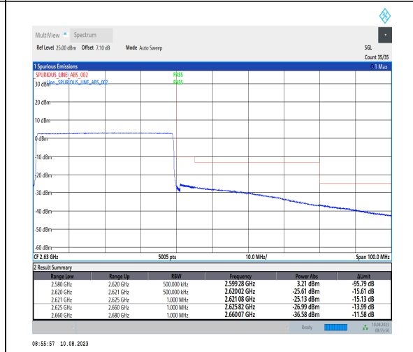
1-N38-PC3-30-40-H-6-CP-QPSK-Outer_Full-106 @0-Ant1-1--PASS-see graph
