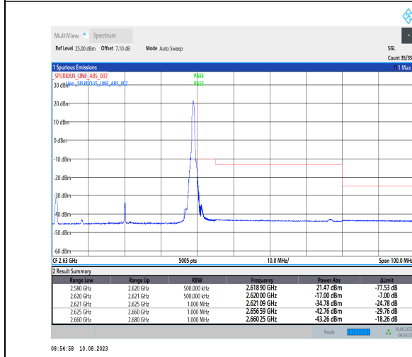
1-N38-PC3-30-40-H-5-CP-QPSK-Edge_1RB_Right-1 @105-Ant1-1--PASS-see graph
