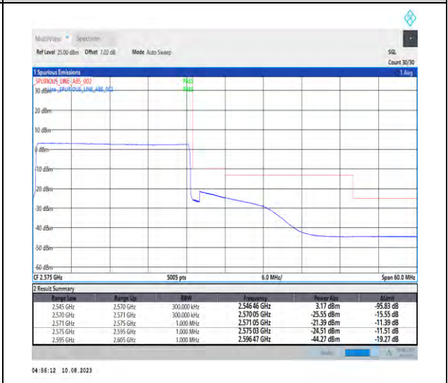
1-N7-PC3-15-25-H-6-CP-QPSK-Outer_Full-133@0-Ant1-1--PASS-see graph
