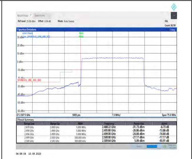
1-N7-PC3-15-30-L-3-DFT-PI2BPSK-Outer_Full-160@0-Ant1-1--PASS-see graph
