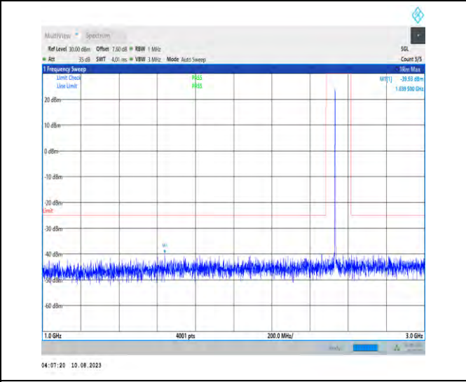
1-N7-PC3-15-40-H-1-N/A-DFT-PI2BPSK-Inner_1RB_Left-1@1-1000-3000-Ant1-2836.00--39.93--25-PASS
