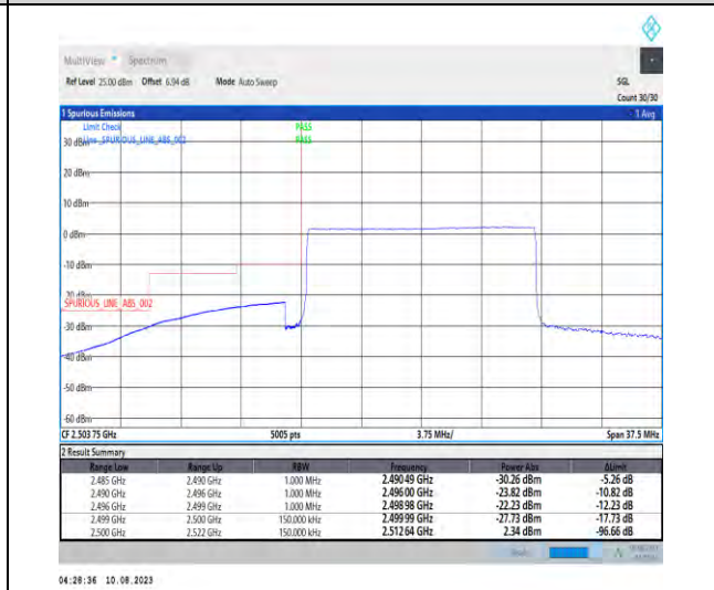
1-N7-PC3-15-15-L-6-CP-QPSK-Outer_Full-79@0-Ant1-1--PASS-see graph
