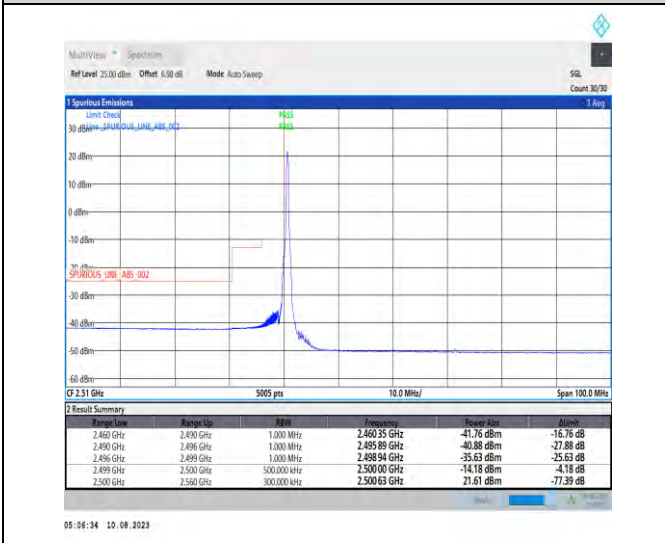
1-N7-PC3-15-40-L-4-CP-QPSK-Edge_1RB_Left-1@0-Ant1-1--PASS-see graph
