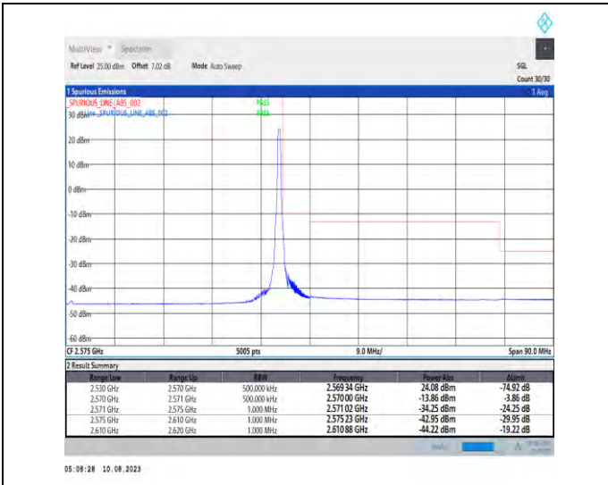
1-N7-PC3-15-40-H-2-DFT-PI2BPSK-Edge_1RB_Right-1@215-Ant1-1--PASS-see graph
