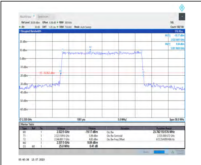
1-N7-PC3-15-25-M-9-CP-256QAM-Outer_Full-133@ 0-Ant1-23.782-25.000-≤25-PASS
