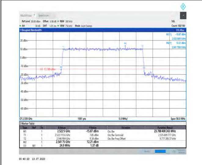
1-N7-PC3-15-25-M-7-CP-16QAM-Outer_Full-133@0- Ant1-23.788-24.900-≤25-PASS
