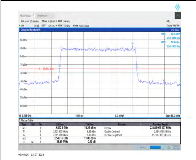
1-N7-PC3-15-25-M-5-DFT-256QAM-Outer_Full-128 @0-Ant1-22.884-23.850-≤25-PASS
