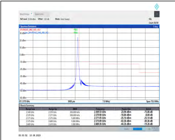
1-N7-PC3-15-30-H-2-DFT-PI2BPSK-Edge_1RB_Right-1@159-Ant1-1--PASS-see graph
