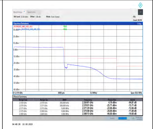
1-N7-PC3-15-20-H-6-CP-QPSK-Outer_Full-106@0-Ant1-1--PASS-see graph
