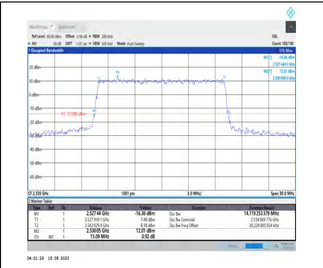
1-N7-PC3-15-15-M-8-CP-64QAM-Outer_Full-79@0- Ant1-14.119-15.090-≤15-PASS
