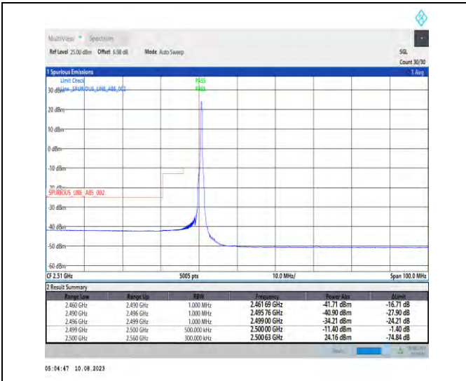
1-N7-PC3-15-40-L-1-DFT-PI2BPSK-Edge_1RB_Left-1@0-Ant1-1--PASS-see graph
