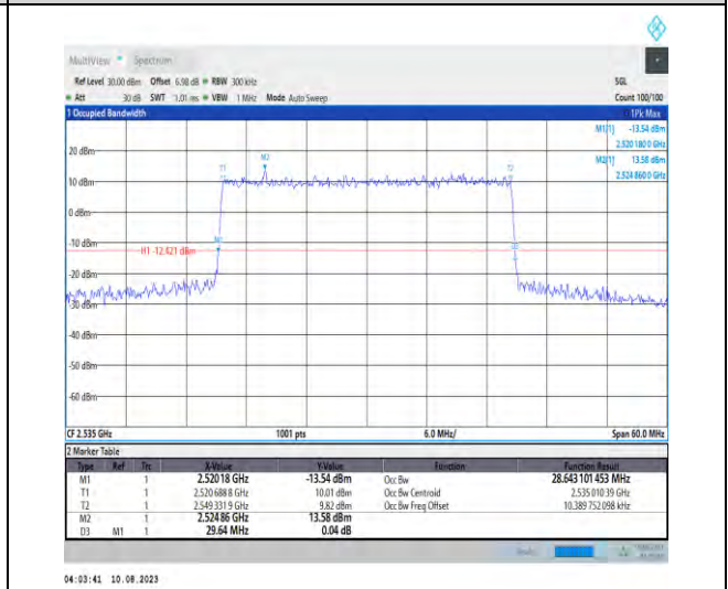
1-N7-PC3-15-30-M-3-DFT-16QAM-Outer_Full-160 @0-Ant1-28.643-29.640-≤30-PASS
