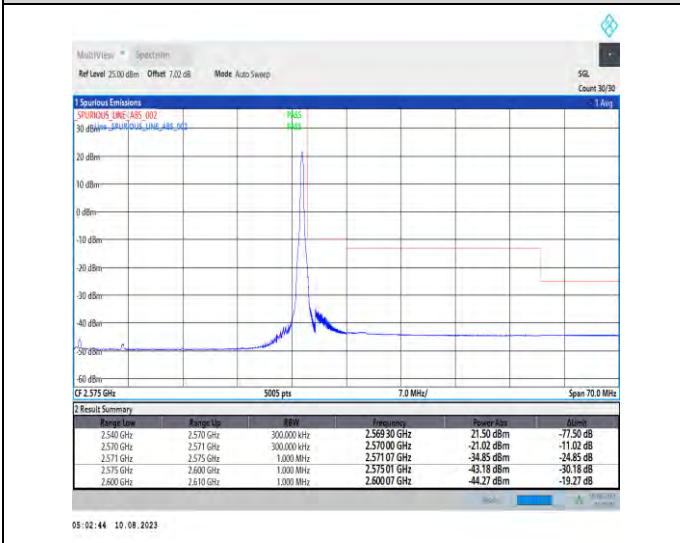
1-N7-PC3-15-30-H-5-CP-QPSK-Edge_1RB_Right-1@159-Ant1-1--PASS-see graph
