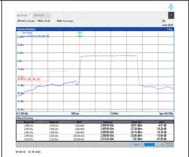
1-N7-PC3-15-20-L-3-DFT-PI2BPSK-Outer_Full-100@0-Ant1-1--PASS-see graph
