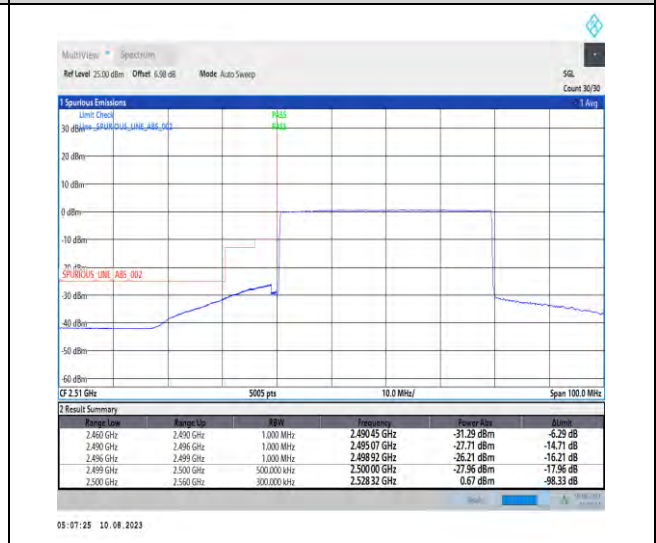
1-N7-PC3-15-40-L-6-CP-QPSK-Outer_Full-216@0-Ant1-1--PASS-see graph
