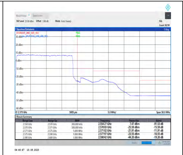
1-N7-PC3-15-20-H-3-DFT-PI2BPSK-Outer_Full-100@0-Ant1-1--PASS-see graph
