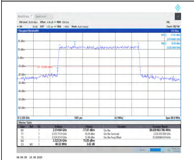
1-N7-PC3-15-40-M-1-DFT-QPSK-Outer_Full-216@ 0-Ant1-38.64-40.320-≤40-PASS
