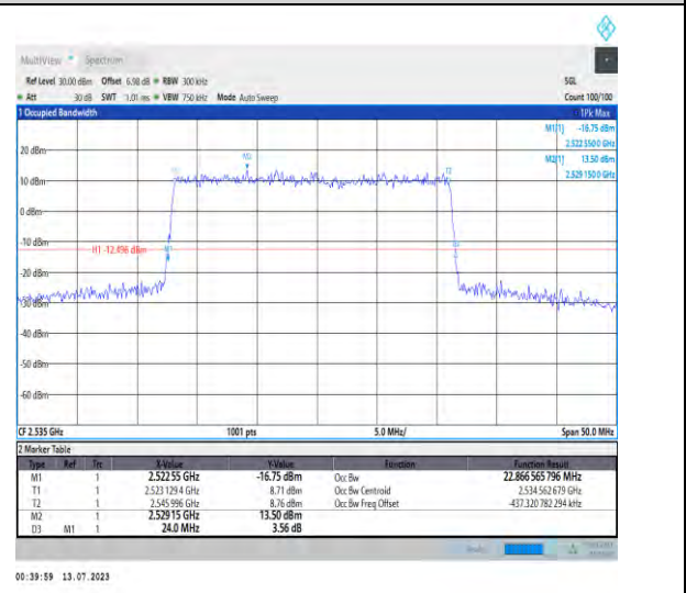
1-N7-PC3-15-25-M-4-DFT-64QAM-Outer_Full-128@ 0-Ant1-22.867-24.000-≤25-PASS
