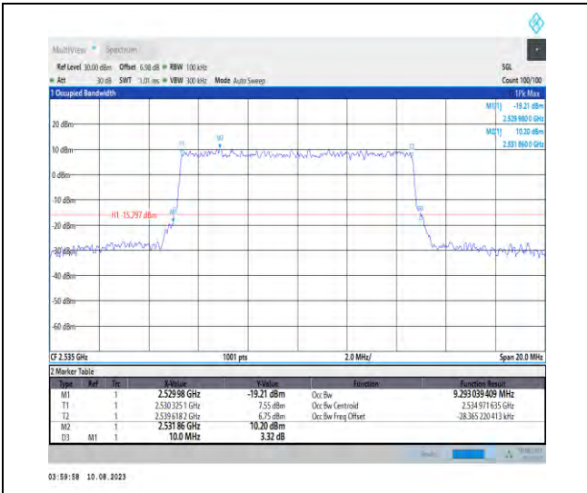
1-N7-PC3-15-10-M-8-CP-64QAM-Outer_Full-52@0 -Ant1-9.293-10.000-≤10-PASS
