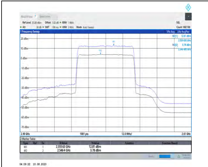
1-N7-PC3-15-40-H-1-DFT-256QAM-Outer_Full-216 @0-Ant1-9.03-100%-0.00-9.03-PASS-≤13
