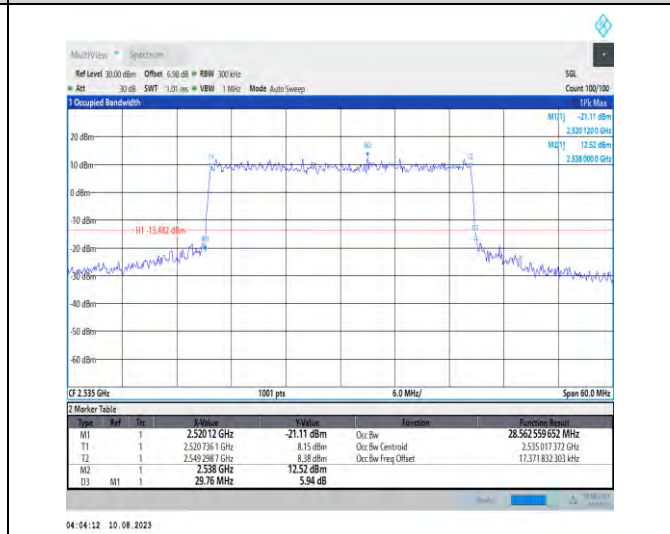
1-N7-PC3-15-30-M-7-CP-16QAM-Outer_Full-160@0- Ant1-28.563-29.760-≤30-PASS
