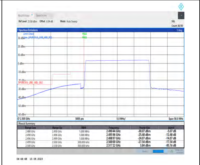
1-N7-PC3-15-20-L-6-CP-QPSK-Outer_Full-106@0-Ant1-1--PASS-see graph
