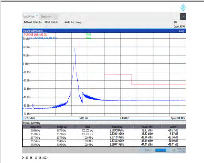
1-N7-PC3-15-10-H-5-CP-QPSK-Edge_1RB_Right-1@51-Ant1-1--PASS-see graph
