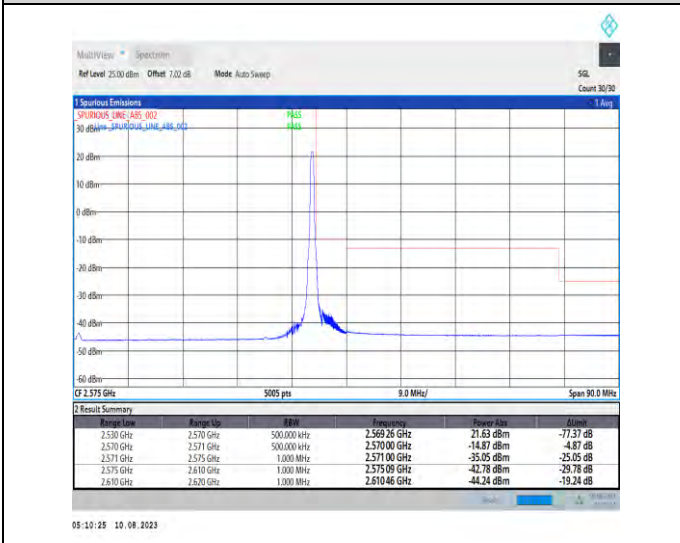
1-N7-PC3-15-40-H-5-CP-QPSK-Edge_1RB_Right-1@215-Ant1-1--PASS-see graph
