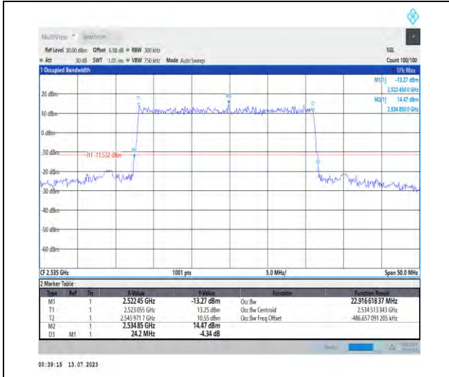
1-N7-PC3-15-25-M-1-DFT-QPSK-Outer_Full-128@ 0-Ant1-22.917-24.200-≤25-PASS
