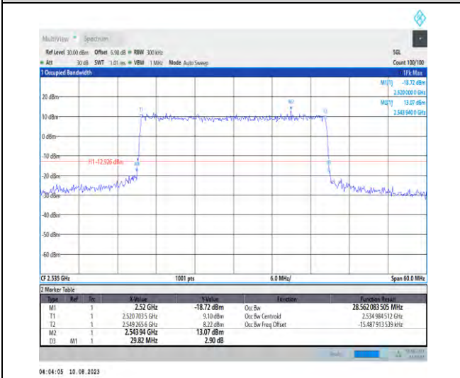
1-N7-PC3-15-30-M-6-CP-QPSK-Outer_Full-160@0- Ant1-28.562-29.820-≤30-PASS
