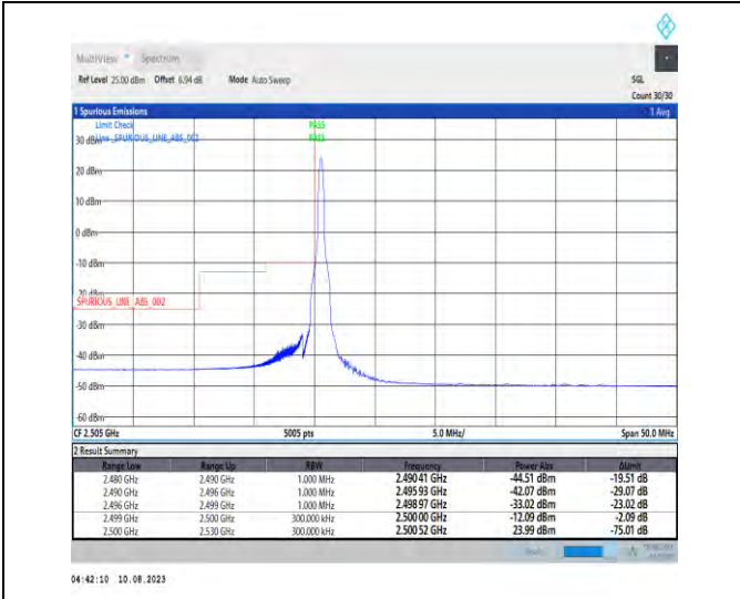
1-N7-PC3-15-20-L-1-DFT-PI2BPSK-Edge_1RB_Left-1@0-Ant1-1--PASS-see graph
