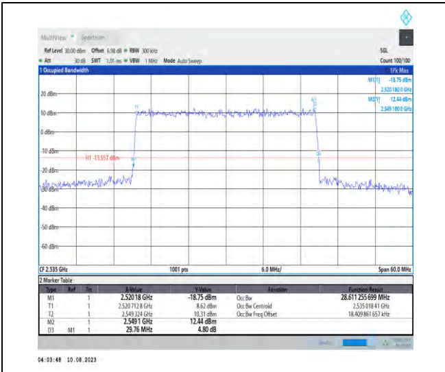
1-N7-PC3-15-30-M-4-DFT-64QAM-Outer_Full-160@ 0-Ant1-28.611-29.760-≤30-PASS
