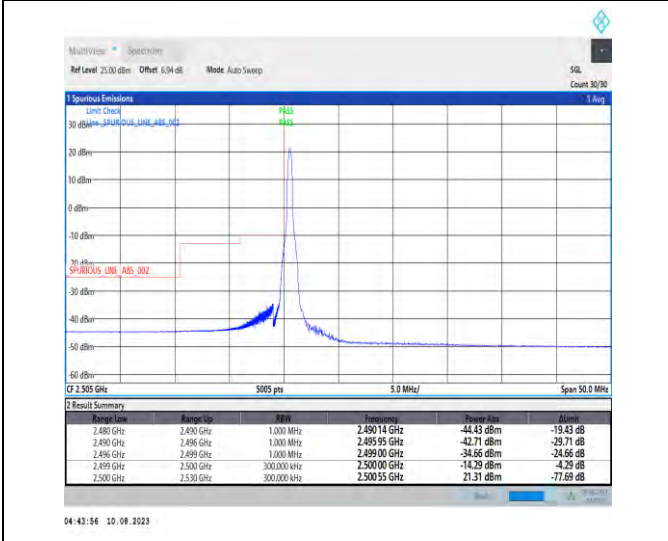
1-N7-PC3-15-20-L-4-CP-QPSK-Edge_1RB_Left-1@0-Ant1-1--PASS-see graph
