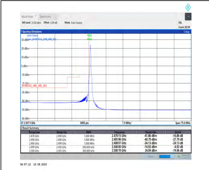
1-N7-PC3-15-30-L-1-DFT-PI2BPSK-Edge_1RB_Left-1@0-Ant1-1--PASS-see graph
