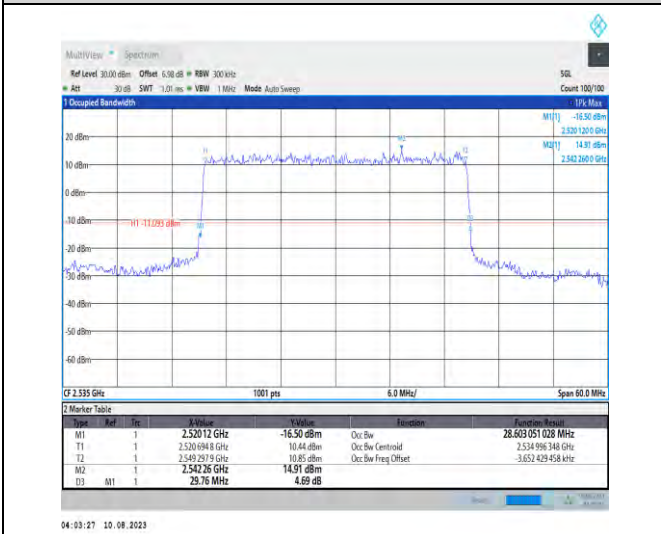
1-N7-PC3-15-30-M-2-DFT-PI2BPSK-Outer_Full-160 @0-Ant1-28.603-29.760-≤30-PASS
