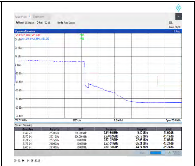
1-N7-PC3-15-30-H-3-DFT-PI2BPSK-Outer_Full-160@0-Ant1-1--PASS-see graph
