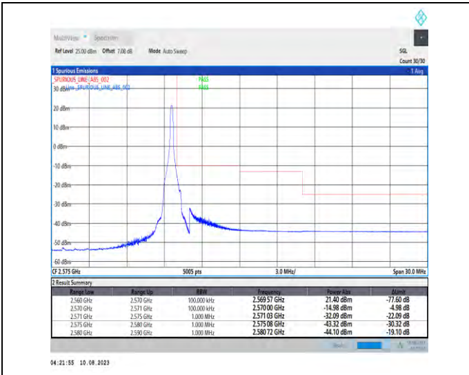
1-N7-PC3-15-10-H-2-DFT-PI2BPSK-Edge_1RB_Right-1@51-Ant1-1--PASS-see graph
