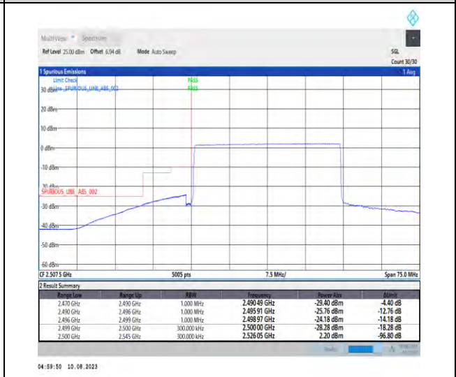
1-N7-PC3-15-30-L-6-CP-QPSK-Outer_Full-160@0-Ant1-1--PASS-see graph
