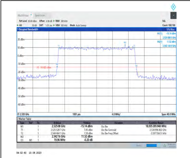
1-N7-PC3-15-20-M-6-CP-QPSK-Outer_Full-106@0-Ant1-18.935-19.960-<=20-PASS
