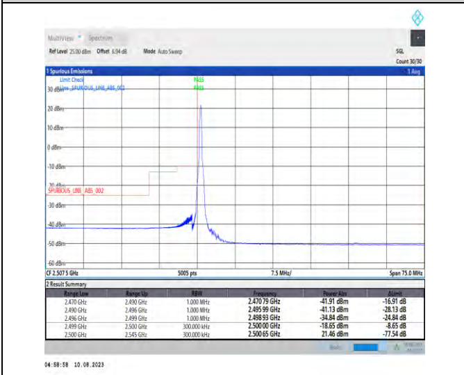
1-N7-PC3-15-30-L-4-CP-QPSK-Edge_1RB_Left-1@0-Ant1-1--PASS-see graph
