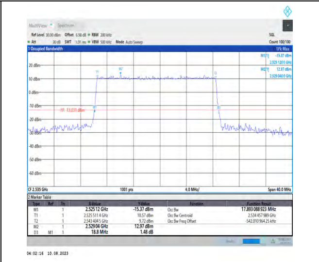
1-N7-PC3-15-20-M-3-DFT-16QAM-Outter_Full-100@0-Ant1-17.893-18.800-≤20-PASS
