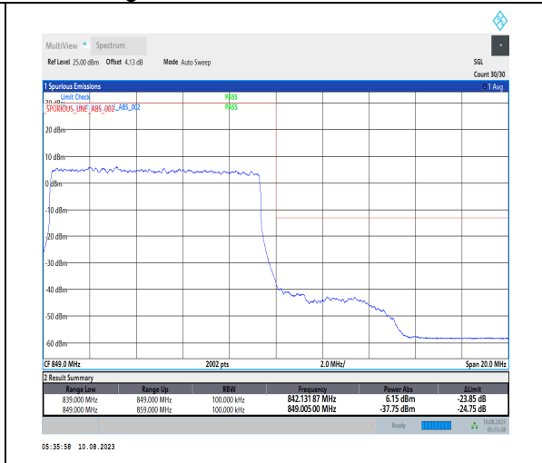
1-N5-PC3-15-10-H-3-DFT-PI2BPSK-Outer_Full-50@0-Ant1-1-seegraph-PASS-see graph
