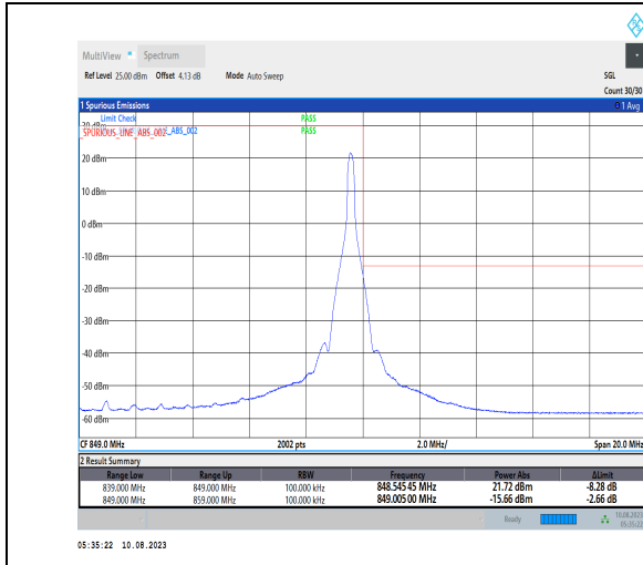
1-N5-PC3-15-10-H-2-DFT-PI2BPSK-Edge_1RB_Right-1@51-Ant1-1-seegraph-PASS-see graph
