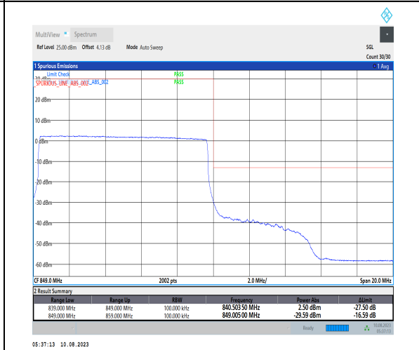
1-N5-PC3-15-10-H-6-CP-QPSK-Outer_Full-52@0-Ant1-1-seegraph-PASS-see graph
