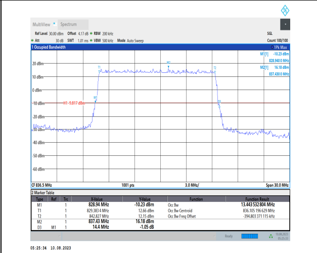
1-N5-PC3-15-15-M-2-DFT-PI2BPSK-Outer_Full-75@0-Ant1-13.444-14.400-≤15-PASS
