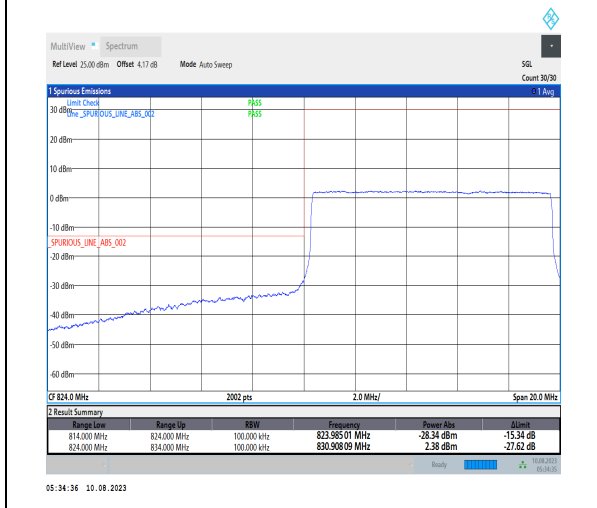
1-N5-PC3-15-10-L-6-CP-QPSK-Outer_Full-52@0-Ant1-1-seegraph-PASS-see graph
