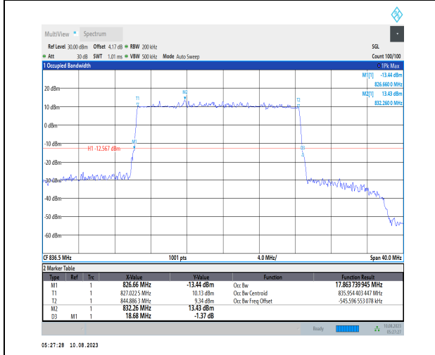
1-N5-PC3-15-20-M-4-DFT-64QAM-Outer_Full-100@0-Ant1-17.864-18.680-≤20-PASS
