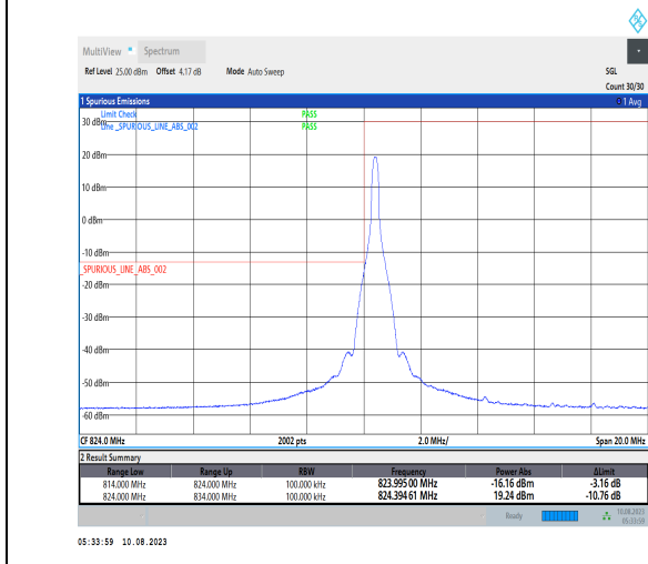
1-N5-PC3-15-10-L-4-CP-QPSK-Edge_1RB_Left-1@0-Ant1-1-seegraph-PASS-see graph
