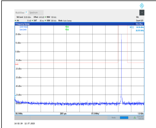
1-N5-PC3-15-20-H-1-N/A-DFT-PI2BPSK-Inner_1RB _Left-1@1-30-1000-Ant1-30.97--54.36--13-PASS
