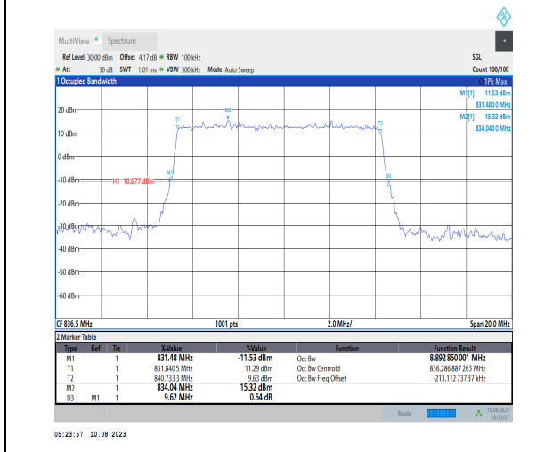
1-N5-PC3-15-10-M-2-DFT-PI2BPSK-Outer_Full-50@0-Ant1-8.893-9.620-≤10-PASS
