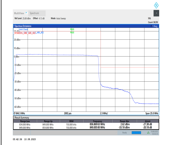
1-N5-PC3-15-15-H-6-CP-QPSK-Outer_Full-79@0-Ant1-1-seegraph-PASS-see graph
