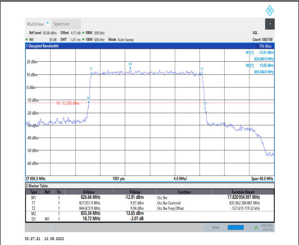
1-N5-PC3-15-20-M-3-DFT-16QAM-Outer_Full-100@0-Ant1-17.821-18.720-≤20-PASS
