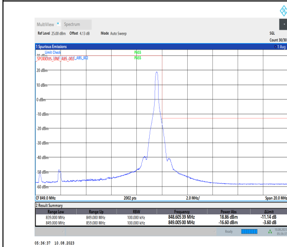
1-N5-PC3-15-10-H-5-CP-QPSK-Edge_1RB_Right-1@51-Ant1-1-seegraph-PASS-see graph
