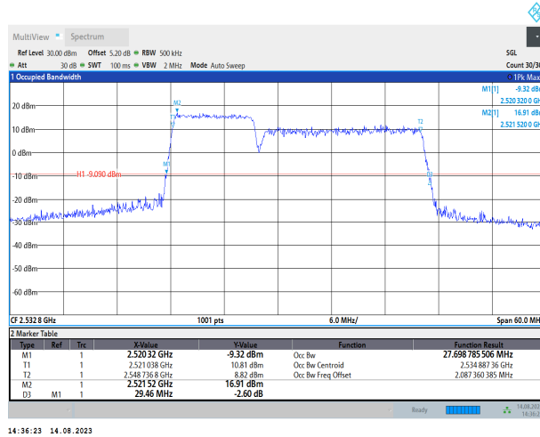
7-7-10MHz-20MHz-16QAM-16QAM-21006-21150-50RB#0-100RB#0
