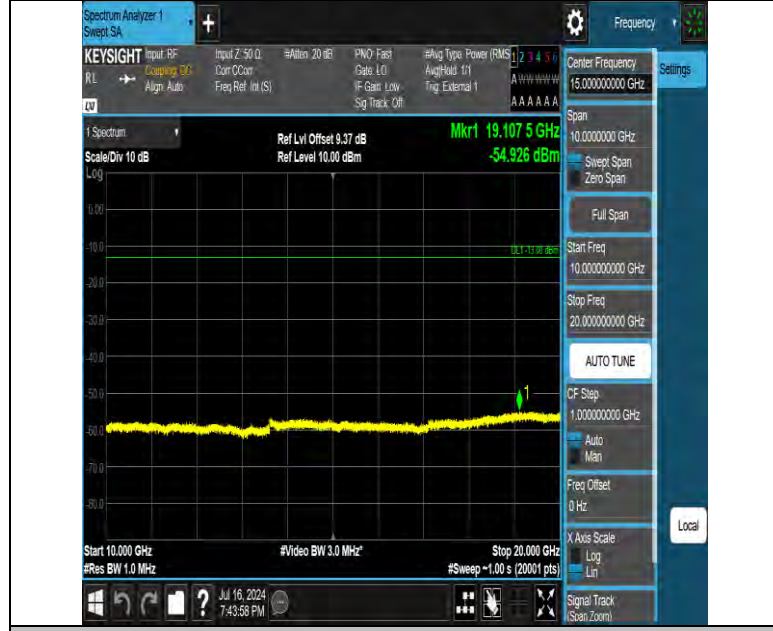
Band42 15MHz QPSK 42590 1RB#0 10000~20000 10000~20000
