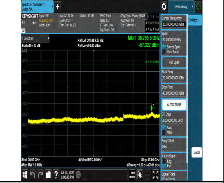
Band42 10MHz QPSK 42590 1RB#0 20000~40000 20000~40000
