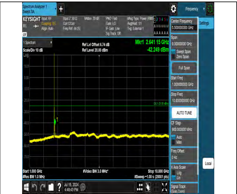
Band41 10MHz QPSK 40620 1RB#0 1000~10000 1000~10000
