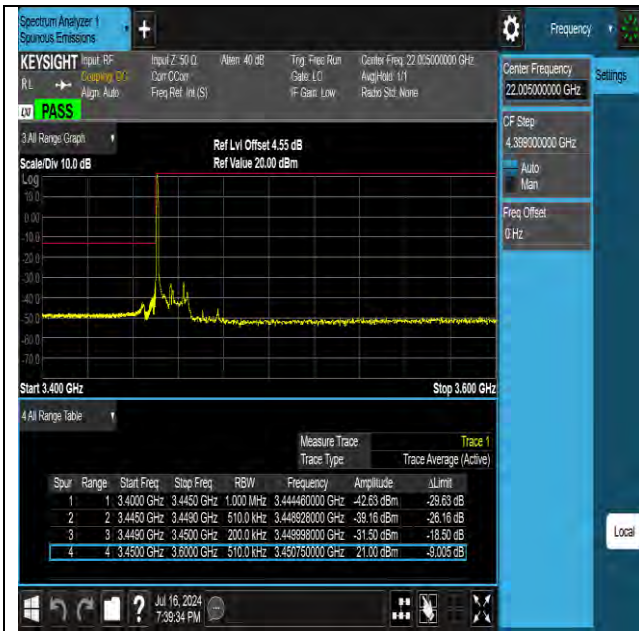
Band42 15MHz 16QAM 42165 1RB#0
