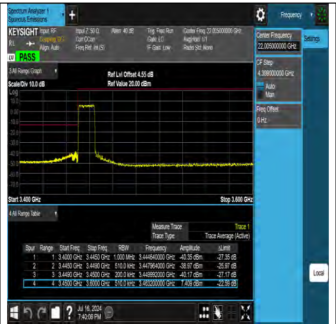
Band42 15MHz 16QAM 42165 75RB#0
