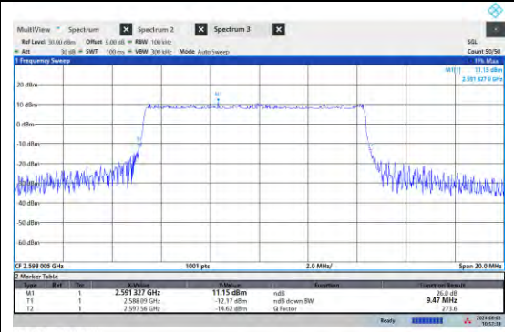
NTNV-N41-PC3-15-10-M-DFT-64QAM-Outer_Full-Ant1-PASS
