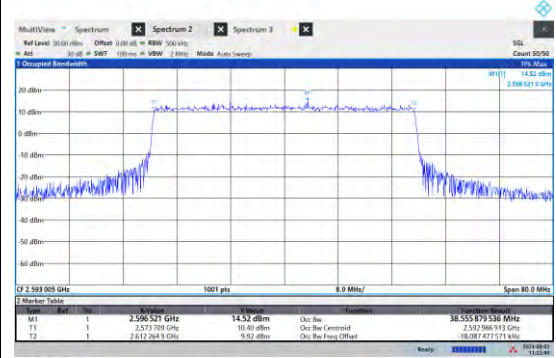
NTNV-N41-PC3-15-40-M-DFT-QPSK-Outer_Full-Ant1-PASS
