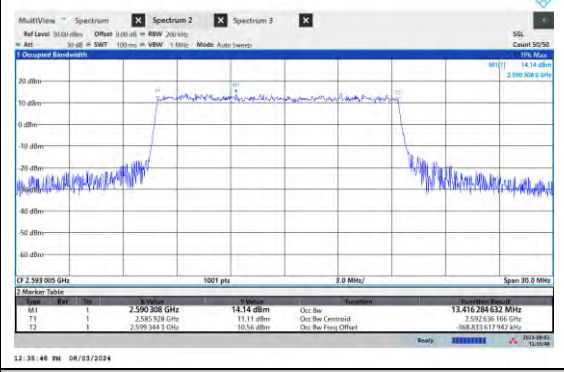
NTN-N41-PC3-15-15-M-DFT-PI2BPSK-Outer_Fu II-Ant1-PASS
