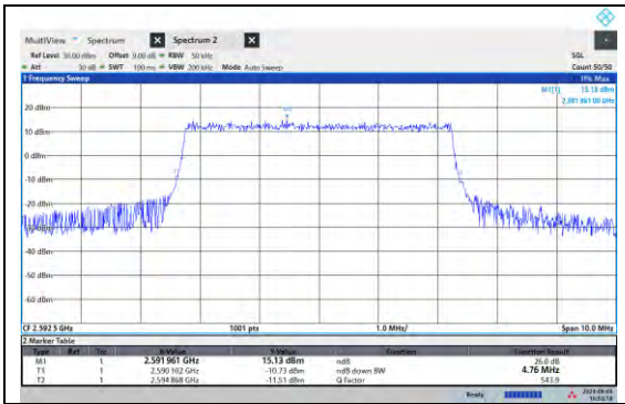
NTNV-N41-PC3-15-10-M-DFT-16QAM-Outer_Full-Ant1-PASS
