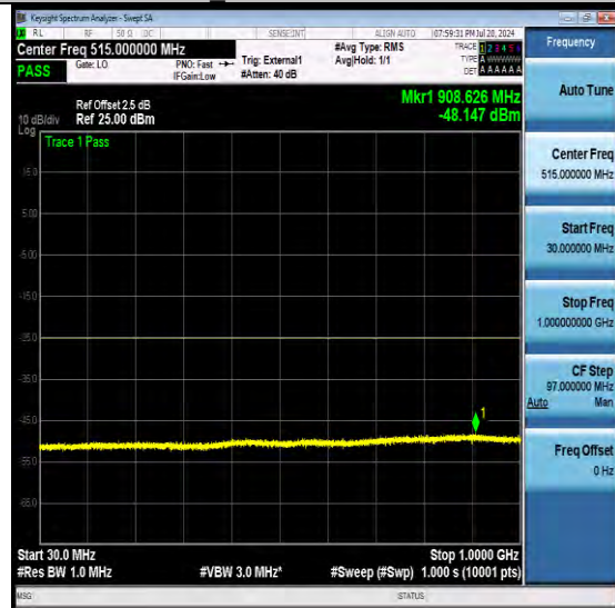
NTN-N41-PC3-30-10-L-DFT-QPSK-Edge_1RB Left-Ant1-PASS
