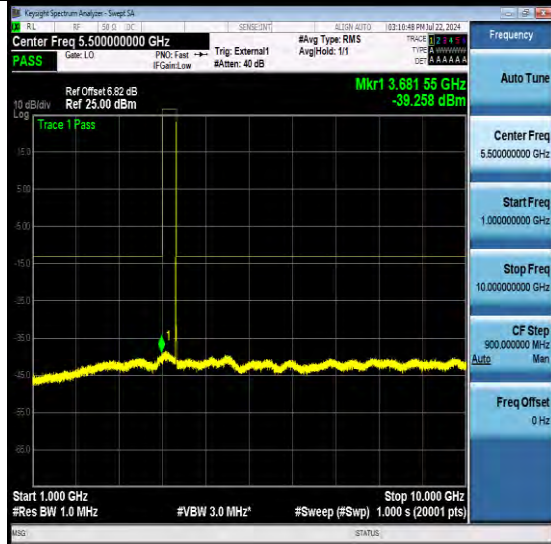
NTNV-N77-3700-3980-PC3-30-10-H-DFT-QPSK-Edge_1RB Left-Ant1-PASS
