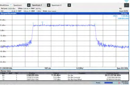
NTNV-N41-PC3-15-30-M-DFT-16QAM-Outer_Full-Ant1-PASS
