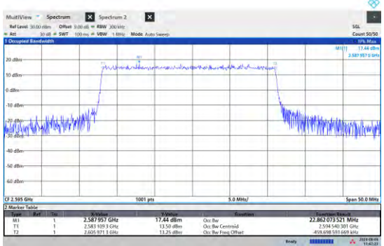
NTNV-N38-PC3-15-25-M-DFT-PI2BPSK-Outer_Fu II-Ant1-PASS
