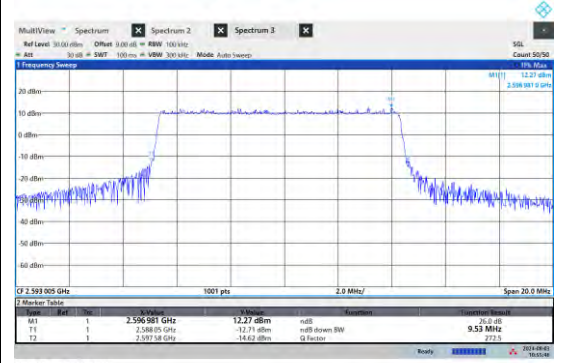
NTNV-N41-PC3-15-10-M-DFT-QPSK-Outer_Full-Ant1-PASS
