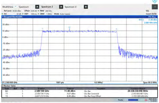
NTNV-N41-PC3-15-30-M-DFT-64QAM-Outer_Full-Ant1-PASS
