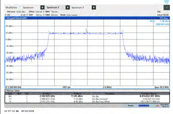
NTN-N41-PC3-15-10-M-DFT-64QAM-Outer_Full-Ant1-PASS
