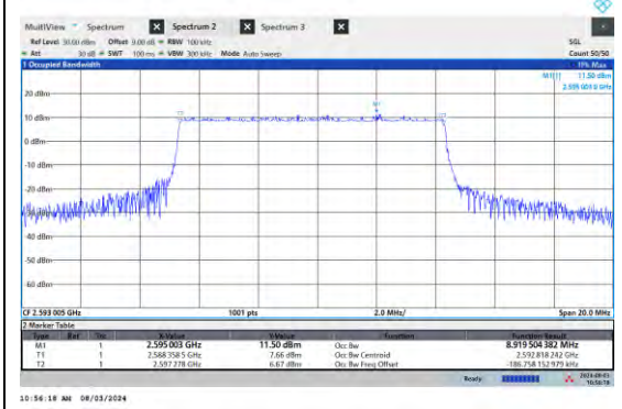
NTN-N41-PC3-15-10-M-DFT-16QAM-Outer_Full-Ant1-PASS
