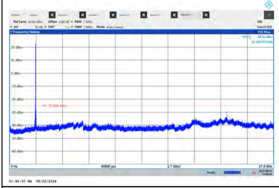
NTNV-N41-PC3-15-50-H-DFT-QPSK-Edge_1RB_ Left-Ant1-PAS
