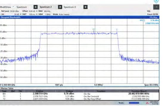
NTNV-N41-PC3-15-30-M-DFT-256QAM-Outer_Ful I-Ant1-PASS
