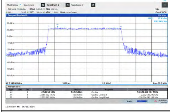
NTN-N41-PC3-15-15-M-DFT-QPSK-Outer_Full-Ant1-PASS
