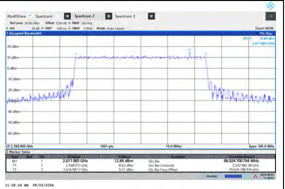
NTNV-N41-PC3-15-50-M-DFT-QPSK-Outer_Full-Ant1-PASS
