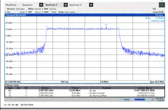
NTN-N41-PC3-15-15-M-DFT-16QAM-Outer_Full-Ant1-PASS
