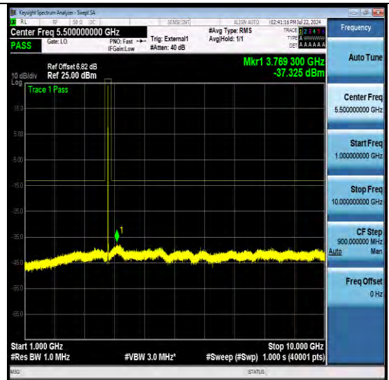
NTNV-N77-3450-3550-PC2-30-10-M-DFT-QPSK-Edge 1RB Left-Ant1-PASS
