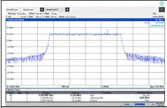
NTNV-N41-PC3-15-10-M-DFT-256QAM-Outer_Full-Ant1-PASS
