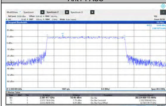
NTNV-N41-PC3-15-40-M-DFT-16QAM-Outer_Full-Ant1-PASS
