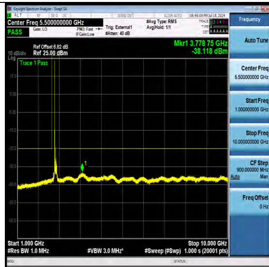
NTN-N41-PC3-30-100-H-DFT-QPSK-Edge_1RB Left-Ant1-PASS
