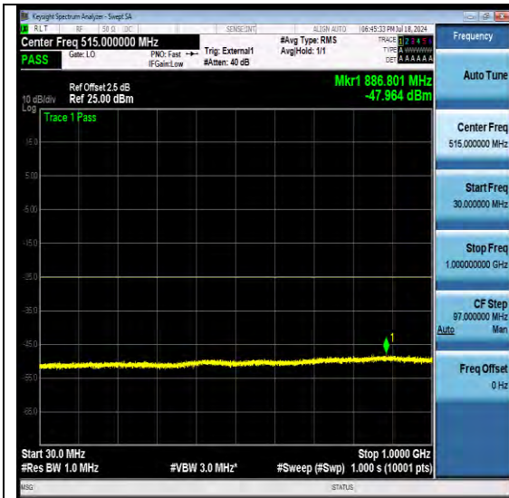
NTN-N41-PC3-30-100-H-DFT-QPSK-Edge_1RB Left-Ant1-PASS
