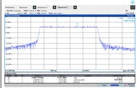
NTNV-N41-PC3-15-10-M-DFT-PI2BPSK-Outer_Full-Ant1-PASS
