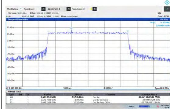
NTNV-N41-PC3-40-M-DFT-PI2BPSK-Outer_Full-Ant1-PASS
