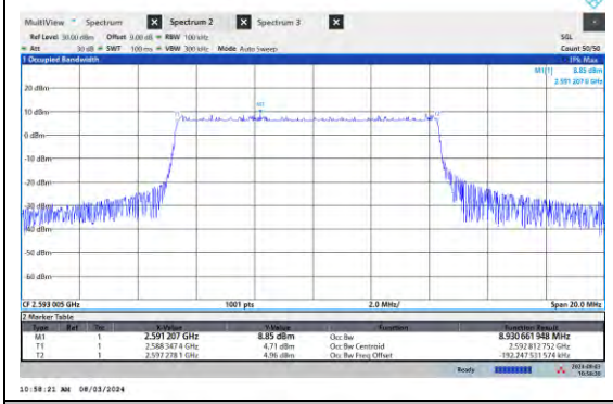
NTN-N41-PC3-15-10-M-DFT-256QAM-Outer_Full-I-Ant1-PASS
