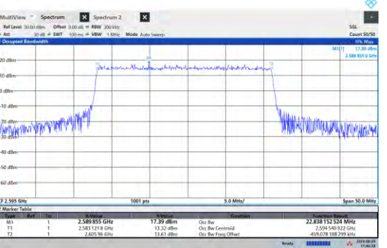
NTNV-N38-PC3-15-25-M-DFT-QPSK-Outer_Full-Ant1-PASS
