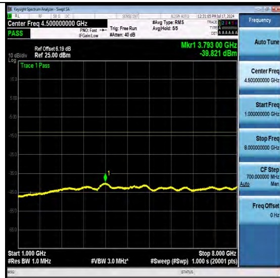
NTNV-N12-PC3-15-15-M-DFT-QPSK-Edge_1RB_Left-Ant1-PASS
