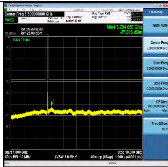
NTNV-N77-3450-3550-PC2-30-30-H-DFT-QPSK-Edge 1RB Left-Ant1-PASS
