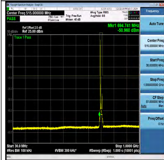
NTNV-N12-PC3-15-15-H-DFT-QPSK-Edge_1RB_Left-Ant1-PASS
