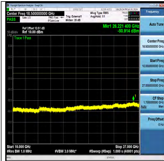
NTNV-N41-PC3-30-60-H-DFT-QPSK-Edge_1RB_Left-Ant1-PASS
