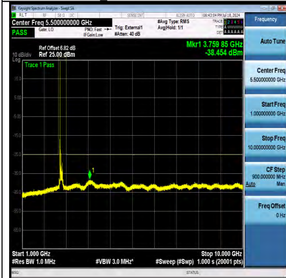
NTN-N41-PC3-30-100-M-DFT-QPSK-Edge_1RB Left-Ant1-PASS
