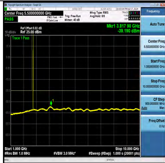
NTN-N7-PC3-15-5-H-DFT-QPSK-Edge_1RB_Lef t-Ant1-PASS
