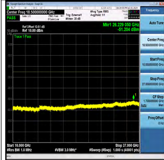
NTNV-N41-PC3-30-80-M-DFT-QPSK-Edge_1RB_ Left-Ant1-PASS
