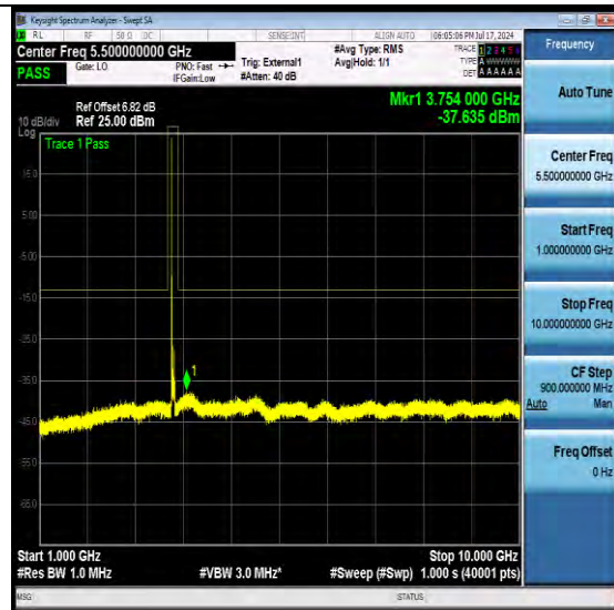
NTNV-N77-3450-3550-PC2-30-60-M-DFT-QPSK-Edge 1RB Left-Ant1-PASS
