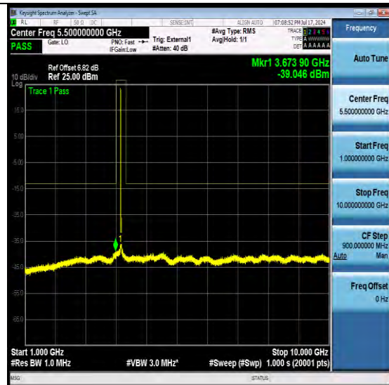
NTNV-N77-3700-3980-PC2-30-30-M-DFT-QPSK-Edge 1RB Left-Ant1-PASS
