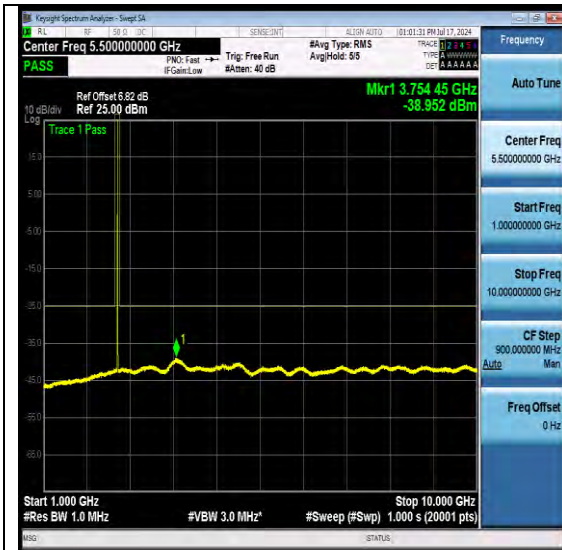
NTN-N7-PC3-15-5-M-DFT-QPSK-Edge_1RB_Le ft-Ant1-PASS
