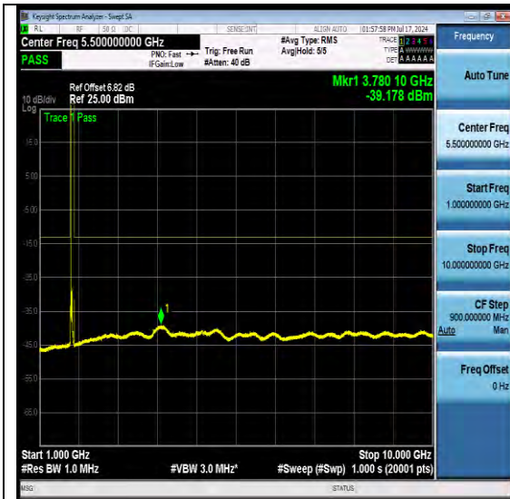
NTNV-N66-PC3-15-40-L-DFT-QPSK-Edge_1RB_Left-Ant1-PASS
