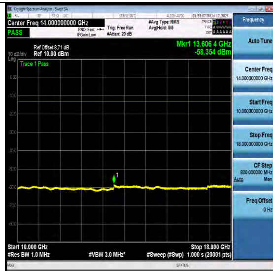
NTNV-N66-PC3-15-40-L-DFT-QPSK-Edge_1RB_Left-Ant1-PASS
