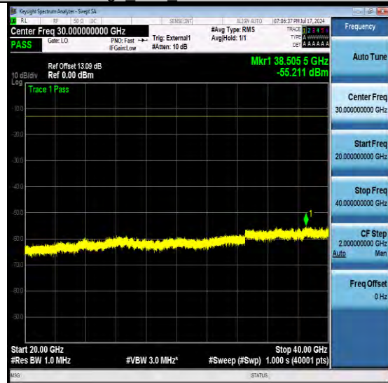
NTNV-N77-3700-3980-PC2-30-30-L-DFT-QPSK-E dge_1RB_Left-Ant1-PASS
