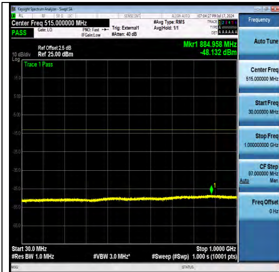
NTNV-N77-3700-3980-PC2-30-30-L-DFT-QPSK-E dge_1RB_Left-Ant1-PASS
