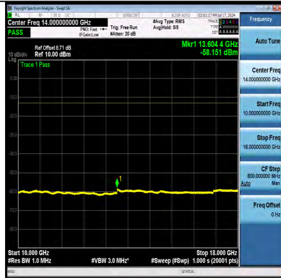
NTNV-N66-PC3-15-40-H-DFT-QPSK-Edge_1RB_Left-Ant1-PASS
