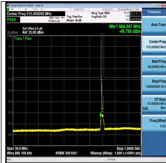
NTNV-N12-PC3-15-15-M-DFT-QPSK-Edge_1RB_Left-Ant1-PASS
