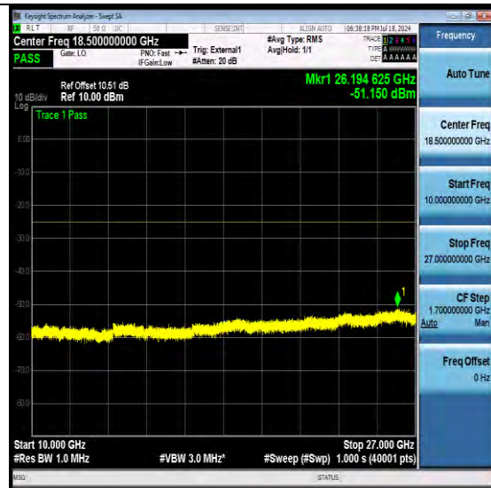
NTN-N41-PC3-30-80-H-DFT-QPSK-Edge_1RB_Left-Ant1-PASS
