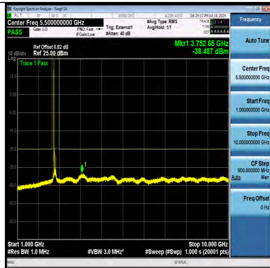
NTNV-N41-PC3-30-80-M-DFT-QPSK-Edge_1RB_ Left-Ant1-PASS
