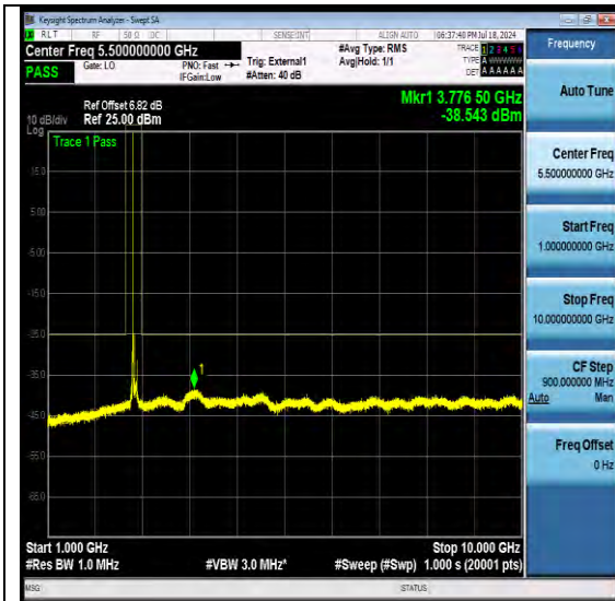
NTN-N41-PC3-30-80-H-DFT-QPSK-Edge_1RB_Left-Ant1-PASS
