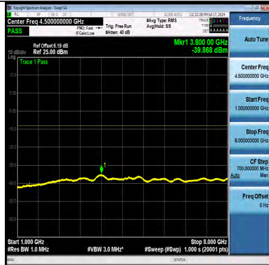
NTNV-N12-PC3-15-15-H-DFT-QPSK-Edge_1RB_Left-Ant1-PASS
