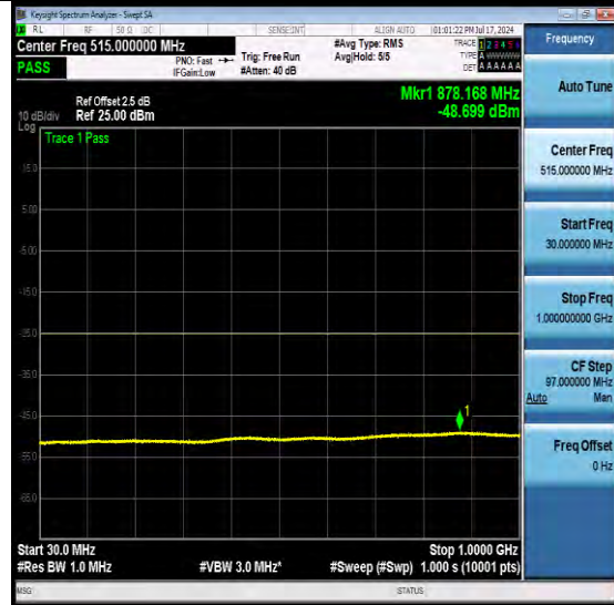
NTNV-N7-PC3-15-5-M-DFT-QPSK-Edge_1RB_Le ft-Ant1-PASS
