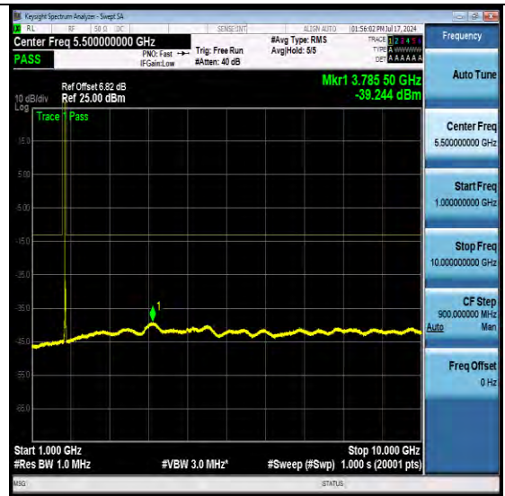
NTNV-N66-PC3-15-20-H-DFT-QPSK-Edge_1RB_Left-Ant1-PASS
