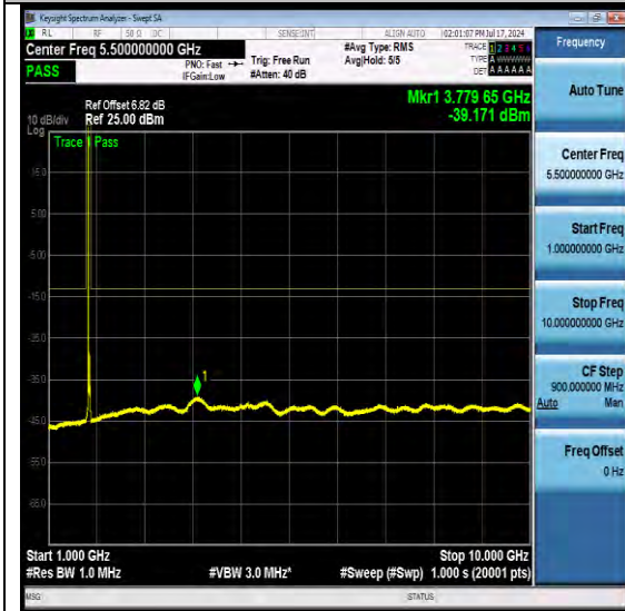
NTNV-N66-PC3-15-40-H-DFT-QPSK-Edge_1RB_Left-Ant1-PASS
