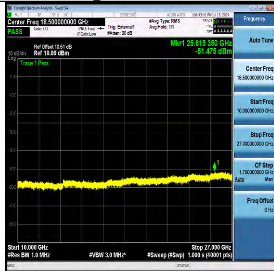
NTN-N41-PC3-30-100-M-DFT-QPSK-Edge_1RB Left-Ant1-PASS
