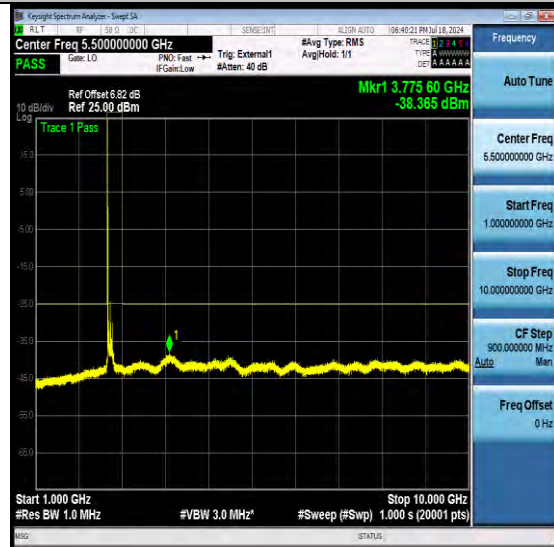
NTN-N41-PC3-30-100-L-DFT-QPSK-Edge_1RB_Left-Ant1-PASS
