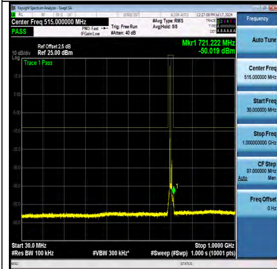
NTNV-N12-PC3-15-10-M-DFT-QPSK-Edge_1RB_Left-Ant1-PASS
