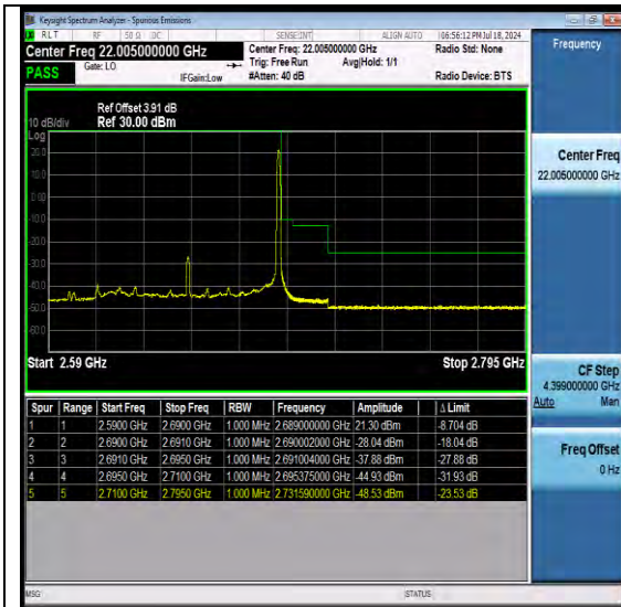
NTNV-N41-PC3-30-80-H-DFT-QPSK-Edge_1RB_Right-Ant1-PASS
