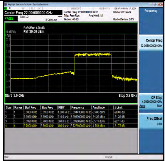
NTNV-N77-3700-3980-PC2-30-60-L-DFT-QPSK-Outer Full-Ant1-PASS
