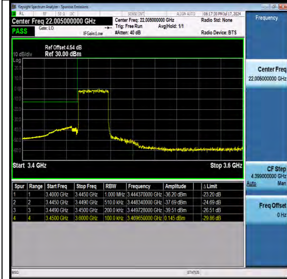
NTNV-N77-3450-3550-PC2-30-30-L-DFT-QPSK-Outer_Full-Ant1-PASS
