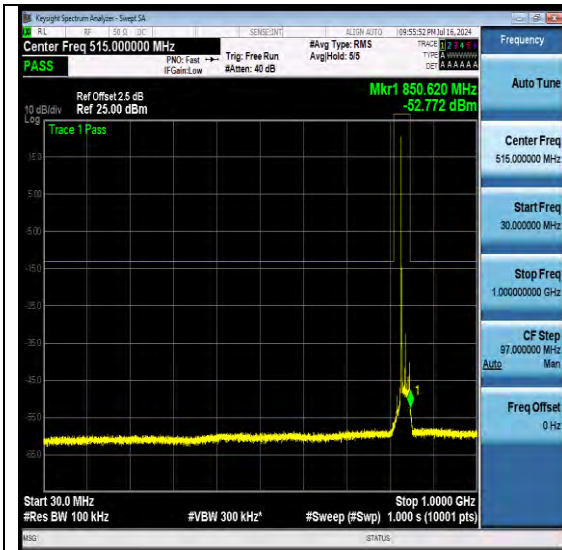
NTN-N26-824-849-PC3-15-20-H-DFT-QPSK-Edge_1RB_Left-Ant1-PASS
