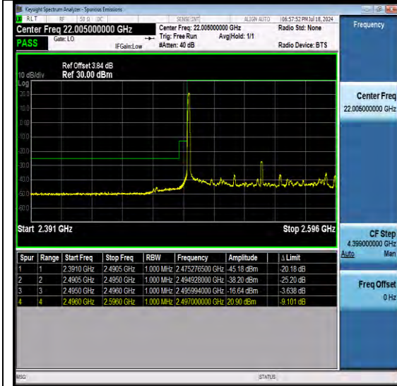
NTNV-N41-PC3-30-100-L-DFT-QPSK-Edge_1RB_Left-Ant1-PASS
