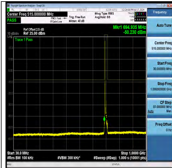
NTNV-N12-PC3-15-10-L-DFT-QPSK-Edge_1RB_Left-Ant1-PASS
