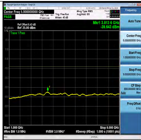
NTN-N26-824-849-PC3-15-20-H-DFT-QPSK-Edge_1RB_Left-Ant1-PASS
