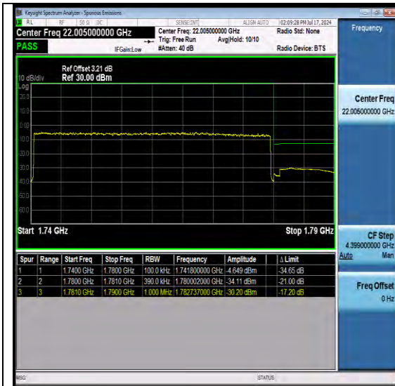
NTNV-N66-PC3-15-40-H-DFT-QPSK-Outer_Full-Ant1-PASS
