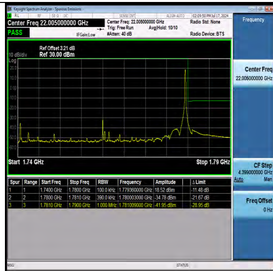
NTNV-N66-PC3-15-40-H-DFT-QPSK-Edge_1RB_Right-Ant1-PASS
