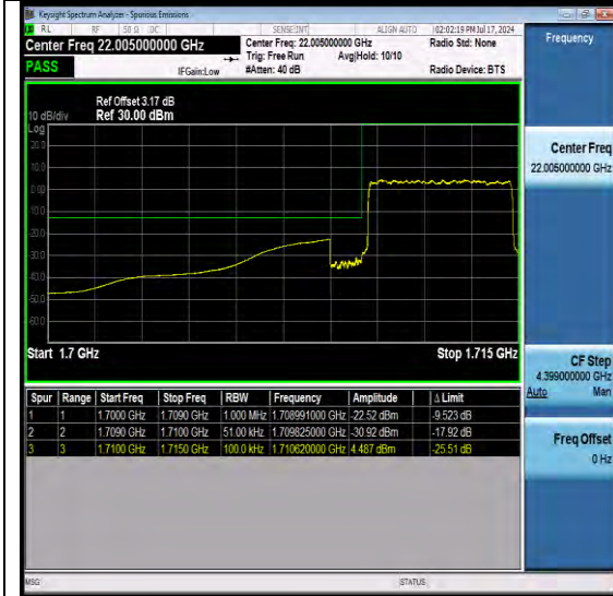
NTNV-N66-PC3-15-5-L-DFT-QPSK-Outer_Full-Ant1-PASS
