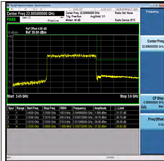
NTNV-N77-3450-3550-PC2-30-60-H-DFT-QPSK-Outer Full-Ant1-PASS
