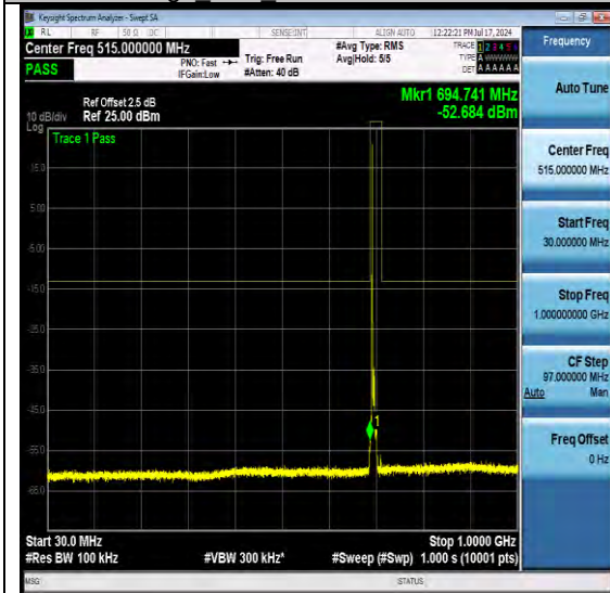
NTN-N12-PC3-15-5-L-DFT-QPSK-Edge_1RB_Left-Ant1-PASS
