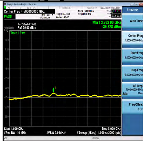
NTN-N12-PC3-15-5-L-DFT-QPSK-Edge_1RB_Left-Ant1-PASS
