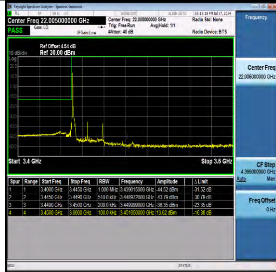
NTNV-N77-3450-3550-PC2-30-30-L-DFT-QPSK-Edge_1RB_Left-Ant1-PASS
