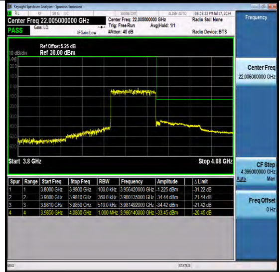
NTNV-N77-3700-3980-PC2-30-60-H-DFT-QPSK-Outer Full-Ant1-PASS
