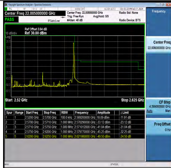
NTNV-N7-PC3-15-50-H-DFT-QPSK-Edge_1RB_Right-Ant1-PASS
