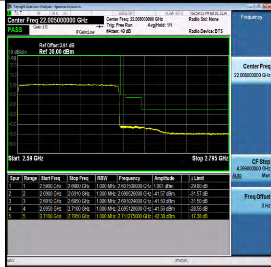
NTNV-N41-PC3-30-100-H-DFT-QPSK-Outer_Full-Ant1-PASS
