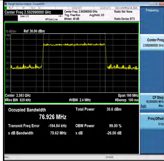
NTNV-N41-PC3-30-80-M-DFT-QPSK-Outer_Full-Ant1-PASS
