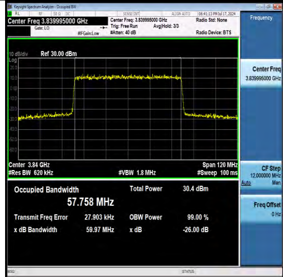
NTNV-N77-3700-3980-PC2-30-60-M-DFT-256QAM-M-Outer Full-Ant1-PASS
