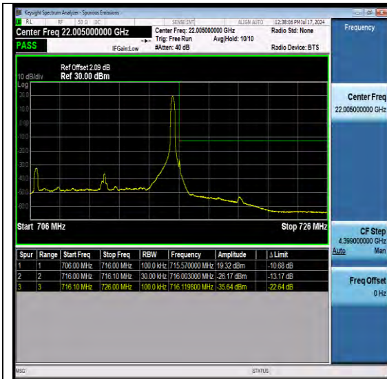
NTNV-N12-PC3-15-10-H-DFT-QPSK-Edge_1RB_Right-Ant1-PASS
