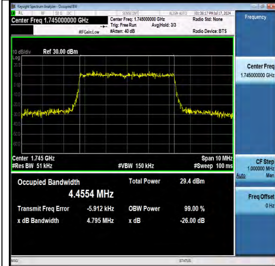
NTNV-N66-PC3-15-5-M-DFT-QPSK-Outer_Full-Ant1-PASS
