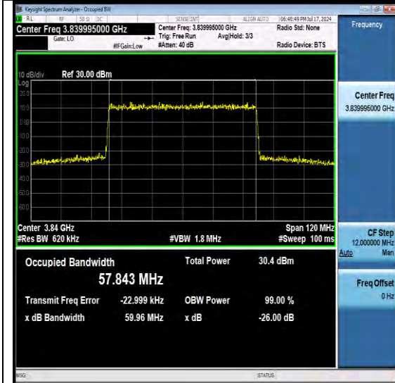
NTNV-N77-3700-3980-PC2-30-60-M-DFT-64QAM-Outer Full-Ant1-PASS
