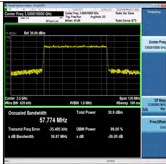
NTNV-N77-3450-3550-PC2-30-60-M-DFT-64QAM -Outer Full-Ant1-PASS
