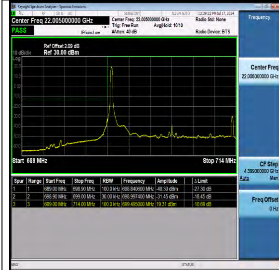
NTNV-N12-PC3-15-15-L-DFT-QPSK-Edge_1RB_Left-Ant1-PASS
