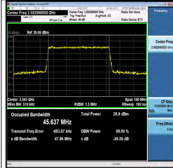
NTNV-N41-PC3-30-50-M-DFT-64QAM-Outer_Full-Ant1-PASS
