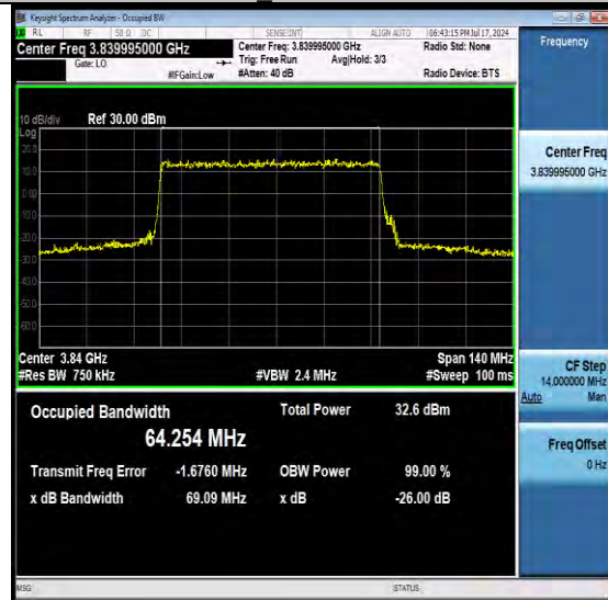
NTNV-N77-3700-3980-PC2-30-70-M-DFT-QPSK- Outer Full-Ant1-PASS
