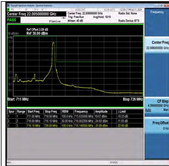
NTNV-N12-PC3-15-5-H-DFT-QPSK-Edge_1RB_R ight-Ant1-PASS
