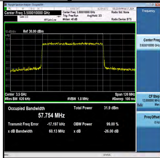
NTNV-N77-3450-3550-PC2-30-60-M-DFT-QPSK- Outer Full-Ant1-PASS
