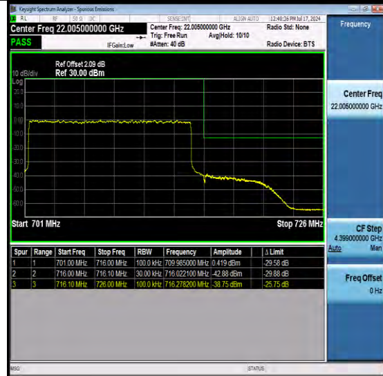
NTNV-N12-PC3-15-15-H-DFT-QPSK-Outer_Full-Ant1-PASS
