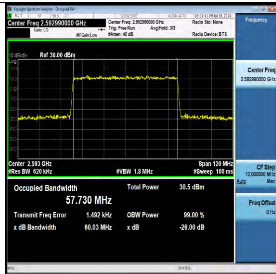
NTNV-N41-PC3-30-60-M-DFT-QPSK-Outer_Full-Ant1-PASS
