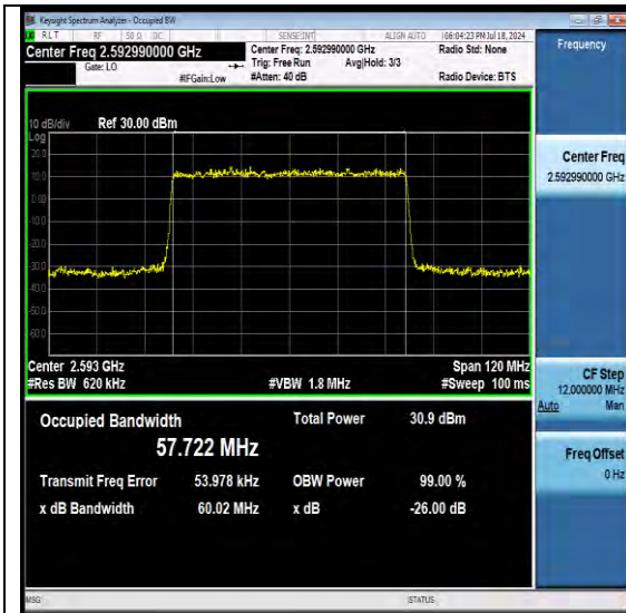
NTNV-N41-PC3-30-60-M-DFT-PI2BPSK-Outer_Fu II-Ant1-PASS
