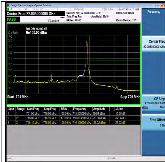
NTNV-N12-PC3-15-15-H-DFT-QPSK-Edge_1RB_Right-Ant1-PASS
