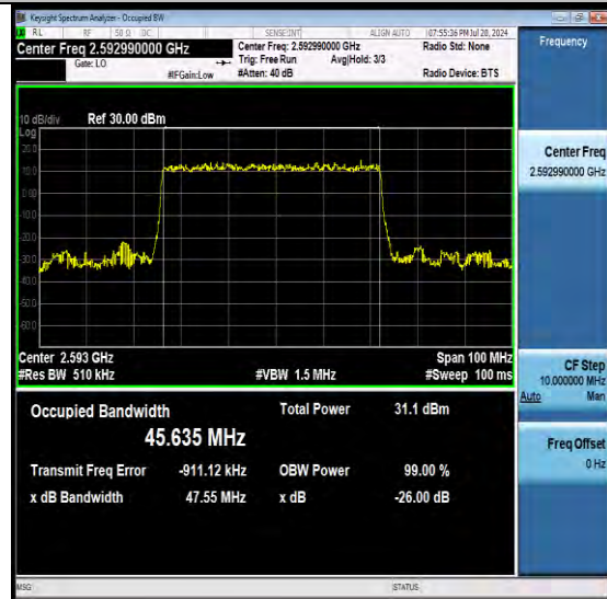
NTNV-N41-PC3-30-50-M-DFT-PI2BPSK-Outer_FuII-Ant1-PASS
