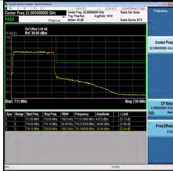
NTNV-N12-PC3-15-5-H-DFT-QPSK-Outer_Full-Ant1-PASS
