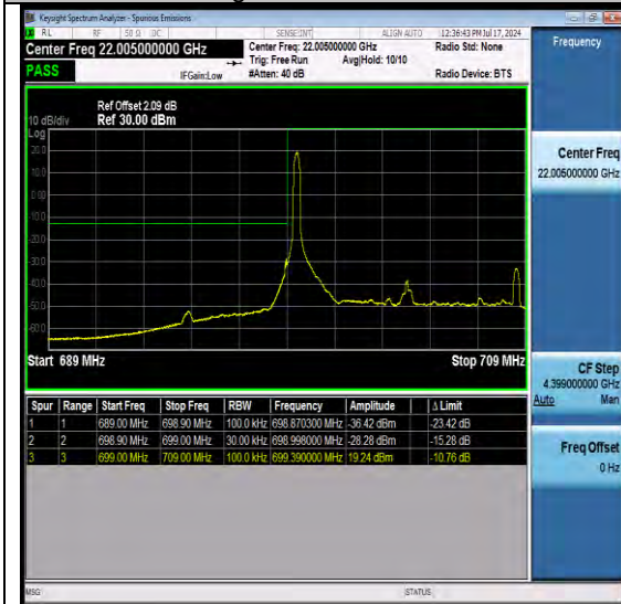
NTNV-N12-PC3-15-10-L-DFT-QPSK-Edge_1RB_ Left-Ant1-PASS
