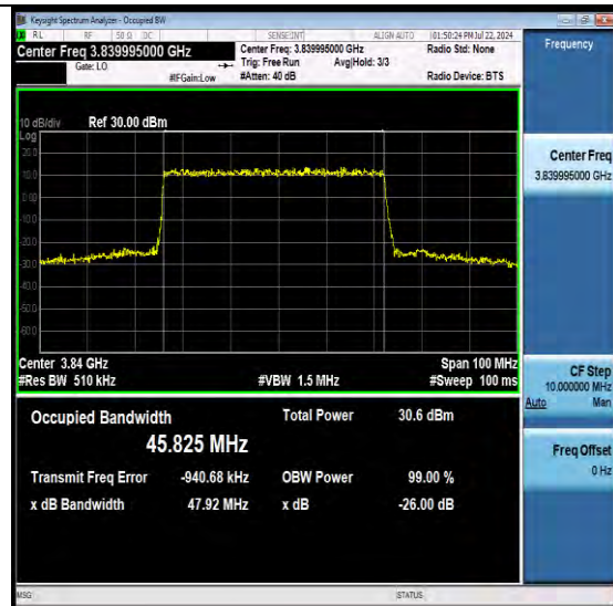
NTNV-N77-3700-3980-PC2-30-50-M-DFT-256QA M-Outer Full-Ant1-PASS
