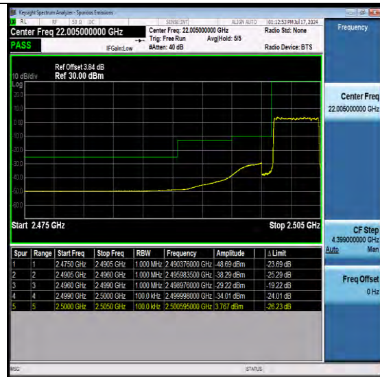
NTNV-N7-PC3-15-5-L-DFT-QPSK-Outer_Full-Ant1-PASS
