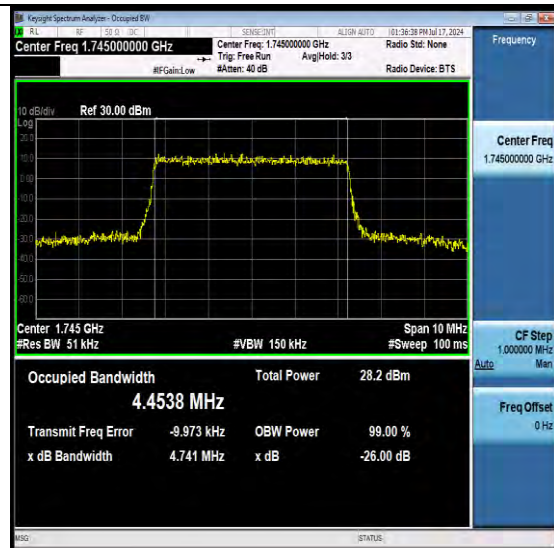
NTNV-N66-PC3-15-5-M-DFT-256QAM-Outer_Full-Ant1-PASS
