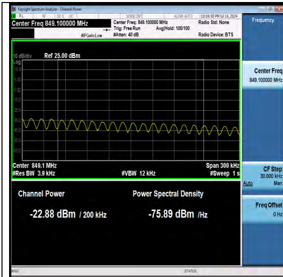
NTNV-N26-824-849-PC3-15-20-H-DFT-QPSK-Edge_1RB_Right-Ant1-PASS
