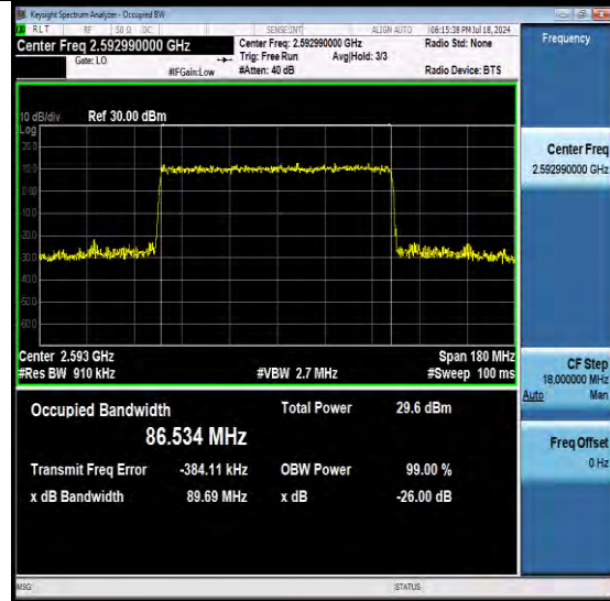
NTNV-N41-PC3-30-90-M-DFT-16QAM-Outer_Full-Ant1-PASS
