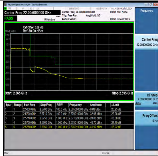
NTNV-N7-PC3-15-5-H-DFT-QPSK-Outer_Full-Ant1-PASS
