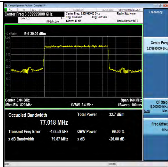
NTNV-N77-3700-3980-PC2-30-80-M-DFT-PI2BPS K-Outer Full-Ant1-PASS
