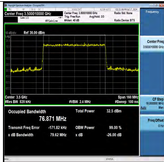
NTNV-N77-3450-3550-PC2-30-80-M-DFT-QPSK- Outer Full-Ant1-PASS
