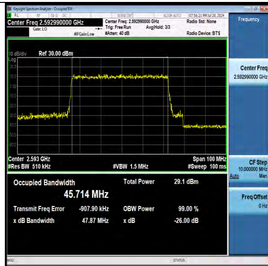
NTNV-N41-PC3-30-50-M-DFT-16QAM-Outer_Full-Ant1-PASS
