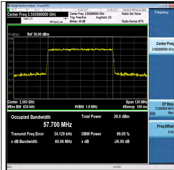
NTNV-N41-PC3-30-60-M-DFT-256QAM-Outer_Ful I-Ant1-PASS
