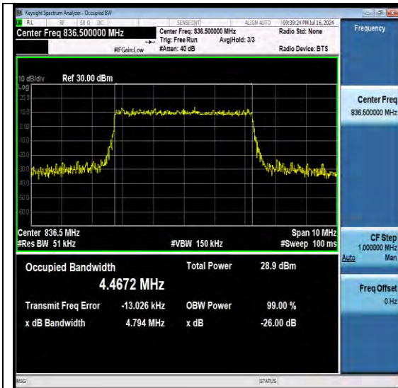
NTNV-N26-824-849-PC3-15-5-M-DFT-16QAM-Outer Full-Ant1-PASS
