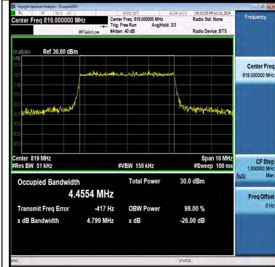
NTNV-N26-814-824-PC3-15-5-M-DFT-QPSK-Oute r Full-Ant1-PASS
