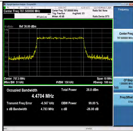
NTNV-N12-PC3-15-5-M-DFT-16QAM-Outer_Full-Ant1-PASS
