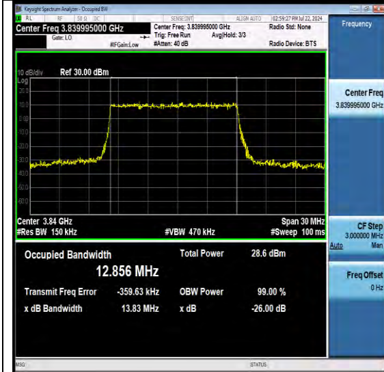
NTNV-N77-3700-3980-PC3-30-15-M-DFT-QPSK-Outer Full-Ant1-PASS
