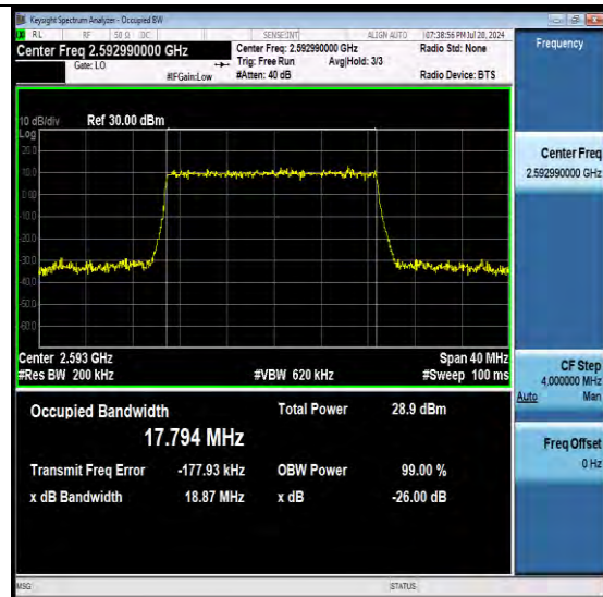
NTNV-N41-PC3-30-20-M-DFT-256QAM-Outer_Full-Ant1-PASS
