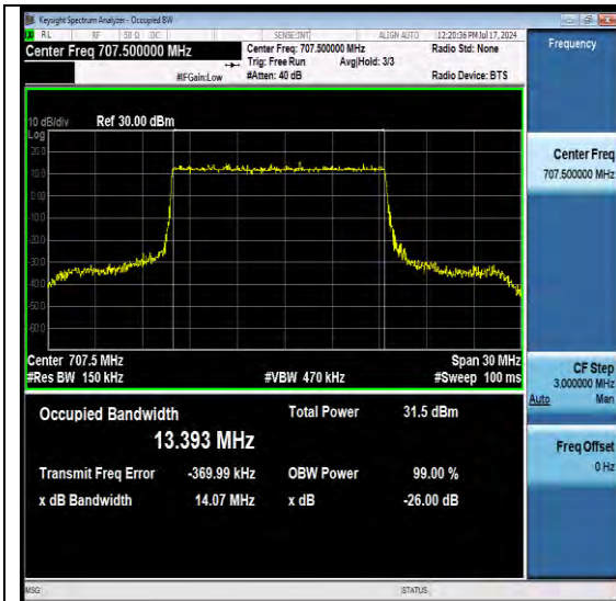
NTNV-N12-PC3-15-15-M-DFT-PI2BPSK-Outer_Fu II-Ant1-PASS
