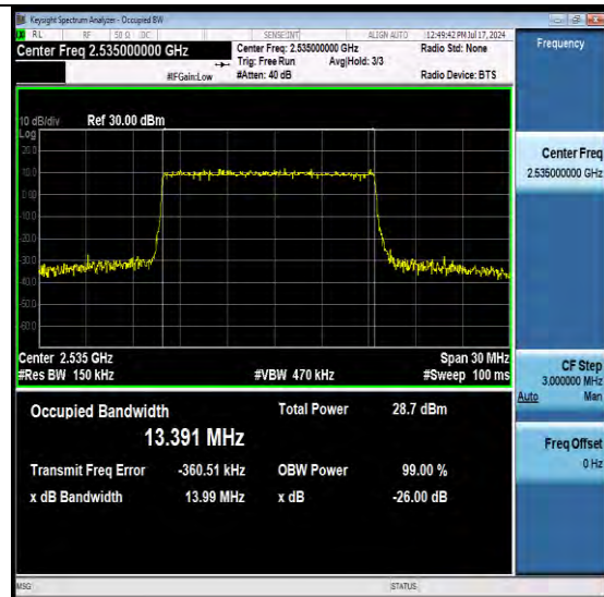
NTNV-N7-PC3-15-15-M-DFT-256QAM-Outer_Full-Ant1-PASS
