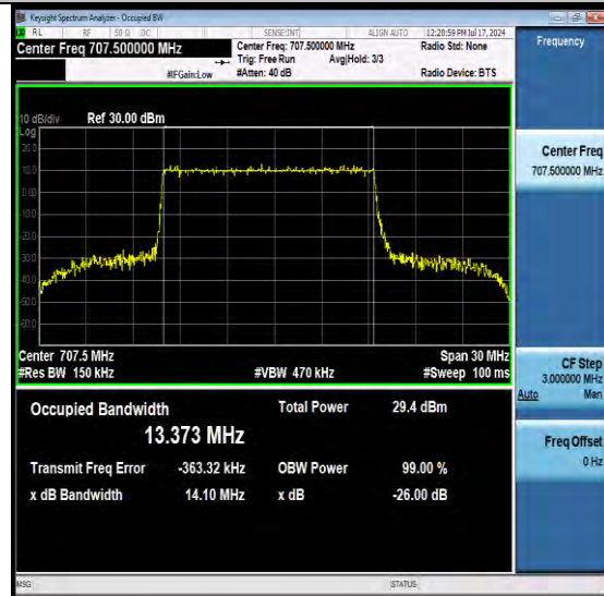
NTNV-N12-PC3-15-15-M-DFT-64QAM-Outer_Full-Ant1-PASS
