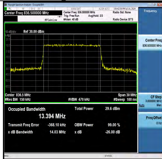
NTNV-N26-824-849-PC3-15-15-M-DFT-256QAM-Outer Full-Ant1-PASS
