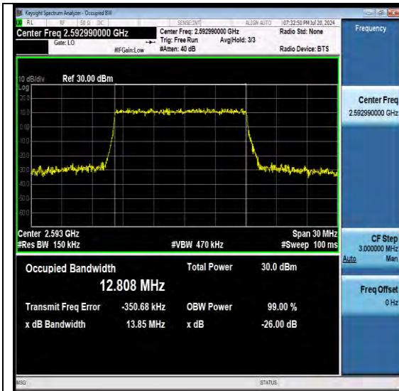
NTNV-N41-PC3-30-15-M-DFT-QPSK-Outer_Full-Ant1-PASS
