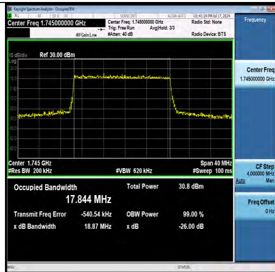
NTNV-N66-PC3-15-20-M-DFT-QPSK-Outer_Full-Ant1-PASS
