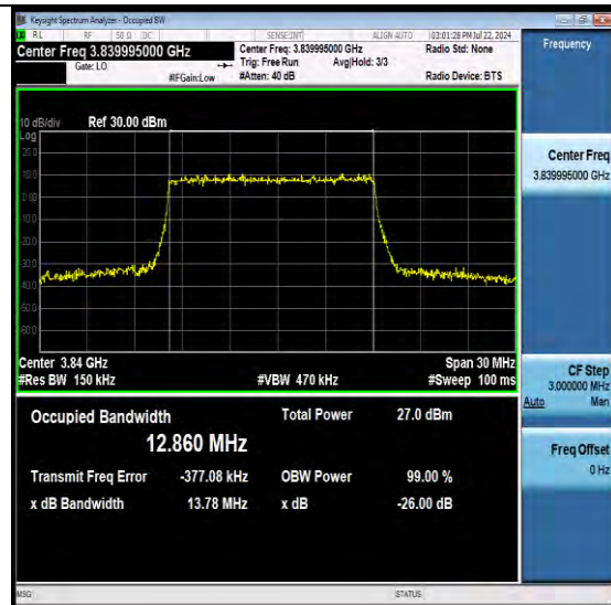
NTNV-N77-3700-3980-PC3-30-15-M-DFT-256QA M-Outer Full-Ant1-PASS
