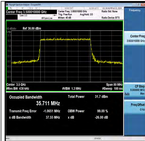
NTNV-N77-3450-3550-PC2-30-40-M-DFT-QPSK-Outer Full-Ant1-PASS
