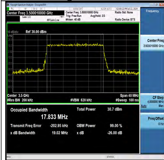
NTNV-N77-3450-3550-PC2-30-20-M-DFT-256QA M-Outer Full-Ant1-PASS
