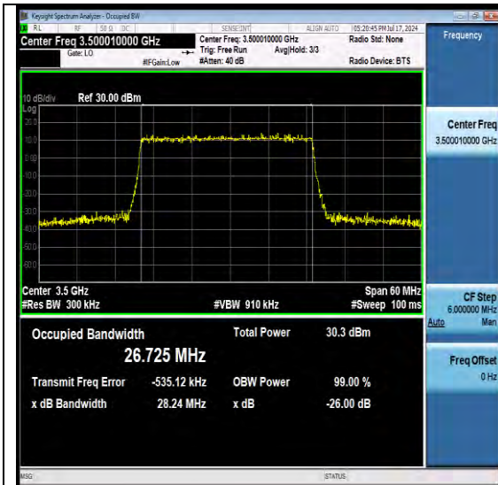
NTNV-N77-3450-3550-PC2-30-30-M-DFT-64QAM -Outer Full-Ant1-PASS
