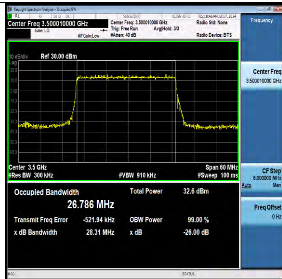
NTNV-N77-3450-3550-PC2-30-30-M-DFT-PI2BPS K-Outer Full-Ant1-PASS
