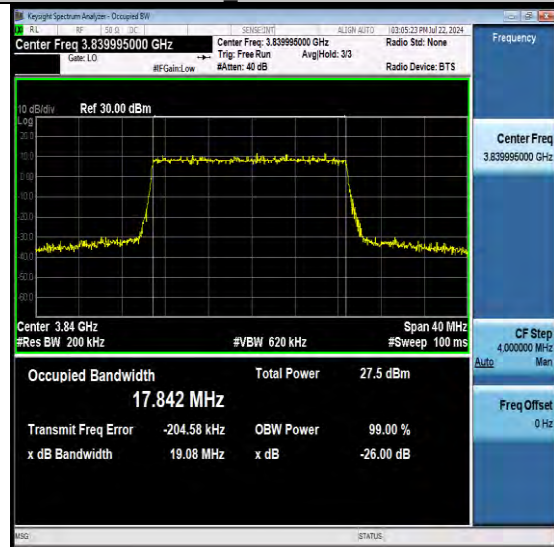
NTNV-N77-3700-3980-PC3-30-20-M-DFT-256QAM-M-Outer Full-Ant1-PASS
