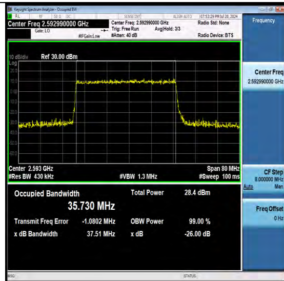
NTNV-N41-PC3-30-40-M-DFT-64QAM-Outer_Full-Ant1-PASS
