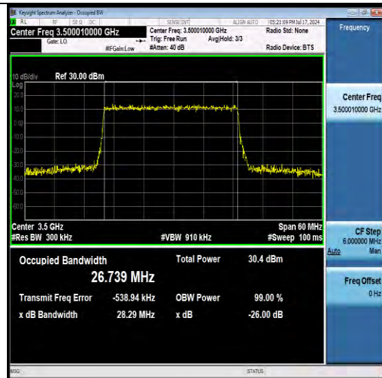
NTNV-N77-3450-3550-PC2-30-30-M-DFT-256QA M-Outer Full-Ant1-PASS
