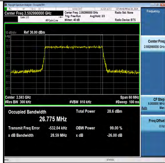
NTNV-N41-PC3-30-30-M-DFT-256QAM-Outer_Full-Ant1-PASS
