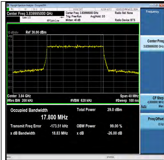
NTNV-N77-3700-3980-PC3-30-20-M-DFT-QPSK-Outer Full-Ant1-PASS
