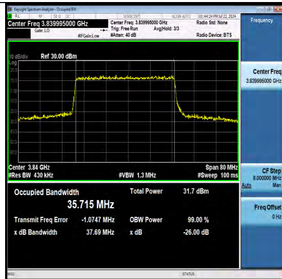
NTNV-N77-3700-3980-PC2-30-40-M-DFT-QPSK- Outer Full-Ant1-PASS
