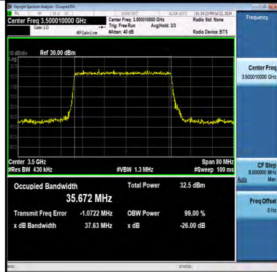
NTNV-N77-3450-3550-PC2-30-40-M-DFT-PI2BPS K-Outer_Full-Ant1-PASS
