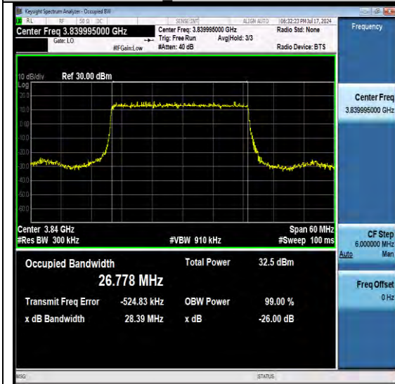
NTNV-N77-3700-3980-PC2-30-30-M-DFT-PI2BPS K-Outer Full-Ant1-PASS
