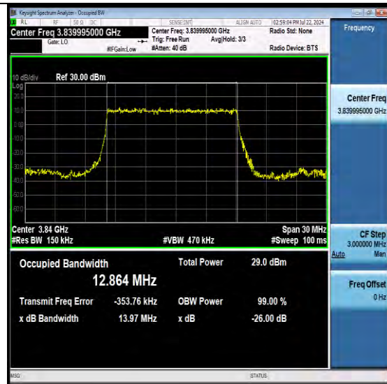
NTNV-N77-3700-3980-PC3-30-15-M-DFT-PI2BPS K-Outer Full-Ant1-PASS
