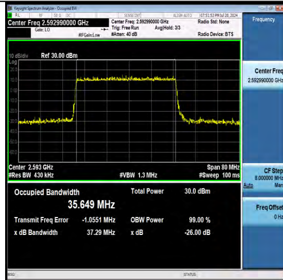
NTNV-N41-PC3-30-40-M-DFT-QPSK-Outer_Full-Ant1-PASS
