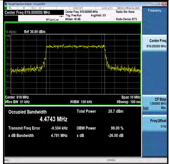
NTNV-N26-814-824-PC3-15-5-M-DFT-16QAM-Ou ter Full-Ant1-PASS
