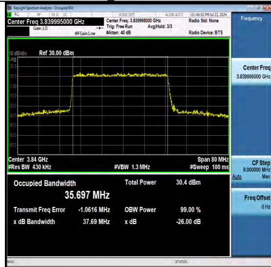
NTNV-N77-3700-3980-PC2-30-40-M-DFT-64QAM -Outer Full-Ant1-PASS
