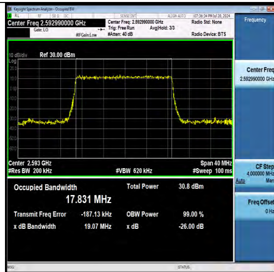
NTNV-N41-PC3-30-20-M-DFT-PI2BPSK-Outer_Fu II-Ant1-PASS
