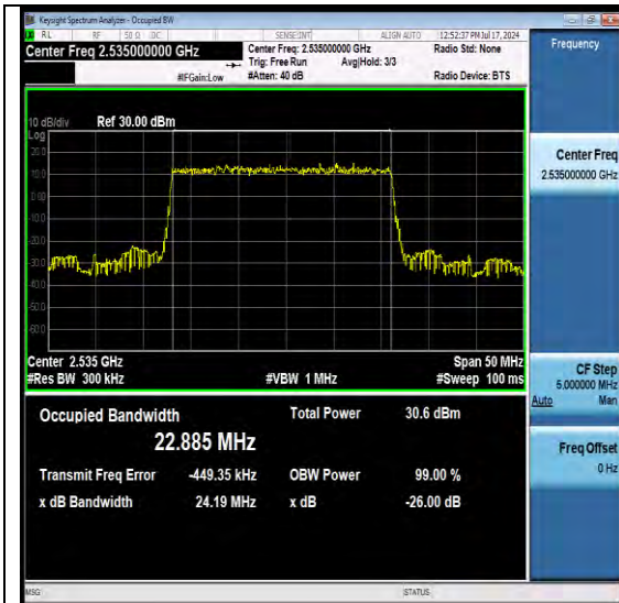
NTNV-N7-PC3-15-25-M-DFT-PI2BPSK-Outer_Full-Ant1-PASS
