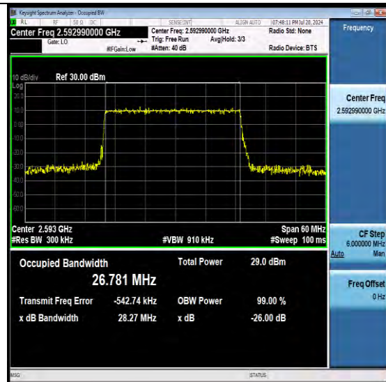
NTNV-N41-PC3-30-30-M-DFT-16QAM-Outer_Full-Ant1-PASS
