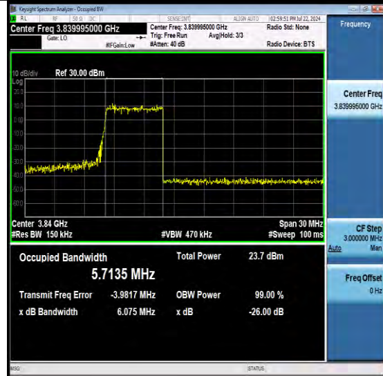
NTNV-N77-3700-3980-PC3-30-15-M-DFT-16QAM-Outer Full-Ant1-PASS
