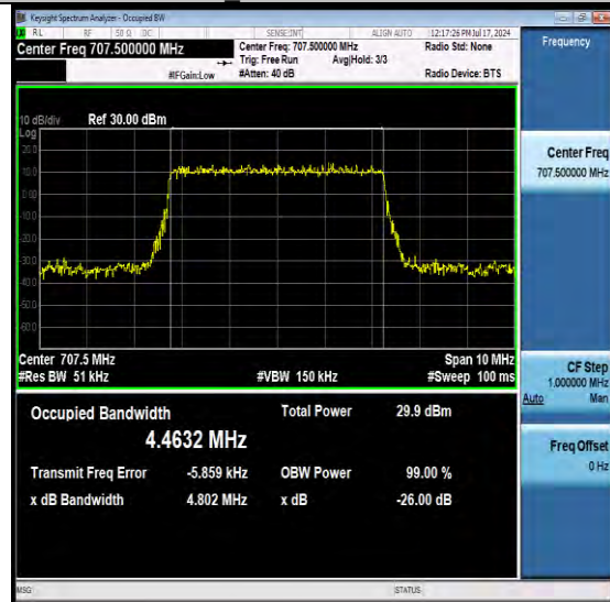
NTNV-N12-PC3-15-5-M-DFT-PI2BPSK-Outer Full-Ant1-PASS
