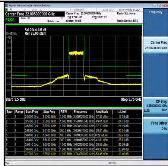
NTNV-N48-PC3-30-30-M-DFT-QPSK-Outer_Full- Ant1-PASS
