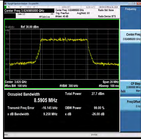
NTNV-N48-PC3-30-10-M-DFT-64QAM-Outer_Full-Ant1-PASS
