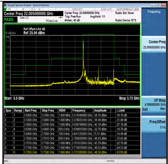
NTNV-N48-PC3-30-60-H-DFT-QPSK-Edge_1RB Left-Ant1-PASS
