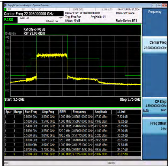
NTNV-N48-PC3-30-60-L-DFT-QPSK-Outer_Full-A nt1-PASS
