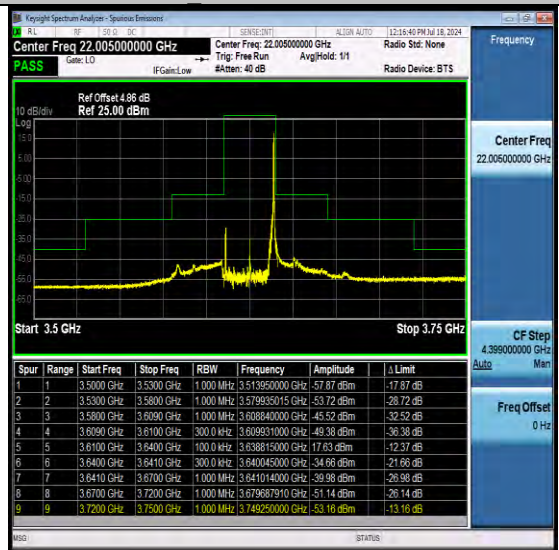
NTNV-N48-PC3-30-100-M-DFT-QPSK-Edge_1RB Left-Ant1-PASS
