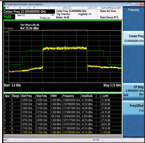
NTNV-N48-PC3-30-60-H-DFT-QPSK-Outer_Full-A nt1-PASS
