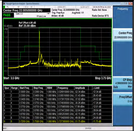
NTNV-N48-PC3-30-100-M-DFT-QPSK-Edge_1RB Left-Ant1-PASS
