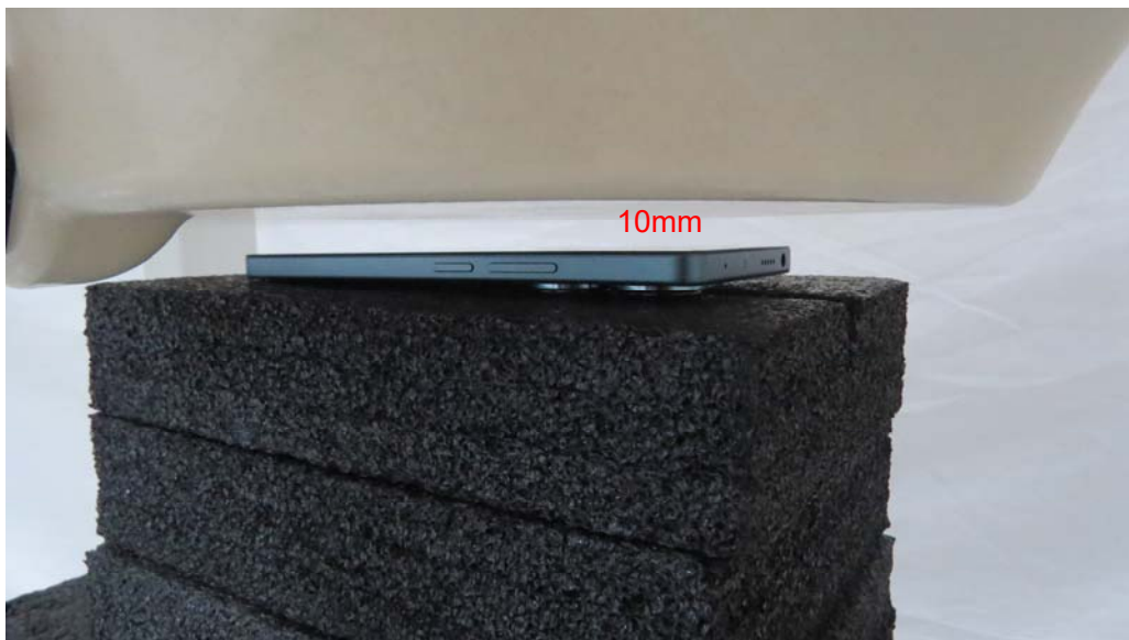
Picture 8: Front Side, the distance from EUT to the bottom of the Phantom is 10mm
