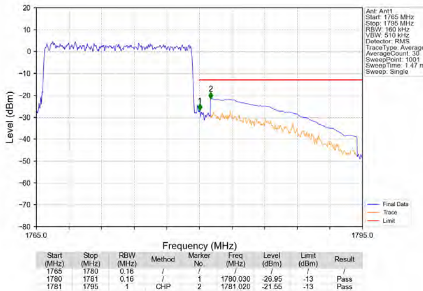
Band66_15MHz_64QAM_HCH_1772.5MHz_RB_75_0_NTNV
