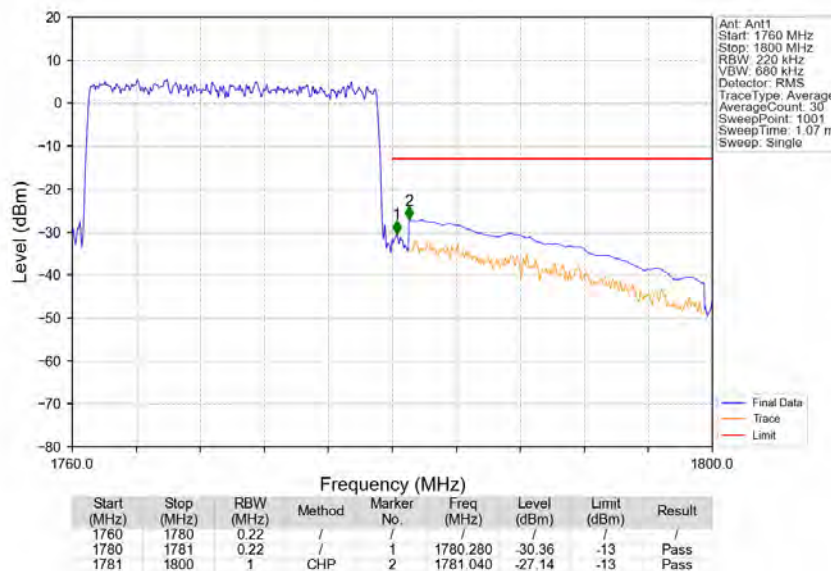
Band66_20MHz_16QAM_HCH_1770MHz_RB_100_0_NTNV
