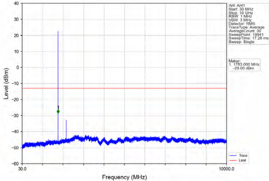
Band66_1.4MHz_16QAM_HCH_1779.3MHz_RB_1_0_NTNV
