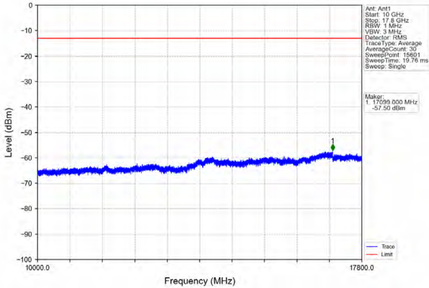
Band66_3MHz_16QAM_LCH_1711.5MHz_RB_15_0_NTNV
