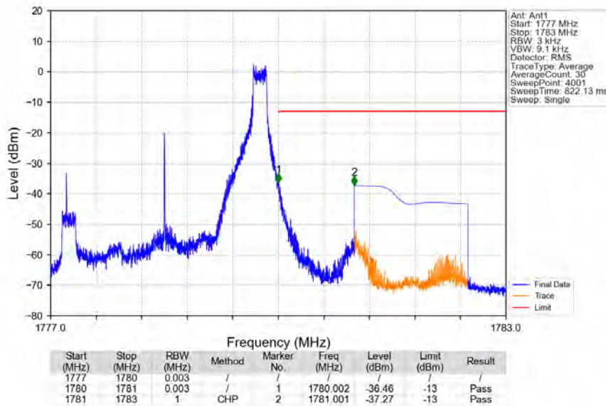
Band66_3MHz_64QAM_HCH_1778.5MHz_RB_1_14_NTNV
