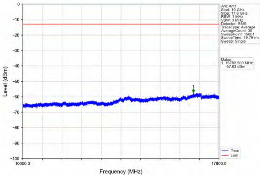
Band66_10MHz_16QAM_MCH_1745MHz_RB_1_0_NTNV
