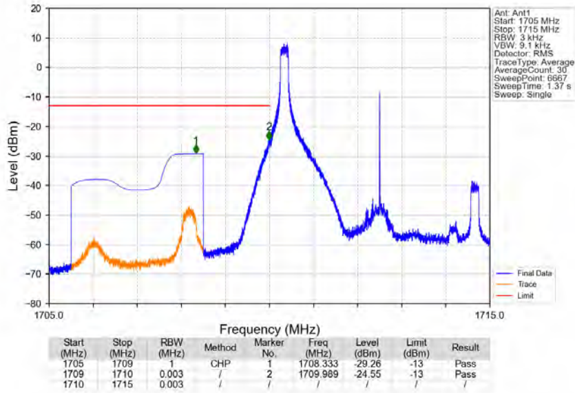
Band66_5MHz_16QAM_LCH_1712.5MHz_RB_1_0_NTV
