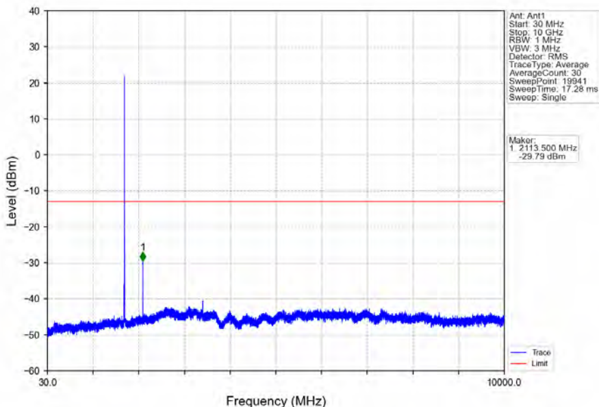
Band66_5MHz_64QAM_LCH_1712.5MHz_RB_1_0_NTV
