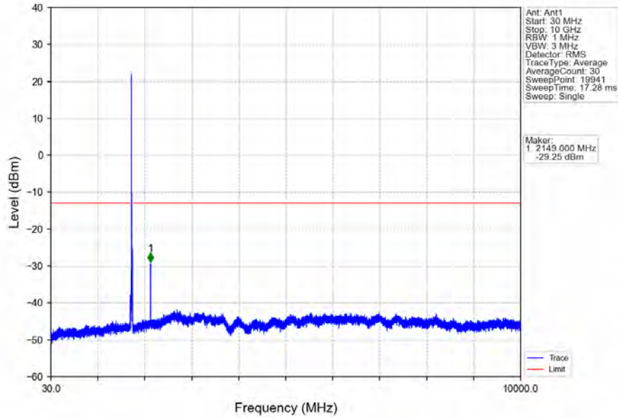
Band66_15MHz_64QAM_MCH_1745MHz_RB_1_0_NTNV
