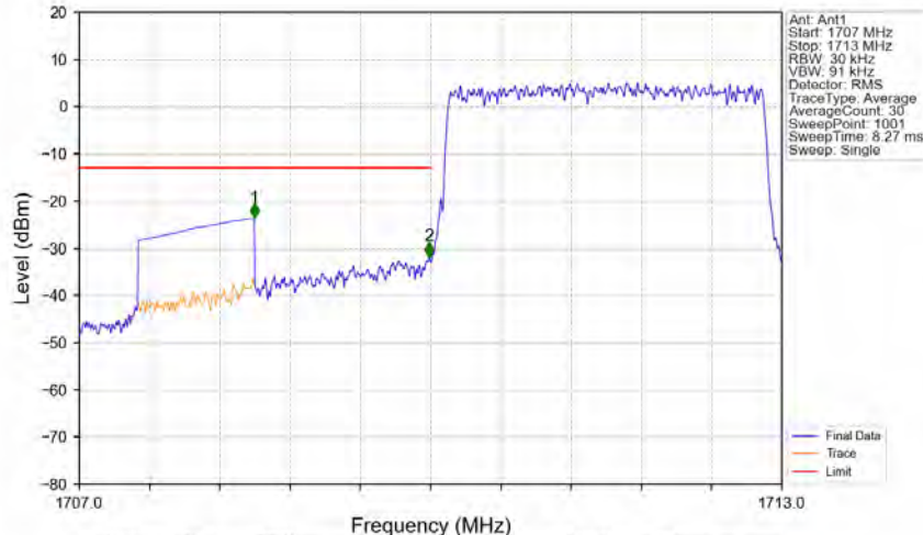
Band66_3MHz_16QAM_LCH_1711.5MHz_RB_15_0_NTNV
