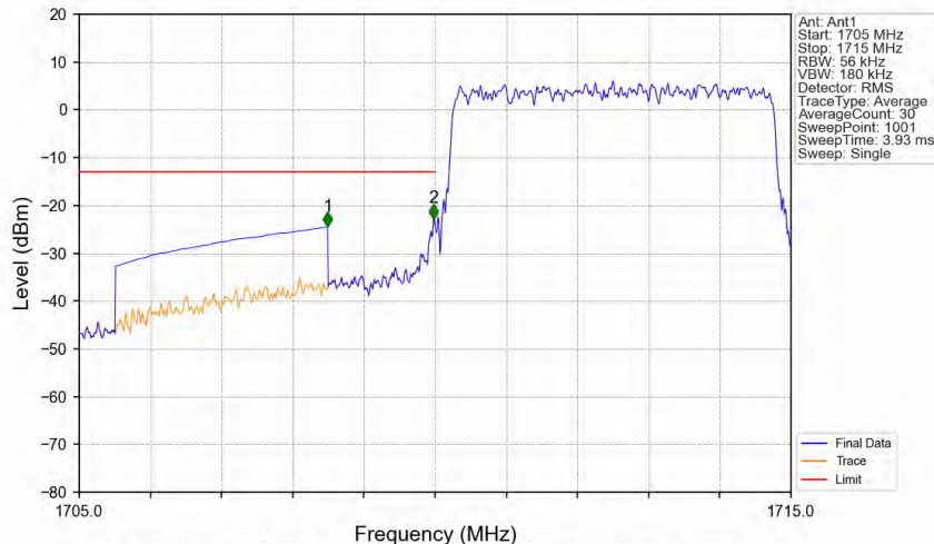
Band66_5MHz_16QAM_LCH_1712.5MHz_RB_25_0_NTNV
