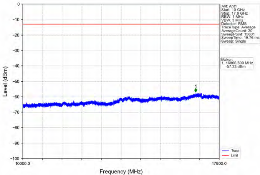
Band66_10MHz_16QAM_HCH_1775MHz_RB_1_0_NTNV
