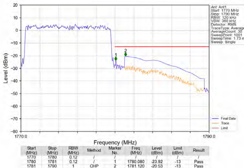
Band66_10MHz_64QAM_HCH_1775MHz_RB_50_0_NTNV
