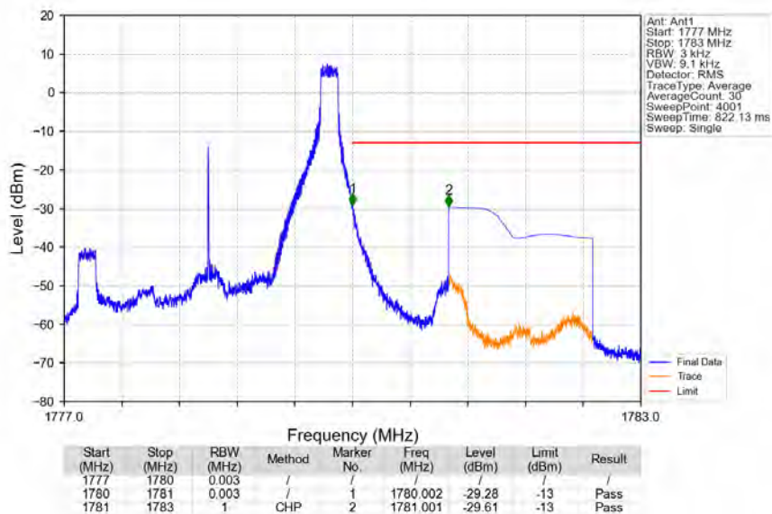
Band66_3MHz_16QAM_HCH_1778.5MHz_RB_1_14_NTNV
