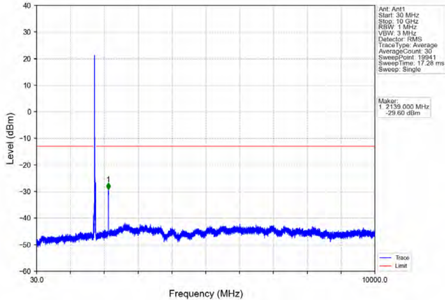
Band66_20MHz_64QAM_MCH_1745MHz_RB_1_0_NTNV
