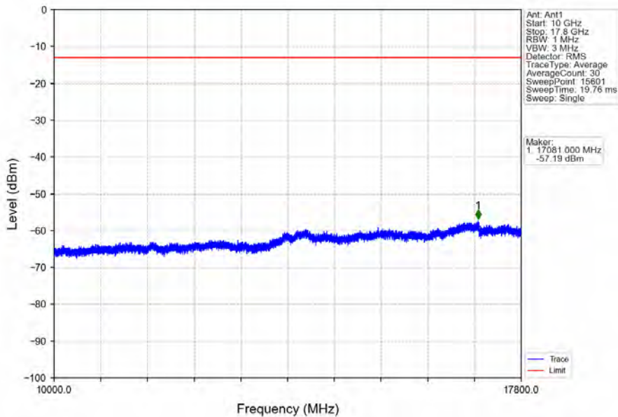
Band66_5MHz_QPSK_HCH_1777.5MHz_RB_1_0_NTNV
