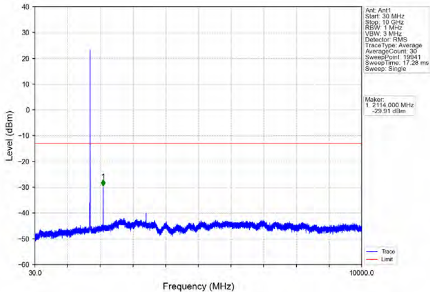
Band66_5MHz_16QAM_LCH_1712.5MHz_RB_1_0_NTV
