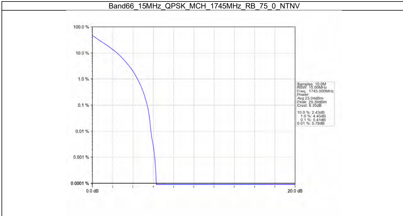
Band66_15MHz_QPSK_MCH_1745MHz_RB_75_0_NTNV
