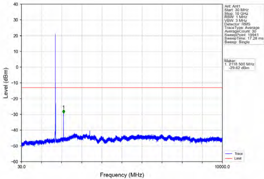
Band66_10MHz_64QAM_LCH_1715MHz_RB_1_0_NTNV
