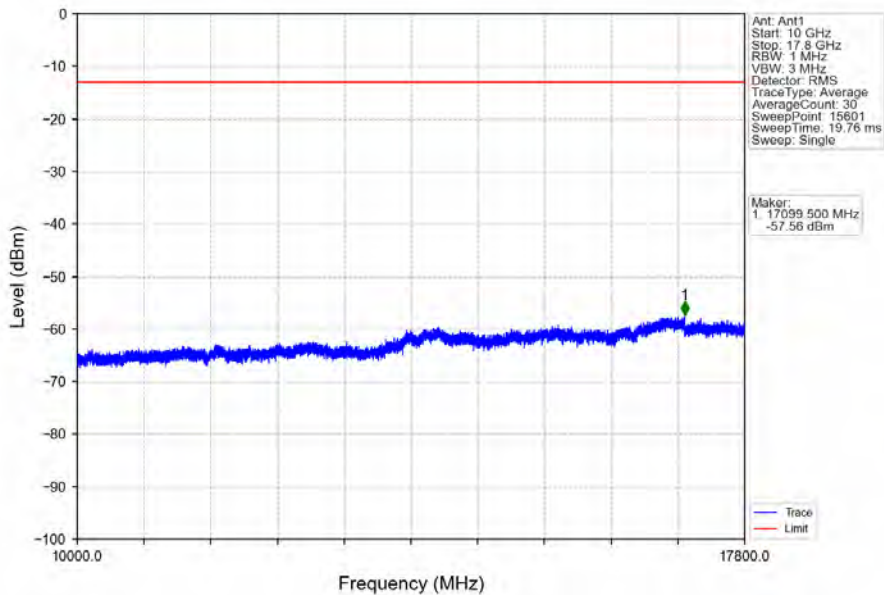
Band66_3MHz_16QAM_MCH_1745MHz_RB_1_0_NTNV
