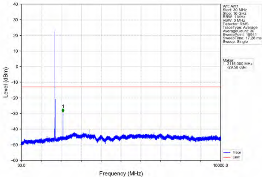
Band66_10MHz_16QAM_LCH_1715MHz_RB_1_0_NTNV
