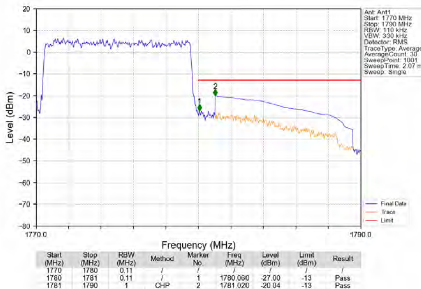
Band66_10MHz_QPSK_HCH_1775MHz_RB_50_0_NTNV
