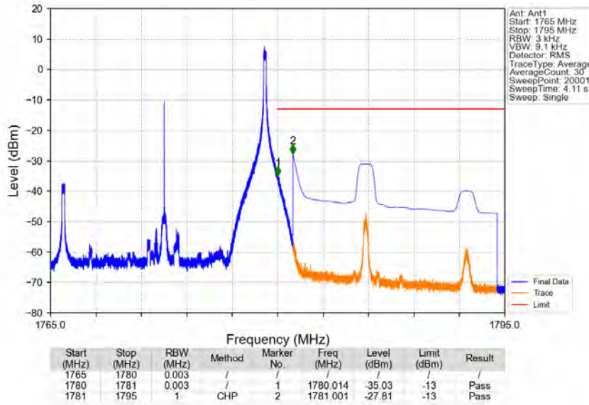
Band66_15MHz_64QAM_HCH_1772.5MHz_RB_1_74_NTNV
