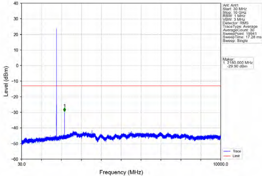
Band66_3MHz_QPSK_HCH_1778.5MHz_RB_1_0_NTNV
