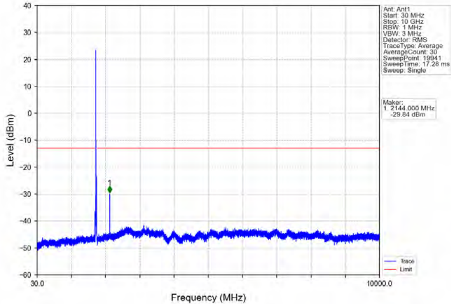
Band66_15MHz_QPSK_MCH_1745MHz_RB_1_0_NTNV
