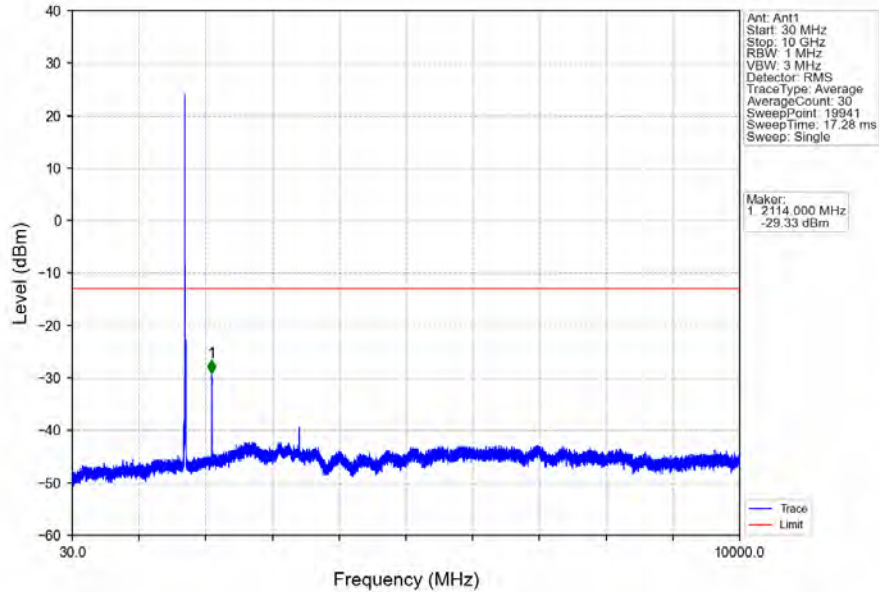
Band66_10MHz_QPSK_LCH_1715MHz_RB_1_0_NTNV
