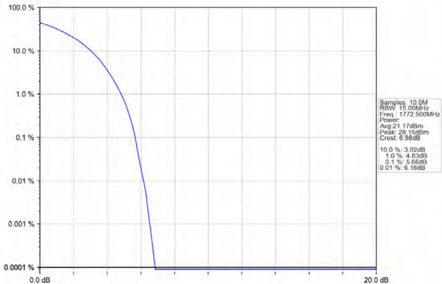
Band66_15MHz_64QAM_HCH_1772.5MHz_RB_75_0_NTNV
