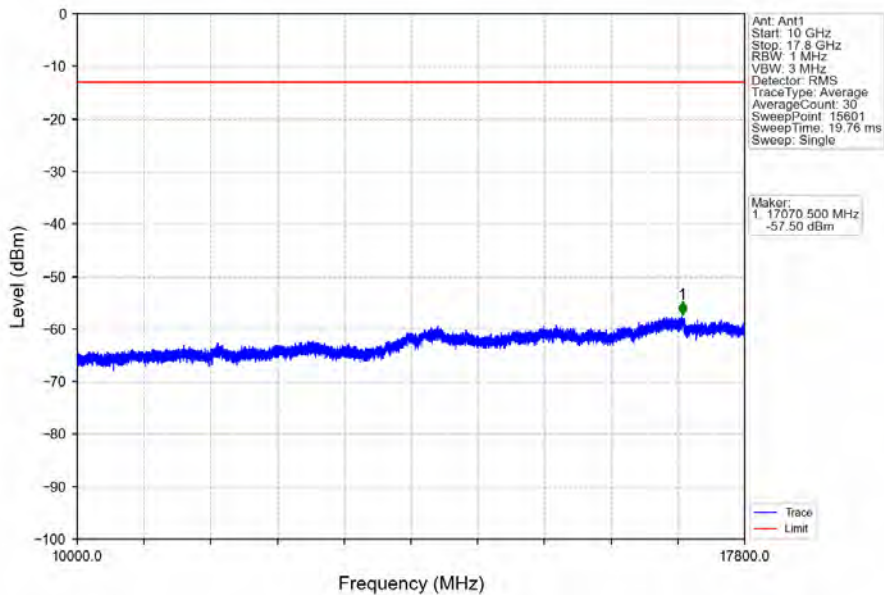
Band66_3MHz_64QAM_MCH_1745MHz_RB_1_0_NTNV
