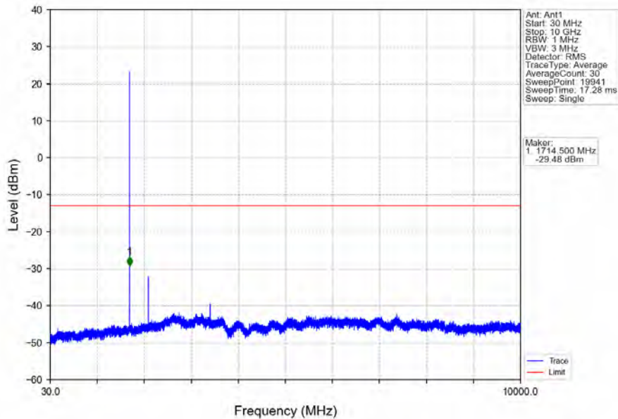
Band66_1.4MHz_16QAM_LCH_1710.7MHz_RB_1_0_NTNV
