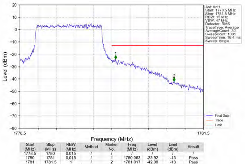
Band66_1.4MHz_64QAM_HCH_1779.3MHz_RB_6_0_NTNV
