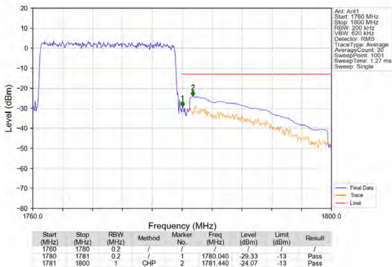
Band66_20MHz_64QAM_HCH_1770MHz_RB_100_0_NTNV
