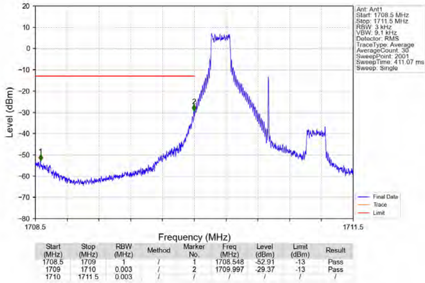
Band66_1.4MHz_64QAM_LCH_1710.7MHz_RB_1_0_NTNV
