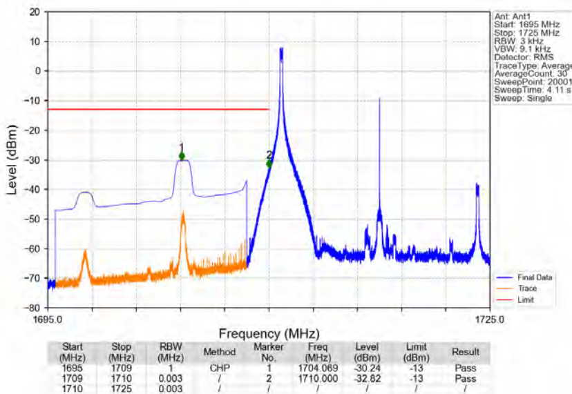
Band66_15MHz_16QAM_LCH_1717.5MHz_RB_1_0_NTNV
