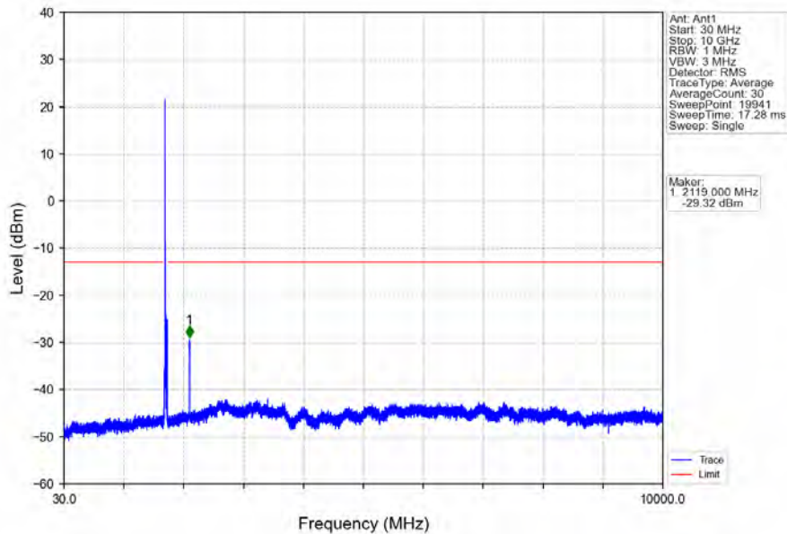
Band66_20MHz_64QAM_LCH_1720MHz_RB_1_0_NTNV
