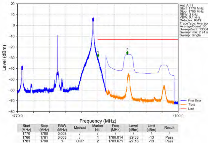
Band66_10MHz_16QAM_HCH_1775MHz_RB_1_49_NTNV
