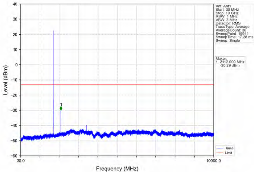
Band66_3MHz_16QAM_LCH_1711.5MHz_RB_1_0_NTV
