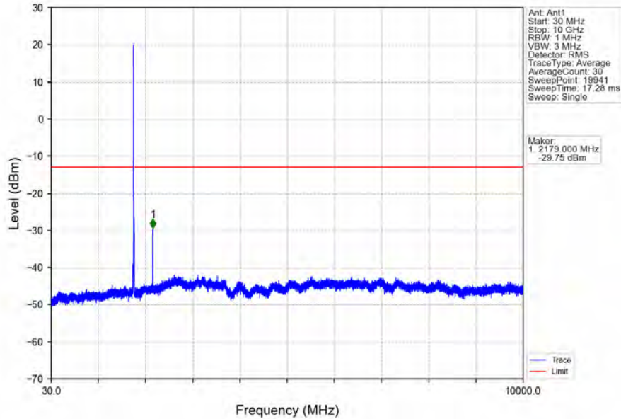
Band66_10MHz_64QAM_HCH_1775MHz_RB_1_0_NTNV
