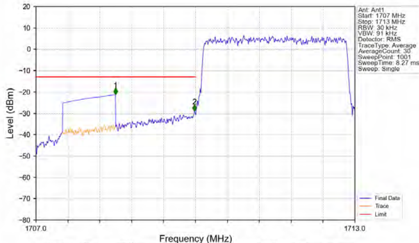
Band66_3MHz_QPSK_LCH_1711.5MHz_RB_15_0_NTNV
