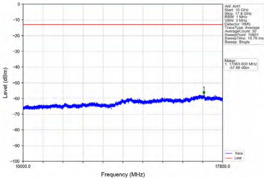
Band66_1.4MHz_16QAM_HCH_1779.3MHz_RB_1_0_NTNV
