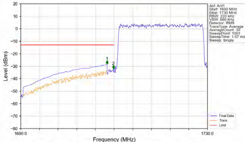
Band66_20MHz_64QAM_LCH_1720MHz_RB_100_0_NTNV
