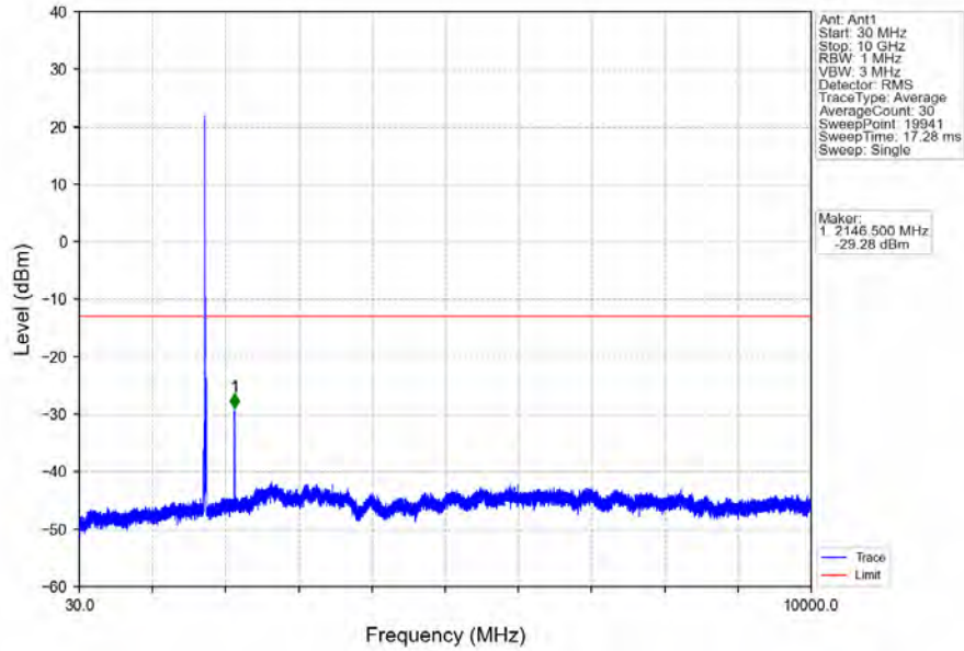
Band66_10MHz_16QAM_MCH_1745MHz_RB_1_0_NTNV
