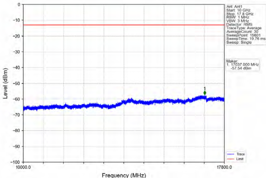
Band66_1.4MHz_64QAM_LCH_1710.7MHz_RB_6_0_NTNV
