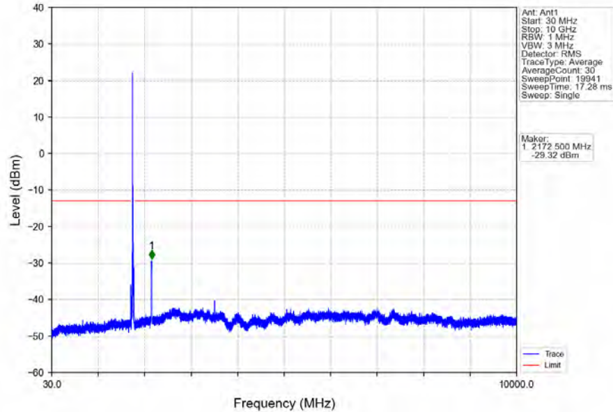
Band66_20MHz_16QAM_HCH_1770MHz_RB_1_0_NTNV
