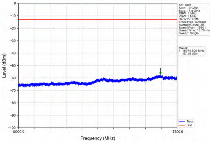
Band66_3MHz_QPSK_HCH_1778.5MHz_RB_1_0_NTNV
