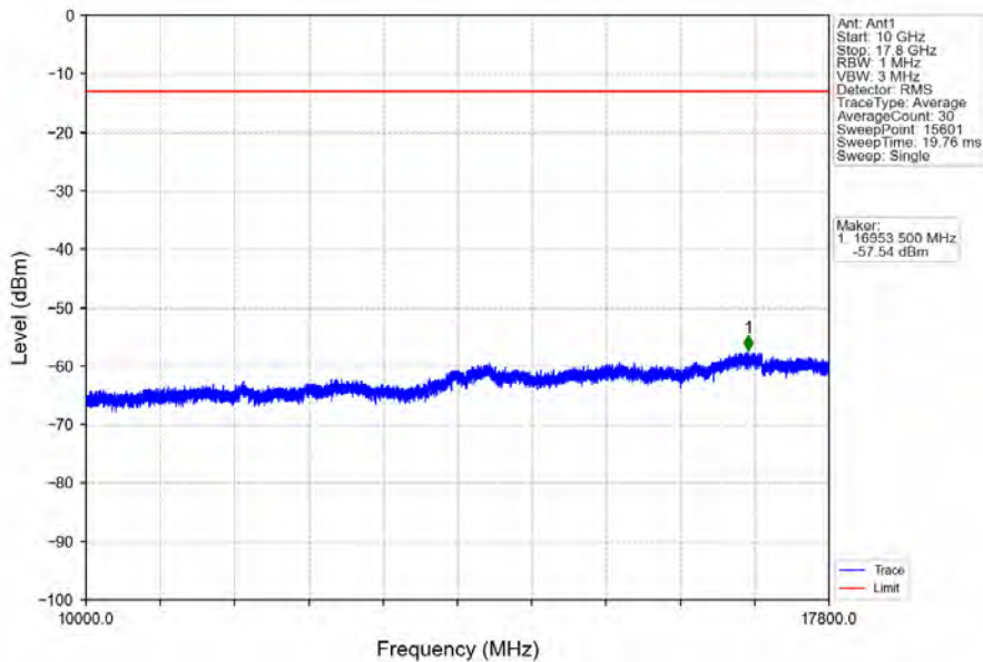
Band66_10MHz_64QAM_MCH_1745MHz_RB_1_0_NTNV
