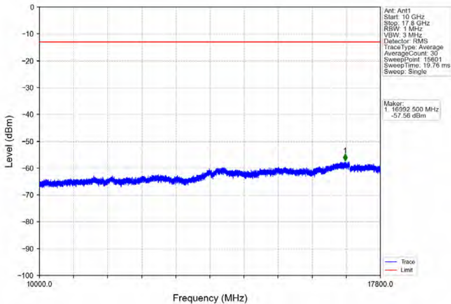
Band66_5MHz_64QAM_HCH_1777.5MHz_RB_1_0_NTNV
