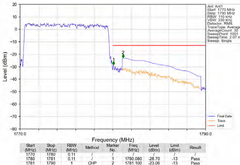
Band66_10MHz_16QAM_HCH_1775MHz_RB_50_0_NTNV
