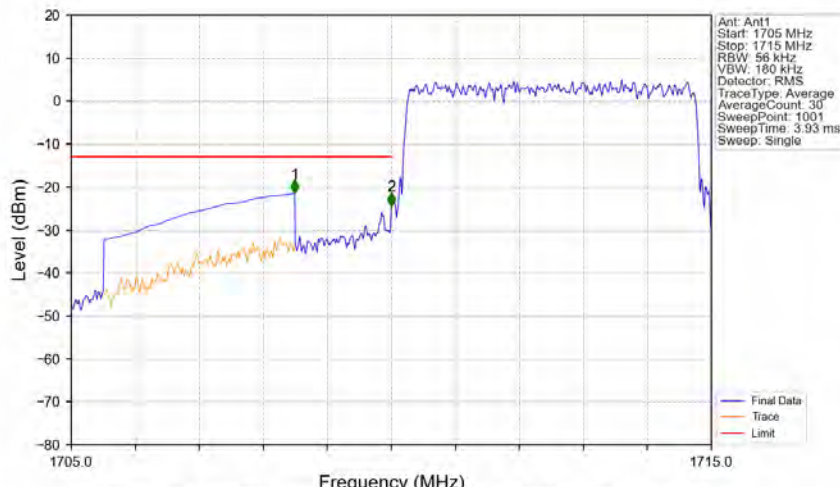
Band66_5MHz_64QAM_LCH_1712.5MHz_RB_25_0_NTNV
