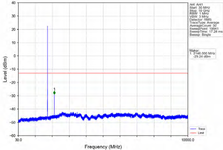
Band66_3MHz_QPSK_MCH_1745MHz_RB_1_0_NTNV
