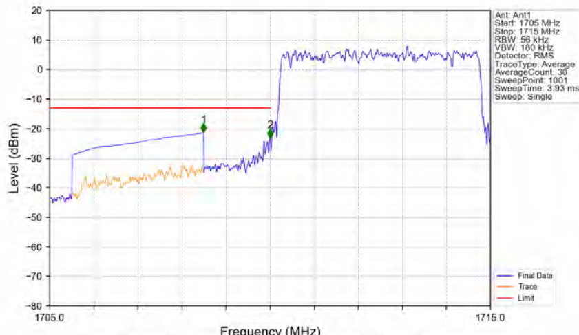
Band66_5MHz_QPSK_LCH_1712.5MHz_RB_25_0_NTNV
