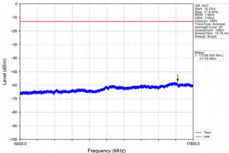
Band66_5MHz_64QAM_LCH_1712.5MHz_RB_25_0_NTNV
