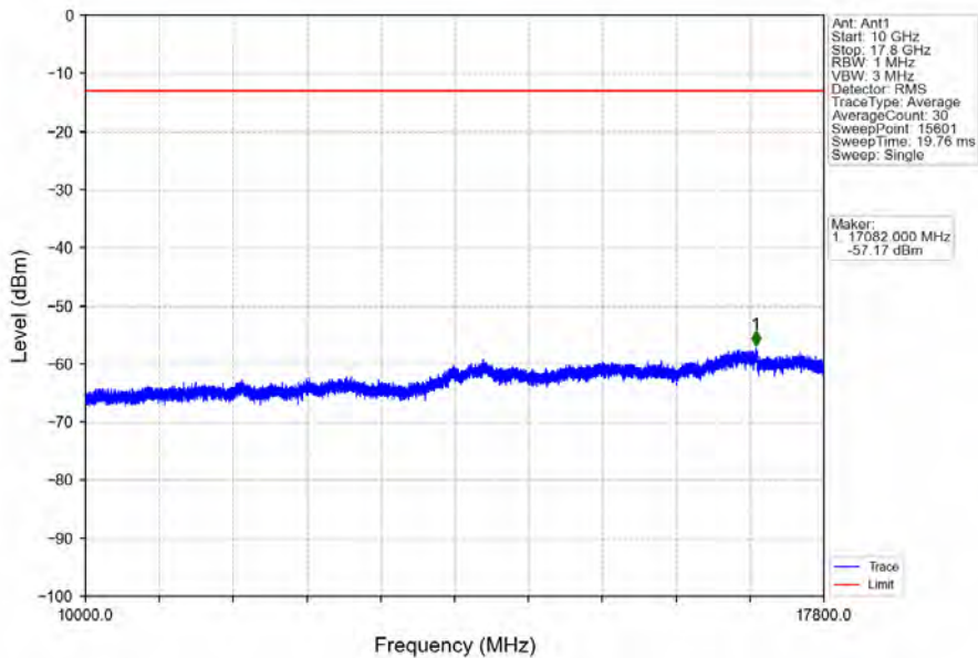
Band66_15MHz_16QAM_MCH_1745MHz_RB_1_0_NTNV
