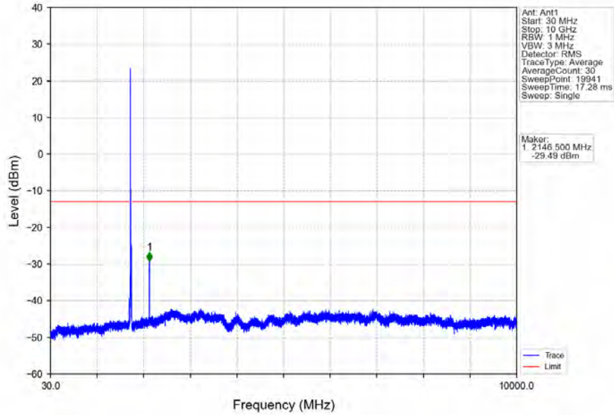
Band66_15MHz_16QAM_MCH_1745MHz_RB_1_0_NTNV
