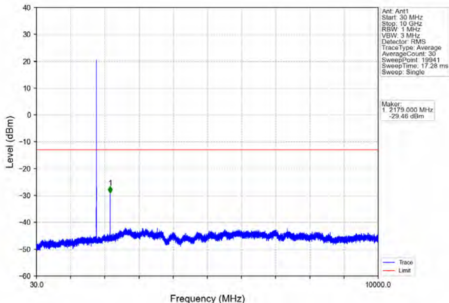
Band66_3MHz_64QAM_HCH_1778.5MHz_RB_1_0_NTNV
