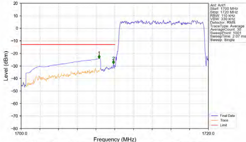
Band66_10MHz_QPSK_LCH_1715MHz_RB_50_0_NTNV
