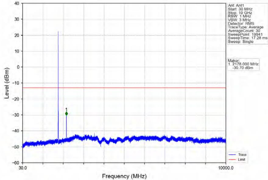
Band66_5MHz_16QAM_HCH_1777.5MHz_RB_1_0_NTNV
