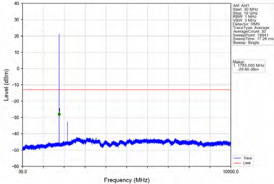
Band66_1.4MHz_64QAM_HCH_1779.3MHz_RB_1_0_NTNV
