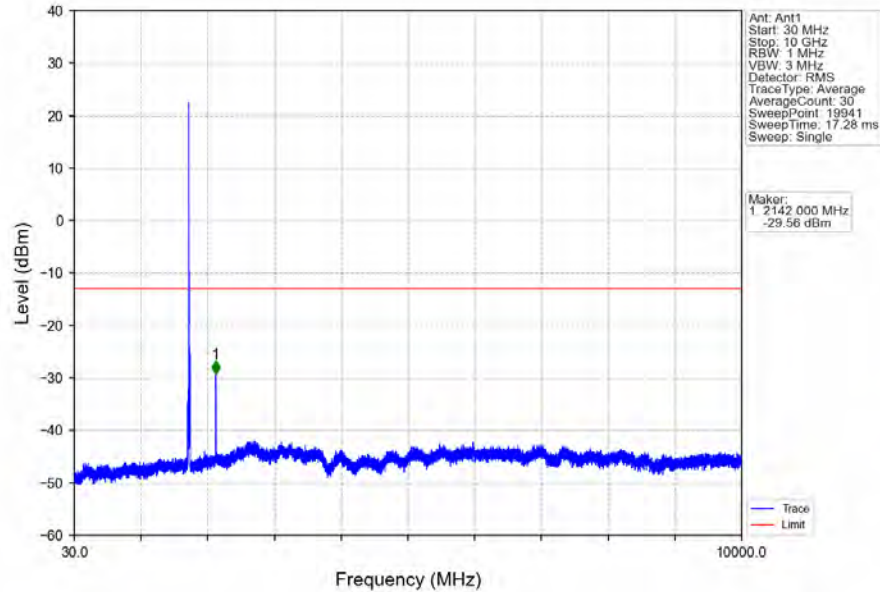
Band66_10MHz_QPSK_MCH_1745MHz_RB_1_0_NTNV
