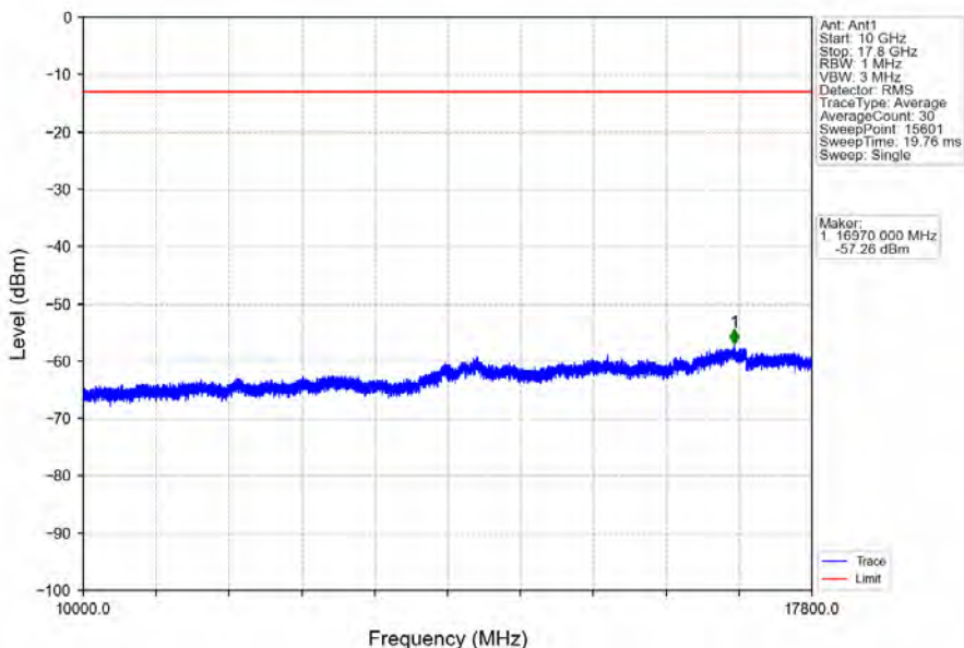
Band66_20MHz_16QAM_MCH_1745MHz_RB_1_0_NTNV
