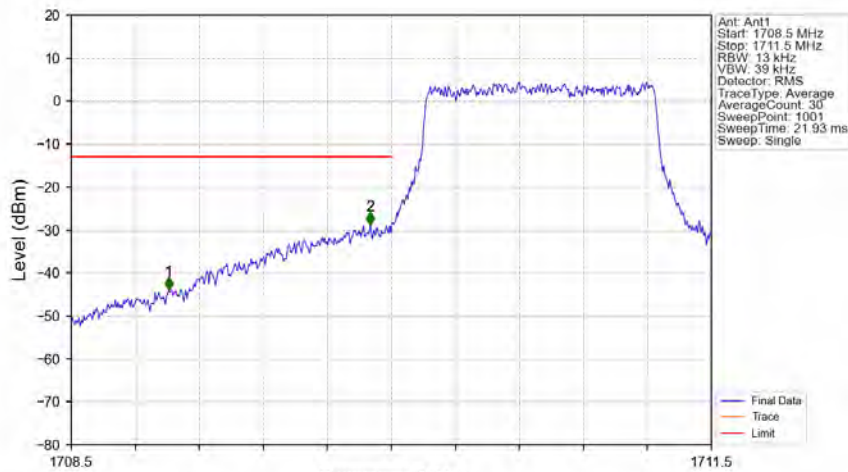
Band66_1.4MHz_64QAM_LCH_1710.7MHz_RB_6_0_NTNV
