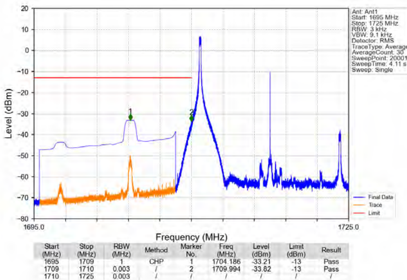
Band66_15MHz_64QAM_LCH_1717.5MHz_RB_1_0_NTNV
