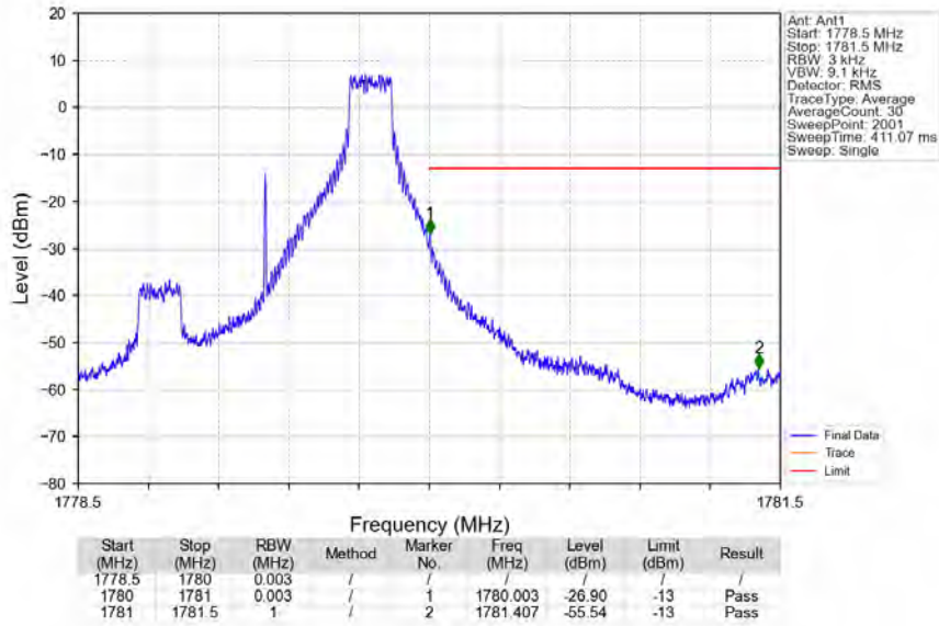
Band66_1.4MHz_16QAM_HCH_1779.3MHz_RB_1_5_NTNV
