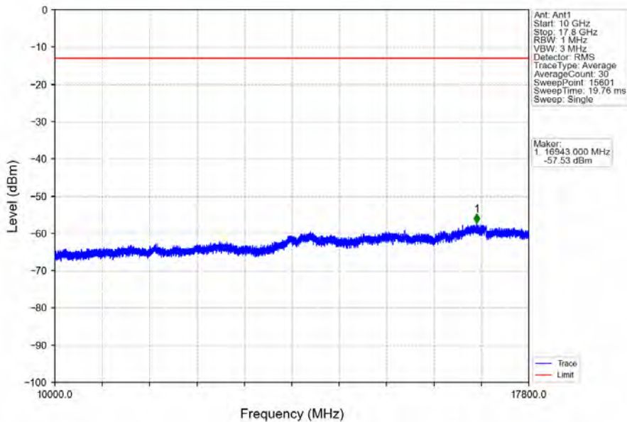
Band66_20MHz_64QAM_MCH_1745MHz_RB_1_0_NTNV
