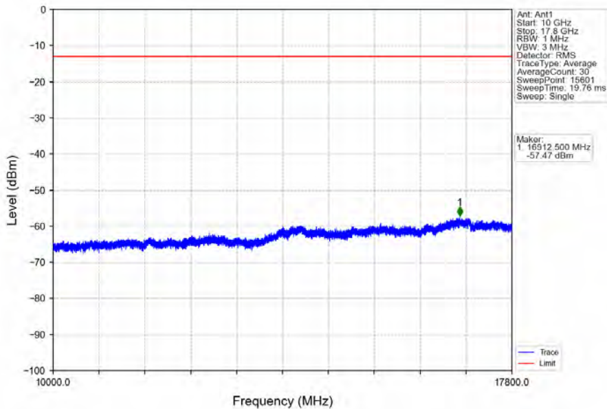
Band66_20MHz_16QAM_HCH_1770MHz_RB_1_0_NTNV
