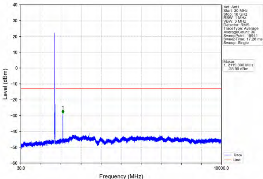
Band66_15MHz_16QAM_LCH_1717.5MHz_RB_1_0_NTNV
