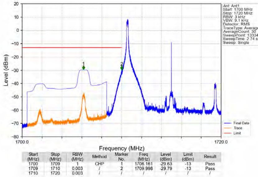
Band66_10MHz_16QAM_LCH_1715MHz_RB_1_0_NTNV
