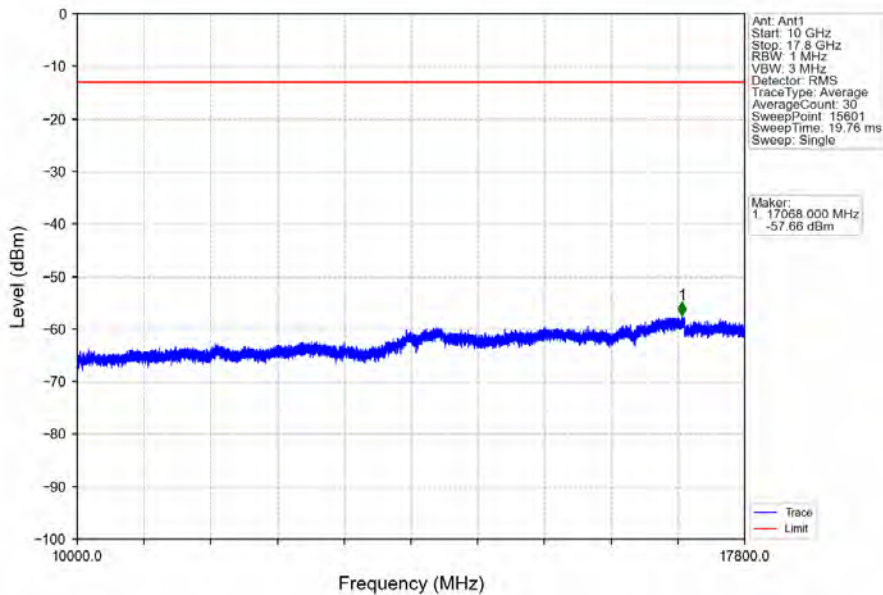
Band66_1.4MHz_64QAM_HCH_1779.3MHz_RB_1_0_NTNV
