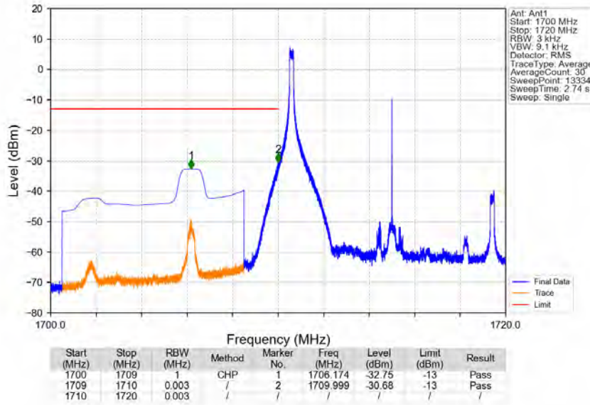
Band66_10MHz_64QAM_LCH_1715MHz_RB_1_0_NTNV
