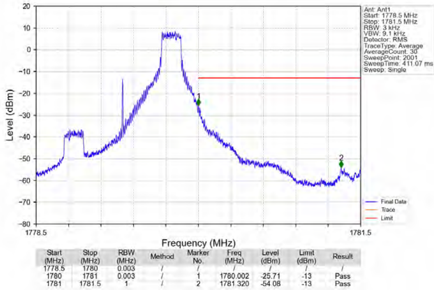
Band66_1.4MHz_QPSK_HCH_1779.3MHz_RB_1_5_NTNV
