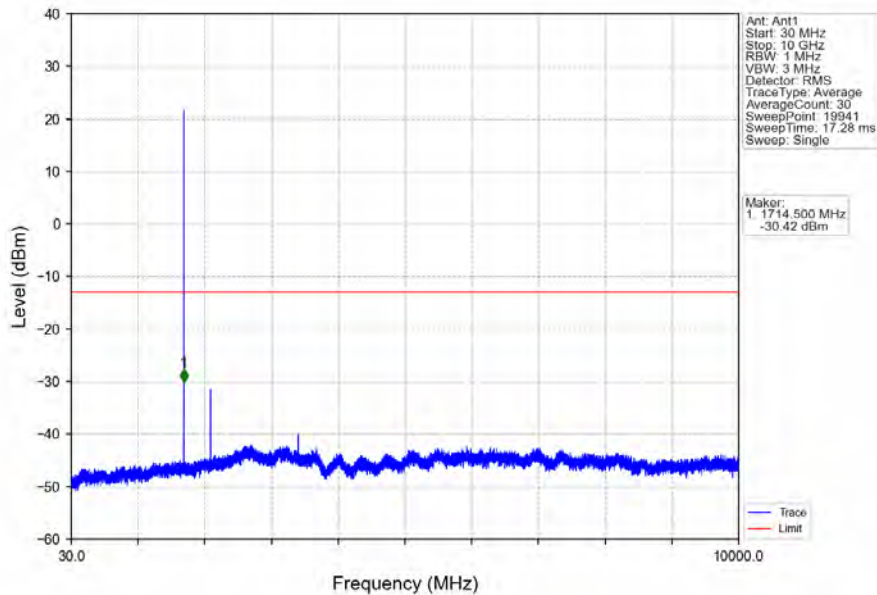
Band66_1.4MHz_64QAM_LCH_1710.7MHz_RB_1_0_NTNV
