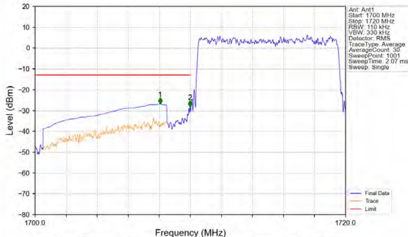
Band66_10MHz_16QAM_LCH_1715MHz_RB_50_0_NTNV
