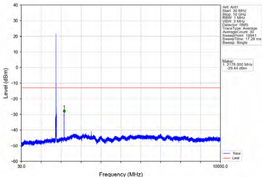
Band66_15MHz_16QAM_HCH_1772.5MHz_RB_1_0_NTNV
