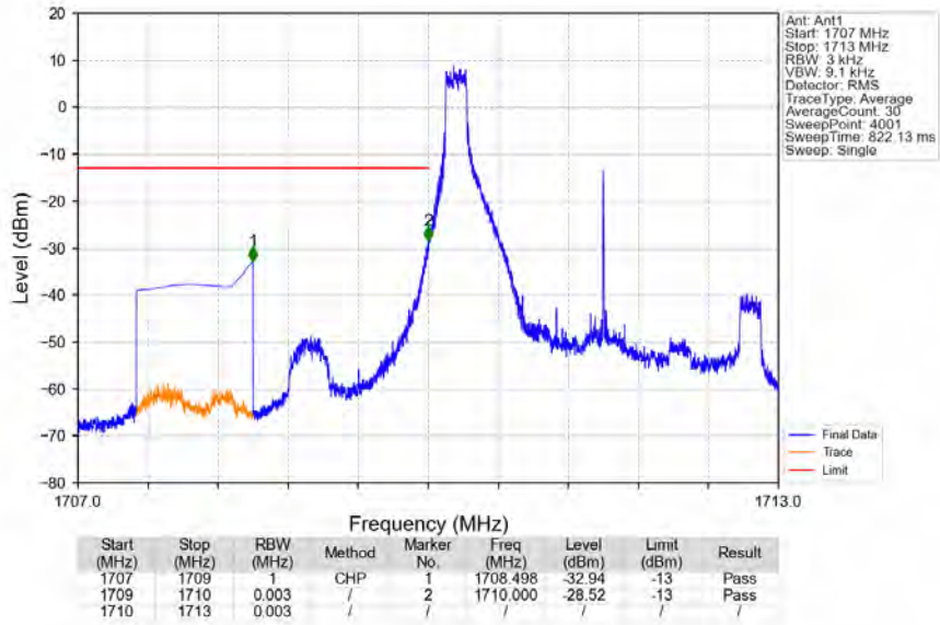
Band66_3MHz_16QAM_LCH_1711.5MHz_RB_1_0_NTV
