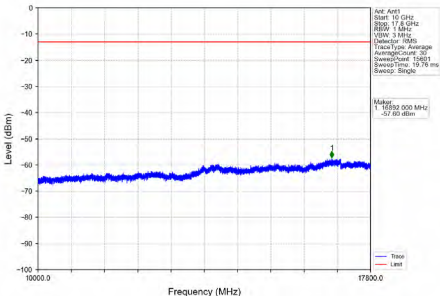
Band66_15MHz_16QAM_HCH_1772.5MHz_RB_1_0_NTNV
