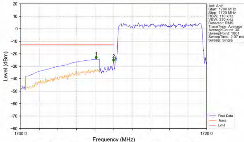
Band66_10MHz_64QAM_LCH_1715MHz_RB_50_0_NTNV
