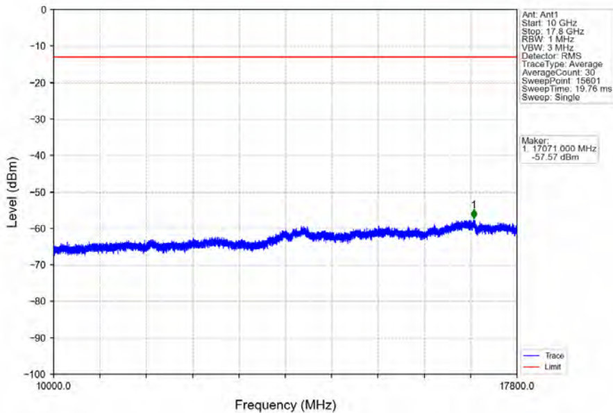
Band66_15MHz_64QAM_MCH_1745MHz_RB_1_0_NTNV
