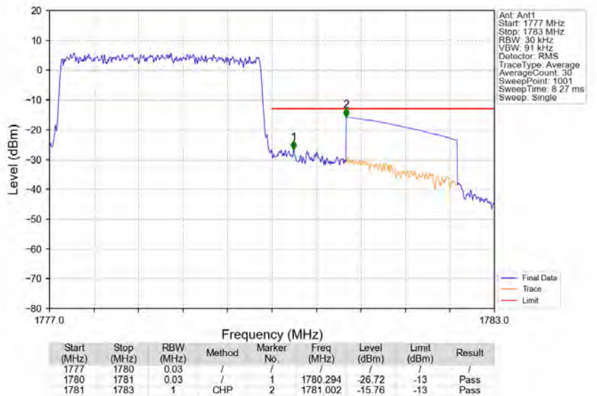
Band66_3MHz_QPSK_HCH_1778.5MHz_RB_15_0_NTNV
