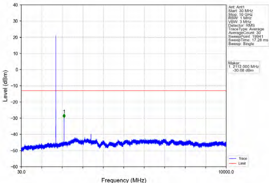
Band66_3MHz_64QAM_LCH_1711.5MHz_RB_1_0_NTV
