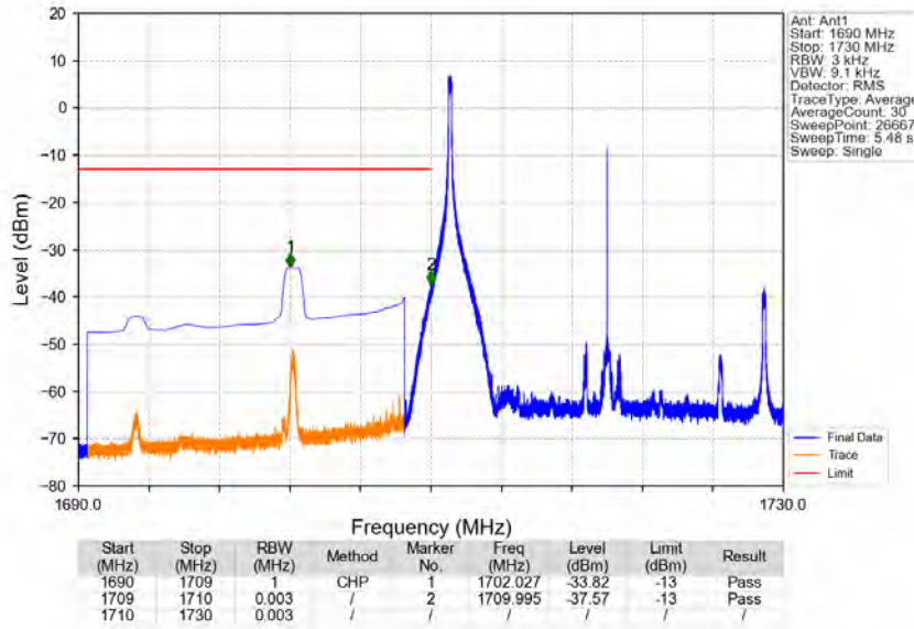
Band66_20MHz_64QAM_LCH_1720MHz_RB_1_0_NTNV
