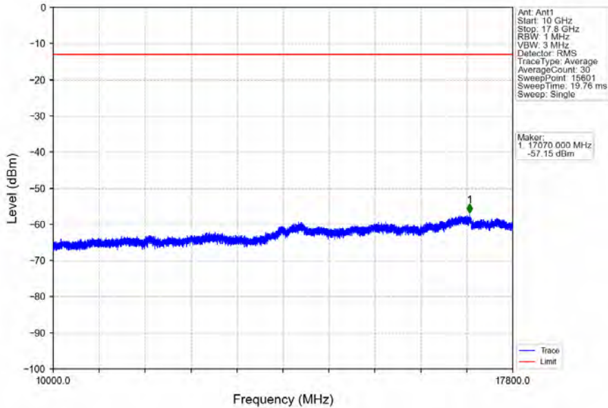
Band66_5MHz_16QAM_LCH_1712.5MHz_RB_25_0_NTNV
