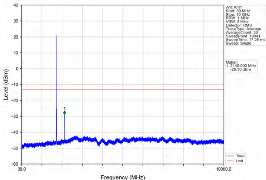
Band66_5MHz_64QAM_MCH_1745MHz_RB_1_0_NTNV
