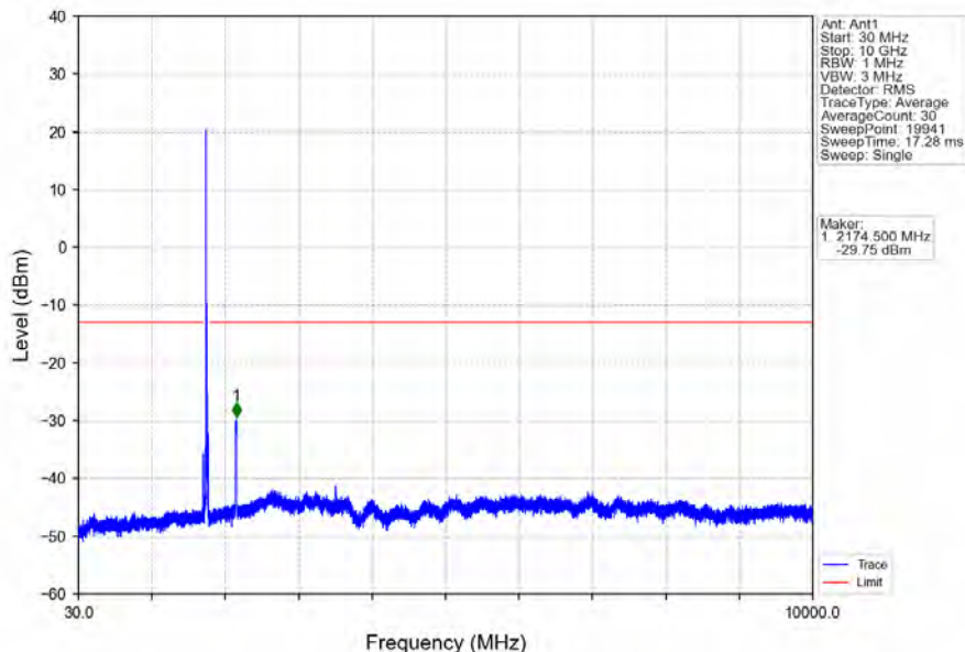
Band66_20MHz_64QAM_HCH_1770MHz_RB_1_0_NTNV
