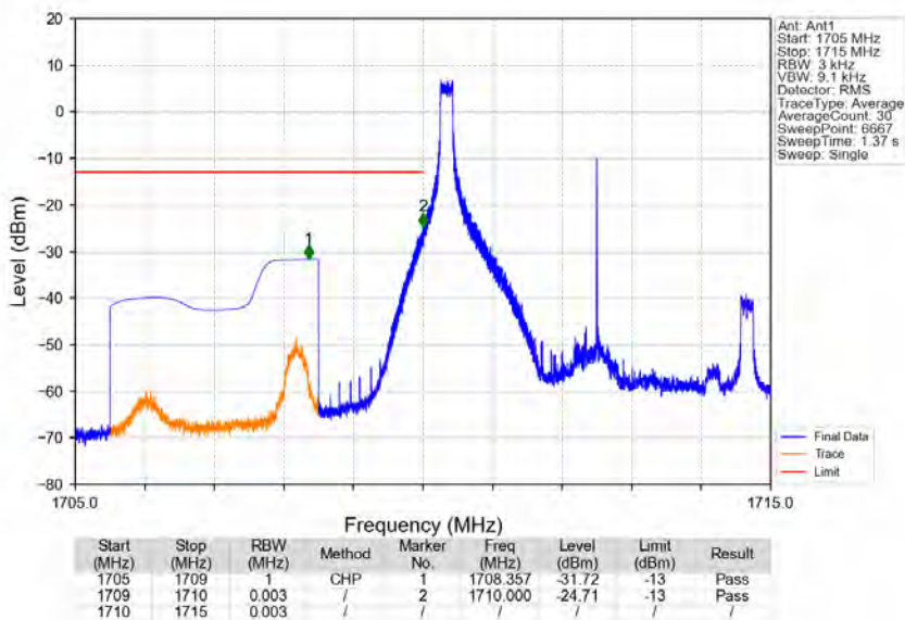
Band66_5MHz_64QAM_LCH_1712.5MHz_RB_1_0_NTV
