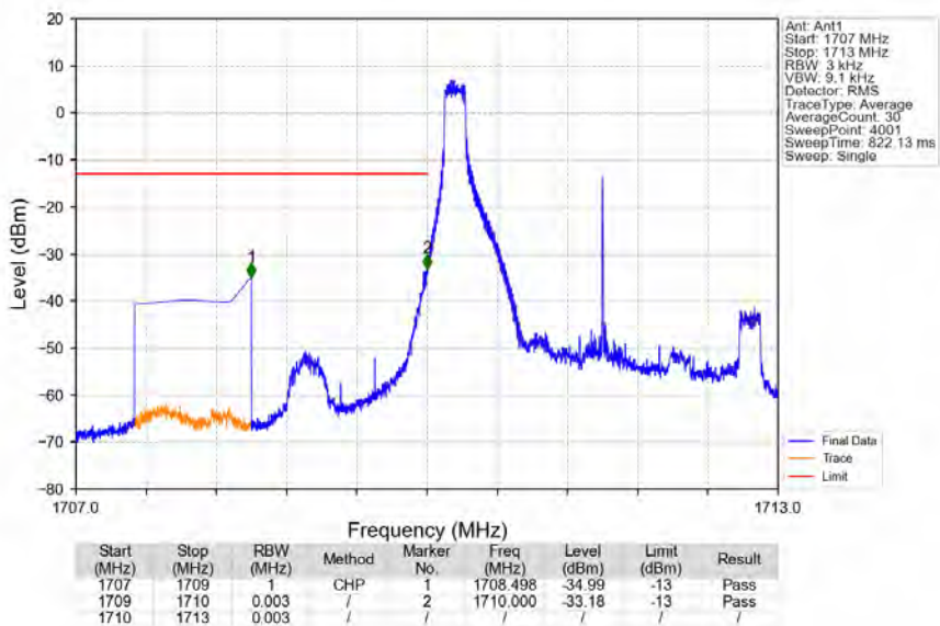
Band66_3MHz_64QAM_LCH_1711.5MHz_RB_1_0_NTV
