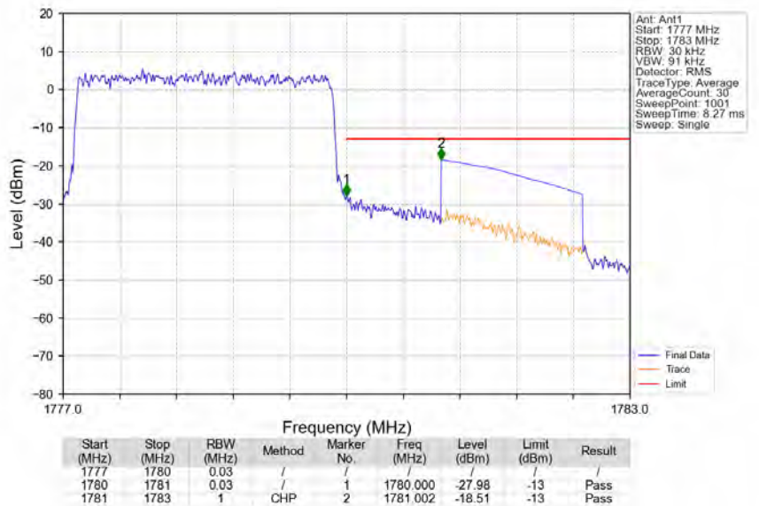
Band66_3MHz_16QAM_HCH_1778.5MHz_RB_15_0_NTNV
