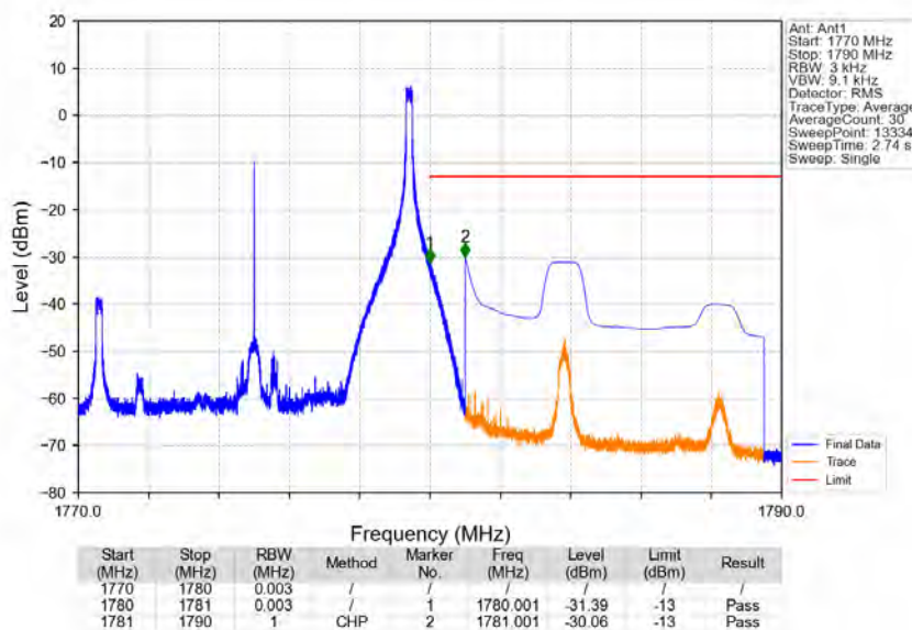
Band66_10MHz_64QAM_HCH_1775MHz_RB_1_49_NTNV
