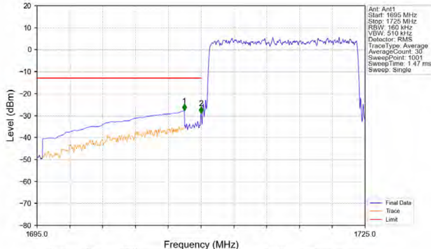
Band66_15MHz_16QAM_LCH_1717.5MHz_RB_75_0_NTNV
