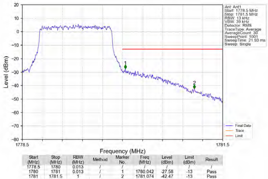
Band66_1.4MHz_16QAM_HCH_1779.3MHz_RB_6_0_NTNV
