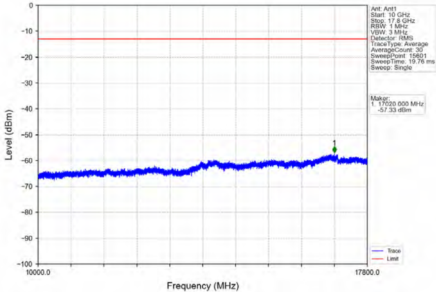
Band66_10MHz_64QAM_LCH_1715MHz_RB_50_0_NTNV
