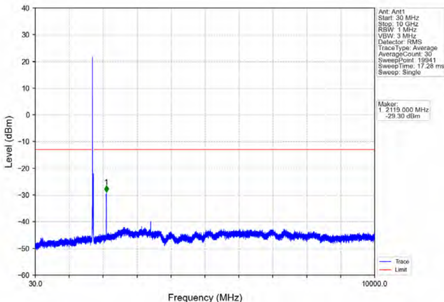
Band66_15MHz_64QAM_LCH_1717.5MHz_RB_1_0_NTNV
