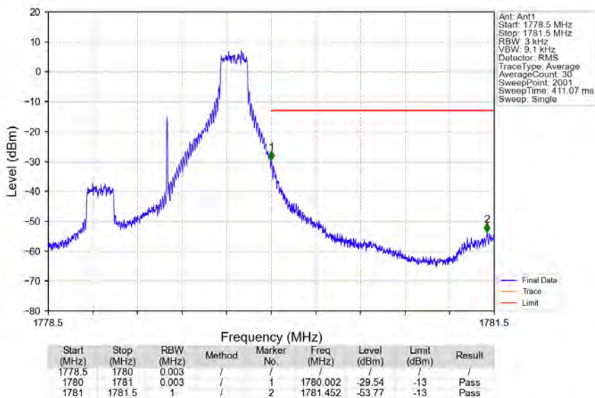
Band66_1.4MHz_64QAM_HCH_1779.3MHz_RB_1_5_NTNV
