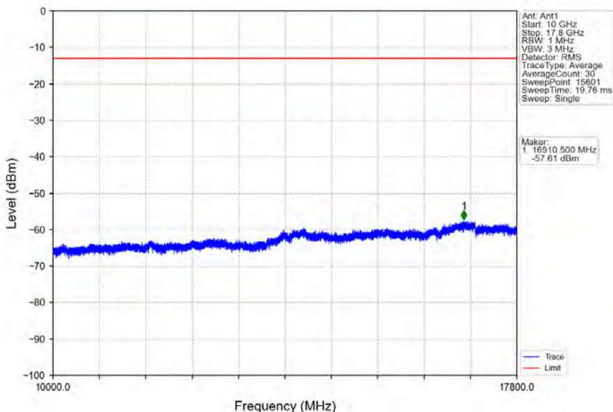
Band66_3MHz_64QAM_HCH_1778.5MHz_RB_1_0_NTNV
