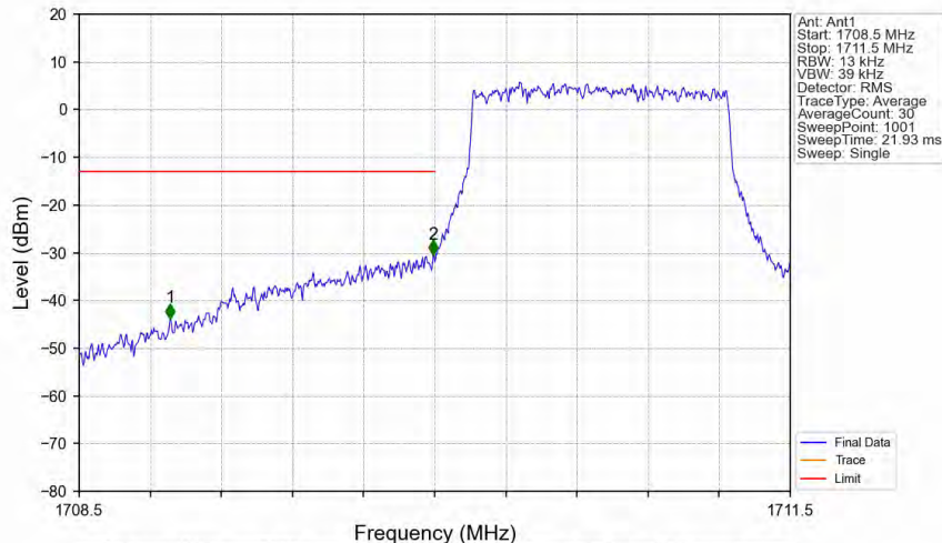
Band66_1.4MHz_16QAM_LCH_1710.7MHz_RB_6_0_NTNV
