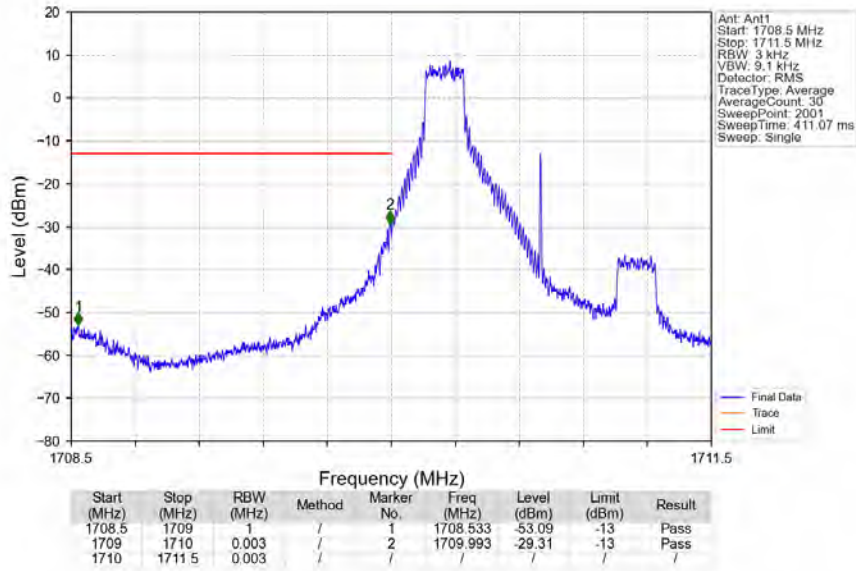
Band66_1.4MHz_16QAM_LCH_1710.7MHz_RB_1_0_NTNV
