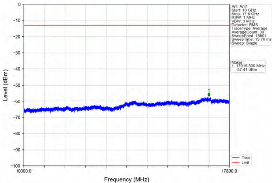
Band66_10MHz_QPSK_MCH_1745MHz_RB_1_0_NTNV
