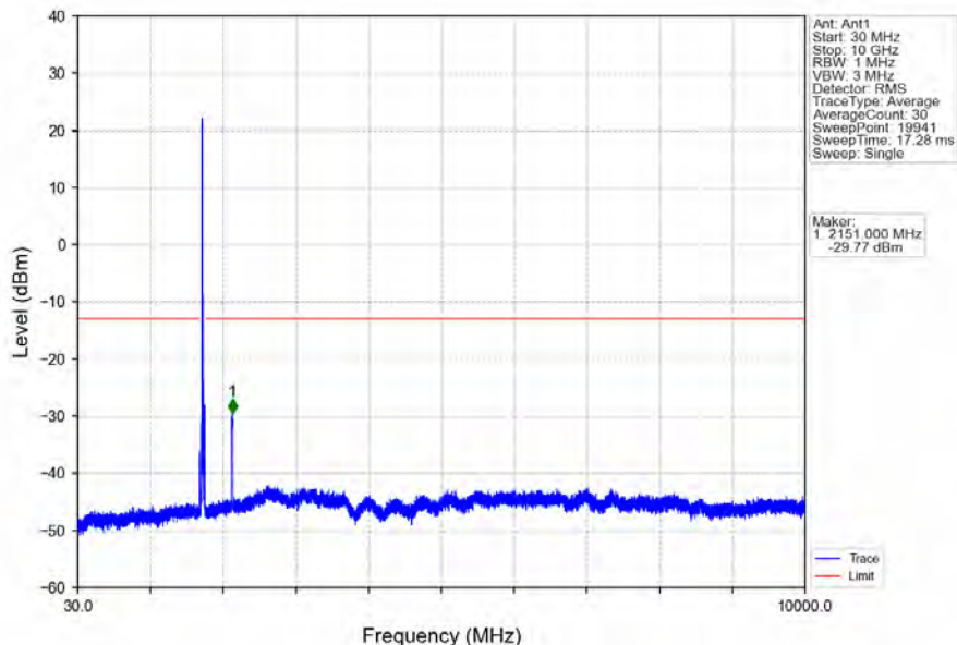
Band66_20MHz_16QAM_MCH_1745MHz_RB_1_0_NTNV
