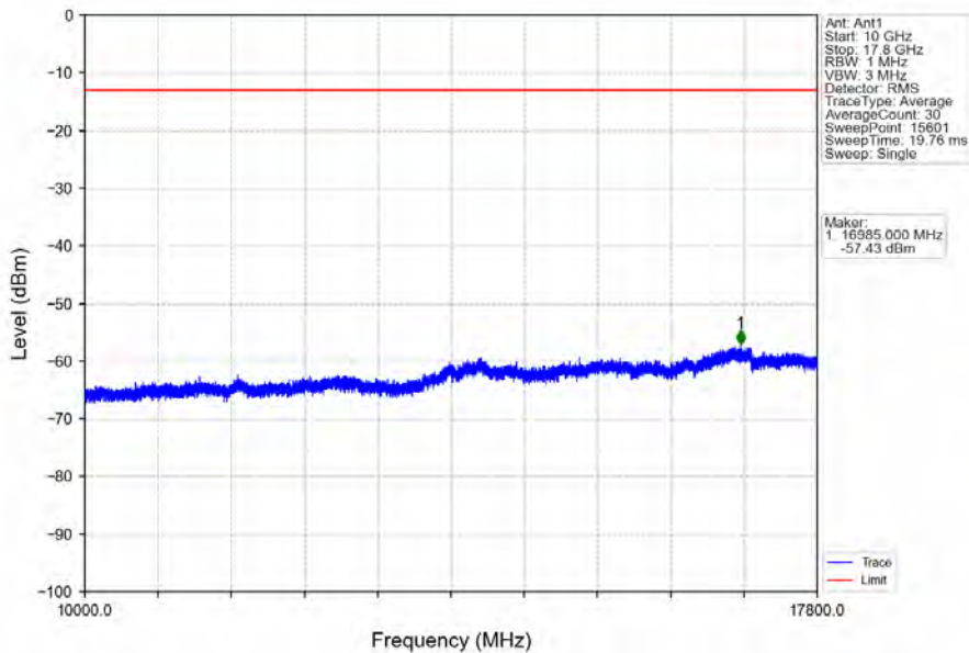
Band66_10MHz_QPSK_HCH_1775MHz_RB_1_0_NTNV
