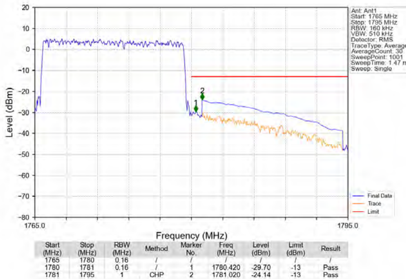
Band66_15MHz_16QAM_HCH_1772.5MHz_RB_75_0_NTNV
