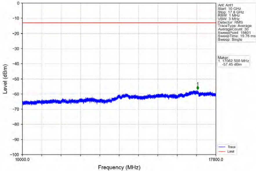
Band66_20MHz_64QAM_LCH_1720MHz_RB_100_0_NTNV
