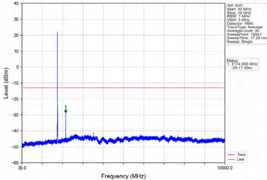
Band66_10MHz_16QAM_HCH_1775MHz_RB_1_0_NTNV
