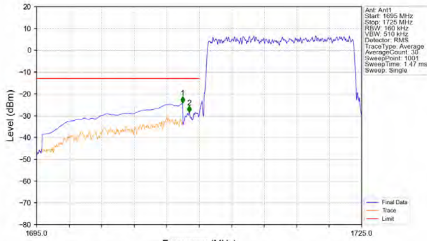
Band66_15MHz_QPSK_LCH_1717.5MHz_RB_75_0_NTNV
