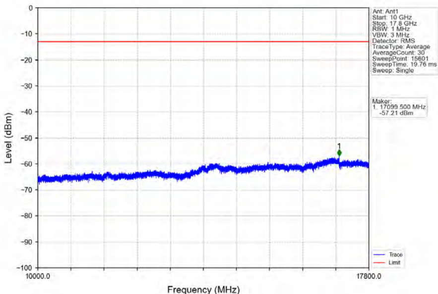
Band66_5MHz_64QAM_MCH_1745MHz_RB_1_0_NTNV
