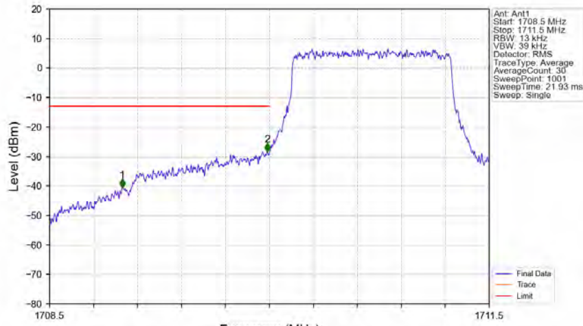
Band66_1.4MHz_QPSK_LCH_1710.7MHz_RB_6_0_NTNV
