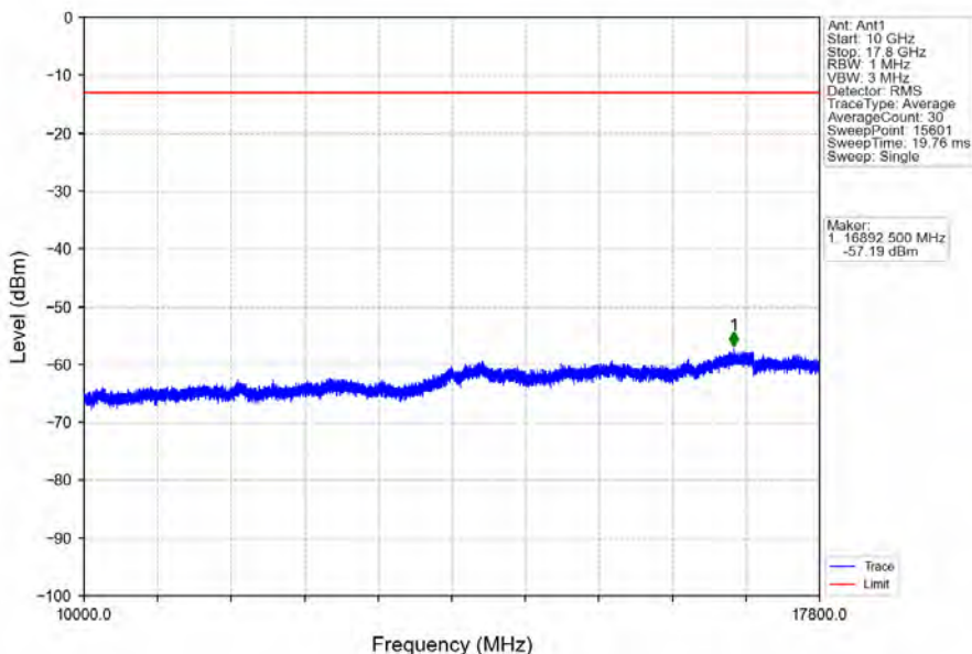
Band66_20MHz_64QAM_HCH_1770MHz_RB_1_0_NTNV
