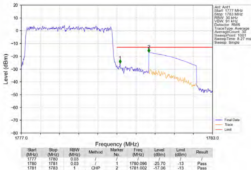
Band66_3MHz_64QAM_HCH_1778.5MHz_RB_15_0_NTNV
