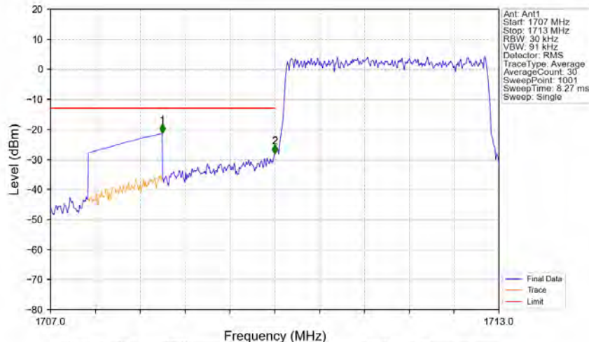
Band66_3MHz_64QAM_LCH_1711.5MHz_RB_15_0_NTNV
