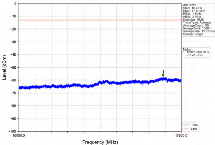
Band66_5MHz_16QAM_HCH_1777.5MHz_RB_1_0_NTNV
