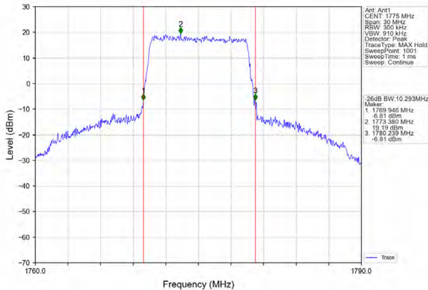
Band66_10MHz_QPSK_HCH_1775MHz_RB_50_0_NTNV
