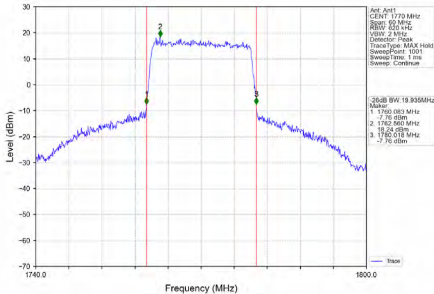
Band66_20MHz_64QAM_HCH_1770MHz_RB_100_0_NTNV
