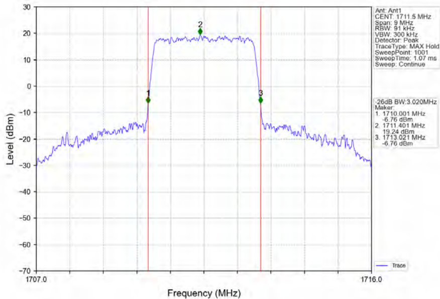
Band66_3MHz_QPSK_LCH_1711.5MHz_RB_15_0_NTNV
