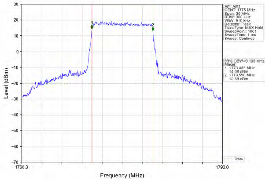
Band66_10MHz_QPSK_HCH_1775MHz_RB_50_0_NTV
