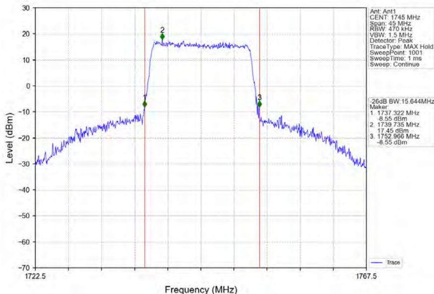
Band66_15MHz_64QAM_MCH_1745MHz_RB_75_0_NTNV
