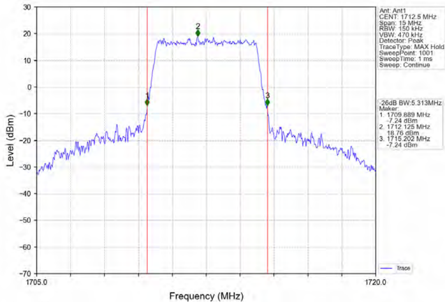
Band66_5MHz_16QAM_LCH_1712.5MHz_RB_25_0_NTNV
