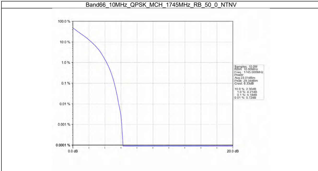
Band66_10MHz_QPSK_MCH_1745MHz_RB_50_0_NTNV
