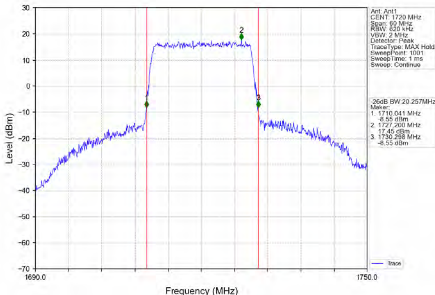
Band66_20MHz_64QAM_LCH_1720MHz_RB_100_0_NTNV
