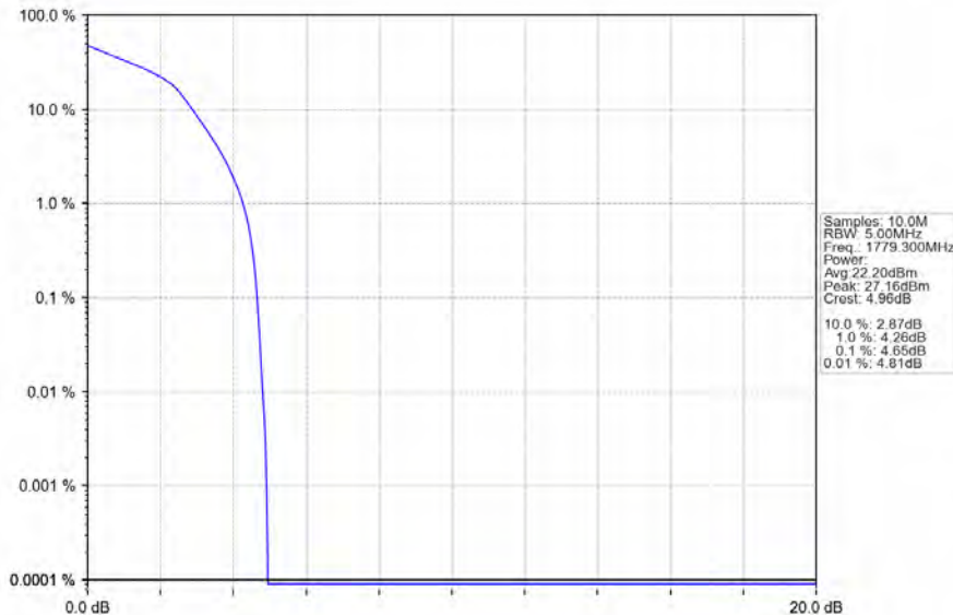
Band66_1.4MHz_16QAM_HCH_1779.3MHz_RB_6_0_NTNV
