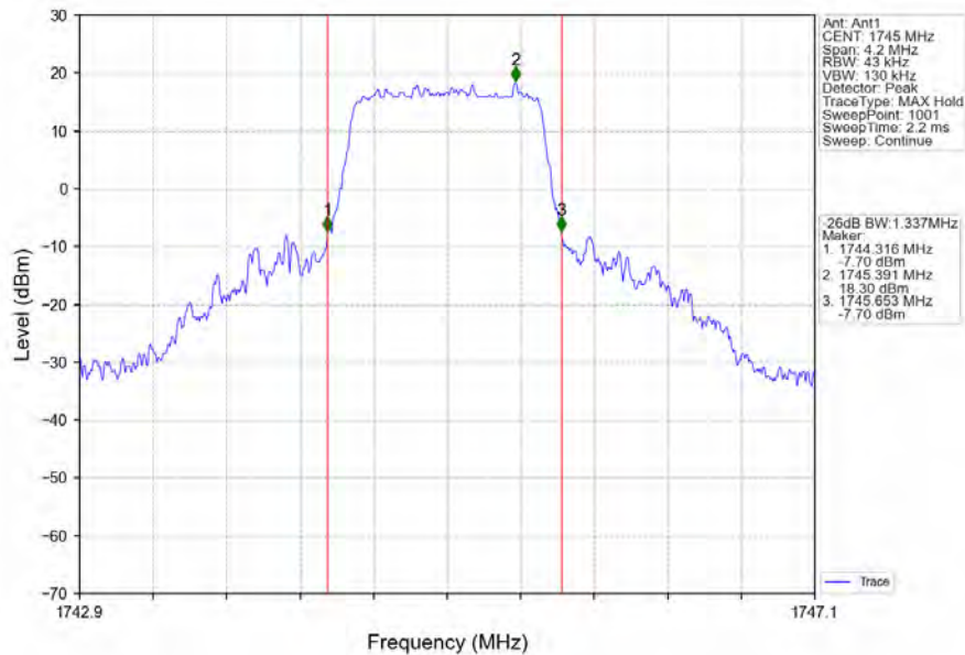
Band66_1.4MHz_64QAM_MCH_1745MHz_RB_6_0_NTNV
