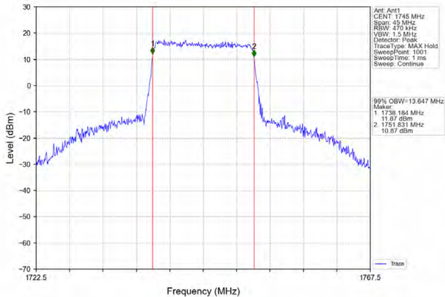
Band66_15MHz_64QAM_MCH_1745MHz_RB_75_0_NTNV
