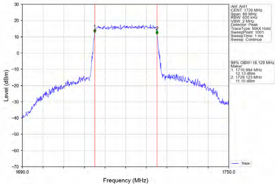
Band66_20MHz_64QAM_LCH_1720MHz_RB_100_0_NTNV
