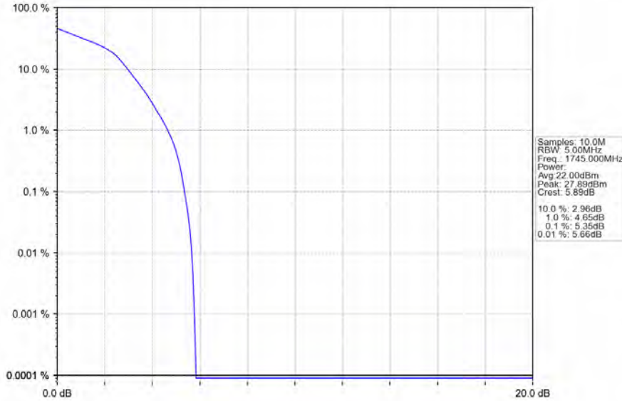
Band66_1.4MHz_16QAM_MCH_1745MHz_RB_6_0_NTNV
