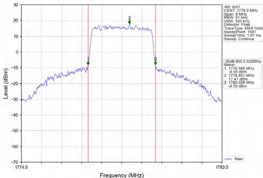
Band66_3MHz_64QAM_HCH_1778.5MHz_RB_15_0_NTNV
