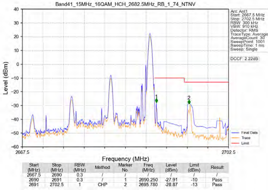
Band41_15MHz_16QAM_HCH_2682.5MHz_RB_1_74_NTNV
