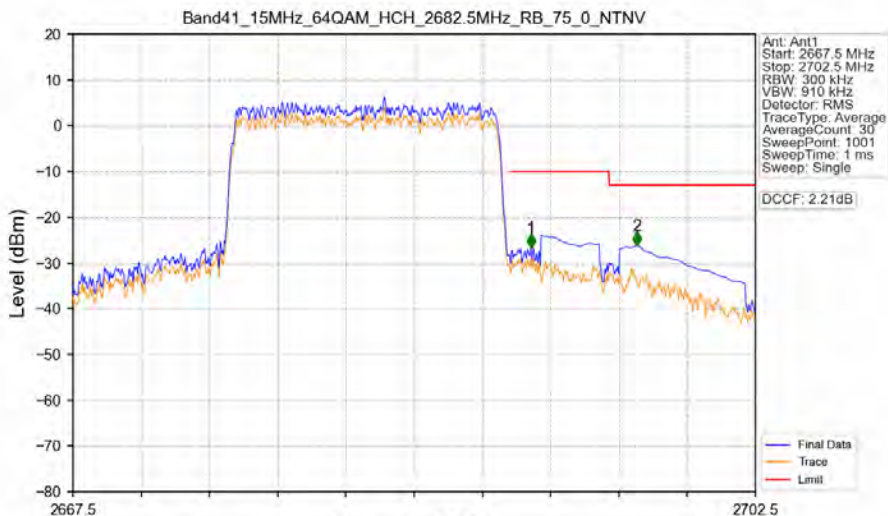
Band41_15MHz_64QAM_HCH_2682.5MHz_RB_75_0_NTNV
