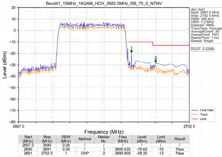
Band41_15MHz_16QAM_HCH_2682.5MHz_RB_75_0_NTNV
