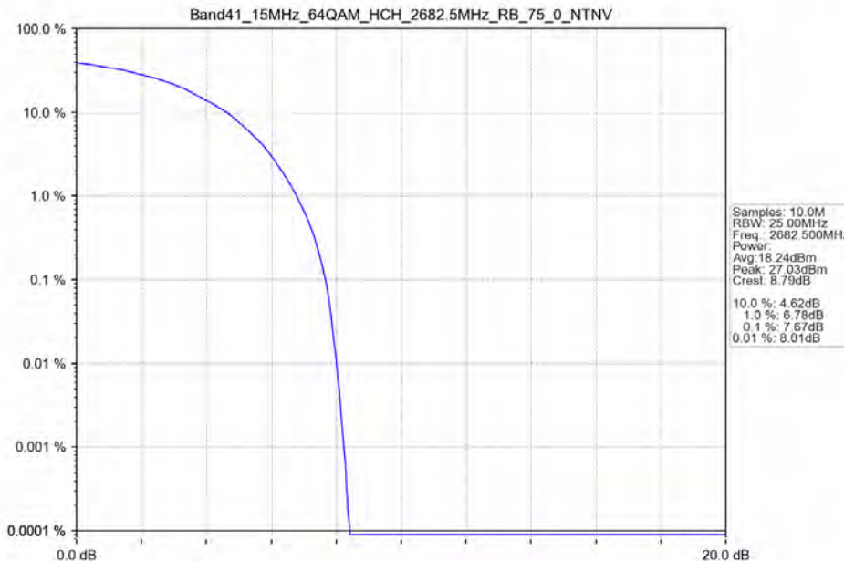
Band41_15MHz_64QAM_HCH_2682.5MHz_RB_75_0_NTNV
