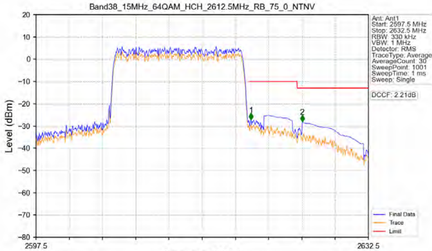
Band38_15MHz_64QAM_HCH_2612.5MHz_RB_75_0_NTNV
