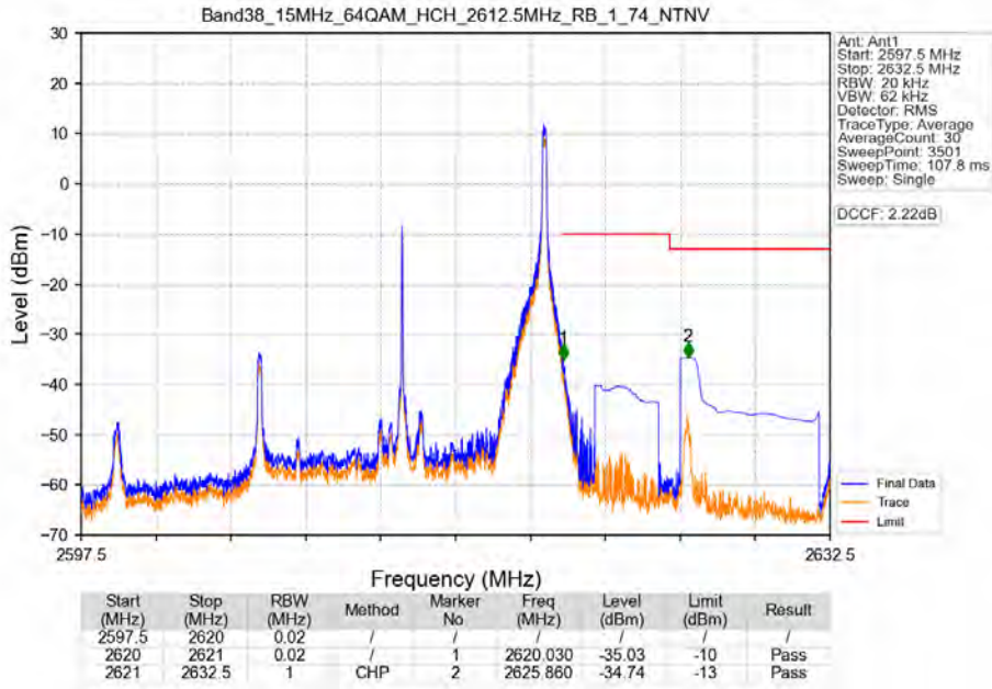
Band38_15MHz_64QAM_HCH_2612.5MHz_RB_1_74_NTNV
