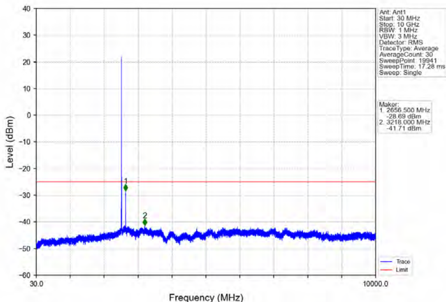
Band7_5MHz_16QAM_MCH_2535MHz_RB_1_0_NTNV
