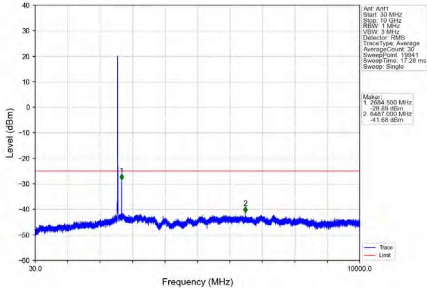
Band7_10MHz_64QAM_HCH_2565MHz_RB_1_0_NTNV
