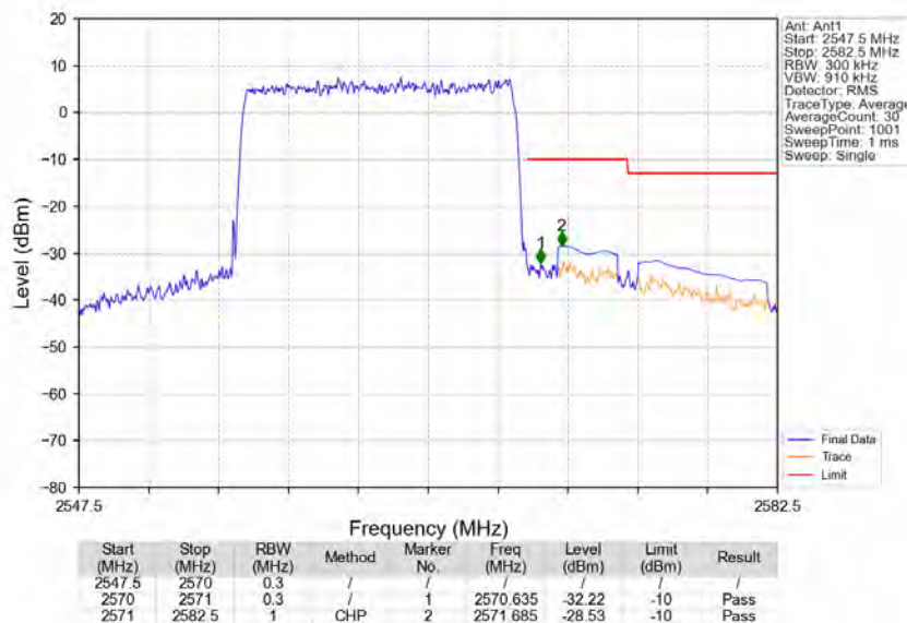
Band7_15MHz_16QAM_HCH_2562.5MHz_RB_75_0_NTNV
