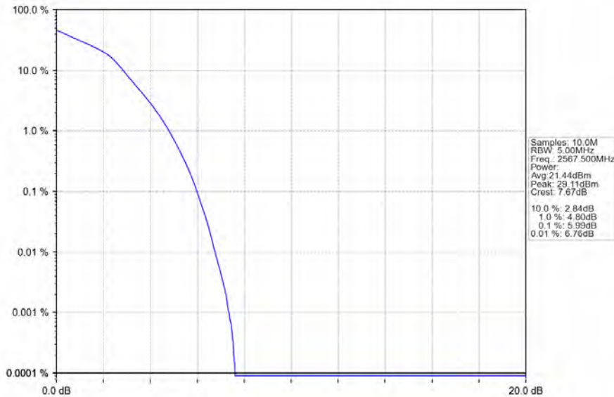
Band7_5MHz_16QAM_HCH_2567.5MHz_RB_25_0_NTNV
