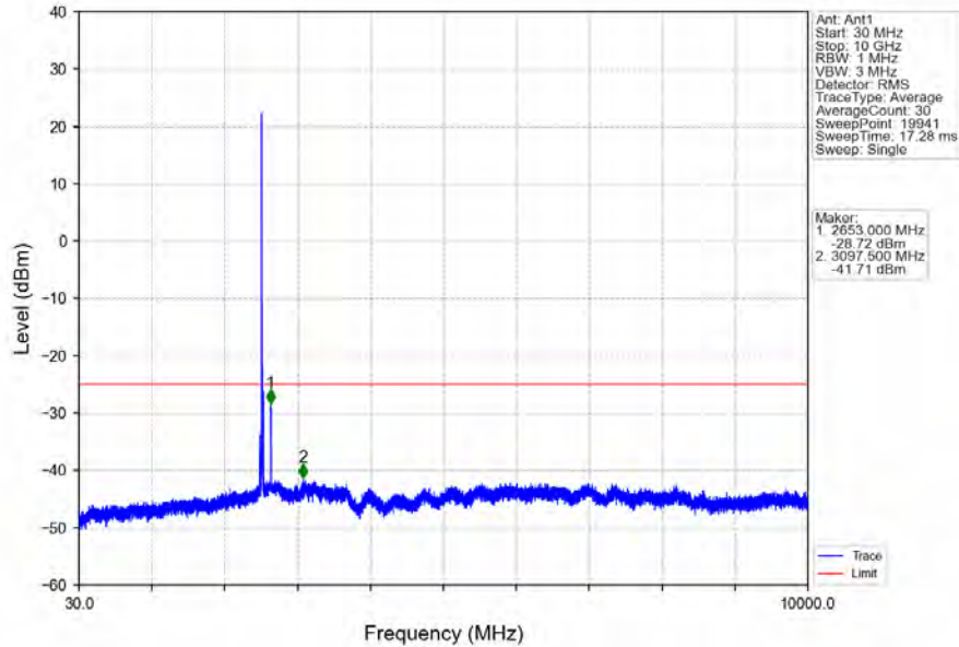
Band7_15MHz_16QAM_MCH_2535MHz_RB_1_0_NTNV
