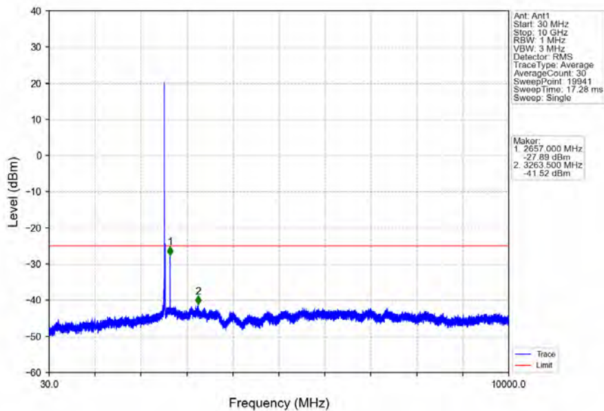
Band7_10MHz_64QAM_MCH_2535MHz_RB_1_0_NTNV
