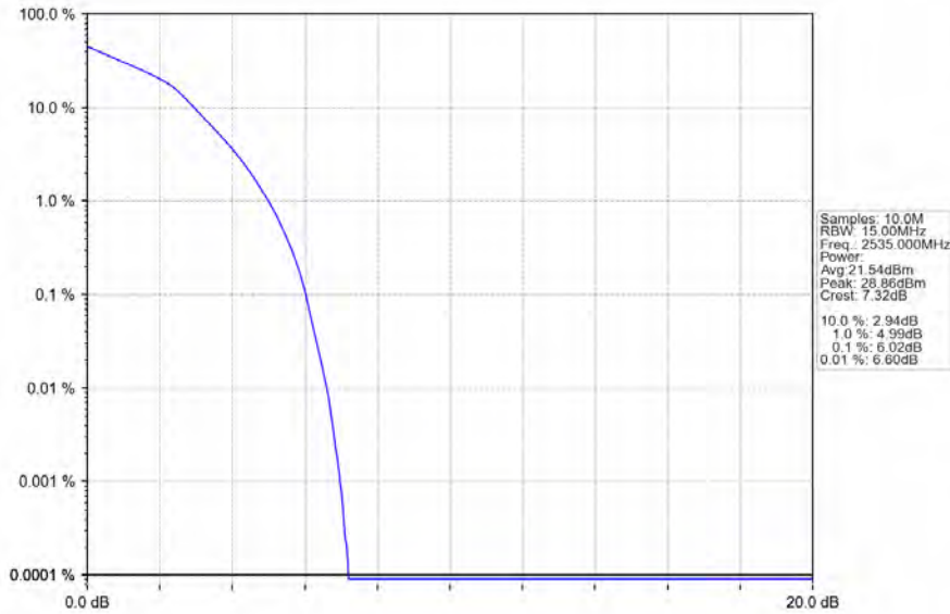
Band7_15MHz_16QAM_MCH_2535MHz_RB_75_0_NTNV
