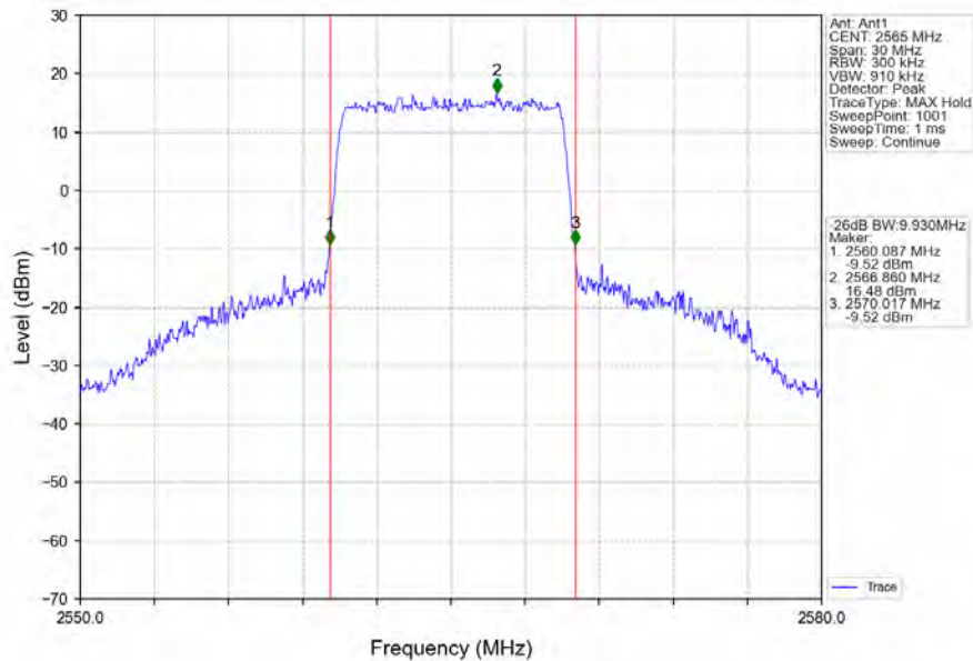
Band7_10MHz_64QAM_HCH_2565MHz_RB_50_0_NTNV
