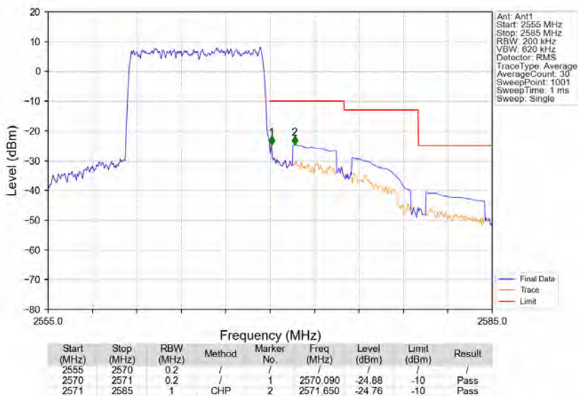
Band7 10MHz QPSK_HCH_2565MHz RB 50_0 NTN
