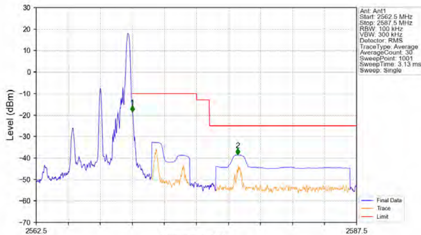
Band7_5MHz_64QAM_HCH_2567.5MHz_RB_1_24_NTNV
