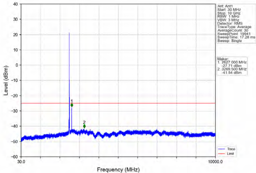
Band7_10MHz_64QAM_LCH_2505MHz_RB_1_0_NTNV
