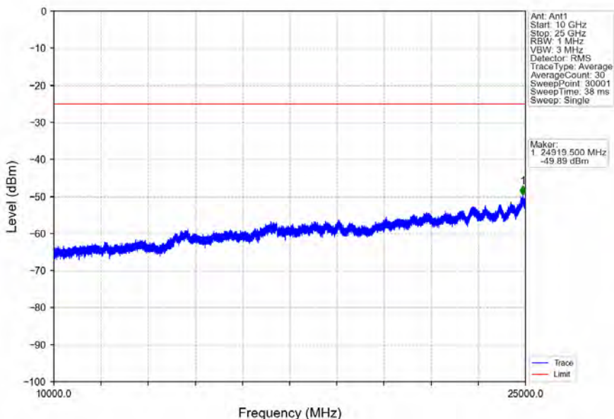
Band7_15MHz_16QAM_LCH_2507.5MHz_RB_1_0_NTNV
