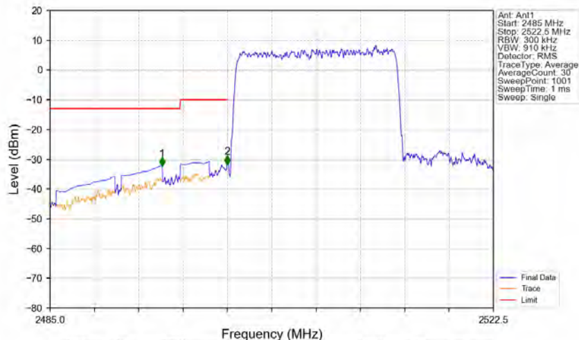
Band7_15MHz_16QAM_LCH_2507.5MHz_RB_75_0_NTNV
