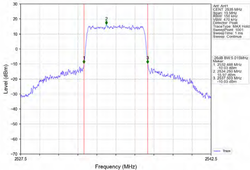
Band7_5MHz_64QAM_MCH_2535MHz_RB_25_0_NTNV
