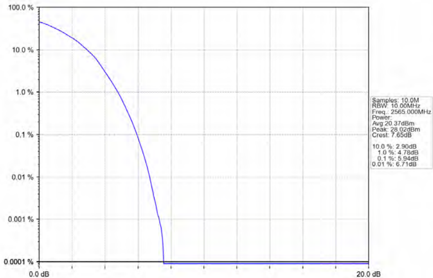
Band7_10MHz_64QAM_HCH_2565MHz_RB_50_0_NTNV
