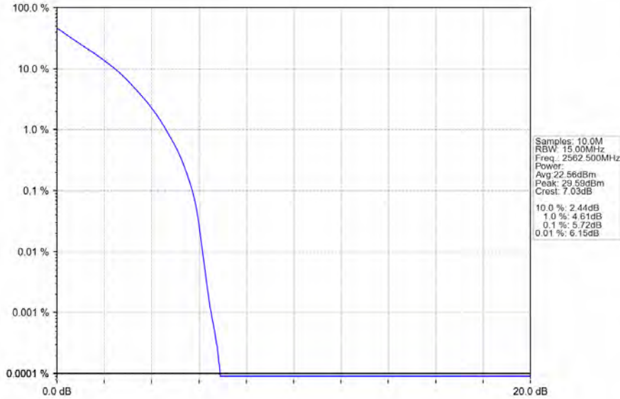
Band7_15MHz_QPSK_HCH_2562.5MHz_RB_75_0_NTNV
