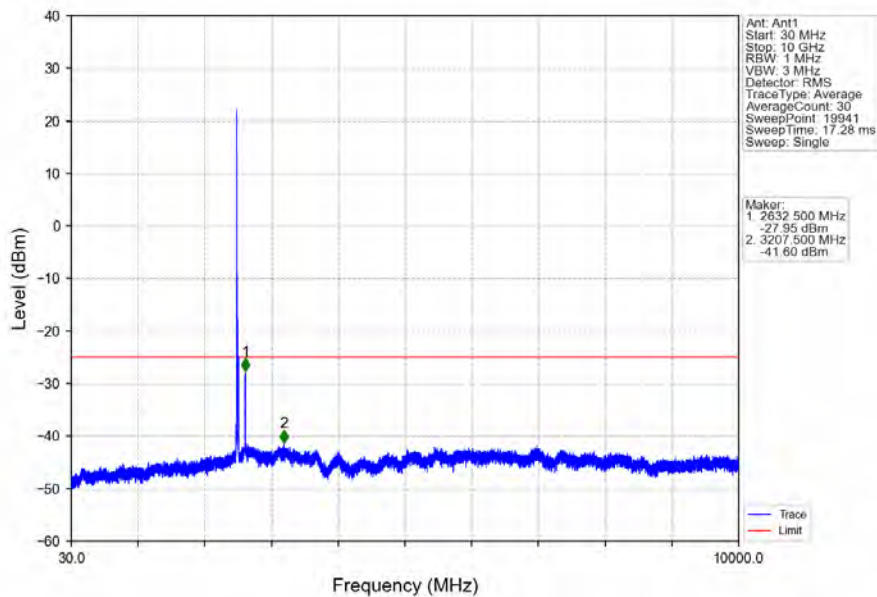
Band7_15MHz_64QAM_LCH_2507.5MHz_RB_1_0_NTV
