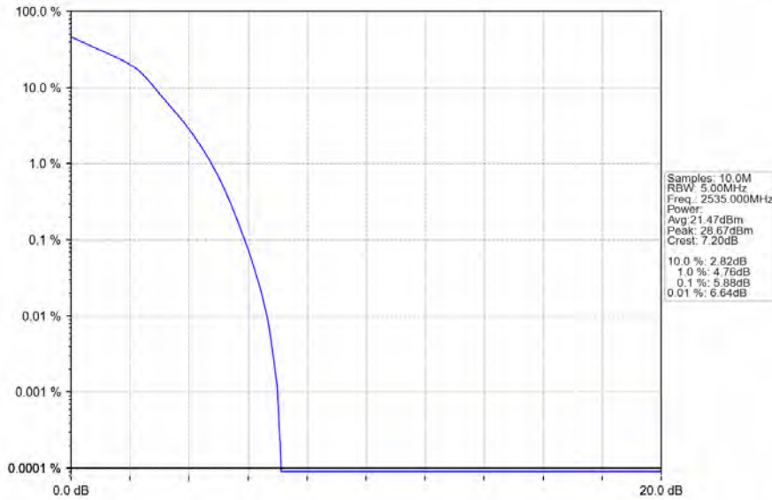
Band7_5MHz_16QAM_MCH_2535MHz_RB_25_0_NTNV
