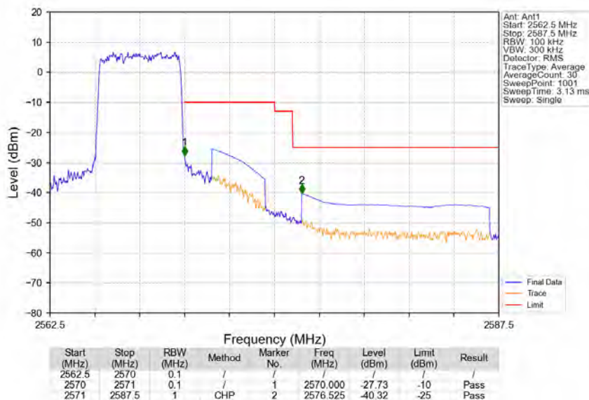
Band7_5MHz_16QAM_HCH_2567.5MHz_RB_25_0_NTNV
