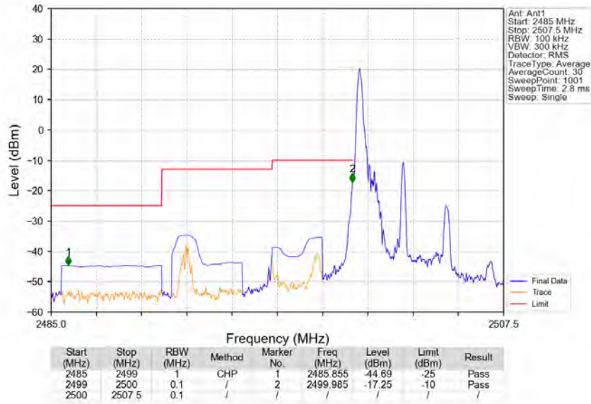
Band7_5MHz_64QAM_LCH_2502.5MHz_RB_1_0_NTNV
