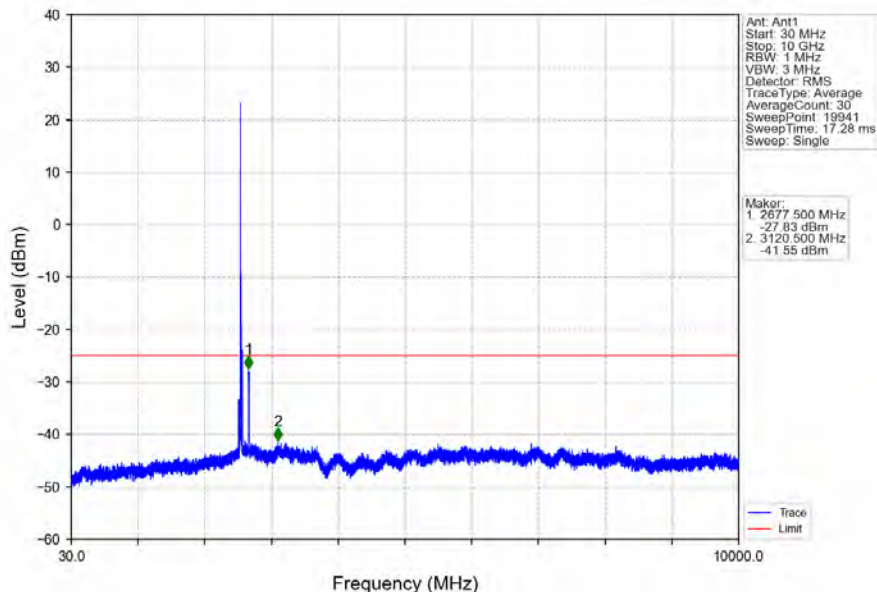
Band7_15MHz_QPSK_HCH_2562.5MHz_RB_1_0_NTNV
