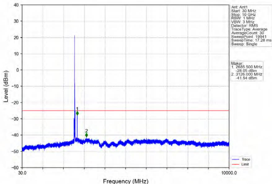
Band7_15MHz_16QAM_HCH_2562.5MHz_RB_1_0_NTNV
