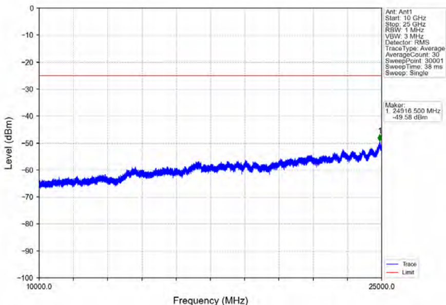
Band7_5MHz_16QAM_MCH_2535MHz_RB_1_0_NTNV
