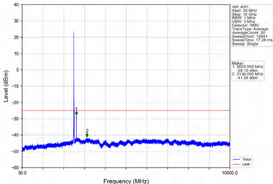
Band7_15MHz_16QAM_LCH_2507.5MHz_RB_1_0_NTNV
