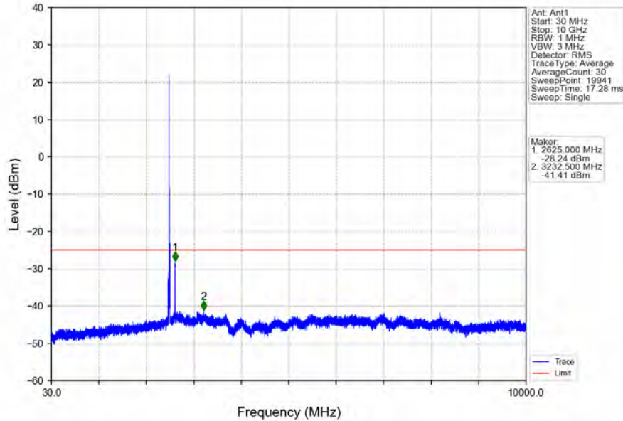
Band7_10MHz_16QAM_LCH_2505MHz_RB_1_0_NTNV
