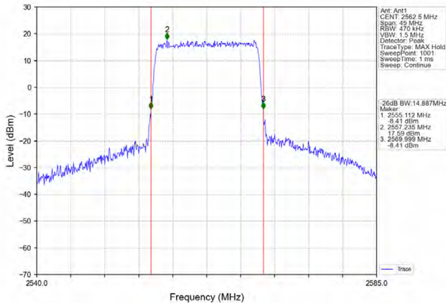
Band7_15MHz_16QAM_HCH_2562.5MHz_RB_75_0_NTNV
