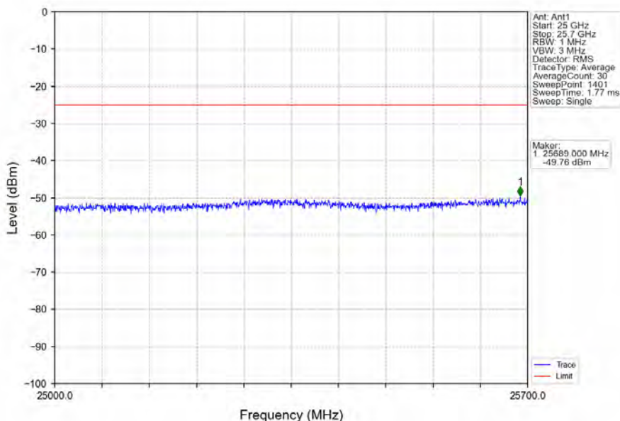
Band7_5MHz_64QAM_HCH_2567.5MHz_RB_1_24_NTNV
