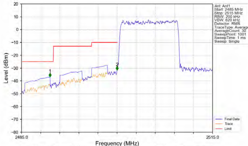
Band7_10MHz_16QAM_LCH_2505MHz_RB_50_0_NTNV
