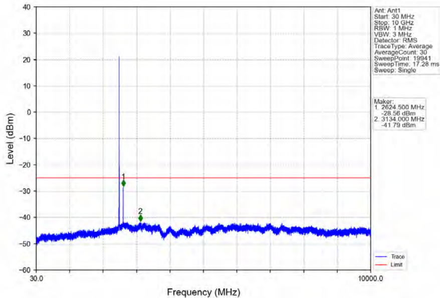
Band7_5MHz_64QAM_LCH_2502.5MHz_RB_1_0_NTNV
