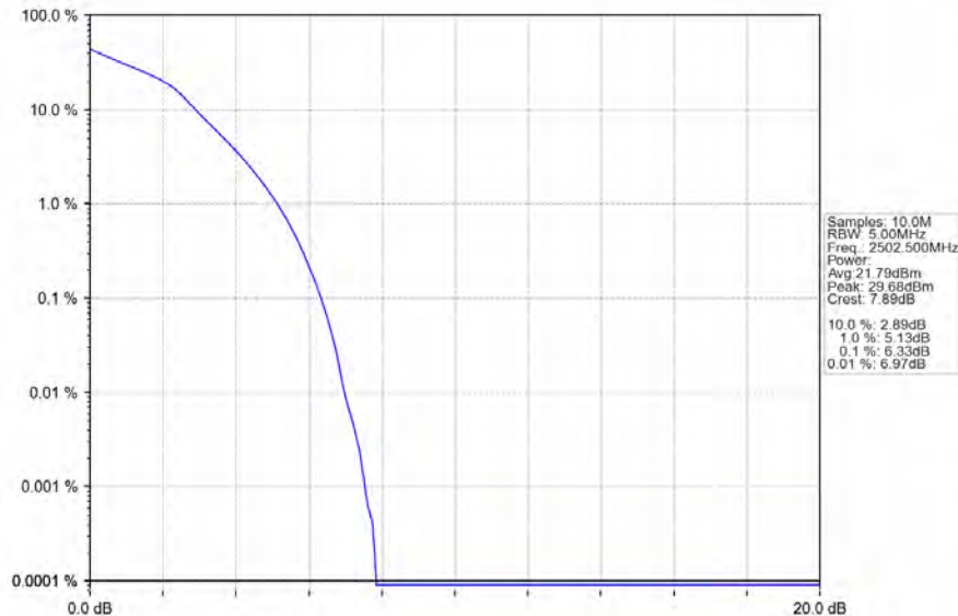
Band7_5MHz_16QAM_LCH_2502.5MHz_RB_25_0_NTNV
