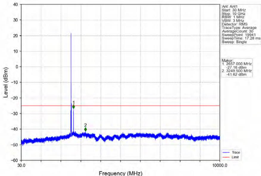
Band7_10MHz_16QAM_MCH_2535MHz_RB_1_0_NTNV
