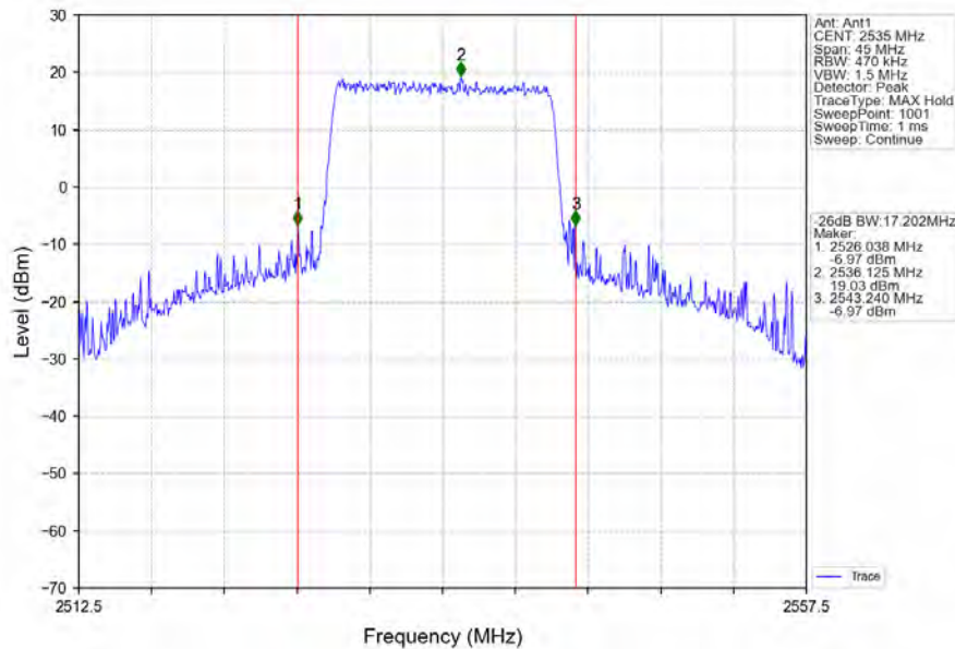
Band7_15MHz_QPSK_MCH_2535MHz_RB_75_0_NTNV
