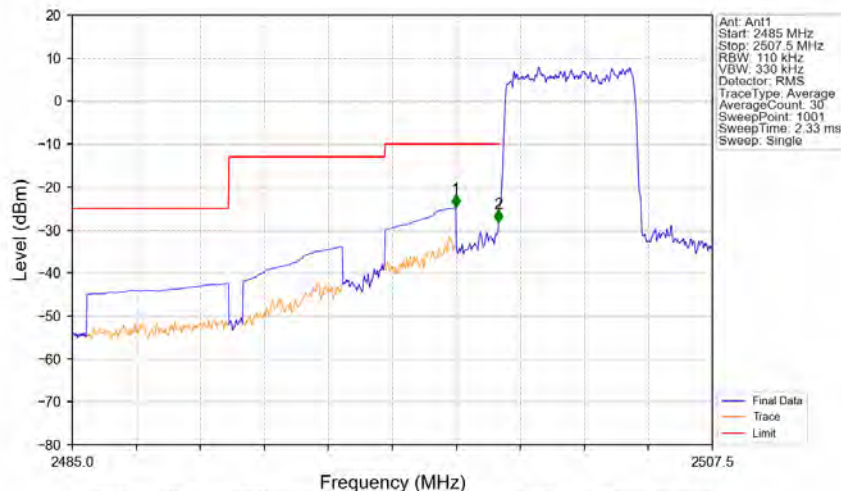
Band7_5MHz_16QAM_LCH_2502.5MHz_RB_25_0_NTNV
