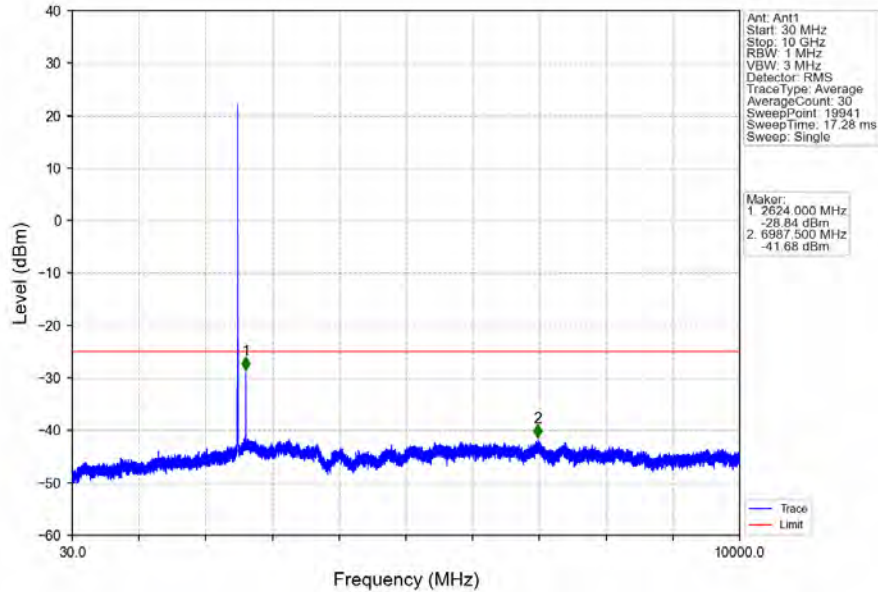
Band7_5MHz_16QAM_LCH_2502.5MHz_RB_1_0_NTNV
