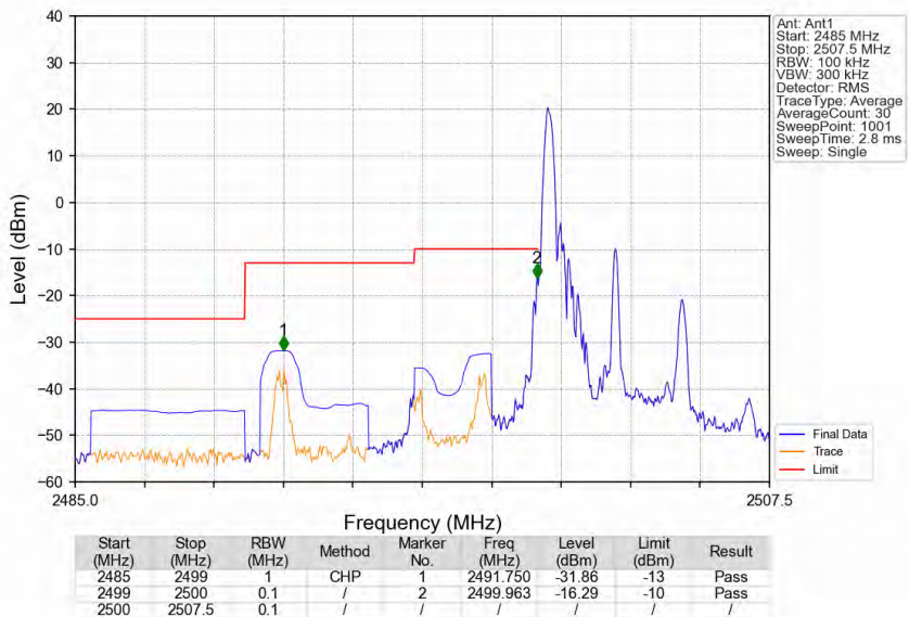
Band7_5MHz_16QAM_LCH_2502.5MHz_RB_1_0_NTNV
