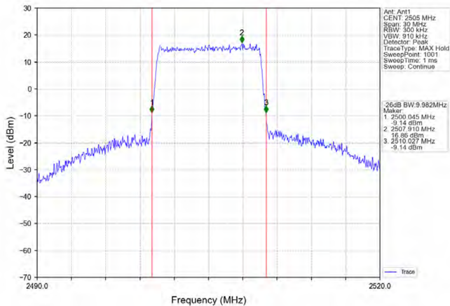
Band7_10MHz_64QAM_LCH_2505MHz_RB_50_0_NTNV
