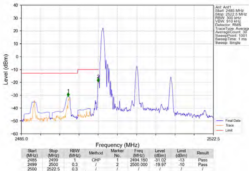
Band7_15MHz_16QAM_LCH_2507.5MHz_RB_1_0_NTNV
