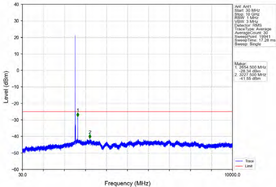
Band7_5MHz_64QAM_MCH_2535MHz_RB_1_0_NTNV
