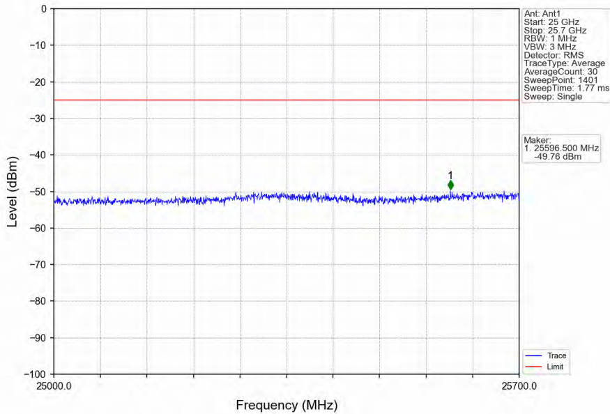
Band7_10MHz_16QAM_LCH_2505MHz_RB_50_0_NTNV
