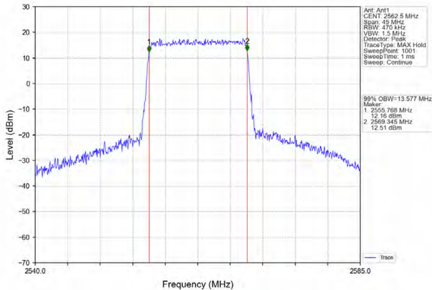
Band7_15MHz_16QAM_HCH_2562.5MHz_RB_75_0_NTNV
