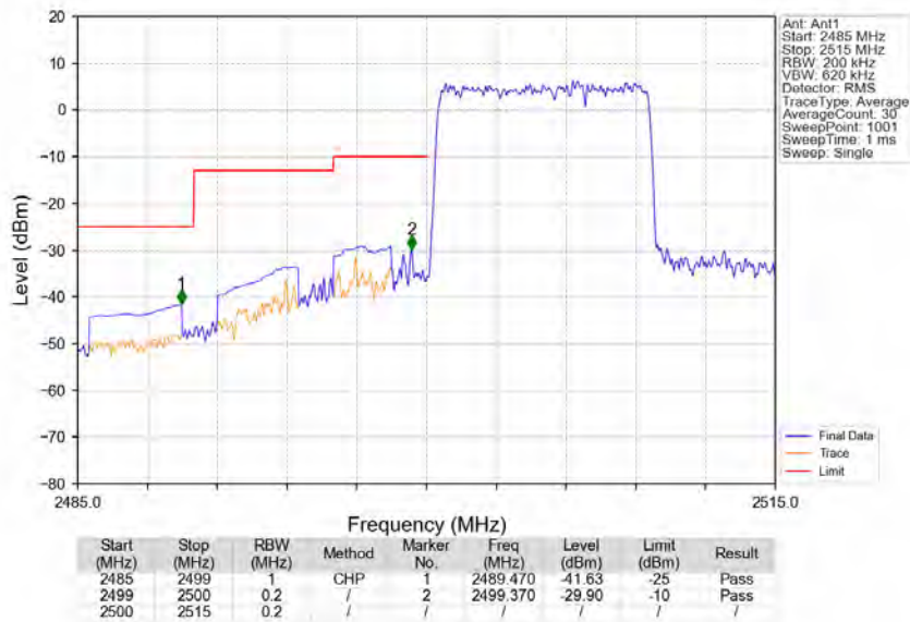
Band7_10MHz_64QAM_LCH_2505MHz_RB_50_0_NTNV
