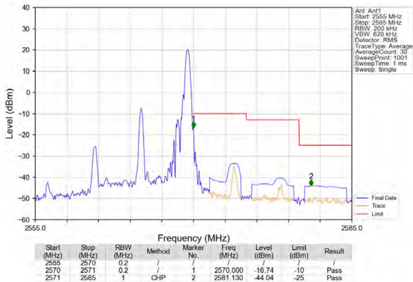
Band7_10MHz_64QAM_HCH_2565MHz_RB_1_49_NTNV
