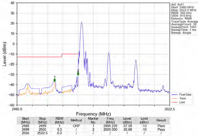
Band7_15MHz_64QAM_LCH_2507.5MHz_RB_1_0_NTV
