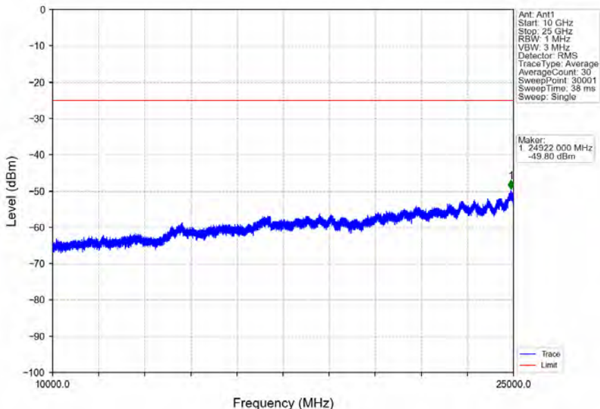
Band7_10MHz_16QAM_MCH_2535MHz_RB_1_0_NTNV
