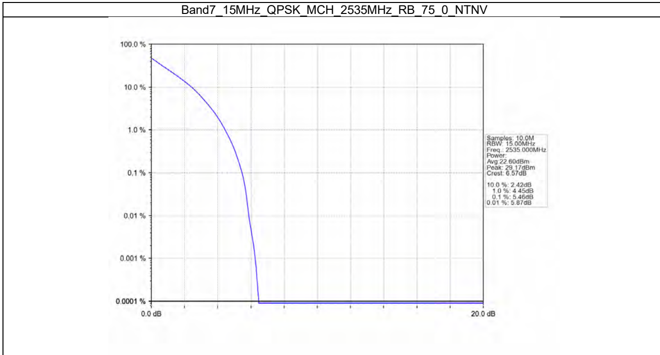
Band7 15MHz_QPSK_MCH_2535MHz_RB_75_0_NTNV
