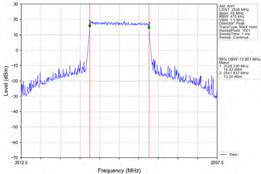
Band7_15MHz_QPSK_MCH_2535MHz_RB_75_0_NTNV
