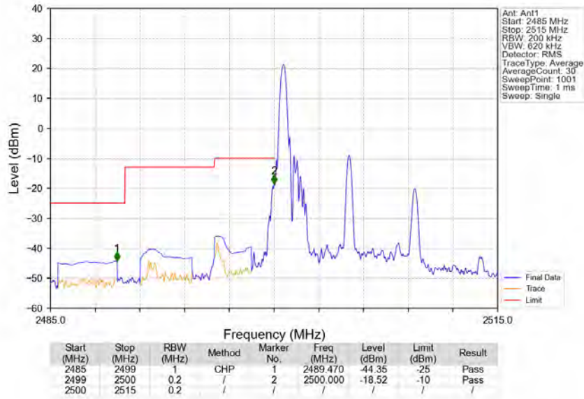
Band7_10MHz_64QAM_LCH_2505MHz_RB_1_0_NTNV
