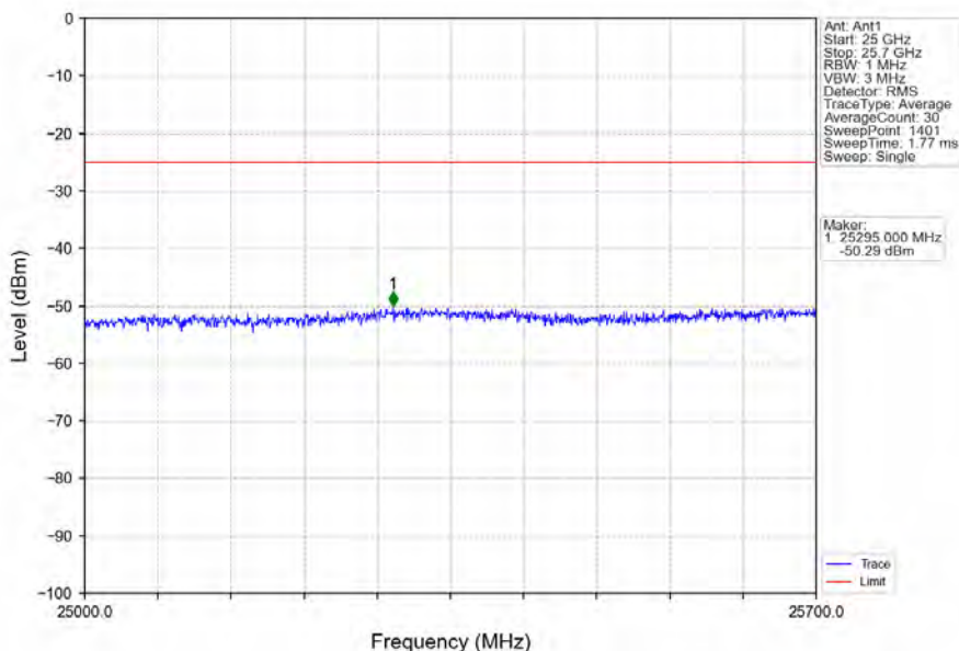
Band7_15MHz_16QAM_LCH_2507.5MHz_RB_75_0_NTNV
