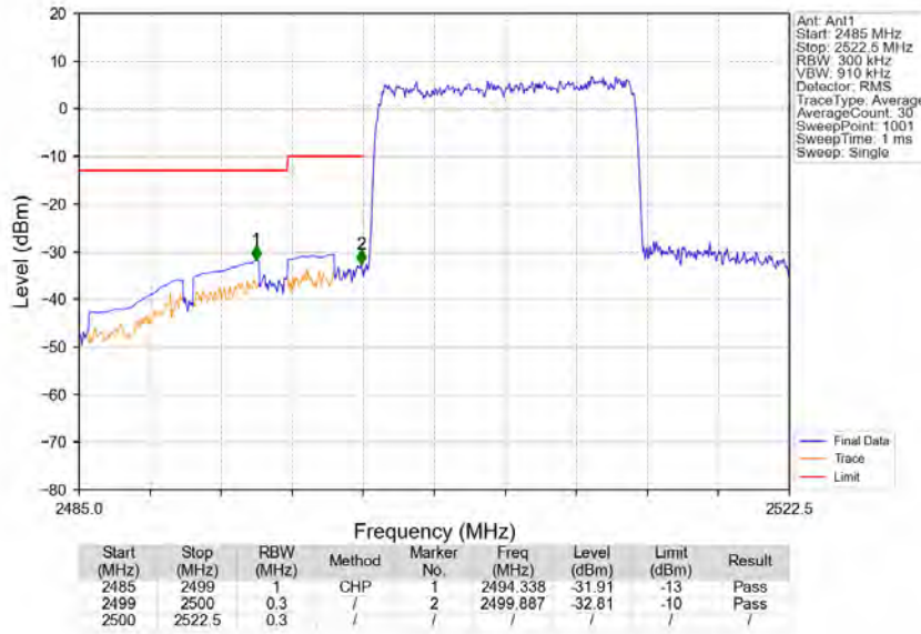
Band7_15MHz_64QAM_LCH_2507.5MHz_RB_75_0_NTNV
