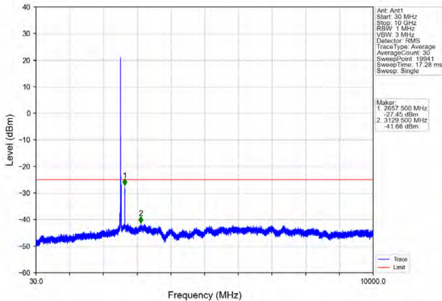
Band7_15MHz_64QAM_MCH_2535MHz_RB_1_0_NTNV
