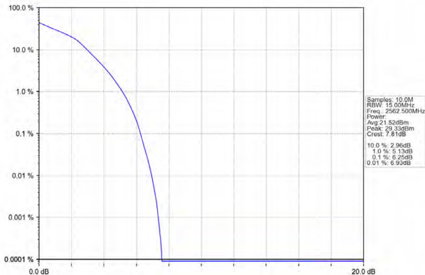
Band7_15MHz_16QAM_HCH_2562.5MHz_RB_75_0_NTNV
