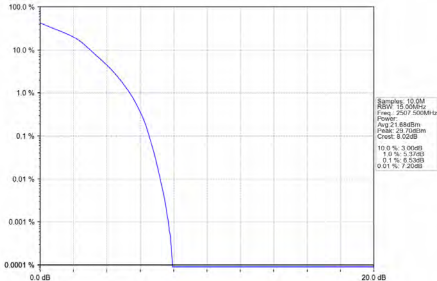
Band7_15MHz_16QAM_LCH_2507.5MHz_RB_75_0_NTNV
