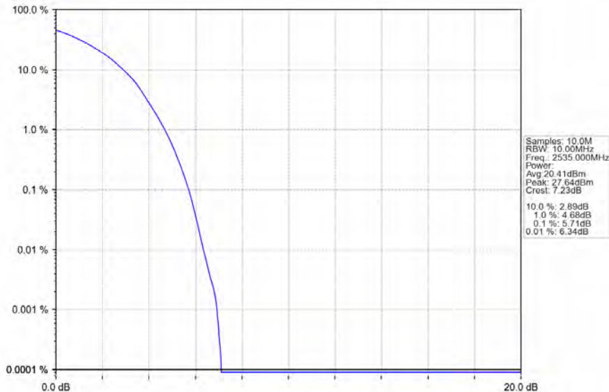
Band7_10MHz_64QAM_MCH_2535MHz_RB_50_0_NTNV
