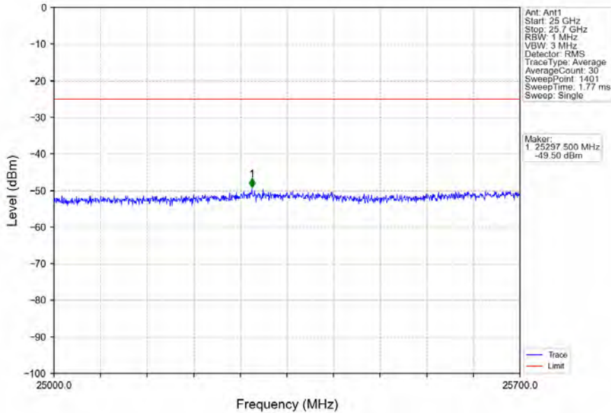
Band7_5MHz_16QAM_HCH_2567.5MHz_RB_1_0_NTNV
