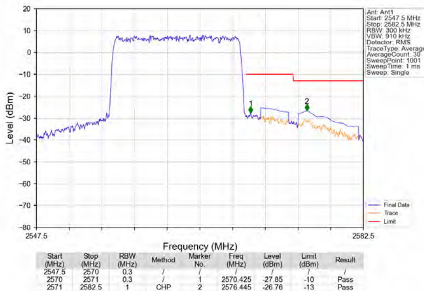
Band7_15MHz_QPSK_HCH_2562.5MHz_RB_75_0_NTNV
