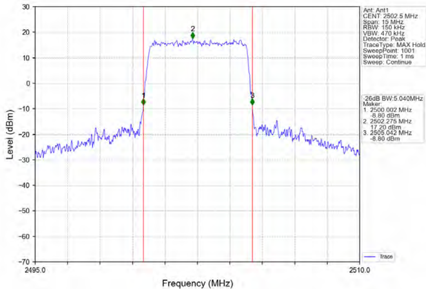
Band7_5MHz_16QAM_LCH_2502.5MHz_RB_25_0_NTNV
