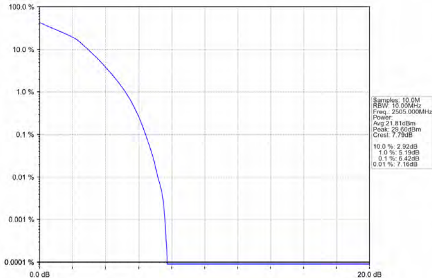
Band7_10MHz_16QAM_LCH_2505MHz_RB_50_0_NTNV
