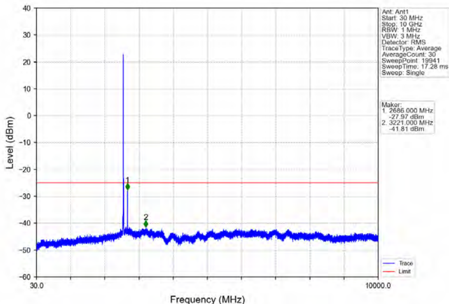
Band7_10MHz_16QAM_HCH_2565MHz_RB_1_0_NTNV
