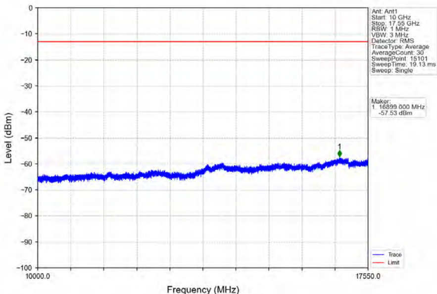
Band4_3MHz_64QAM_MCH_1732.5MHz_RB_1_0_NTNV
