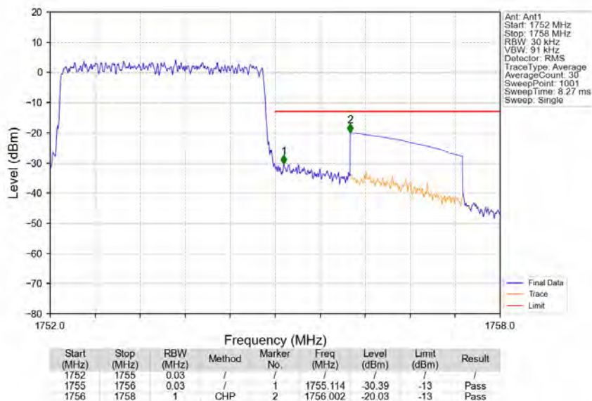
Band4_3MHz_64QAM_HCH_1753.5MHz_RB_15_0_NTNV
