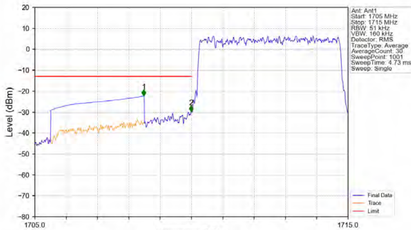
Band4_5MHz_QPSK_LCH_1712.5MHz_RB_25_0_NTNV
