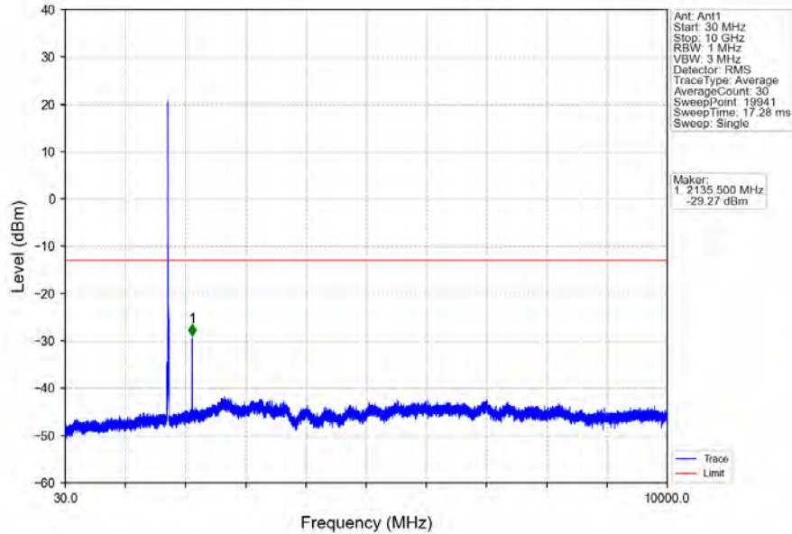
Band4_10MHz_64QAM_MCH_1732.5MHz_RB_1_0_NTNV
