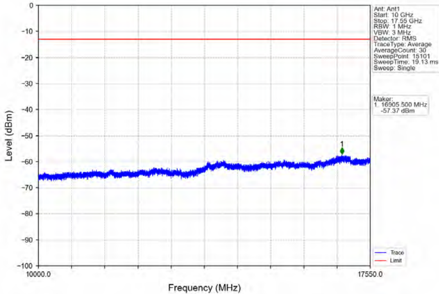
Band4_15MHz_64QAM_LCH_1717.5MHz_RB_75_0_NTNV
