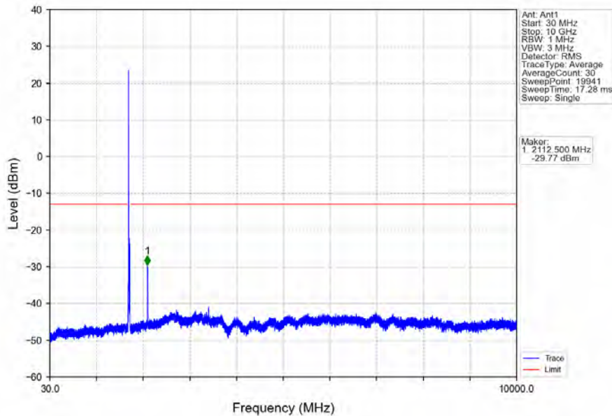
Band4_15MHz_16QAM_LCH_1717.5MHz_RB_1_0_NTNV
