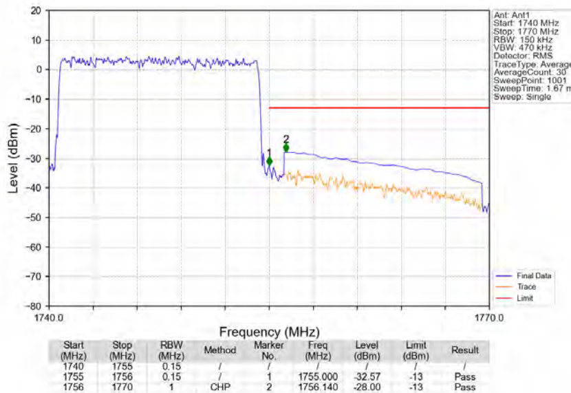
Band4_15MHz_16QAM_HCH_1747.5MHz_RB_75_0_NTNV
