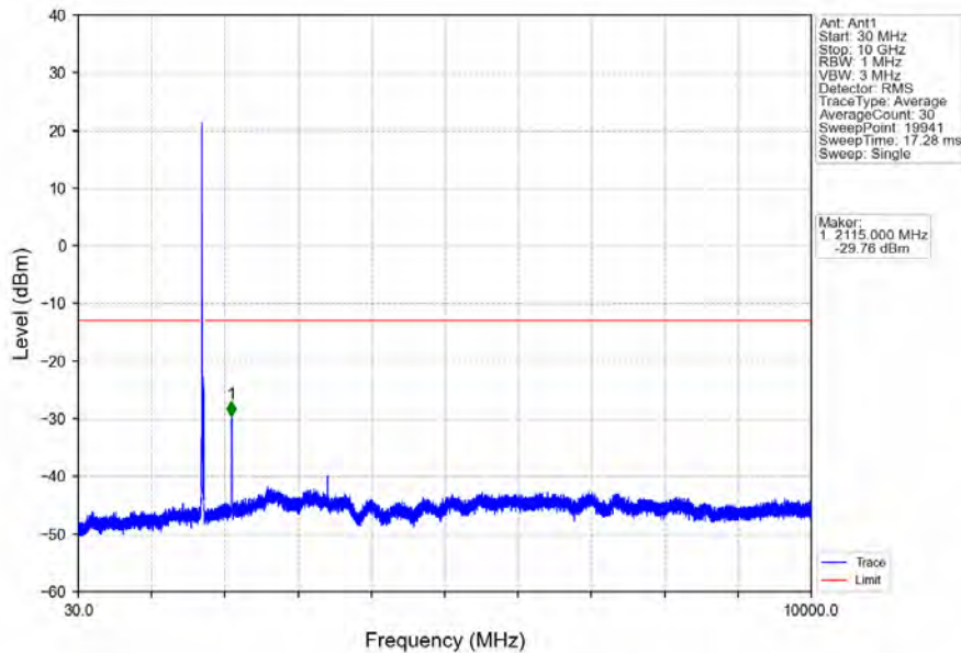
Band4_15MHz_64QAM_LCH_1717.5MHz_RB_1_0_NTNV
