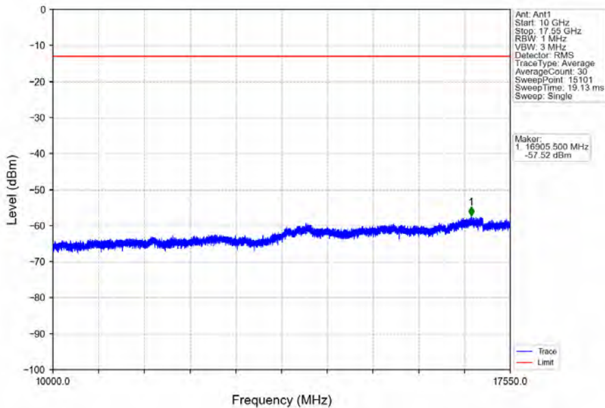
Band4_10MHz_16QAM_HCH_1750MHz_RB_1_0_NTNV
