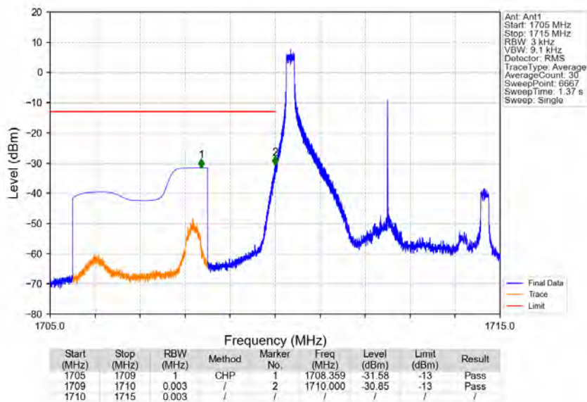
Band4_5MHz_64QAM_LCH_1712.5MHz_RB_1_0_NTNV
