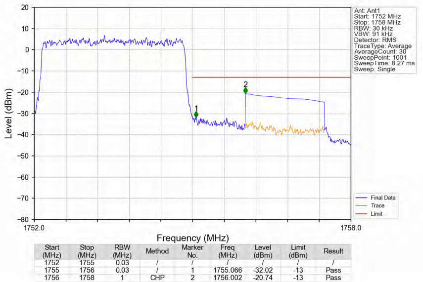
Band4_3MHz_QPSK_HCH_1753.5MHz_RB_15_0_NTNV
