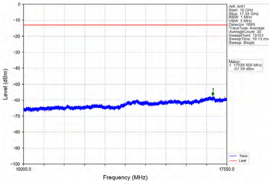
Band4_5MHz_64QAM_MCH_1732.5MHz_RB_1_0_NTNV
