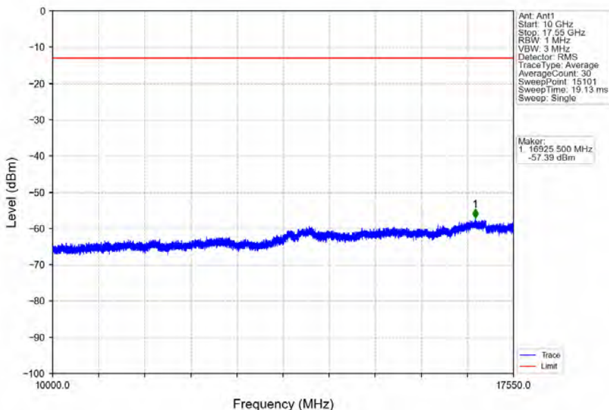
Band4_5MHz_16QAM_HCH_1752.5MHz_RB_1_0_NTNV
