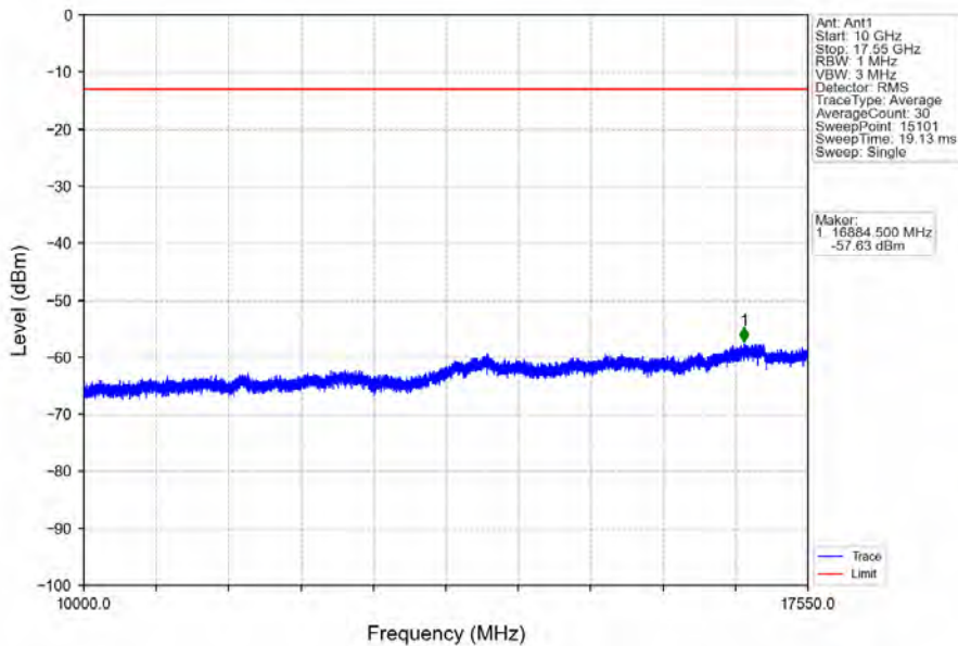
Band4_5MHz_64QAM_HCH_1752.5MHz_RB_1_0_NTNV
