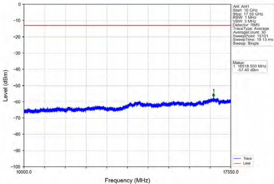
Band4_15MHz_16QAM_HCH_1747.5MHz_RB_1_0_NTNV
