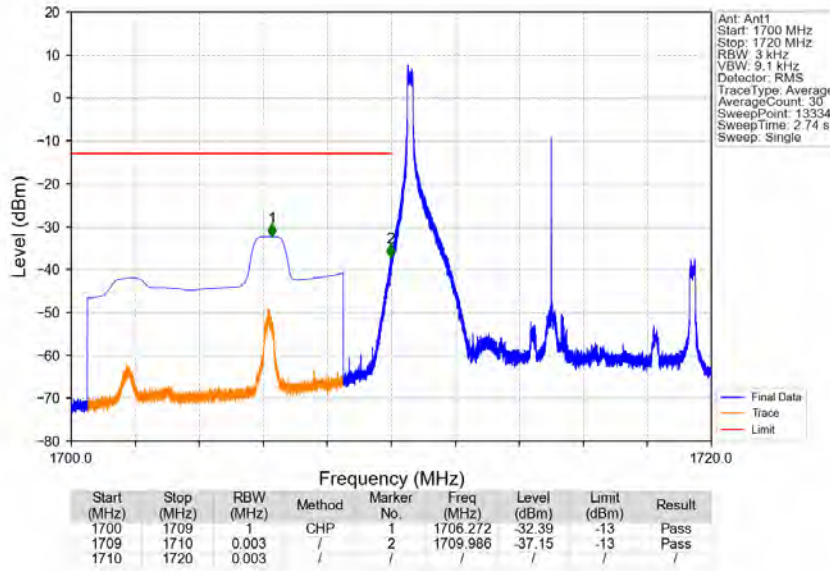
Band4_10MHz_64QAM_LCH_1715MHz_RB_1_0_NTNV
