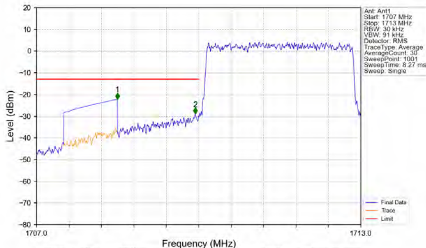
Band4_3MHz_64QAM_LCH_1711.5MHz_RB_15_0_NTNV
