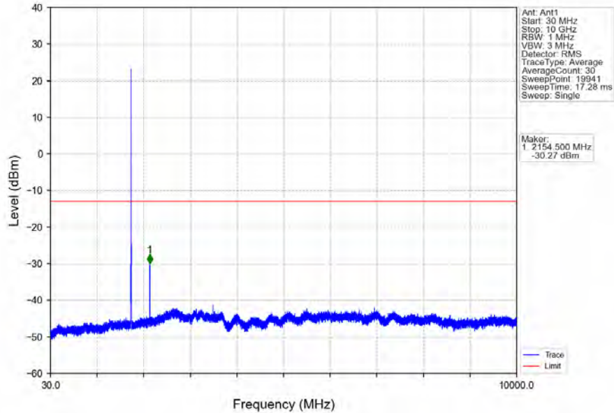
Band4_3MHz_QPSK_HCH_1753.5MHz_RB_1_0_NTNV
