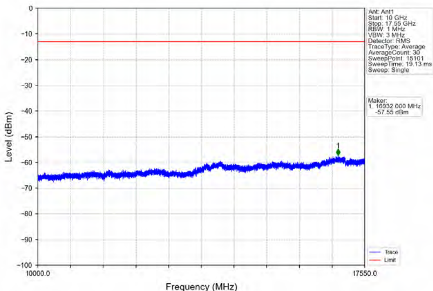
Band4_10MHz_QPSK_LCH_1715MHz_RB_50_0_NTNV
