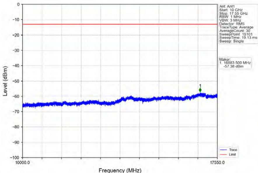
Band4_20MHz_64QAM_LCH_1720MHz_RB_100_0_NTNV
