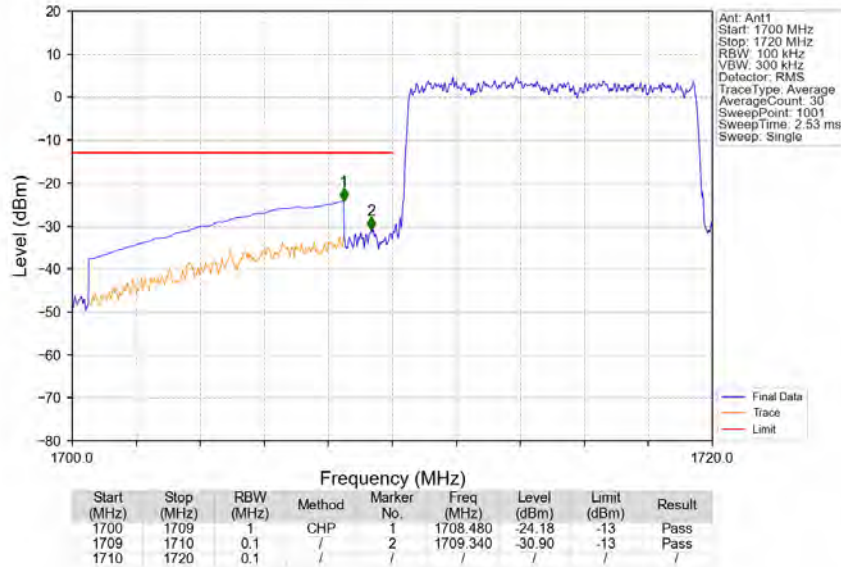
Band4_10MHz_64QAM_LCH_1715MHz_RB_50_0_NTNV
