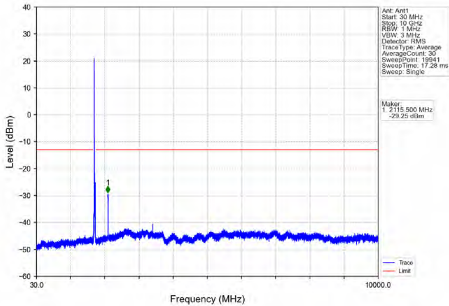
Band4_20MHz_64QAM_LCH_1720MHz_RB_1_0_NTNV
