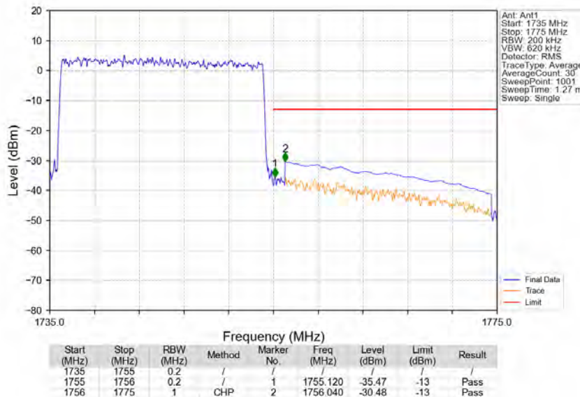
Band4_20MHz_16QAM_HCH_1745MHz_RB_100_0_NTNV
