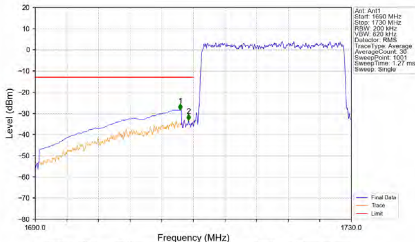
Band4_20MHz_64QAM_LCH_1720MHz_RB_100_0_NTNV
