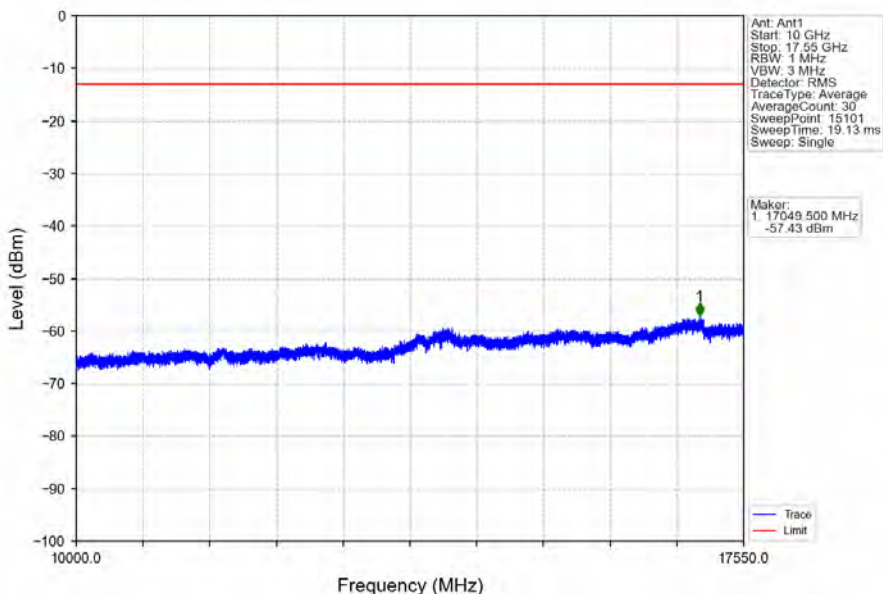
Band4_3MHz_64QAM_HCH_1753.5MHz_RB_1_0_NTNV
