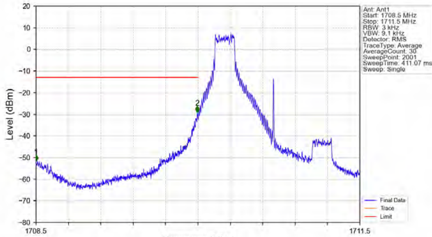
Band4_1.4MHz_64QAM_LCH_1710.7MHz_RB_1_0_NTNV
