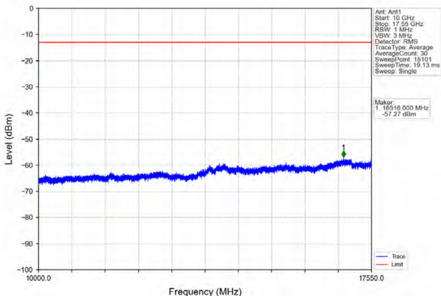
Band4_3MHz_64QAM_LCH_1711.5MHz_RB_15_0_NTNV
