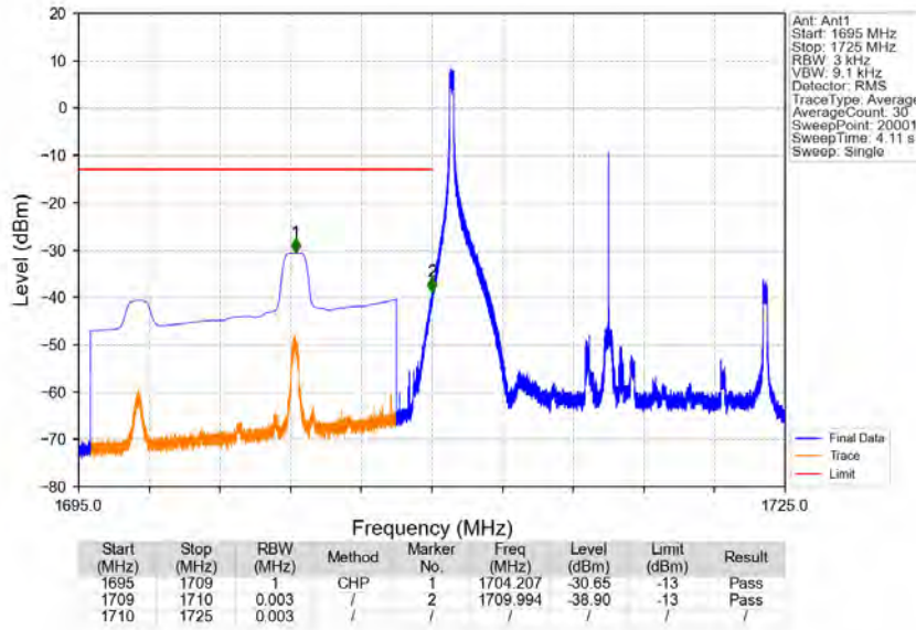
Band4_15MHz_16QAM_LCH_1717.5MHz_RB_1_0_NTNV
