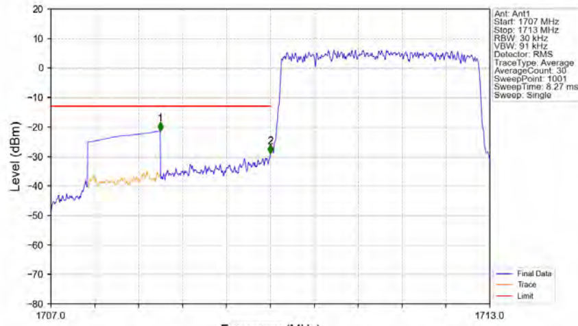
Band4_3MHz_QPSK_LCH_1711.5MHz_RB_15_0_NTNV
