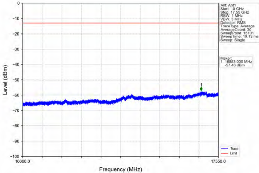
Band4_3MHz_QPSK_LCH_1711.5MHz_RB_15_0_NTNV
