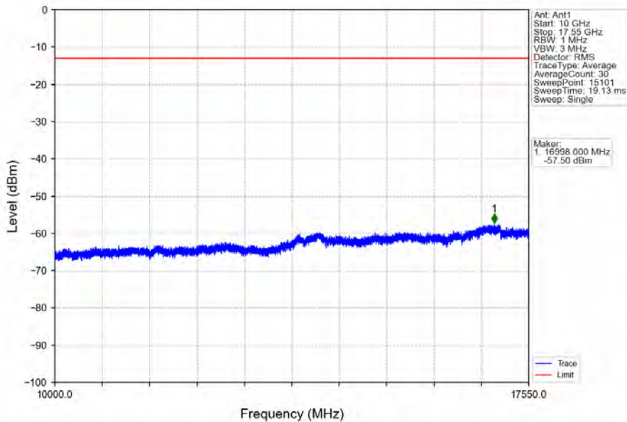
Band4_1.4MHz_QPSK_MCH_1732.5MHz_RB_1_0_NTV
