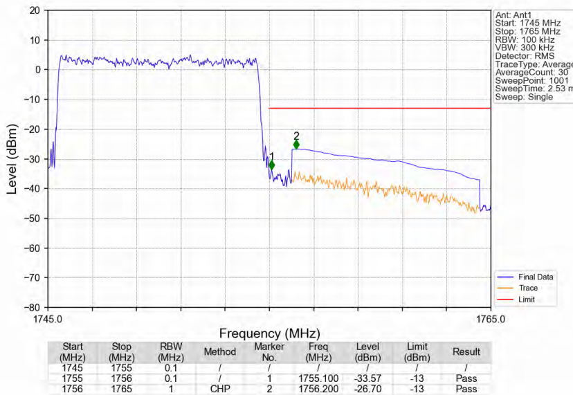
Band4_10MHz_16QAM_HCH_1750MHz_RB_50_0_NTNV
