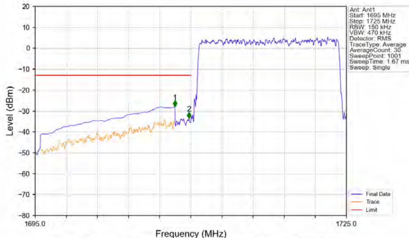
Band4_15MHz_16QAM_LCH_1717.5MHz_RB_75_0_NTNV
