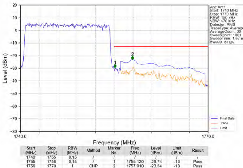
Band4_15MHz_QPSK_HCH_1747.5MHz_RB_75_0_NTNV
