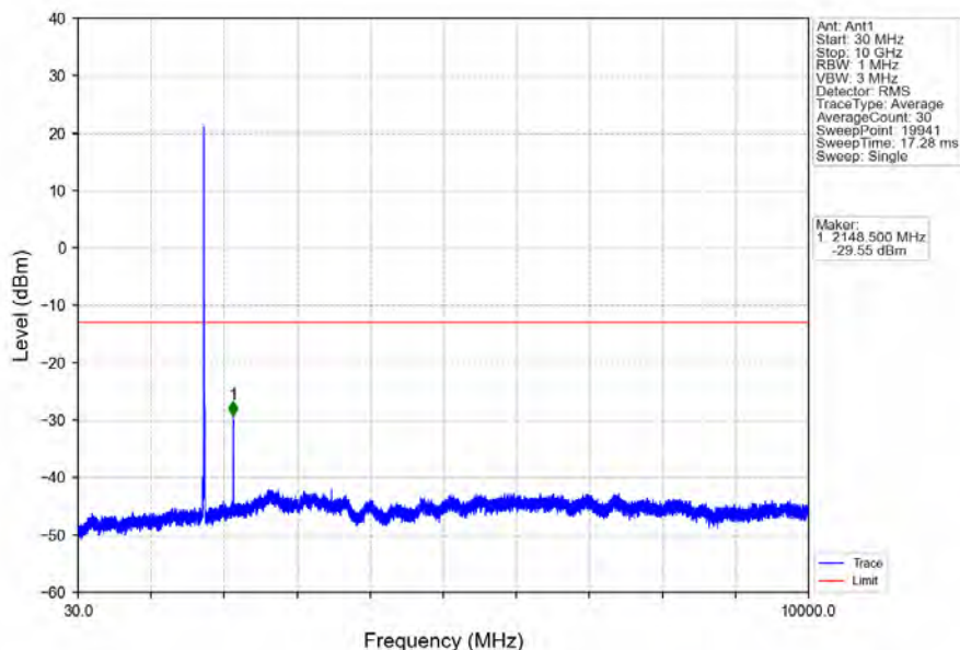
Band4_10MHz_64QAM_HCH_1750MHz_RB_1_0_NTNV
