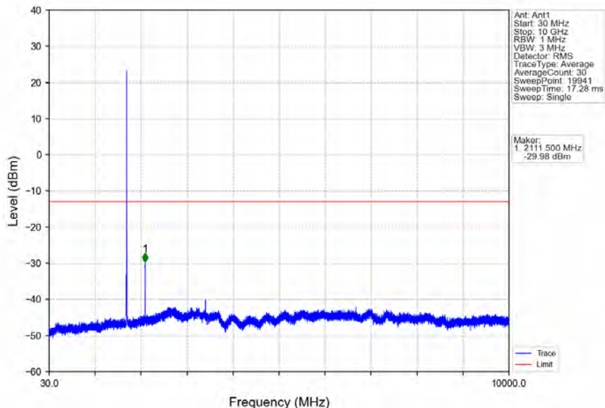
Band4_5MHz_QPSK_LCH_1712.5MHz_RB_1_0_NTNV
