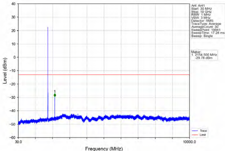
Band4_5MHz_16QAM_HCH_1752.5MHz_RB_1_0_NTNV
