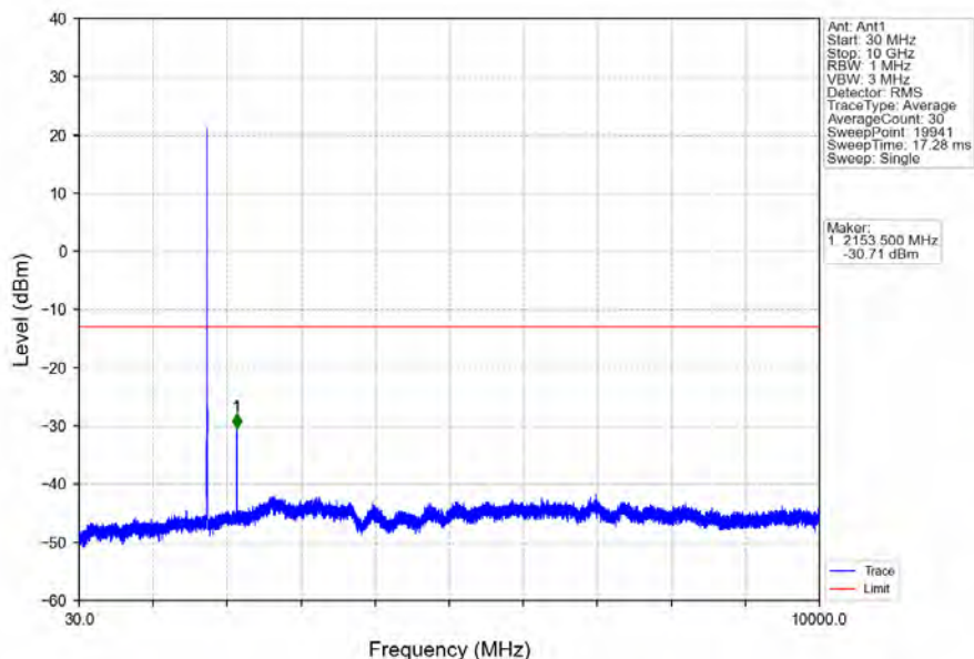
Band4_3MHz_64QAM_HCH_1753.5MHz_RB_1_0_NTNV
