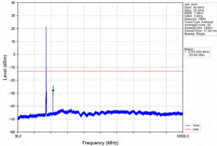
Band4_20MHz_16QAM_HCH_1745MHz_RB_1_0_NTNV
