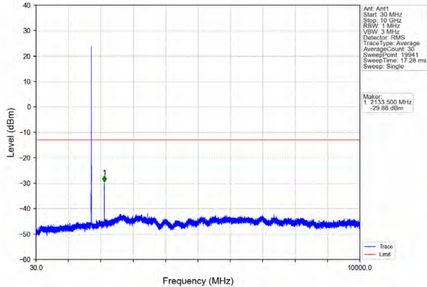
Band4_3MHz_QPSK_MCH_1732.5MHz_RB_1_0_NTNV
