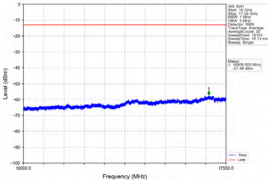
Band4_3MHz_16QAM_MCH_1732.5MHz_RB_1_0_NTNV
