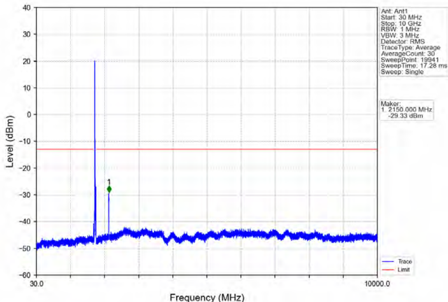
Band4_20MHz_64QAM_HCH_1745MHz_RB_1_0_NTNV
