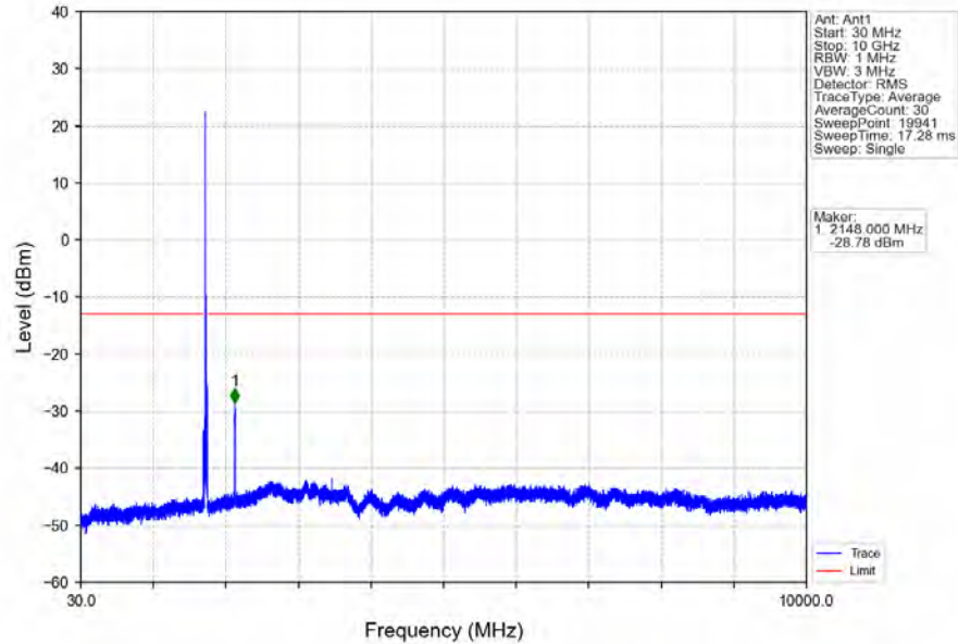
Band4_15MHz_16QAM_HCH_1747.5MHz_RB_1_0_NTNV
