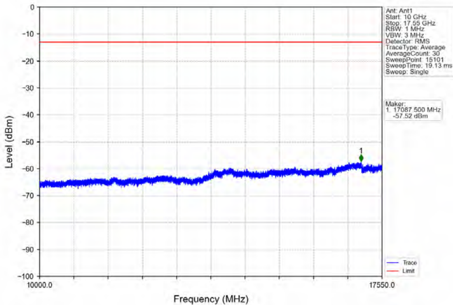
Band4_10MHz_64QAM_MCH_1732.5MHz_RB_1_0_NTNV
