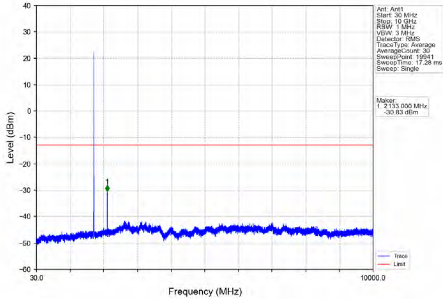
Band4_5MHz_64QAM_MCH_1732.5MHz_RB_1_0_NTNV
