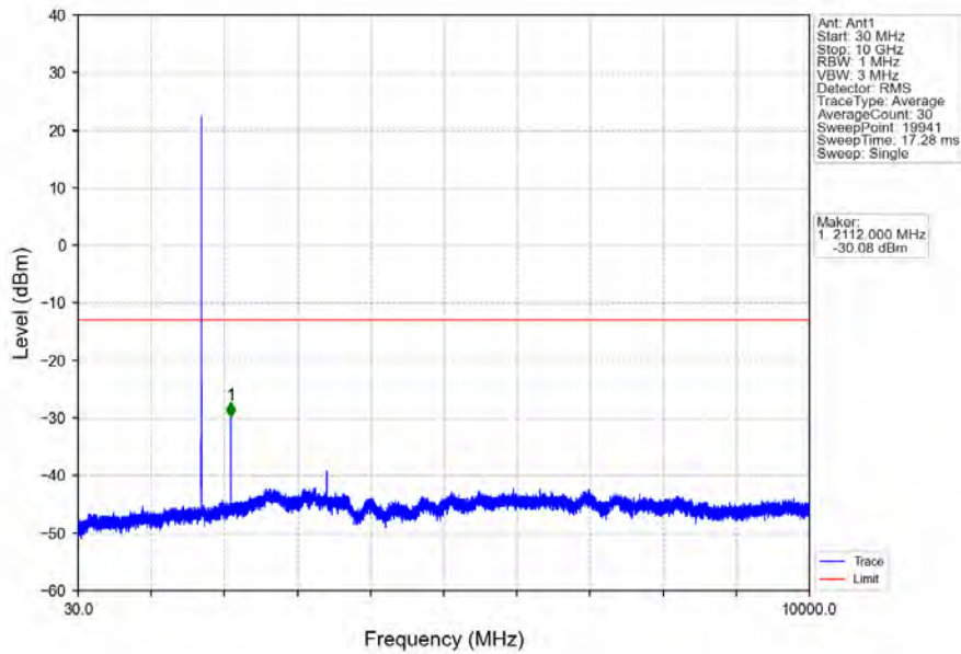
Band4_3MHz_16QAM_LCH_1711.5MHz_RB_1_0_NTNV
