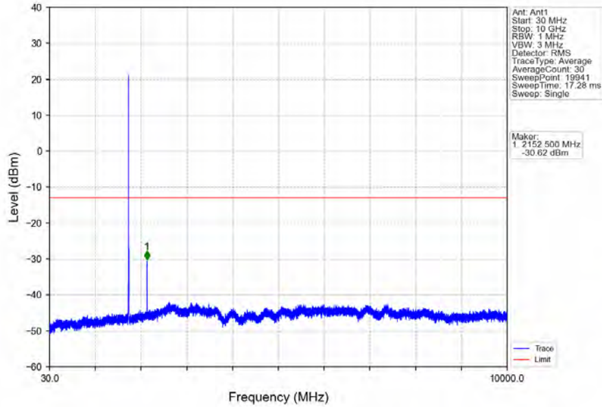
Band4_5MHz_64QAM_HCH_1752.5MHz_RB_1_0_NTNV
