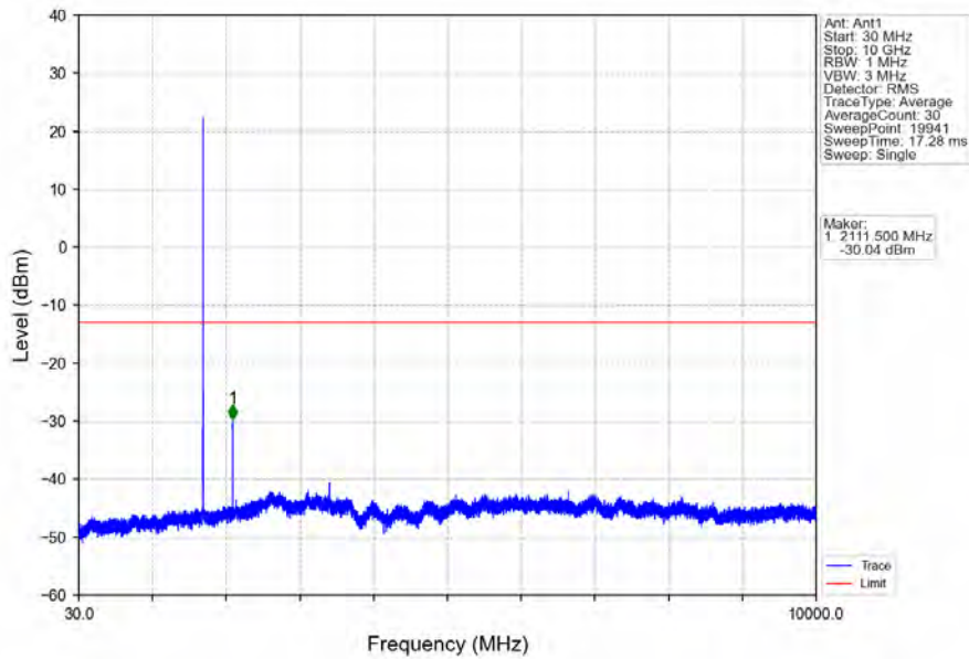
Band4_3MHz_64QAM_LCH_1711.5MHz_RB_1_0_NTNV
