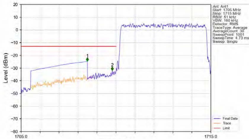
Band4_5MHz_16QAM_LCH_1712.5MHz_RB_25_0_NTNV
