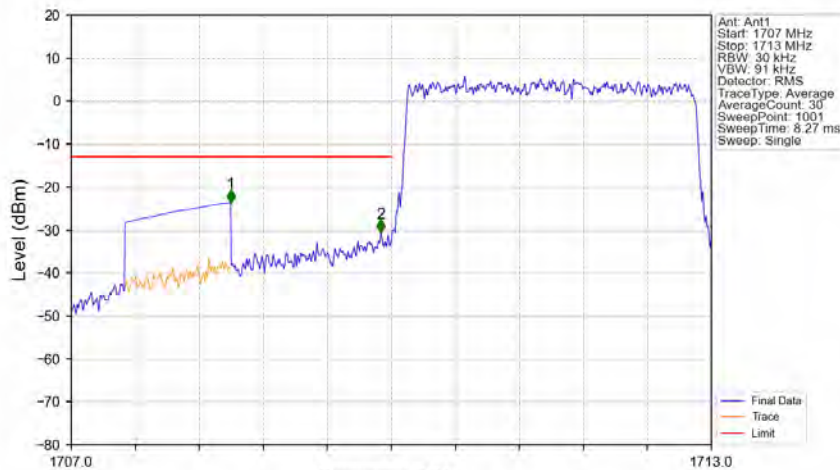
Band4_3MHz_16QAM_LCH_1711.5MHz_RB_15_0_NTNV
