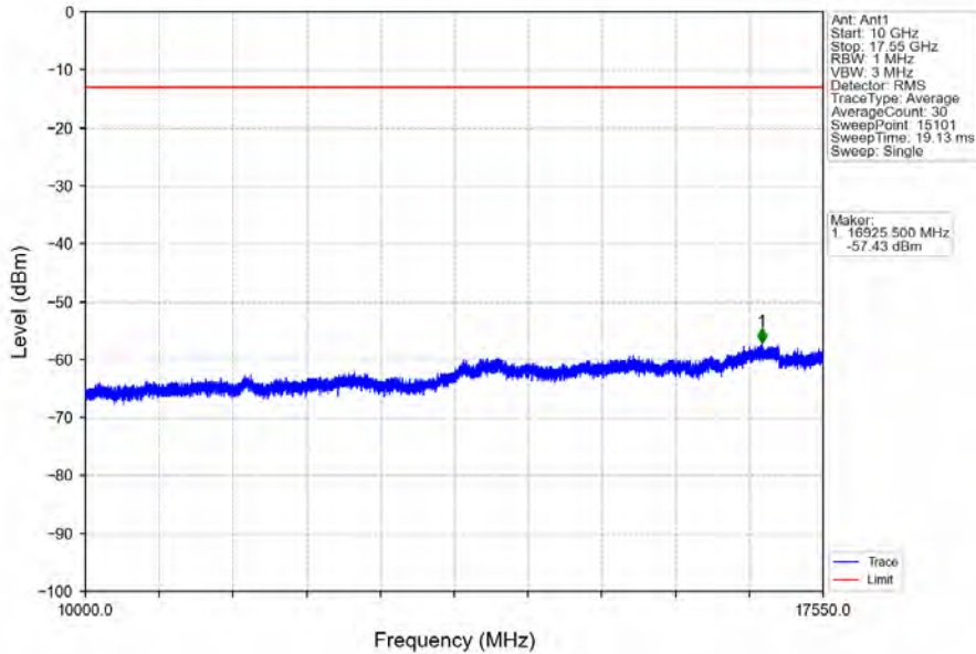
Band4_15MHz_16QAM_LCH_1717.5MHz_RB_75_0_NTNV
