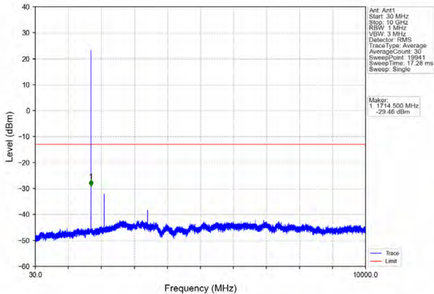
Band4_1.4MHz_16QAM_LCH_1710.7MHz_RB_1_0_NTNV
