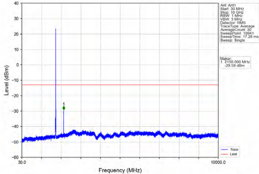
Band4_10MHz_16QAM_HCH_1750MHz_RB_1_0_NTNV
