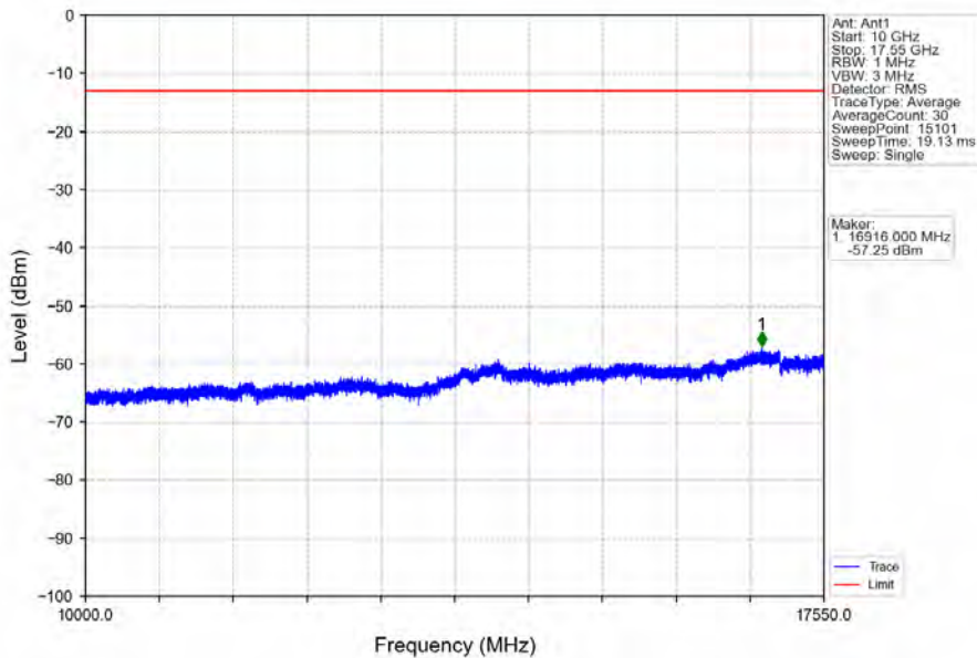
Band4_15MHz_64QAM_HCH_1747.5MHz_RB_1_0_NTNV
