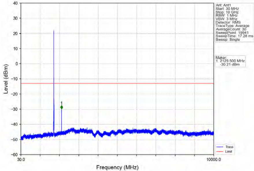
Band4_10MHz_16QAM_MCH_1732.5MHz_RB_1_0_NTNV
