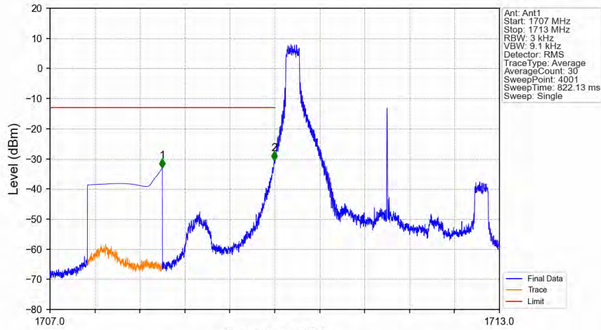
Band4_3MHz_16QAM_LCH_1711.5MHz_RB_1_0_NTNV
