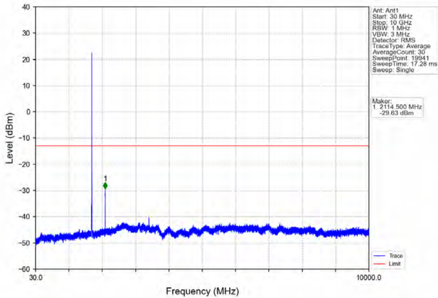
Band4_5MHz_16QAM_LCH_1712.5MHz_RB_1_0_NTNV
