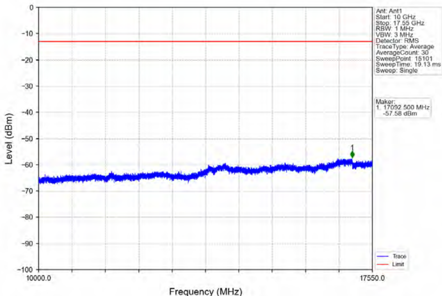
Band4_5MHz_64QAM_LCH_1712.5MHz_RB_25_0_NTNV
