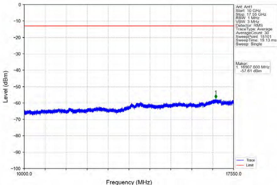
Band4_5MHz_QPSK_LCH_1712.5MHz_RB_25_0_NTNV
