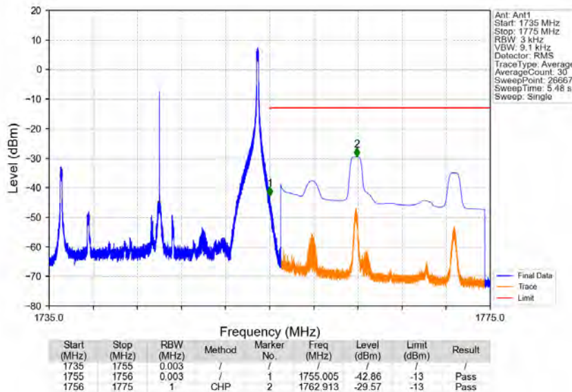
Band4_20MHz_16QAM_HCH_1745MHz_RB_1_99_NTNV
