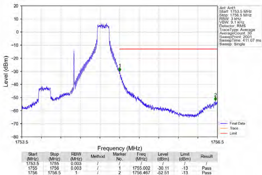
Band4_1.4MHz_64QAM_HCH_1754.3MHz_RB_1_5_NTNV
