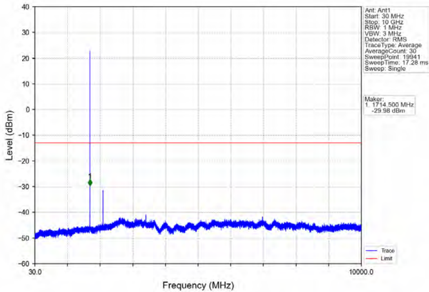
Band4_1.4MHz_64QAM_LCH_1710.7MHz_RB_1_0_NTNV
