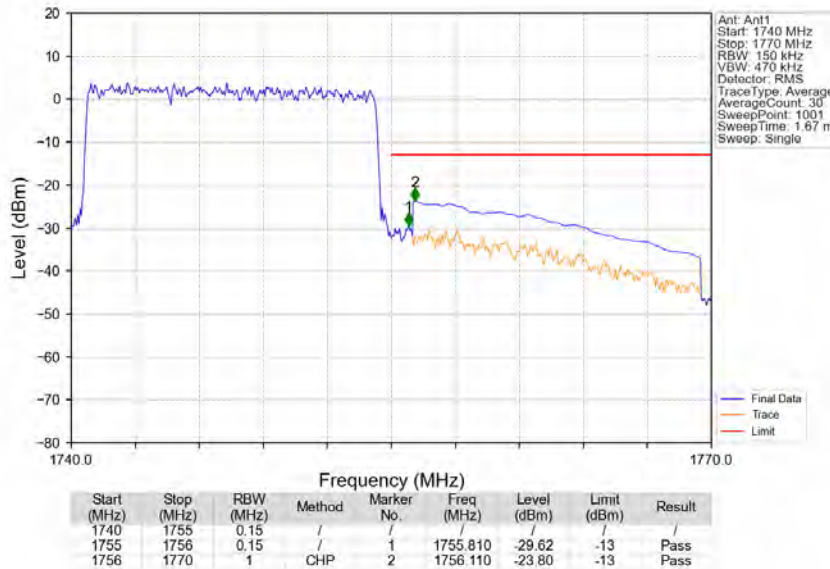
Band4_15MHz_64QAM_HCH_1747.5MHz_RB_75_0_NTNV
