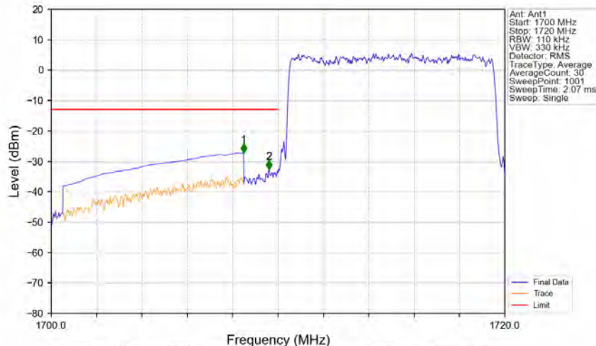
Band4_10MHz_16QAM_LCH_1715MHz_RB_50_0_NTNV
