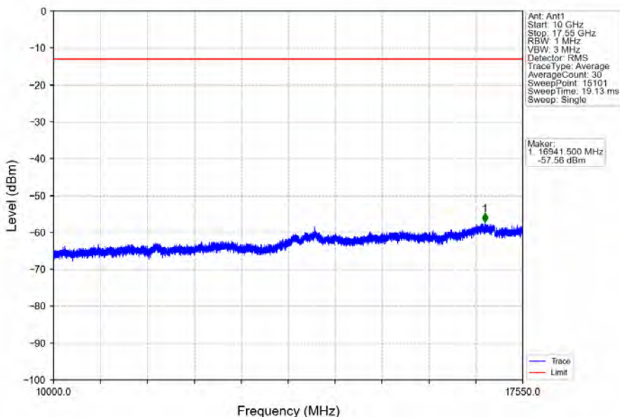
Band4_10MHz_64QAM_HCH_1750MHz_RB_1_0_NTNV
