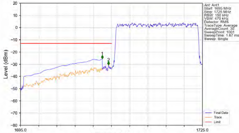
Band4_15MHz_64QAM_LCH_1717.5MHz_RB_75_0_NTNV
