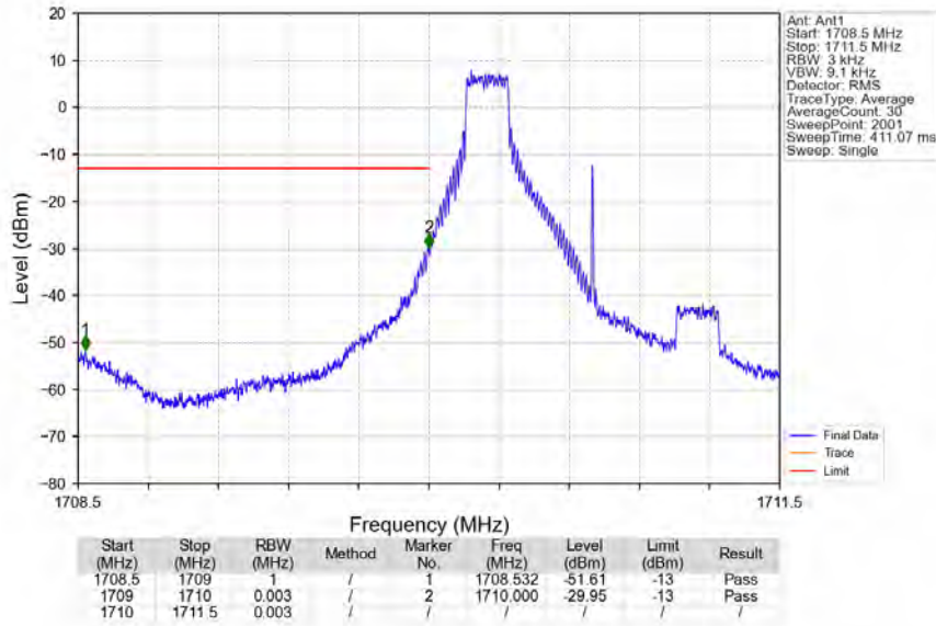
Band4_1.4MHz_16QAM_LCH_1710.7MHz_RB_1_0_NTNV
