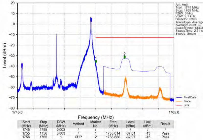
Band4_10MHz_64QAM_HCH_1750MHz_RB_1_49_NTNV
