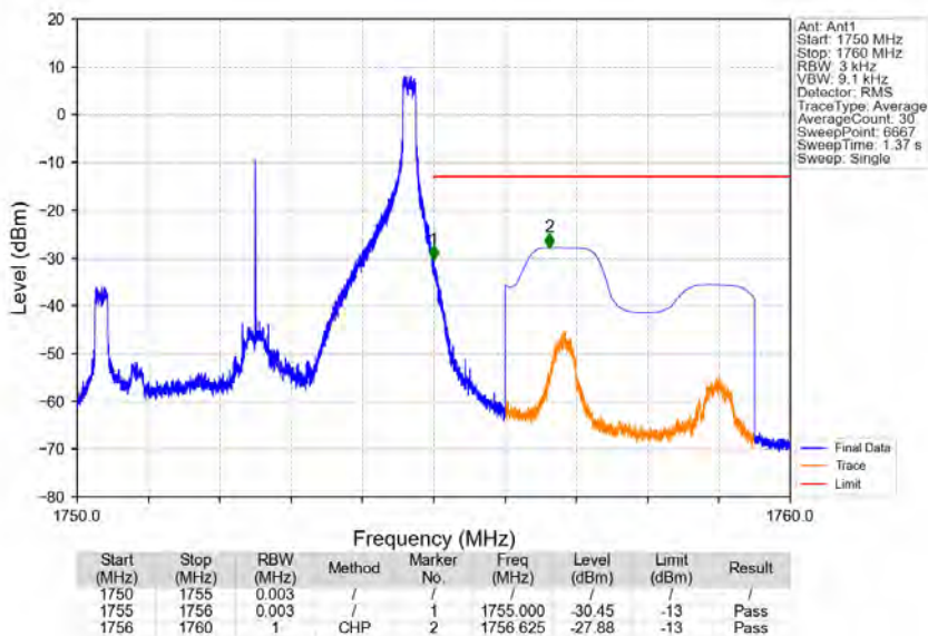
Band4_5MHz_QPSK_HCH_1752.5MHz_RB_1_24_NTNV
