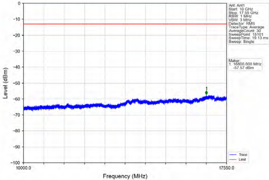
Band4_10MHz_16QAM_LCH_1715MHz_RB_50_0_NTNV
