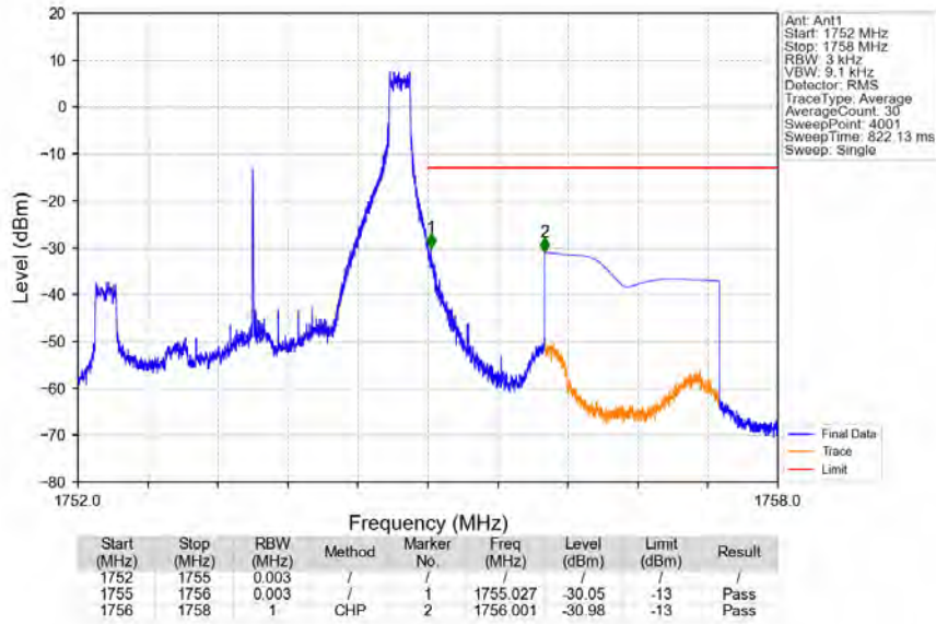
Band4_3MHz_16QAM_HCH_1753.5MHz_RB_1_14_NTNV
