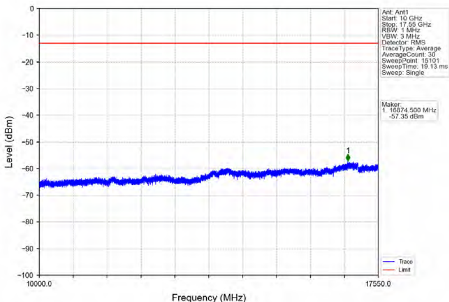
Band4_15MHz_QPSK_LCH_1717.5MHz_RB_75_0_NTNV
