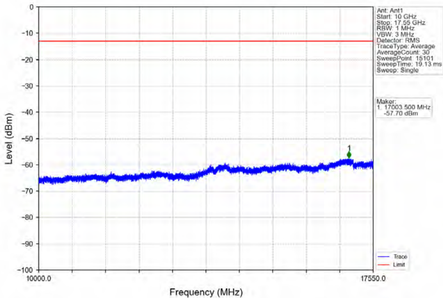
Band4_10MHz_16QAM_MCH_1732.5MHz_RB_1_0_NTNV
