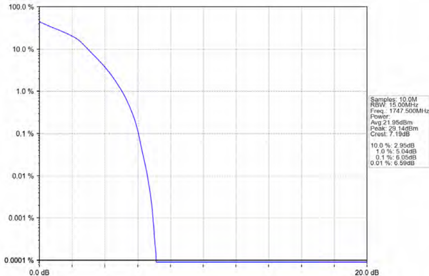
Band4_15MHz_16QAM_HCH_1747.5MHz_RB_75_0_NTNV
