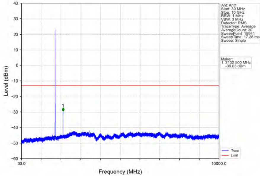
Band4_5MHz_16QAM_MCH_1732.5MHz_RB_1_0_NTNV
