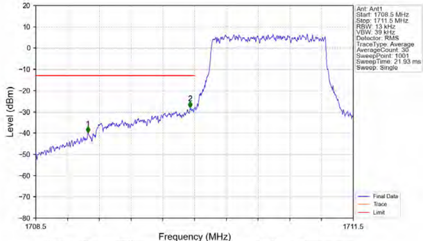
Band4_1.4MHz_QPSK_LCH_1710.7MHz_RB_6_0_NTNV
