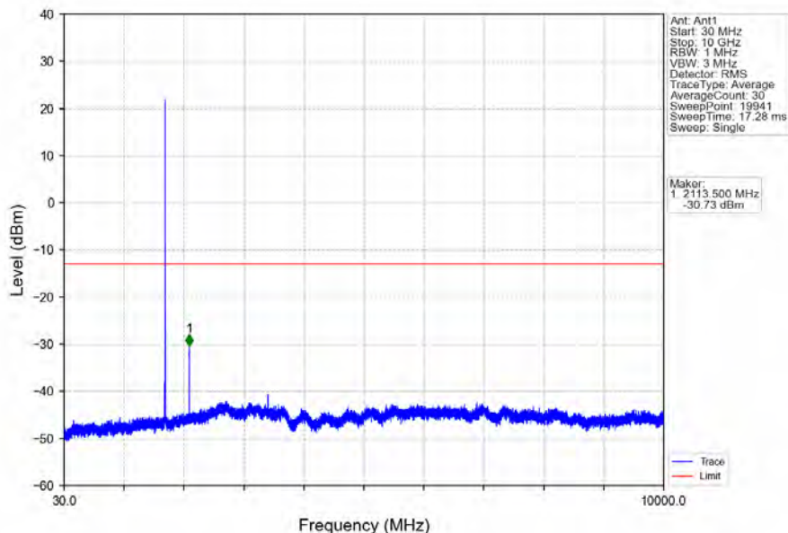
Band4_5MHz_64QAM_LCH_1712.5MHz_RB_1_0_NTNV
