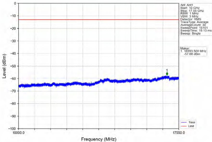
Band4_20MHz_16QAM_HCH_1745MHz_RB_1_0_NTNV
