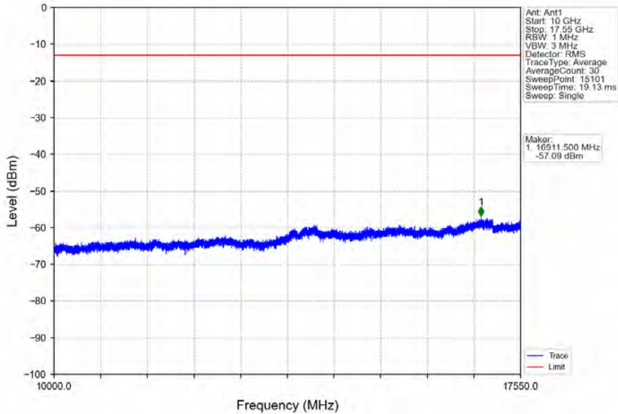
Band4_1.4MHz_QPSK_LCH_1710.7MHz_RB_6_0_NTNV
