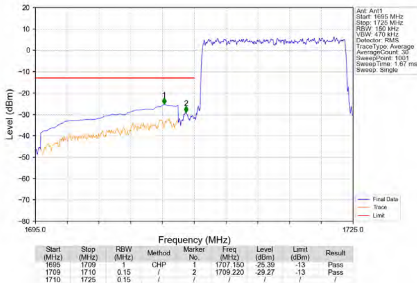
Band4_15MHz_QPSK_LCH_1717.5MHz_RB_75_0_NTNV
