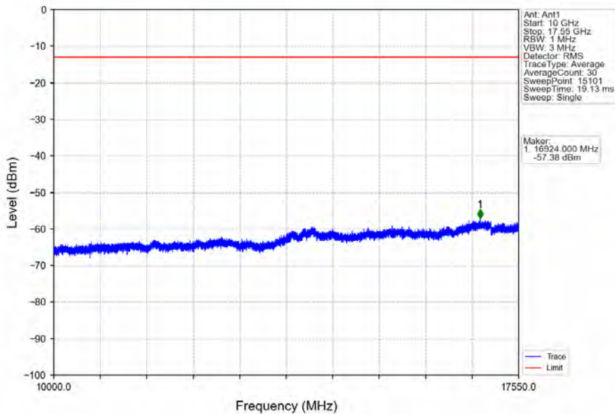
Band4_15MHz_QPSK_MCH_1732.5MHz_RB_1_0_NTNV
