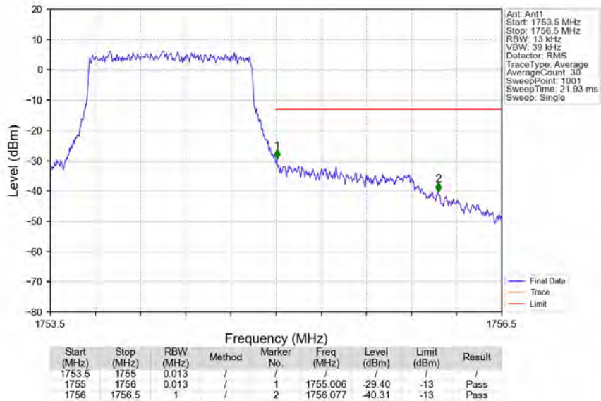
Band4_1.4MHz_QPSK_HCH_1754.3MHz_RB_6_0_NTNV
