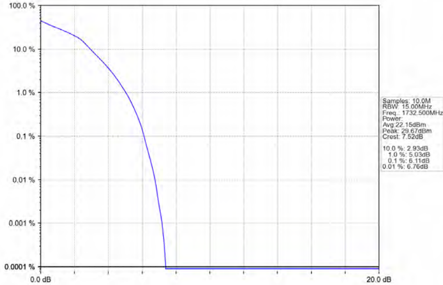
Band4_15MHz_16QAM_MCH_1732.5MHz_RB_75_0_NTNV
