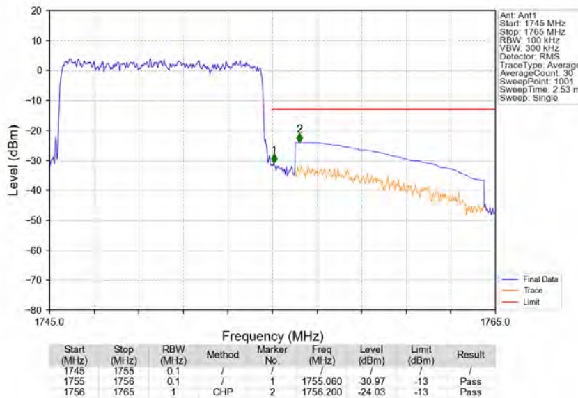
Band4_10MHz_64QAM_HCH_1750MHz_RB_50_0_NTNV
