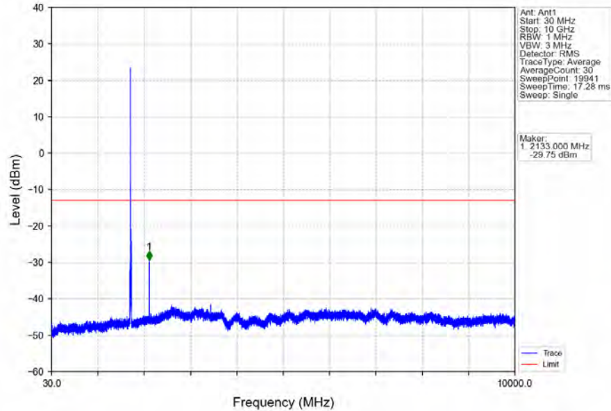
Band4_10MHz_QPSK_MCH_1732.5MHz_RB_1_0_NTNV
