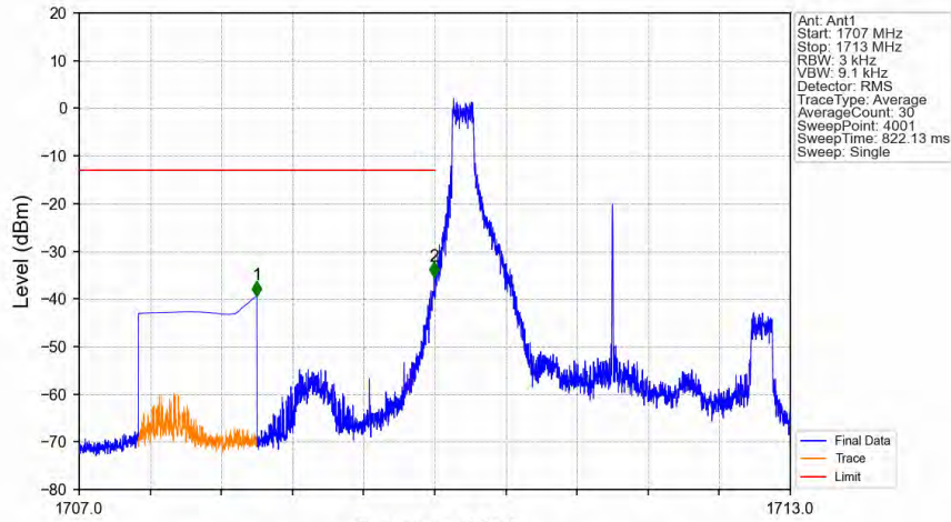
Band4_3MHz_64QAM_LCH_1711.5MHz_RB_1_0_NTNV
