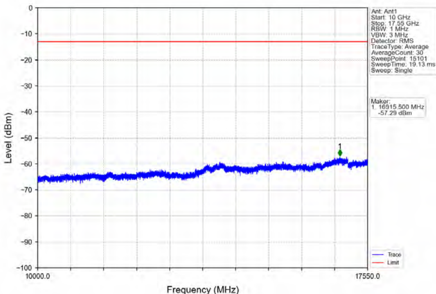
Band4_3MHz_16QAM_HCH_1753.5MHz_RB_1_0_NTNV
