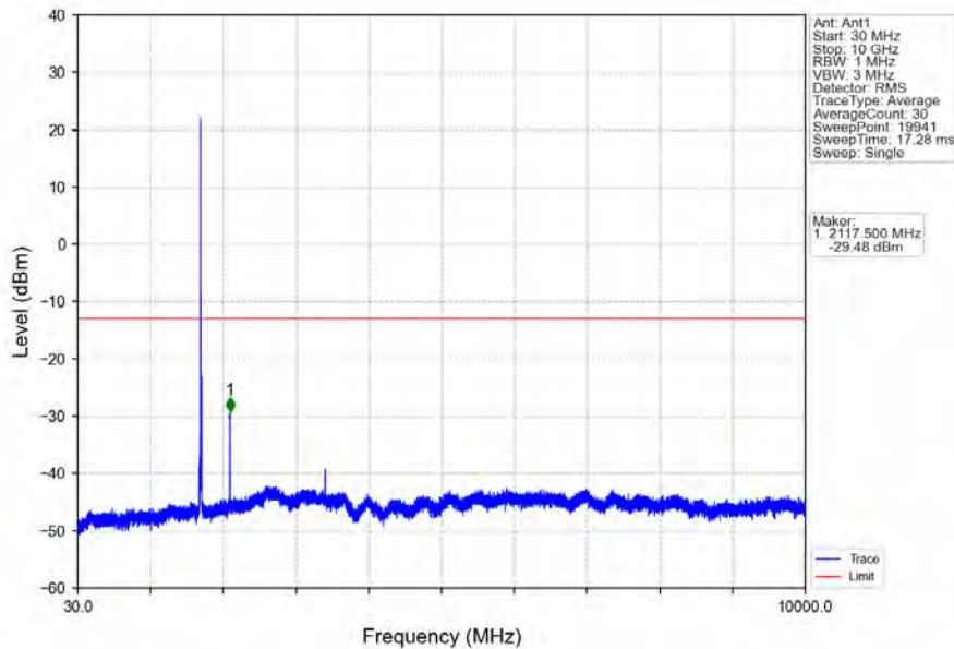
Band4_10MHz_16QAM_LCH_1715MHz_RB_1_0_NTNV
