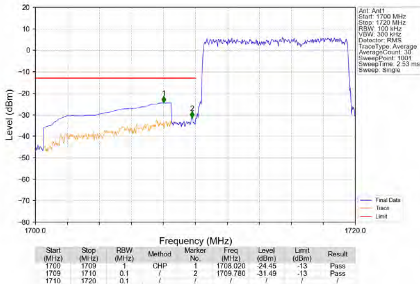
Band4_10MHz_QPSK_LCH_1715MHz_RB_50_0_NTNV
