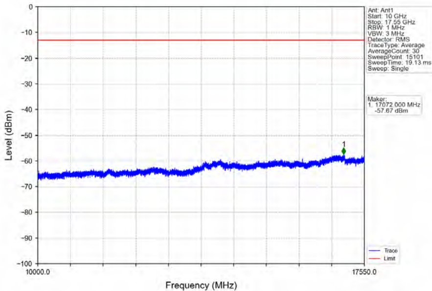
Band4_5MHz_16QAM_MCH_1732.5MHz_RB_1_0_NTNV
