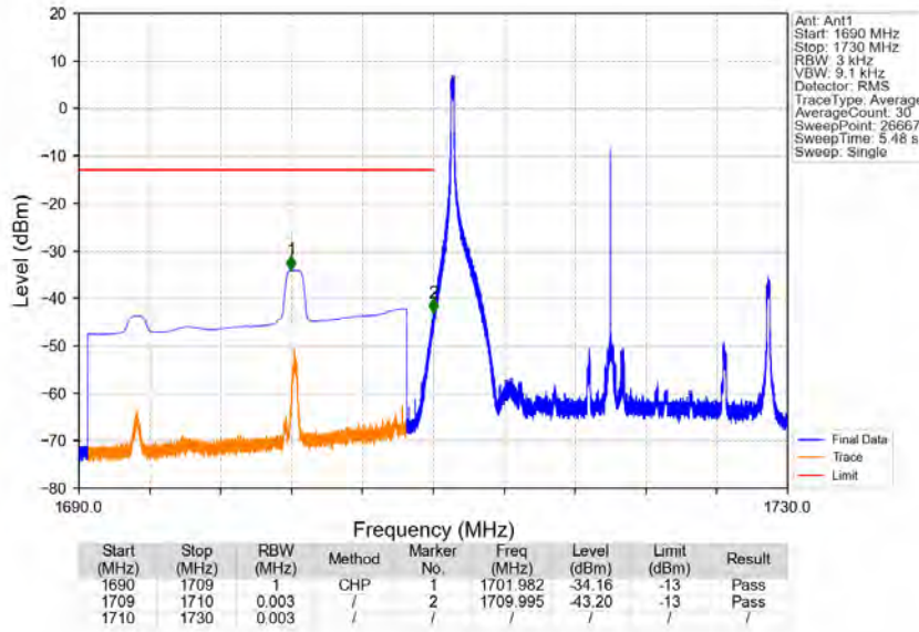
Band4_20MHz_64QAM_LCH_1720MHz_RB_1_0_NTNV
