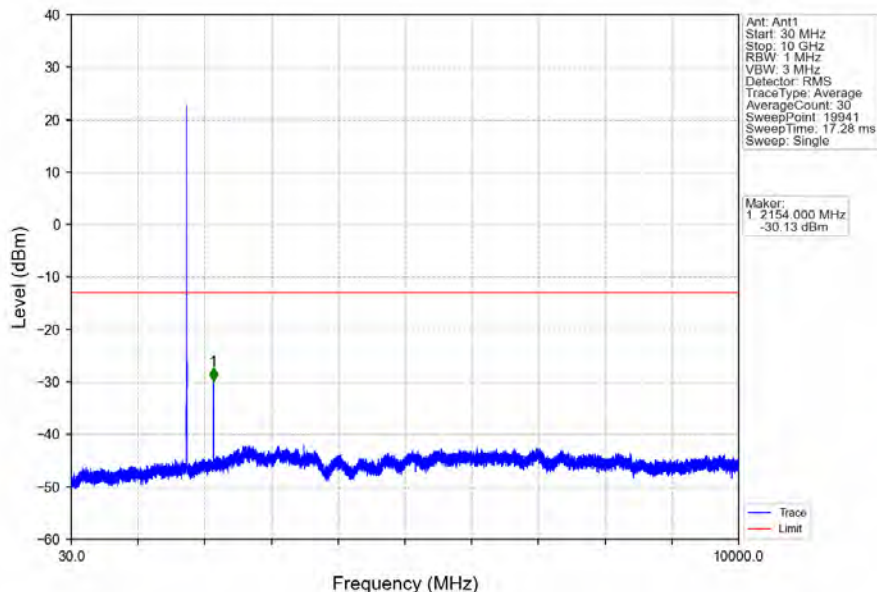
Band4_3MHz_16QAM_HCH_1753.5MHz_RB_1_0_NTNV
