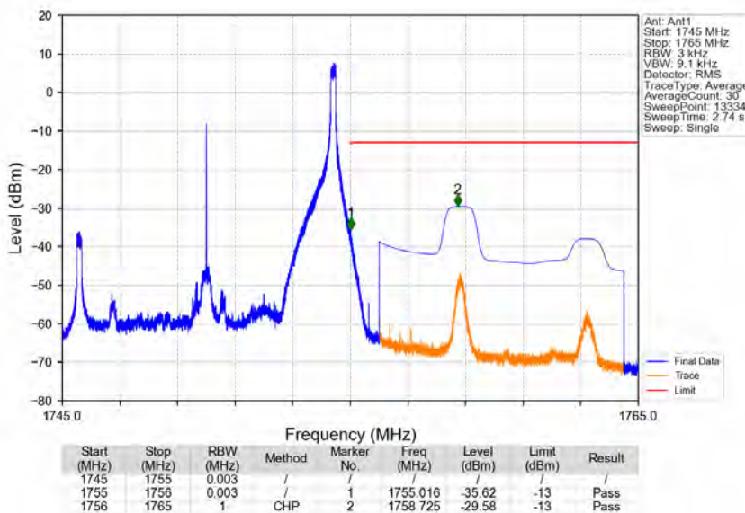
Band4_10MHz_16QAM_HCH_1750MHz_RB_1_49_NTNV
