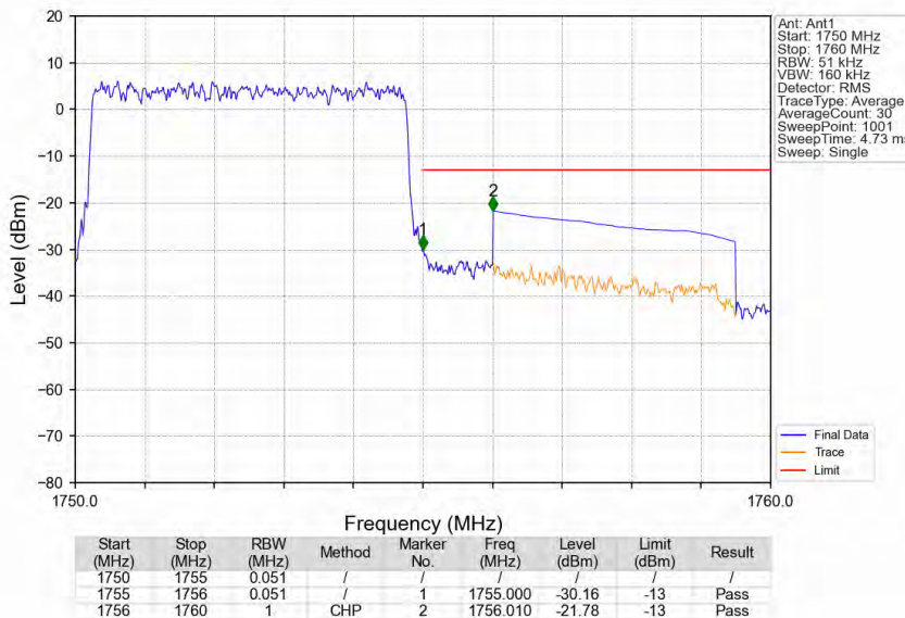
Band4_5MHz_QPSK_HCH_1752.5MHz_RB_25_0_NTNV
