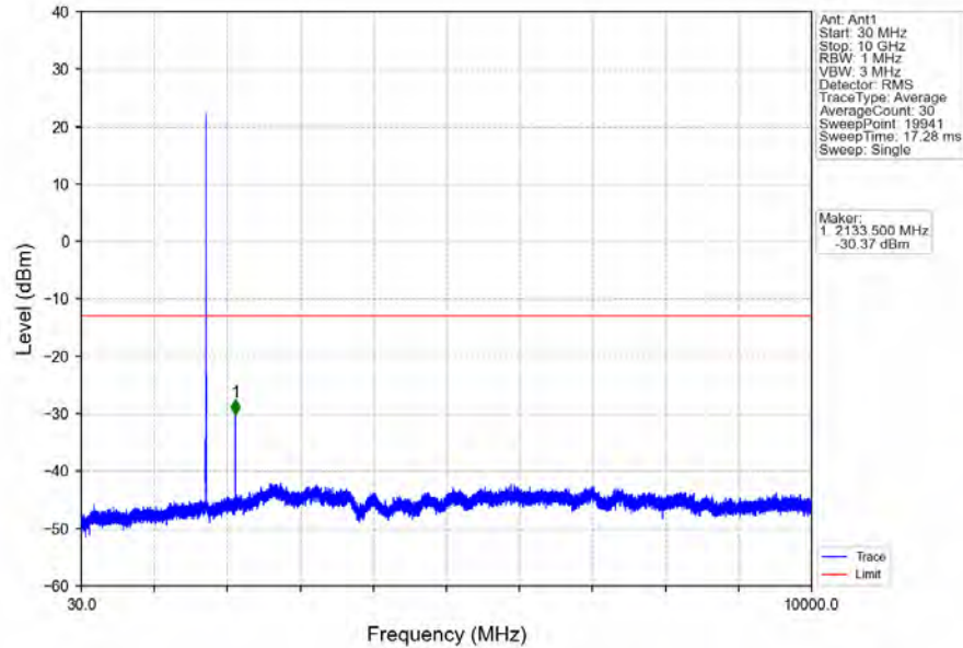
Band4_3MHz_16QAM_MCH_1732.5MHz_RB_1_0_NTNV
