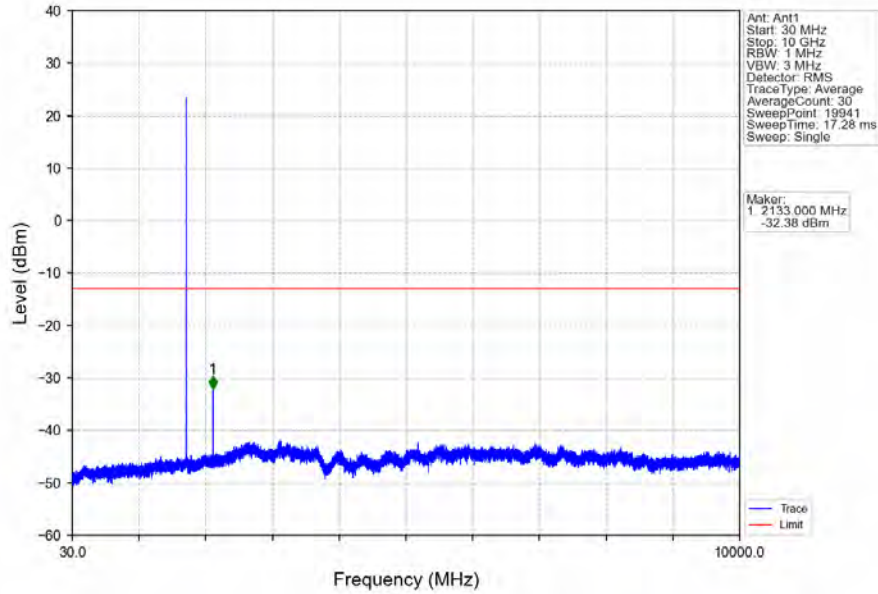
Band4_1.4MHz_QPSK_MCH_1732.5MHz_RB_1_0_NTV
