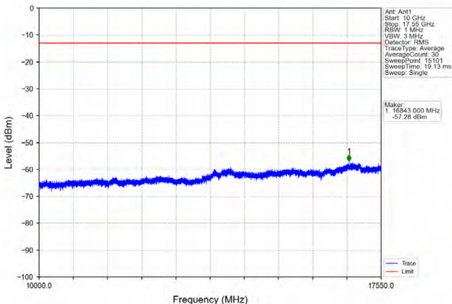
Band4_20MHz_64QAM_HCH_1745MHz_RB_1_0_NTNV
