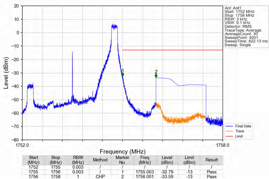
Band4_3MHz_64QAM_HCH_1753.5MHz_RB_1_14_NTNV
