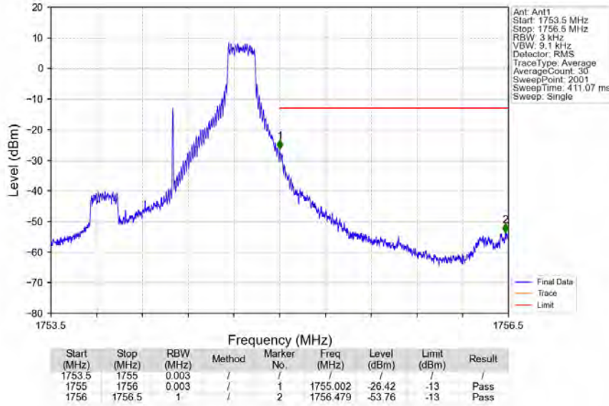
Band4_1.4MHz_QPSK_HCH_1754.3MHz_RB_1_5_NTNV
