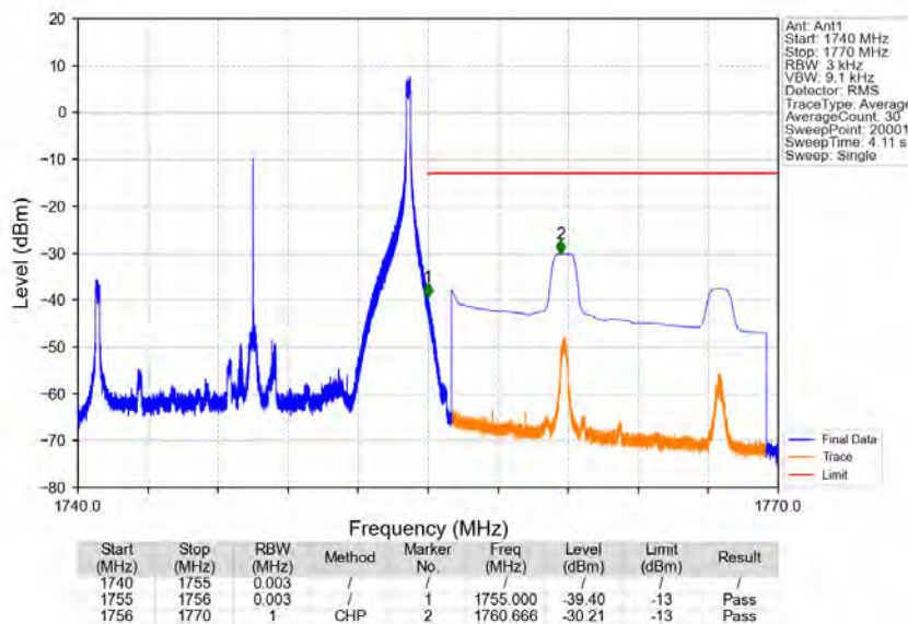
Band4_15MHz_16QAM_HCH_1747.5MHz_RB_1_74_NTNV
