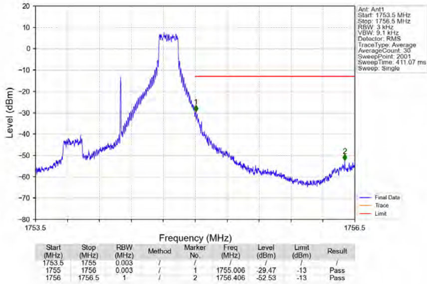
Band4_1.4MHz_16QAM_HCH_1754.3MHz_RB_1_5_NTNV
