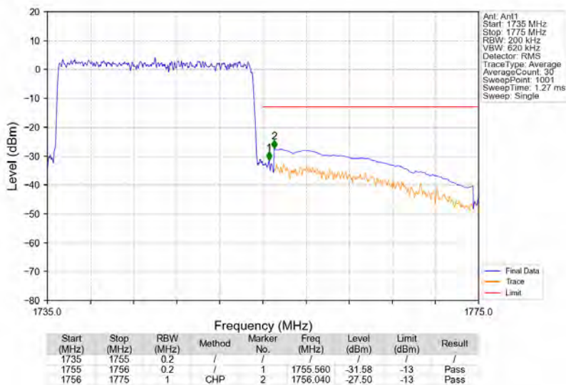
Band4_20MHz_64QAM_HCH_1745MHz_RB_100_0_NTNV
