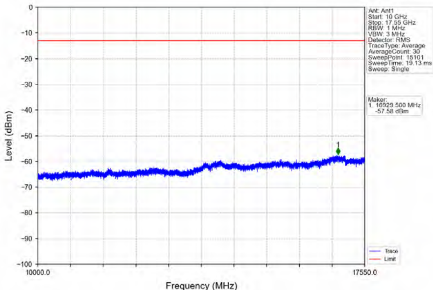
Band4_3MHz_16QAM_LCH_1711.5MHz_RB_15_0_NTNV
