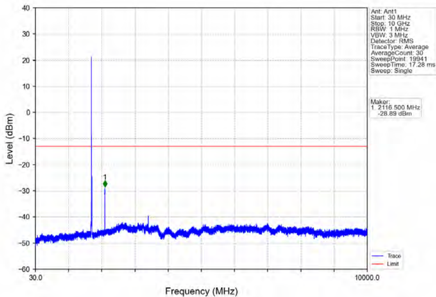
Band4_10MHz_64QAM_LCH_1715MHz_RB_1_0_NTNV
