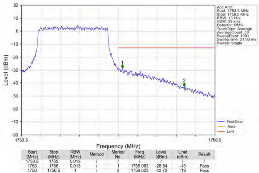
Band4_1.4MHz_64QAM_HCH_1754.3MHz_RB_6_0_NTNV
