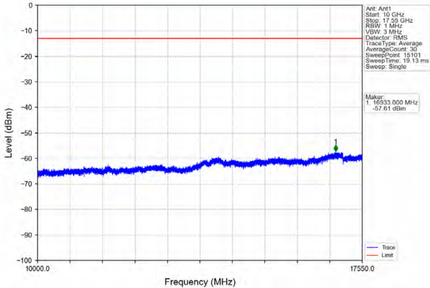
Band4_10MHz_64QAM_LCH_1715MHz_RB_50_0_NTNV
