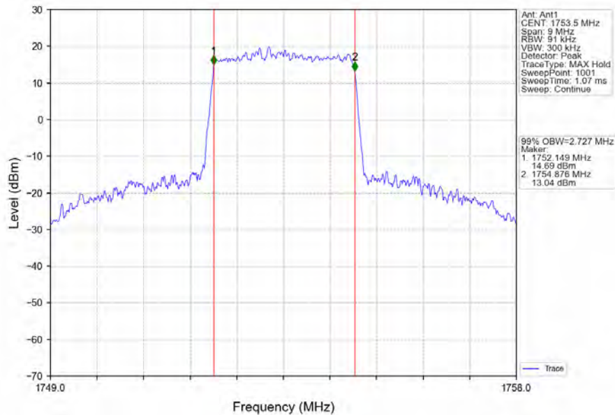
Band4_3MHz_QPSK_HCH_1753.5MHz_RB_15_0_NTNV
