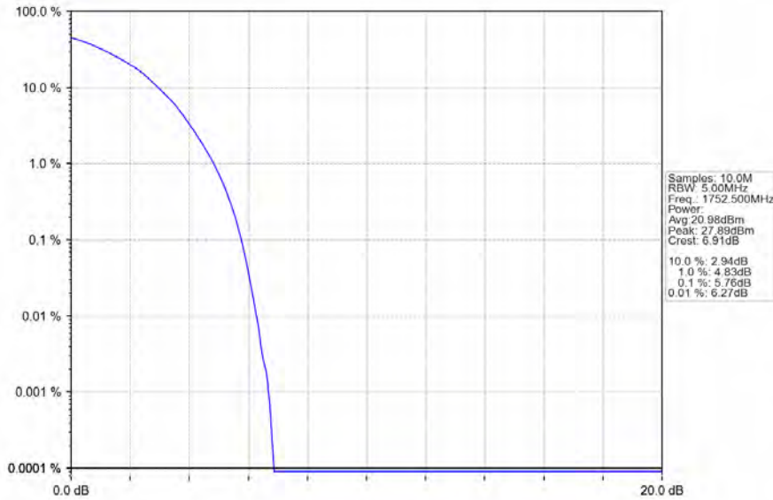
Band4_5MHz_64QAM_HCH_1752.5MHz_RB_25_0_NTNV
