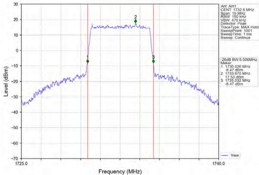
Band4_5MHz_64QAM_MCH_1732.5MHz_RB_25_0_NTNV
