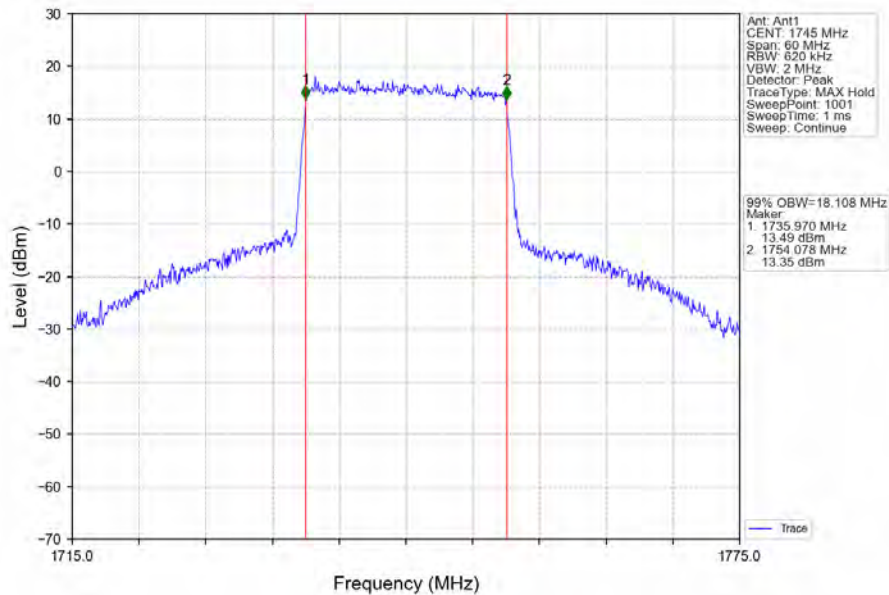
Band4_20MHz_64QAM_HCH_1745MHz_RB_100_0_NTNV
