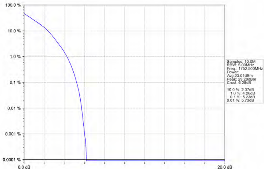
Band4_5MHz_QPSK_HCH_1752.5MHz_RB_25_0_NTNV
