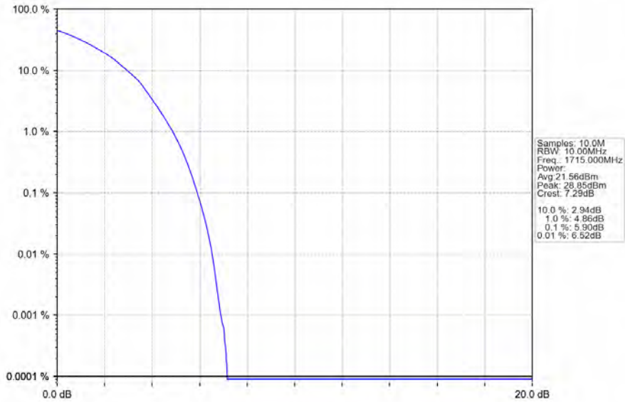
Band4_10MHz_64QAM_LCH_1715MHz_RB_50_0_NTNV
