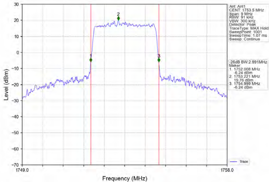
Band4_3MHz_QPSK_HCH_1753.5MHz_RB_15_0_NTNV
