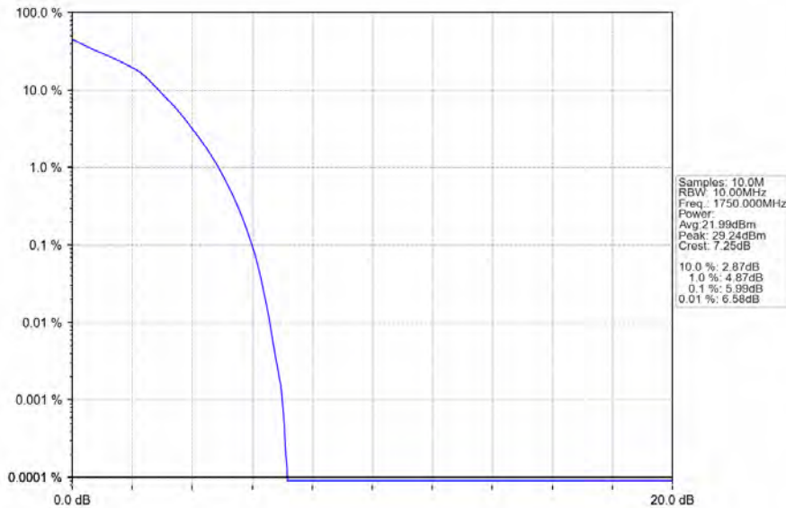
Band4_10MHz_16QAM_HCH_1750MHz_RB_50_0_NTNV
