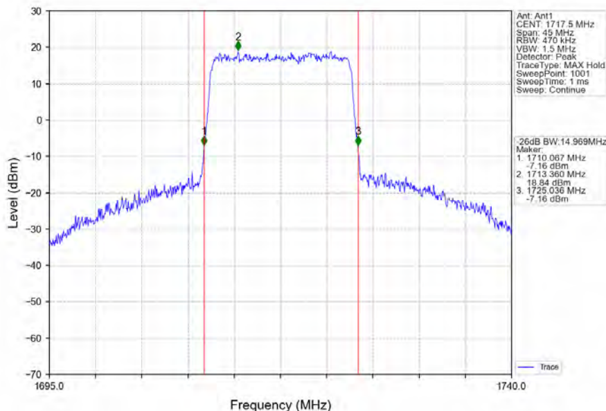
Band4_15MHz_16QAM_LCH_1717.5MHz_RB_75_0_NTNV
