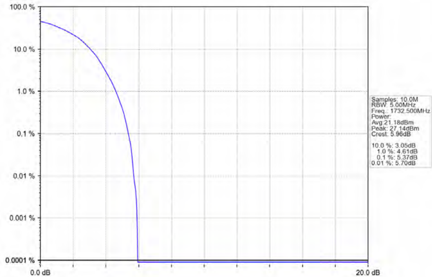
Band4_1.4MHz_64QAM_MCH_1732.5MHz_RB_6_0_NTNV
