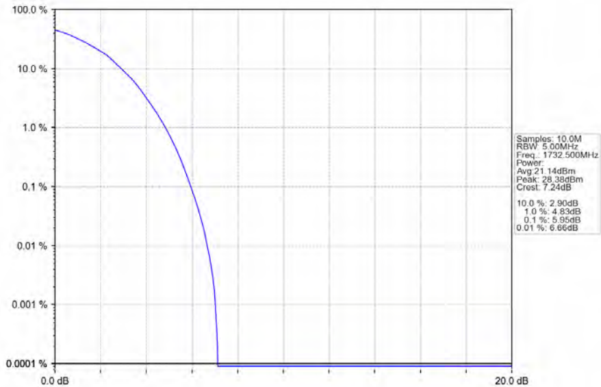
Band4_5MHz_64QAM_MCH_1732.5MHz_RB_25_0_NTNV
