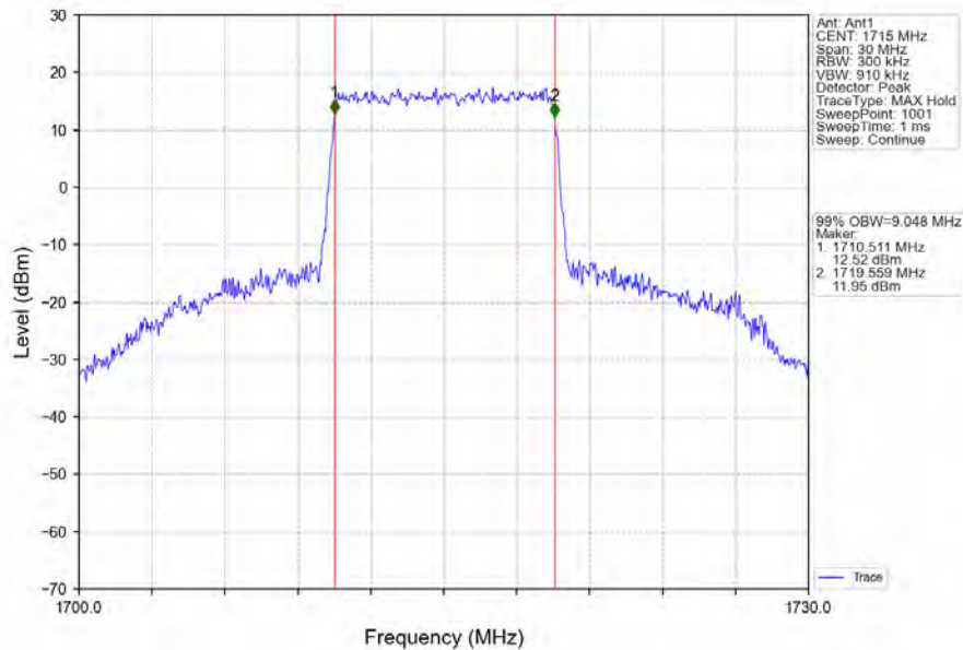
Band4_10MHz_64QAM_LCH_1715MHz_RB_50_0_NTNV
