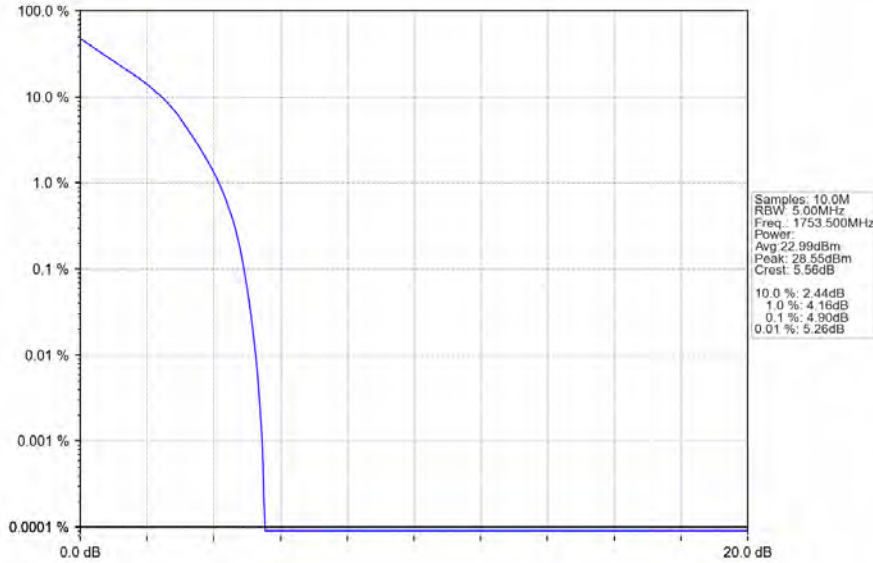
Band4_3MHz_QPSK_HCH_1753.5MHz_RB_15_0_NTNV
