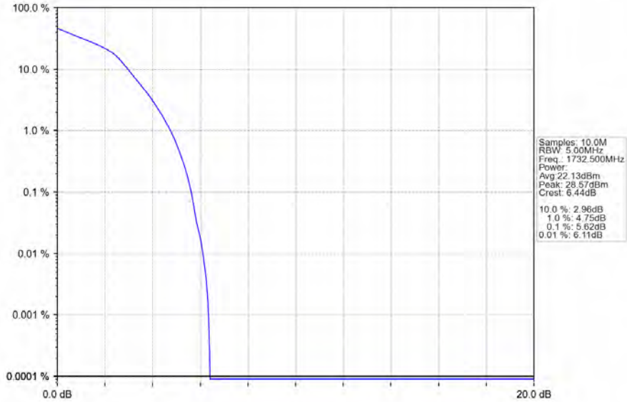
Band4_1.4MHz_16QAM_MCH_1732.5MHz_RB_6_0_NTNV
