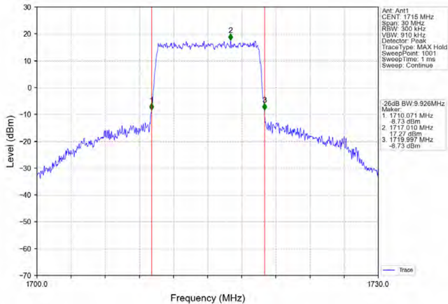
Band4_10MHz_64QAM_LCH_1715MHz_RB_50_0_NTNV
