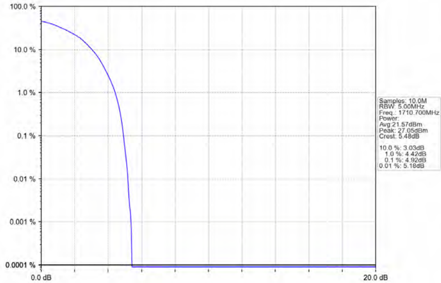
Band4_1.4MHz_64QAM_LCH_1710.7MHz_RB_6_0_NTNV
