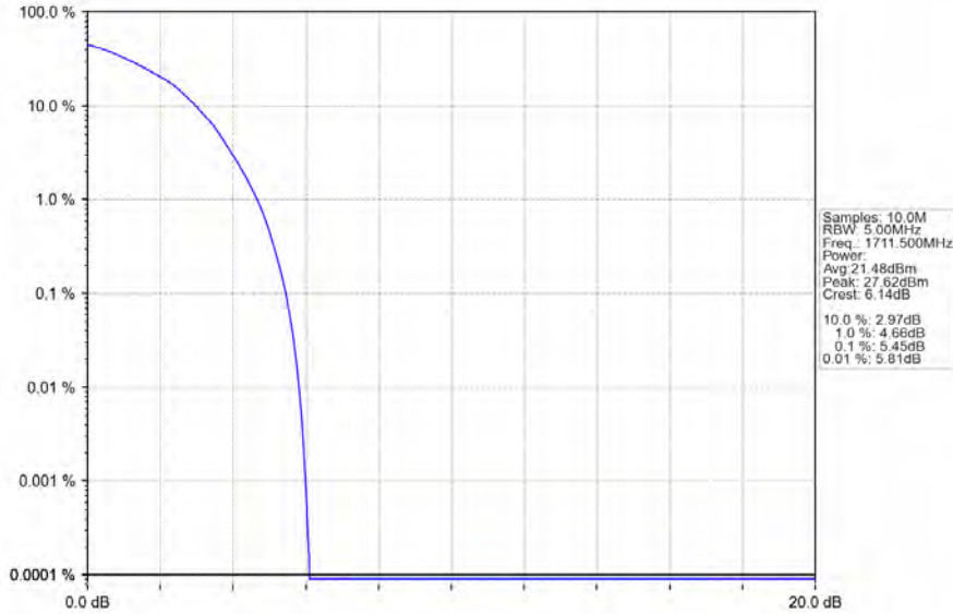
Band4_3MHz_64QAM_LCH_1711.5MHz_RB_15_0_NTNV
