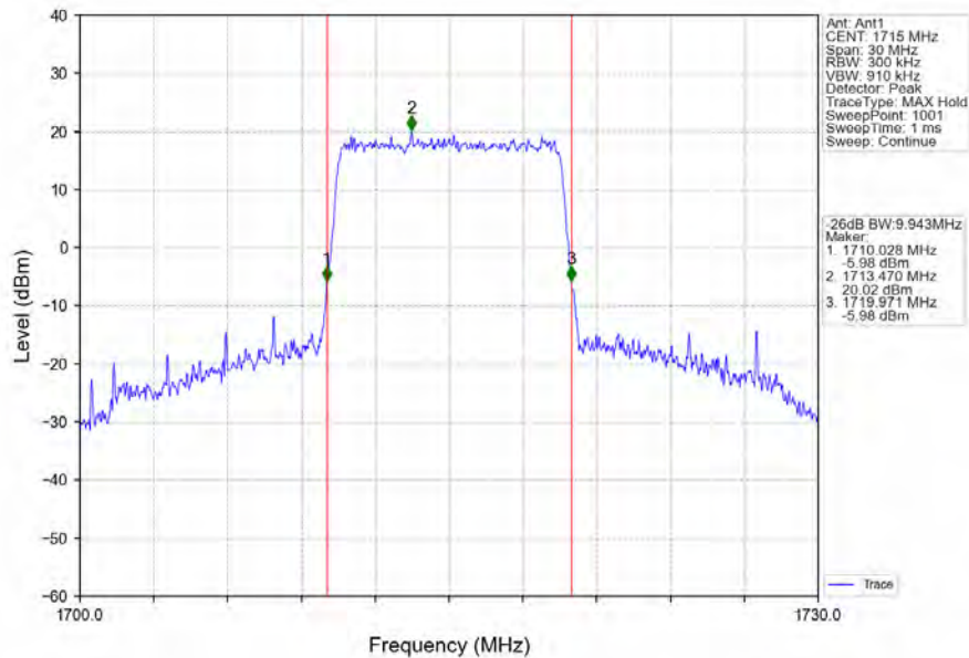
Band4_10MHz_QPSK_LCH_1715MHz_RB_50_0_NTNV
