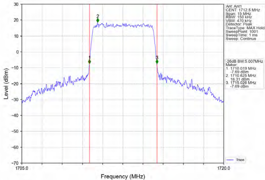
Band4_5MHz_16QAM_LCH_1712.5MHz_RB_25_0_NTNV
