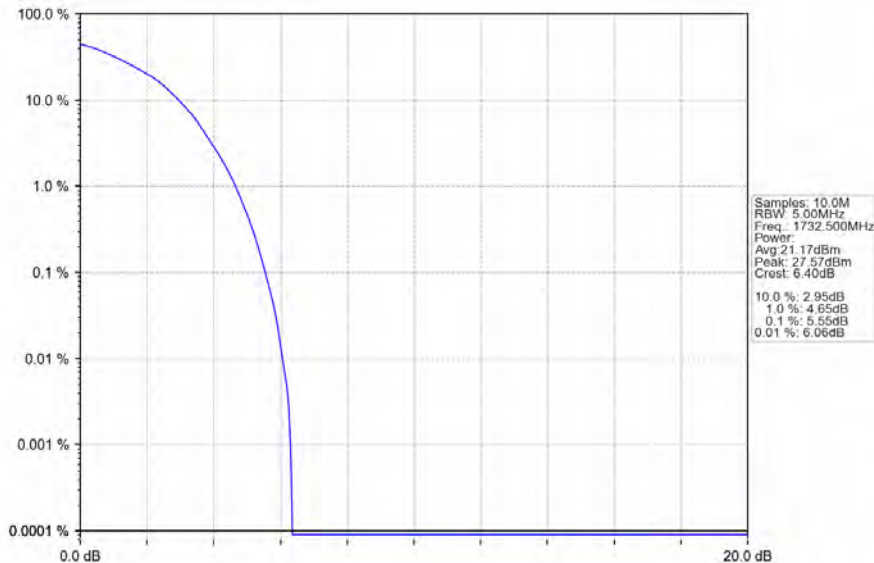
Band4_3MHz_64QAM_MCH_1732.5MHz_RB_15_0_NTNV
