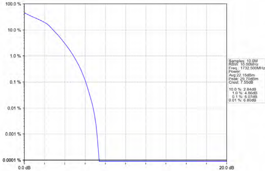
Band4_10MHz_16QAM_MCH_1732.5MHz_RB_50_0_NTNV
