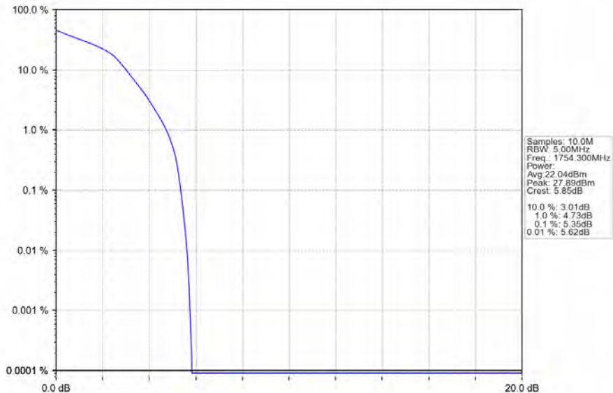
Band4_1.4MHz_16QAM_HCH_1754.3MHz_RB_6_0_NTNV
