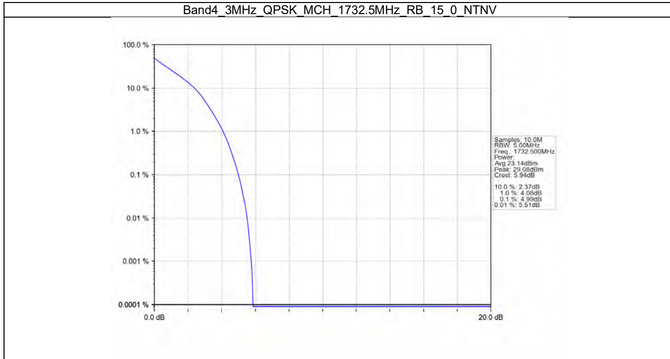
Band4_3MHz_QPSK_MCH_1732.5MHz_RB_15_0_NTNV
