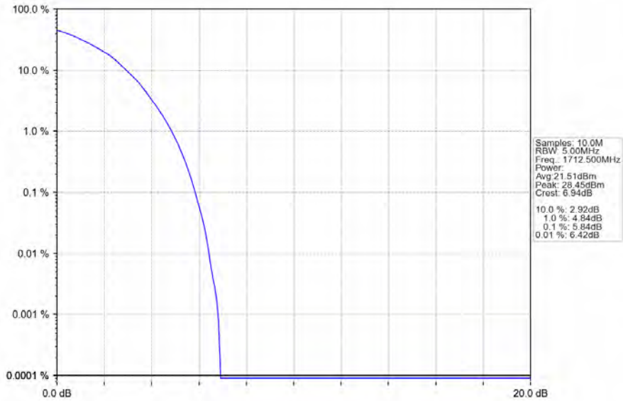
Band4_5MHz_64QAM_LCH_1712.5MHz_RB_25_0_NTNV
