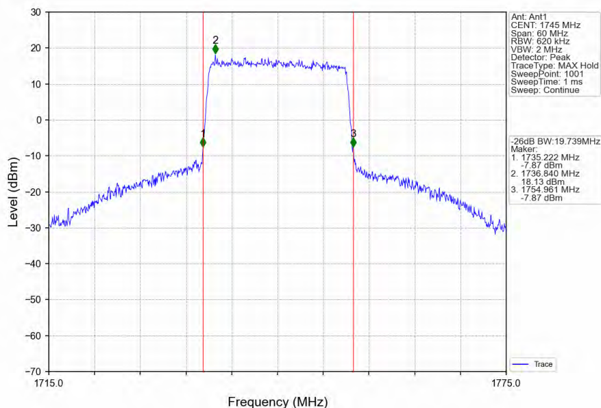
Band4_20MHz_64QAM_HCH_1745MHz_RB_100_0_NTNV
