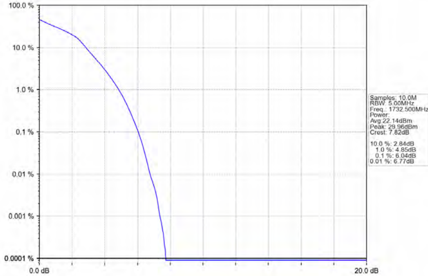
Band4_5MHz_16QAM_MCH_1732.5MHz_RB_25_0_NTNV
