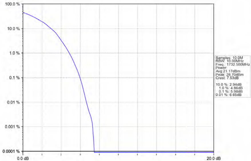
Band4_10MHz_64QAM_MCH_1732.5MHz_RB_50_0_NTNV
