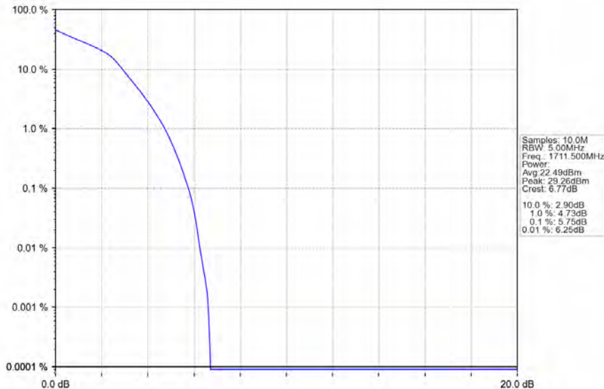
Band4_3MHz_16QAM_LCH_1711.5MHz_RB_15_0_NTNV
