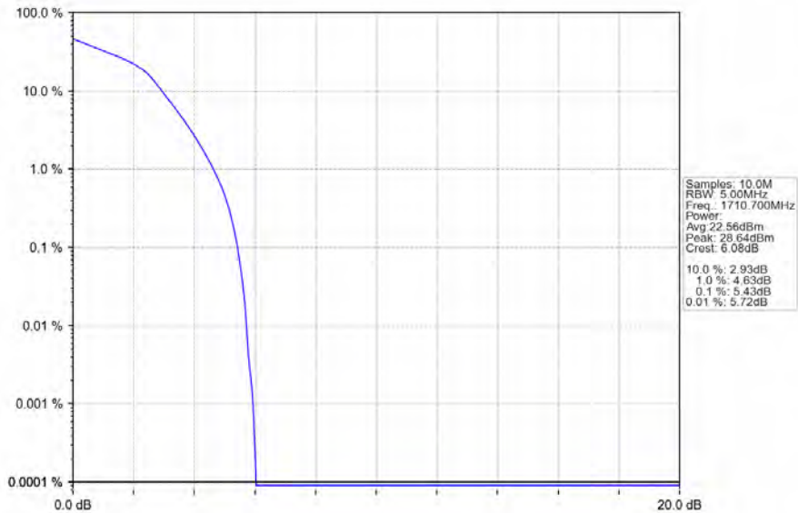
Band4_1.4MHz_16QAM_LCH_1710.7MHz_RB_6_0_NTNV
