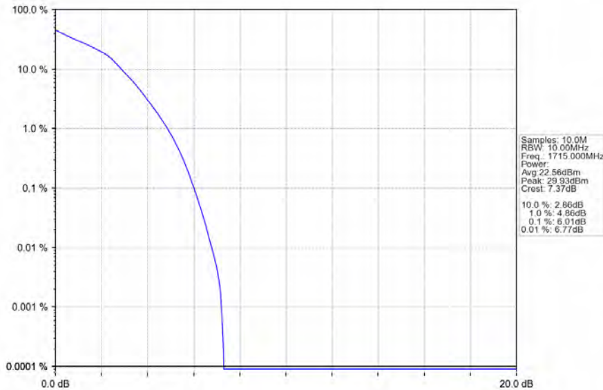
Band4_10MHz_16QAM_LCH_1715MHz_RB_50_0_NTNV
