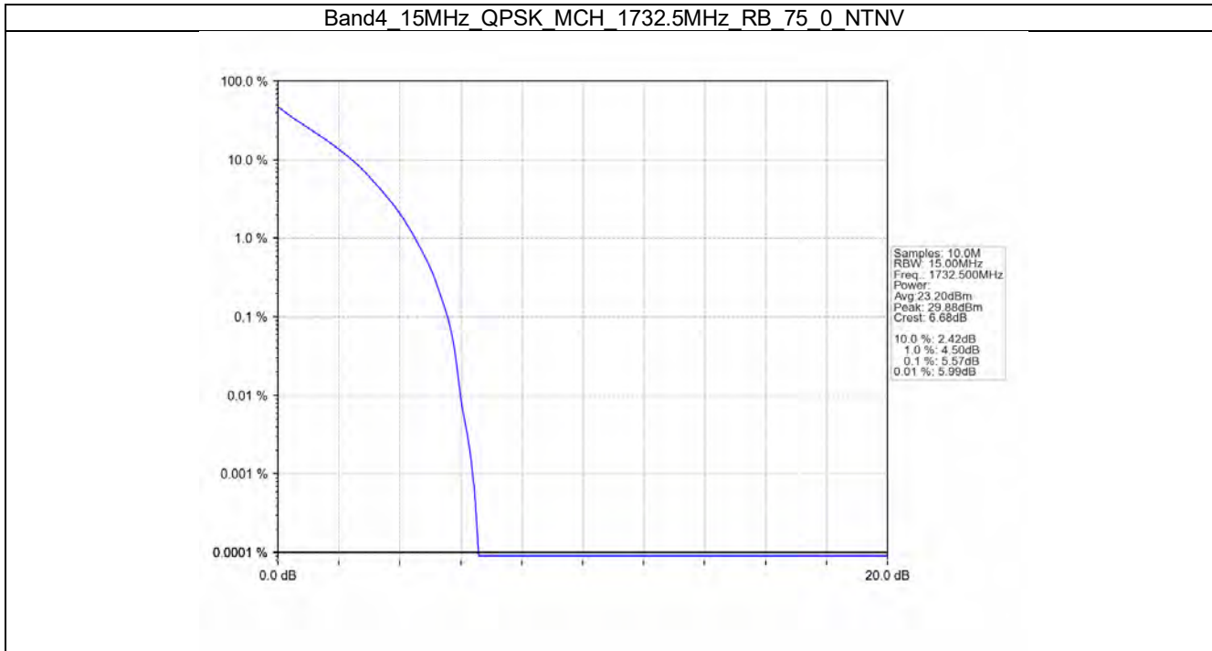
Band4_15MHz_QPSK_MCH_1732.5MHz_RB_75_0_NTNV
