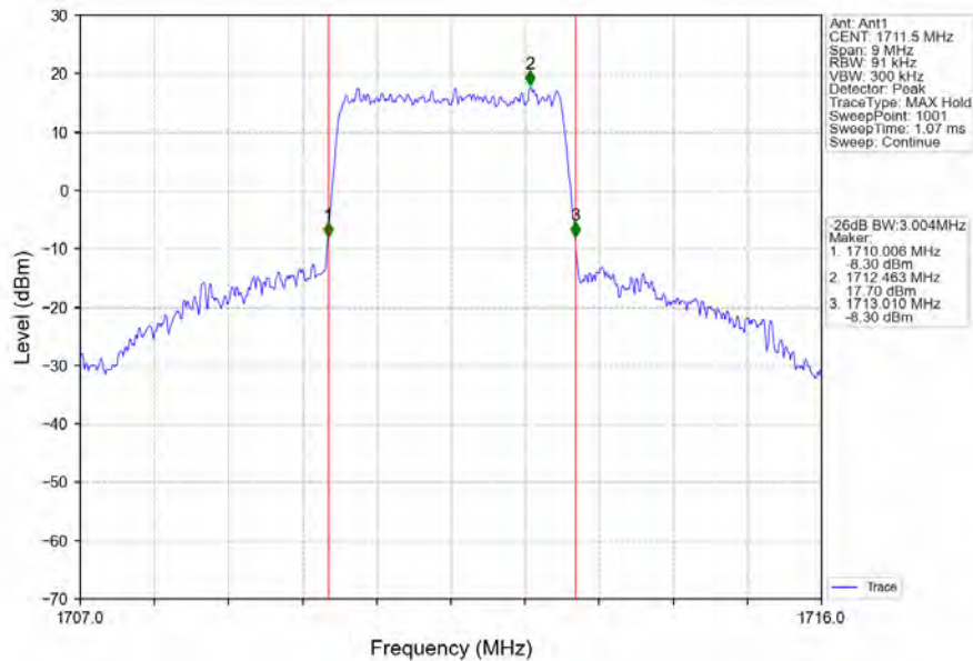
Band4_3MHz_64QAM_LCH_1711.5MHz_RB_15_0_NTNV
