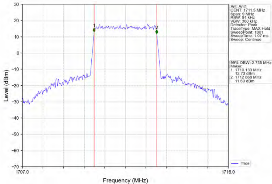
Band4_3MHz_64QAM_LCH_1711.5MHz_RB_15_0_NTNV
