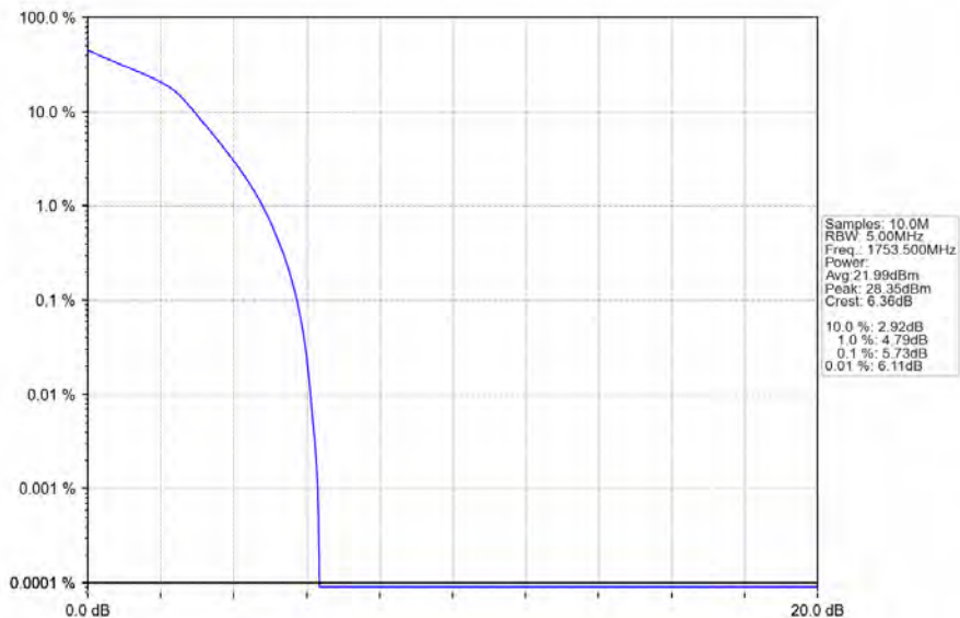
Band4_3MHz_16QAM_HCH_1753.5MHz_RB_15_0_NTNV
