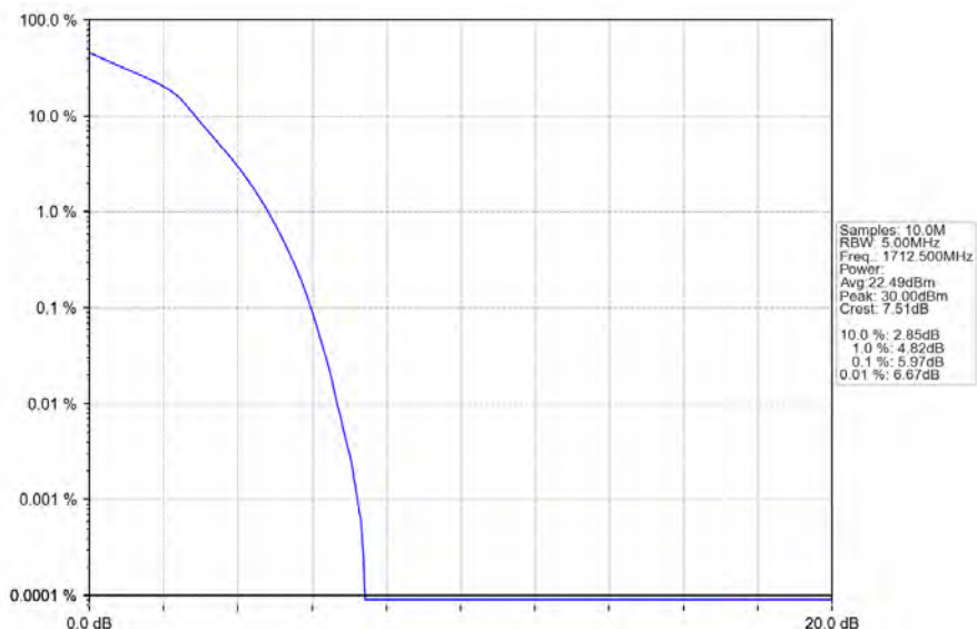
Band4_5MHz_16QAM_LCH_1712.5MHz_RB_25_0_NTNV
