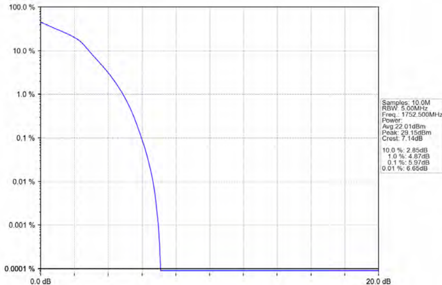
Band4_5MHz_16QAM_HCH_1752.5MHz_RB_25_0_NTNV
