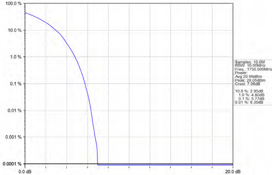
Band4_10MHz_64QAM_HCH_1750MHz_RB_50_0_NTNV
