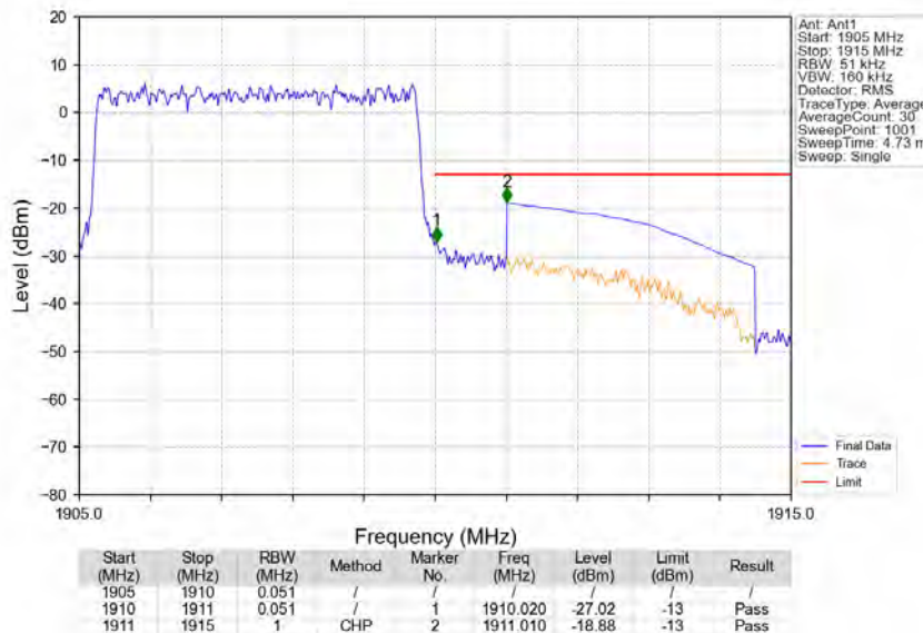
Band2_5MHz_QPSK_HCH_1907.5MHz_RB_25_0_NTNV
