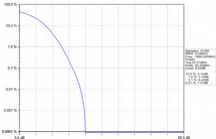
Band2_1.4MHz_64QAM_MCH_1880MHz_RB_6_0_NTNV
