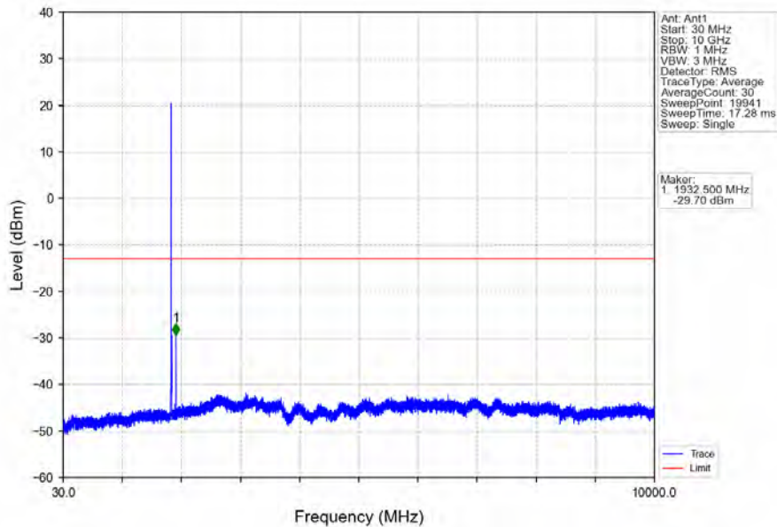
Band2_5MHz_64QAM_LCH_1852.5MHz_RB_1_0_NTNV
