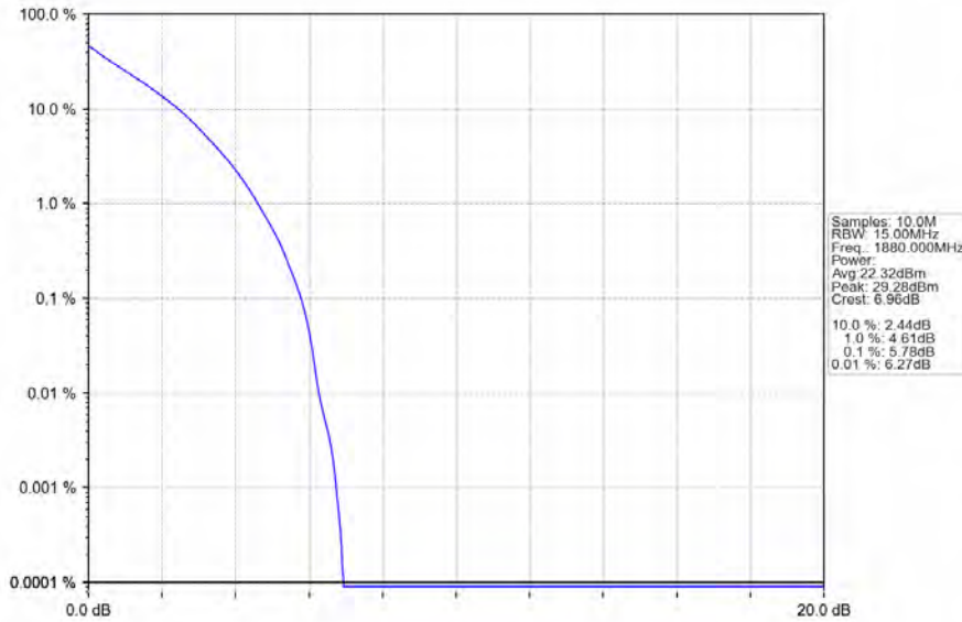
Band2_15MHz_QPSK_MCH_1880MHz_RB_75_0_NTNV
