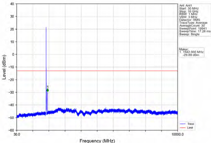
Band2_15MHz_16QAM_LCH_1857.5MHz_RB_1_0_NTV
