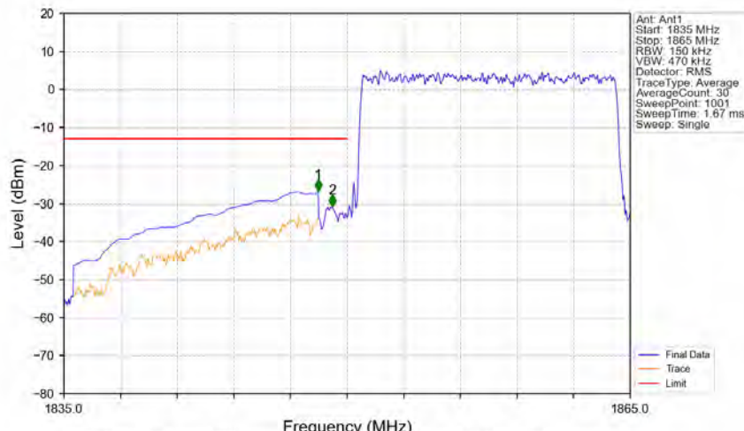
Band2_15MHz_QPSK_LCH_1857.5MHz_RB_75_0_NTNV
