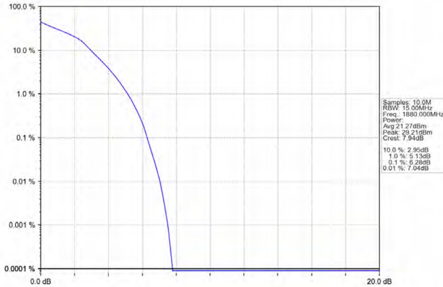
Band2_15MHz_16QAM_MCH_1880MHz_RB_75_0_NTNV
