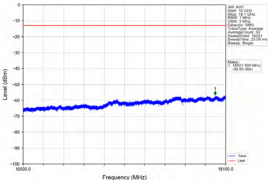
Band2_3MHz_64QAM_MCH_1880MHz_RB_1_0_NTNV
