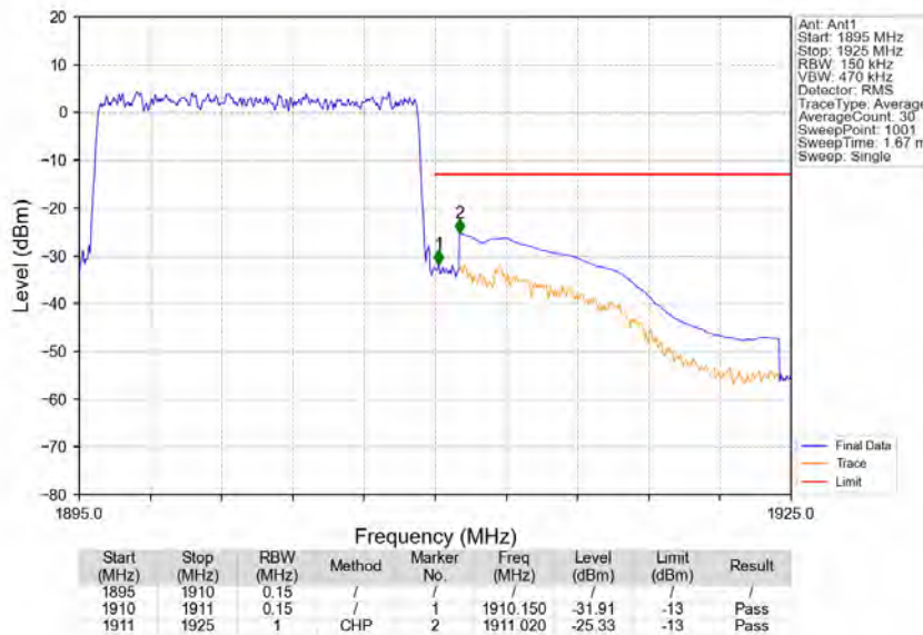
Band2_15MHz_16QAM_HCH_1902.5MHz_RB_75_0_NTNV
