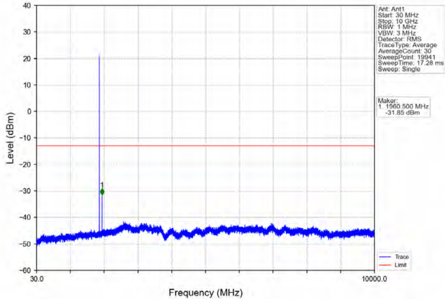
Band2_1.4MHz_64QAM_MCH_1880MHz_RB_1_0_NTV
