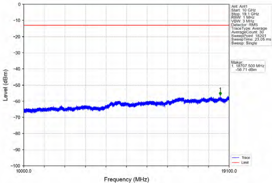
Band2_10MHz_64QAM_MCH_1880MHz_RB_1_0_NTNV
