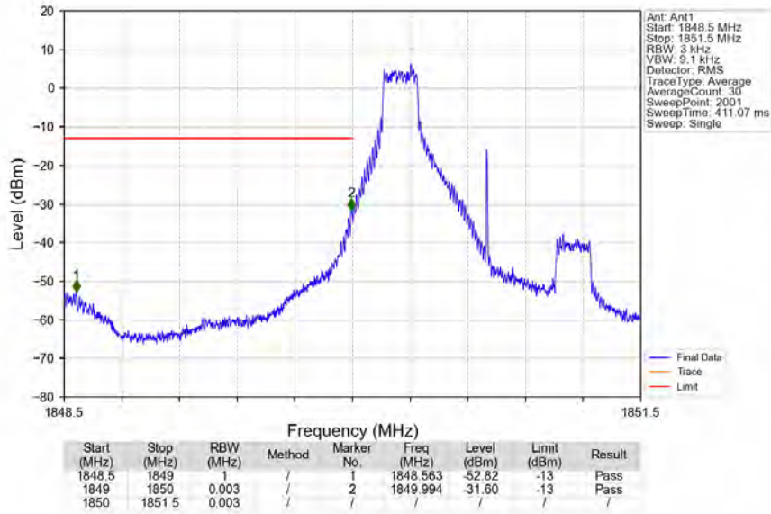
Band2_1.4MHz_64QAM_LCH_1850.7MHz_RB_1_0_NTNV
