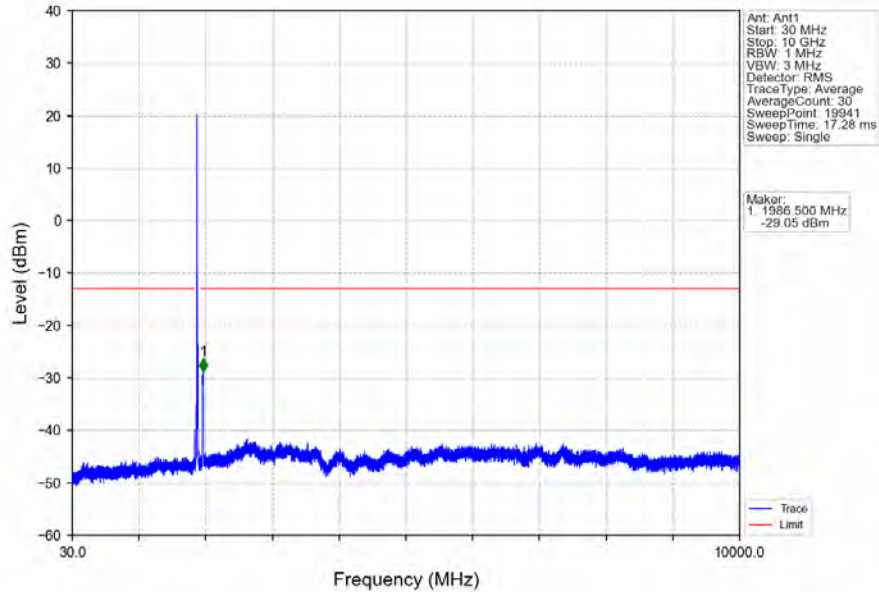
Band2_20MHz_64QAM_HCH_1900MHz_RB_1_0_NTNV
