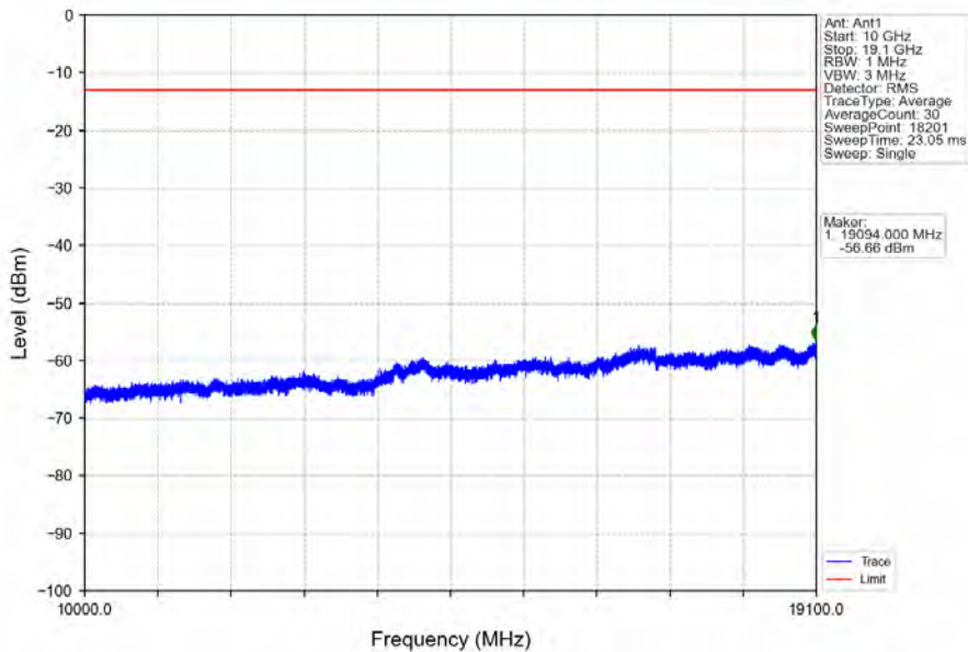
Band2_15MHz_64QAM_HCH_1902.5MHz_RB_1_0_NTNV
