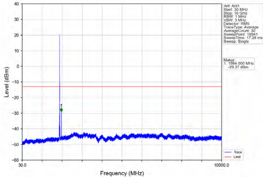
Band2_10MHz_64QAM_HCH_1905MHz_RB_1_0_NTNV
