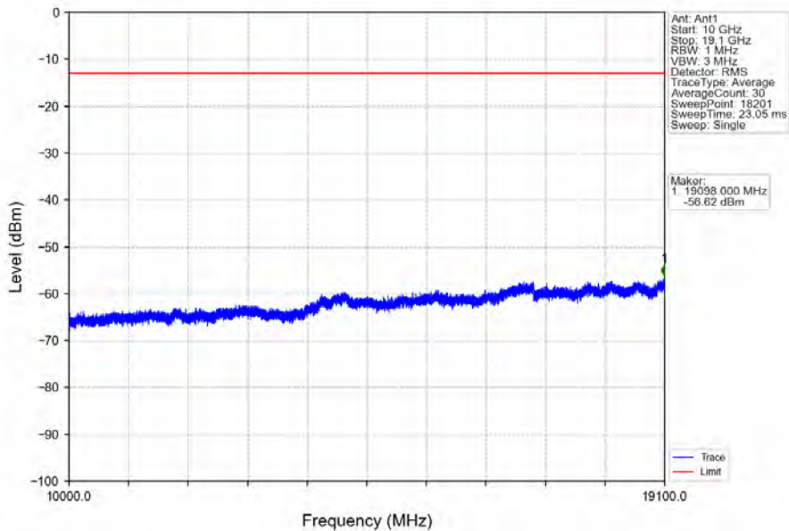
Band2_1.4MHz_16QAM_MCH_1880MHz_RB_1_0_NTV
