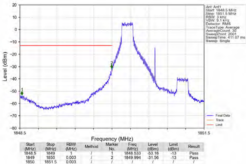
Band2_1.4MHz_16QAM_LCH_1850.7MHz_RB_1_0_NTNV
