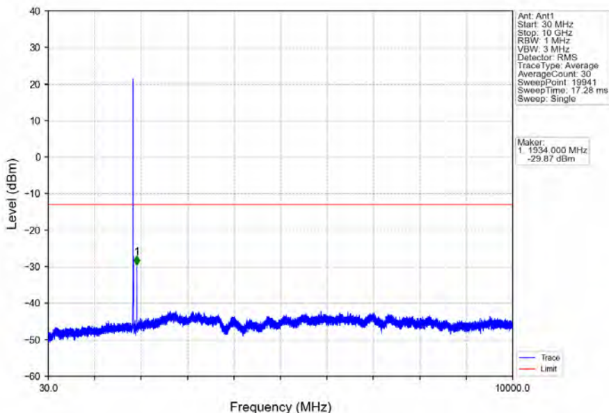
Band2_5MHz_16QAM_LCH_1852.5MHz_RB_1_0_NTNV
