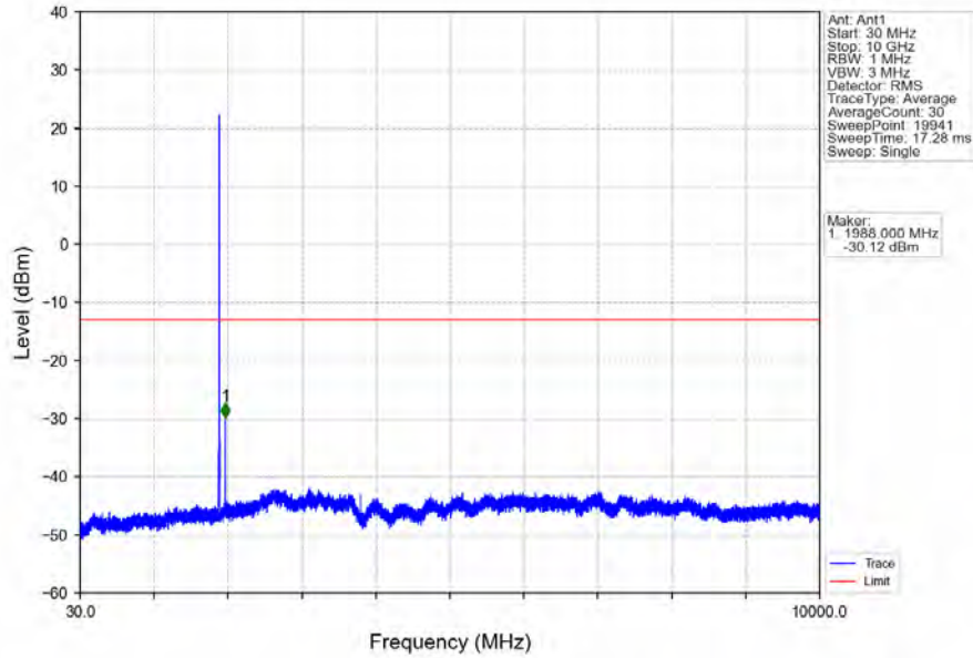
Band2_5MHz_16QAM_HCH_1907.5MHz_RB_1_0_NTNV
