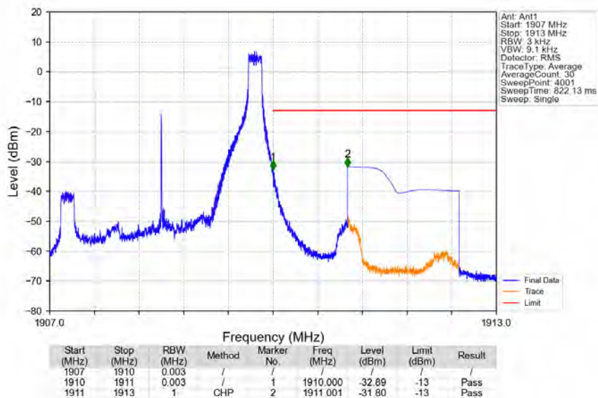
Band2_3MHz_64QAM_HCH_1908.5MHz_RB_1_14_NTNV
