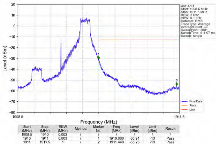
Band2_1.4MHz_16QAM_HCH_1909.3MHz_RB_1_5_NTNV
