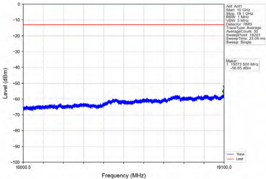
Band2_15MHz_64QAM_MCH_1880MHz_RB_1_0_NTNV
