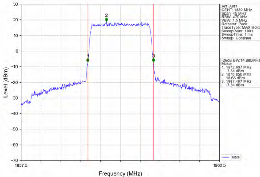
Band2_15MHz_QPSK_MCH_1880MHz_RB_75_0_NTNV
