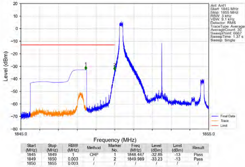
Band2_5MHz_64QAM_LCH_1852.5MHz_RB_1_0_NTNV
