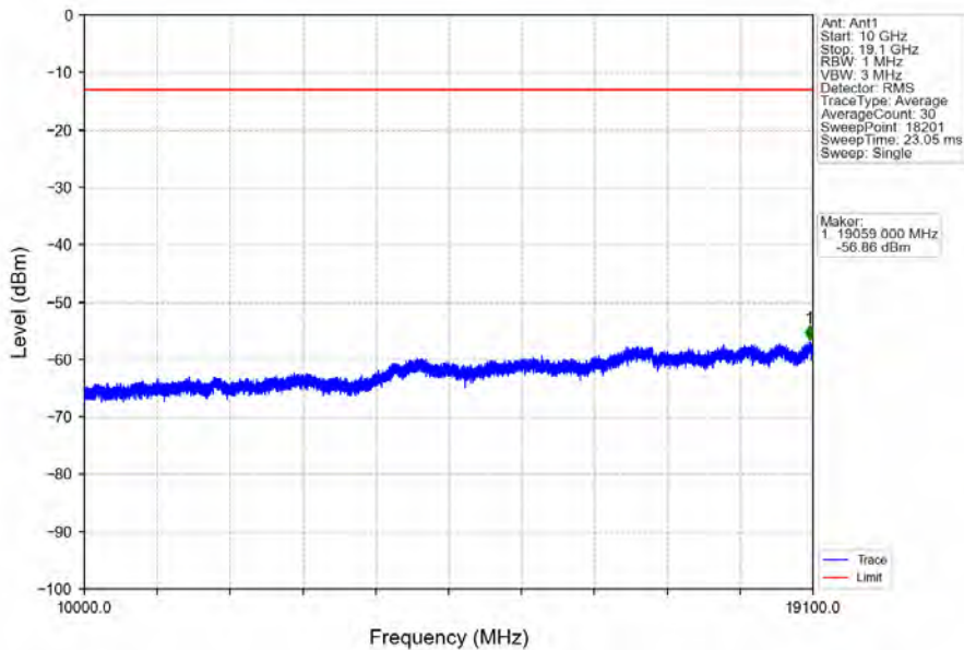
Band2_10MHz_64QAM_HCH_1905MHz_RB_1_0_NTNV
