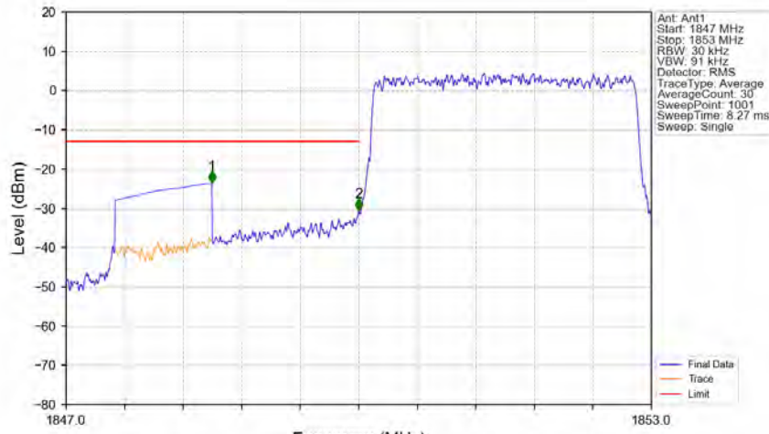
Band2_3MHz_QPSK_LCH_1851.5MHz_RB_15_0_NTNV
