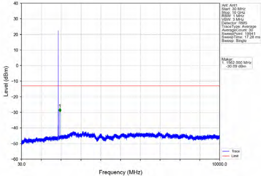
Band2_5MHz_16QAM_MCH_1880MHz_RB_1_0_NTNV
