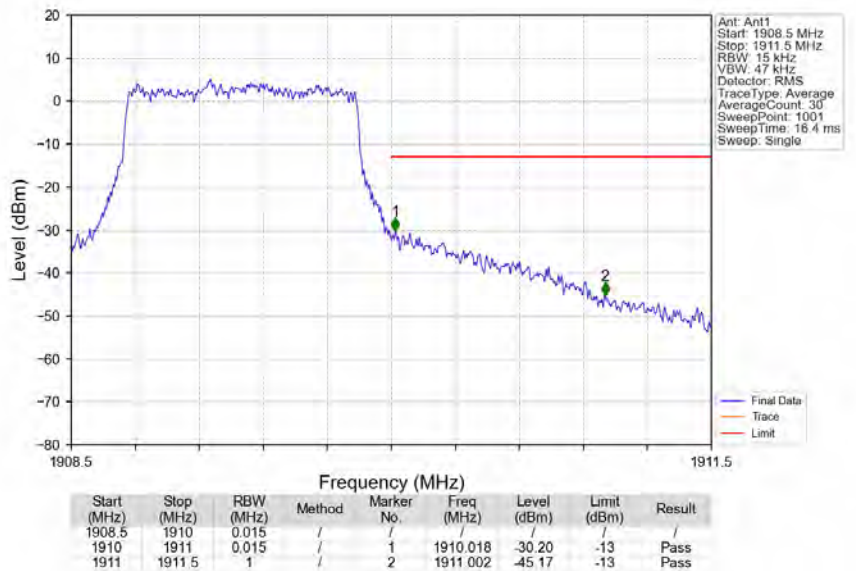
Band2_1.4MHz_64QAM_HCH_1909.3MHz_RB_6_0_NTNV
