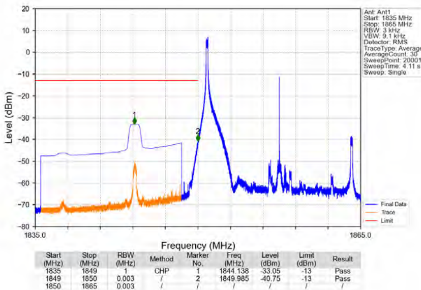
Band2_15MHz_16QAM_LCH_1857.5MHz_RB_1_0_NTV
