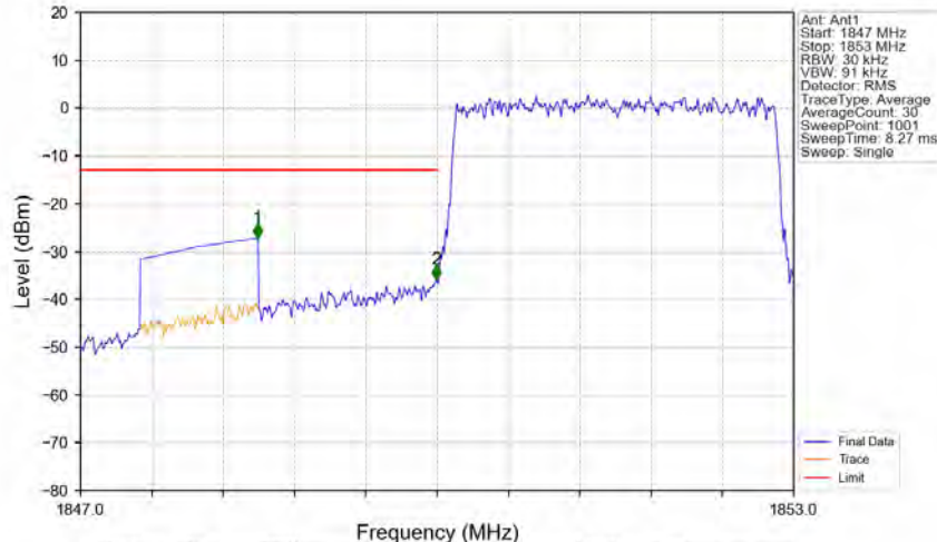
Band2_3MHz_64QAM_LCH_1851.5MHz_RB_15_0_NTNV
