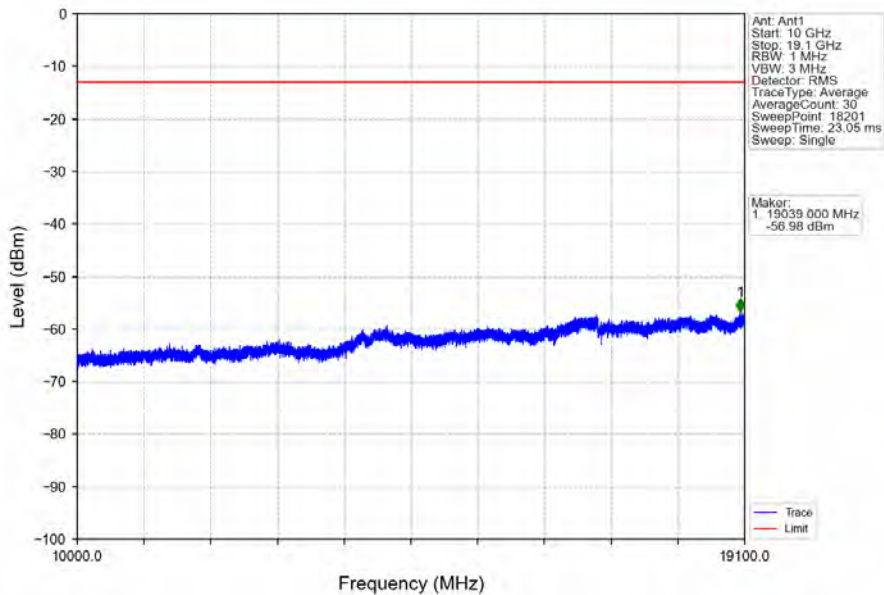
Band2_1.4MHz_64QAM_MCH_1880MHz_RB_1_0_NTV
