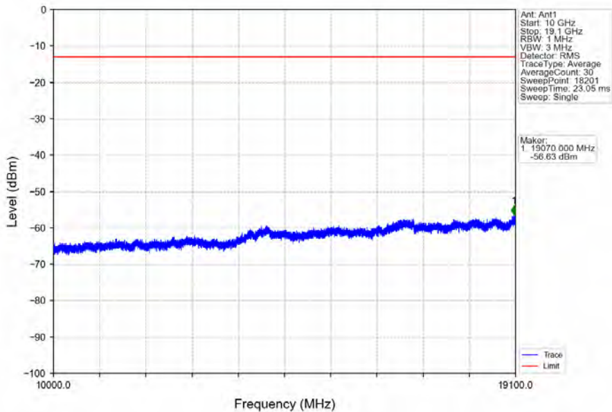
Band2_20MHz_64QAM_HCH_1900MHz_RB_1_0_NTNV
