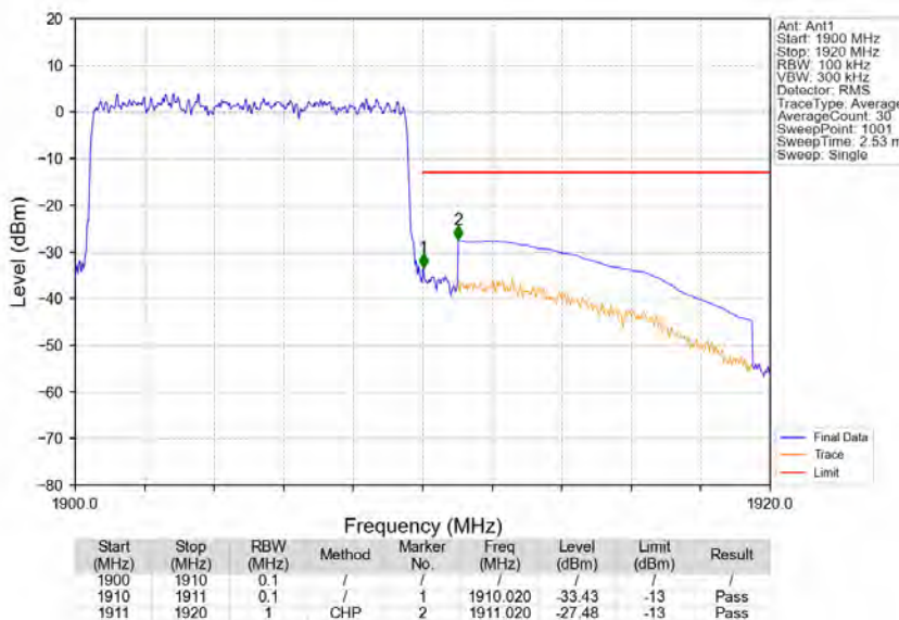
Band2_10MHz_64QAM_HCH_1905MHz_RB_50_0_NTNV
