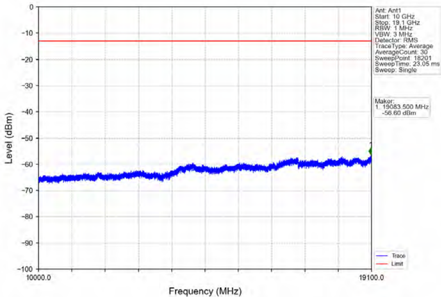
Band2_5MHz_64QAM_HCH_1907.5MHz_RB_1_0_NTNV
