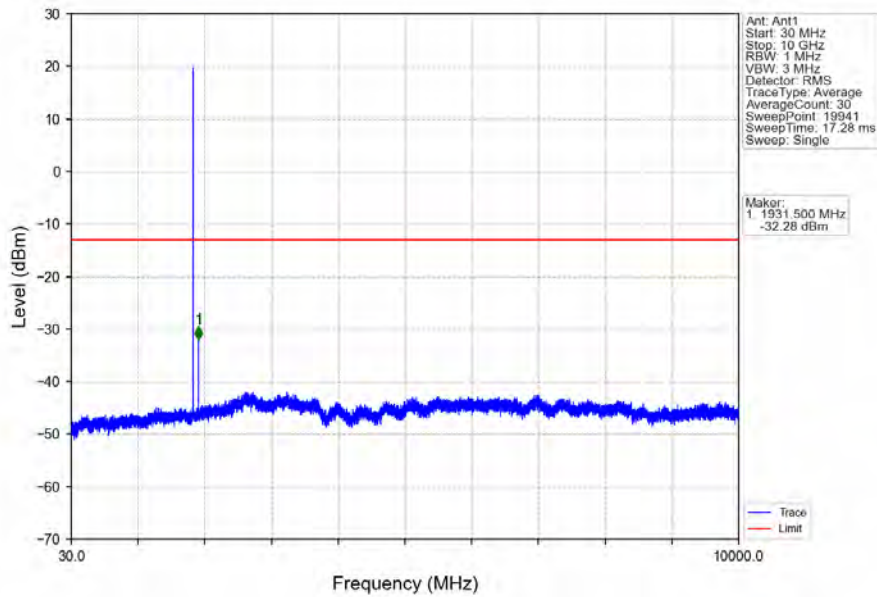
Band2_1.4MHz_64QAM_LCH_1850.7MHz_RB_1_0_NTNV
