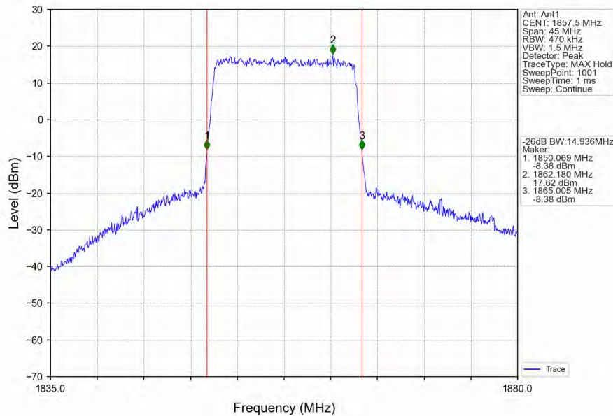
Band2_15MHz_16QAM_LCH_1857.5MHz_RB_75_0_NTNV
