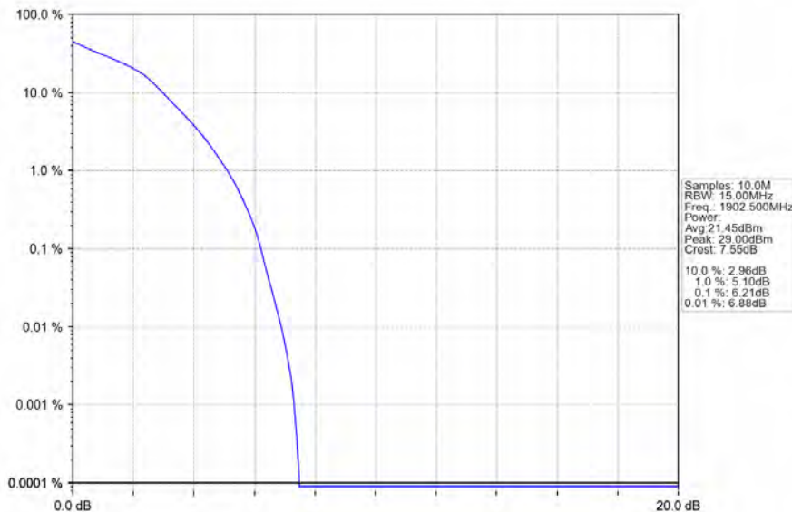
Band2_15MHz_16QAM_HCH_1902.5MHz_RB_75_0_NTNV
