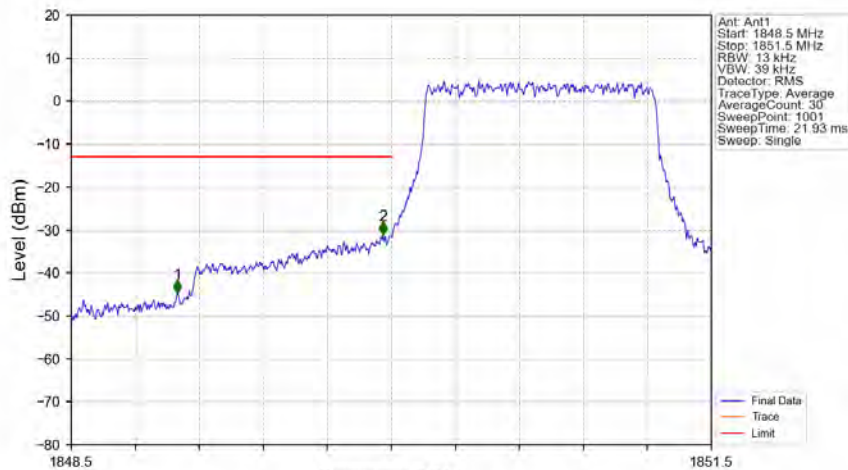
Band2_1.4MHz_QPSK_LCH_1850.7MHz_RB_6_0_NTNV
