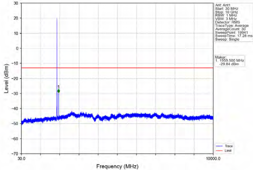
Band2_5MHz_64QAM_MCH_1880MHz_RB_1_0_NTNV
