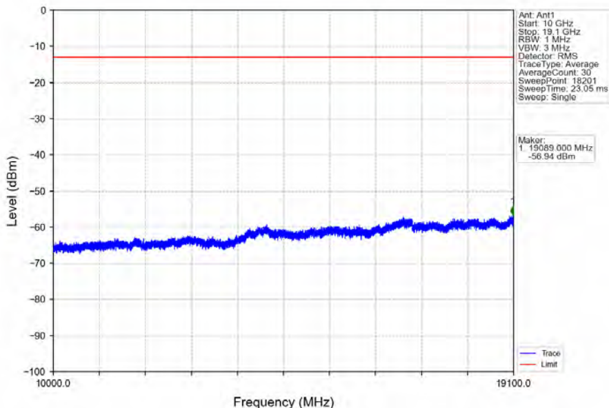
Band2_15MHz_64QAM_LCH_1857.5MHz_RB_75_0_NTNV
