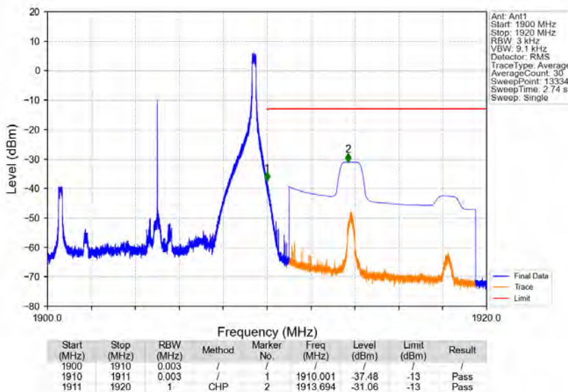
Band2_10MHz_64QAM_HCH_1905MHz_RB_1_49_NTNV
