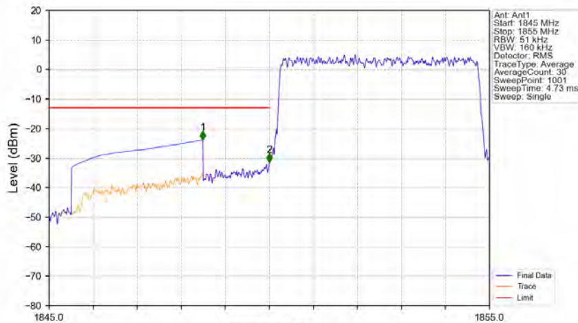
Band2_5MHz_QPSK_LCH_1852.5MHz_RB_25_0_NTNV
