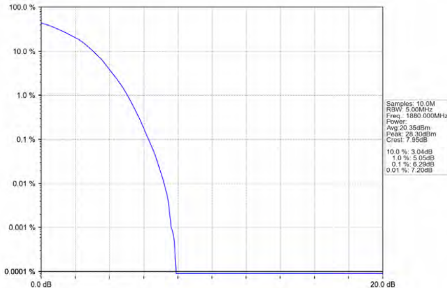
Band2_3MHz_64QAM_MCH_1880MHz_RB_15_0_NTNV
