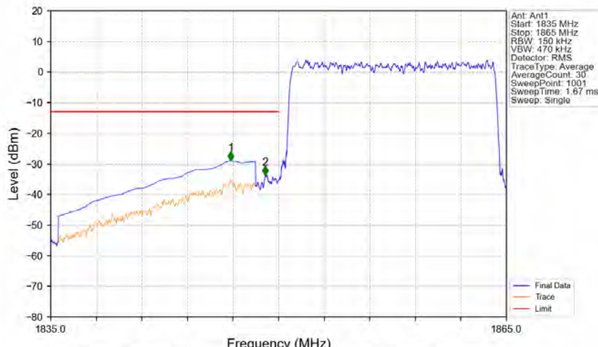
Band2_15MHz_16QAM_LCH_1857.5MHz_RB_75_0_NTNV
