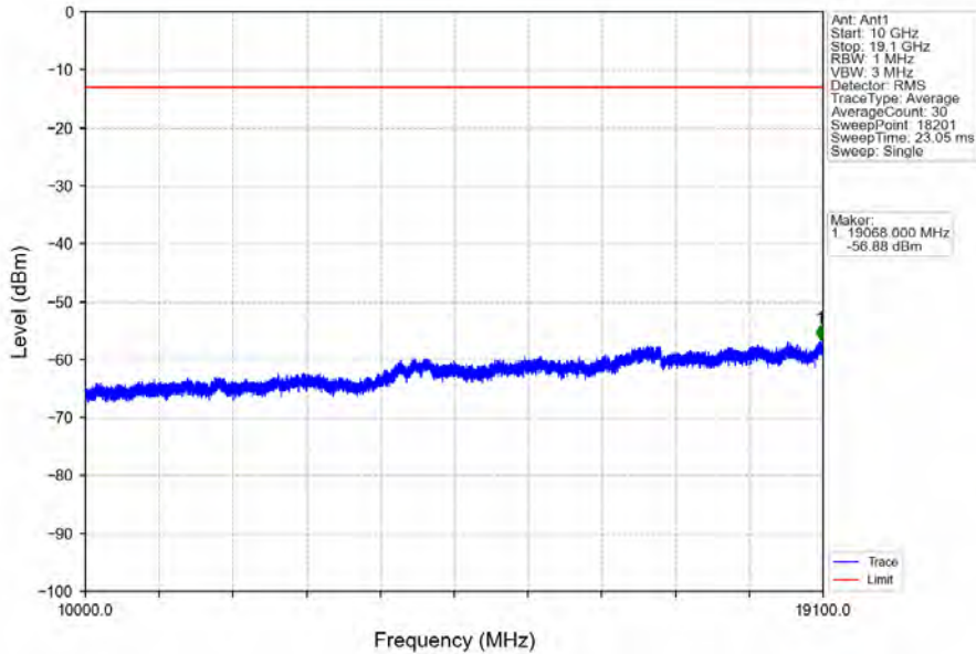
Band2_5MHz_64QAM_LCH_1852.5MHz_RB_25_0_NTNV
