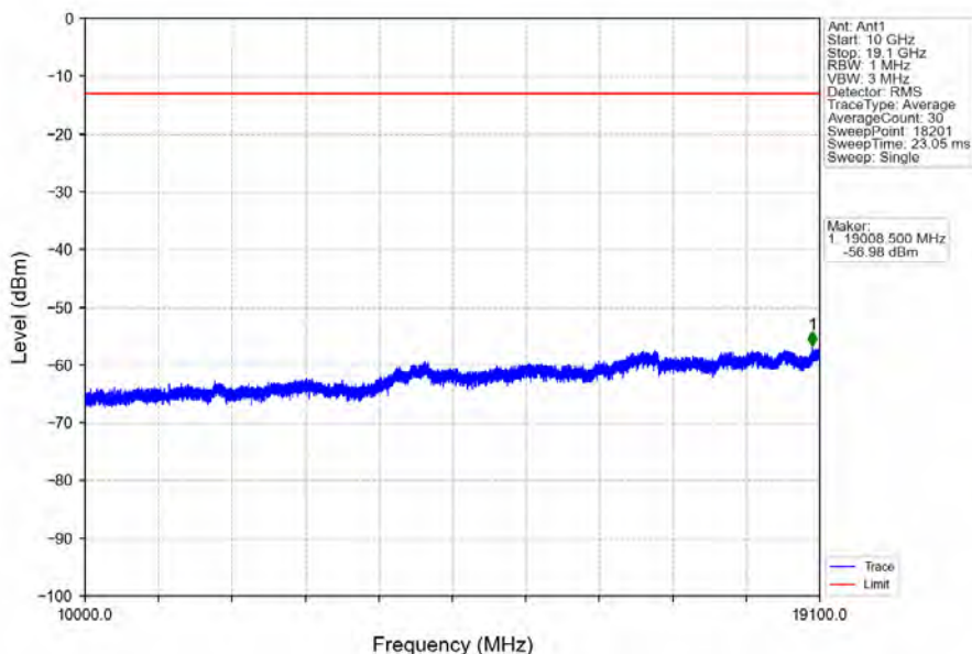
Band2_15MHz_QPSK_LCH_1857.5MHz_RB_75_0_NTNV
