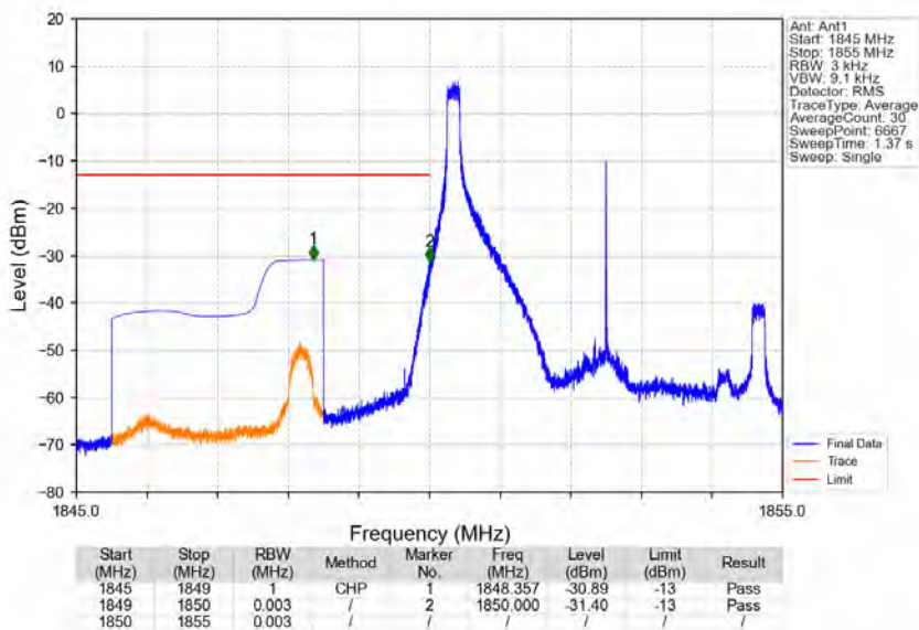
Band2_5MHz_16QAM_LCH_1852.5MHz_RB_1_0_NTNV
