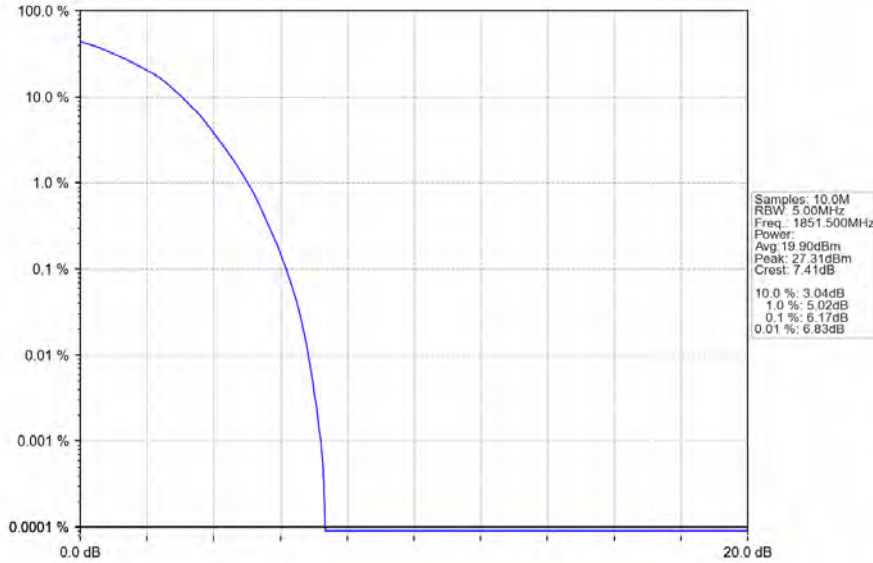
Band2_3MHz_64QAM_LCH_1851.5MHz_RB_15_0_NTNV
