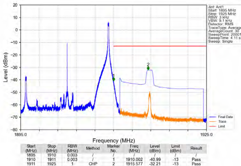
Band2_15MHz_64QAM_HCH_1902.5MHz_RB_1_74_NTNV
