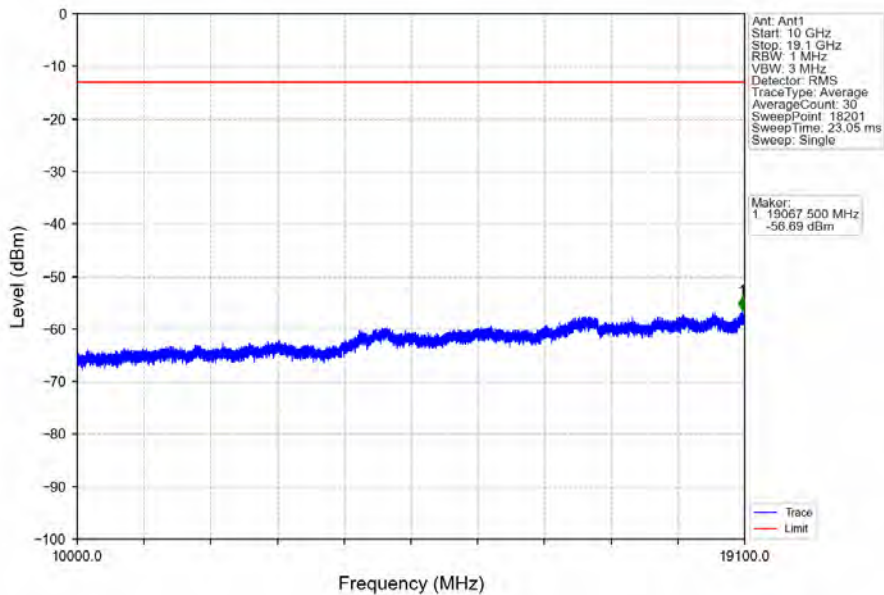
Band2_15MHz_16QAM_MCH_1880MHz_RB_1_0_NTNV
