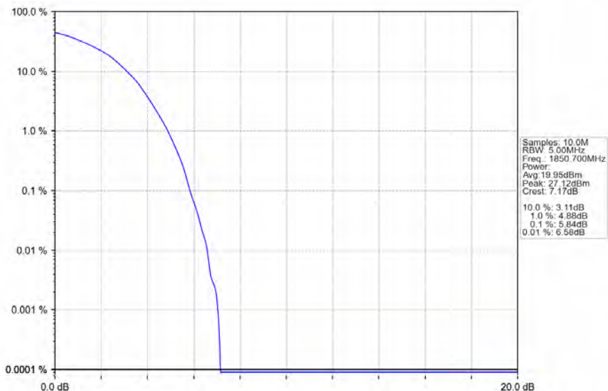
Band2_1.4MHz_64QAM_LCH_1850.7MHz_RB_6_0_NTNV
