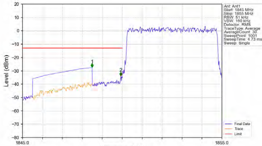
Band2_5MHz_64QAM_LCH_1852.5MHz_RB_25_0_NTNV
