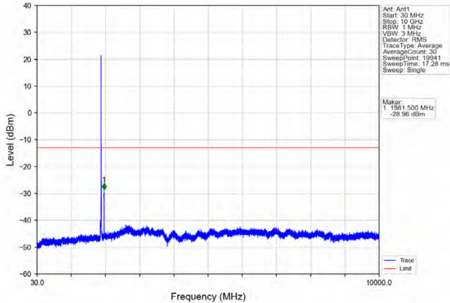
Band2_15MHz_64QAM_HCH_1902.5MHz_RB_1_0_NTNV
