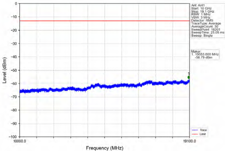
Band2_3MHz_64QAM_HCH_1908.5MHz_RB_1_0_NTNV
