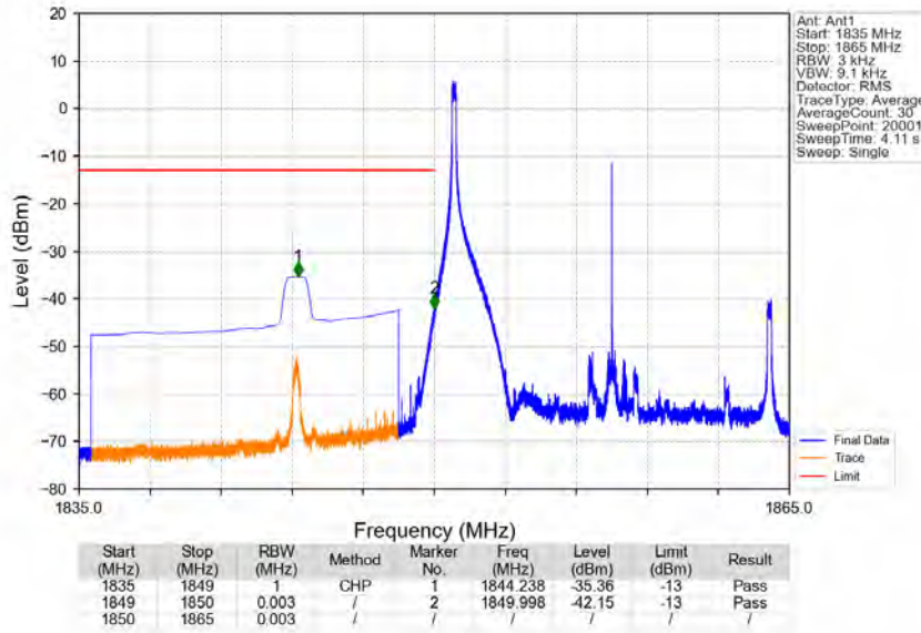
Band2_15MHz_64QAM_LCH_1857.5MHz_RB_1_0_NTNV
