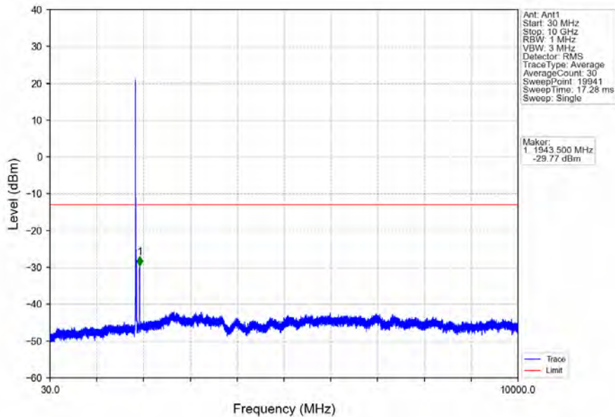
Band2_15MHz_64QAM_LCH_1857.5MHz_RB_1_0_NTNV
