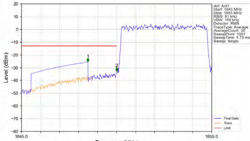
Band2_5MHz_16QAM_LCH_1852.5MHz_RB_25_0_NTNV
