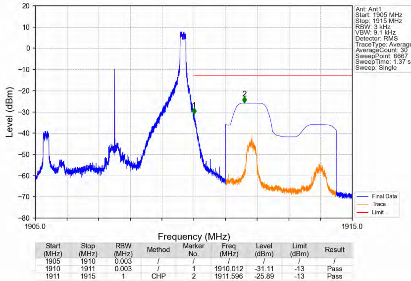
Band2_5MHz_QPSK_HCH_1907.5MHz_RB_1_24_NTNV
