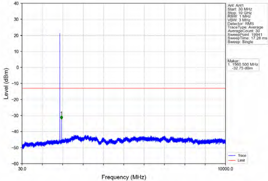
Band2_1.4MHz_16QAM_MCH_1880MHz_RB_1_0_NTV
