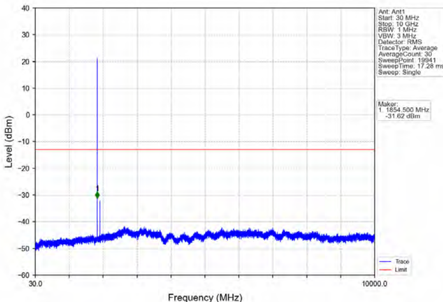
Band2_1.4MHz_16QAM_LCH_1850.7MHz_RB_1_0_NTNV
