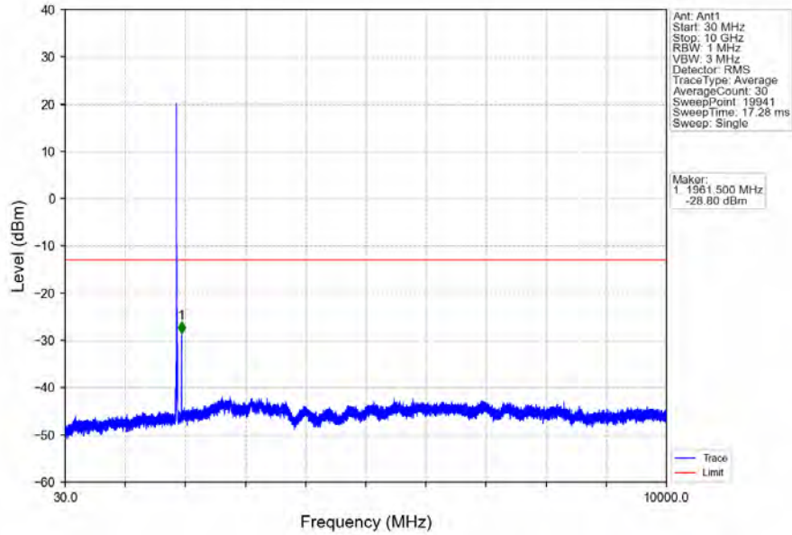
Band2_10MHz_64QAM_MCH_1880MHz_RB_1_0_NTNV
