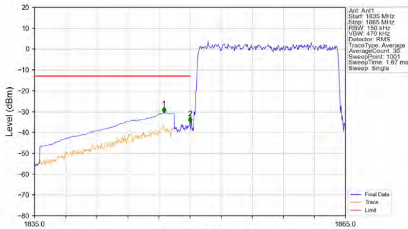
Band2_15MHz_64QAM_LCH_1857.5MHz_RB_75_0_NTNV
