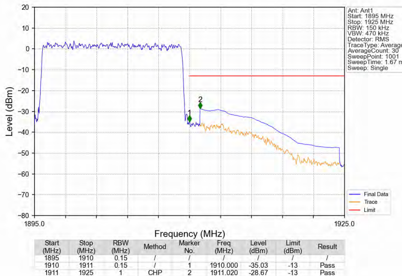
Band2_15MHz_64QAM_HCH_1902.5MHz_RB_75_0_NTNV
