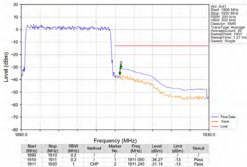
Band2_20MHz_64QAM_HCH_1900MHz_RB_100_0_NTNV
