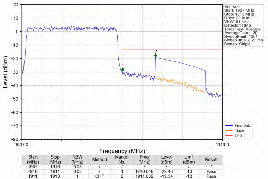
Band2_3MHz_16QAM_HCH_1908.5MHz_RB_15_0_NTNV
