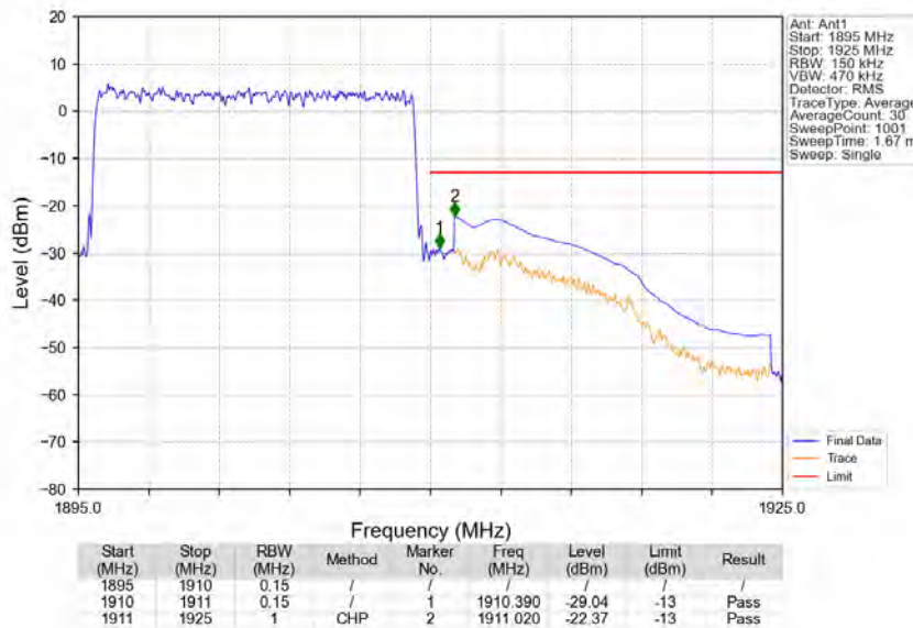
Band2_15MHz_QPSK_HCH_1902.5MHz_RB_75_0_NTNV
