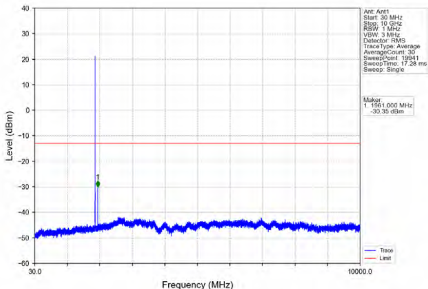
Band2_3MHz_64QAM_MCH_1880MHz_RB_1_0_NTNV
