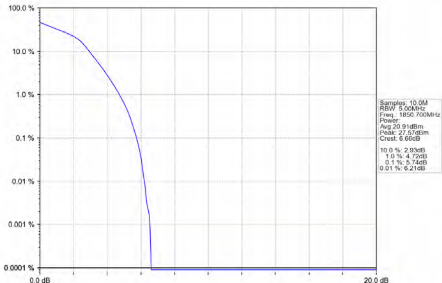
Band2_1.4MHz_16QAM_LCH_1850.7MHz_RB_6_0_NTNV
