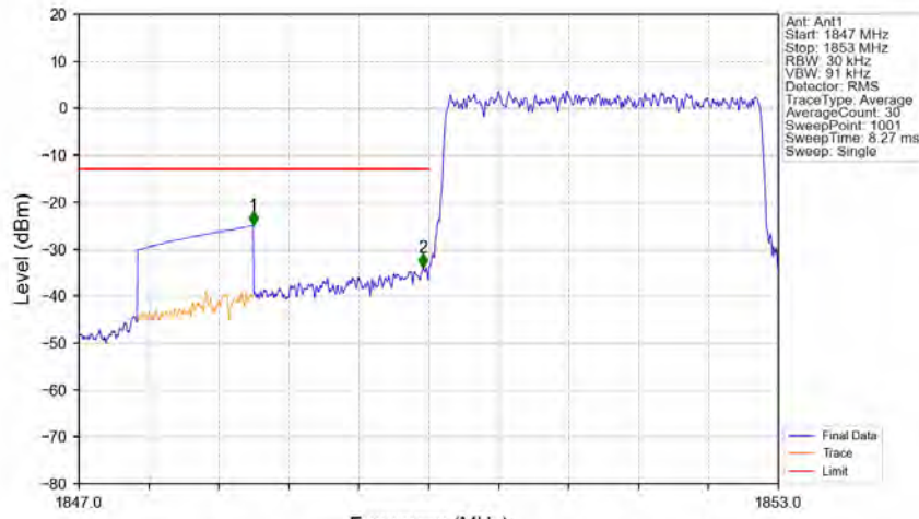
Band2_3MHz_16QAM_LCH_1851.5MHz_RB_15_0_NTNV
