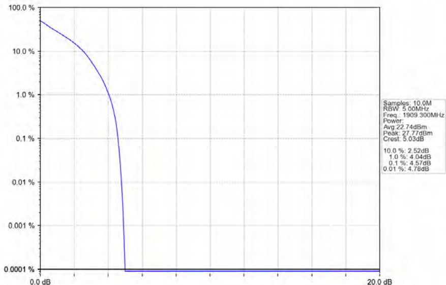
Band2_1.4MHz_QPSK_HCH_1909.3MHz_RB_6_0_NTNV
