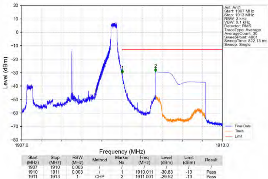
Band2_3MHz_16QAM_HCH_1908.5MHz_RB_1_14_NTNV
