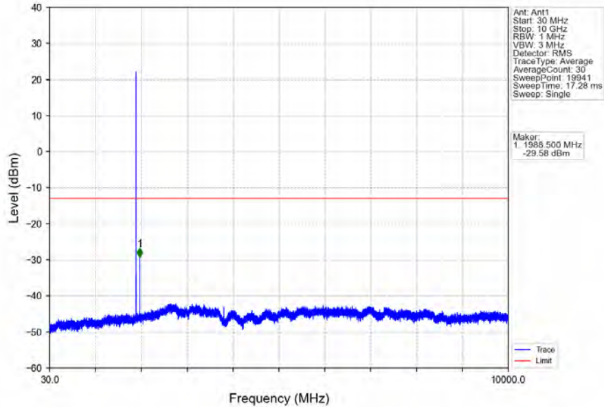
Band2_3MHz_16QAM_HCH_1908.5MHz_RB_1_0_NTNV
