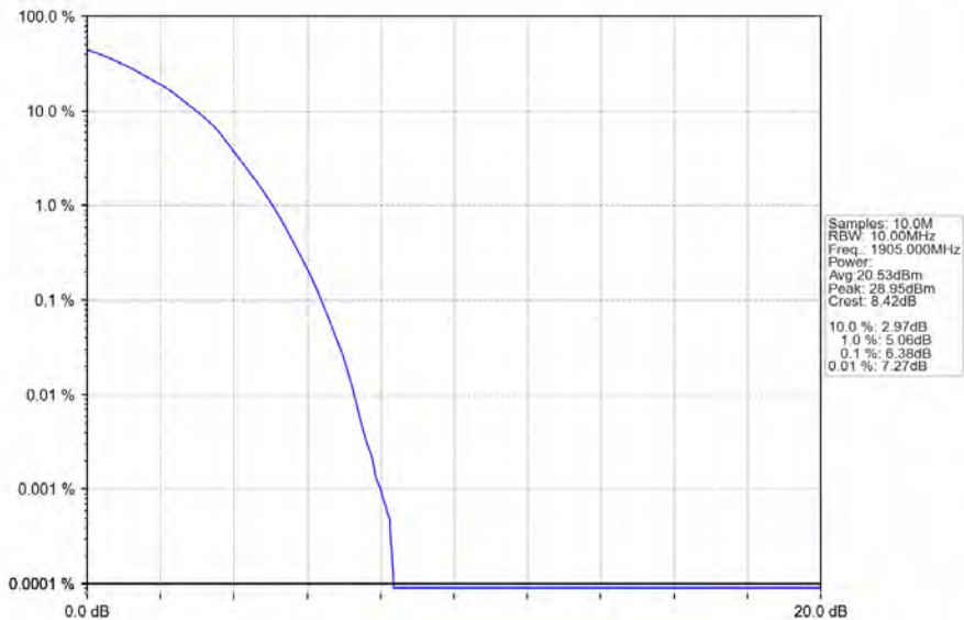
Band2_10MHz_64QAM_HCH_1905MHz_RB_50_0_NTNV
