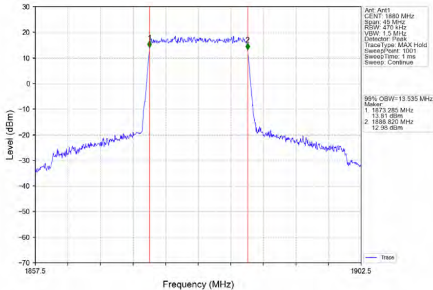
Band2_15MHz_QPSK_MCH_1880MHz_RB_75_0_NTNV
