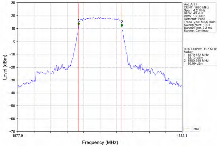
Band2_1.4MHz_QPSK_MCH_1880MHz_RB_6_0_NTNV
