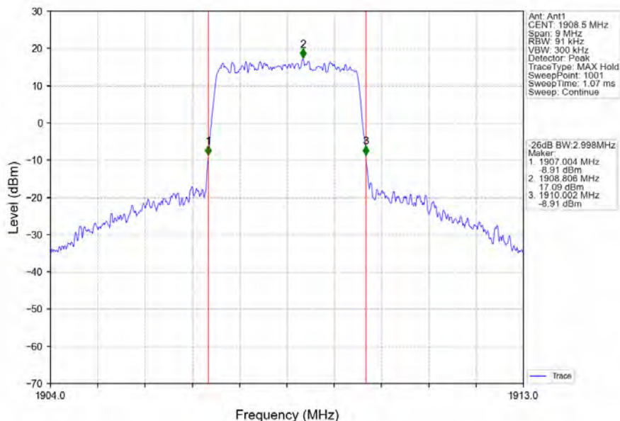
Band2_3MHz_64QAM_HCH_1908.5MHz_RB_15_0_NTNV
