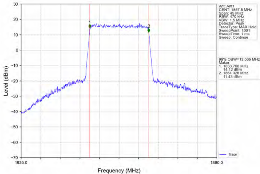
Band2_15MHz_16QAM_LCH_1857.5MHz_RB_75_0_NTNV
