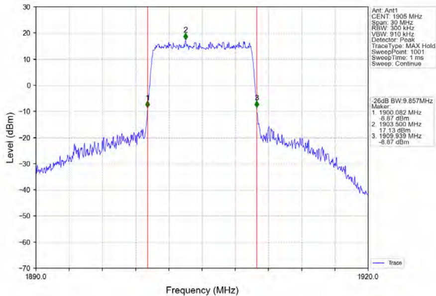
Band2_10MHz_64QAM_HCH_1905MHz_RB_50_0_NTNV
