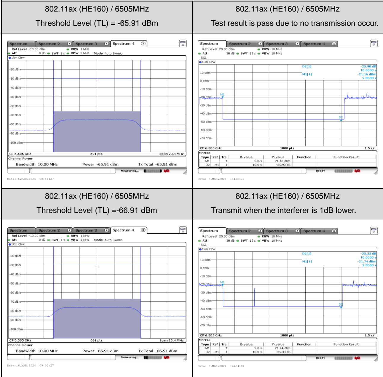
Contention Based Protocol Result Plots on U-NII 6 (AWGN Interference)
