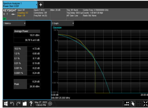
N77(100M)_DFT-s-OFDM_QPSK_Edge_1RB_Left_Mid_CH
