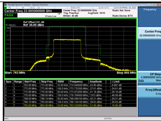
Band13_10MHz_16QAM_23230_50RB#0
