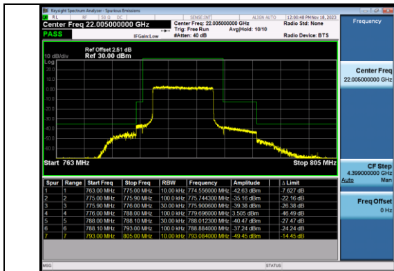
Band13_10MHz_QPSK_23230_50RB#0
