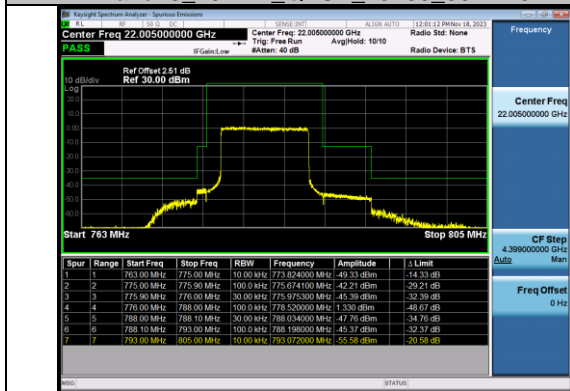
Band13_10MHz_64QAM_23230_50RB#0
