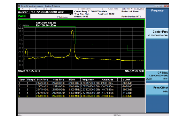
Band7_15MHz_16QAM_21375_1RB#74
