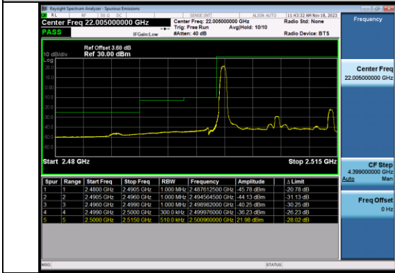
Band7_15MHz_16QAM_20825_1RB#0
