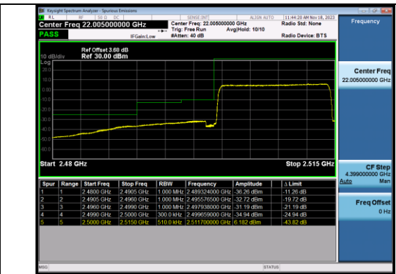
Band7_15MHz_64QAM_20825_75RB#0
