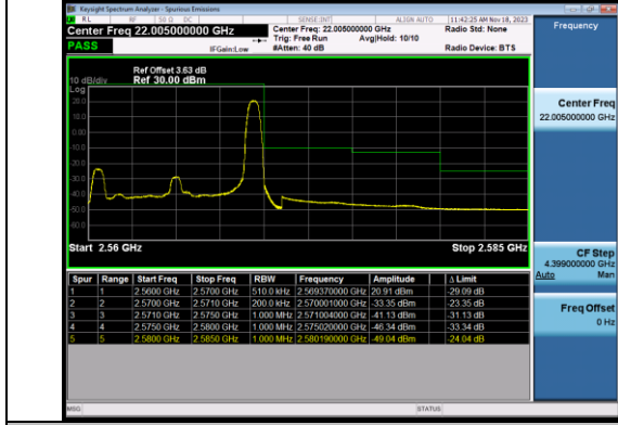
Band7_10MHz_64QAM_20800_1RB#0
