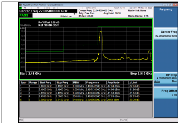
Band7_15MHz_64QAM_20825_1RB#0
