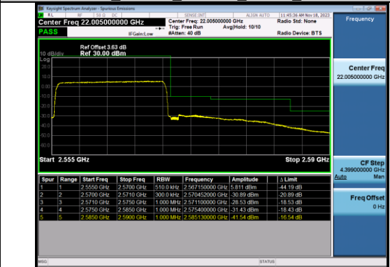
Band7_15MHz_64QAM_21375_75RB#0
