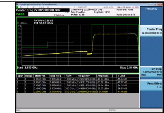
Band7_10MHz_16QAM_20800_50RB#0
