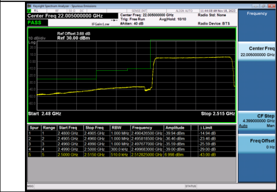
Band7_15MHz_16QAM_20825_75RB#0
