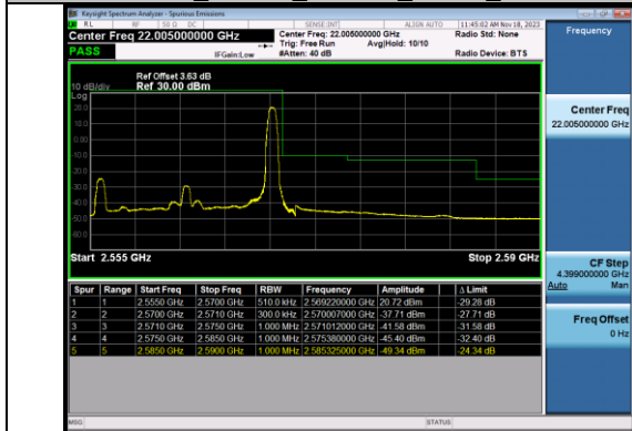
Band7_15MHz_64QAM_21375_1RB#74
