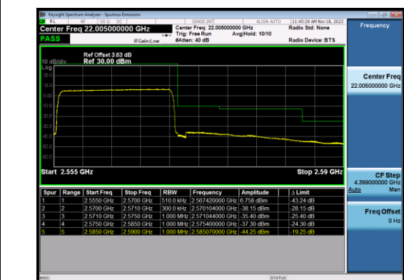
Band7_15MHz_16QAM_21375_75RB#0
