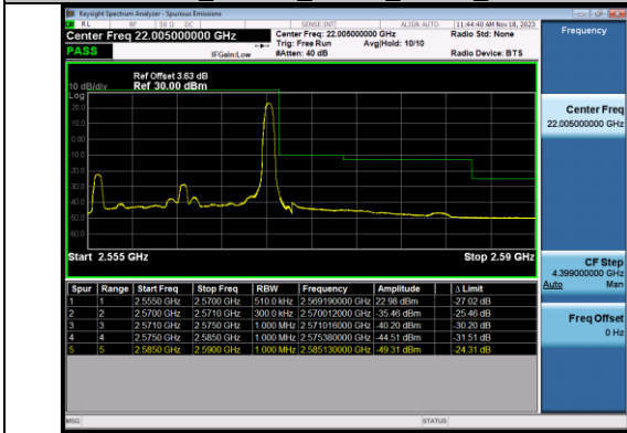
Band7_15MHz_QPSK_21375_1RB#74
