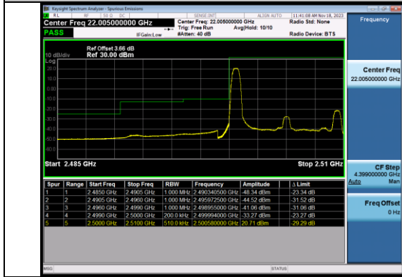
Band7_10MHz_16QAM_21400_1RB#49
