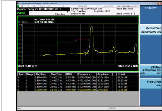
Band7_15MHz_QPSK_20825_1RB#0
