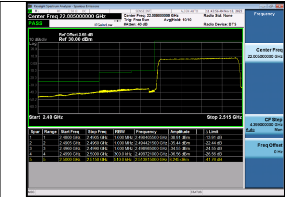
Band7_15MHz_QPSK_20825_75RB#0
