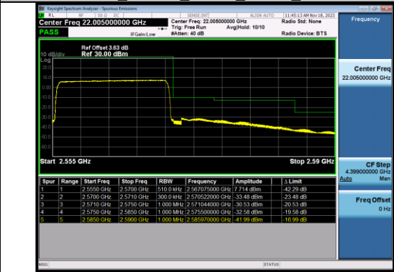
Band7_15MHz_QPSK_21375_75RB#0
